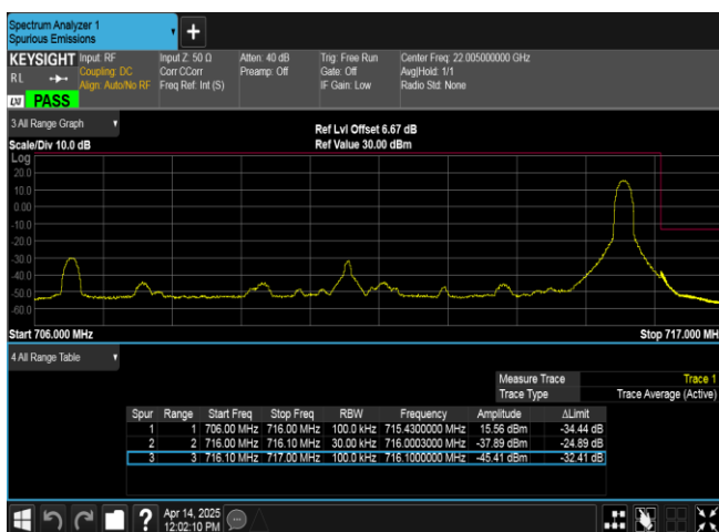
Band17-10MHz-16QAM-23800-1RB#49-PASS
