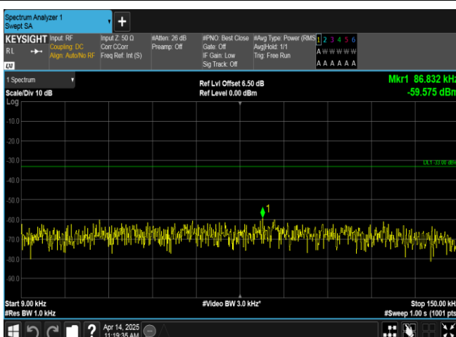
Band17-5MHz-QPSK-23755-25RB#0-0.009~0.15-PASS
