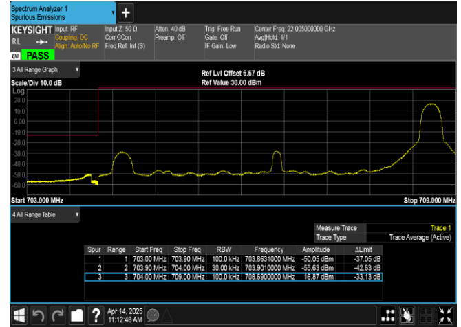
Band17-5MHz-16QAM-23755-1RB#24-PASS
