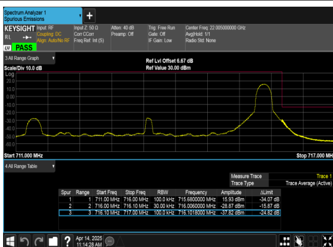
Band17-5MHz-16QAM-23825-1RB#24-PASS
