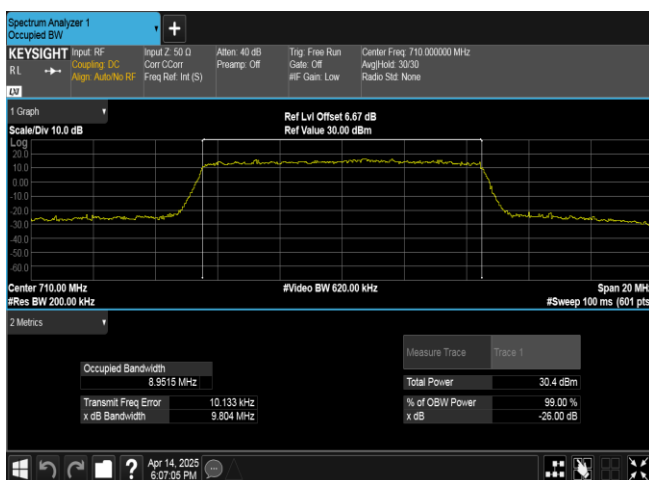
Band17-10MHz-16QAM-23790-50RB#0-PASS
