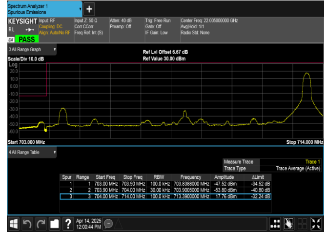
Band17-10MHz-QPSK-23780-1RB#49-PASS
