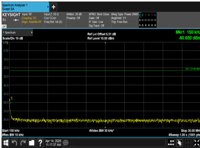
Band17-5MHz-QPSK-23755-1RB#24-0.15~30-PASS
