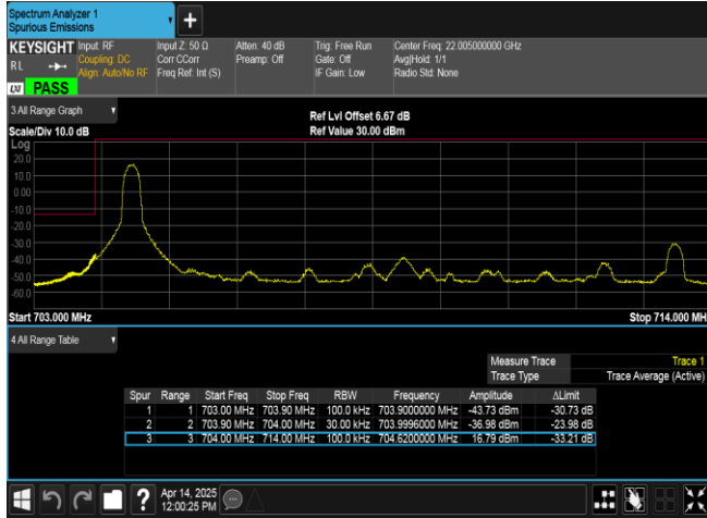
Band17-10MHz-16QAM-23780-1RB#0-PASS
