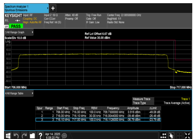
Band17-10MHz-QPSK-23800-50RB#0-PASS
