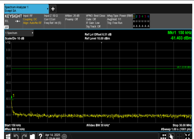
Band17-5MHz-QPSK-23755-25RB#0-0.15~30-PASS
