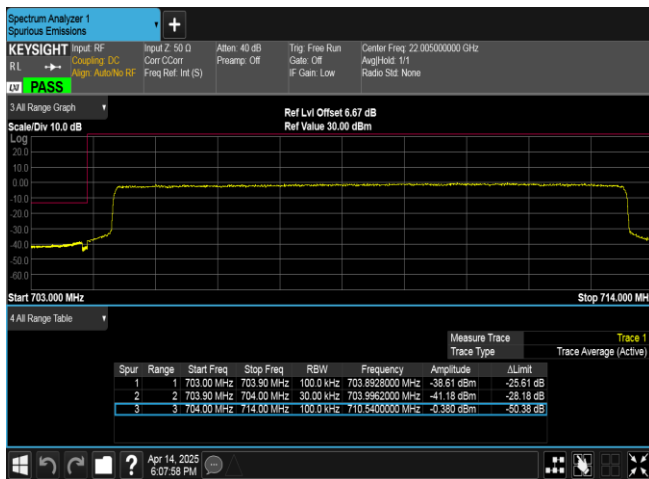
Band17-10MHz-16QAM-23780-50RB#0-PASS
