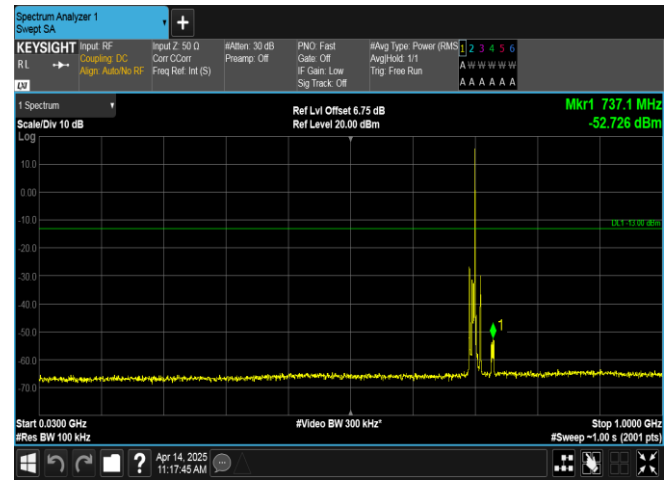
Band17-5MHz-QPSK-23755-1RB#24-30~1000-PASS
