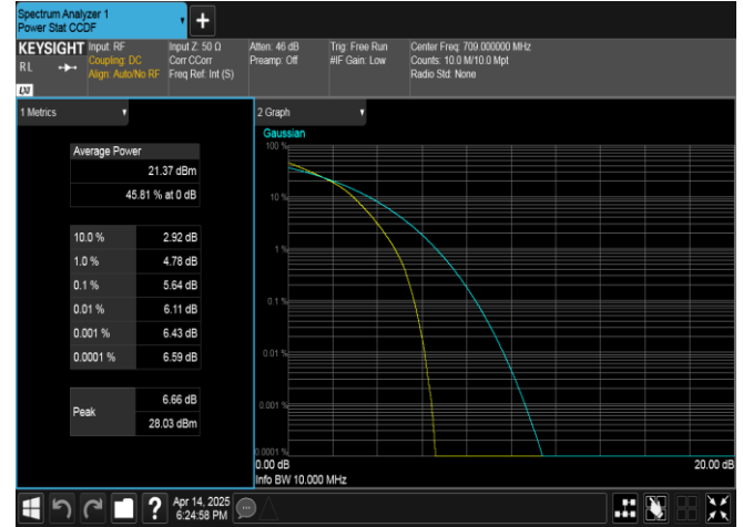
Band17-10MHz-16QAM-23780-50RB#0-PASS
