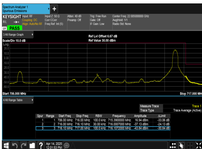
Band17-10MHz-QPSK-23800-1RB#49-PASS
