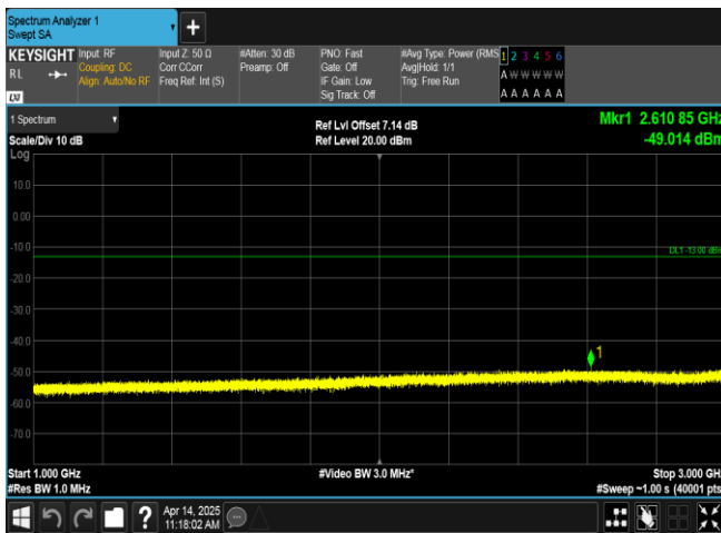
Band17-5MHz-QPSK-23755-1RB#24-1000~3000-PASS
