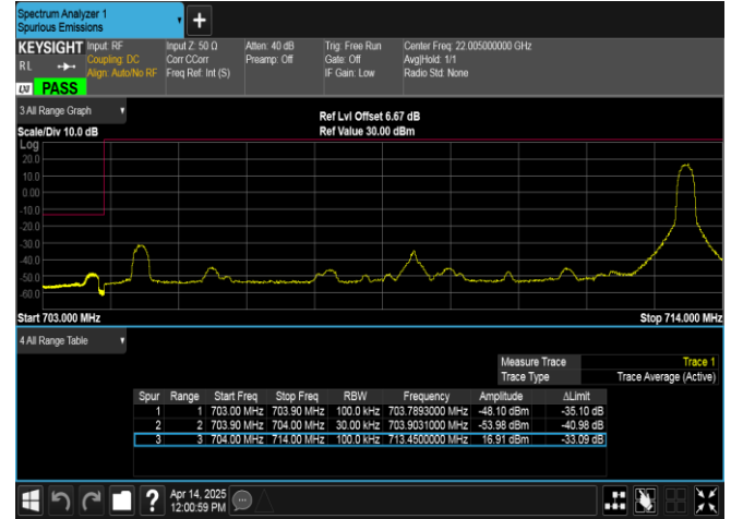
Band17-10MHz-16QAM-23780-1RB#49-PASS
