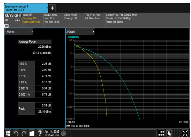
Band17-10MHz-QPSK-23800-50RB#0-PASS
