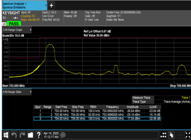
Band17-5MHz-16QAM-23755-1RB#0-PASS
