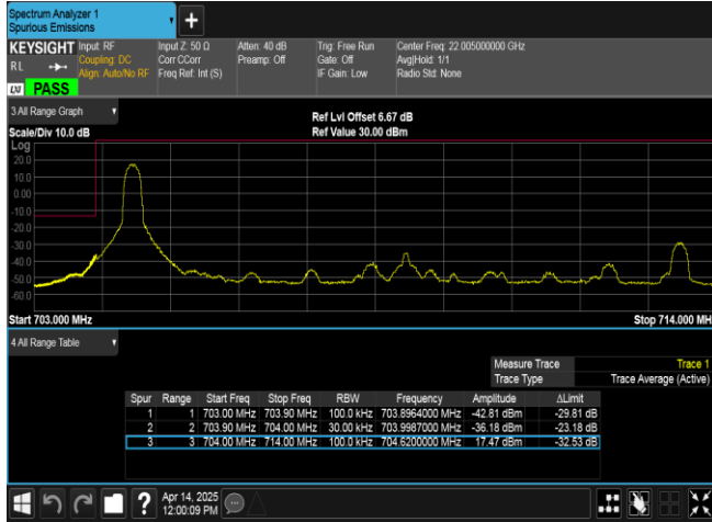
Band17-10MHz-QPSK-23780-1RB#0-PASS
