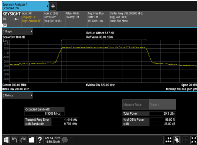
Band17-10MHz-QPSK-23780-50RB#0-PASS
