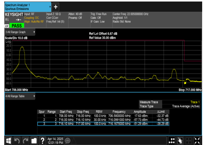
Band17-10MHz-QPSK-23800-1RB#0-PASS
