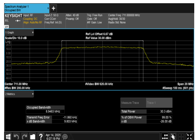
Band17-10MHz-16QAM-23800-50RB#0-PASS
