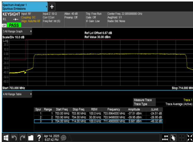
Band17-10MHz-QPSK-23780-50RB#0-PASS
