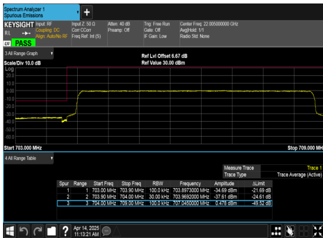
Band17-5MHz-16QAM-23755-25RB#0-PASS
