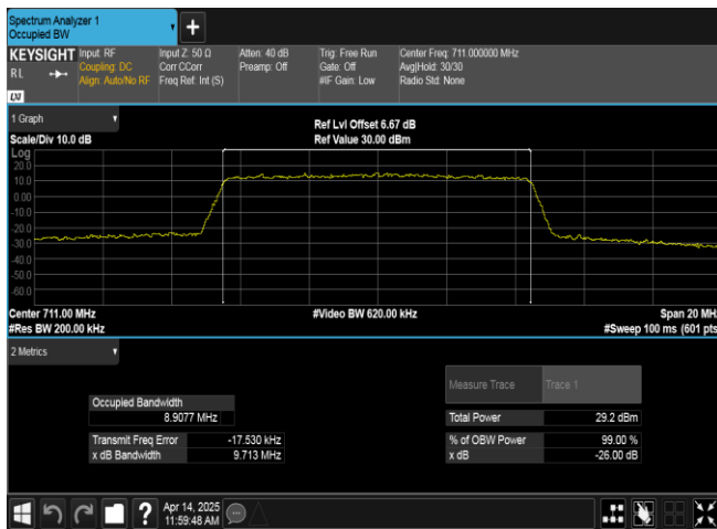
Band17-10MHz-QPSK-23800-50RB#0-PASS
