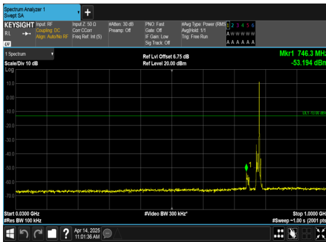
Band13-10MHz-16QAM-23230-1RB#49-30~1000-PASS
