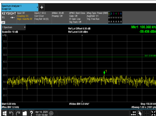
Band13-10MHz-16QAM-23230-1RB#49-0.009~0.15-PASS
