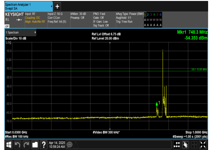
Band13-10MHz-16QAM-23230-1RB#0-30~1000-PASS
