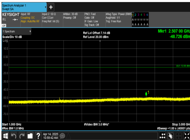
Band13-10MHz-16QAM-23230-1RB#0-1000~3000-PASS
