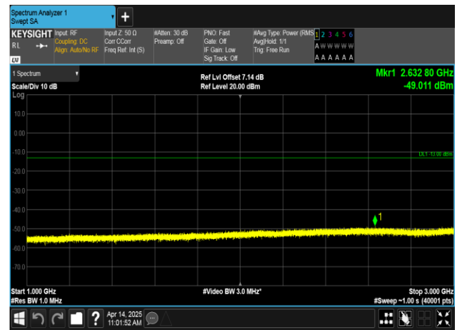
Band13-10MHz-16QAM-23230-1RB#49-1000~3000-PASS
