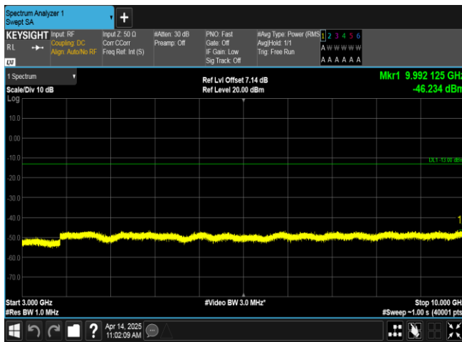
Band13-10MHz-16QAM-23230-1RB#49-3000~10000-PASS
