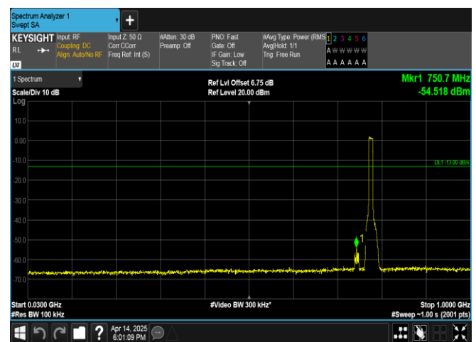
Band13-10MHz-16QAM-23230-50RB#0-30~1000-PASS
