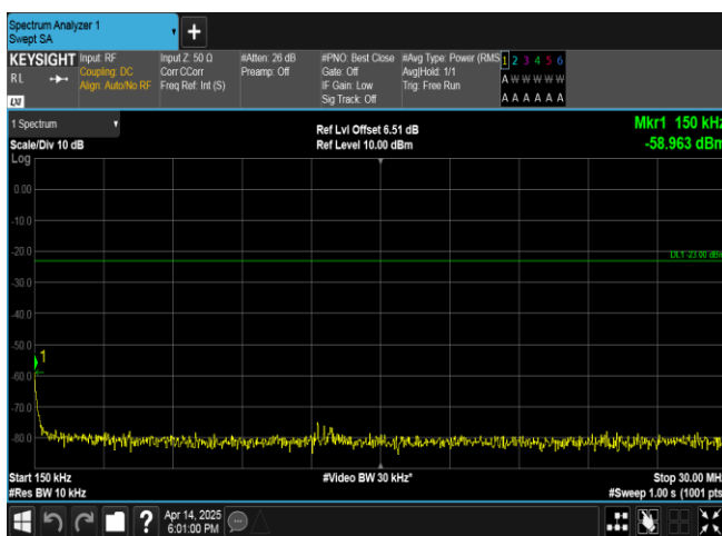
Band13-10MHz-16QAM-23230-50RB#0-0.15~30-PASS
