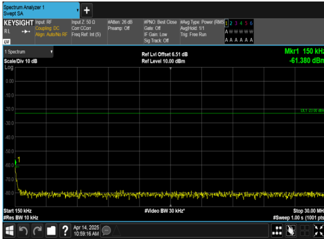
Band13-10MHz-16QAM-23230-1RB#0-0.15~30-PASS
