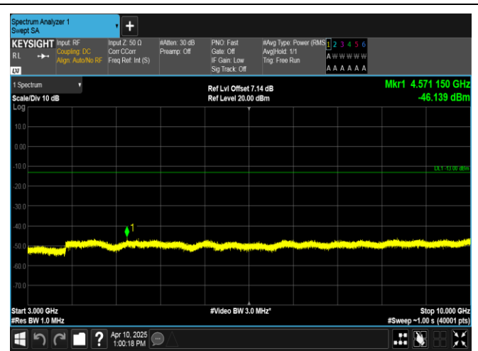
Band13-5MHz-16QAM-23205-25RB#0-3000~10000-PASS
