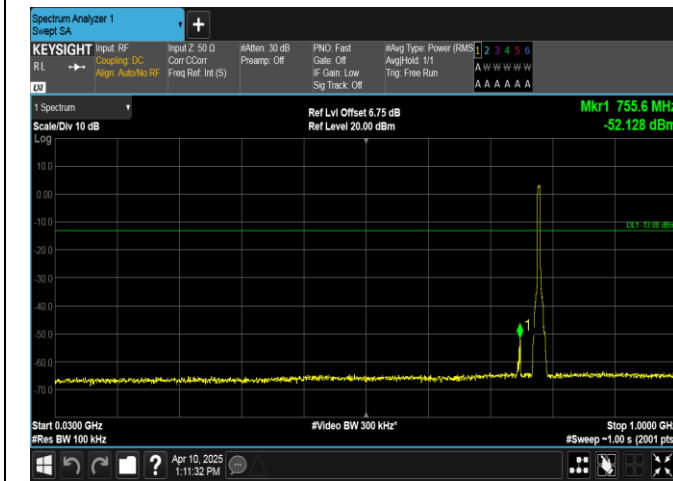
Band13-5MHz-QPSK-23255-25RB#0-30~1000-PASS
