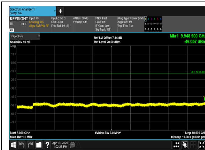
Band13-5MHz-16QAM-23230-1RB#0-3000~10000-PASS
