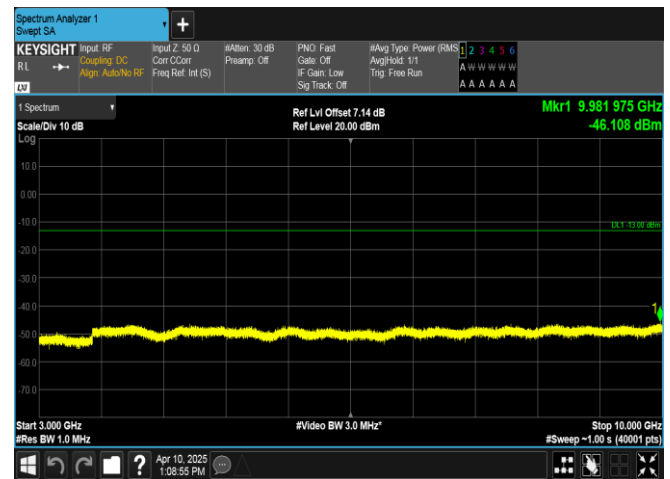
Band13-5MHz-16QAM-23255-1RB#0-3000~10000-PASS
