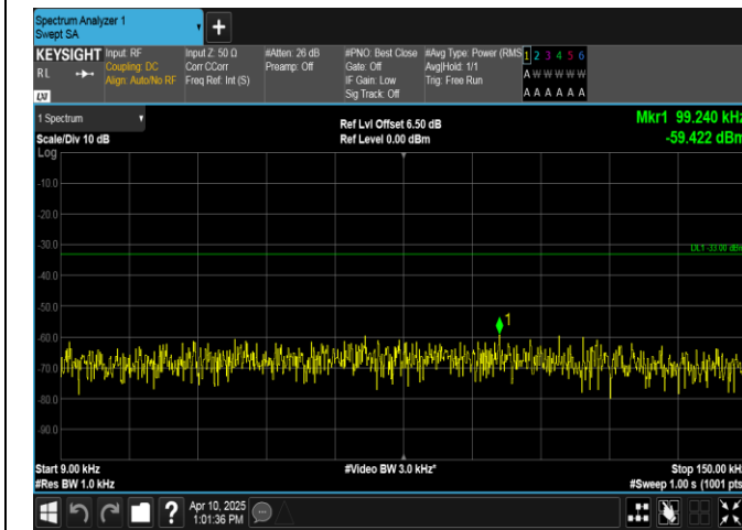
Band13-5MHz-16QAM-23230-1RB#0-0.009~0.15-PASS
