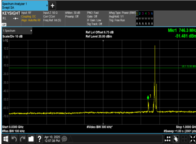
Band13-5MHz-16QAM-23205-1RB#24-30~1000-PASS
