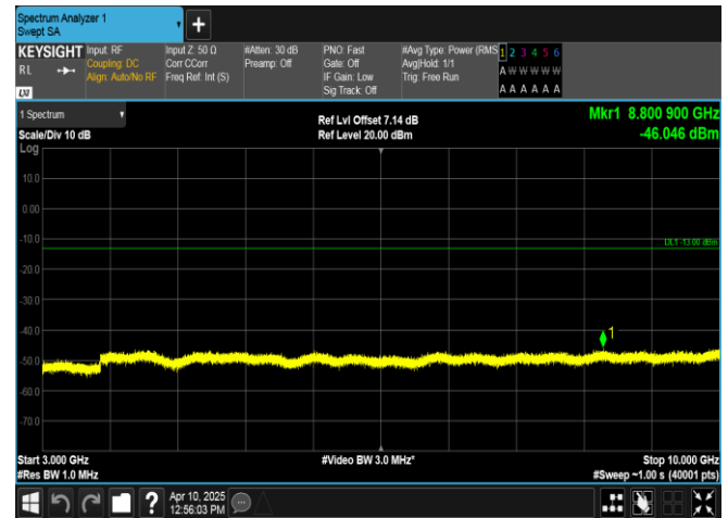
Band13-5MHz-16QAM-23205-1RB#0-3000~10000-PASS
