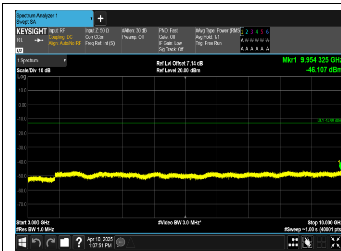
Band13-5MHz-QPSK-23255-1RB#0-3000~10000-PASS
