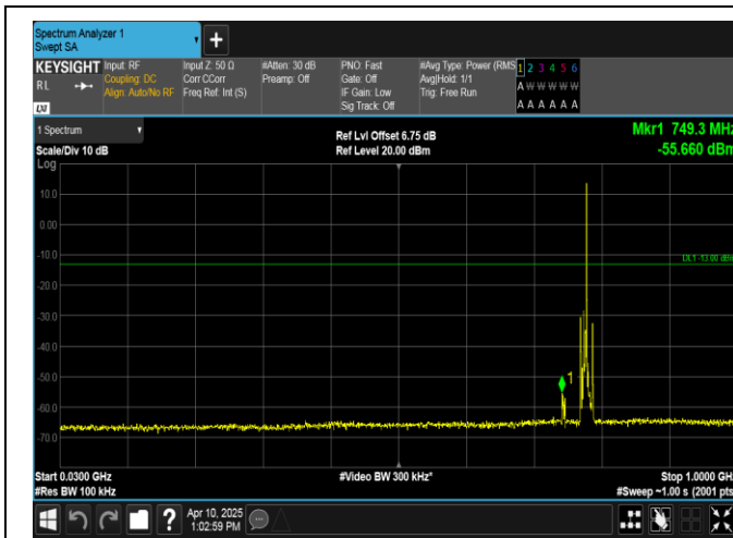
Band13-5MHz-QPSK-23230-1RB#24-30~1000-PASS
