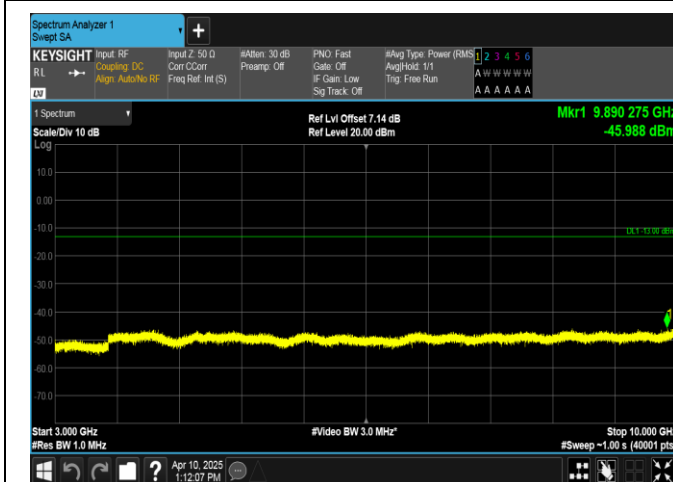
Band13-5MHz-QPSK-23255-25RB#0-3000~10000-PASS
