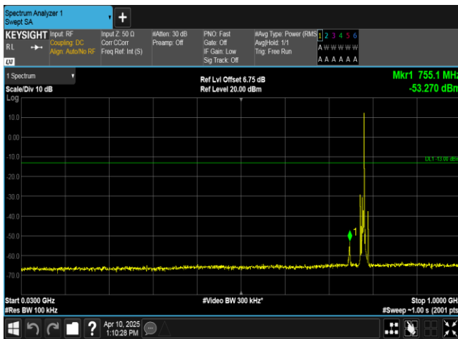
Band13-5MHz-16QAM-23255-1RB#24-30~1000-PASS
