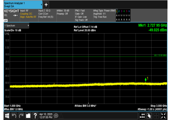
Band13-5MHz-16QAM-23205-1RB#24-1000~3000-PASS
