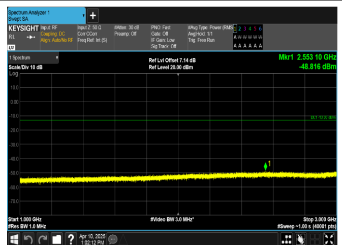
Band13-5MHz-16QAM-23230-1RB#0-1000~3000-PASS
