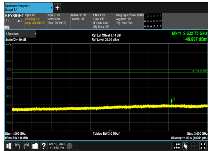
Band13-5MHz-QPSK-23255-25RB#0-1000~3000-PASS
