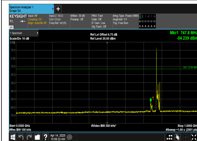
Band13-10MHz-QPSK-23230-1RB#0-30~1000-PASS
