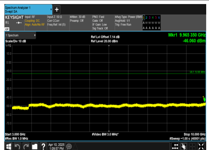
Band13-5MHz-QPSK-23255-1RB#24-3000~10000-PASS
