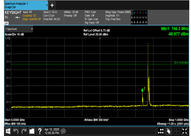
Band13-5MHz-16QAM-23205-1RB#0-30~1000-PASS
