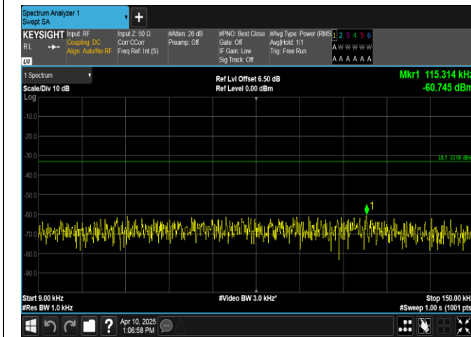
Band13-5MHz-QPSK-23255-1RB#0-0.009~0.15-PASS
