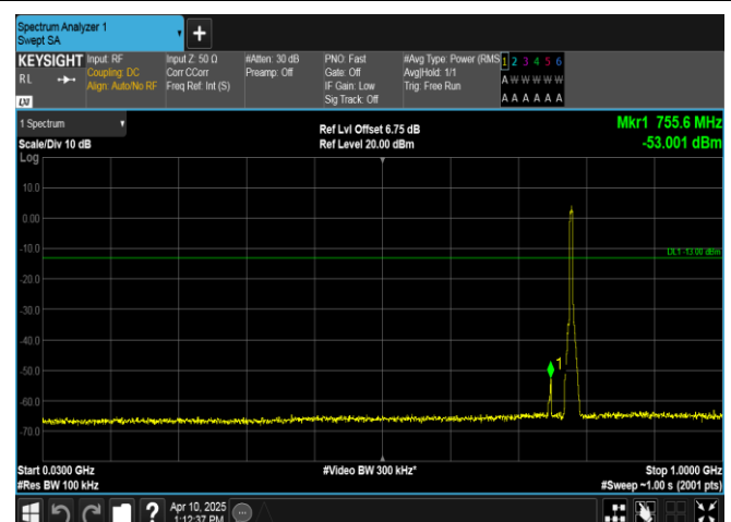
Band13-5MHz-16QAM-23255-25RB#0-30~1000-PASS
