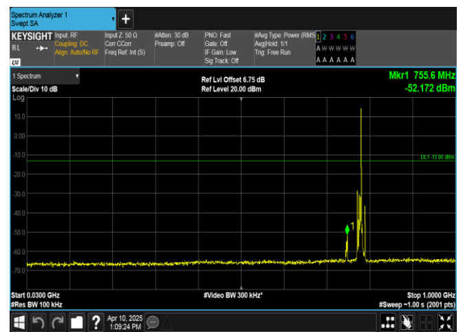
Band13-5MHz-QPSK-23255-1RB#24-30~1000-PASS
