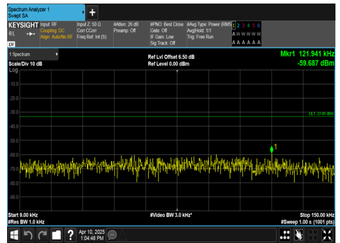
Band13-5MHz-QPSK-23230-25RB#0-0.009~0.15-PASS
