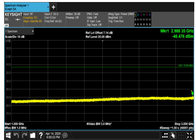
Band13-10MHz-QPSK-23230-50RB#0-1000~3000-PASS
