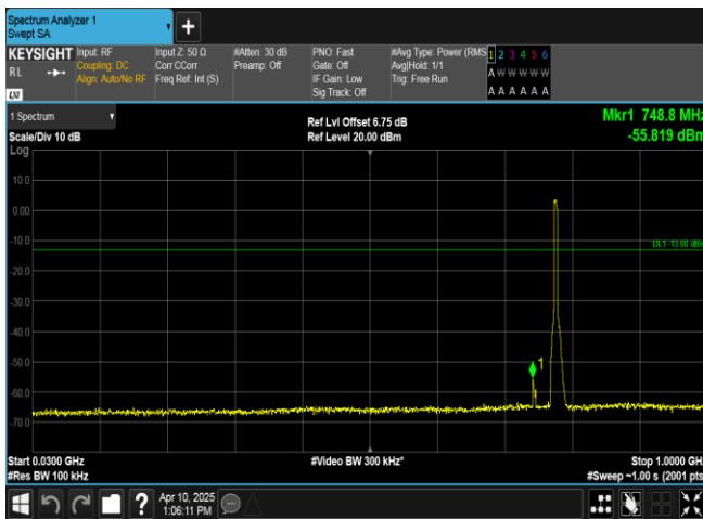
Band13-5MHz-16QAM-23230-25RB#0-30~1000-PASS
