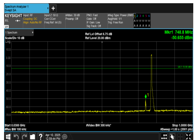
Band13-5MHz-16QAM-23205-25RB#0-30~1000-PASS
