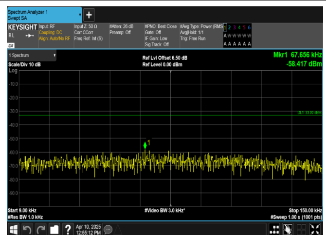
Band13-5MHz-16QAM-23205-1RB#0-0.009~0.15-PASS
