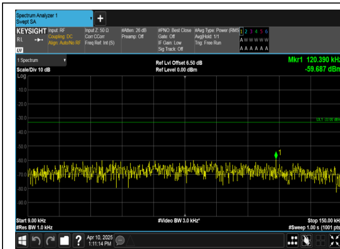
Band13-5MHz-QPSK-23255-25RB#0-0.009~0.15-PASS
