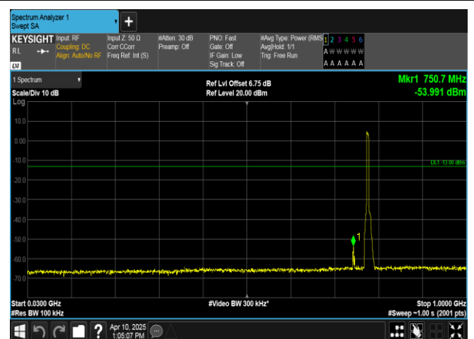
Band13-5MHz-QPSK-23230-25RB#0-30~1000-PASS
