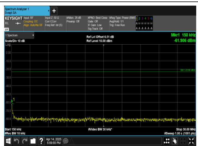
Band13-10MHz-QPSK-23230-50RB#0-0.15~30-PASS
