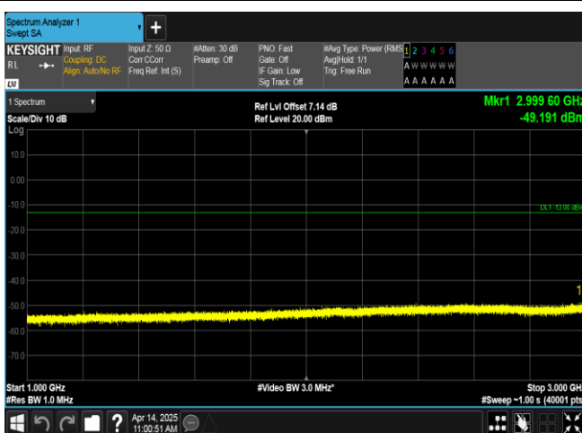
Band13-10MHz-QPSK-23230-1RB#49-1000~3000-PASS
