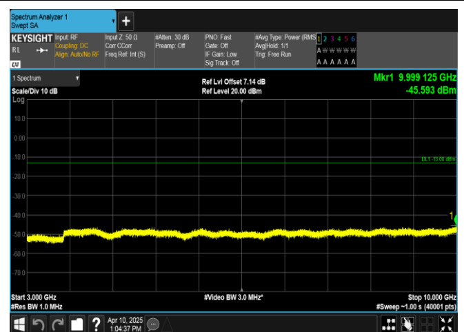
Band13-5MHz-16QAM-23230-1RB#24-3000~10000-PASS
