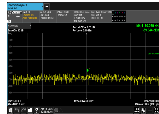
Band13-10MHz-QPSK-23230-1RB#0-0.009~0.15-PASS
