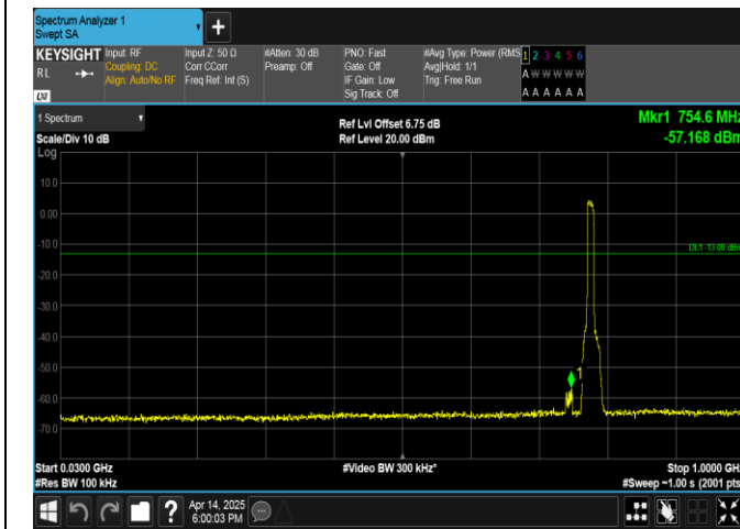
Band13-10MHz-QPSK-23230-50RB#0-30~1000-PASS
