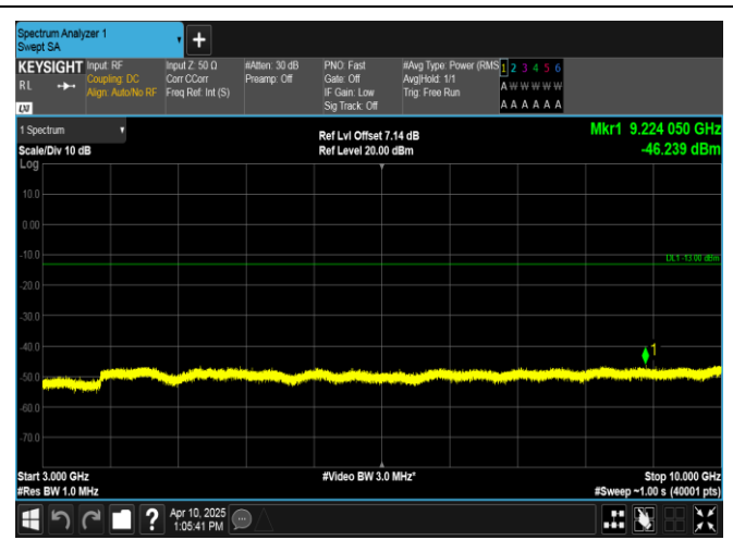
Band13-5MHz-QPSK-23230-25RB#0-3000~10000-PASS
