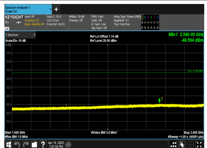
Band13-5MHz-QPSK-23255-1RB#0-1000~3000-PASS
