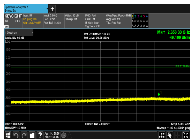
Band13-10MHz-QPSK-23230-1RB#0-1000~3000-PASS
