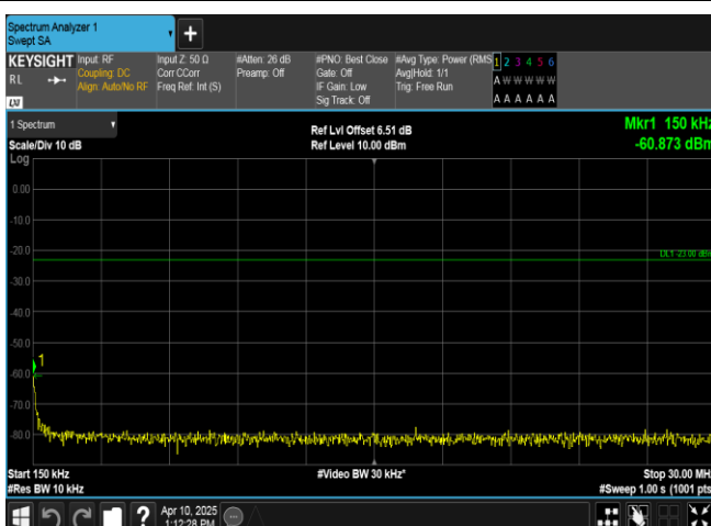
Band13-5MHz-16QAM-23255-25RB#0-0.15~30-PASS
