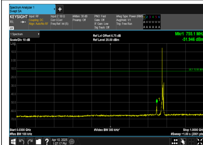
Band13-5MHz-QPSK-23255-1RB#0-30~1000-PASS
