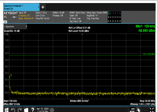
Band13-5MHz-16QAM-23255-1RB#24-0.15~30-PASS
