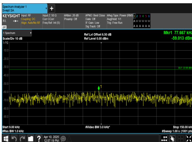
Band13-5MHz-16QAM-23205-1RB#24-0.009~0.15-PASS
