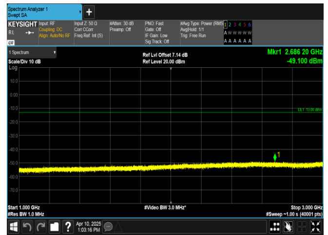
Band13-5MHz-QPSK-23230-1RB#24-1000~3000-PASS
