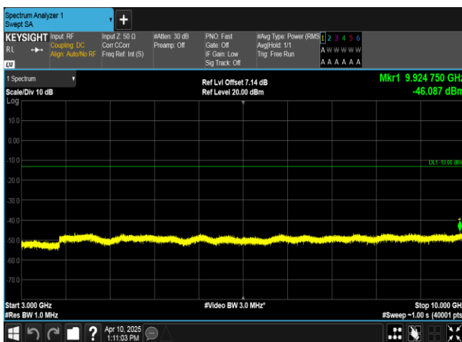
Band13-5MHz-16QAM-23255-1RB#24-3000~10000-PASS
