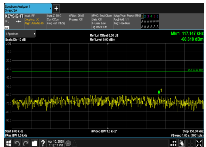
Band13-5MHz-16QAM-23255-25RB#0-0.009~0.15-PASS
