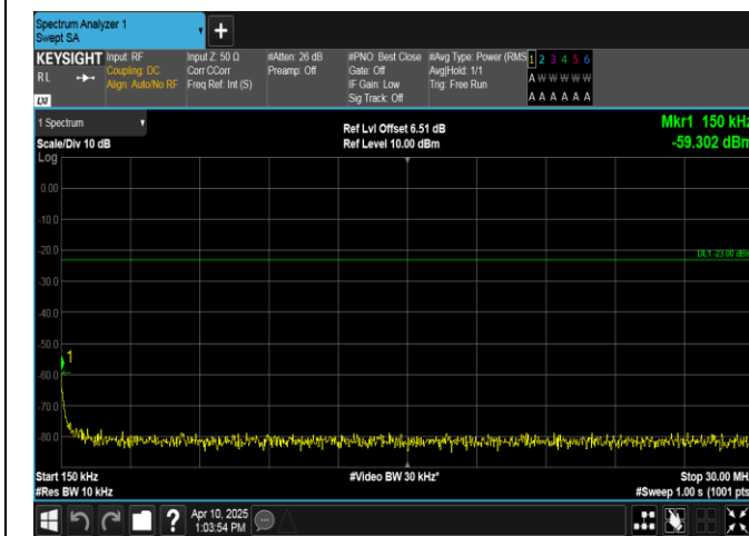
Band13-5MHz-16QAM-23230-1RB#24-0.15~30-PASS
