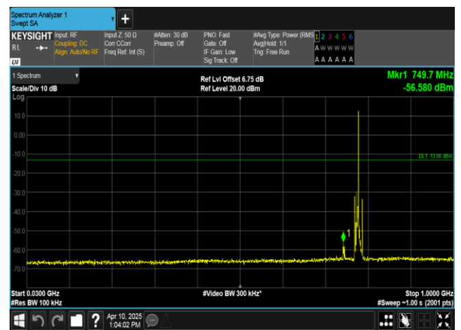
Band13-5MHz-16QAM-23230-1RB#24-30~1000-PASS
