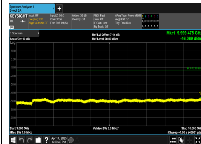
Band13-10MHz-QPSK-23230-50RB#0-3000~10000-PASS
