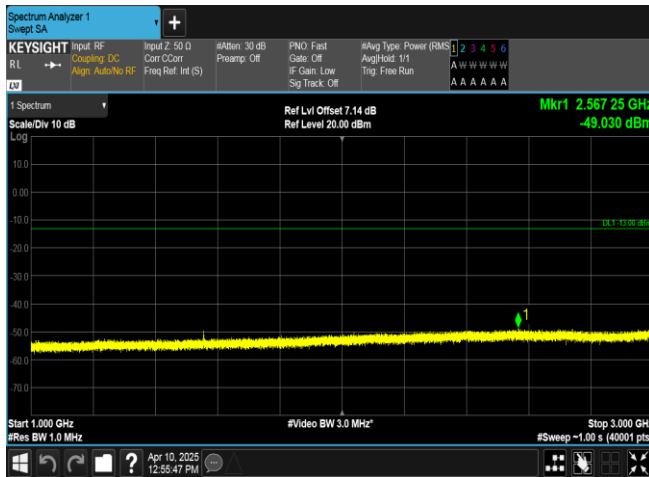
Band13-5MHz-16QAM-23205-1RB#0-1000~3000-PASS
