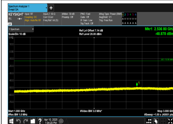
Band13-5MHz-16QAM-23230-1RB#24-1000~3000-PASS
