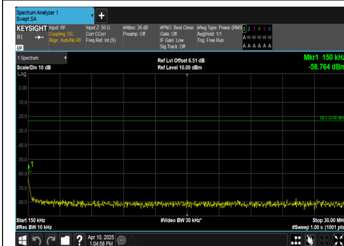
Band13-5MHz-QPSK-23230-25RB#0-0.15~30-PASS
