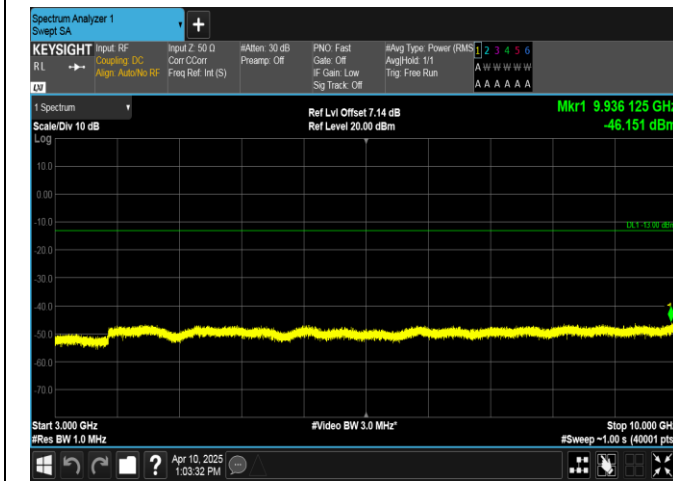
Band13-5MHz-QPSK-23230-1RB#24-3000~10000-PASS
