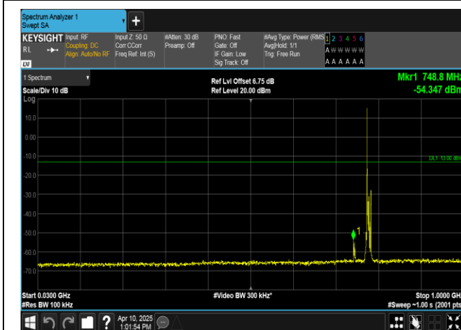
Band13-5MHz-16QAM-23230-1RB#0-30~1000-PASS
