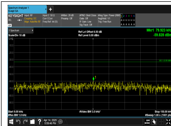
Band13-10MHz-QPSK-23230-50RB#0-0.009~0.15-PASS
