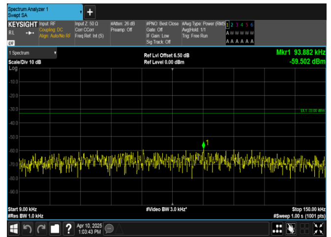
Band13-5MHz-16QAM-23230-1RB#24-0.009~0.15-PASS
