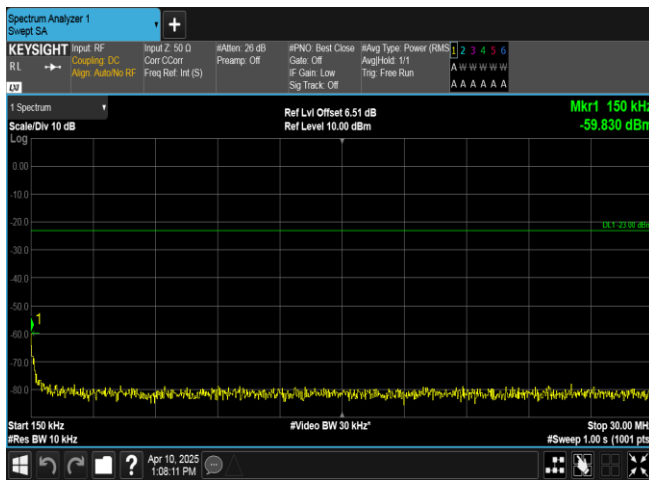
Band13-5MHz-16QAM-23255-1RB#0-0.15~30-PASS
