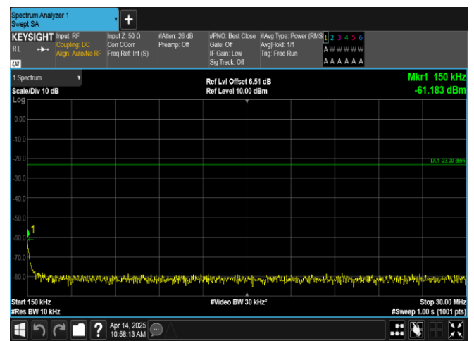
Band13-10MHz-QPSK-23230-1RB#0-0.15~30-PASS
