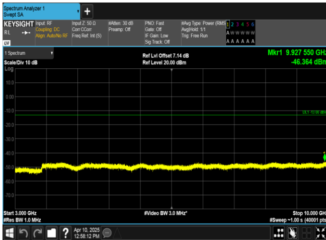
Band13-5MHz-16QAM-23205-1RB#24-3000~10000-PASS
