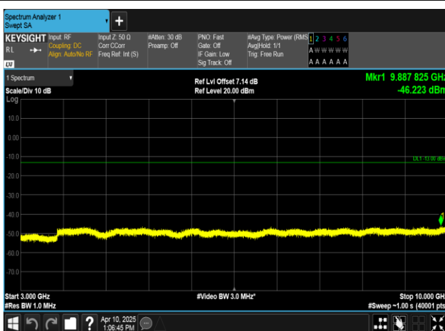
Band13-5MHz-16QAM-23230-25RB#0-3000~10000-PASS
