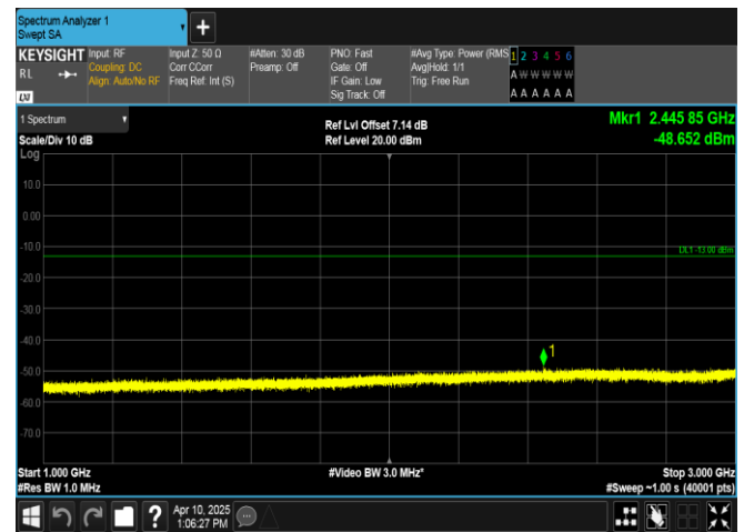
Band13-5MHz-16QAM-23230-25RB#0-1000~3000-PASS
