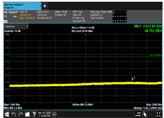
Band13-5MHz-16QAM-23255-1RB#24-1000~3000-PASS
