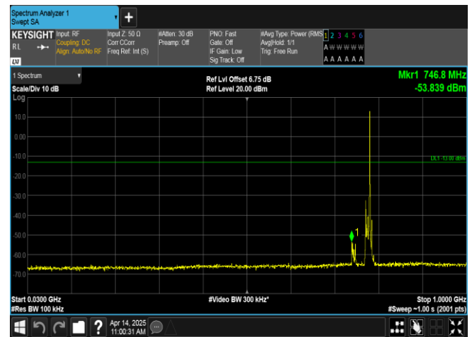
Band13-10MHz-QPSK-23230-1RB#49-30~1000-PASS
