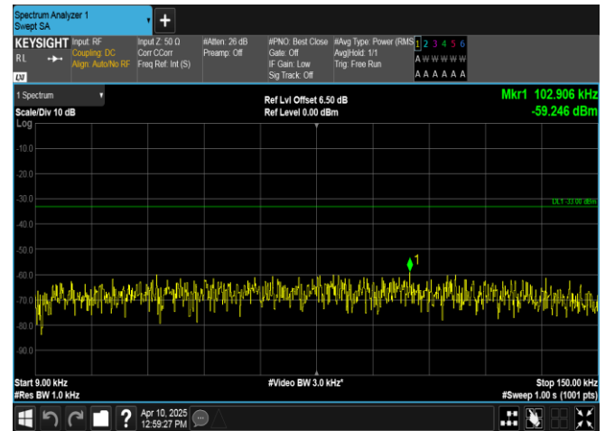
Band13-5MHz-16QAM-23205-25RB#0-0.009~0.15-PASS
