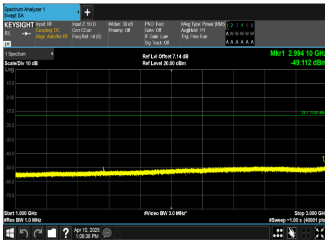
Band13-5MHz-16QAM-23255-1RB#0-1000~3000-PASS
