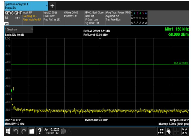
Band13-5MHz-16QAM-23230-25RB#0-0.15~30-PASS
