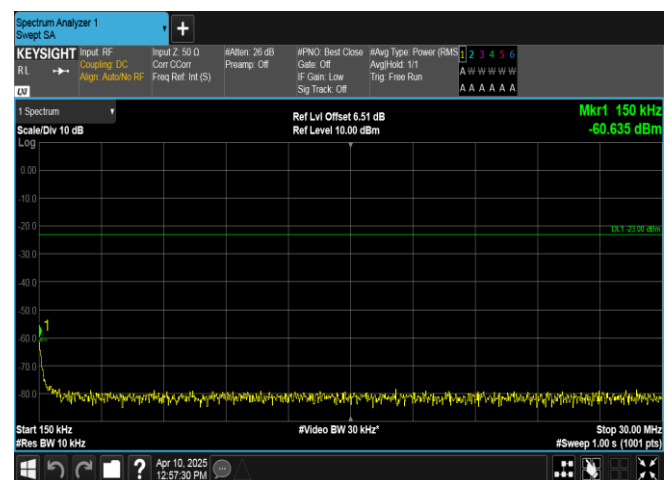
Band13-5MHz-16QAM-23205-1RB#24-0.15~30-PASS
