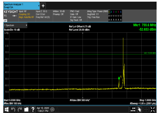
Band13-5MHz-16QAM-23255-1RB#0-30~1000-PASS
