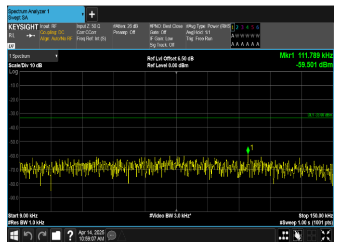
Band13-10MHz-16QAM-23230-1RB#0-0.009~0.15-PASS
