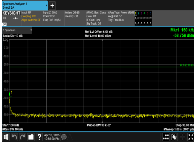
Band13-5MHz-16QAM-23205-1RB#0-0.15~30-PASS
