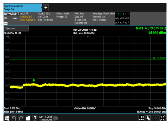
Band13-10MHz-QPSK-23230-1RB#49-3000~10000-PASS
