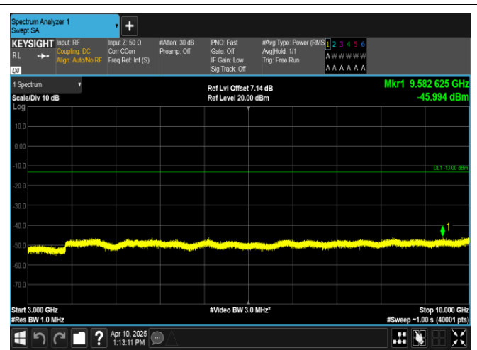
Band13-5MHz-16QAM-23255-25RB#0-3000~10000-PASS
