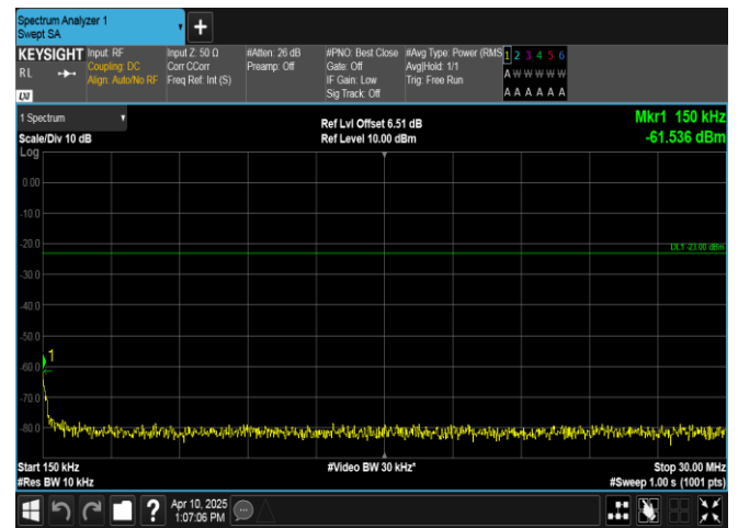
Band13-5MHz-QPSK-23255-1RB#0-0.15~30-PASS
