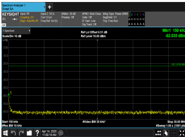
Band13-10MHz-QPSK-23230-1RB#49-0.15~30-PASS
