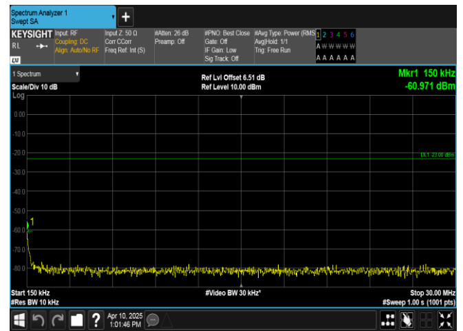
Band13-5MHz-16QAM-23230-1RB#0-0.15~30-PASS
