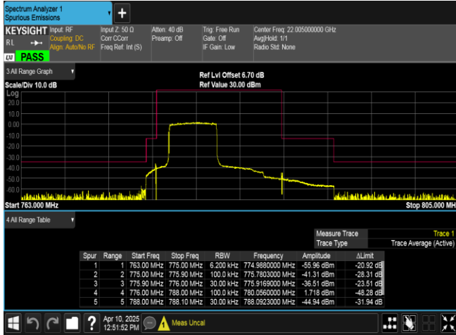
Band13-5MHz-QPSK-23205-25RB#0-PASS
