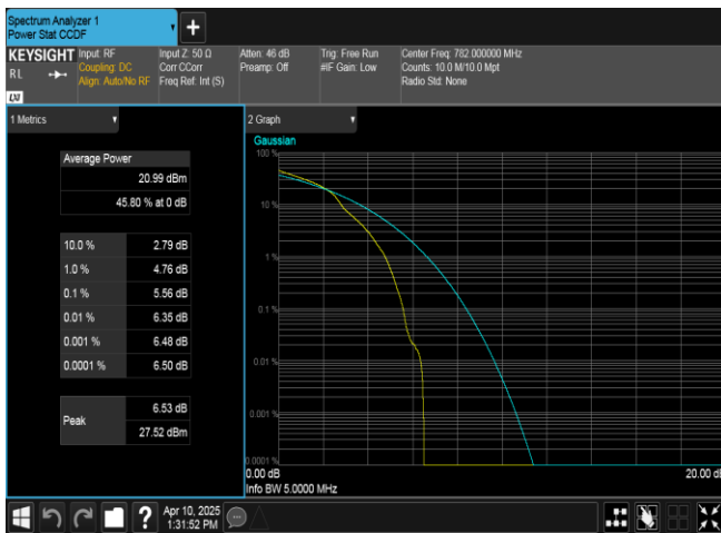
Band13-5MHz-16QAM-23230-1RB#0-PASS
