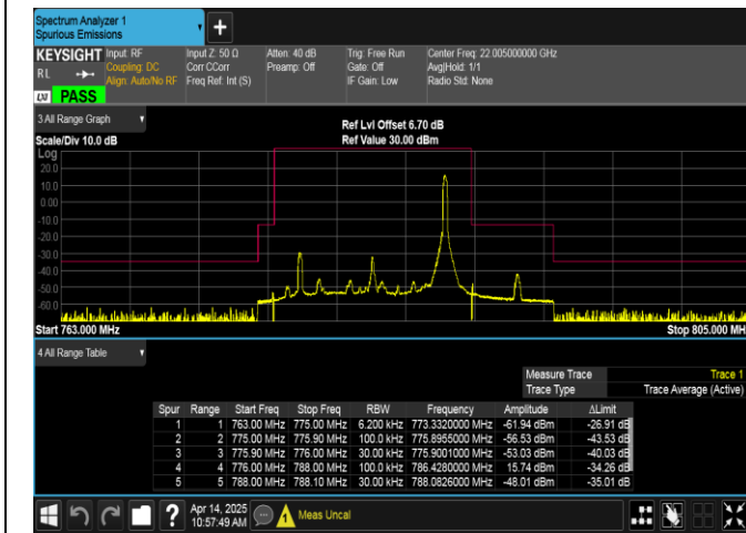
Band13-10MHz-16QAM-23230-1RB#49-PASS
