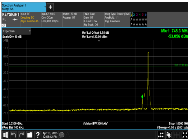
Band13-5MHz-QPSK-23205-25RB#0-30~1000-PASS
