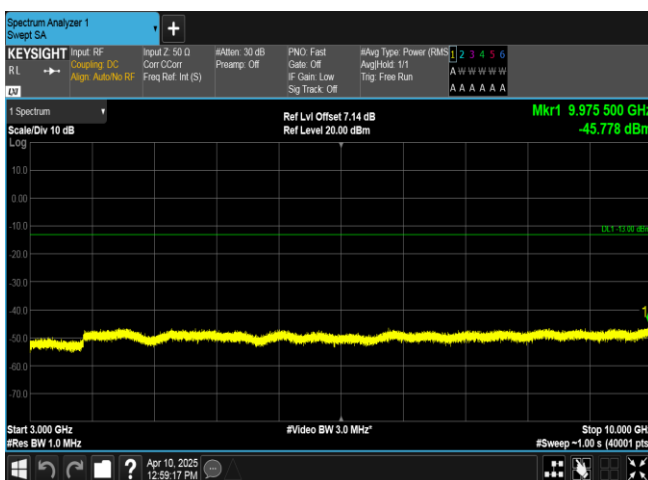
Band13-5MHz-QPSK-23205-25RB#0-3000~10000-PASS
