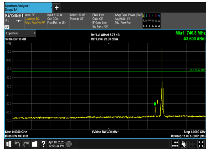
Band13-5MHz-QPSK-23205-1RB#24-30~1000-PASS
