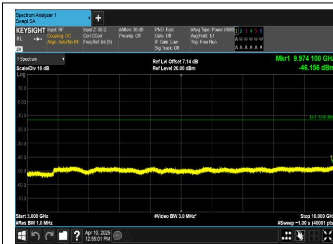
Band13-5MHz-QPSK-23205-1RB#0-3000~10000-PASS
