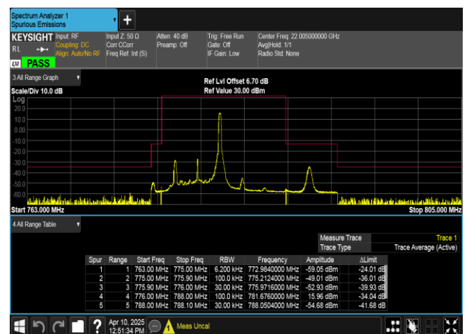
Band13-5MHz-16QAM-23205-1RB#24-PASS
