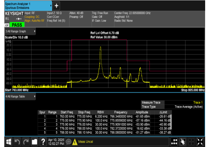
Band13-5MHz-QPSK-23255-1RB#0-PASS
