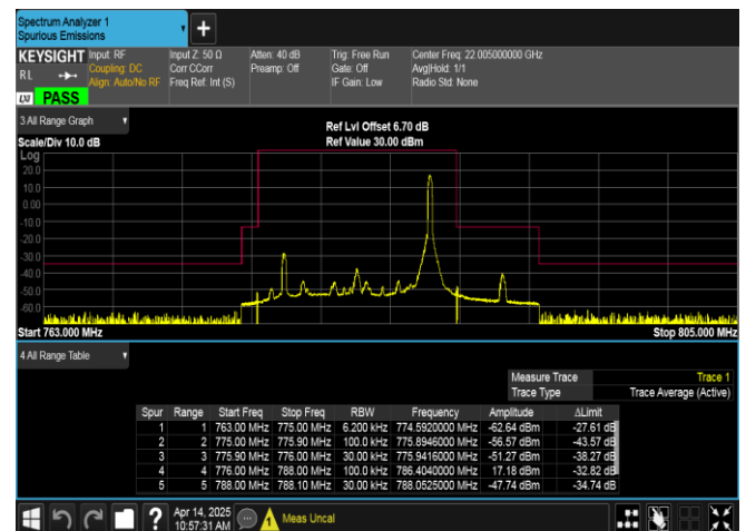
Band13-10MHz-QPSK-23230-1RB#49-PASS
