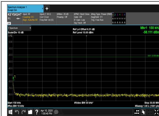
Band13-5MHz-QPSK-23230-1RB#0-0.15~30-PASS
