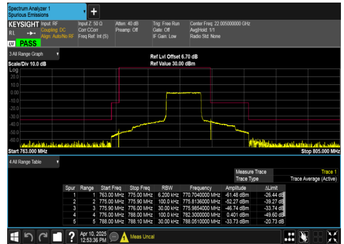
Band13-5MHz-QPSK-23255-25RB#0-PASS
