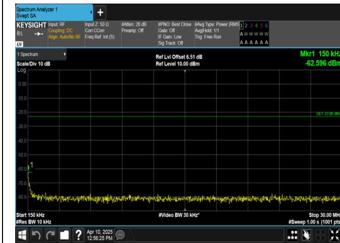
Band13-5MHz-QPSK-23205-1RB#24-0.15~30-PASS
