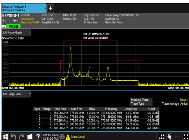
Band13-5MHz-16QAM-23205-1RB#0-PASS
