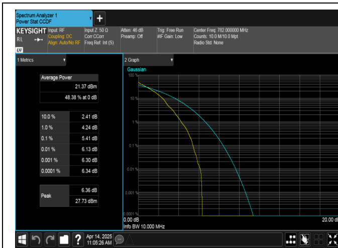
Band13-10MHz-QPSK-23230-1RB#0-PASS
