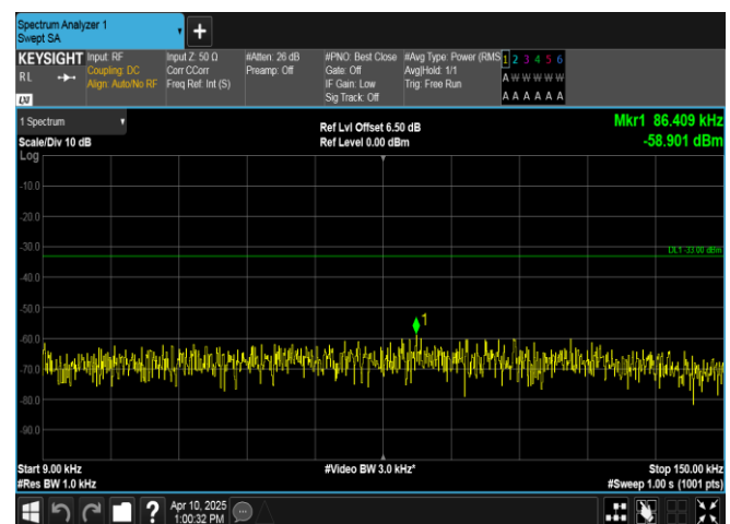
Band13-5MHz-QPSK-23230-1RB#0-0.009~0.15-PASS
