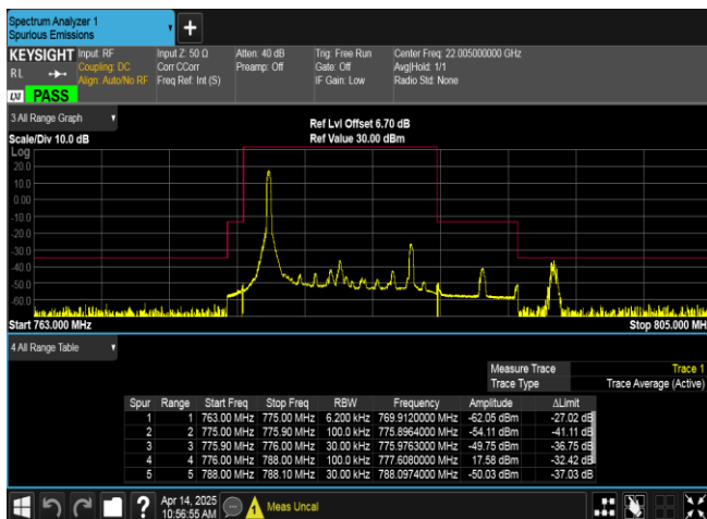
Band13-10MHz-QPSK-23230-1RB#0-PASS
