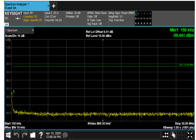
Band13-5MHz-QPSK-23205-25RB#0-0.15~30-PASS
