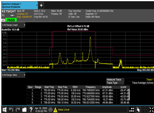
Band13-5MHz-QPSK-23255-1RB#24-PASS
