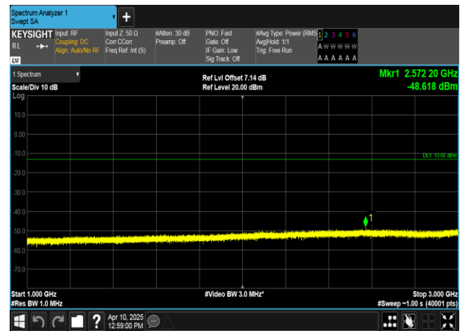
Band13-5MHz-QPSK-23205-25RB#0-1000~3000-PASS
