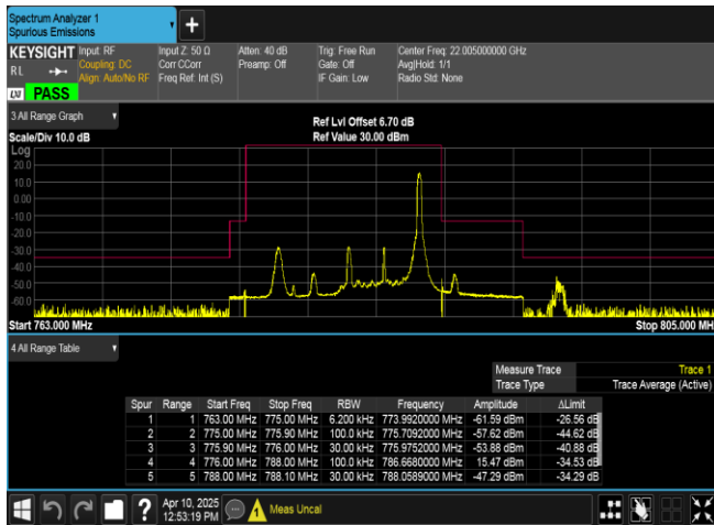
Band13-5MHz-16QAM-23255-1RB#24-PASS
