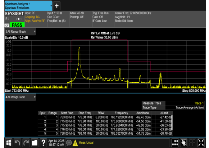
Band13-10MHz-16QAM-23230-1RB#0-PASS
