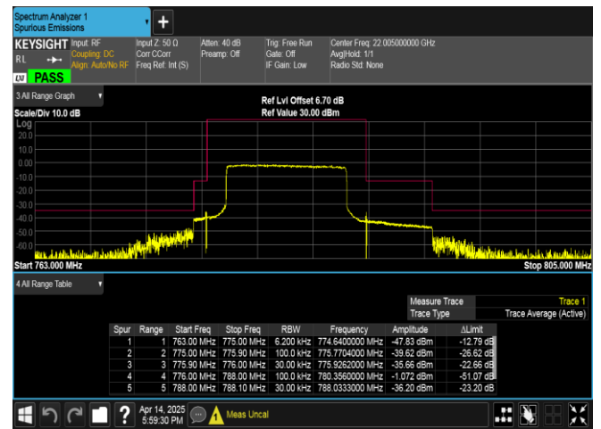
Band13-10MHz-16QAM-23230-50RB#0-PASS
