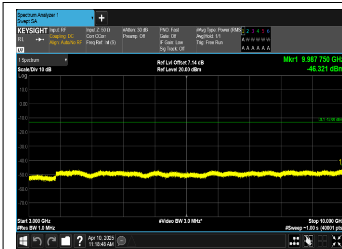
Band12-5MHz-QPSK-23155-1RB#0-3000~10000-PASS
