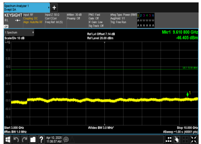
Band12-5MHz-16QAM-23035-1RB#0-3000~10000-PASS
