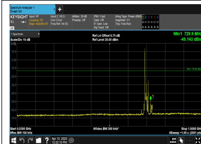
Band12-10MHz-QPSK-23060-1RB#0-30~1000-PASS
