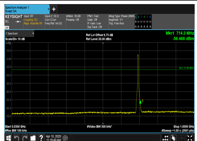
Band12-5MHz-16QAM-23035-25RB#0-30~1000-PASS
