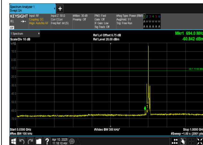
Band12-5MHz-QPSK-23155-1RB#0-30~1000-PASS
