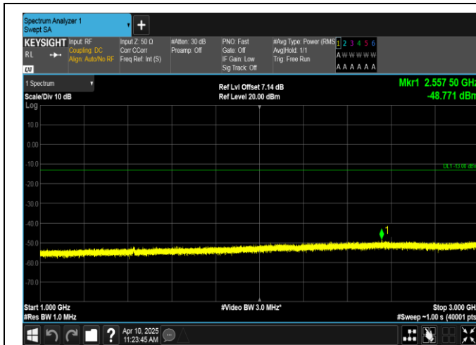
Band12-5MHz-16QAM-23155-25RB#0-1000~3000-PASS
