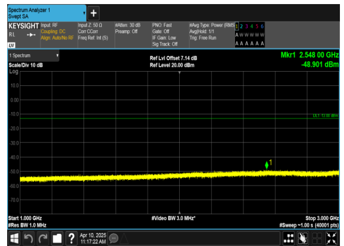
Band12-5MHz-16QAM-23095-25RB#0-1000~3000-PASS
