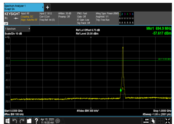
Band12-5MHz-QPSK-23095-25RB#0-30~1000-PASS
