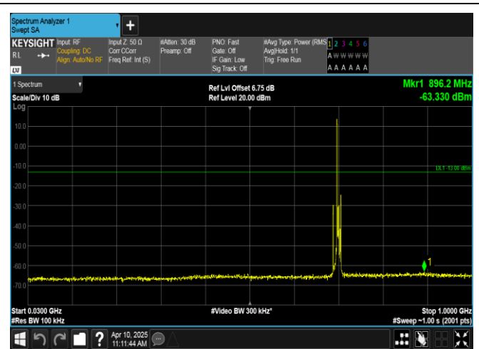
Band12-5MHz-QPSK-23095-1RB#0-30~1000-PASS
