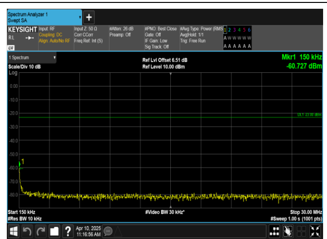
Band12-5MHz-16QAM-23095-25RB#0-0.15~30-PASS
