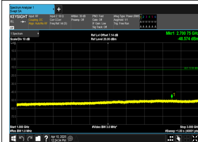
Band12-10MHz-QPSK-23060-1RB#49-1000~3000-PASS
