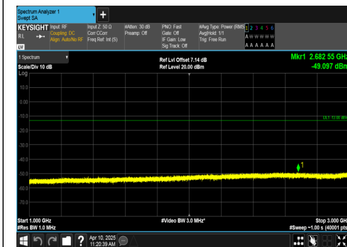
Band12-5MHz-QPSK-23155-1RB#24-1000~3000-PASS
