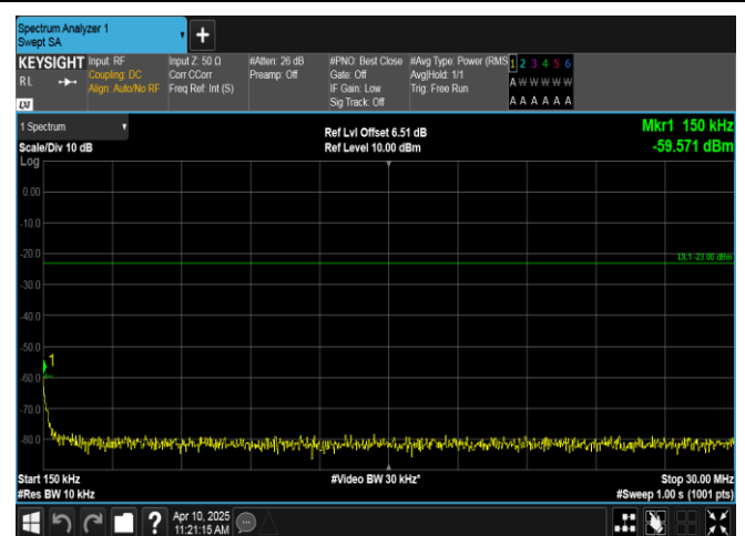
Band12-5MHz-16QAM-23155-1RB#24-0.15~30-PASS
