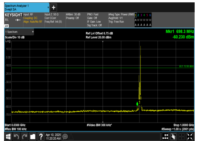
Band12-5MHz-QPSK-23155-1RB#24-30~1000-PASS
