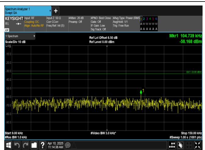
Band12-5MHz-16QAM-23095-1RB#24-0.009~0.15-PASS
