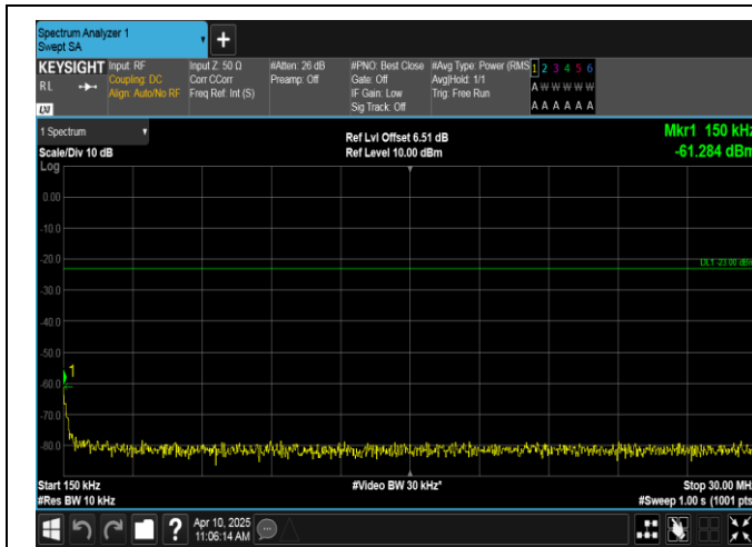
Band12-5MHz-16QAM-23035-1RB#0-0.15~30-PASS
