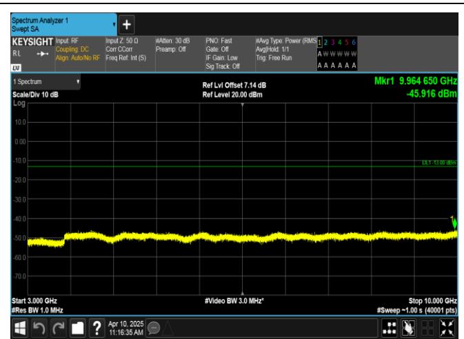
Band12-5MHz-QPSK-23095-25RB#0-3000~10000-PASS
