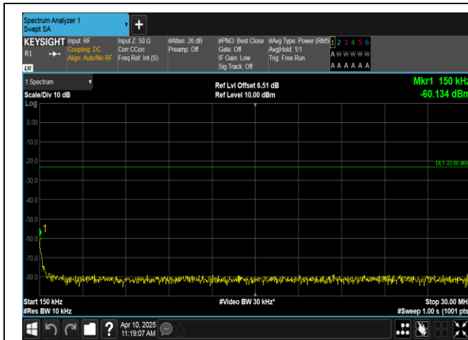
Band12-5MHz-16QAM-23155-1RB#0-0.15~30-PASS
