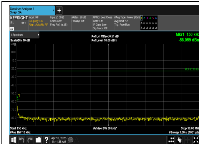
Band12-5MHz-QPSK-23095-1RB#0-0.15~30-PASS
