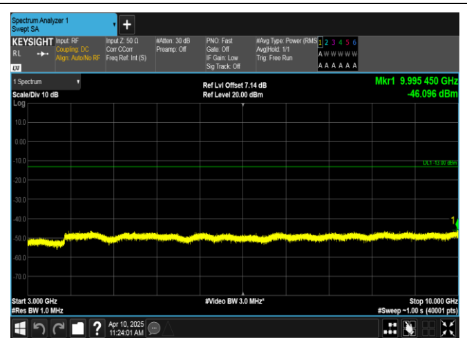
Band12-5MHz-16QAM-23155-25RB#0-3000~10000-PASS
