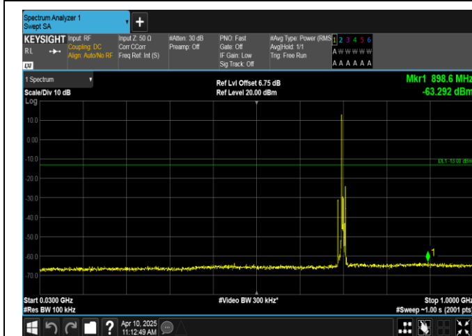
Band12-5MHz-16QAM-23095-1RB#0-30~1000-PASS
