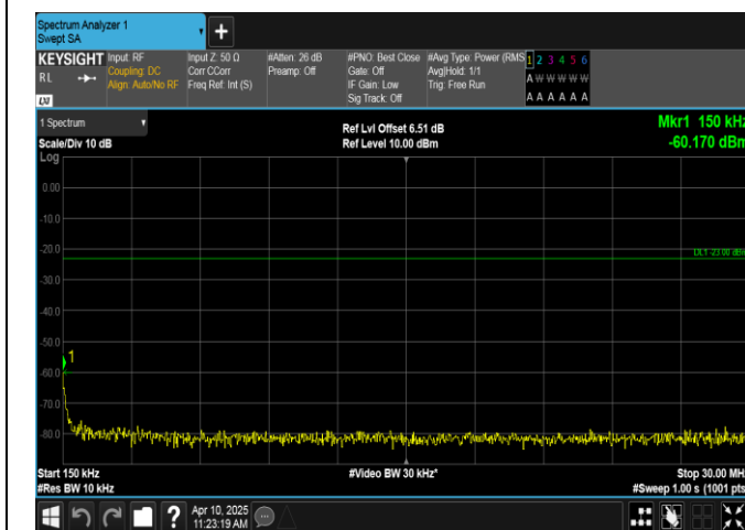
Band12-5MHz-16QAM-23155-25RB#0-0.15~30-PASS
