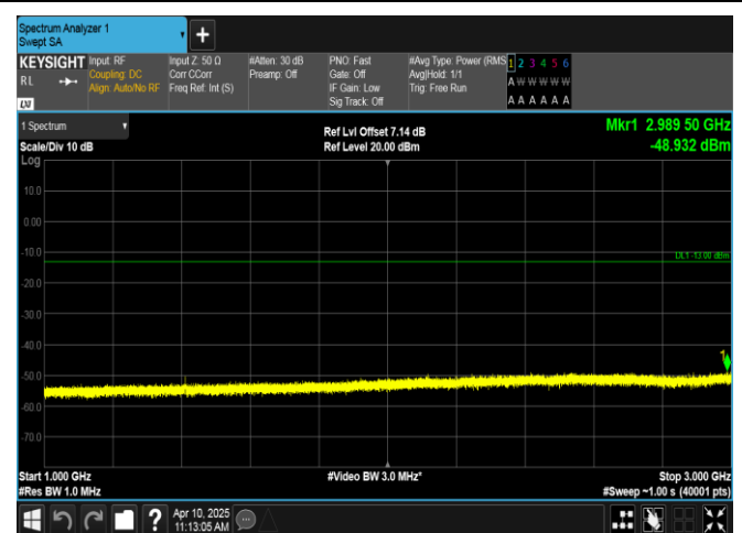
Band12-5MHz-16QAM-23095-1RB#0-1000~3000-PASS
