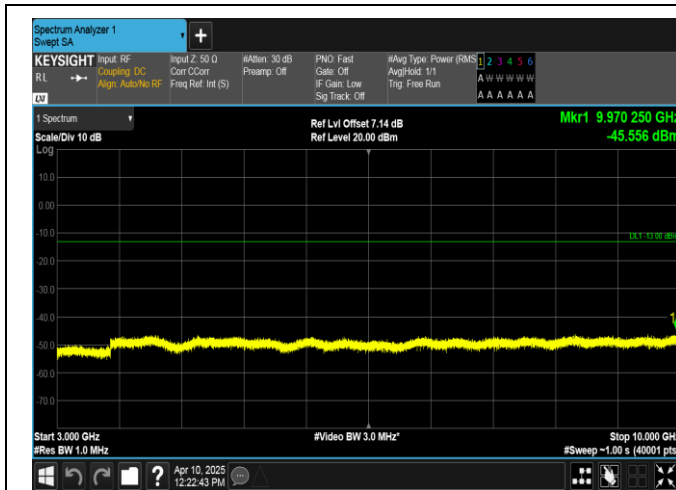
Band12-10MHz-QPSK-23060-1RB#0-3000~10000-PASS
