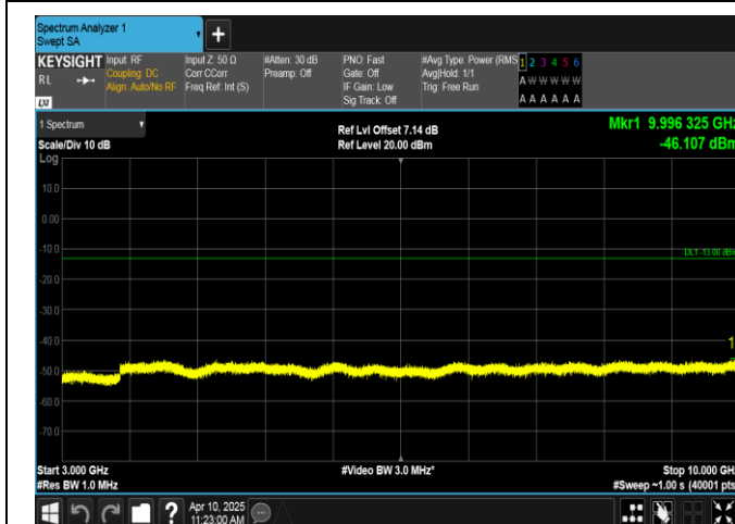
Band12-5MHz-QPSK-23155-25RB#0-3000~10000-PASS
