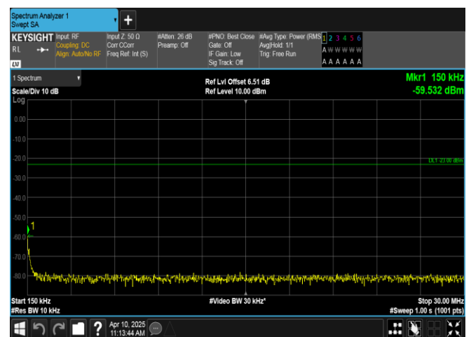
Band12-5MHz-QPSK-23095-1RB#24-0.15~30-PASS
