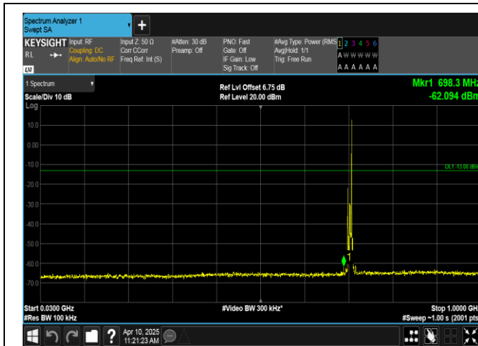
Band12-5MHz-16QAM-23155-1RB#24-30~1000-PASS
