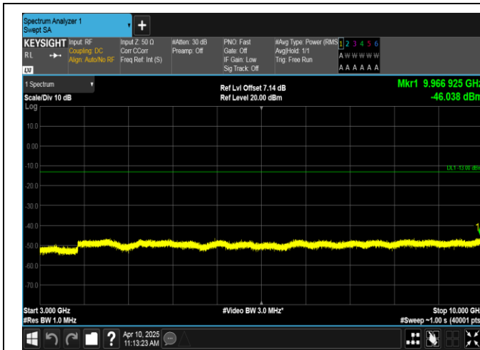
Band12-5MHz-16QAM-23095-1RB#0-3000~10000-PASS
