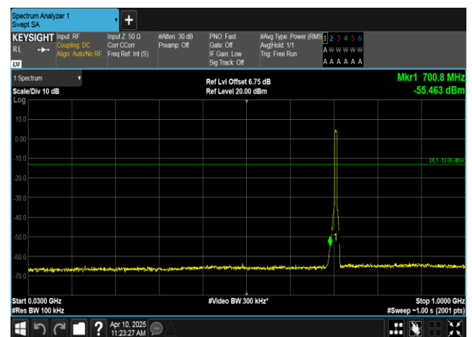
Band12-5MHz-16QAM-23155-25RB#0-30~1000-PASS
