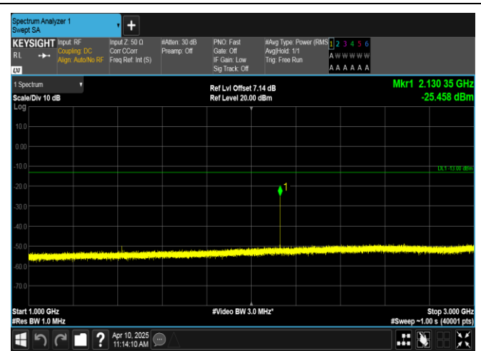
Band12-5MHz-QPSK-23095-1RB#24-1000~3000-PASS
