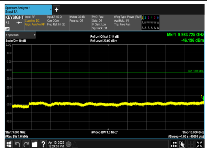
Band12-10MHz-QPSK-23060-1RB#49-3000~10000-PASS
