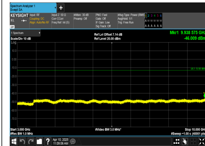
Band12-5MHz-16QAM-23035-1RB#24-3000~10000-PASS
