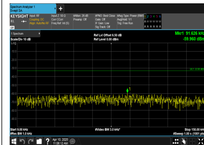
Band12-5MHz-16QAM-23035-1RB#24-0.009~0.15-PASS
