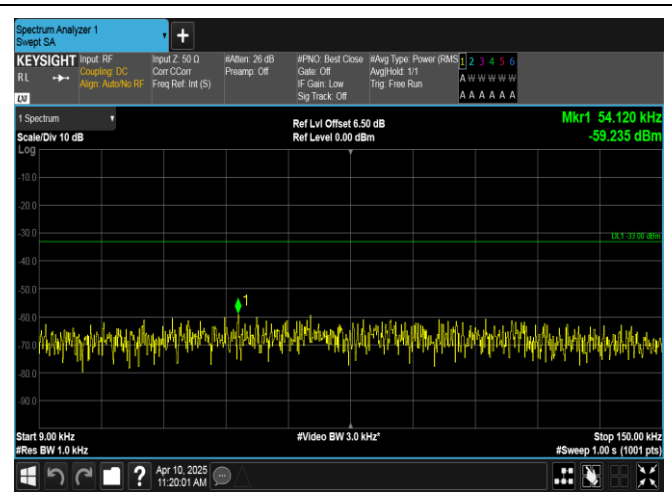
Band12-5MHz-QPSK-23155-1RB#24-0.009~0.15-PASS
