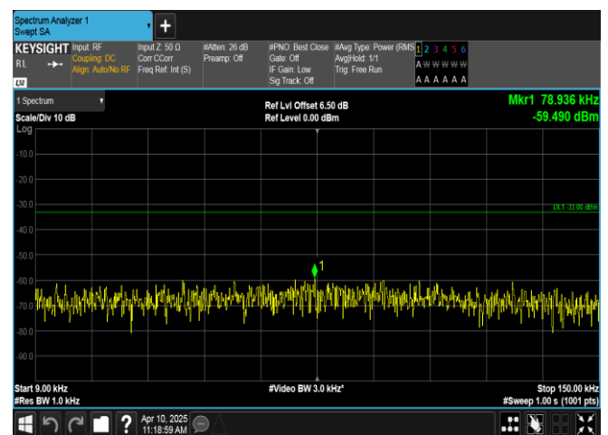
Band12-5MHz-16QAM-23155-1RB#0-0.009~0.15-PASS
