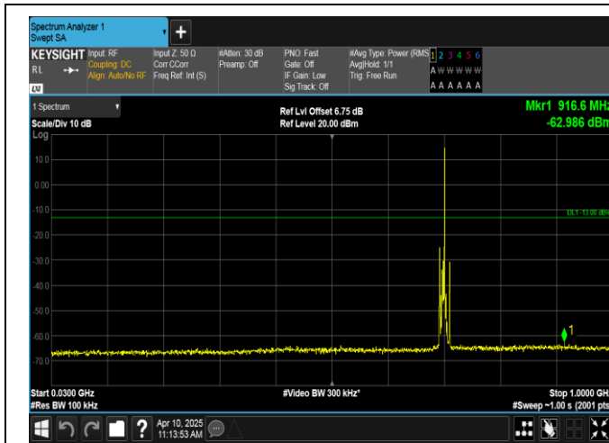
Band12-5MHz-QPSK-23095-1RB#24-30~1000-PASS
