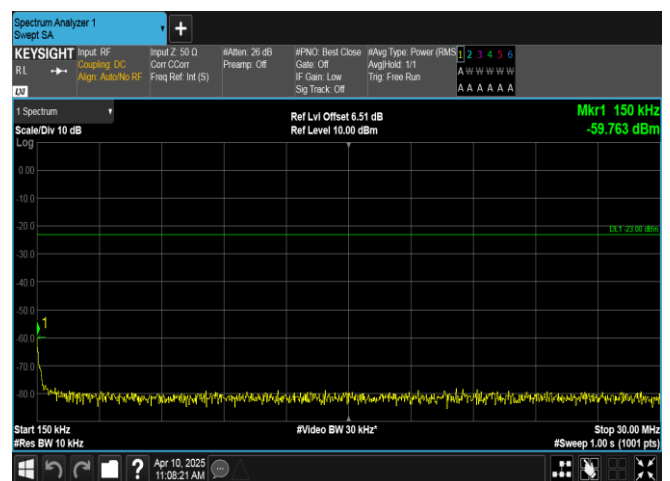
Band12-5MHz-16QAM-23035-1RB#24-0.15~30-PASS
