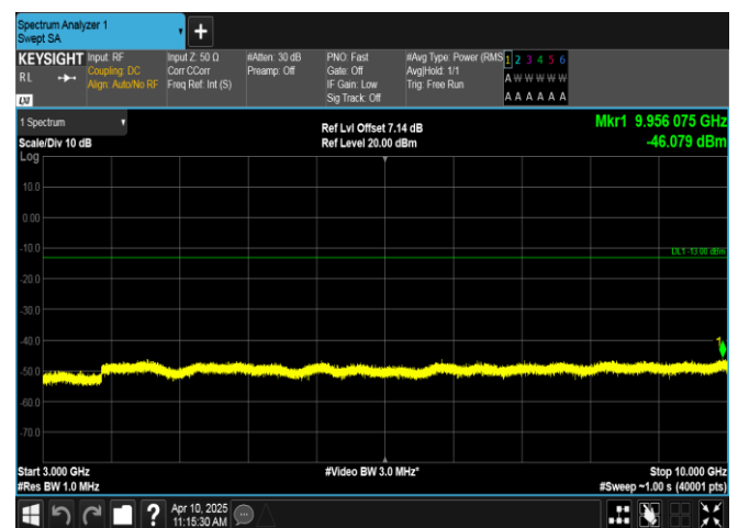
Band12-5MHz-16QAM-23095-1RB#24-3000~10000-PASS
