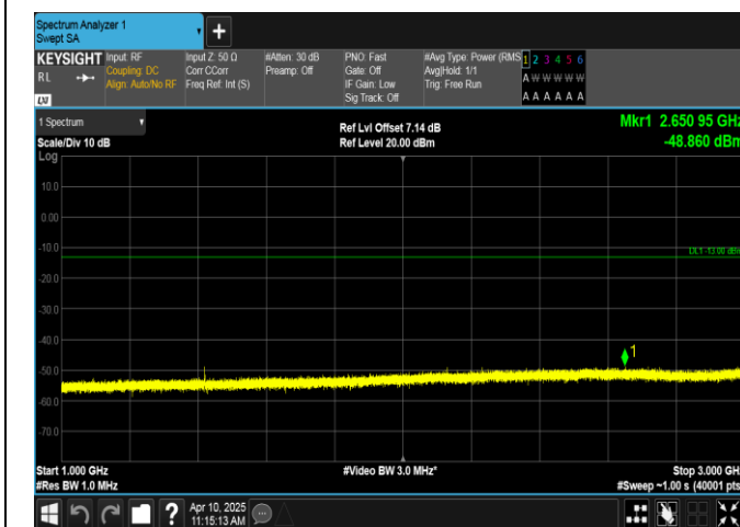
Band12-5MHz-16QAM-23095-1RB#24-1000~3000-PASS
