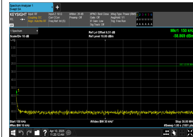
Band12-5MHz-QPSK-23155-1RB#24-0.15~30-PASS
