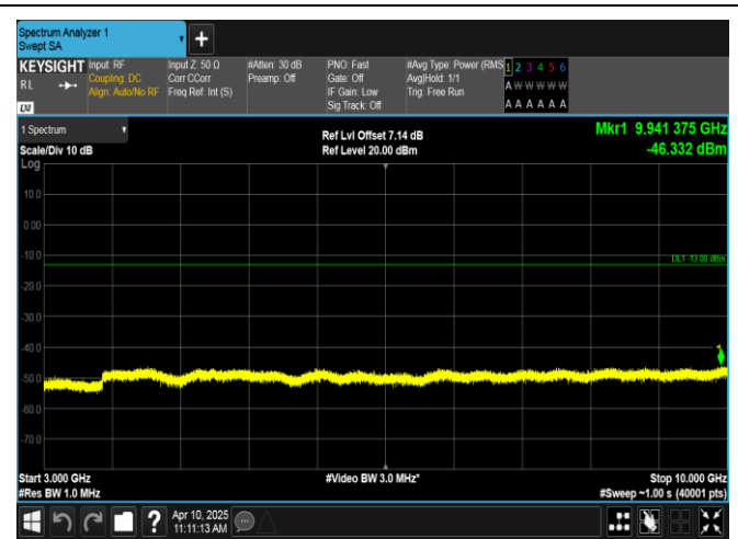
Band12-5MHz-16QAM-23035-25RB#0-3000~10000-PASS
