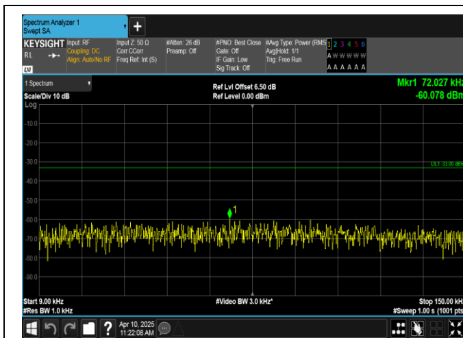
Band12-5MHz-QPSK-23155-25RB#0-0.009~0.15-PASS
