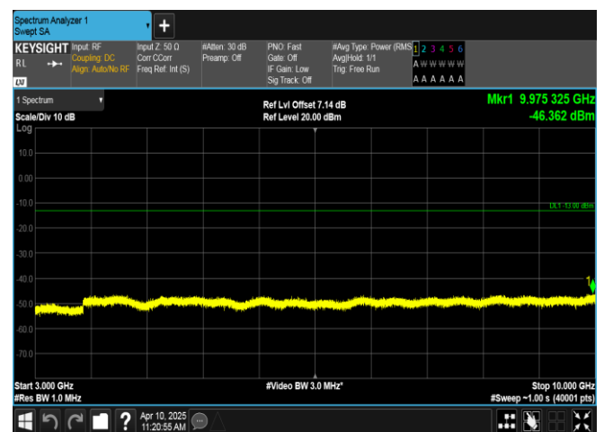
Band12-5MHz-QPSK-23155-1RB#24-3000~10000-PASS
