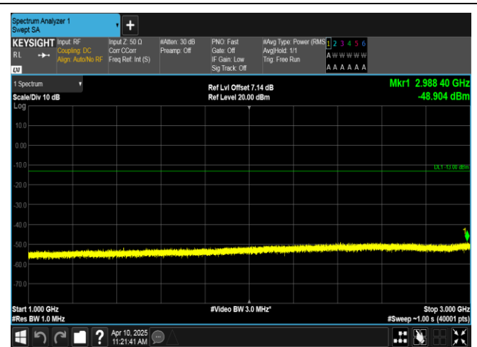
Band12-5MHz-16QAM-23155-1RB#24-1000~3000-PASS
