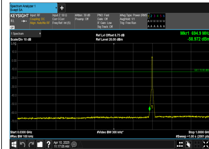
Band12-5MHz-16QAM-23095-25RB#0-30~1000-PASS
