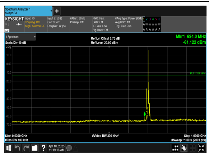
Band12-5MHz-16QAM-23155-1RB#0-30~1000-PASS
