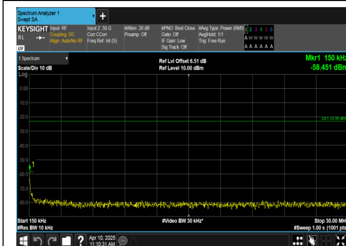
Band12-5MHz-16QAM-23035-25RB#0-0.15~30-PASS
