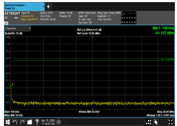
Band12-5MHz-QPSK-23155-1RB#0-0.15~30-PASS
