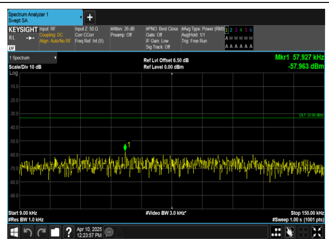
Band12-10MHz-QPSK-23060-1RB#49-0.009~0.15-PASS
