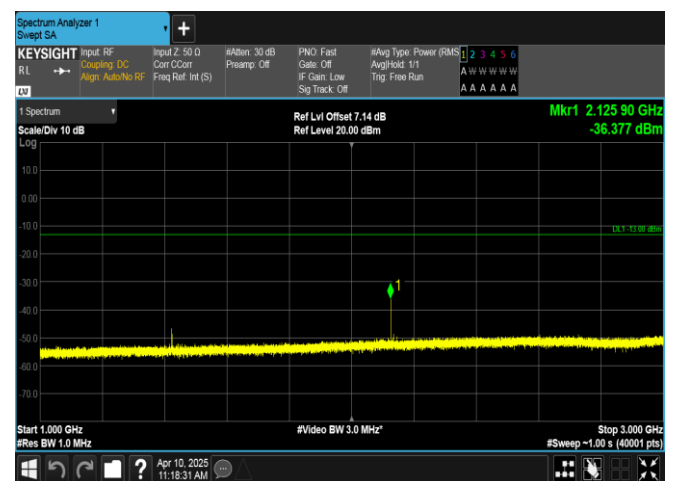
Band12-5MHz-QPSK-23155-1RB#0-1000~3000-PASS
