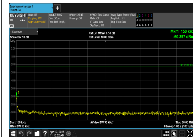
Band12-5MHz-QPSK-23095-25RB#0-0.15~30-PASS
