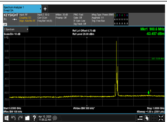
Band12-5MHz-16QAM-23035-1RB#0-30~1000-PASS
