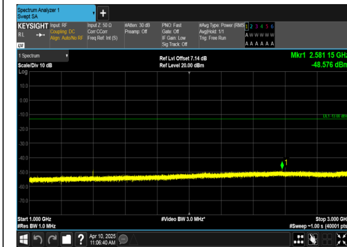
Band12-5MHz-16QAM-23035-1RB#0-1000~3000-PASS
