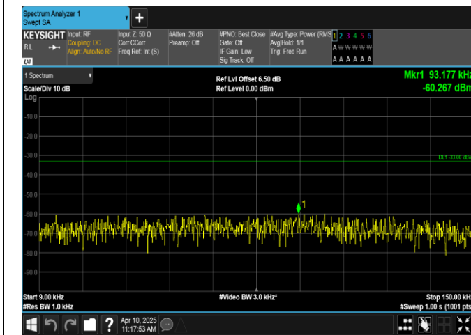
Band12-5MHz-QPSK-23155-1RB#0-0.009~0.15-PASS
