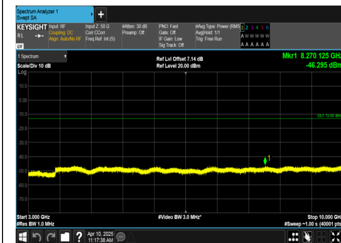
Band12-5MHz-16QAM-23095-25RB#0-3000~10000-PASS
