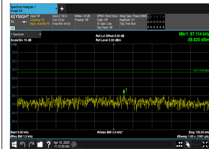
Band12-5MHz-16QAM-23095-1RB#0-0.009~0.15-PASS
