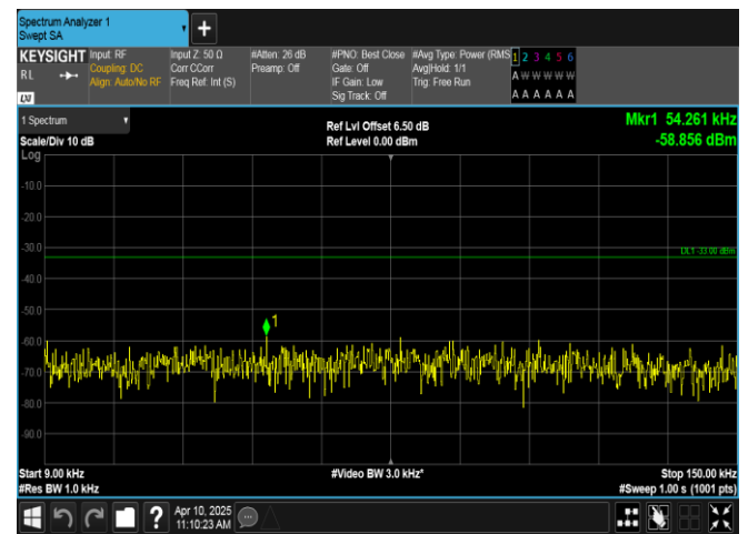
Band12-5MHz-16QAM-23035-25RB#0-0.009~0.15-PASS
