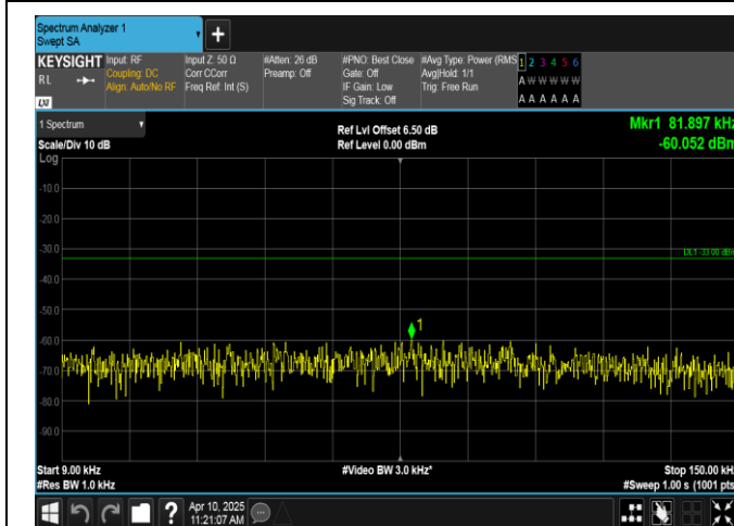
Band12-5MHz-16QAM-23155-1RB#24-0.009~0.15-PASS
