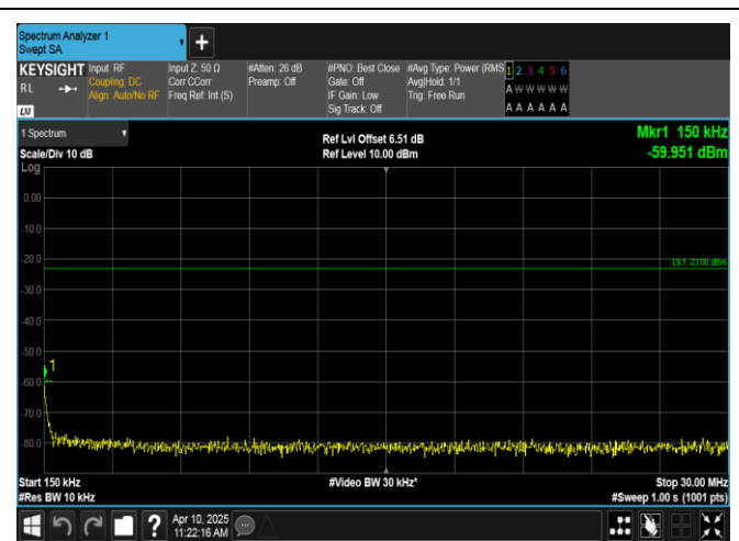
Band12-5MHz-QPSK-23155-25RB#0-0.15~30-PASS
