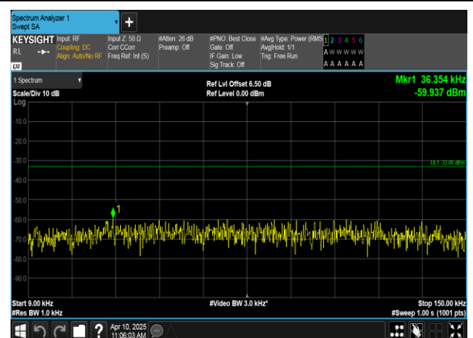
Band12-5MHz-16QAM-23035-1RB#0-0.009~0.15-PASS
