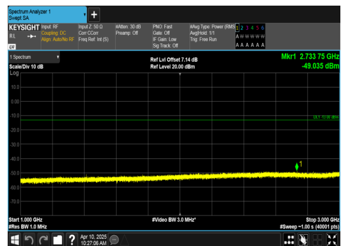
Band12-3MHz-16QAM-23095-1RB#0-1000-3000-PASS
