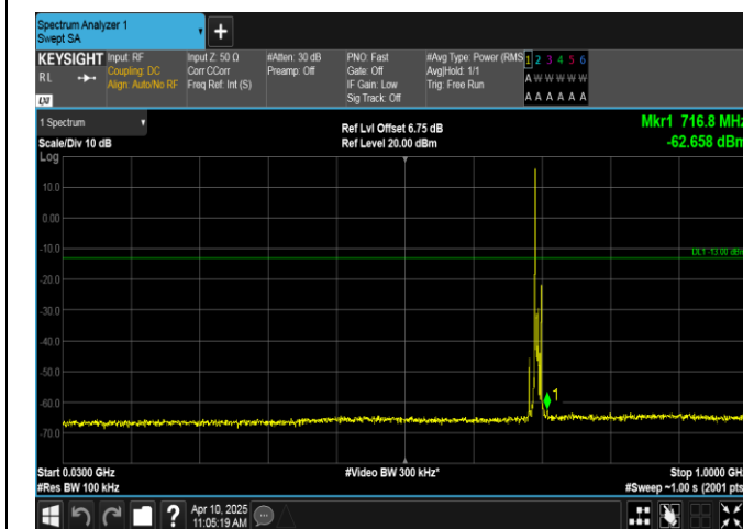
Band12-5MHz-QPSK-23035-1RB#0-30-1000-PASS
