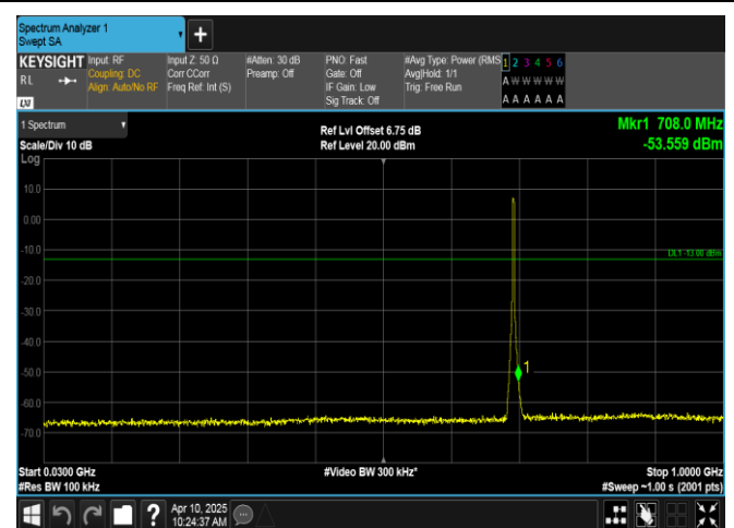
Band12-3MHz-16QAM-23025-15RB#0-30~1000-PASS
