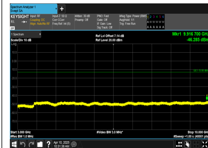
Band12-3MHz-16QAM-23095-15RB#0-3000~10000-PASS
