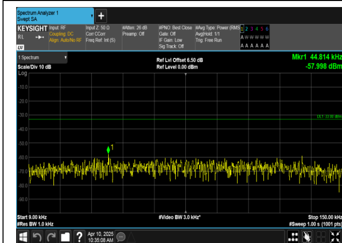
Band12-3MHz-16QAM-23165-1RB#14-0.009~0.15-PASS
