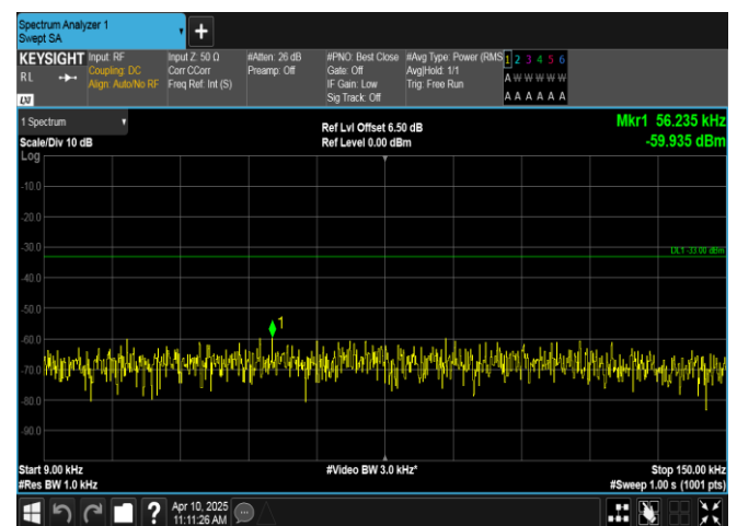
Band12-5MHz-QPSK-23095-1RB#0-0.009~0.15-PASS
