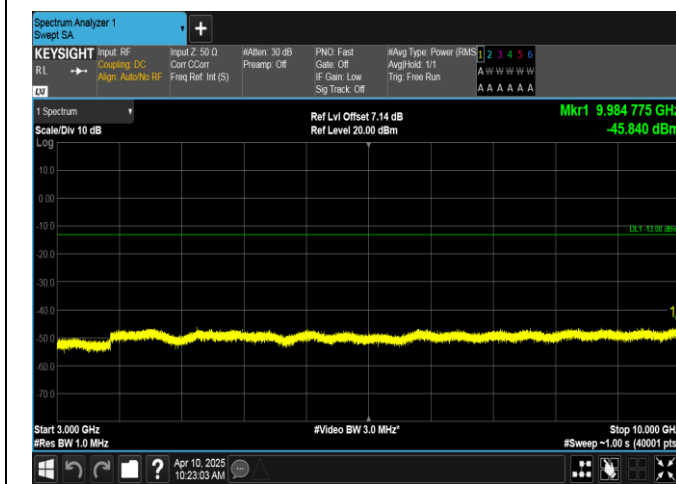
Band12-3MHz-16QAM-23025-1RB#14-3000~10000-PASS
