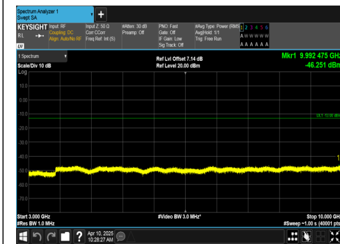
Band12-3MHz-QPSK-23095-1RB#14-3000~10000-PASS
