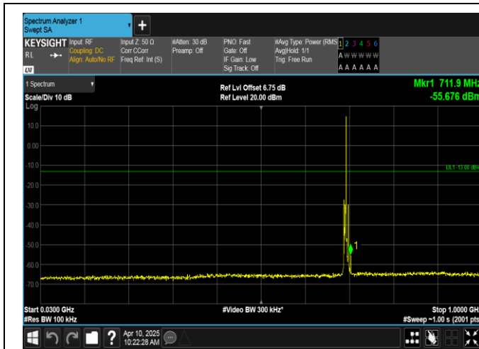
Band12-3MHz-16QAM-23025-1RB#14-30~1000-PASS
