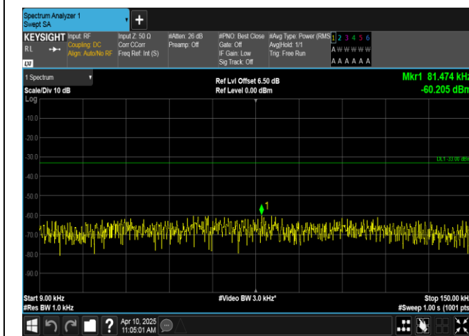
Band12-5MHz-QPSK-23035-1RB#0-0.009-0.15-PASS
