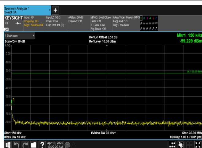
Band12-3MHz-16QAM-23025-1RB#14-0.15~30-PASS
