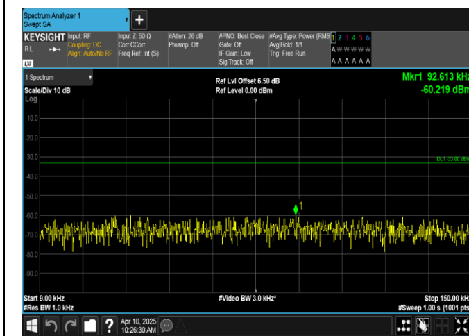
Band12-3MHz-16QAM-23095-1RB#0-0.009-0.15-PASS
