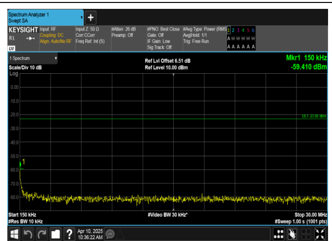
Band12-3MHz-QPSK-23165-15RB#0-0.15~30-PASS
