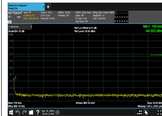
Band12-3MHz-QPSK-23165-1RB#14-0.15~30-PASS
