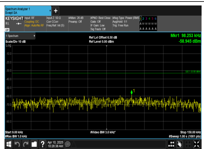
Band12-3MHz-16QAM-23095-1RB#14-0.009~0.15-PASS
