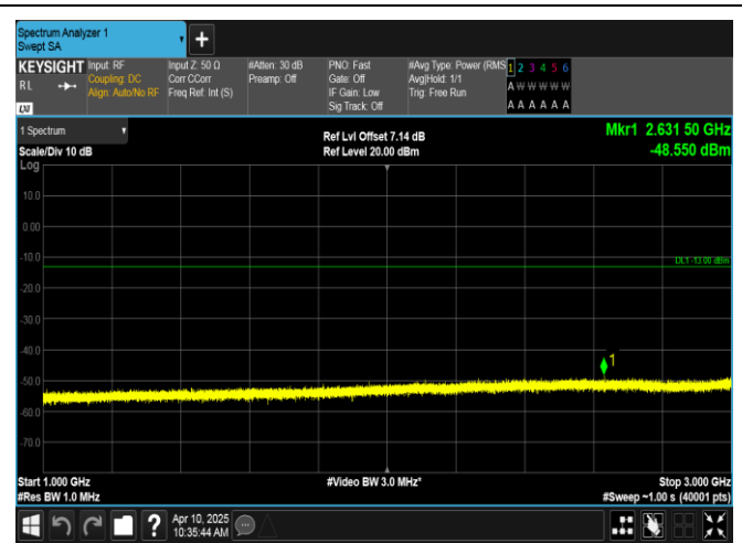
Band12-3MHz-16QAM-23165-1RB#14-1000~3000-PASS
