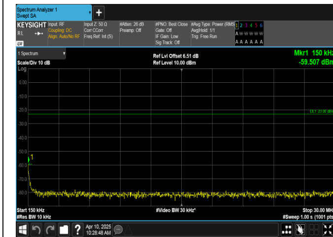
Band12-3MHz-16QAM-23095-1RB#14-0.15~30-PASS
