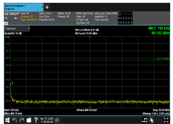
Band12-5MHz-QPSK-23035-1RB#0-0.15-30-PASS
