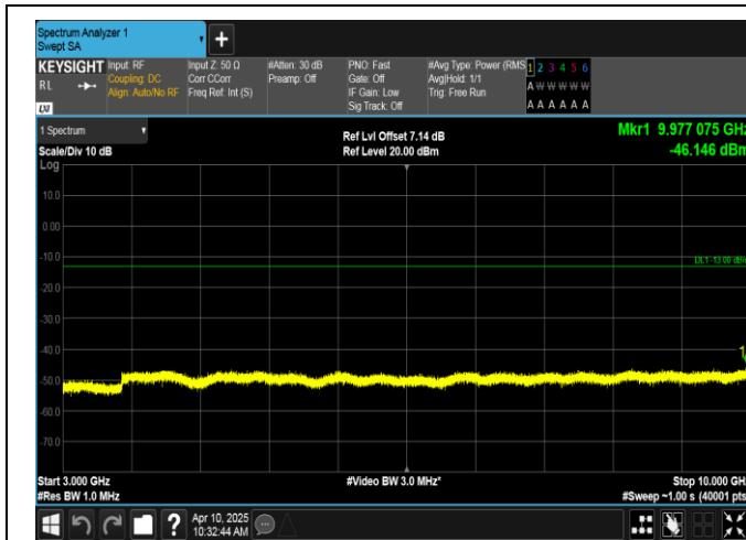
Band12-3MHz-QPSK-23165-1RB#0-3000~10000-PASS
