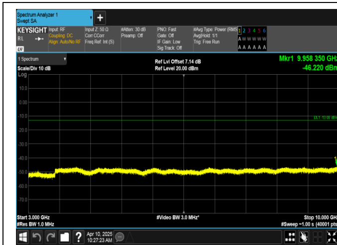
Band12-3MHz-16QAM-23095-1RB#0-3000~10000-PASS
