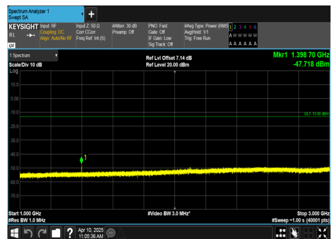
Band12-5MHz-QPSK-23035-1RB#0-1000-3000-PASS
