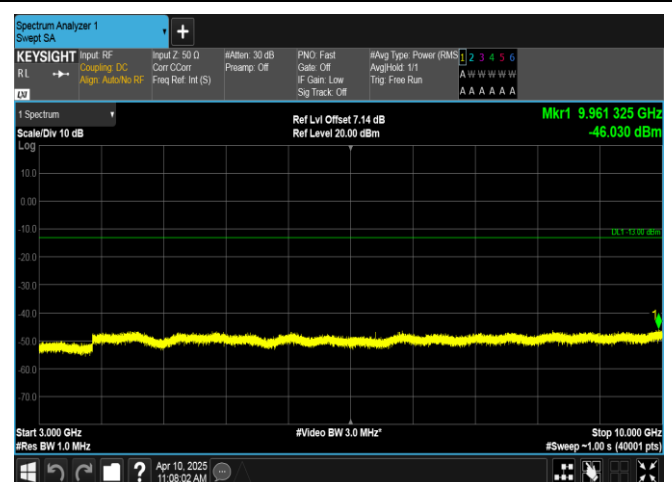
Band12-5MHz-QPSK-23035-1RB#24-3000~10000-PASS
