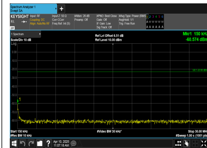
Band12-5MHz-QPSK-23035-1RB#24-0.15~30-PASS
