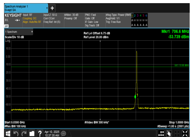
Band12-3MHz-16QAM-23165-15RB#0-30~1000-PASS
