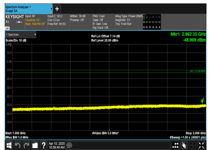
Band12-3MHz-QPSK-23165-15RB#0-1000~3000-PASS
