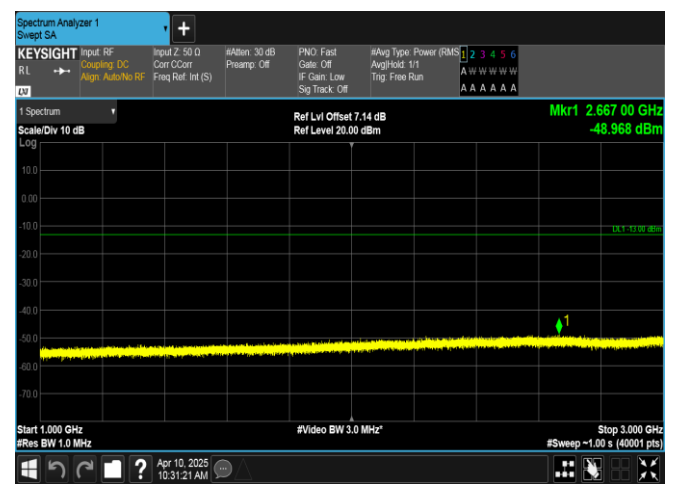
Band12-3MHz-16QAM-23095-15RB#0-1000~3000-PASS
