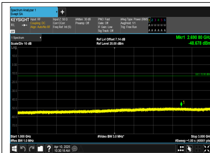
Band12-3MHz-QPSK-23095-15RB#0-1000~3000-PASS
