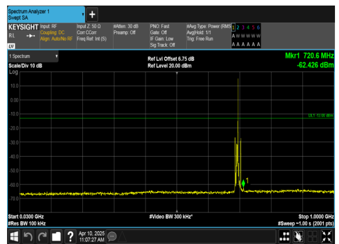
Band12-5MHz-QPSK-23035-1RB#24-30~1000-PASS
