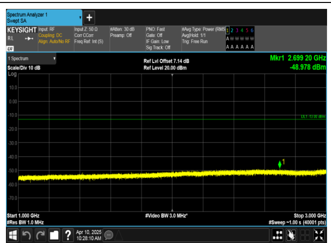
Band12-3MHz-QPSK-23095-1RB#14-1000~3000-PASS
