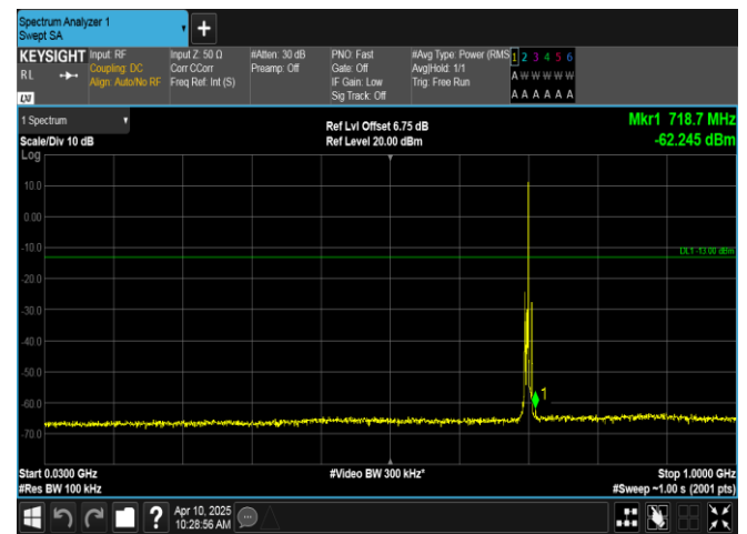
Band12-3MHz-16QAM-23095-1RB#14-30~1000-PASS
