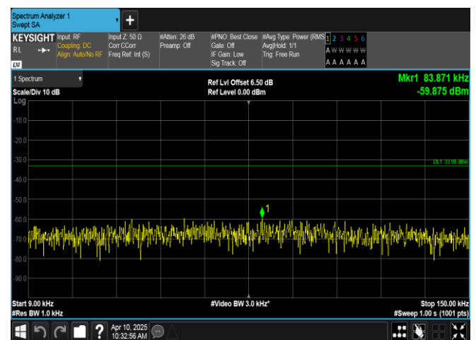
Band12-3MHz-16QAM-23165-1RB#0-0.009~0.15-PASS
