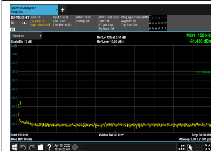
Band12-3MHz-16QAM-23025-15RB#0-0.15~30-PASS
