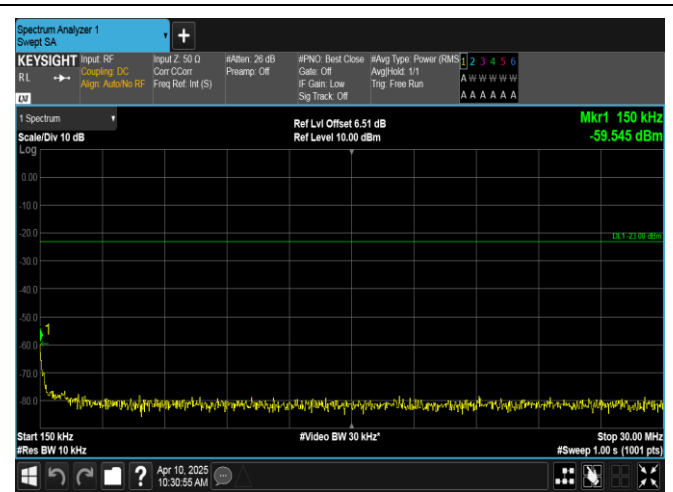
Band12-3MHz-16QAM-23095-15RB#0-0.15~30-PASS
