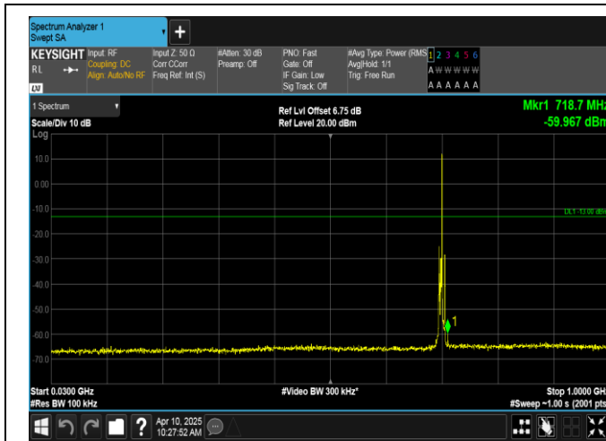
Band12-3MHz-QPSK-23095-1RB#14-30~1000-PASS
