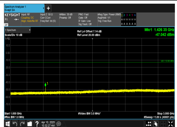
Band12-3MHz-QPSK-23165-1RB#0-1000~3000-PASS
