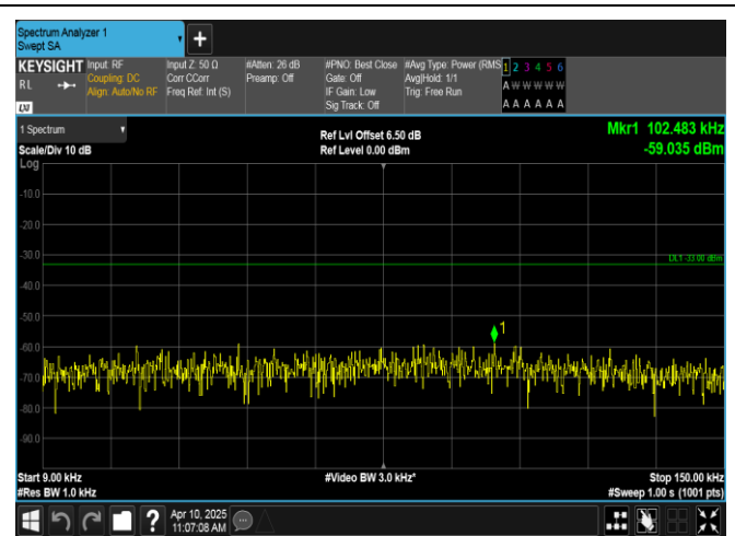
Band12-5MHz-QPSK-23035-1RB#24-0.009~0.15-PASS
