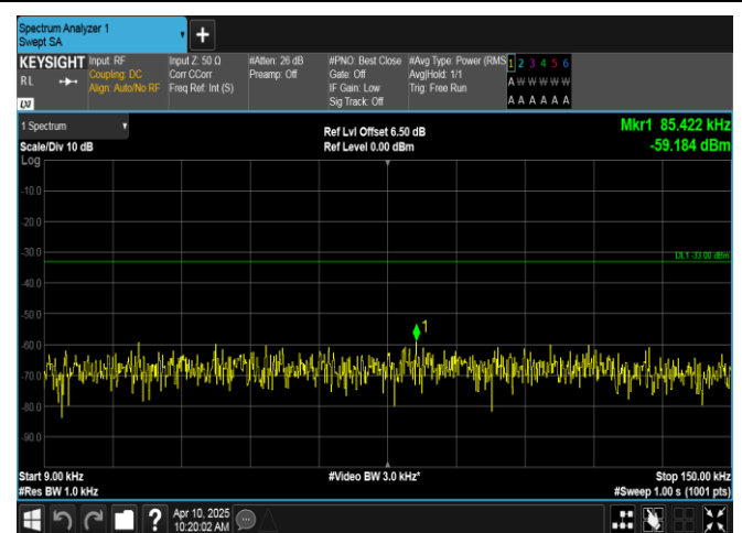
Band12-3MHz-16QAM-23025-1RB#0-0.009~0.15-PASS
