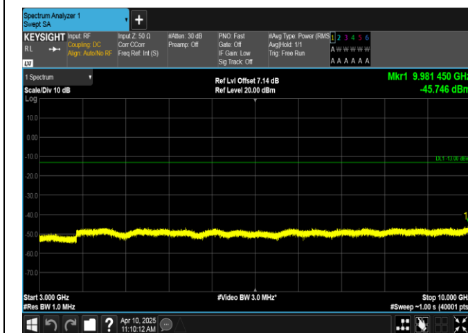
Band12-5MHz-QPSK-23035-25RB#0-3000~10000-PASS
