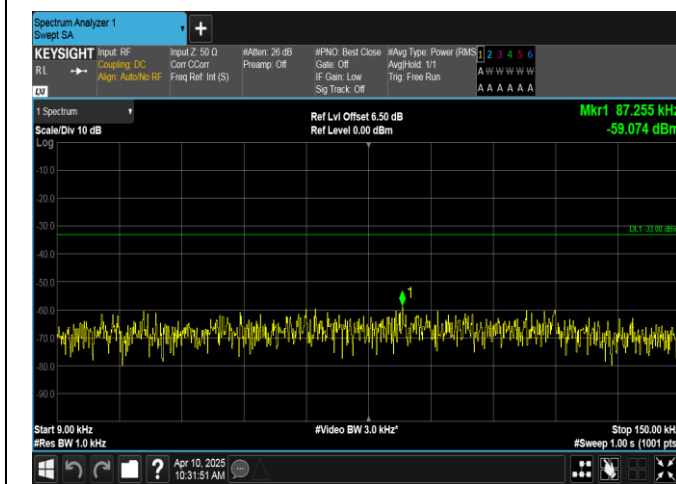
Band12-3MHz-QPSK-23165-1RB#0-0.009~0.15-PASS
