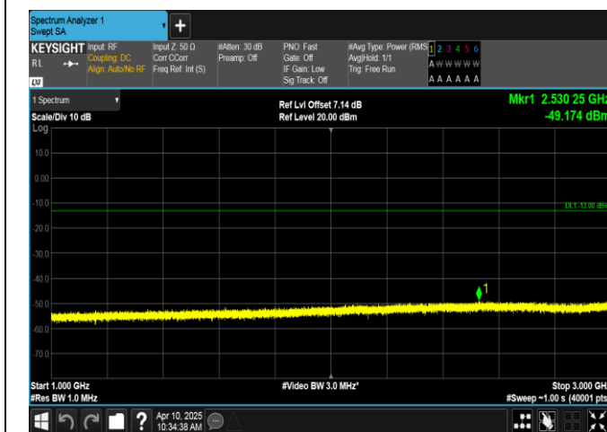
Band12-3MHz-QPSK-23165-1RB#14-1000~3000-PASS
