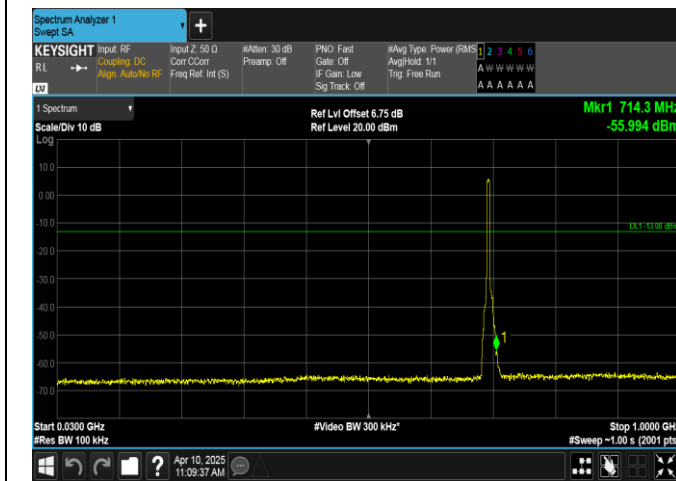
Band12-5MHz-QPSK-23035-25RB#0-30~1000-PASS
