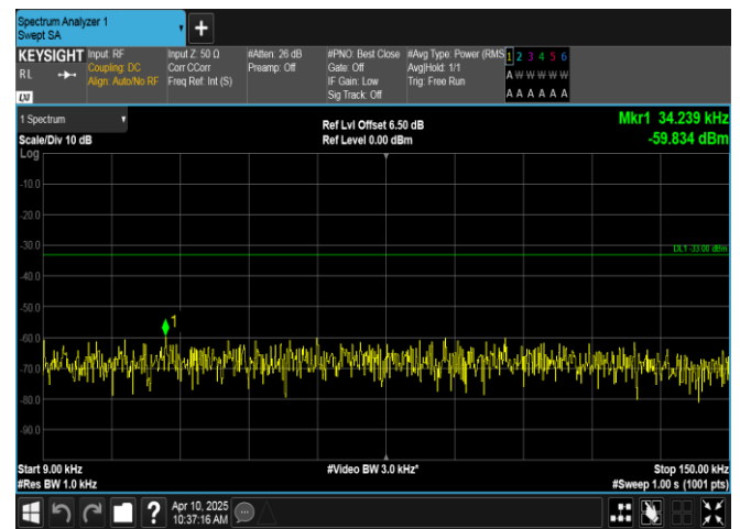
Band12-3MHz-16QAM-23165-15RB#0-0.009~0.15-PASS
