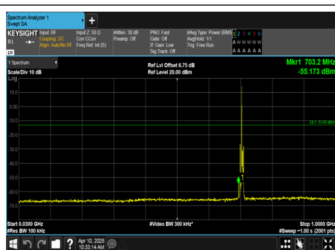
Band12-3MHz-16QAM-23165-1RB#0-30~1000-PASS
