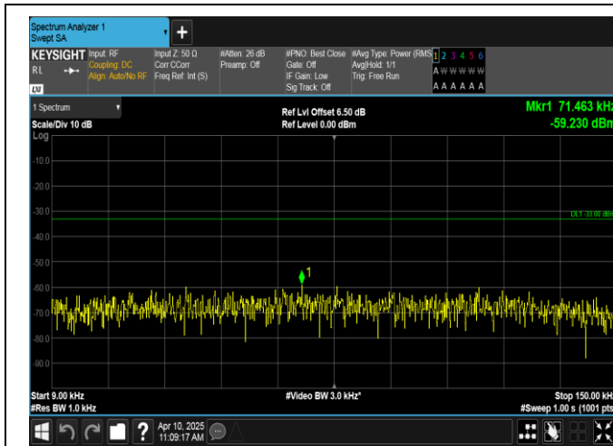
Band12-5MHz-QPSK-23035-25RB#0-0.009~0.15-PASS
