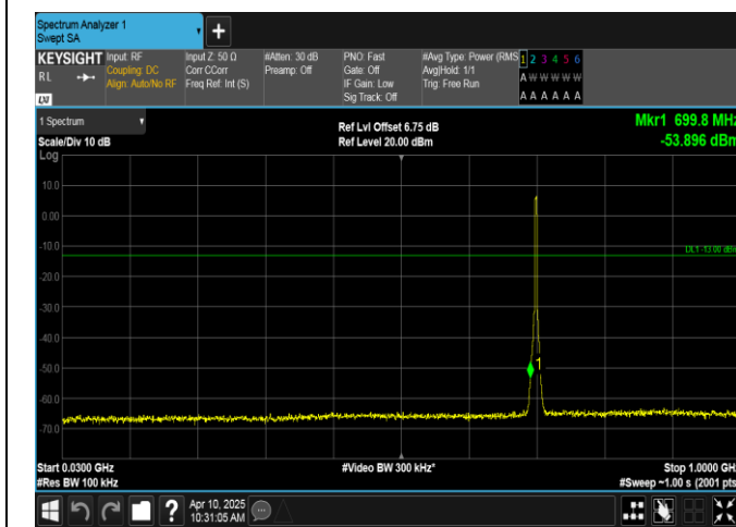
Band12-3MHz-16QAM-23095-15RB#0-30~1000-PASS
