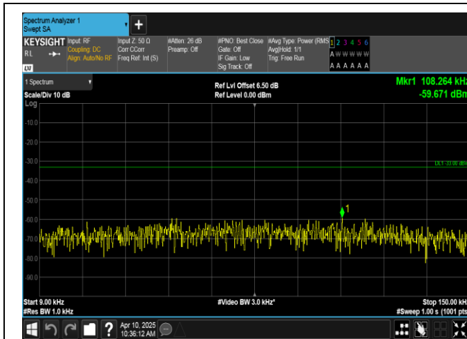
Band12-3MHz-QPSK-23165-15RB#0-0.009~0.15-PASS
