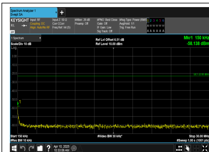
Band12-3MHz-16QAM-23165-1RB#0-0.15~30-PASS
