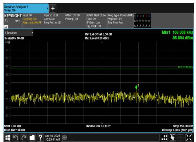
Band12-3MHz-QPSK-23095-15RB#0-0.009~0.15-PASS
