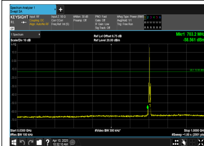
Band12-3MHz-QPSK-23165-1RB#0-30~1000-PASS
