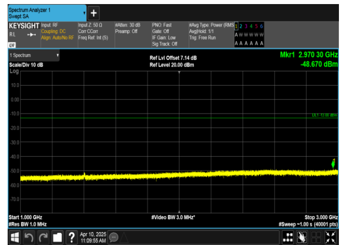
Band12-5MHz-QPSK-23035-25RB#0-1000~3000-PASS
