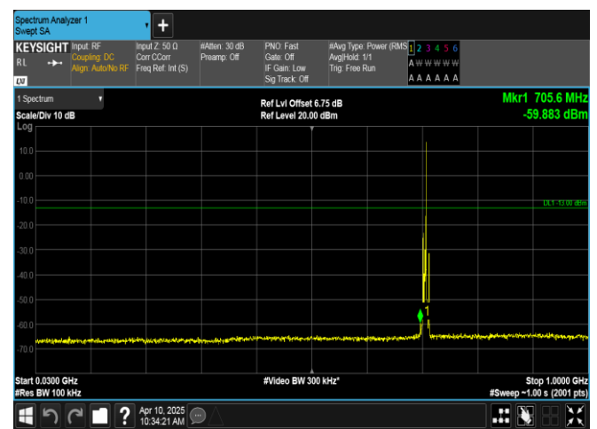
Band12-3MHz-QPSK-23165-1RB#14-30~1000-PASS
