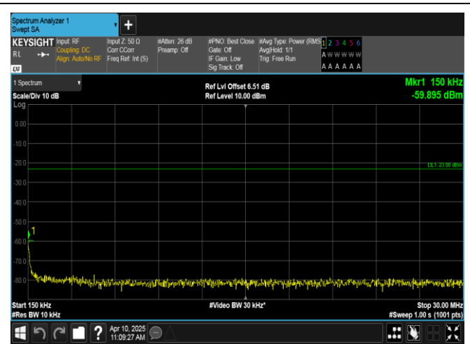
Band12-5MHz-QPSK-23035-25RB#0-0.15~30-PASS
