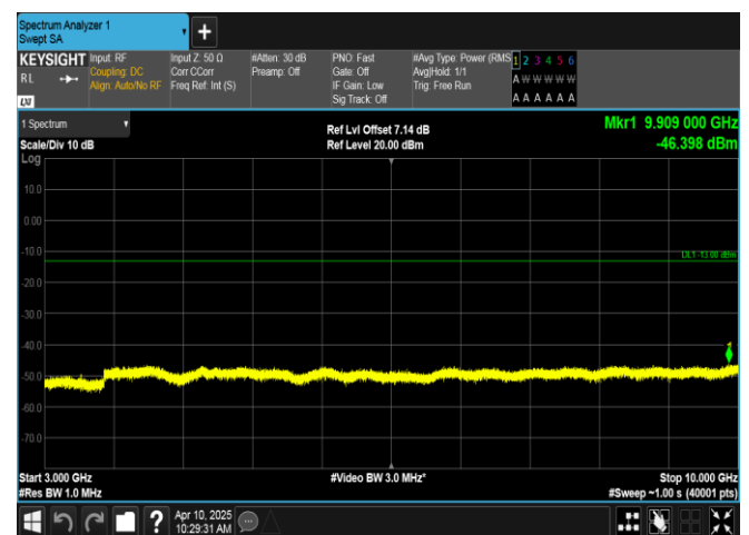
Band12-3MHz-16QAM-23095-1RB#14-3000~10000-PASS
