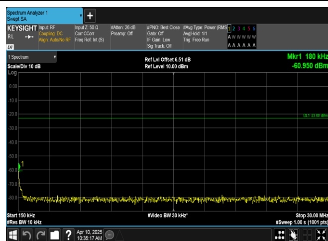
Band12-3MHz-16QAM-23165-1RB#14-0.15~30-PASS
