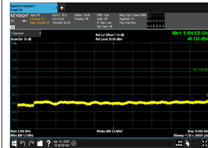
Band12-3MHz-16QAM-23165-1RB#14-3000~10000-PASS
