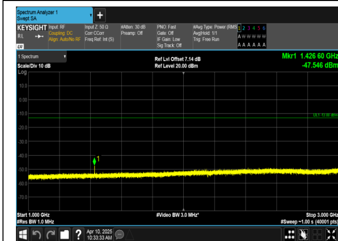
Band12-3MHz-16QAM-23165-1RB#0-1000~3000-PASS
