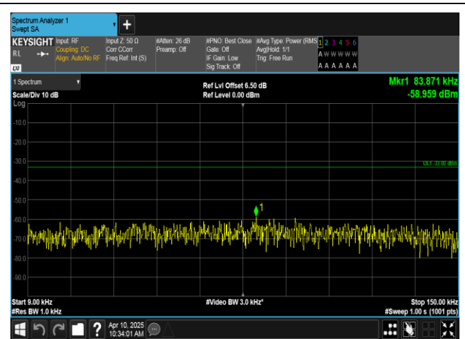
Band12-3MHz-QPSK-23165-1RB#14-0.009~0.15-PASS
