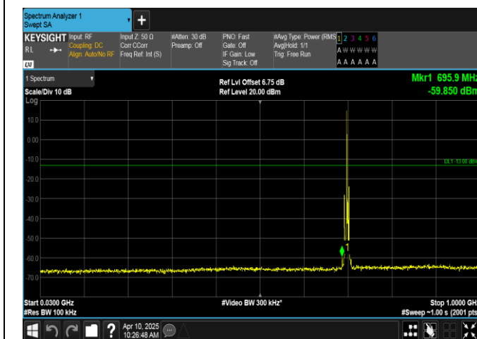
Band12-3MHz-16QAM-23095-1RB#0-30-1000-PASS
