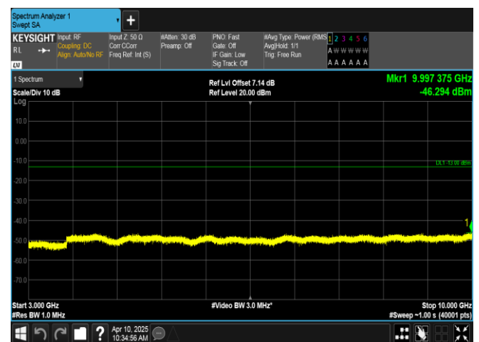
Band12-3MHz-QPSK-23165-1RB#14-3000~10000-PASS
