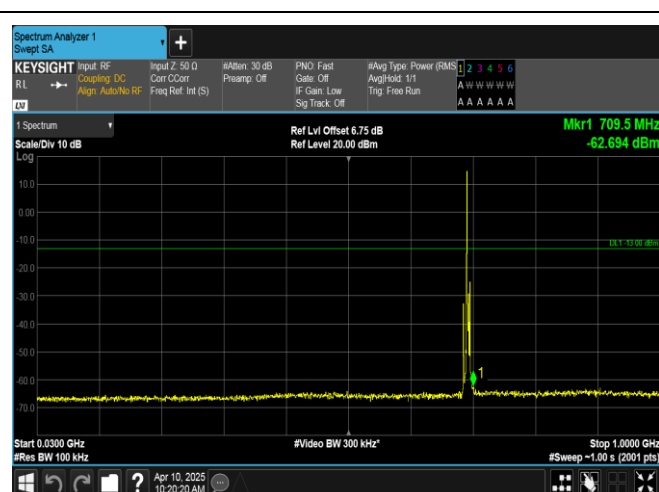
Band12-3MHz-16QAM-23025-1RB#0-30~1000-PASS
