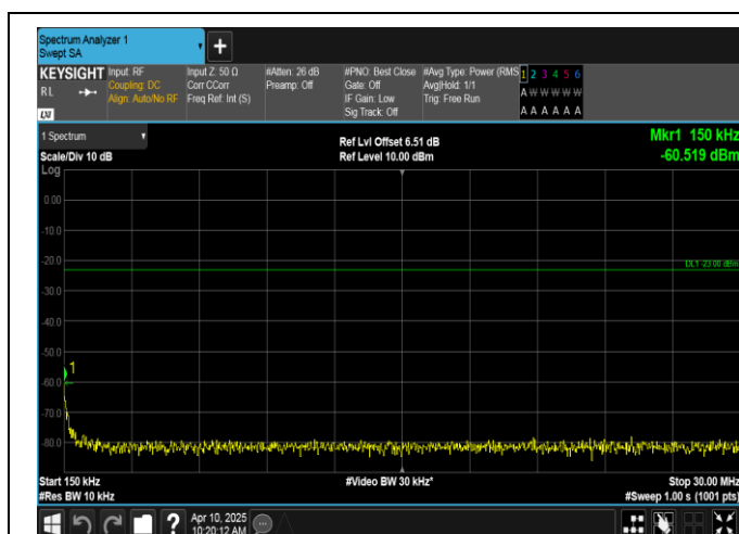
Band12-3MHz-16QAM-23025-1RB#0-0.15~30-PASS
