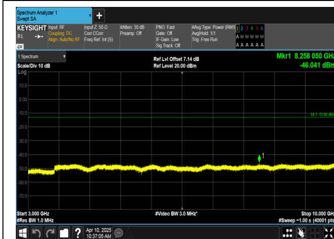
Band12-3MHz-QPSK-23165-15RB#0-3000~10000-PASS
