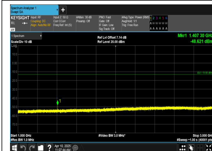
Band12-5MHz-QPSK-23035-1RB#24-1000~3000-PASS
