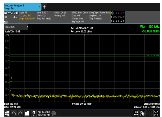
Band12-3MHz-QPSK-23165-1RB#0-0.15~30-PASS
