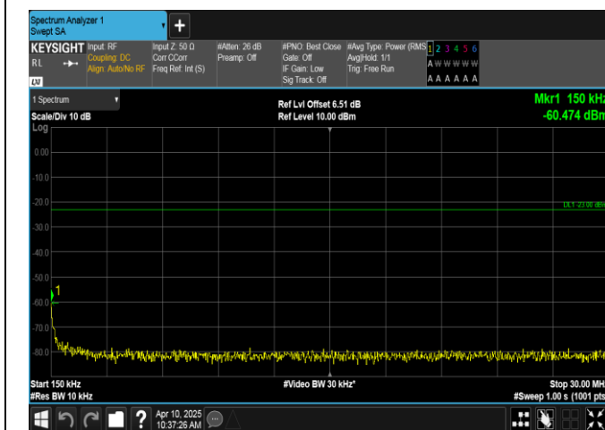
Band12-3MHz-16QAM-23165-15RB#0-0.15~30-PASS
