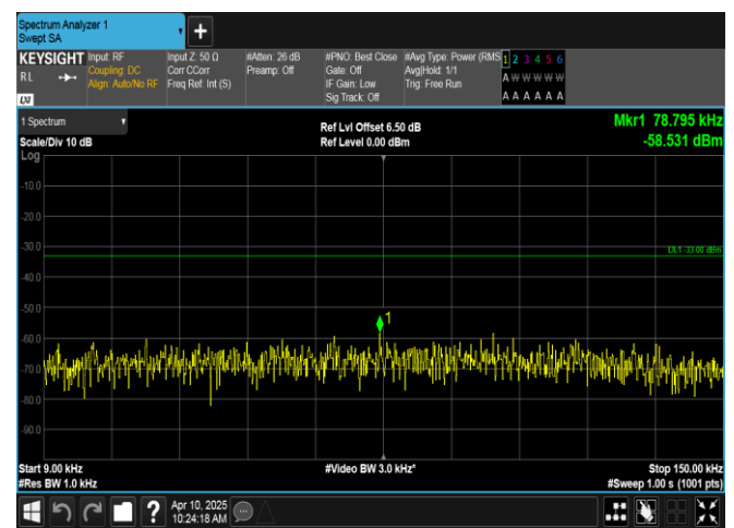
Band12-3MHz-16QAM-23025-15RB#0-0.009~0.15-PASS
