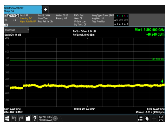
Band12-3MHz-QPSK-23095-15RB#0-3000~10000-PASS
