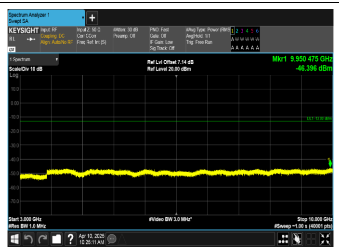
Band12-3MHz-16QAM-23025-15RB#0-3000-10000-PASS
