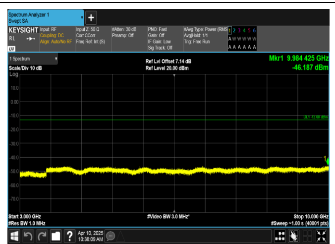
Band12-3MHz-16QAM-23165-15RB#0-3000-10000-PASS
