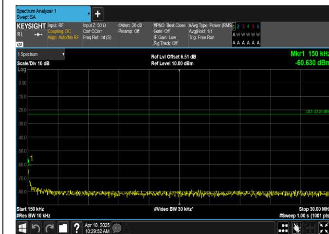
Band12-3MHz-QPSK-23095-15RB#0-0.15~30-PASS
