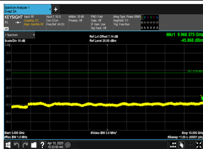
Band12-3MHz-16QAM-23165-1RB#0-3000~10000-PASS
