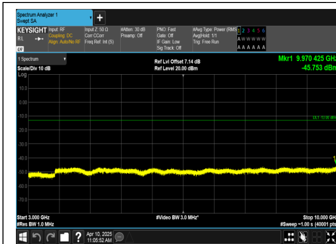
Band12-5MHz-QPSK-23035-1RB#0-3000~10000-PASS
