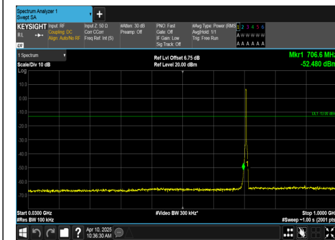
Band12-3MHz-QPSK-23165-15RB#0-30~1000-PASS
