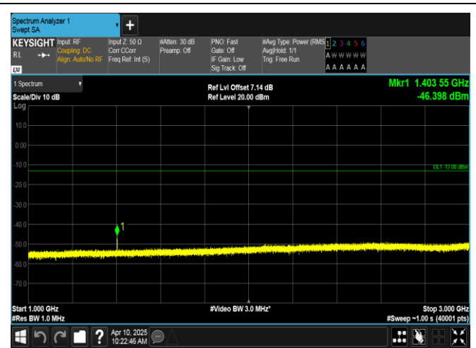
Band12-3MHz-16QAM-23025-1RB#14-1000~3000-PASS
