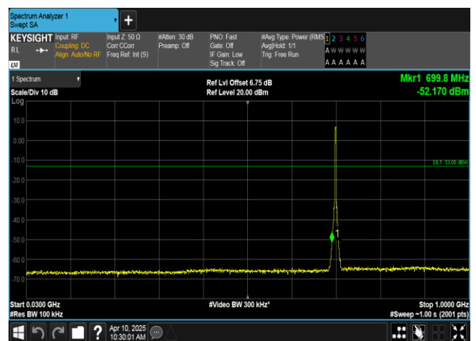
Band12-3MHz-QPSK-23095-15RB#0-30~1000-PASS
