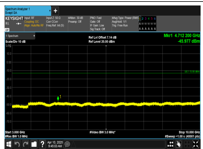
Band12-1.4MHz-QPSK-23095-6RB#0-3000~10000-PASS
