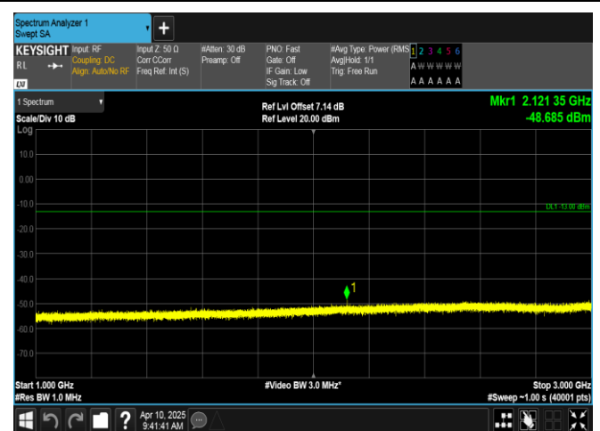
Band12-1.4MHz-16QAM-23095-1RB#0-1000~3000-PASS
