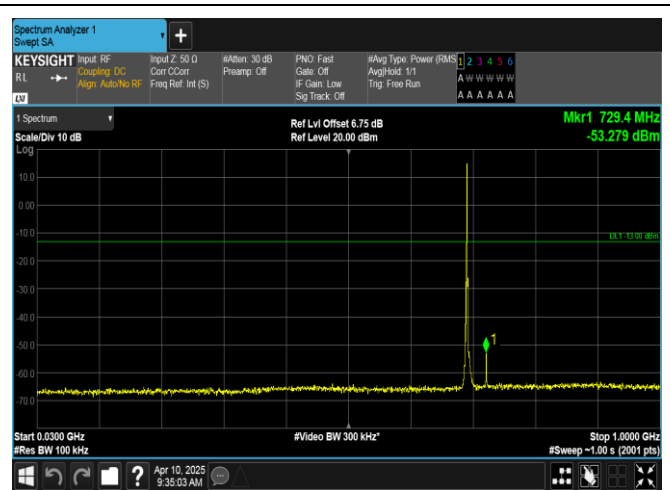
Band12-1.4MHz-16QAM-23017-1RB#0-30~1000-PASS
