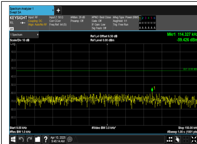
Band12-1.4MHz-16QAM-23095-6RB#0-0.009~0.15-PASS
