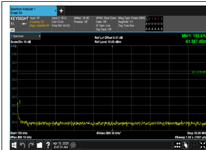
Band12-1.4MHz-16QAM-23173-1RB#0-0.15~30-PASS
