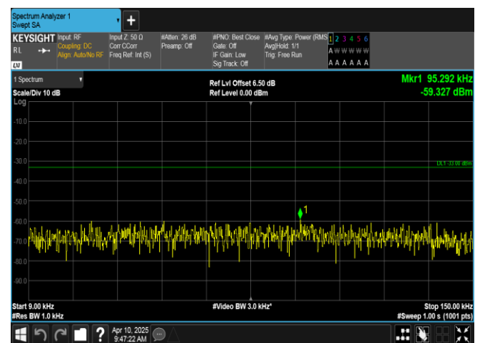
Band12-1.4MHz-16QAM-23173-1RB#0-0.009~0.15-PASS
