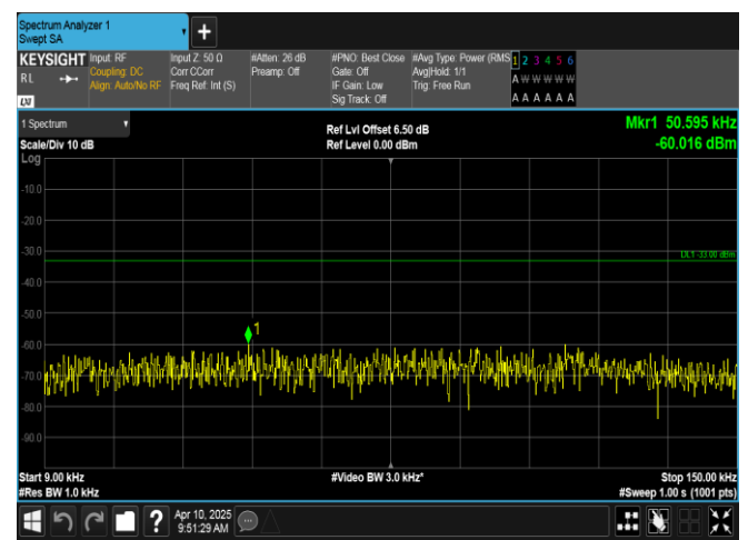
Band12-1.4MHz-16QAM-23173-6RB#0-0.009~0.15-PASS
