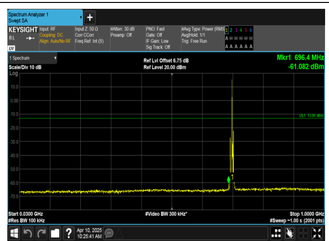
Band12-3MHz-QPSK-23095-1RB#0-30~1000-PASS
