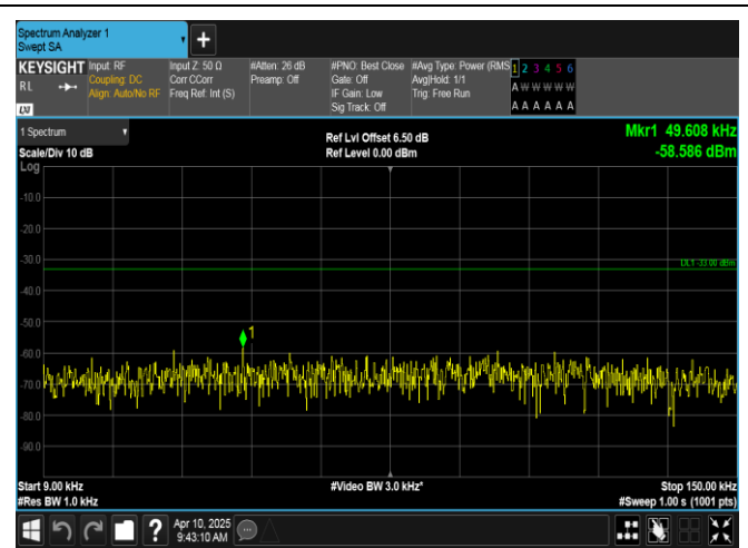
Band12-1.4MHz-16QAM-23095-1RB#5-0.009~0.15-PASS
