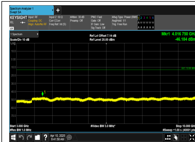
Band12-1.4MHz-16QAM-23095-1RB#0-3000~10000-PASS
