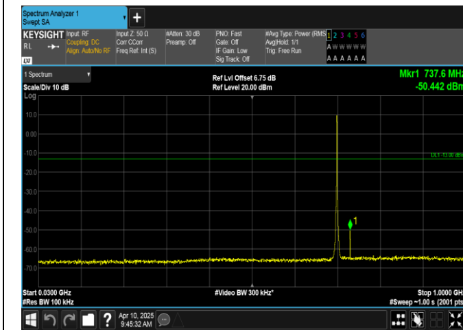
Band12-1.4MHz-16QAM-23095-6RB#0-30~1000-PASS
