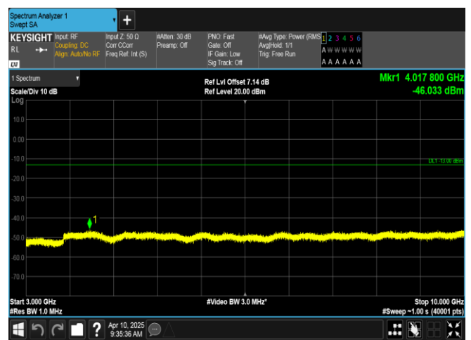
Band12-1.4MHz-16QAM-23017-1RB#0-3000~10000-PASS
