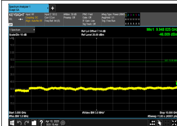
Band12-1.4MHz-QPSK-23173-6RB#0-3000~10000-PASS
