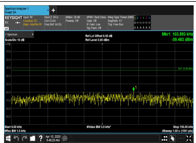
Band12-1.4MHz-QPSK-23173-1RB#5-0.009~0.15-PASS
