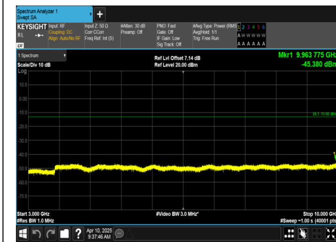
Band12-1.4MHz-16QAM-23017-1RB#5-3000-10000-PASS
