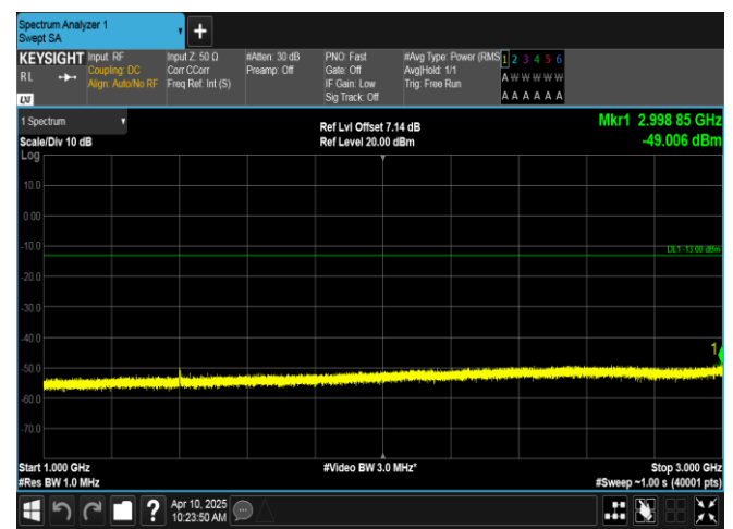
Band12-3MHz-QPSK-23025-15RB#0-1000~3000-PASS
