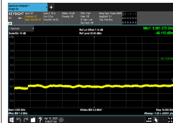
Band12-1.4MHz-16QAM-23095-6RB#0-3000~10000-PASS
