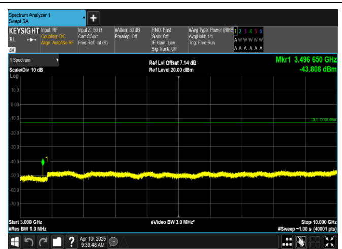
Band12-1.4MHz-16QAM-23017-6RB#0-3000~10000-PASS
