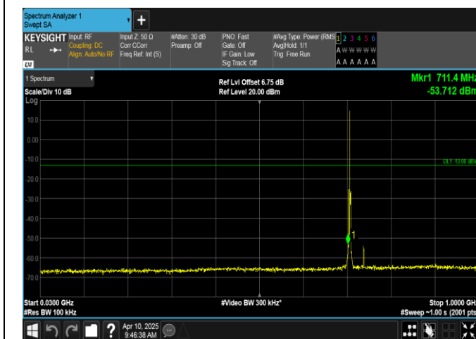
Band12-1.4MHz-QPSK-23173-1RB#0-30~1000-PASS
