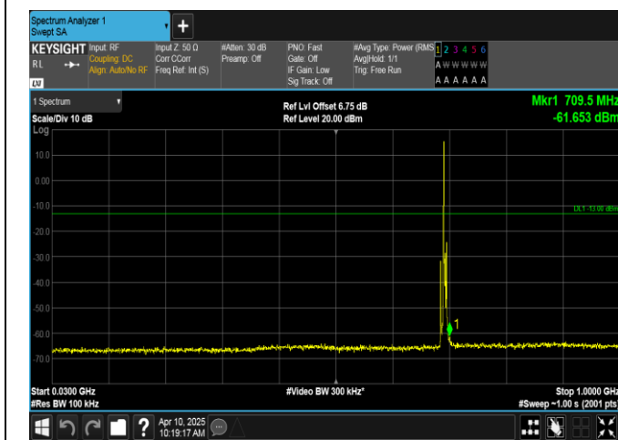
Band12-3MHz-QPSK-23025-1RB#0-30~1000-PASS
