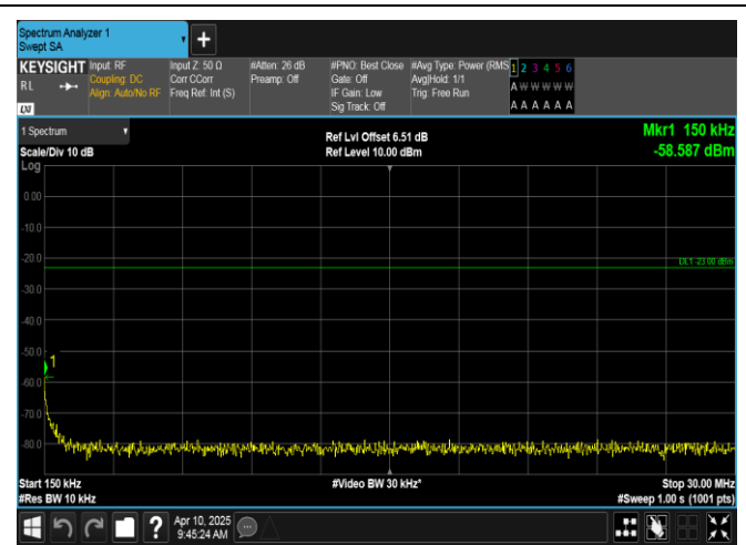
Band12-1.4MHz-16QAM-23095-6RB#0-0.15~30-PASS
