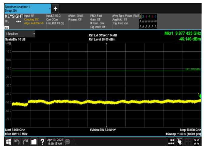
Band12-1.4MHz-QPSK-23173-1RB#5-3000~10000-PASS
