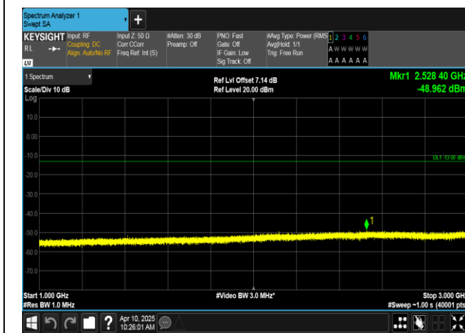
Band12-3MHz-QPSK-23095-1RB#0-1000~3000-PASS
