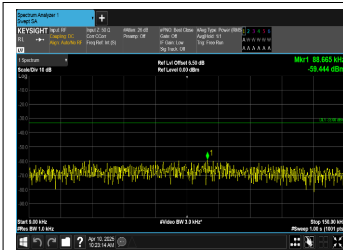
Band12-3MHz-QPSK-23025-15RB#0-0.009~0.15-PASS
