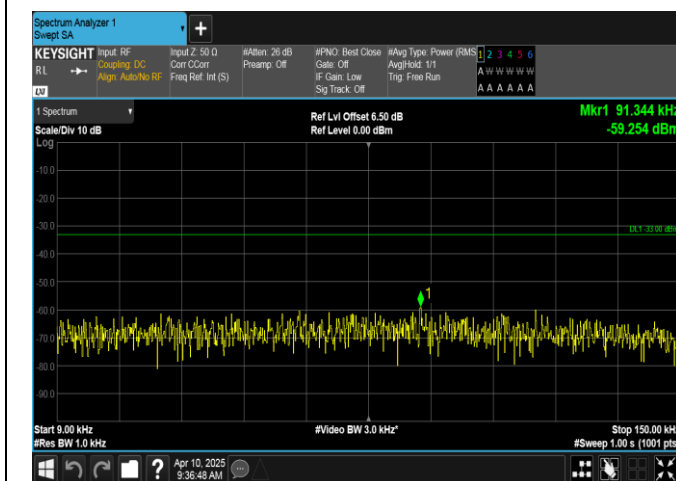
Band12-1.4MHz-16QAM-23017-1RB#5-0.009~0.15-PASS
