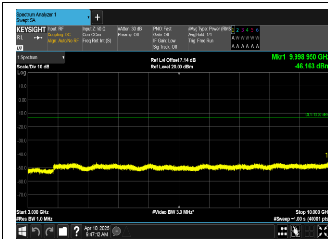
Band12-1.4MHz-QPSK-23173-1RB#0-3000~10000-PASS
