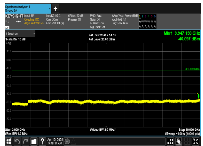
Band12-1.4MHz-16QAM-23173-1RB#0-3000~10000-PASS
