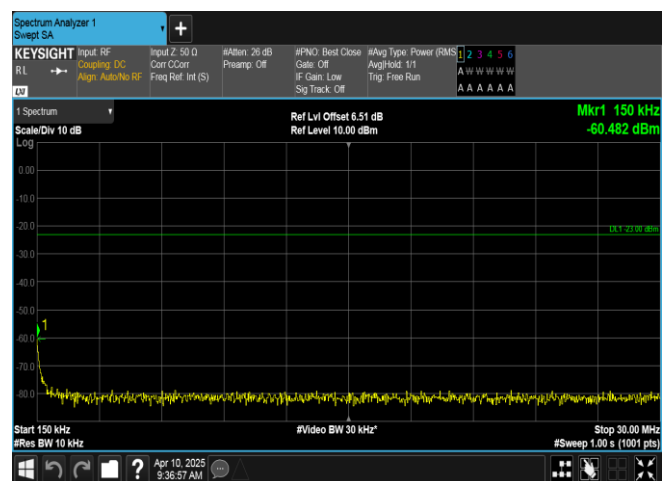
Band12-1.4MHz-16QAM-23017-1RB#5-0.15~30-PASS
