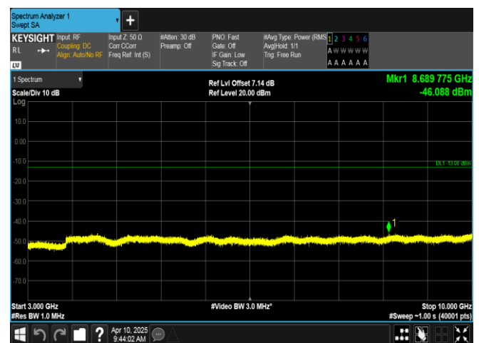
Band12-1.4MHz-16QAM-23095-1RB#5-3000~10000-PASS
