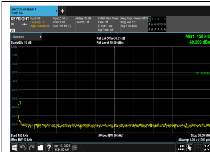
Band12-1.4MHz-16QAM-23017-1RB#0-0.15~30-PASS
