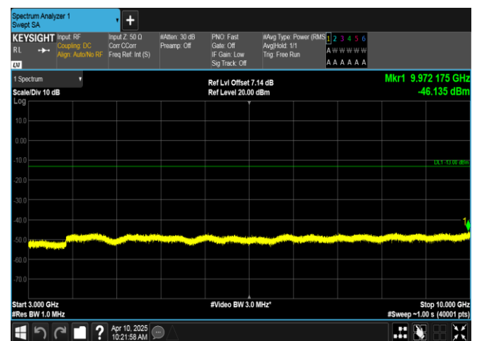
Band12-3MHz-QPSK-23025-1RB#14-3000~10000-PASS
