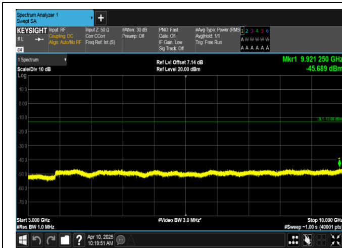
Band12-3MHz-QPSK-23025-1RB#0-3000~10000-PASS
