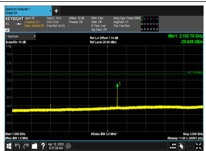
Band12-1.4MHz-16QAM-23017-1RB#5-1000-3000-PASS
