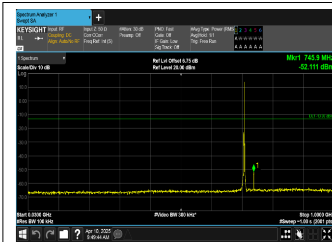
Band12-1.4MHz-16QAM-23173-1RB#5-30~1000-PASS
