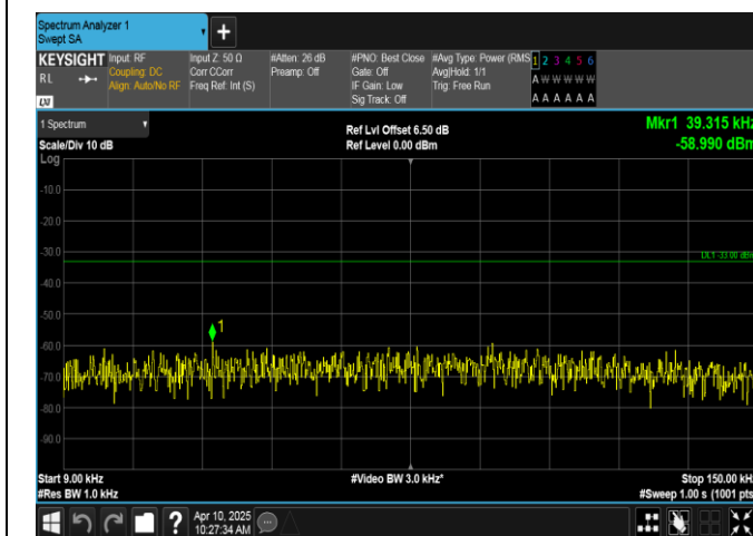
Band12-3MHz-QPSK-23095-1RB#14-0.009~0.15-PASS
