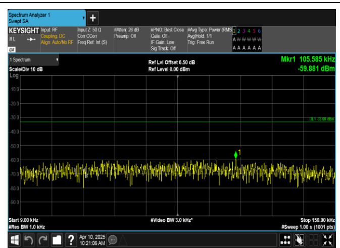
Band12-3MHz-QPSK-23025-1RB#14-0.009~0.15-PASS
