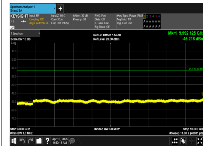
Band12-1.4MHz-16QAM-23173-1RB#5-3000~10000-PASS
