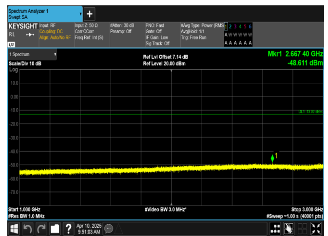
Band12-1.4MHz-QPSK-23173-6RB#0-1000~3000-PASS
