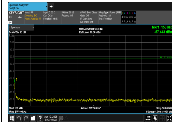
Band12-1.4MHz-16QAM-23095-1RB#5-0.15~30-PASS
