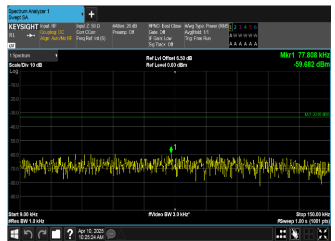
Band12-3MHz-QPSK-23095-1RB#0-0.009~0.15-PASS
