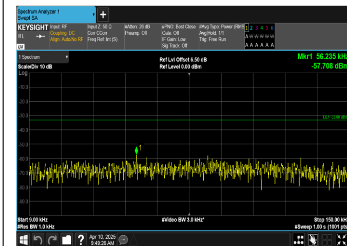
Band12-1.4MHz-16QAM-23173-1RB#5-0.009~0.15-PASS
