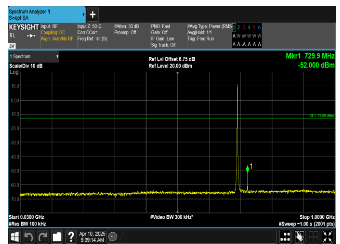
Band12-1.4MHz-16QAM-23017-6RB#0-0.30-1000-PASS
