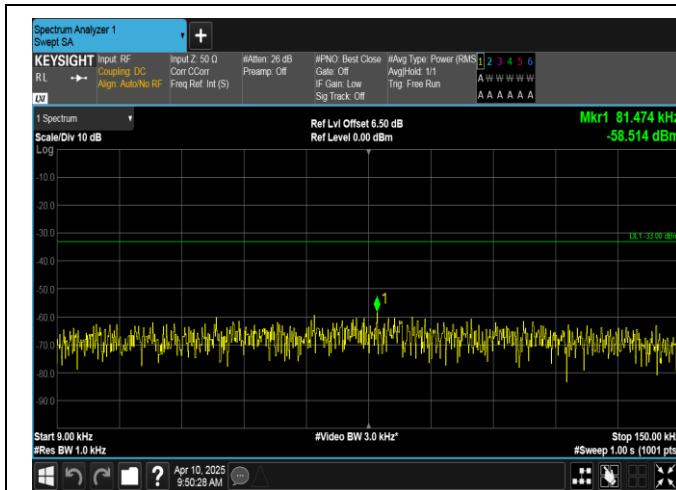
Band12-1.4MHz-QPSK-23173-6RB#0-0.009~0.15-PASS
