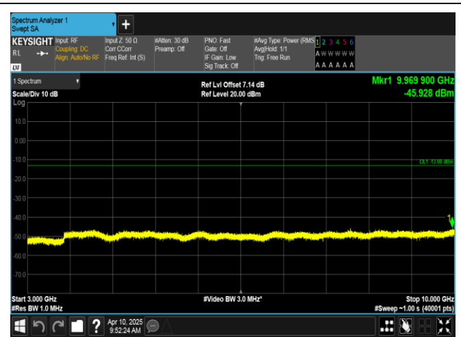
Band12-1.4MHz-16QAM-23173-6RB#0-3000~10000-PASS
