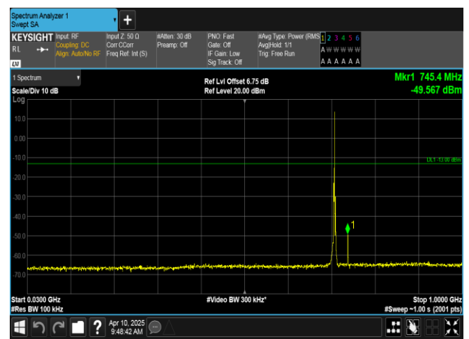
Band12-1.4MHz-QPSK-23173-1RB#5-30~1000-PASS
