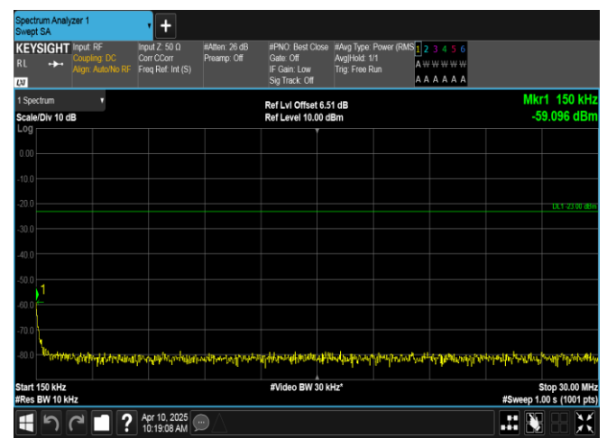
Band12-3MHz-QPSK-23025-1RB#0-0.15~30-PASS
