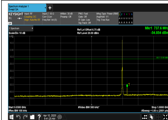
Band12-1.4MHz-16QAM-23095-1RB#0-30~1000-PASS
