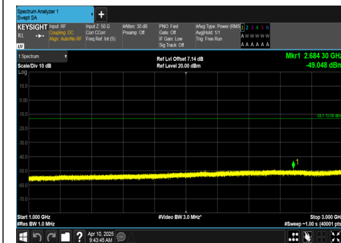
Band12-1.4MHz-16QAM-23095-1RB#5-1000~3000-PASS
