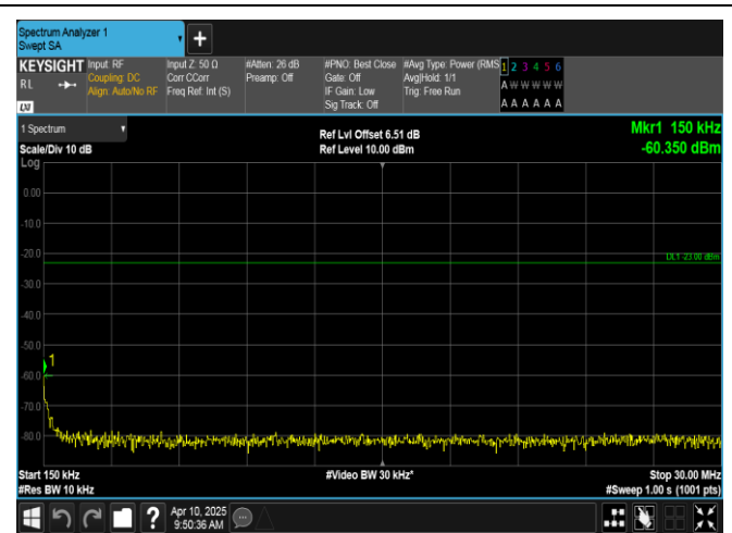
Band12-1.4MHz-QPSK-23173-6RB#0-0.15~30-PASS
