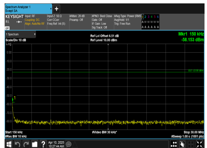
Band12-3MHz-QPSK-23095-1RB#14-0.15~30-PASS
