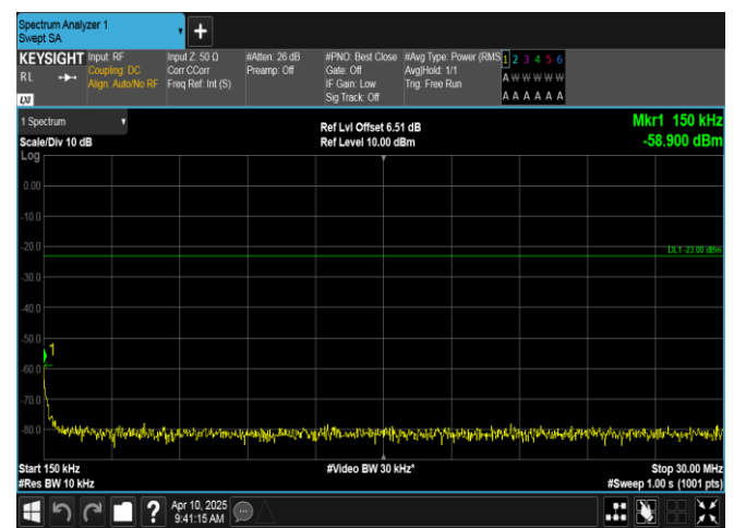
Band12-1.4MHz-16QAM-23095-1RB#0-0.15~30-PASS
