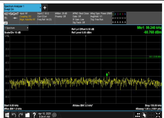
Band12-1.4MHz-16QAM-23017-1RB#0-0.009~0.15-PASS
