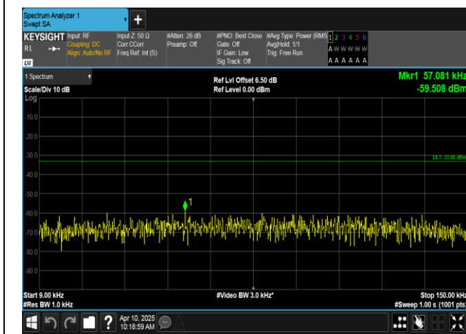
Band12-3MHz-QPSK-23025-1RB#0-0.009~0.15-PASS
