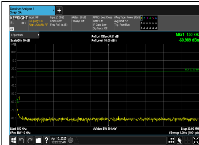
Band12-3MHz-QPSK-23095-1RB#0-0.15~30-PASS
