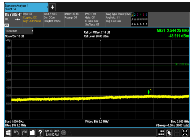
Band12-1.4MHz-16QAM-23095-6RB#0-1000~3000-PASS
