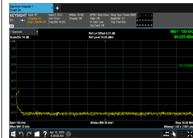
Band12-1.4MHz-16QAM-23017-6RB#0-0.15-30-PASS
