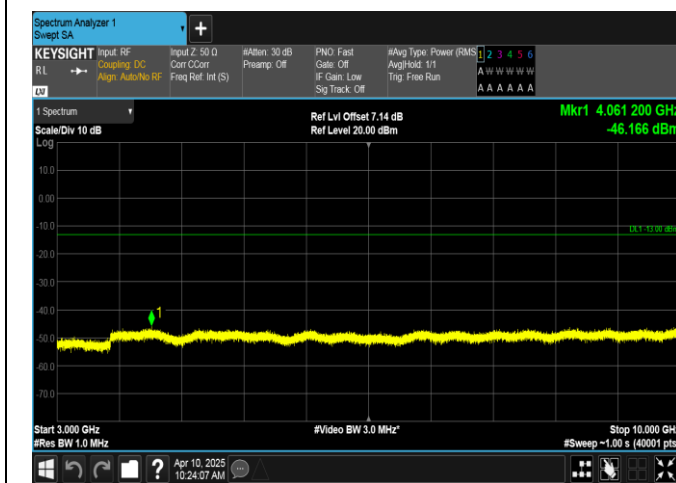
Band12-3MHz-QPSK-23025-15RB#0-3000~10000-PASS
