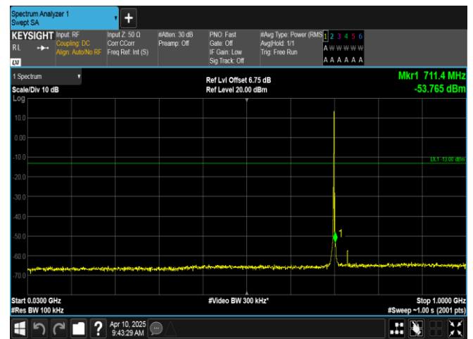
Band12-1.4MHz-16QAM-23095-1RB#5-30~1000-PASS
