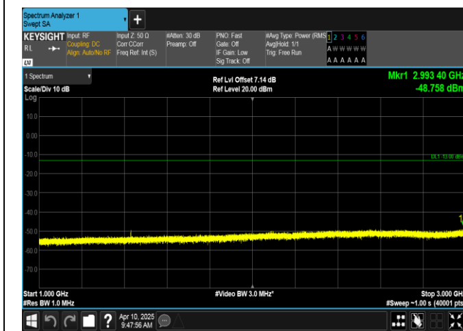
Band12-1.4MHz-16QAM-23173-1RB#0-1000~3000-PASS
