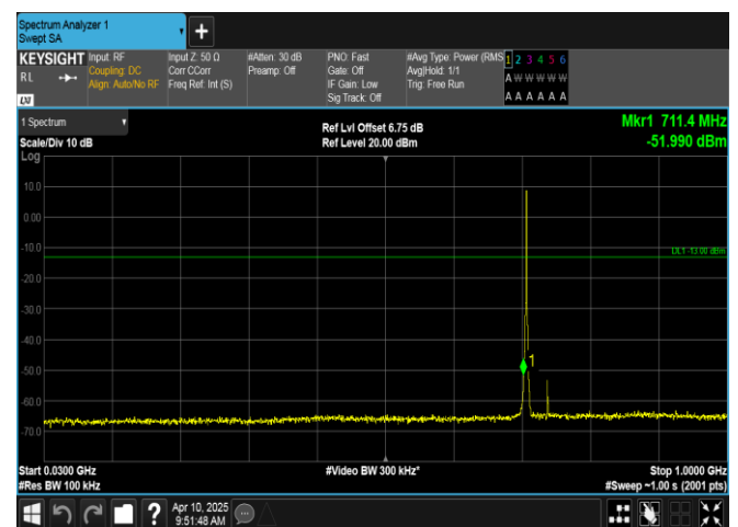
Band12-1.4MHz-16QAM-23173-6RB#0-30~1000-PASS
