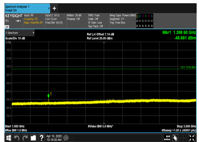
Band12-3MHz-QPSK-23025-1RB#0-1000~3000-PASS
