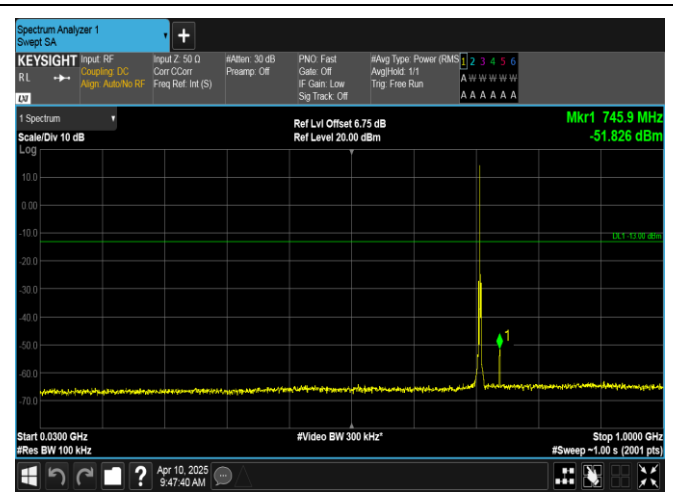
Band12-1.4MHz-16QAM-23173-1RB#0-30~1000-PASS
