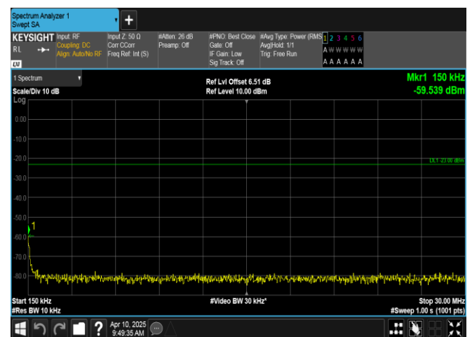
Band12-1.4MHz-16QAM-23173-1RB#5-0.15~30-PASS
