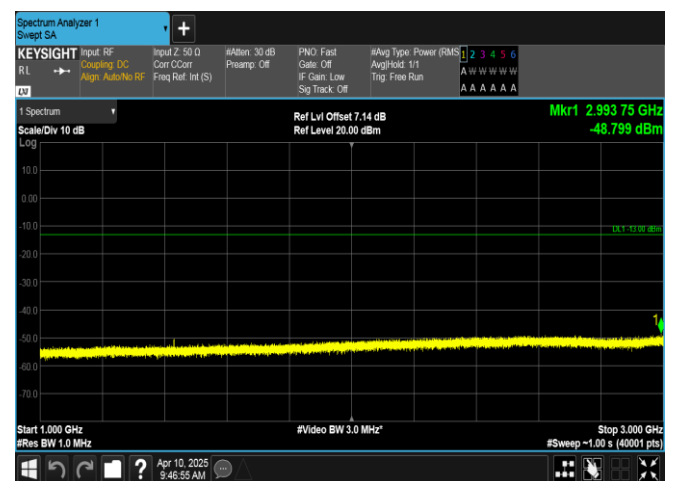
Band12-1.4MHz-QPSK-23173-1RB#0-1000~3000-PASS
