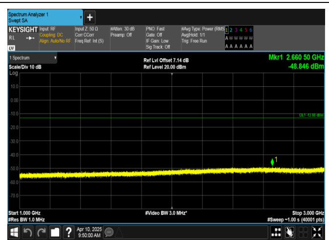
Band12-1.4MHz-16QAM-23173-1RB#5-1000~3000-PASS
