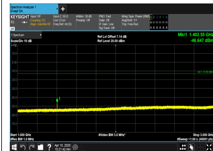
Band12-3MHz-QPSK-23025-1RB#14-1000~3000-PASS
