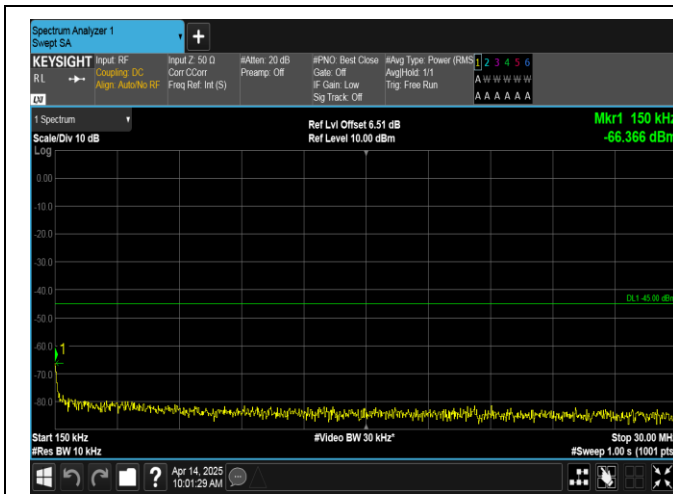
Band7-20MHz-16QAM-21350-100RB#0-0.15~30-PASS
