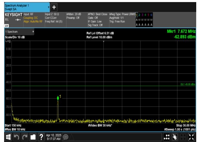
Band7-20MHz-16QAM-21350-1RB#99-0.15~30-PASS
