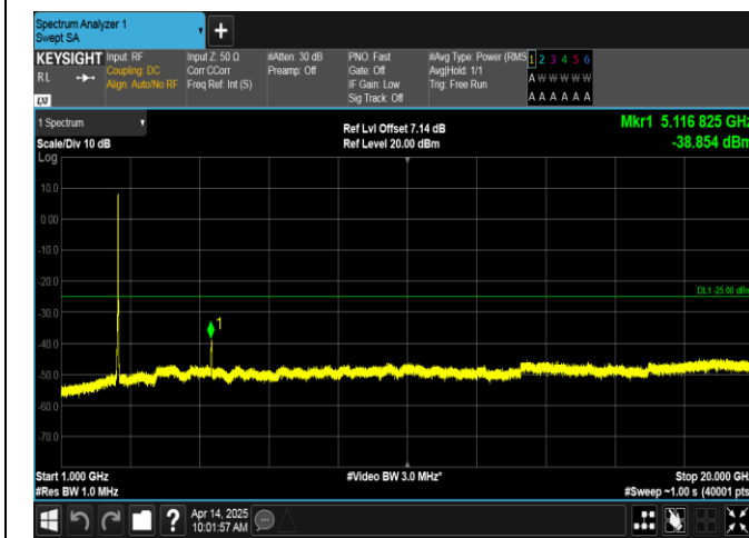
Band7-20MHz-16QAM-21350-100RB#0-1000~20000-PASS
