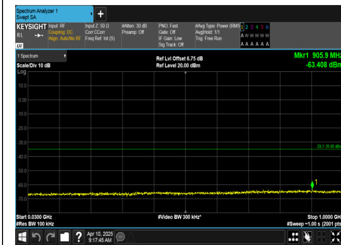
Band7-20MHz-16QAM-21350-1RB#99-30~1000-PASS
