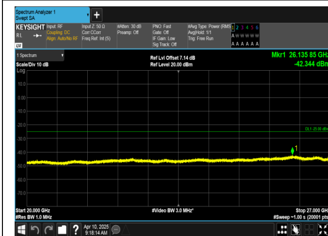
Band7-20MHz-16QAM-21350-1RB#99-20000~27000-PASS
