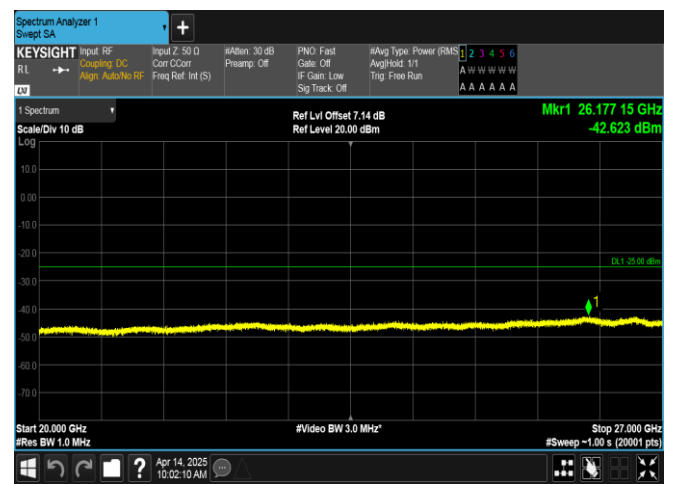
Band7-20MHz-16QAM-21350-100RB#0-20000~27000-PASS
