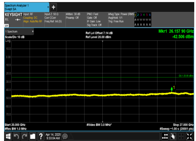
Band7-15MHz-16QAM-21375-75RB#0-20000~27000-PASS
