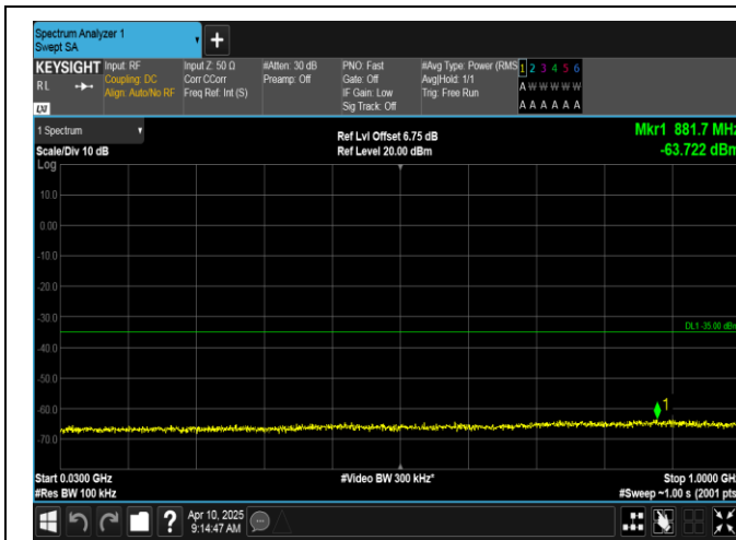
Band7-20MHz-QPSK-21350-1RB#0-30~1000-PASS
