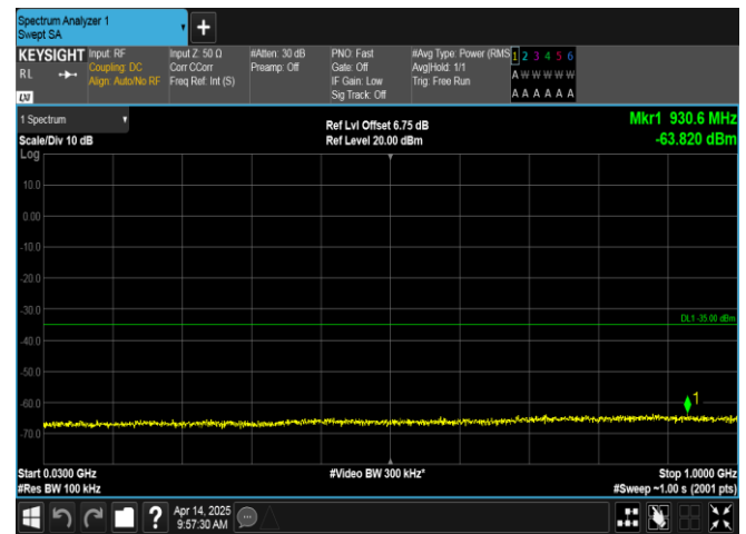
Band7-20MHz-16QAM-20850-100RB#0-30~1000-PASS
