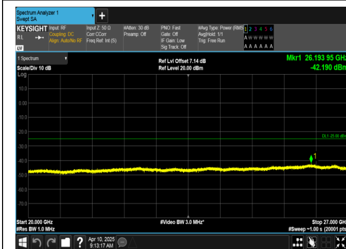
Band7-20MHz-QPSK-21100-1RB#99-20000~27000-PASS
