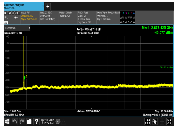
Band7-20MHz-QPSK-21350-1RB#0-1000~20000-PASS
