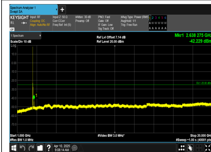
Band7-20MHz-16QAM-20850-1RB#0-1000~20000-PASS
