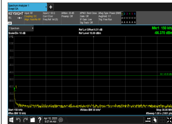
Band7-20MHz-16QAM-20850-1RB#0-0.15~30-PASS
