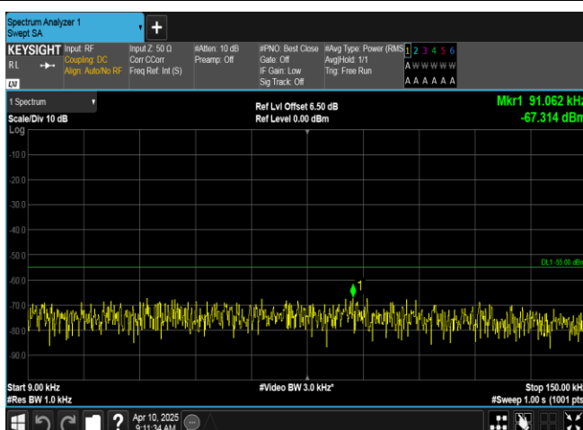
Band7-20MHz-16QAM-21100-1RB#0-0.009~0.15-PASS
