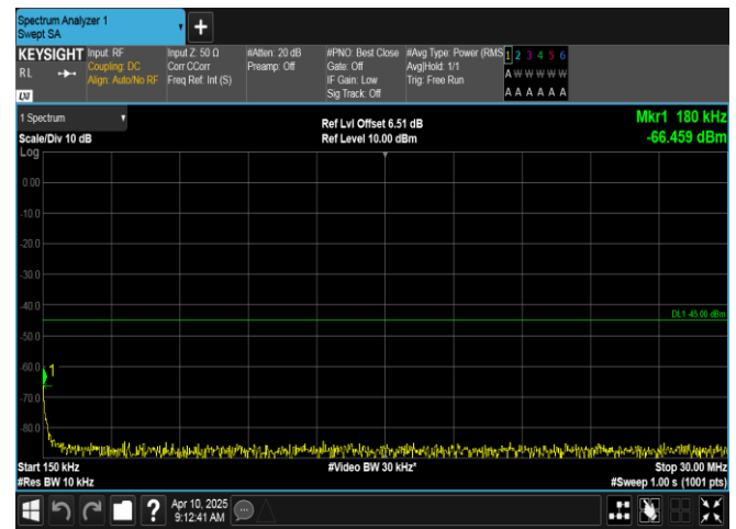
Band7-20MHz-QPSK-21100-1RB#99-0.15~30-PASS
