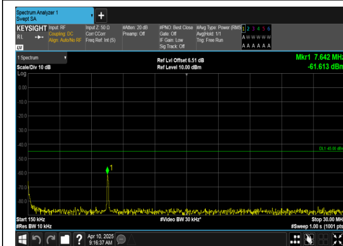
Band7-20MHz-QPSK-21350-1RB#99-0.15~30-PASS
