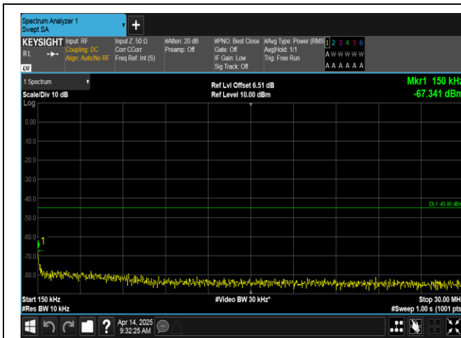
Band7-15MHz-16QAM-21375-75RB#0-0.15~30-PASS
