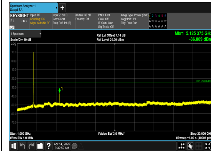
Band7-15MHz-16QAM-21375-75RB#0-1000~20000-PASS
