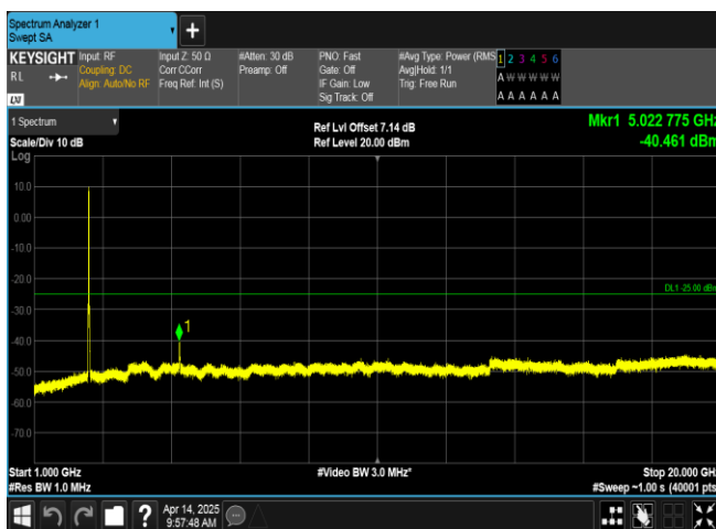
Band7-20MHz-16QAM-20850-100RB#0-1000~20000-PASS
