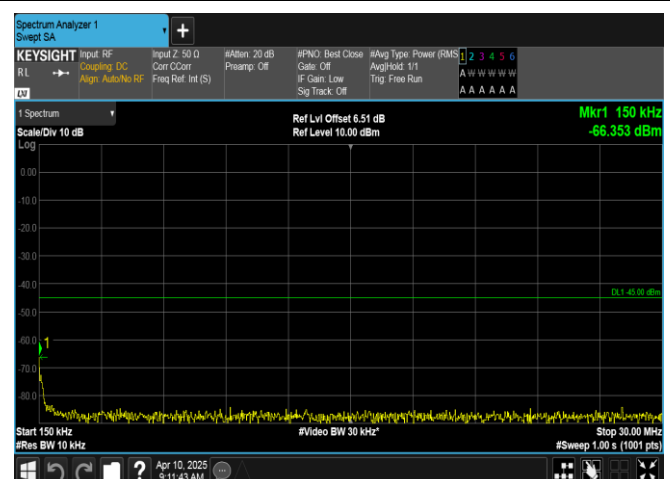
Band7-20MHz-16QAM-21100-1RB#0-0.15~30-PASS
