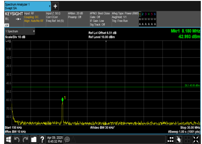
Band7-10MHz-16QAM-21400-1RB#49-0.15~30-PASS
