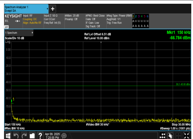
Band7-15MHz-QPSK-20825-1RB#0-0.15~30-PASS
