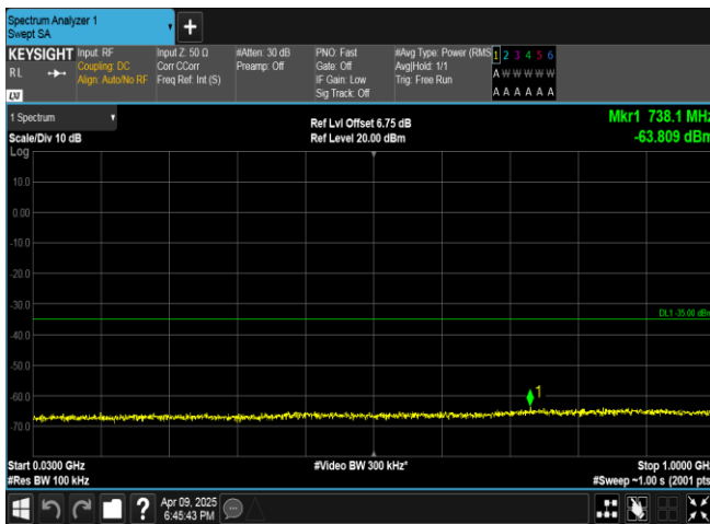
Band7-10MHz-16QAM-21400-1RB#49-30~1000-PASS
