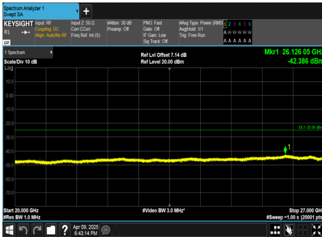
Band7-10MHz-QPSK-21400-1RB#0-20000~27000-PASS
