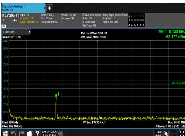
Band7-10MHz-QPSK-21400-1RB#49-0.15~30-PASS
