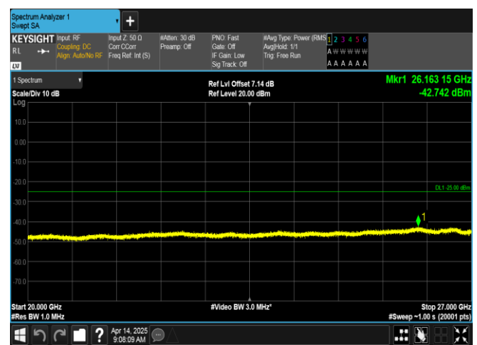
Band7-10MHz-16QAM-21400-50RB#0-20000~27000-PASS
