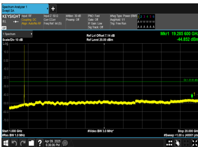
Band7-10MHz-16QAM-20800-1RB#0-1000~20000-PASS
