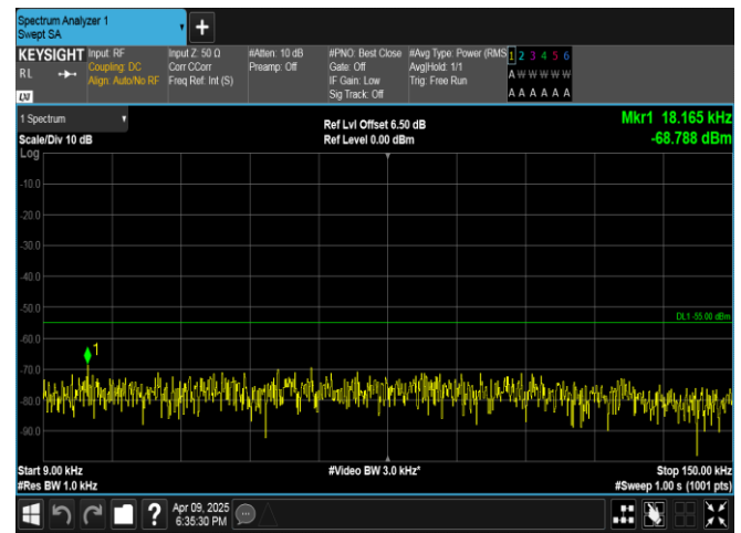
Band7-10MHz-16QAM-20800-1RB#0-0.009~0.15-PASS
