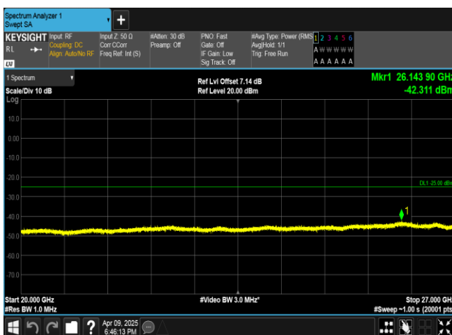
Band7-10MHz-16QAM-21400-1RB#49-20000~27000-PASS
