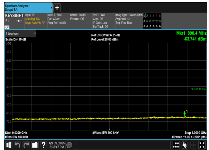
Band7-10MHz-16QAM-20800-1RB#0-30~1000-PASS
