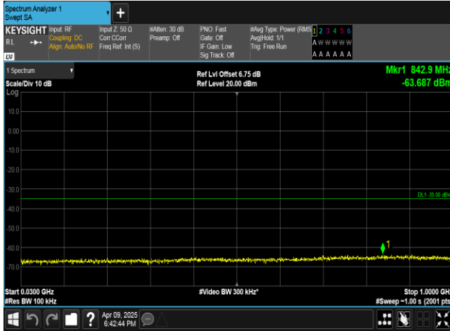
Band7-10MHz-QPSK-21400-1RB#0-30~1000-PASS
