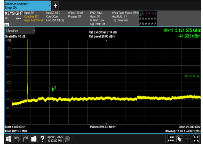
Band7-10MHz-QPSK-21400-1RB#0-1000~20000-PASS
