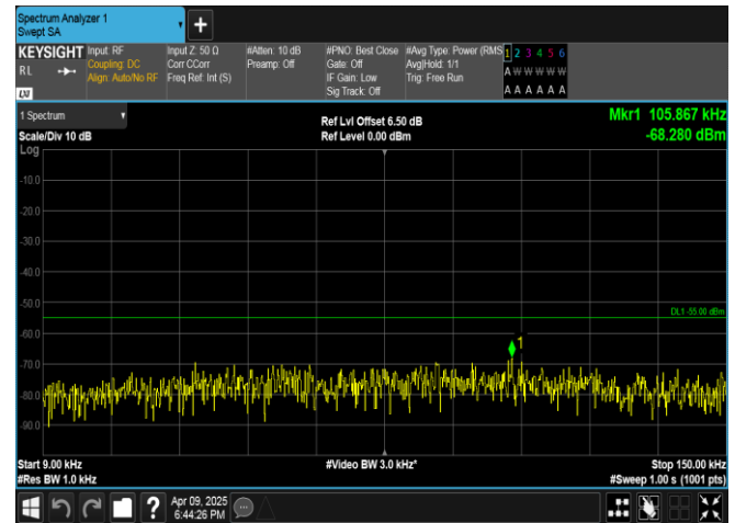
Band7-10MHz-QPSK-21400-1RB#49-0.009~0.15-PASS
