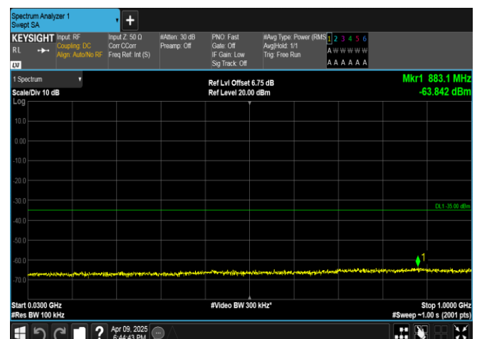
Band7-10MHz-QPSK-21400-1RB#49-30~1000-PASS
