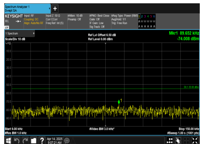
Band7-10MHz-16QAM-21400-50RB#0-0.009~0.15-PASS
