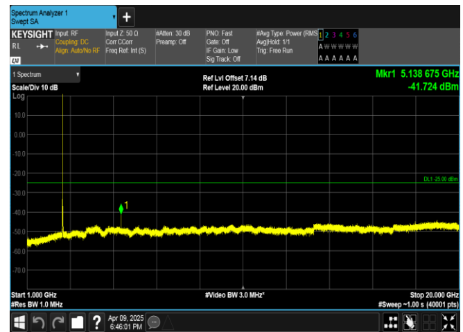
Band7-10MHz-16QAM-21400-1RB#49-1000~20000-PASS
