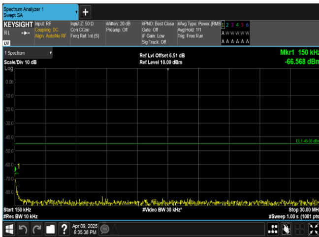
Band7-10MHz-16QAM-20800-1RB#0-0.15~30-PASS
