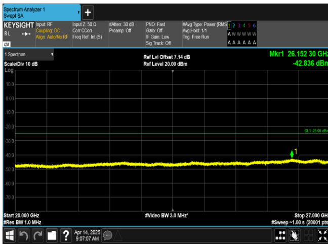
Band7-10MHz-QPSK-21400-50RB#0-20000~27000-PASS
