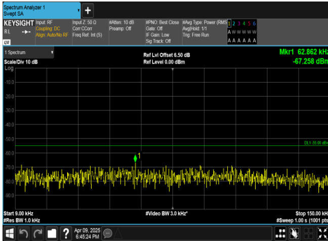
Band7-10MHz-16QAM-21400-1RB#49-0.009~0.15-PASS
