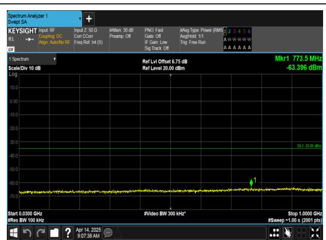
Band7-10MHz-16QAM-21400-50RB#0-30~1000-PASS
