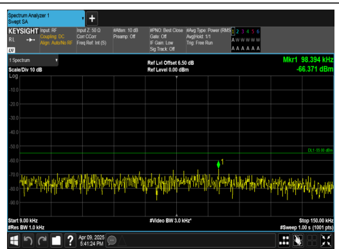
Band7-5MHz-16QAM-21425-1RB#0-0.009~0.15-PASS
