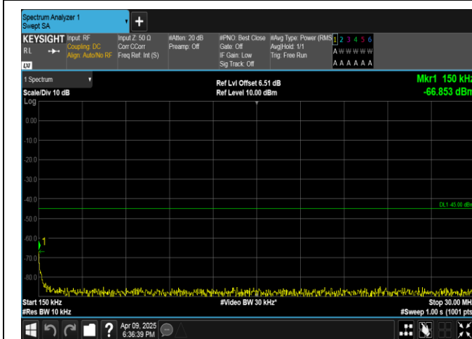
Band7-10MHz-QPSK-20800-1RB#49-0.15~30-PASS
