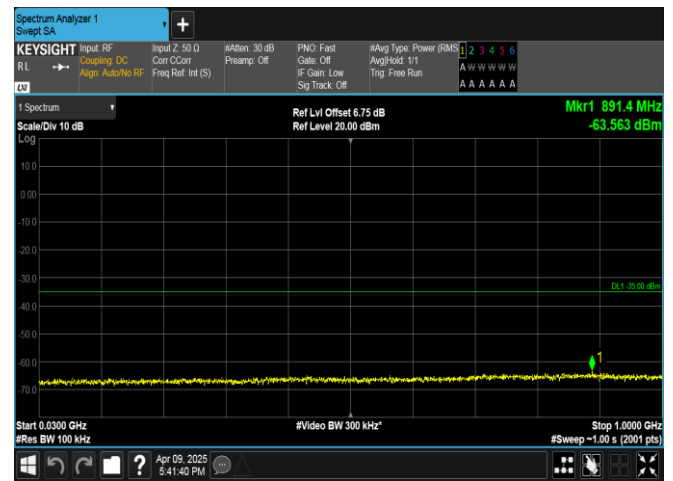
Band7-5MHz-16QAM-21425-1RB#0-30~1000-PASS
