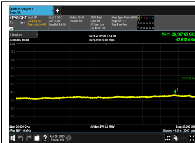
Band7-5MHz-QPSK-21425-25RB#0-20000~27000-PASS
