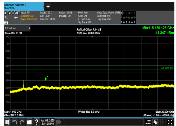
Band7-5MHz-QPSK-21425-1RB#0-1000~20000-PASS
