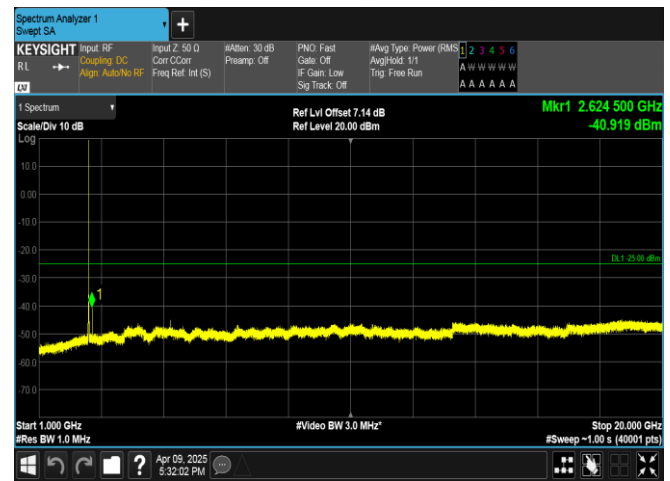
Band7-5MHz-16QAM-20775-1RB#24-1000~20000-PASS
