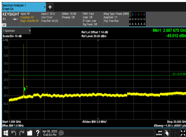
Band7-5MHz-16QAM-21425-25RB#0-1000~20000-PASS
