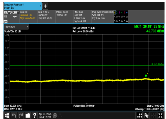
Band7-5MHz-16QAM-20775-25RB#0-20000~27000-PASS
