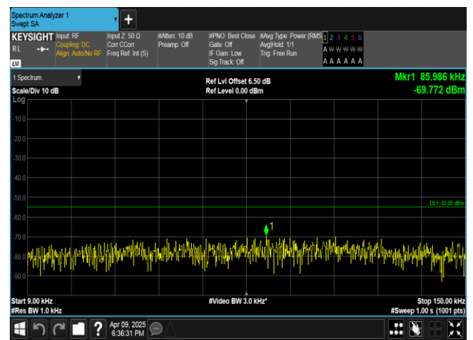
Band7-10MHz-QPSK-20800-1RB#49-0.009~0.15-PASS
