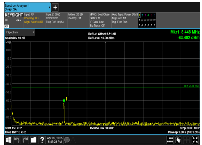
Band7-5MHz-16QAM-21425-1RB#24-0.15~30-PASS
