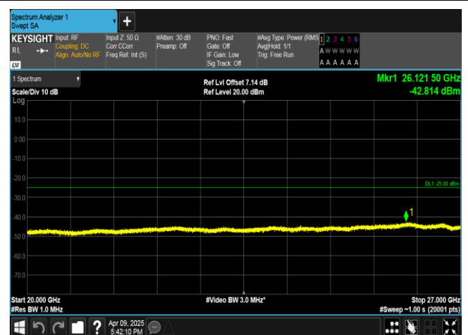
Band7-5MHz-16QAM-21425-1RB#0-20000~27000-PASS
