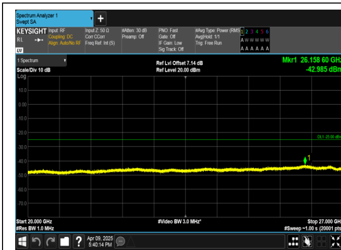
Band7-5MHz-16QAM-21100-25RB#0-20000~27000-PASS
