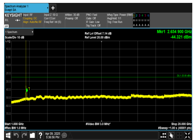
Band7-5MHz-QPSK-21100-1RB#24-1000~20000-PASS
