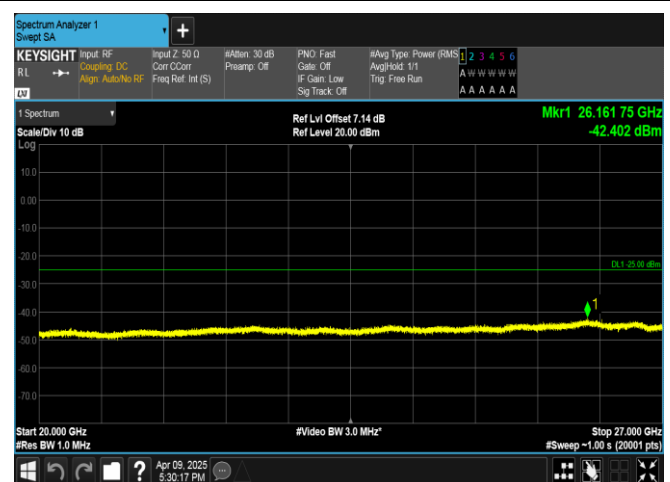
Band7-5MHz-16QAM-20775-1RB#0-20000~27000-PASS
