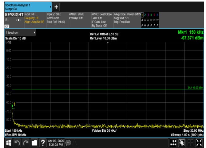
Band7-5MHz-16QAM-20775-1RB#24-0.15~30-PASS
