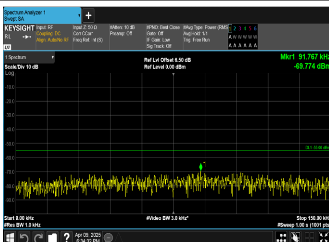
Band7-10MHz-QPSK-20800-1RB#0-0.009~0.15-PASS
