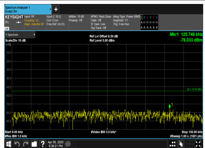
Band7-5MHz-QPSK-21100-25RB#0-0.009~0.15-PASS
