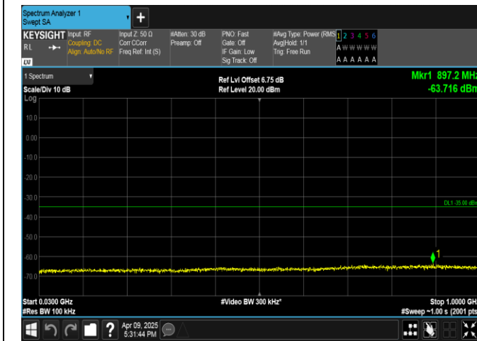
Band7-5MHz-16QAM-20775-1RB#24-30~1000-PASS
