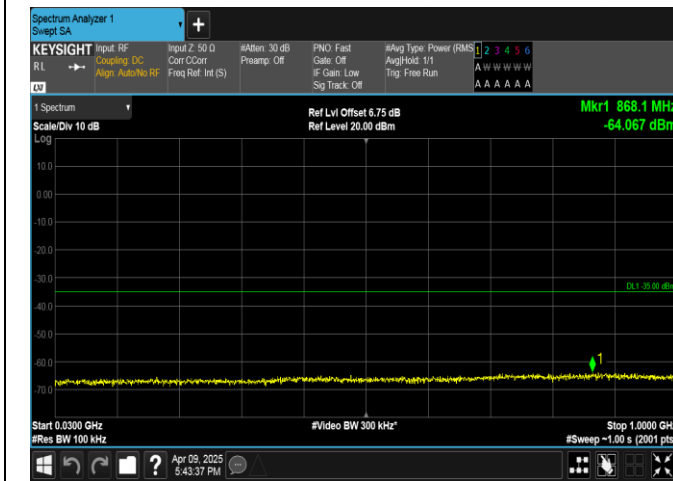
Band7-5MHz-16QAM-21425-1RB#24-30~1000-PASS
