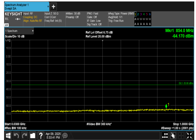
Band7-5MHz-16QAM-20775-25RB#0-30~1000-PASS
