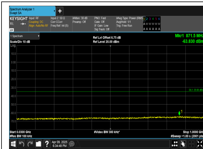
Band7-10MHz-QPSK-20800-1RB#0-30~1000-PASS
