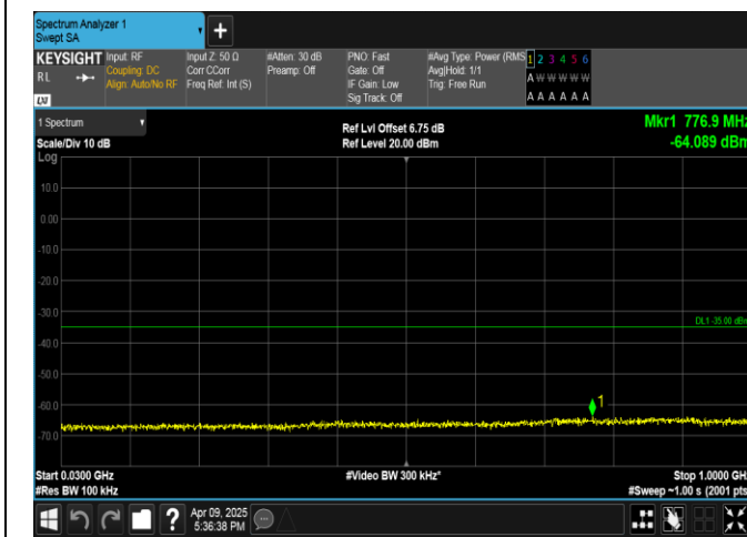
Band7-5MHz-QPSK-21100-1RB#24-30~1000-PASS
