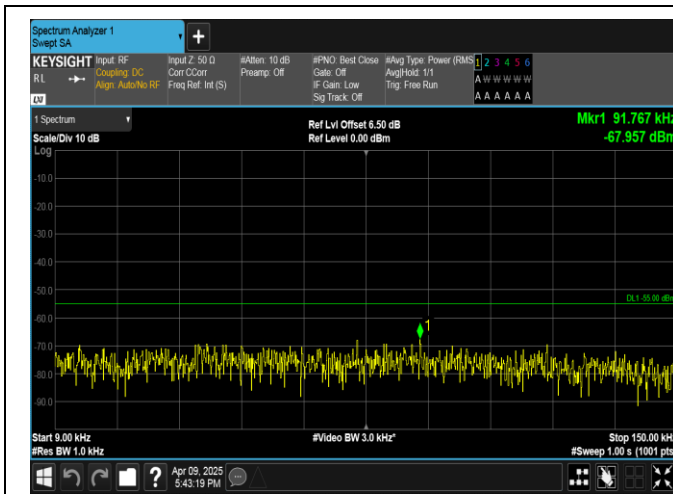
Band7-5MHz-16QAM-21425-1RB#24-0.009~0.15-PASS
