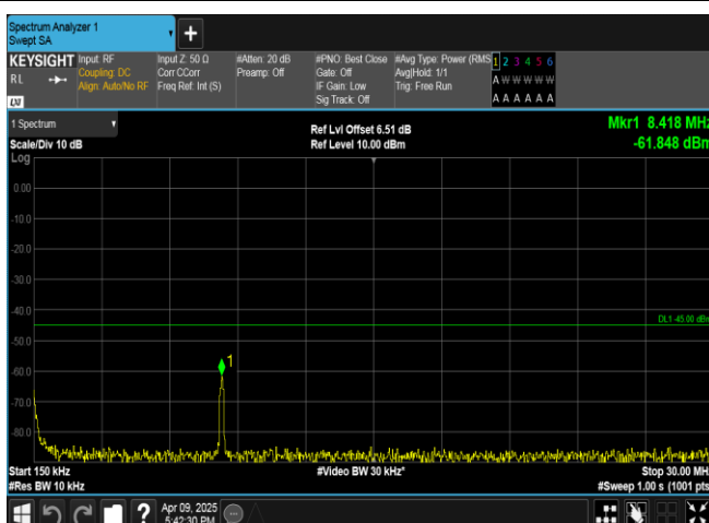
Band7-5MHz-QPSK-21425-1RB#24-0.15~30-PASS
