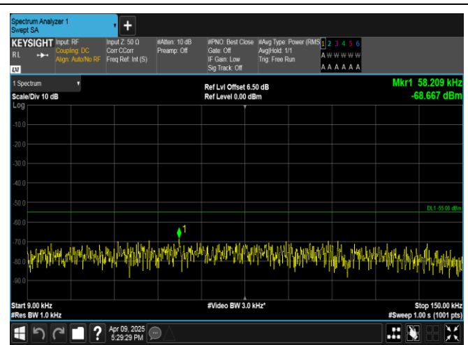
Band7-5MHz-16QAM-20775-1RB#0-0.009~0.15-PASS
