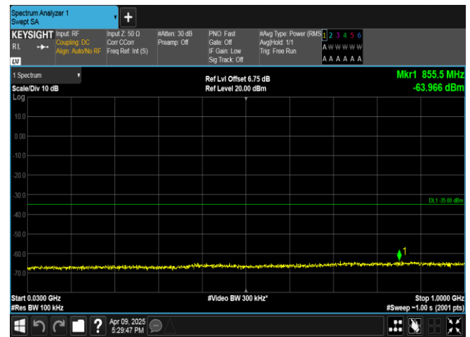
Band7-5MHz-16QAM-20775-1RB#0-30~1000-PASS
