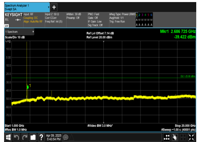
Band7-5MHz-16QAM-21425-1RB#24-1000~20000-PASS
