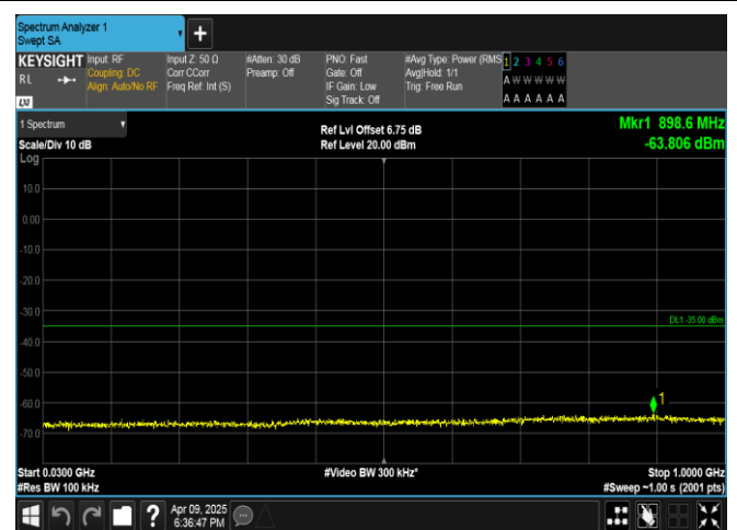
Band7-10MHz-QPSK-20800-1RB#49-30~1000-PASS
