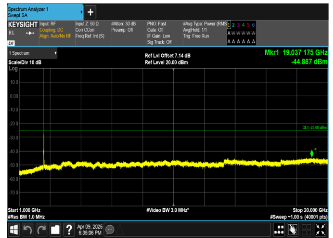
Band7-10MHz-QPSK-20800-1RB#0-1000~20000-PASS
