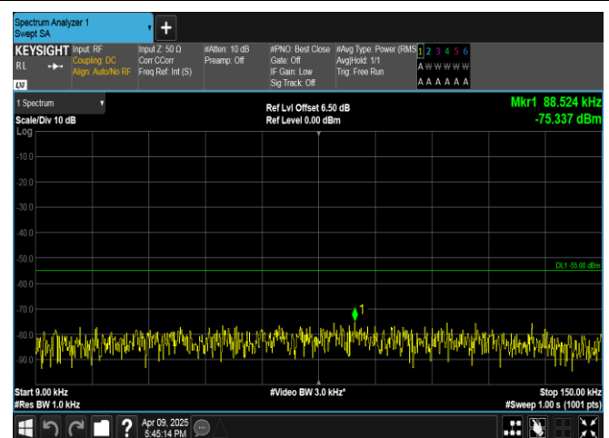
Band7-5MHz-16QAM-21425-25RB#0-0.009~0.15-PASS
