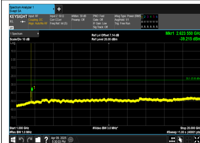
Band7-5MHz-16QAM-20775-1RB#0-1000~20000-PASS
