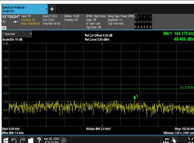
Band7-5MHz-16QAM-21100-1RB#0-0.009~0.15-PASS
