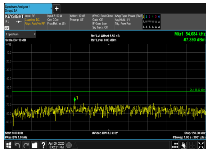
Band7-5MHz-QPSK-21425-1RB#24-0.009~0.15-PASS
