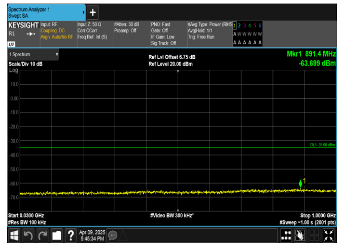
Band7-5MHz-16QAM-21425-25RB#0-30~1000-PASS
