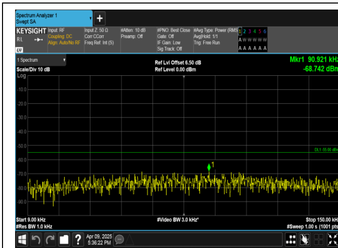
Band7-5MHz-QPSK-21100-1RB#24-0.009~0.15-PASS
