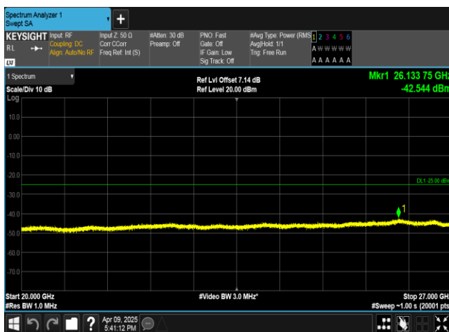
Band7-5MHz-QPSK-21425-1RB#0-20000~27000-PASS
