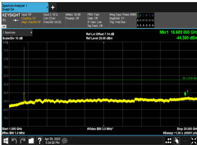
Band7-5MHz-16QAM-20775-25RB#0-1000~20000-PASS
