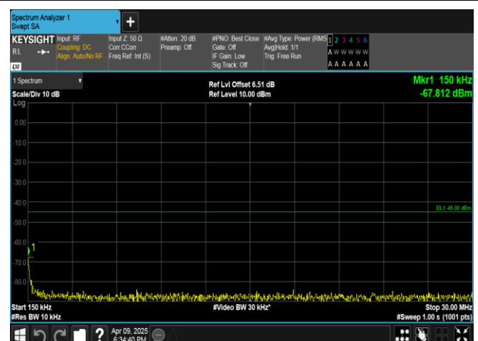
Band7-10MHz-QPSK-20800-1RB#0-0.15~30-PASS
