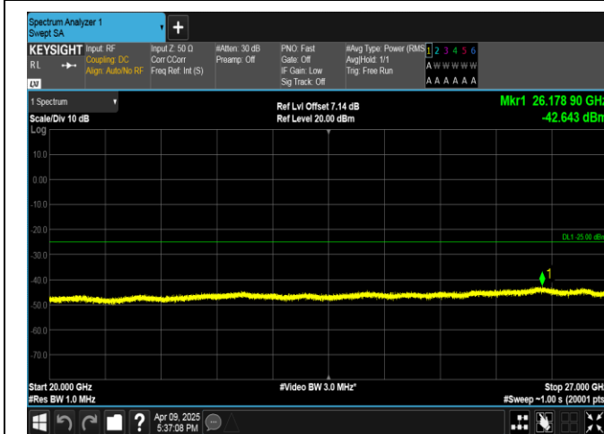
Band7-5MHz-QPSK-21100-1RB#24-20000~27000-PASS
