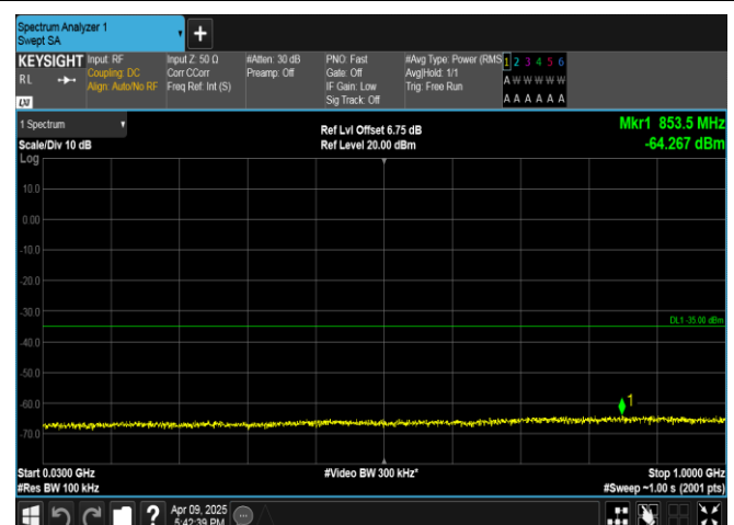
Band7-5MHz-QPSK-21425-1RB#24-30~1000-PASS
