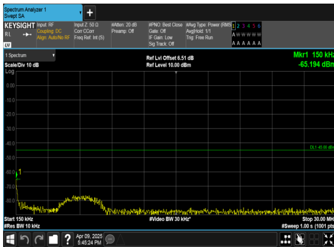
Band7-5MHz-16QAM-21425-25RB#0-0.15~30-PASS
