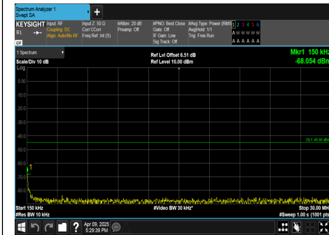
Band7-5MHz-16QAM-20775-1RB#0-0.15~30-PASS
