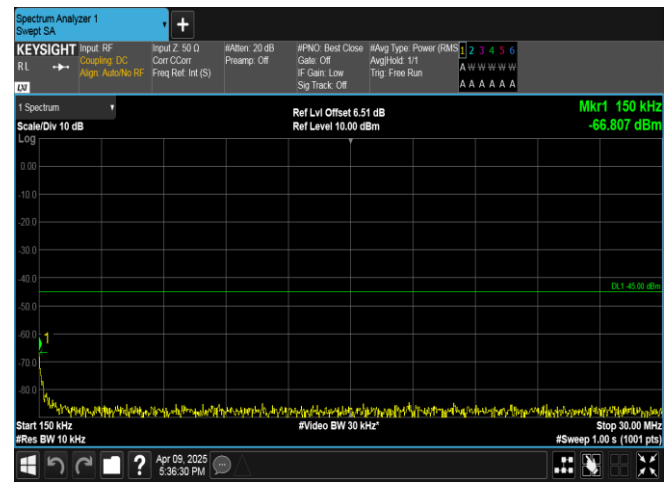
Band7-5MHz-QPSK-21100-1RB#24-0.15~30-PASS
