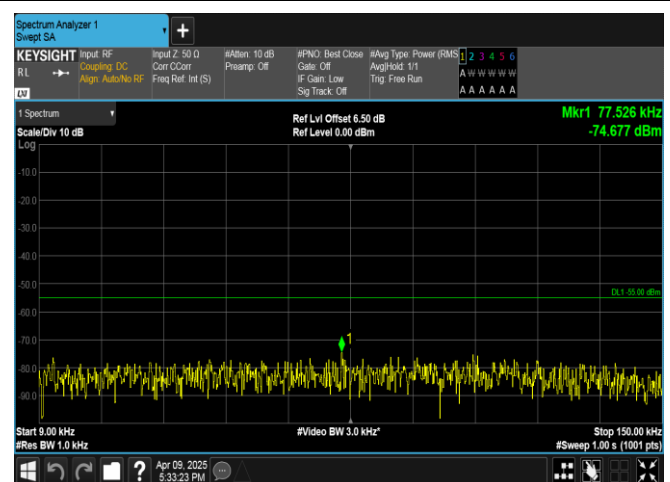
Band7-5MHz-16QAM-20775-25RB#0-0.009~0.15-PASS
