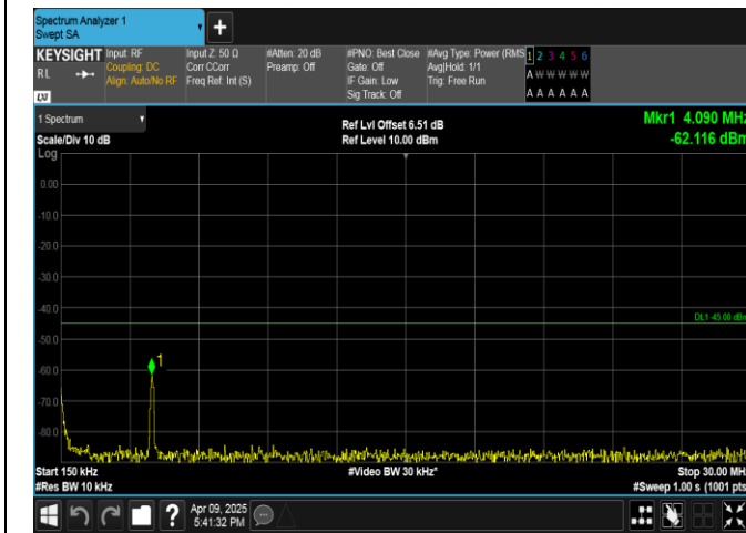
Band7-5MHz-16QAM-21425-1RB#0-0.15~30-PASS
