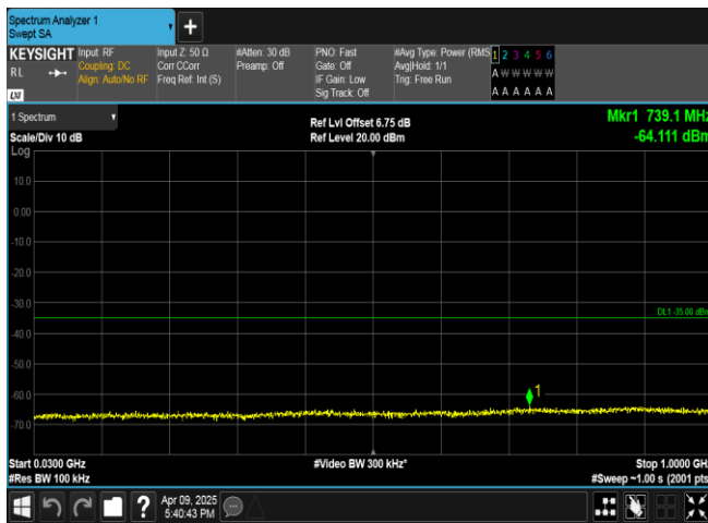
Band7-5MHz-QPSK-21425-1RB#0-30~1000-PASS
