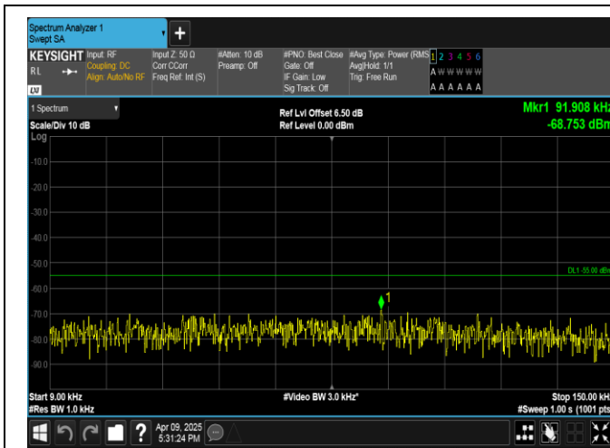
Band7-5MHz-16QAM-20775-1RB#24-0.009~0.15-PASS
