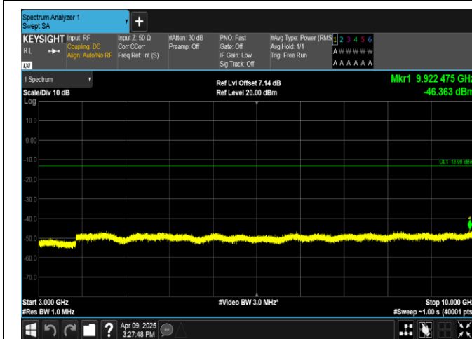
Band5-10MHz-16QAM-20450-1RB#49-3000~10000-PASS
