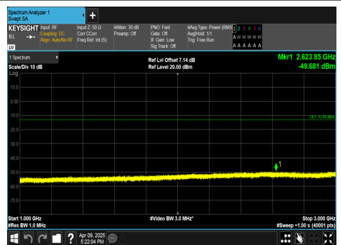
Band5-10MHz-QPSK-20600-50RB#0-1000~3000-PASS
