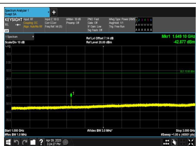
Band5-10MHz-QPSK-20450-1RB#0-1000~3000-PASS
