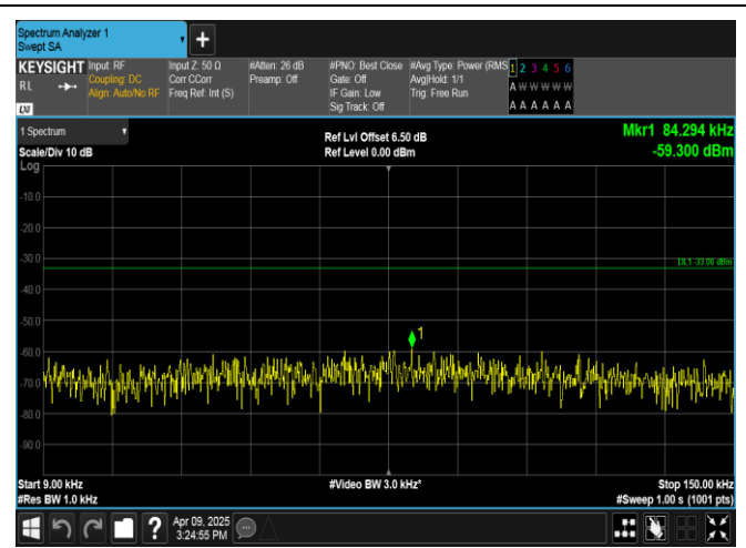
Band5-10MHz-16QAM-20450-1RB#0-0.009~0.15-PASS
