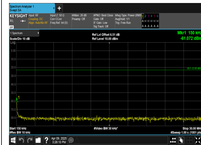
Band5-10MHz-QPSK-20525-1RB#0-0.15~30-PASS
