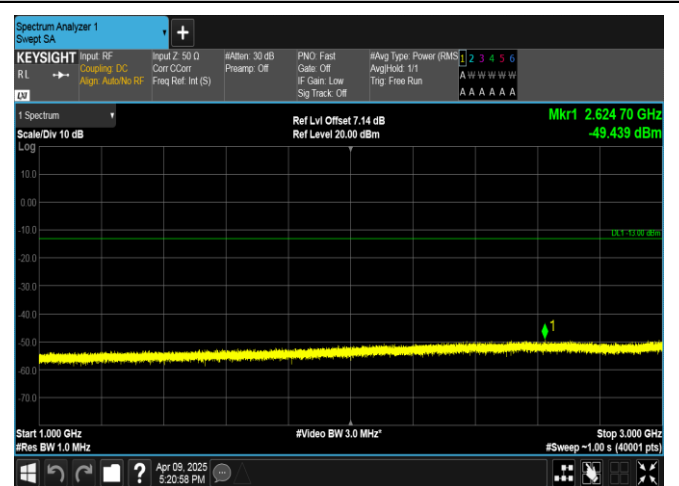
Band5-10MHz-16QAM-20525-50RB#0-1000~3000-PASS
