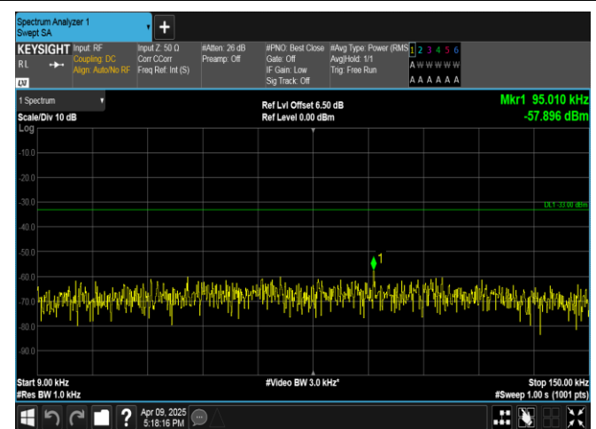
Band5-10MHz-16QAM-20450-50RB#0-0.009~0.15-PASS
