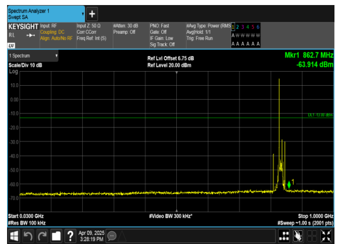
Band5-10MHz-QPSK-20525-1RB#0-30~1000-PASS
