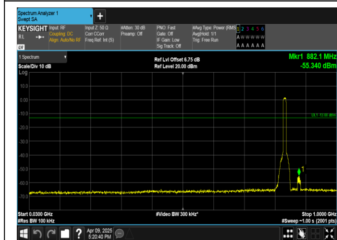
Band5-10MHz-16QAM-20525-50RB#0-30~1000-PASS
