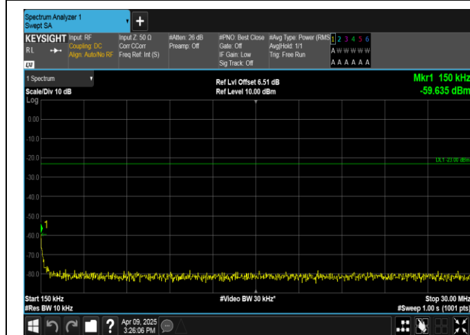
Band5-10MHz-QPSK-20450-1RB#49-0.15~30-PASS
