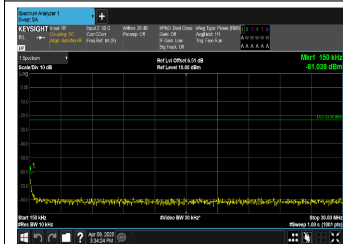
Band5-10MHz-QPSK-20600-1RB#49-0.15~30-PASS
