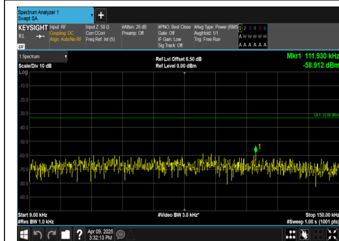
Band5-10MHz-QPSK-20600-1RB#0-0.009~0.15-PASS
