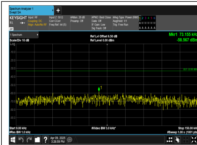
Band5-10MHz-16QAM-20450-1RB#49-0.009~0.15-PASS
