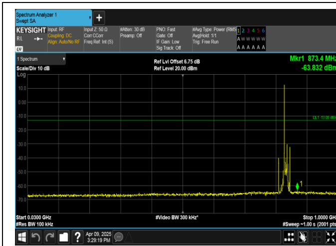
Band5-10MHz-16QAM-20525-1RB#0-30~1000-PASS
