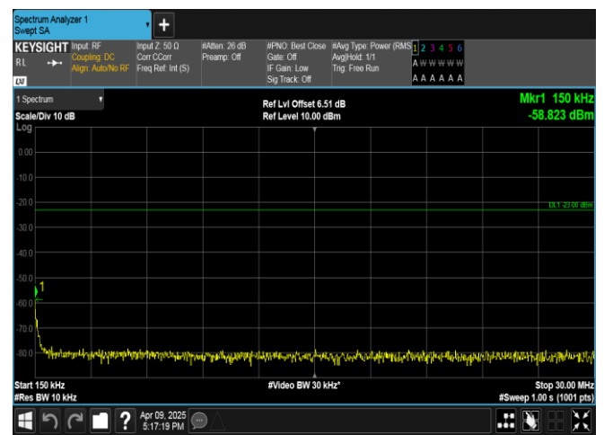
Band5-10MHz-QPSK-20450-50RB#0-0.15~30-PASS
