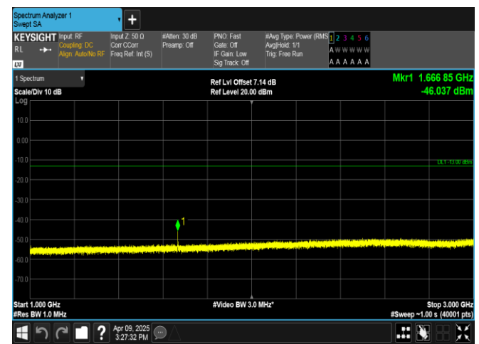
Band5-10MHz-16QAM-20450-1RB#49-1000~3000-PASS
