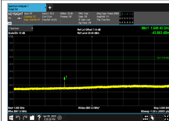
Band5-10MHz-16QAM-20450-1RB#0-1000~3000-PASS
