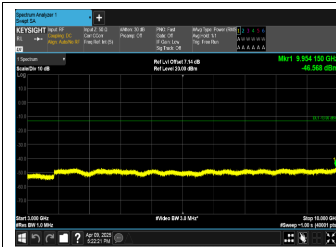
Band5-10MHz-QPSK-20600-50RB#0-3000~10000-PASS
