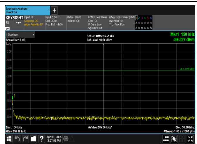
Band5-10MHz-16QAM-20450-1RB#49-0.15~30-PASS
