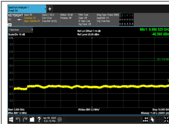
Band5-10MHz-16QAM-20525-50RB#0-3000~10000-PASS
