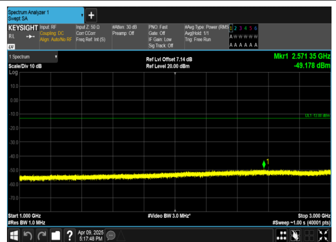
Band5-10MHz-QPSK-20450-50RB#0-1000~3000-PASS
