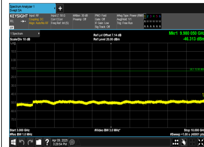
Band5-10MHz-16QAM-20525-1RB#0-3000~10000-PASS
