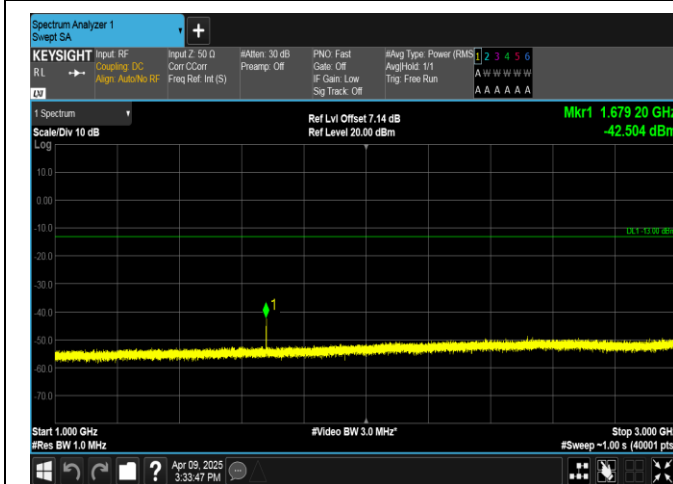
Band5-10MHz-16QAM-20600-1RB#0-1000~3000-PASS
