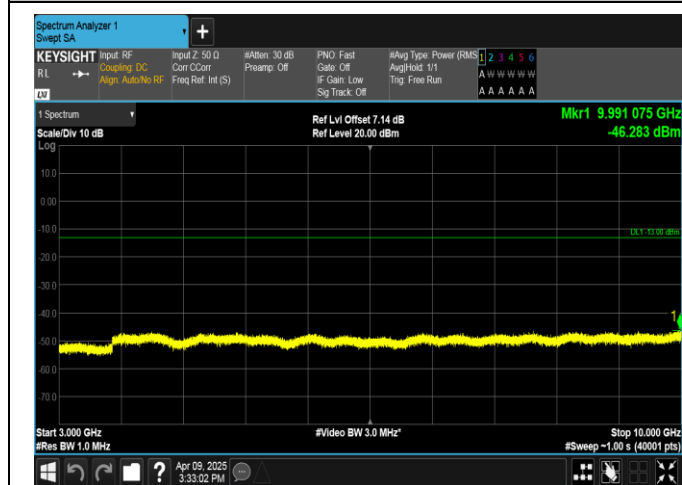
Band5-10MHz-QPSK-20600-1RB#0-3000~10000-PASS
