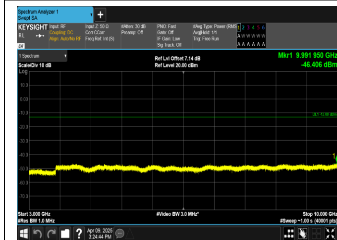
Band5-10MHz-QPSK-20450-1RB#0-3000~10000-PASS
