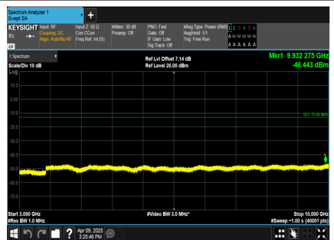
Band5-10MHz-16QAM-20450-1RB#0-3000~10000-PASS
