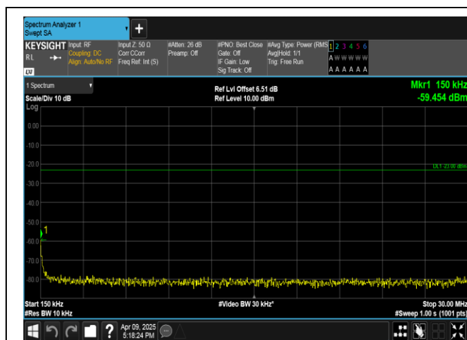
Band5-10MHz-16QAM-20450-50RB#0-0.15~30-PASS
