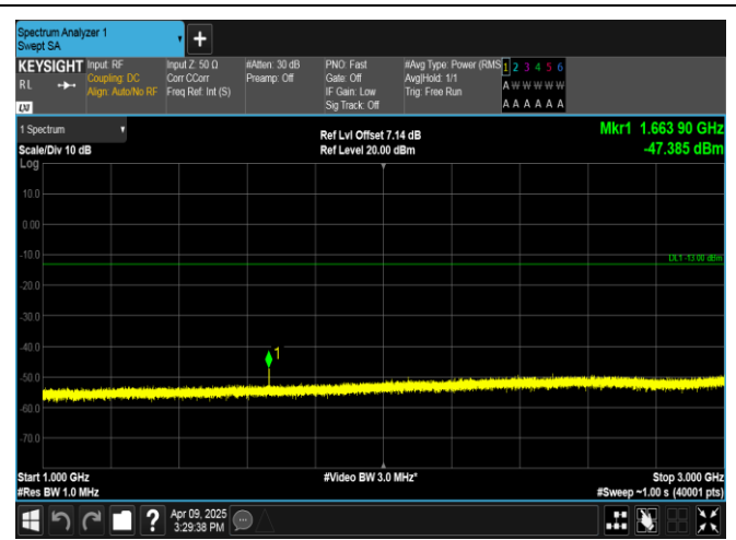
Band5-10MHz-16QAM-20525-1RB#0-1000~3000-PASS
