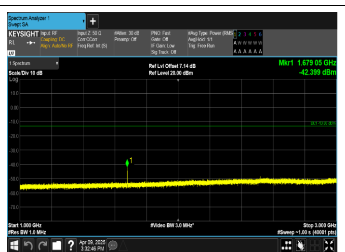
Band5-10MHz-QPSK-20600-1RB#0-1000~3000-PASS
