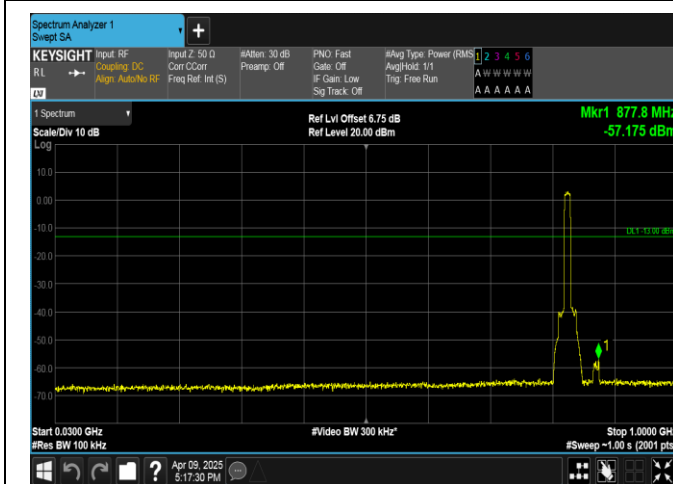
Band5-10MHz-QPSK-20450-50RB#0-30~1000-PASS
