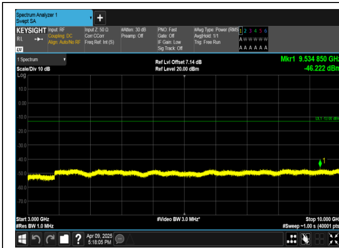
Band5-10MHz-QPSK-20450-50RB#0-3000~10000-PASS
