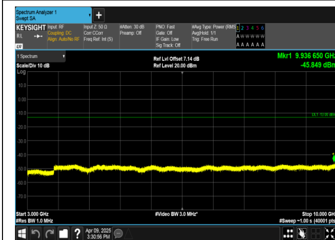
Band5-10MHz-QPSK-20525-1RB#49-3000~10000-PASS
