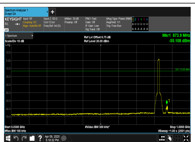
Band5-10MHz-16QAM-20450-50RB#0-30~1000-PASS
