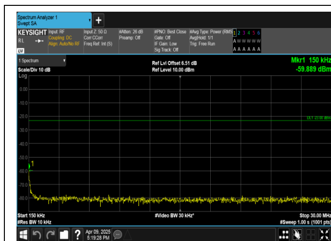
Band5-10MHz-QPSK-20525-50RB#0-0.15~30-PASS
