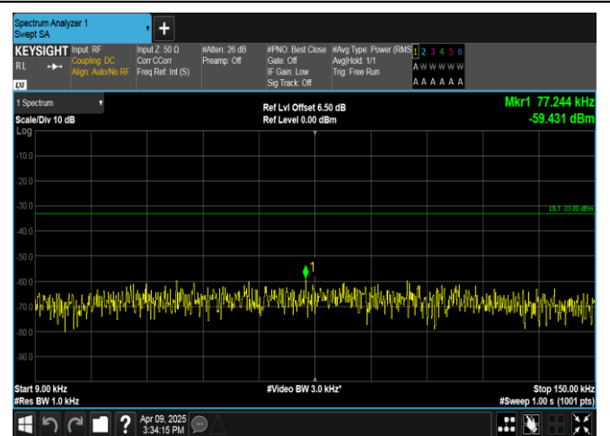
Band5-10MHz-QPSK-20600-1RB#49-0.009~0.15-PASS
