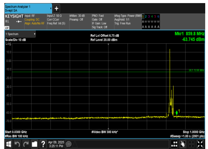
Band5-10MHz-16QAM-20450-1RB#0-30~1000-PASS
