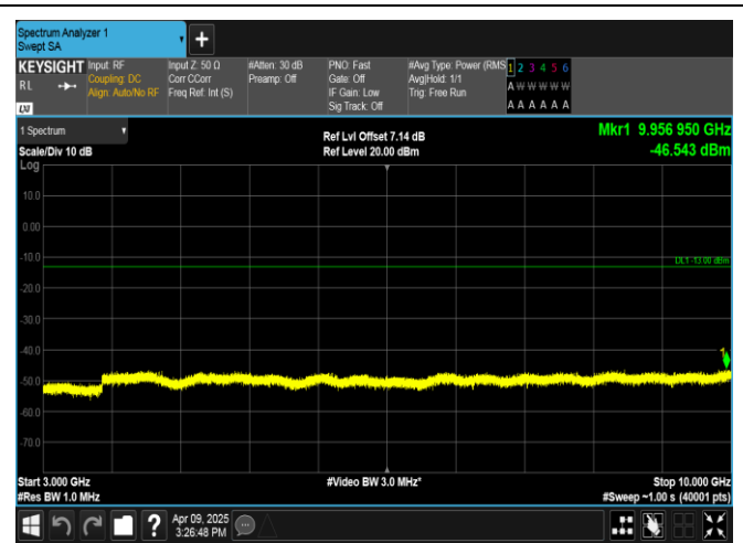
Band5-10MHz-QPSK-20450-1RB#49-3000~10000-PASS
