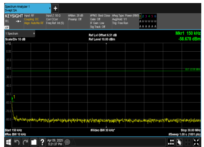
Band5-10MHz-QPSK-20600-50RB#0-0.15~30-PASS
