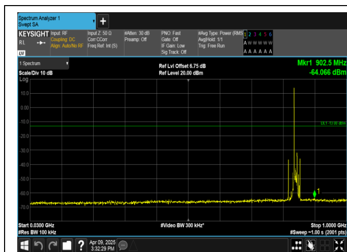
Band5-10MHz-QPSK-20600-1RB#0-30~1000-PASS
