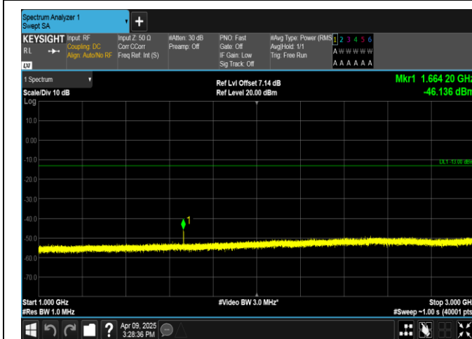
Band5-10MHz-QPSK-20525-1RB#0-1000~3000-PASS
