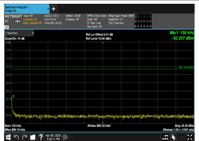
Band5-10MHz-16QAM-20525-1RB#0-0.15~30-PASS
