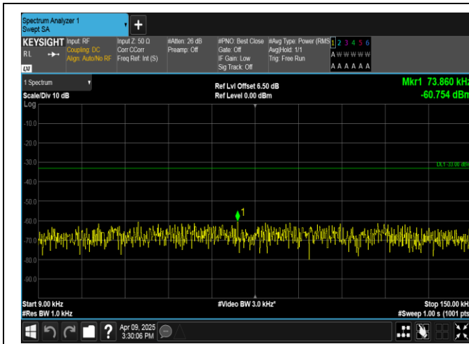
Band5-10MHz-QPSK-20525-1RB#49-0.009~0.15-PASS
