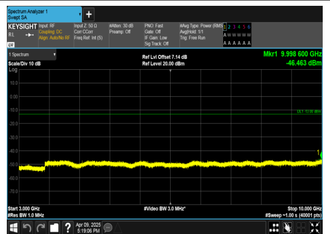
Band5-10MHz-16QAM-20450-50RB#0-3000~10000-PASS
