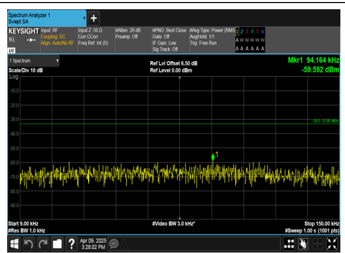
Band5-10MHz-QPSK-20525-1RB#0-0.009~0.15-PASS
