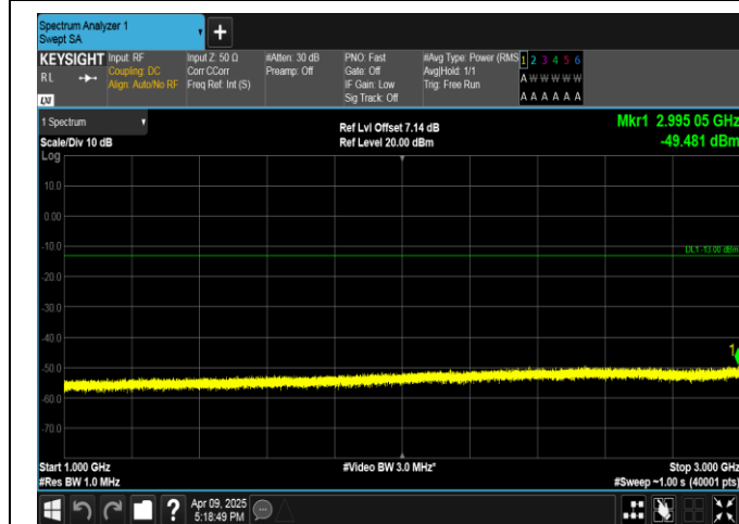
Band5-10MHz-16QAM-20450-50RB#0-1000~3000-PASS
