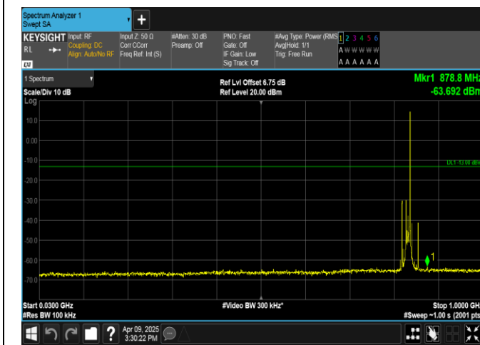
Band5-10MHz-QPSK-20525-1RB#49-30~1000-PASS
