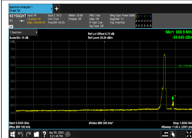
Band5-10MHz-QPSK-20600-50RB#0-30~1000-PASS
