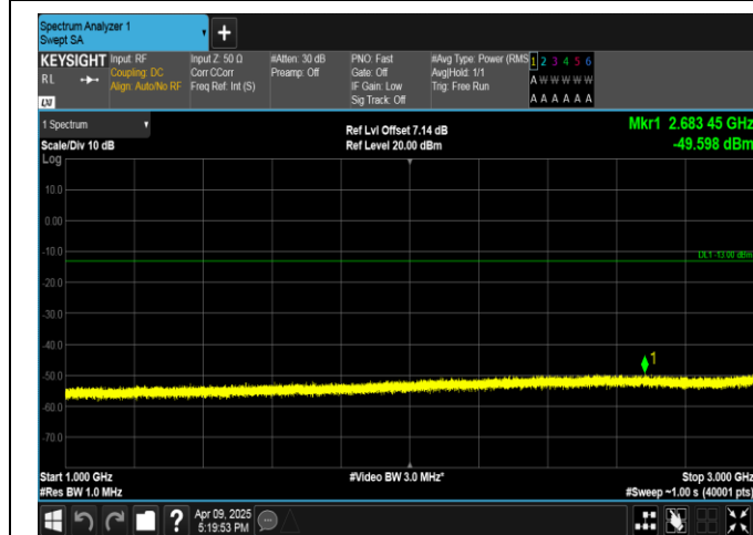
Band5-10MHz-QPSK-20525-50RB#0-1000~3000-PASS
