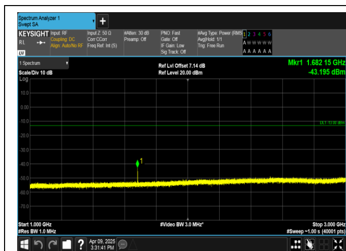
Band5-10MHz-16QAM-20525-1RB#49-1000~3000-PASS
