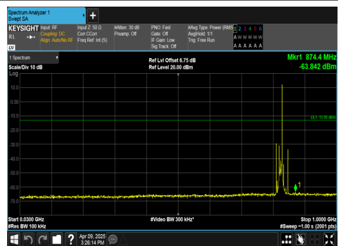
Band5-10MHz-QPSK-20450-1RB#49-30~1000-PASS
