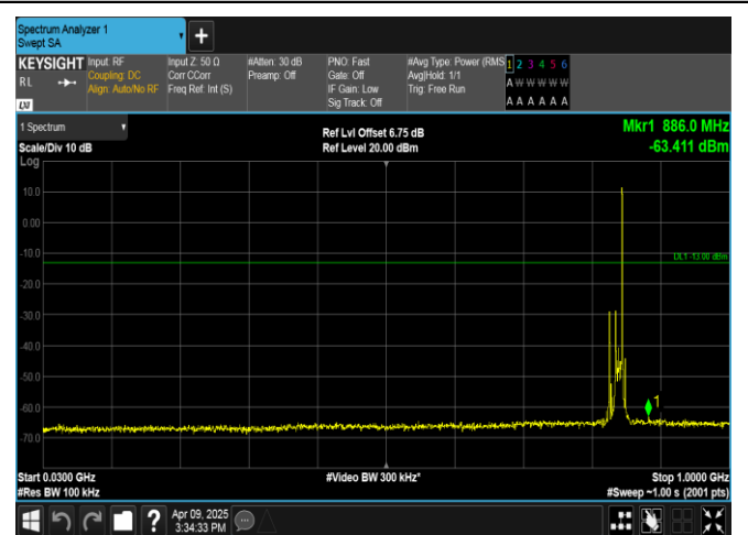
Band5-10MHz-QPSK-20600-1RB#49-30~1000-PASS
