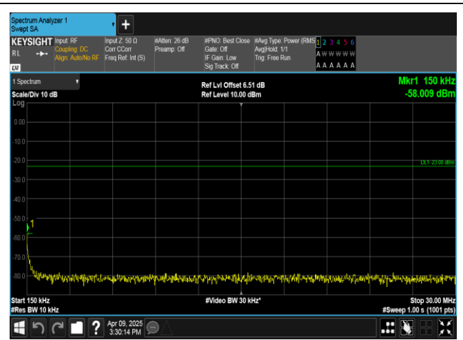
Band5-10MHz-QPSK-20525-1RB#49-0.15~30-PASS
