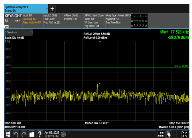
Band5-10MHz-QPSK-20525-50RB#0-0.009~0.15-PASS
