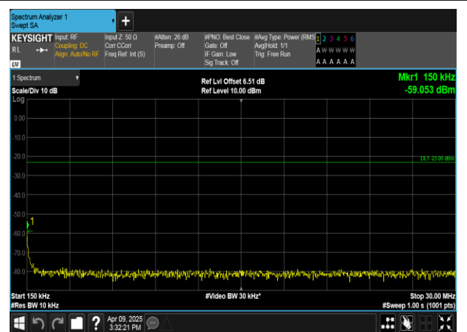
Band5-10MHz-QPSK-20600-1RB#0-0.15~30-PASS
