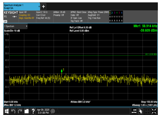
Band5-10MHz-16QAM-20525-1RB#49-0.009~0.15-PASS
