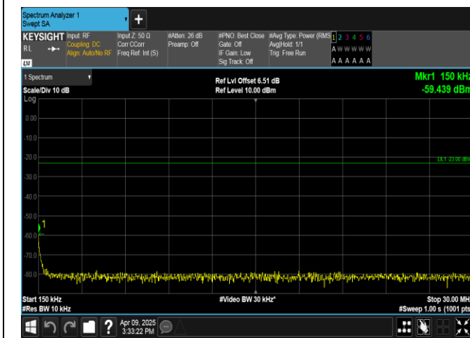
Band5-10MHz-16QAM-20600-1RB#0-0.15~30-PASS
