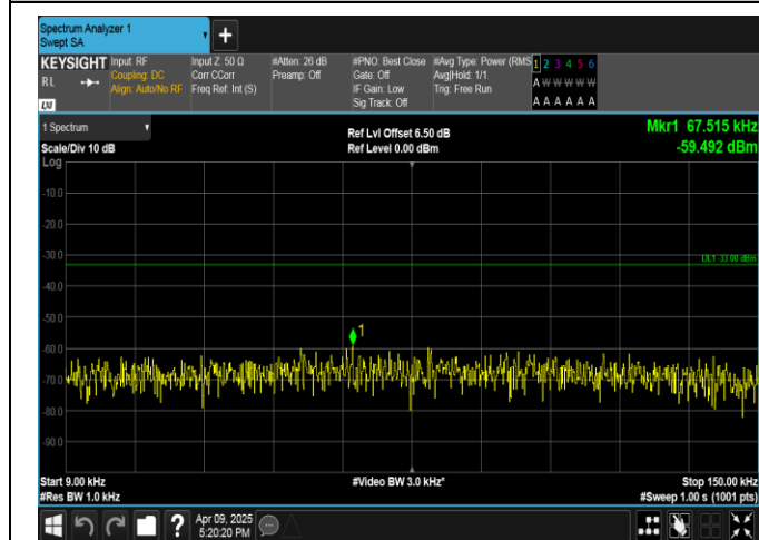
Band5-10MHz-16QAM-20525-50RB#0-0.009~0.15-PASS
