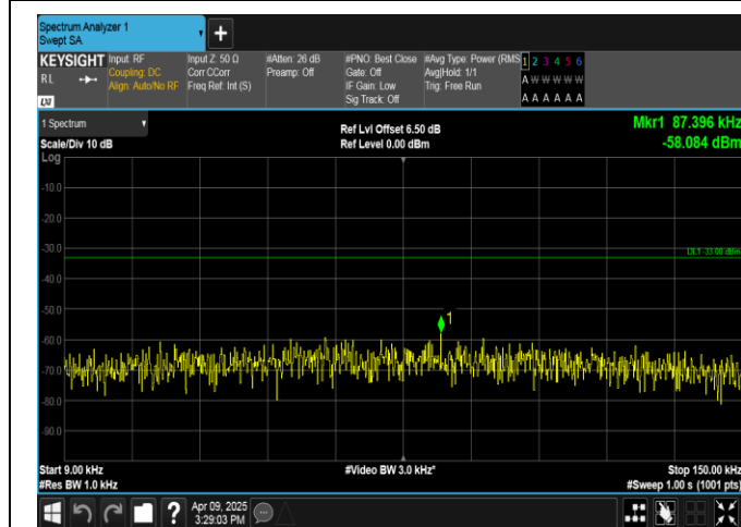
Band5-10MHz-16QAM-20525-1RB#0-0.009~0.15-PASS
