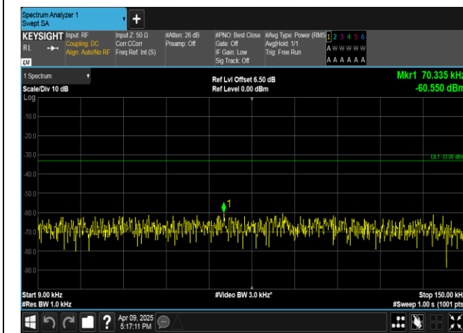
Band5-10MHz-QPSK-20450-50RB#0-0.009~0.15-PASS
