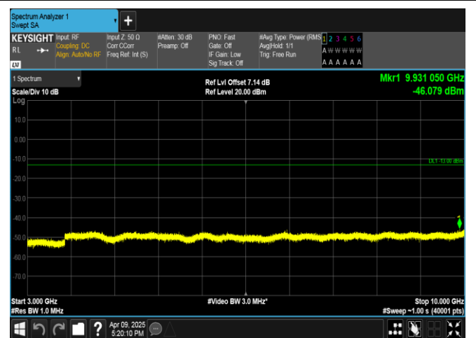
Band5-10MHz-QPSK-20525-50RB#0-3000~10000-PASS
