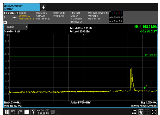
Band5-10MHz-16QAM-20525-1RB#49-30~1000-PASS
