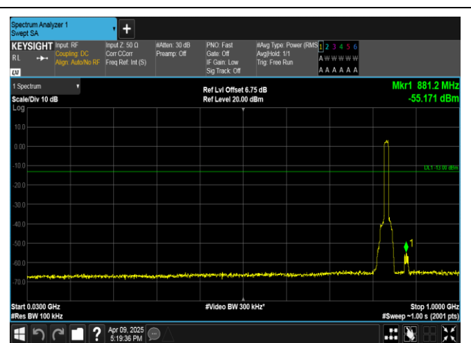
Band5-10MHz-QPSK-20525-50RB#0-30~1000-PASS
