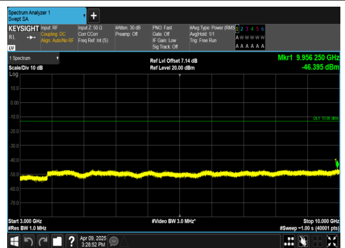
Band5-10MHz-QPSK-20525-1RB#0-3000~10000-PASS
