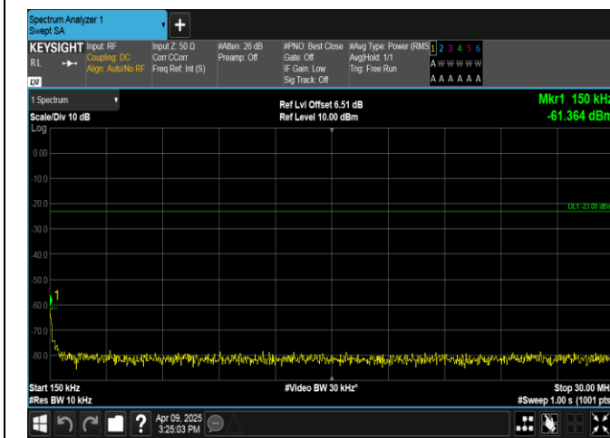
Band5-10MHz-16QAM-20450-1RB#0-0.15~30-PASS
