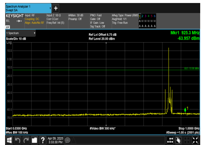
Band5-10MHz-16QAM-20600-1RB#0-30~1000-PASS
