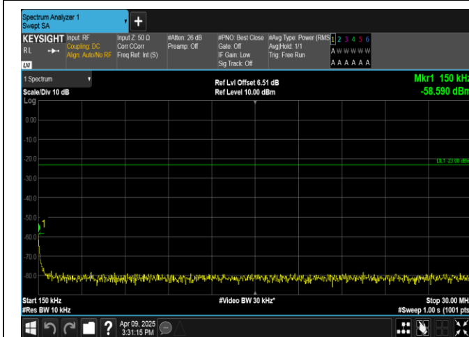
Band5-10MHz-16QAM-20525-1RB#49-0.15~30-PASS
