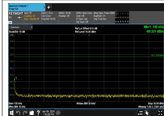
Band5-3MHz-16QAM-20525-1RB#14-0.15~30-PASS
