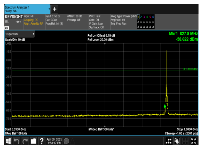
Band5-3MHz-16QAM-20525-1RB#14-30~1000-PASS
