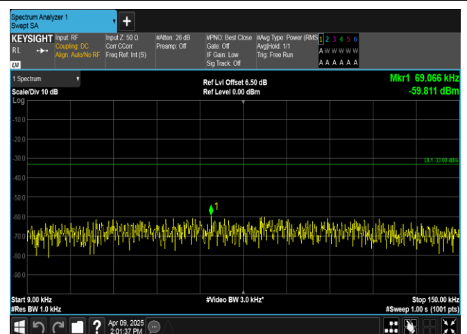
Band5-3MHz-16QAM-20635-15RB#0-0.009~0.15-PASS
