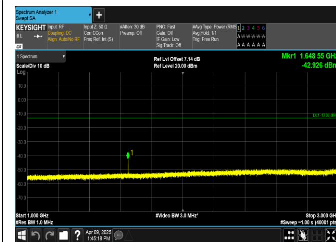
Band5-3MHz-16QAM-20415-1RB#0-1000~3000-PASS
