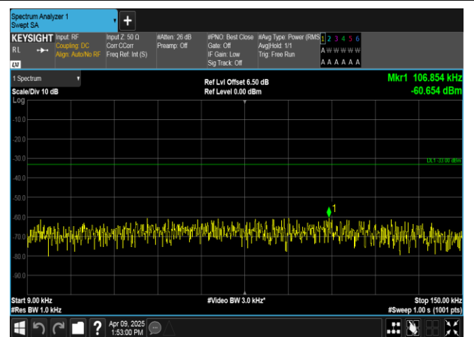
Band5-3MHz-16QAM-20525-1RB#14-0.009~0.15-PASS
