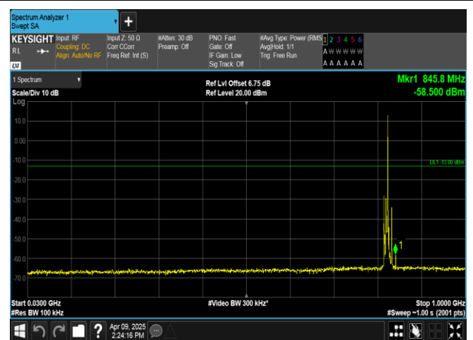
Band5-5MHz-QPSK-20425-1RB#24-30~1000-PASS
