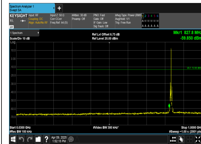
Band5-3MHz-QPSK-20525-1RB#14-30~1000-PASS
