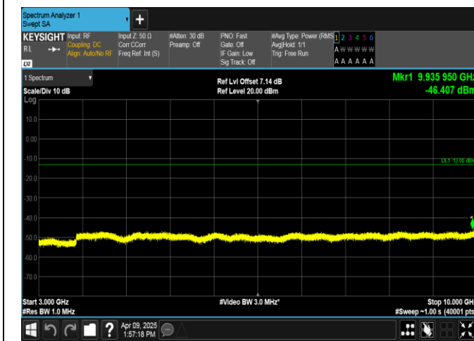
Band5-3MHz-QPSK-20635-1RB#0-3000~10000-PASS
