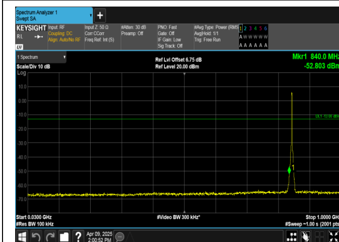
Band5-3MHz-QPSK-20635-15RB#0-30~1000-PASS
