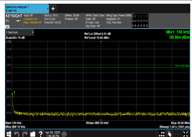
Band5-3MHz-QPSK-20635-1RB#0-0.15~30-PASS
