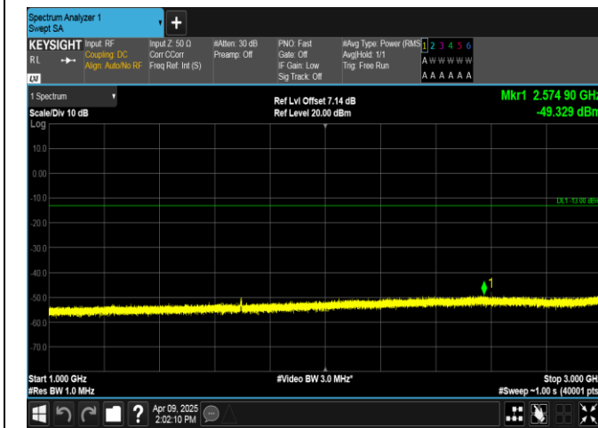
Band5-3MHz-16QAM-20635-15RB#0-1000~3000-PASS
