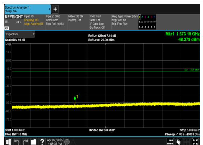
Band5-3MHz-16QAM-20525-15RB#0-1000~3000-PASS
