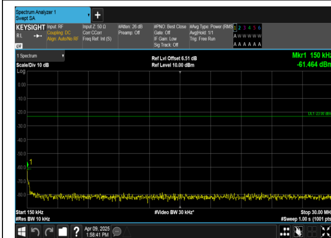
Band5-3MHz-QPSK-20635-1RB#14-0.15~30-PASS
