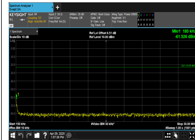
Band5-3MHz-16QAM-20635-1RB#0-0.15~30-PASS
