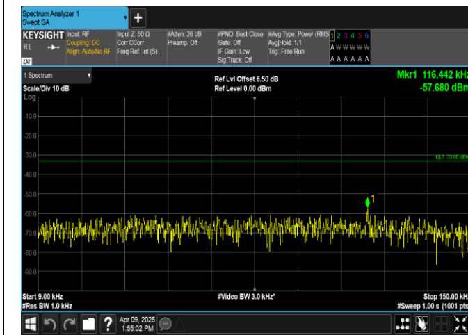
Band5-3MHz-16QAM-20525-15RB#0-0.009~0.15-PASS
