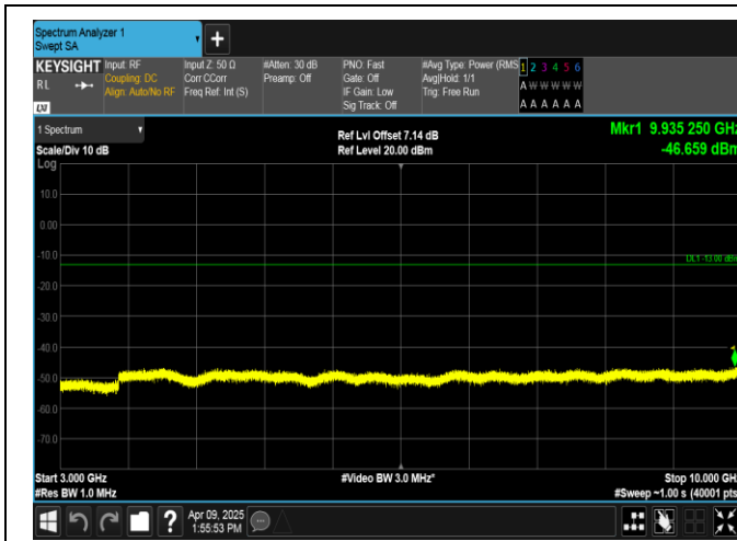
Band5-3MHz-16QAM-20525-15RB#0-3000~10000-PASS
