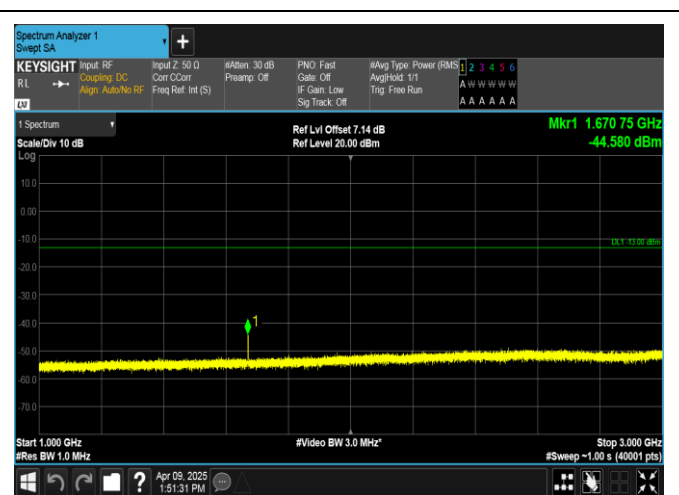
Band5-3MHz-16QAM-20525-1RB#0-1000~3000-PASS
