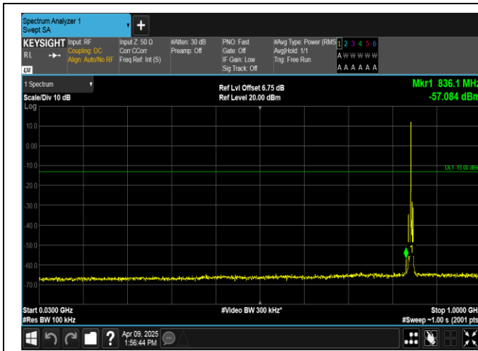
Band5-3MHz-QPSK-20635-1RB#0-30~1000-PASS
