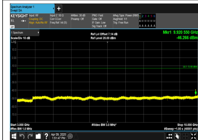
Band5-3MHz-16QAM-20525-1RB#0-3000~10000-PASS
