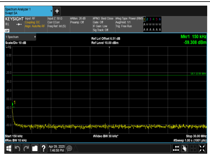
Band5-3MHz-16QAM-20415-1RB#14-0.15~30-PASS
