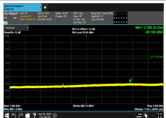
Band5-3MHz-QPSK-20635-15RB#0-1000~3000-PASS
