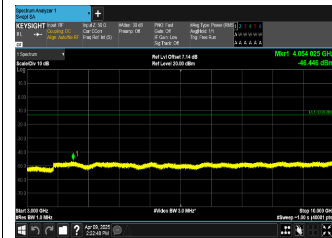
Band5-5MHz-QPSK-20425-1RB#0-3000~10000-PASS
