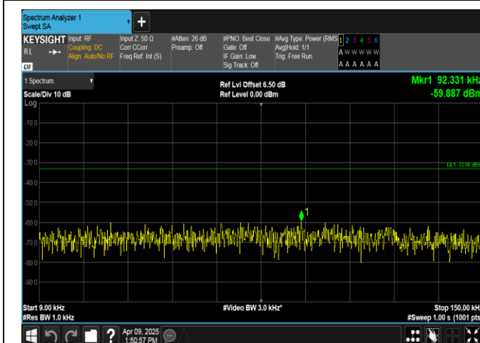
Band5-3MHz-16QAM-20525-1RB#0-0.009~0.15-PASS
