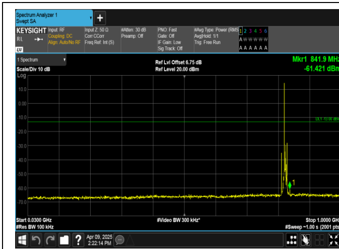
Band5-5MHz-QPSK-20425-1RB#0-30~1000-PASS
