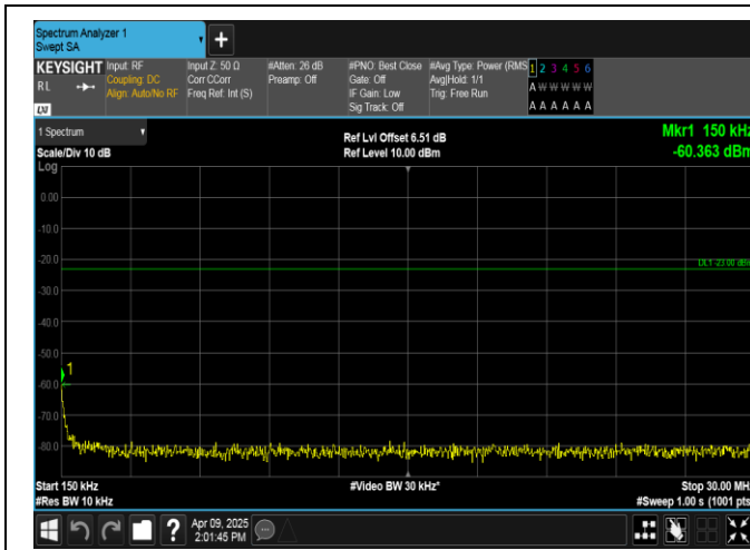
Band5-3MHz-16QAM-20635-15RB#0-0.15~30-PASS
