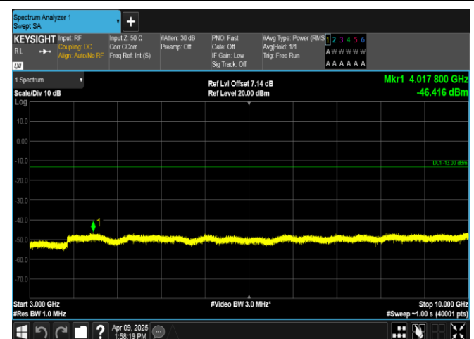
Band5-3MHz-16QAM-20635-1RB#0-3000~10000-PASS
