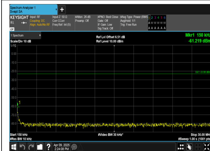
Band5-5MHz-QPSK-20425-1RB#24-0.15~30-PASS
