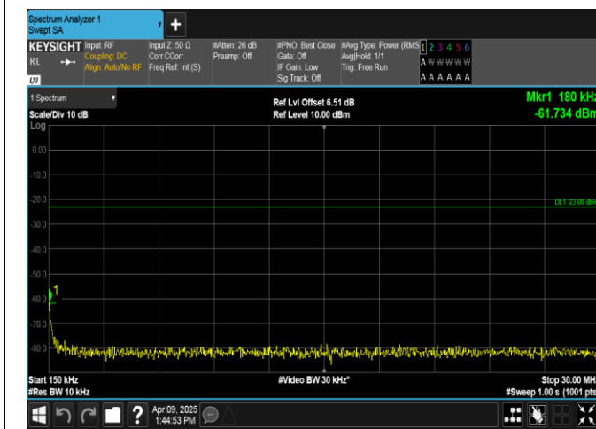
Band5-3MHz-16QAM-20415-1RB#0-0.15~30-PASS
