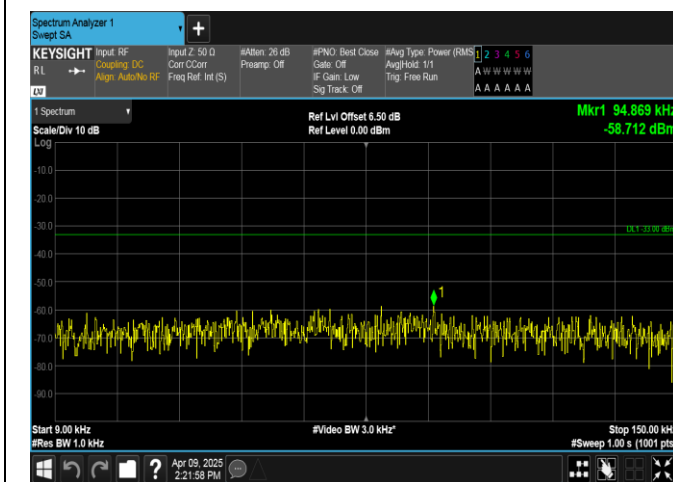
Band5-5MHz-QPSK-20425-1RB#0-0.009~0.15-PASS
