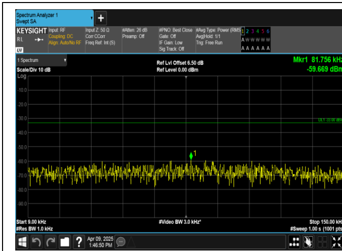
Band5-3MHz-16QAM-20415-1RB#14-0.009~0.15-PASS
