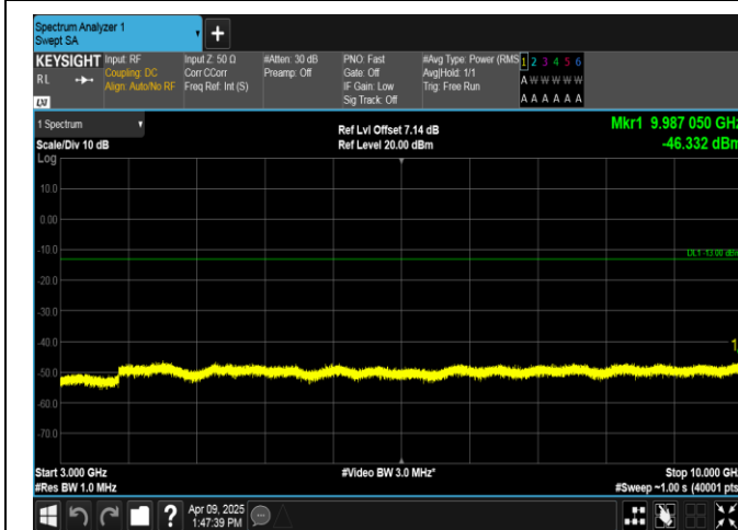
Band5-3MHz-16QAM-20415-1RB#14-3000~10000-PASS
