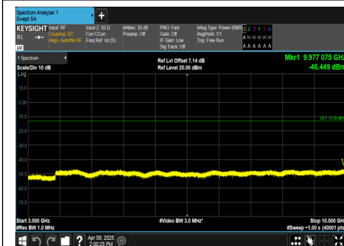
Band5-3MHz-16QAM-20635-1RB#14-3000~10000-PASS
