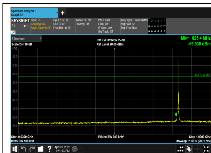
Band5-3MHz-16QAM-20525-1RB#0-30~1000-PASS
