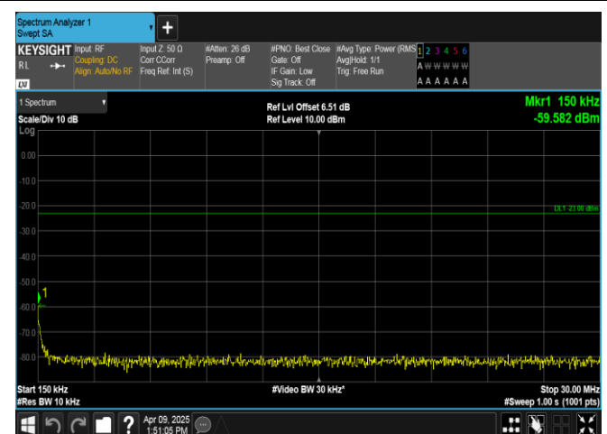
Band5-3MHz-16QAM-20525-1RB#0-0.15~30-PASS
