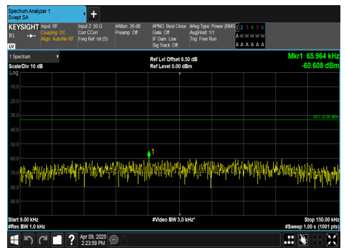
Band5-5MHz-QPSK-20425-1RB#24-0.009~0.15-PASS
