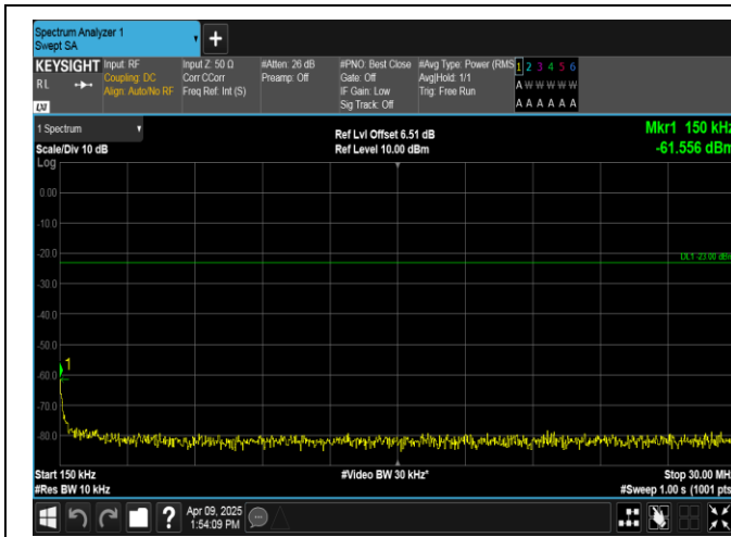
Band5-3MHz-QPSK-20525-15RB#0-0.15~30-PASS
