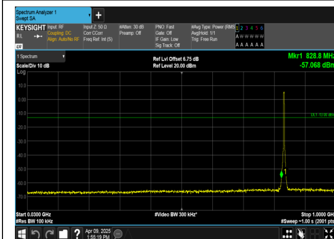
Band5-3MHz-16QAM-20525-15RB#0-30~1000-PASS
