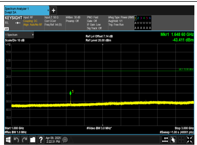
Band5-5MHz-QPSK-20425-1RB#0-1000~3000-PASS
