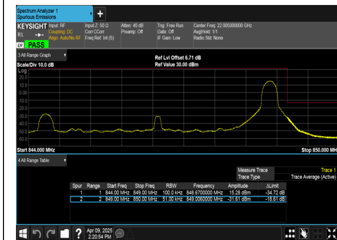
Band5-5MHz-16QAM-20625-1RB#24-PASS
