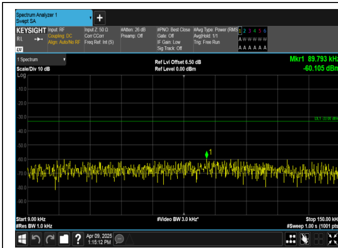
Band5-1.4MHz-QPSK-20525-1RB#5-0.009~0.15-PASS
