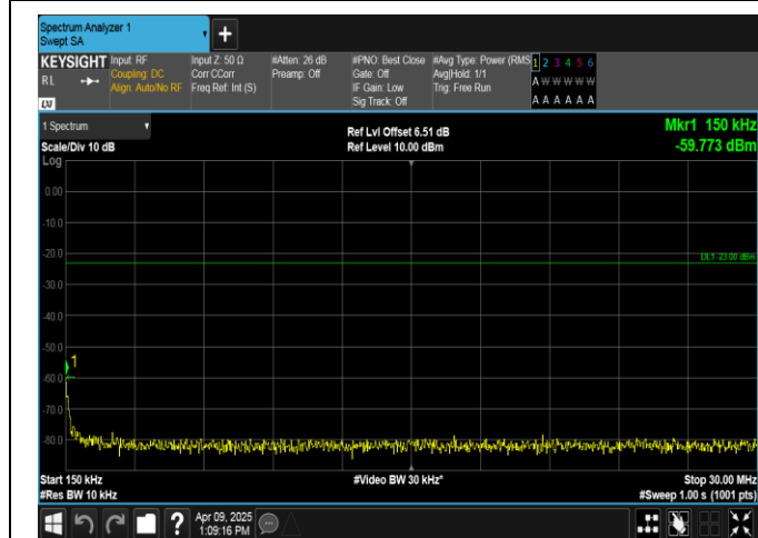
Band5-1.4MHz-QPSK-20407-1RB#5-0.15~30-PASS
