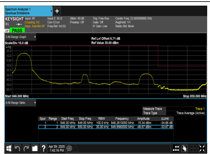
Band5-3MHz-16QAM-20635-1RB#0-PASS
