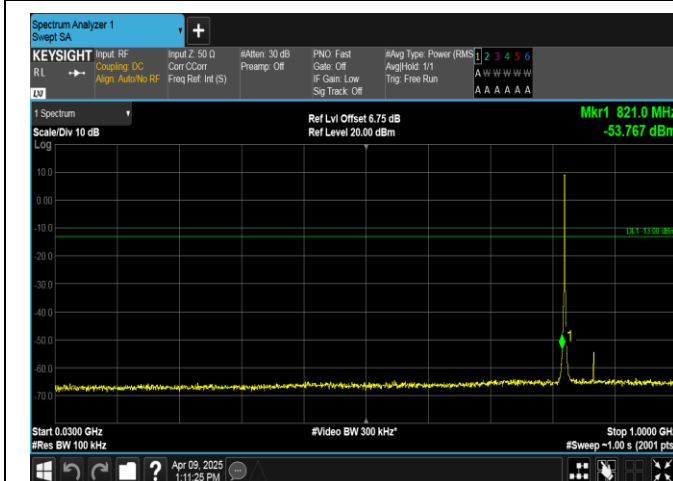
Band5-1.4MHz-QPSK-20407-6RB#0-30~1000-PASS
