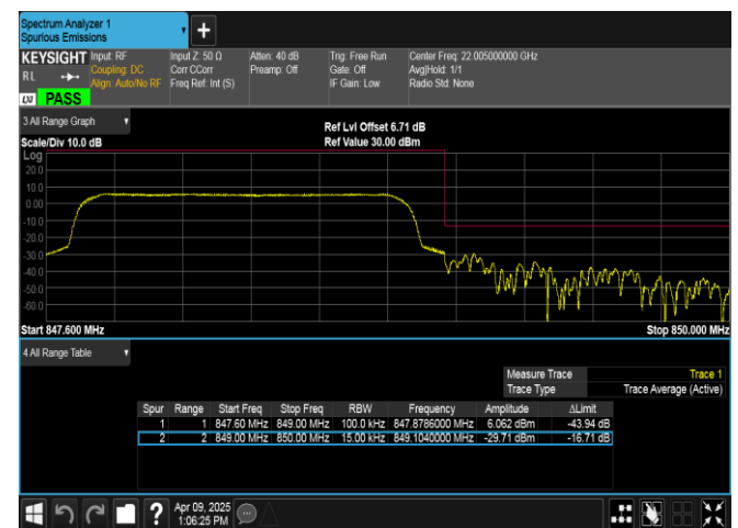
Band5-1.4MHz-QPSK-20643-6RB#0-PASS
