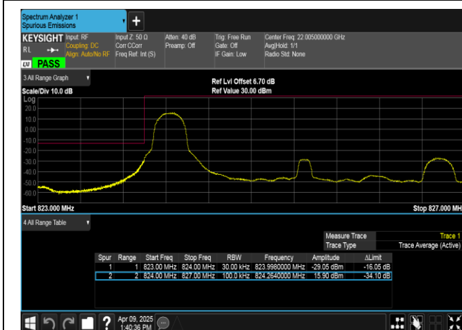
Band5-3MHz-16QAM-20415-1RB#0-PASS
