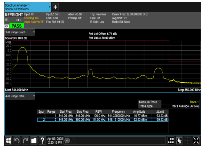
Band5-5MHz-QPSK-20625-1RB#0-PASS
