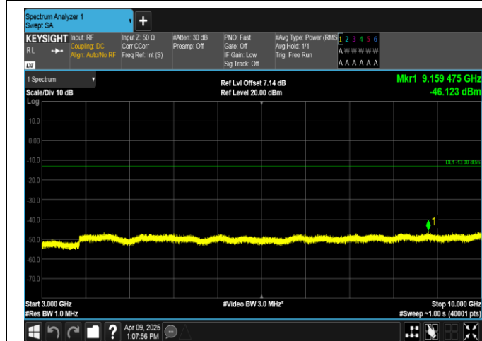
Band5-1.4MHz-QPSK-20407-1RB#0-3000~10000-PASS
