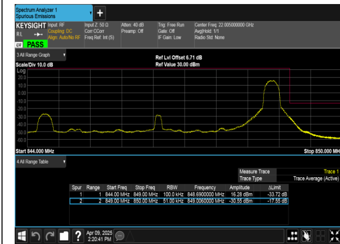
Band5-5MHz-QPSK-20625-1RB#24-PASS
