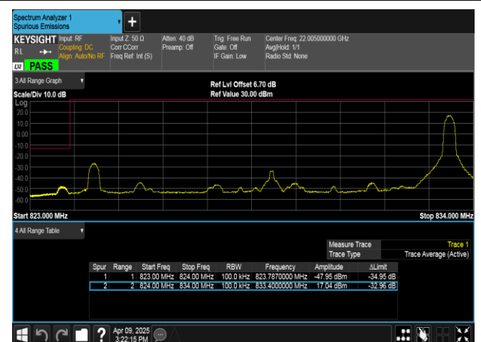
Band5-10MHz-QPSK-20450-1RB#49-PASS
