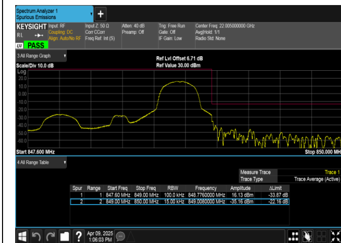
Band5-1.4MHz-QPSK-20643-1RB#5-PASS
