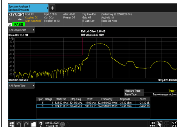
Band5-1.4MHz-16QAM-20407-1RB#0-PASS
