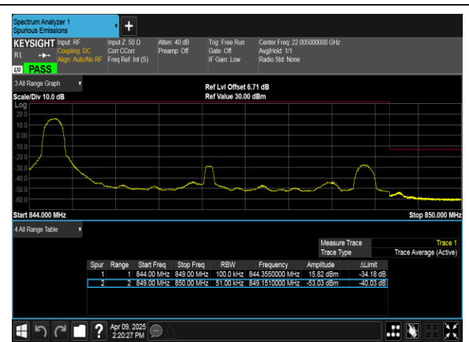
Band5-5MHz-16QAM-20625-1RB#0-PASS
