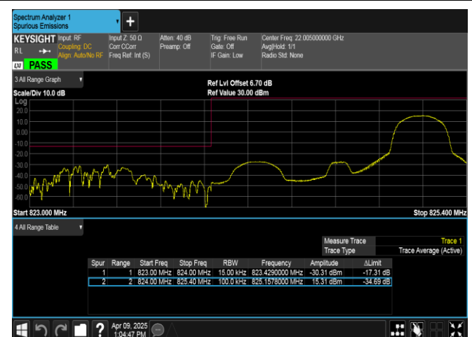
Band5-1.4MHz-16QAM-20407-1RB#5-PASS
