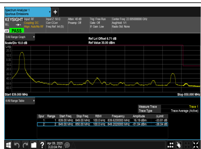
Band5-10MHz-16QAM-20600-1RB#0-PASS
