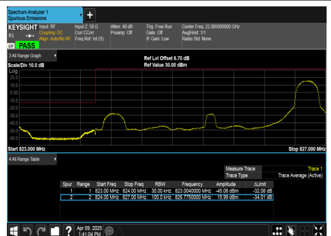
Band5-3MHz-16QAM-20415-1RB#14-PASS
