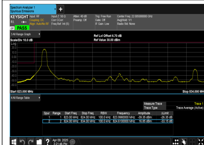
Band5-10MHz-QPSK-20450-1RB#0-PASS
