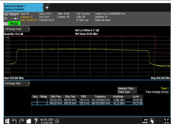
Band5-10MHz-16QAM-20600-50RB#0-PASS
