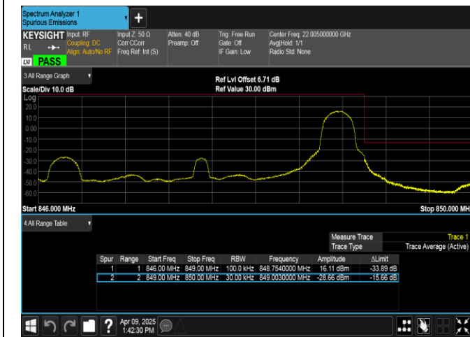
Band5-3MHz-QPSK-20635-1RB#14-PASS
