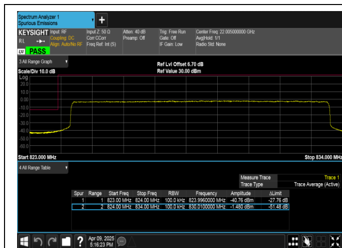
Band5-10MHz-16QAM-20450-50RB#0-PASS
