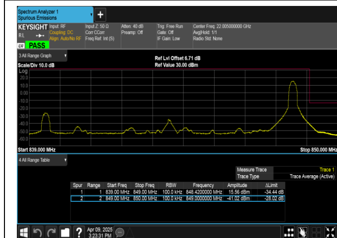
Band5-10MHz-16QAM-20600-1RB#49-PASS
