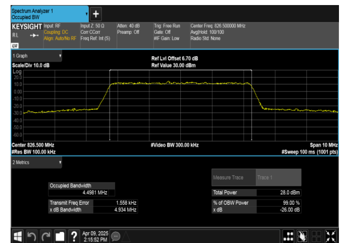
Band5-5MHz-16QAM-20425-25RB#0-PASS
