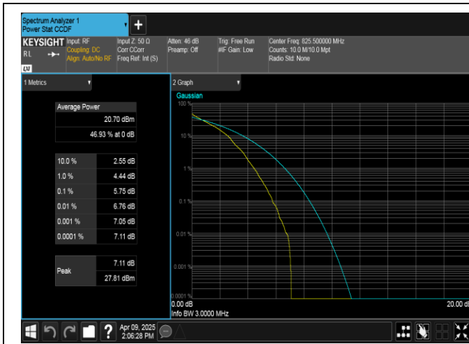
Band5-3MHz-QPSK-20415-1RB#0-PASS
