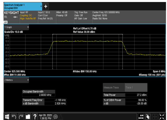
Band5-3MHz-16QAM-20415-15RB#0-PASS
