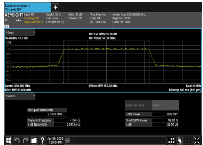
Band5-3MHz-QPSK-20525-15RB#0-PASS
