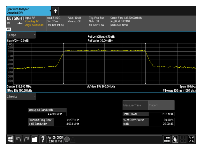
Band5-5MHz-QPSK-20525-25RB#0-PASS
