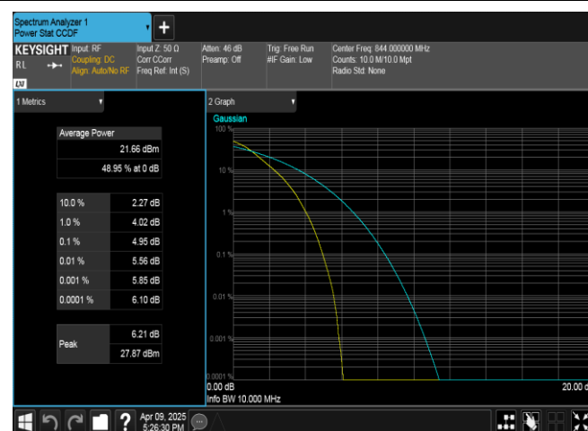
Band5-10MHz-QPSK-20600-50RB#0-PASS
