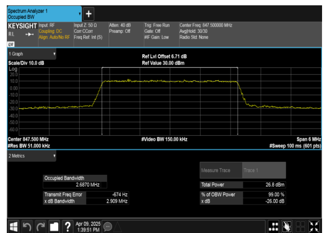
Band5-3MHz-16QAM-20635-15RB#0-PASS
