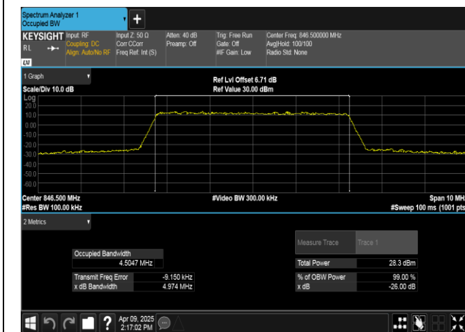
Band5-5MHz-QPSK-20625-25RB#0-PASS
