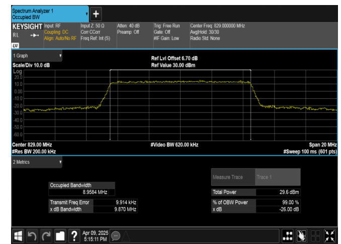
Band5-10MHz-16QAM-20450-50RB#0-PASS
