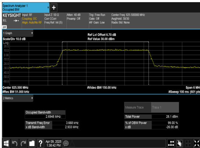
Band5-3MHz-QPSK-20415-15RB#0-PASS
