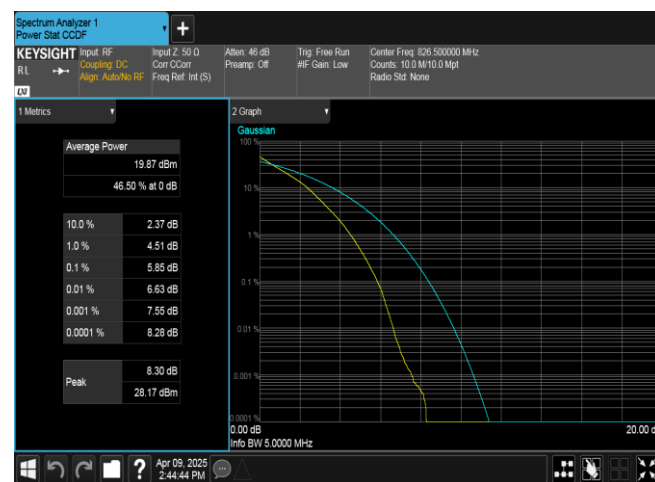
Band5-5MHz-QPSK-20425-25RB#0-PASS
