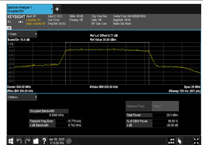
Band5-10MHz-16QAM-20600-50RB#0-PASS
