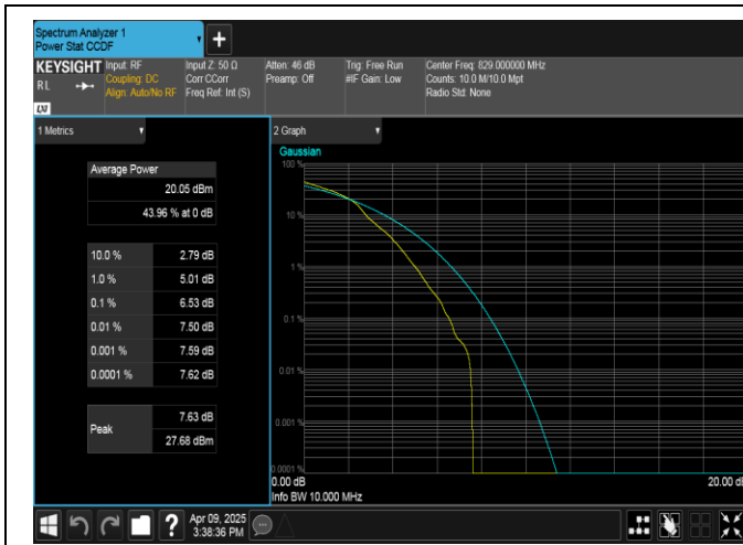
Band5-10MHz-16QAM-20450-1RB#0-PASS
