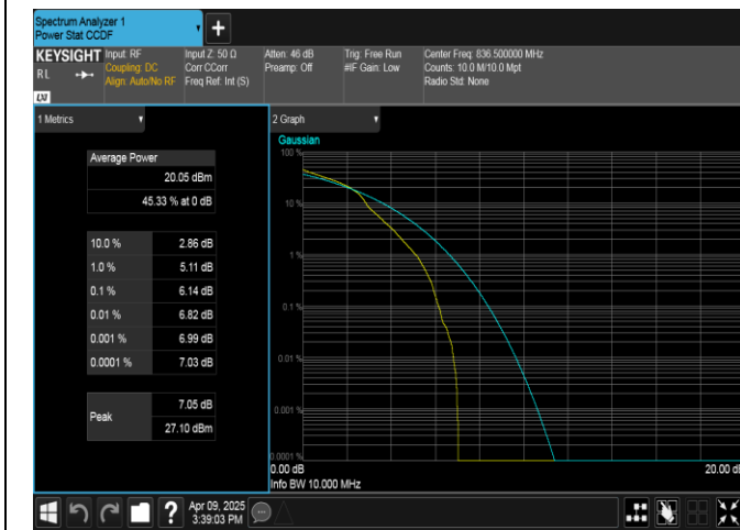
Band5-10MHz-16QAM-20525-1RB#0-PASS
