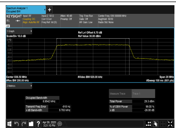
Band5-10MHz-QPSK-20525-50RB#0-PASS
