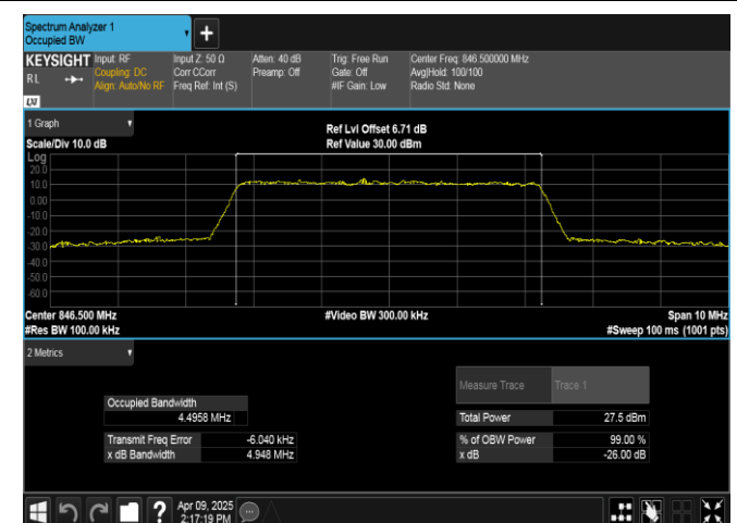
Band5-5MHz-16QAM-20625-25RB#0-PASS
