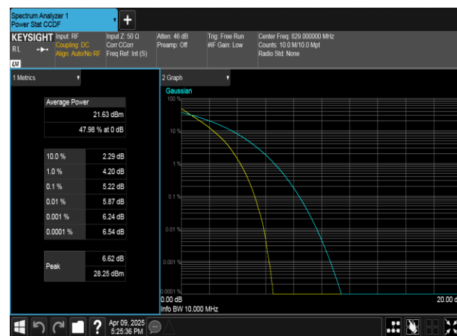
Band5-10MHz-QPSK-20450-50RB#0-PASS
