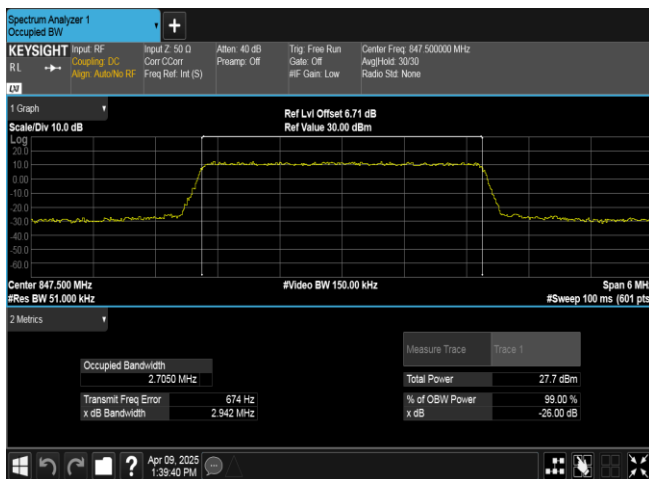
Band5-3MHz-QPSK-20635-15RB#0-PASS
