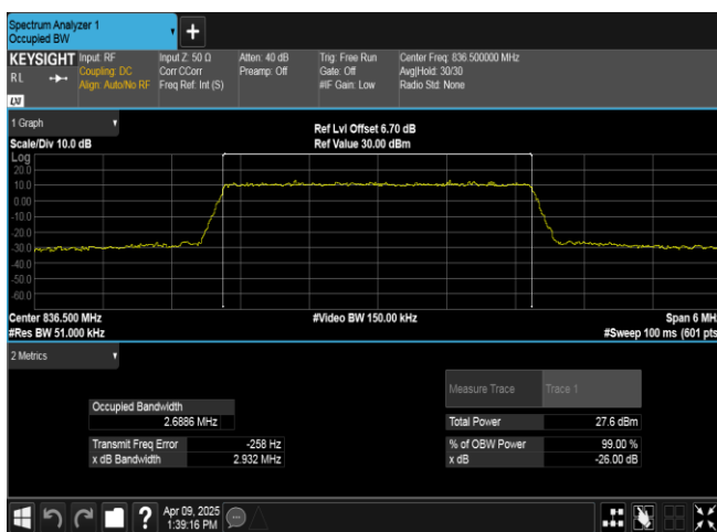
Band5-3MHz-16QAM-20525-15RB#0-PASS
