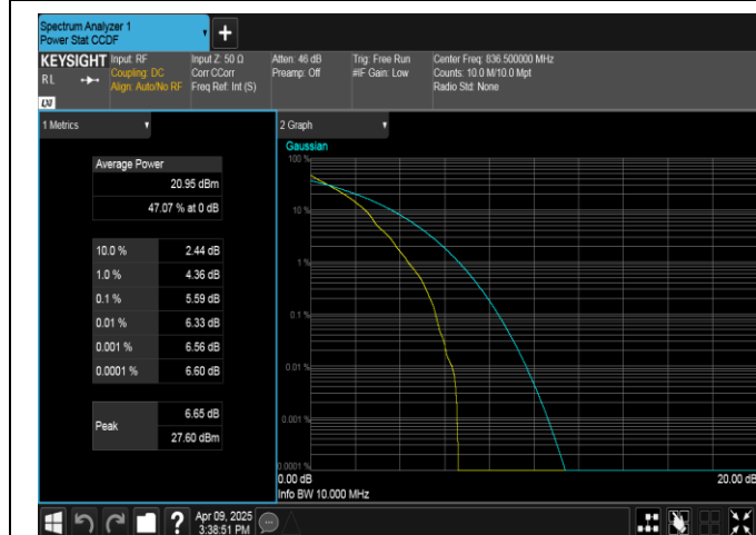
Band5-10MHz-QPSK-20525-1RB#0-PASS
