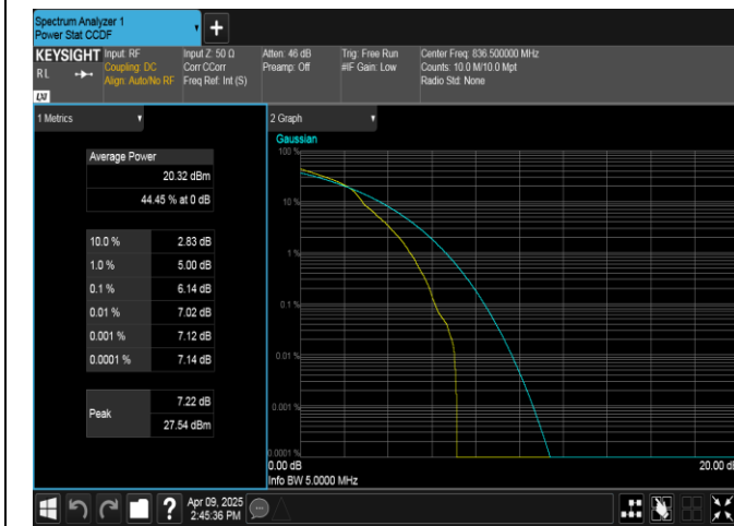
Band5-5MHz-16QAM-20525-1RB#0-PASS
