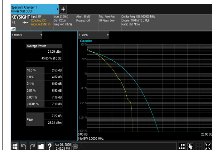
Band5-5MHz-QPSK-20525-1RB#0-PASS
