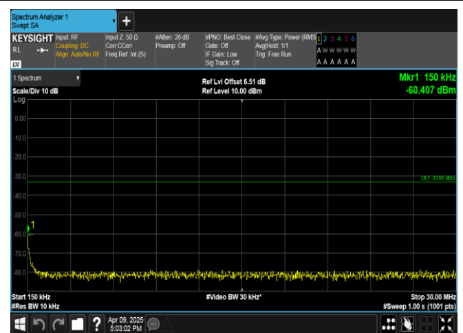
Band4-20MHz-16QAM-20175-100RB#0-0.15~30-PASS
