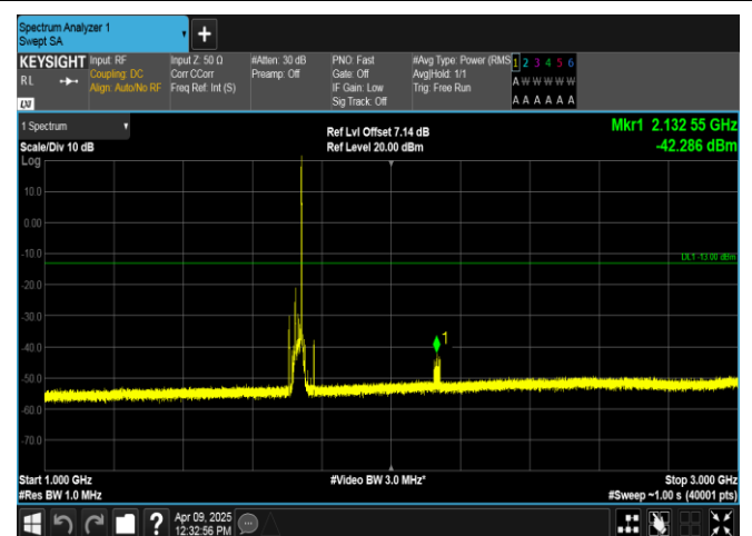
Band4-20MHz-QPSK-20175-1RB#99-1000~3000-PASS
