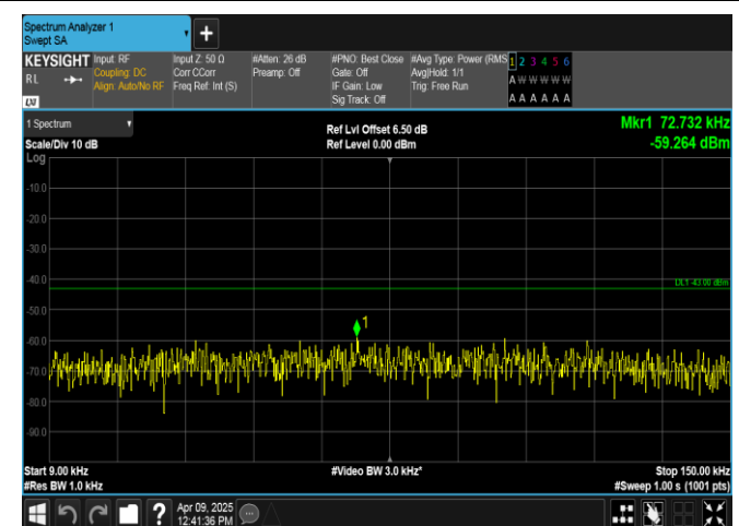
Band4-20MHz-QPSK-20300-1RB#99-0.009~0.15-PASS
