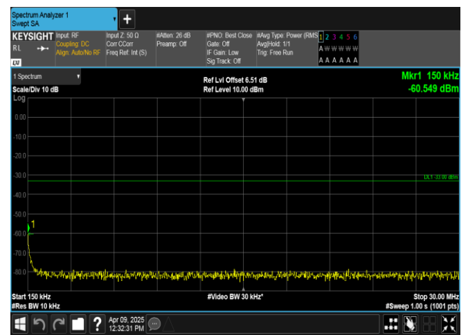
Band4-20MHz-QPSK-20175-1RB#99-0.15~30-PASS
