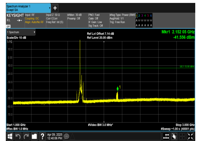
Band4-20MHz-QPSK-20300-1RB#0-1000~3000-PASS
