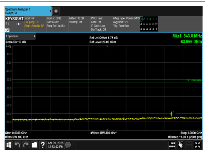
Band4-20MHz-16QAM-20175-1RB#99-30~1000-PASS
