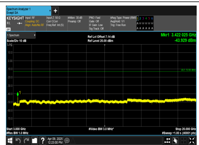
Band4-20MHz-16QAM-20050-1RB#0-3000~20000-PASS
