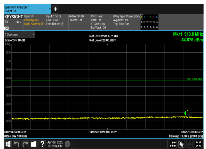
Band4-20MHz-16QAM-20050-100RB#0-30~1000-PASS
