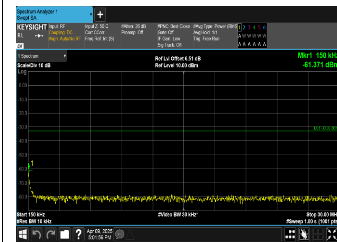
Band4-20MHz-16QAM-20050-100RB#0-0.15~30-PASS
