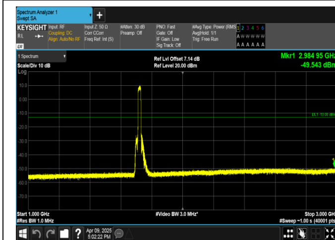
Band4-20MHz-16QAM-20050-100RB#0-1000~3000-PASS
