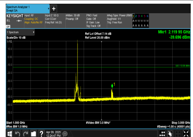
Band4-20MHz-16QAM-20050-1RB#99-1000~3000-PASS
