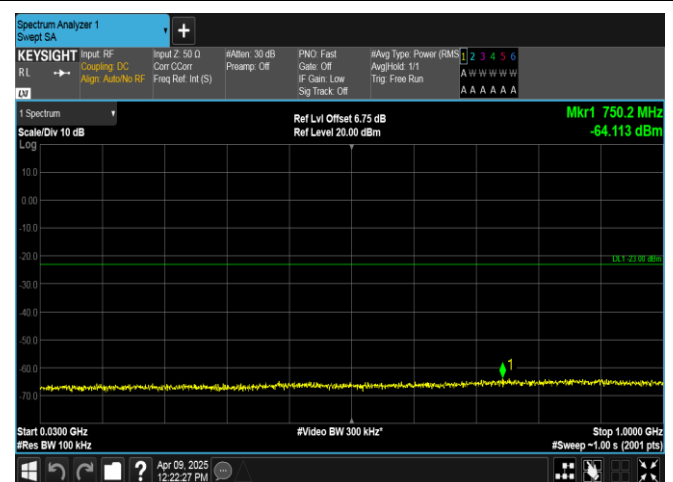
Band4-20MHz-16QAM-20050-1RB#0-30~1000-PASS
