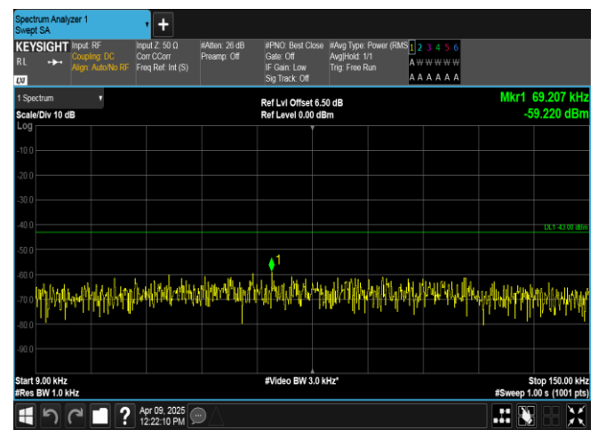
Band4-20MHz-16QAM-20050-1RB#0-0.009~0.15-PASS
