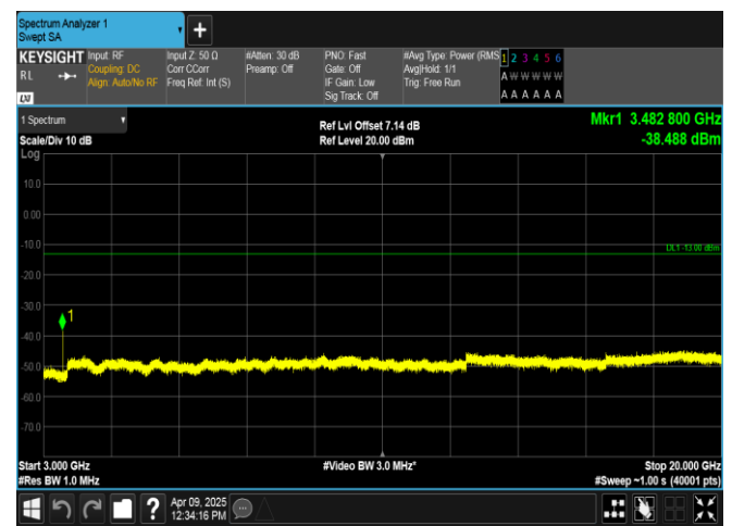
Band4-20MHz-16QAM-20175-1RB#99-3000~20000-PASS
