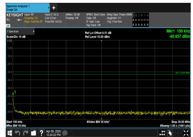
Band4-20MHz-16QAM-20050-1RB#99-0.15~30-PASS
