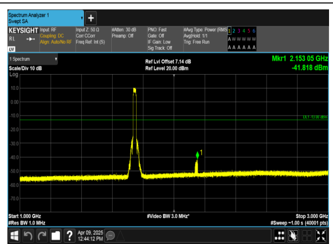
Band4-20MHz-QPSK-20300-100RB#0-1000~3000-PASS
