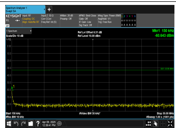
Band4-20MHz-QPSK-20300-1RB#0-0.15~30-PASS
