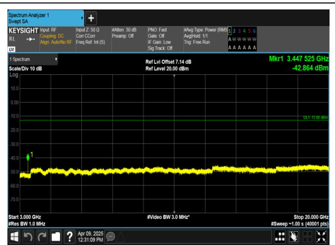
Band4-20MHz-QPSK-20175-1RB#0-3000~20000-PASS
