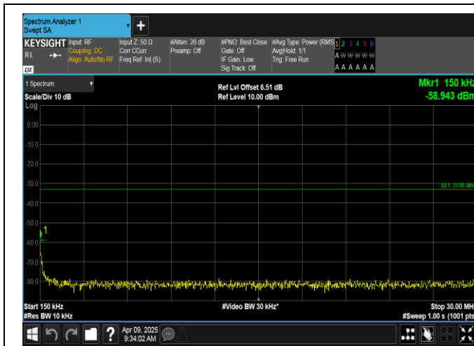
Band4-10MHz-QPSK-20000-1RB#49-0.15~30-PASS
