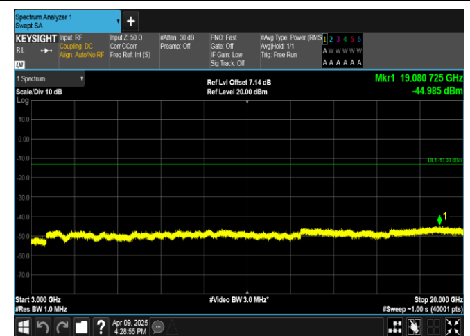
Band4-10MHz-16QAM-20000-50RB#0-3000~20000-PASS
