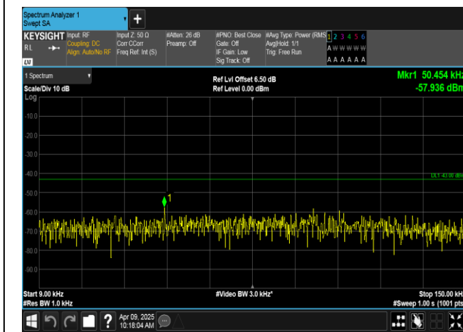
Band4-10MHz-16QAM-20350-1RB#49-0.009~0.15-PASS
