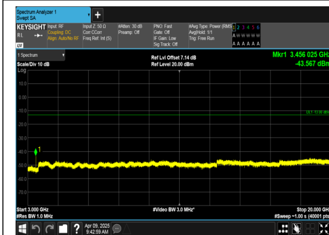
Band4-10MHz-16QAM-20175-1RB#0-3000~20000-PASS
