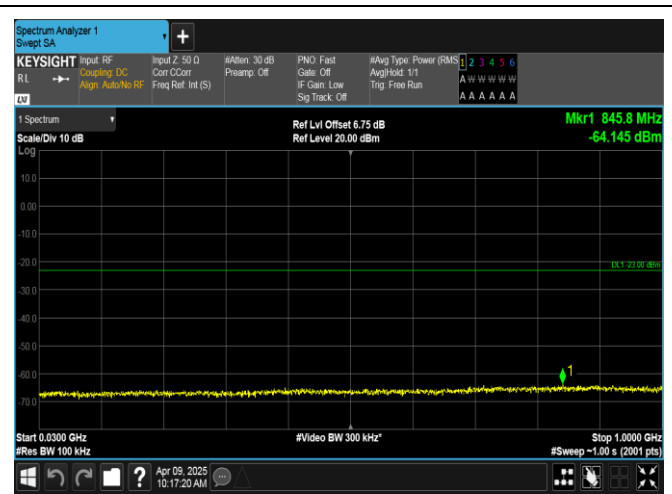
Band4-10MHz-QPSK-20350-1RB#49-30~1000-PASS
