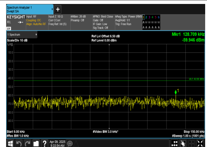
Band4-10MHz-QPSK-20000-1RB#49-0.009~0.15-PASS
