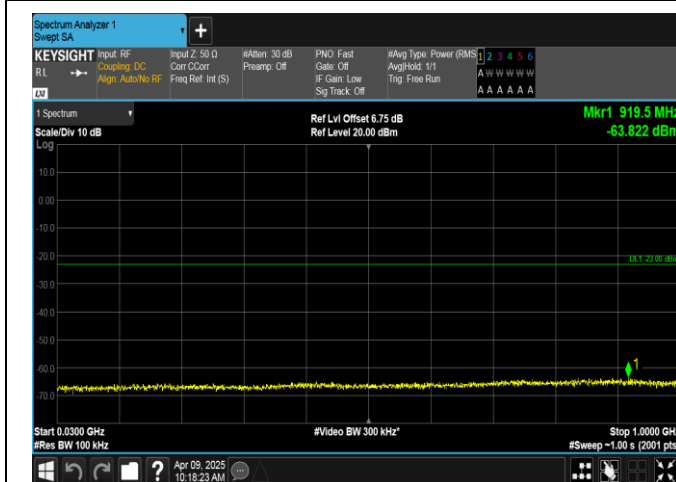
Band4-10MHz-16QAM-20350-1RB#49-30~1000-PASS
