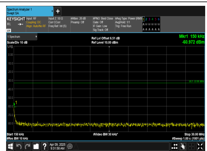
Band4-10MHz-QPSK-20000-1RB#0-0.15~30-PASS
