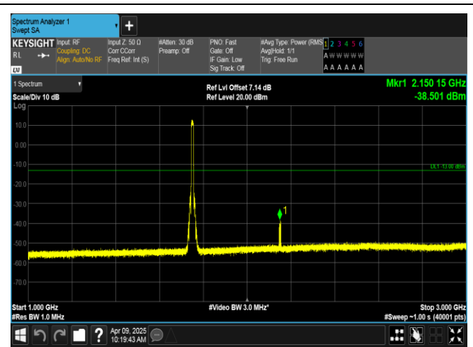
Band4-10MHz-QPSK-20350-50RB#0-1000~3000-PASS
