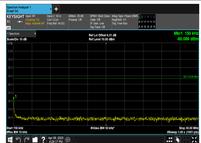
Band4-10MHz-16QAM-20175-50RB#0-0.15~30-PASS
