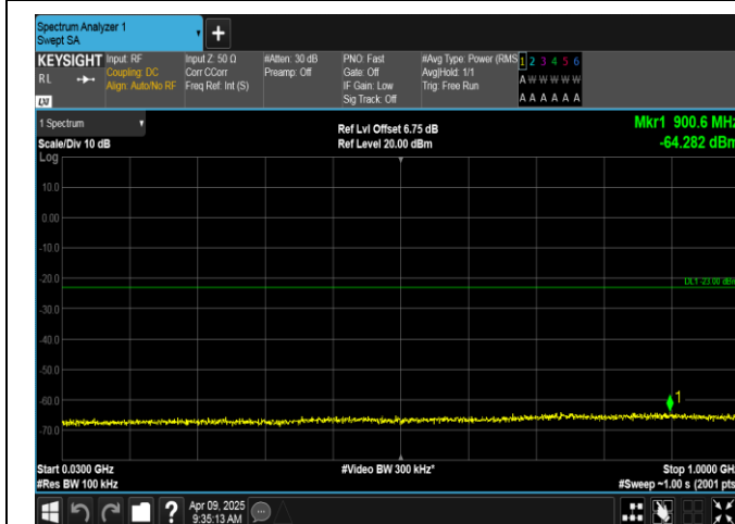
Band4-10MHz-16QAM-20000-1RB#49-30~1000-PASS
