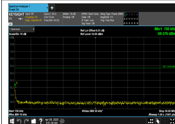
Band4-10MHz-16QAM-20350-1RB#0-0.15~30-PASS
