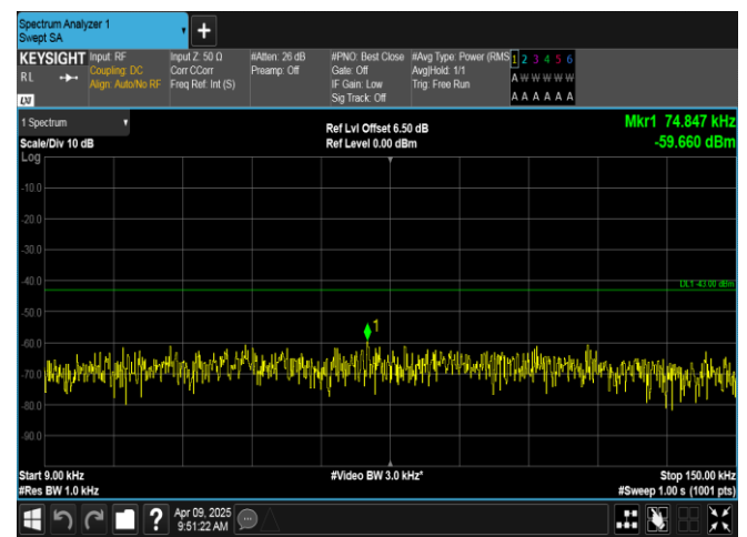
Band4-10MHz-16QAM-20350-1RB#0-0.009~0.15-PASS
