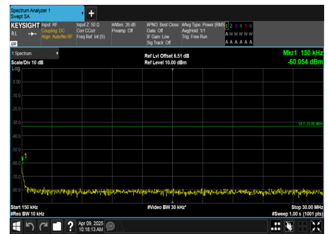
Band4-10MHz-16QAM-20350-1RB#49-0.15~30-PASS
