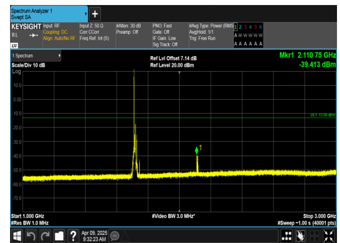
Band4-10MHz-QPSK-20000-1RB#0-1000~3000-PASS
