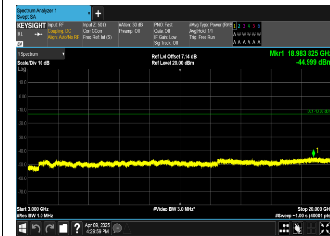
Band4-10MHz-16QAM-20175-50RB#0-3000~20000-PASS
