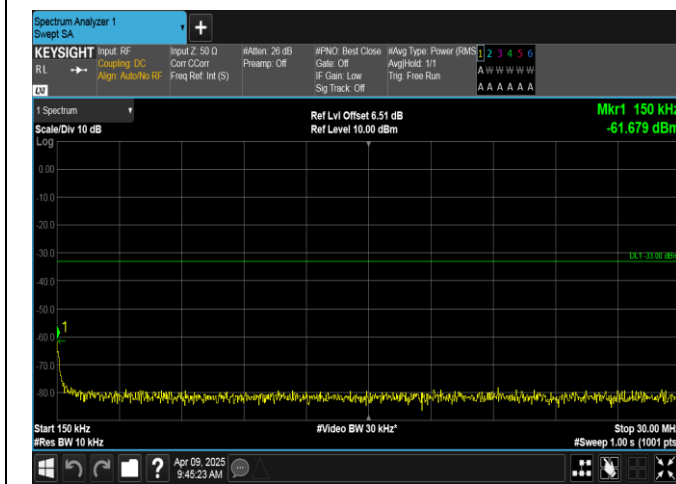
Band4-10MHz-QPSK-20175-50RB#0-0.15~30-PASS
