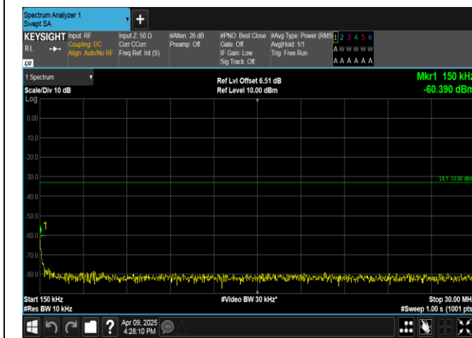
Band4-10MHz-16QAM-20000-50RB#0-0.15~30-PASS
