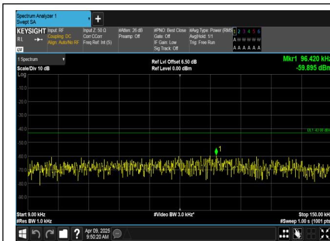
Band4-10MHz-QPSK-20350-1RB#0-0.009~0.15-PASS
