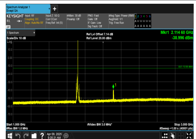
Band4-10MHz-16QAM-20000-1RB#49-1000~3000-PASS
