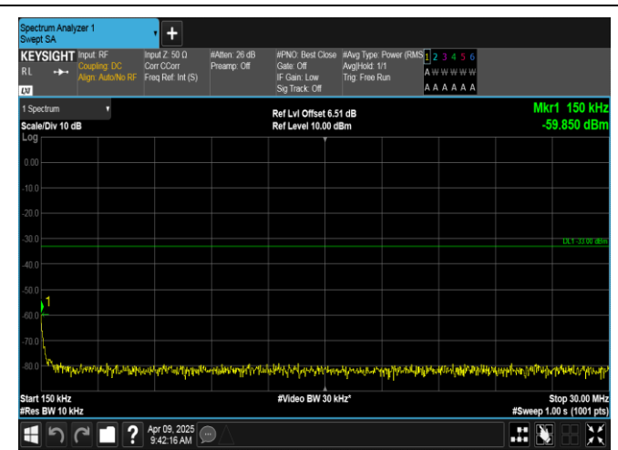
Band4-10MHz-16QAM-20175-1RB#0-0.15~30-PASS
