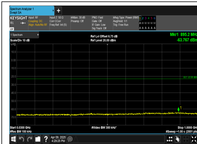
Band4-10MHz-16QAM-20175-50RB#0-30~1000-PASS
