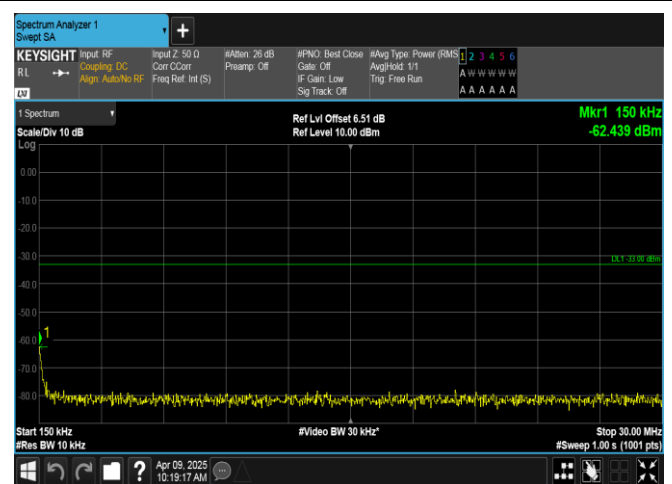
Band4-10MHz-QPSK-20350-50RB#0-0.15~30-PASS
