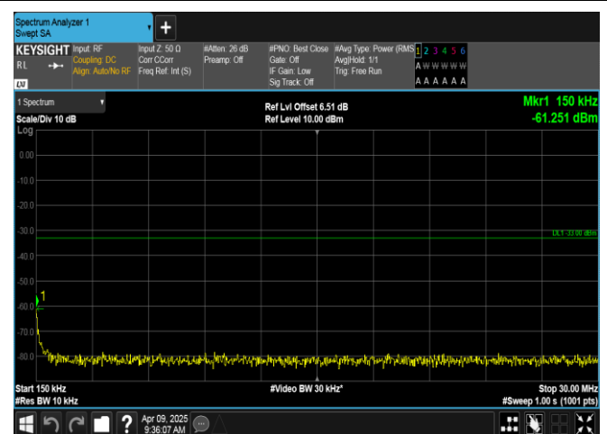
Band4-10MHz-QPSK-20000-50RB#0-0.15~30-PASS
