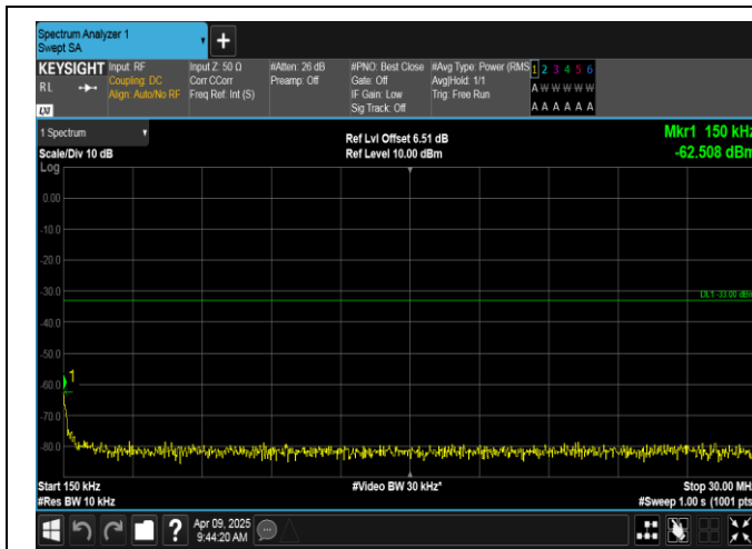
Band4-10MHz-16QAM-20175-1RB#49-0.15~30-PASS
