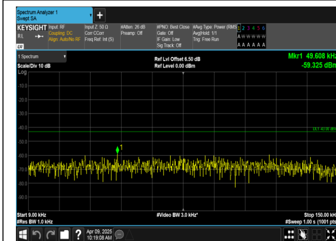
Band4-10MHz-QPSK-20350-50RB#0-0.009~0.15-PASS
