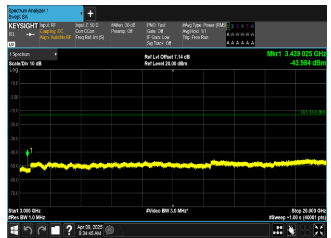
Band4-10MHz-QPSK-20000-1RB#49-3000~20000-PASS
