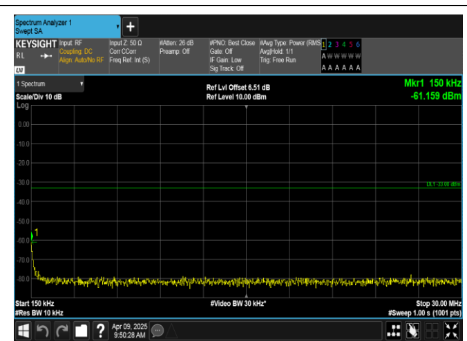
Band4-10MHz-QPSK-20350-1RB#0-0.15~30-PASS
