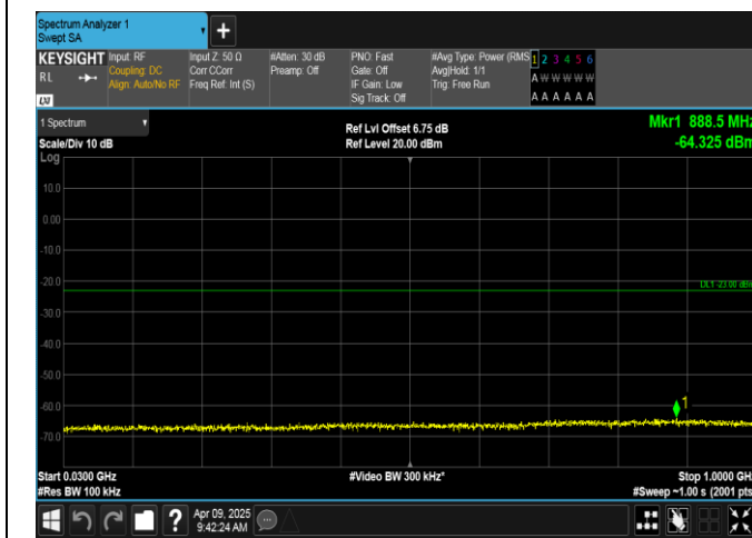
Band4-10MHz-16QAM-20175-1RB#0-30~1000-PASS
