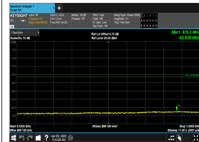
Band4-10MHz-QPSK-20000-1RB#0-30~1000-PASS
