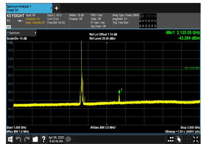
Band4-10MHz-16QAM-20175-1RB#0-1000~3000-PASS
