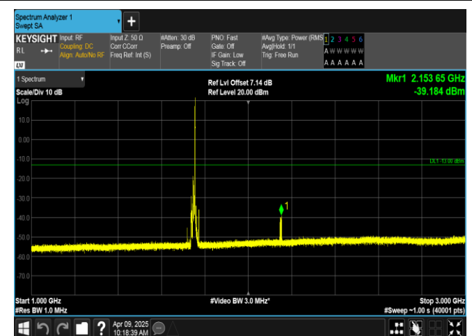
Band4-10MHz-16QAM-20350-1RB#49-1000~3000-PASS
