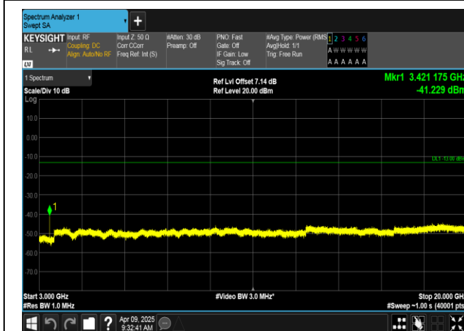
Band4-10MHz-QPSK-20000-1RB#0-3000~20000-PASS
