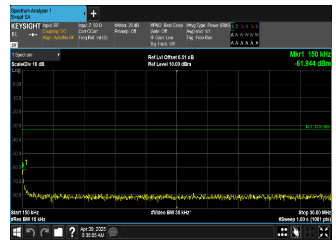
Band4-10MHz-16QAM-20000-1RB#49-0.15~30-PASS
