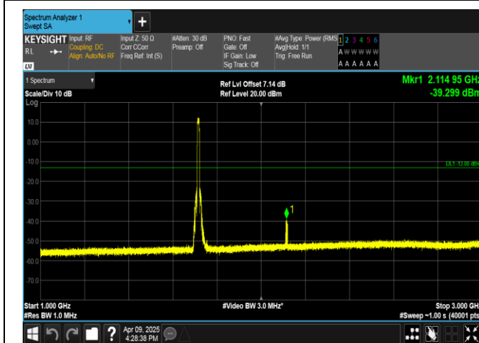
Band4-10MHz-16QAM-20000-50RB#0-1000~3000-PASS
