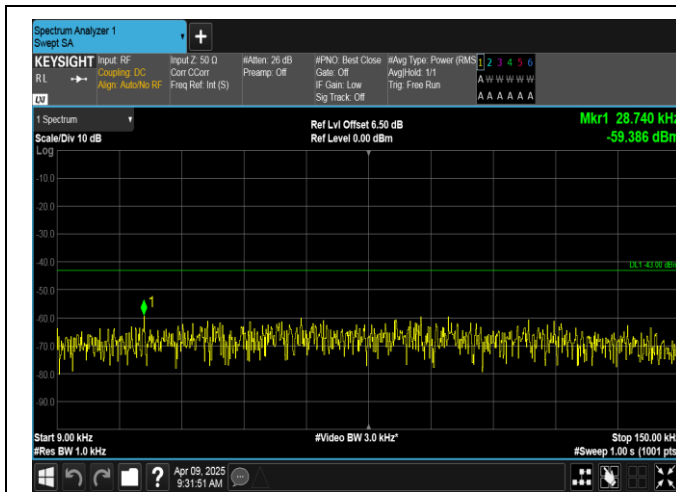
Band4-10MHz-QPSK-20000-1RB#0-0.009~0.15-PASS
