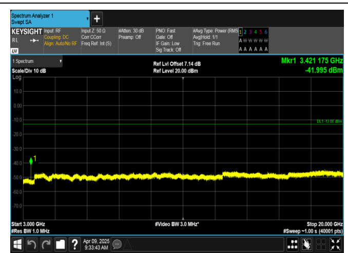
Band4-10MHz-16QAM-20000-1RB#0-3000~20000-PASS
