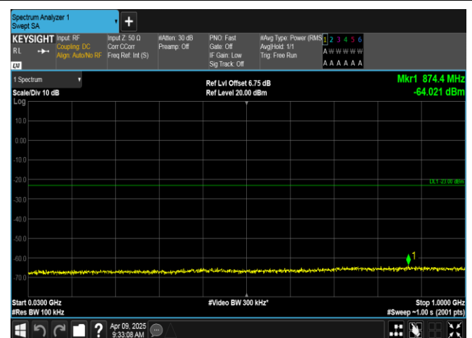
Band4-10MHz-16QAM-20000-1RB#0-30~1000-PASS
