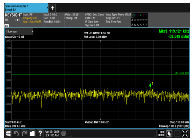
Band4-10MHz-QPSK-20175-1RB#0-0.009~0.15-PASS
