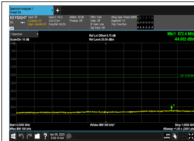
Band4-10MHz-QPSK-20000-50RB#0-30~1000-PASS
