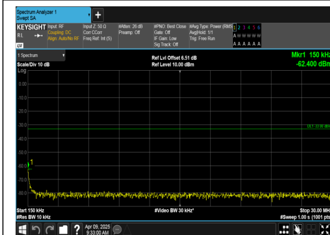
Band4-10MHz-16QAM-20000-1RB#0-0.15~30-PASS
