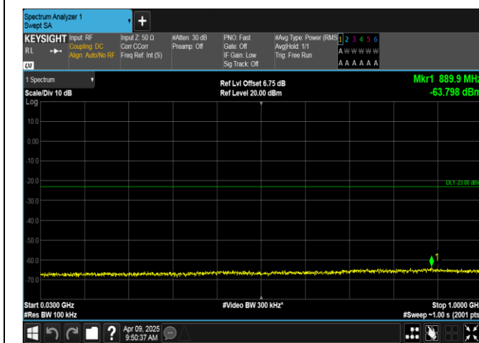
Band4-10MHz-QPSK-20350-1RB#0-30~1000-PASS
