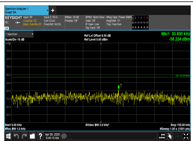
Band4-10MHz-QPSK-20175-50RB#0-0.009~0.15-PASS
