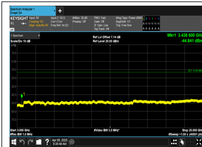
Band4-10MHz-16QAM-20000-1RB#49-3000~20000-PASS
