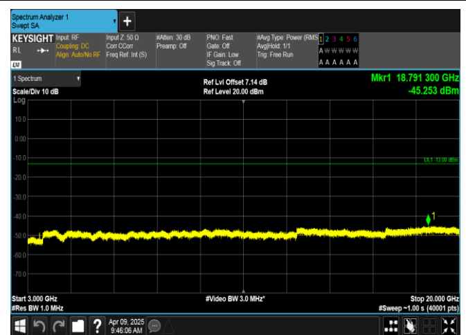
Band4-10MHz-QPSK-20175-50RB#0-3000~20000-PASS
