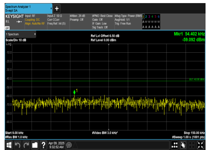
Band4-10MHz-16QAM-20000-1RB#0-0.009~0.15-PASS
