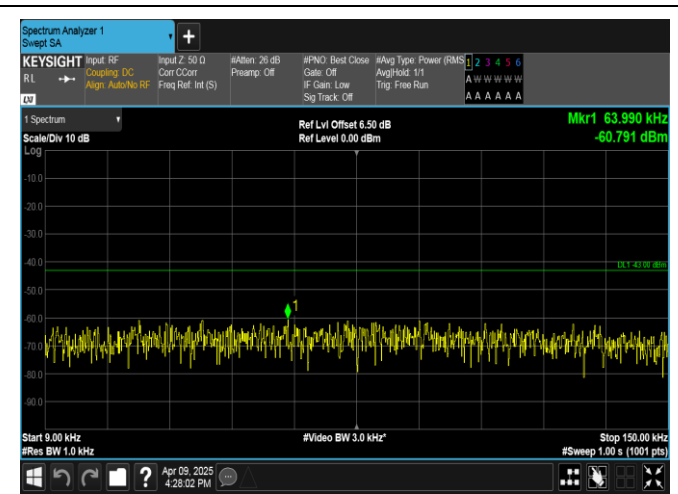
Band4-10MHz-16QAM-20000-50RB#0-0.009~0.15-PASS
