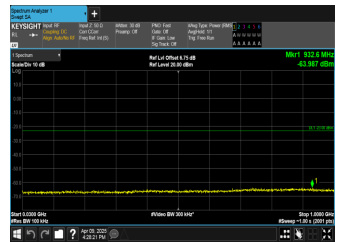
Band4-10MHz-16QAM-20000-50RB#0-30~1000-PASS
