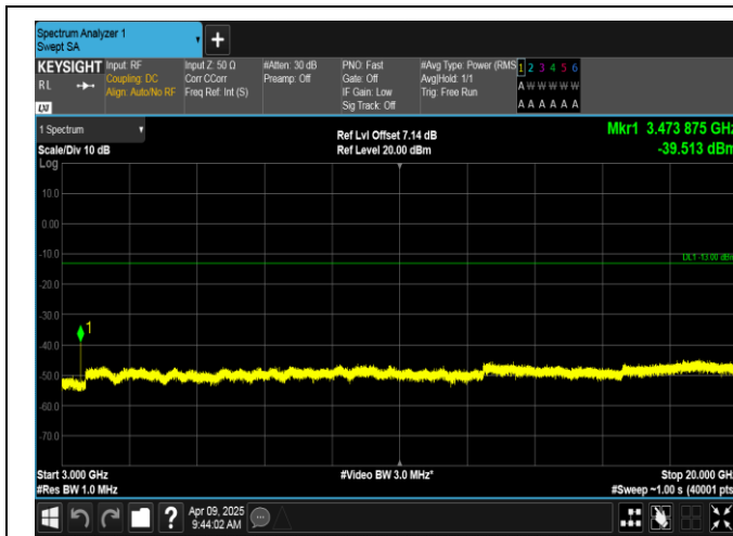
Band4-10MHz-QPSK-20175-1RB#49-3000~20000-PASS
