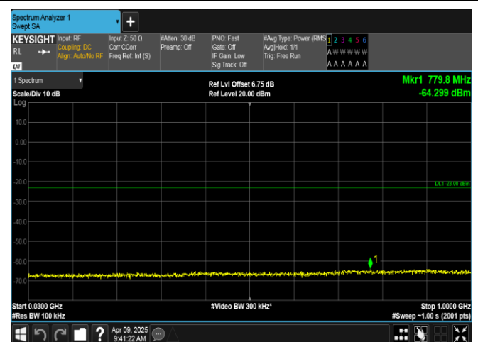
Band4-10MHz-QPSK-20175-1RB#0-30~1000-PASS
