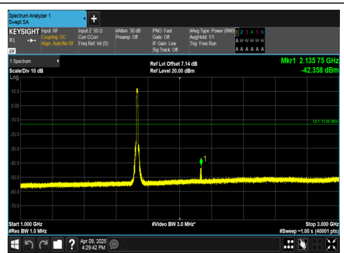
Band4-10MHz-16QAM-20175-50RB#0-1000~3000-PASS
