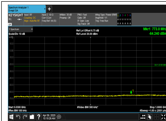
Band4-10MHz-QPSK-20350-50RB#0-30~1000-PASS
