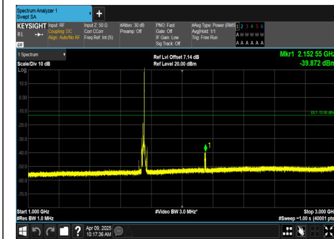
Band4-10MHz-QPSK-20350-1RB#49-1000~3000-PASS
