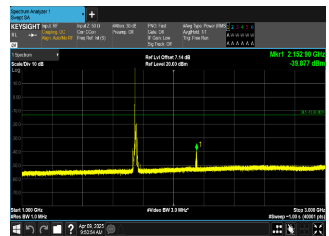
Band4-10MHz-QPSK-20350-1RB#0-1000~3000-PASS
