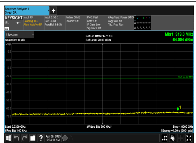
Band4-10MHz-QPSK-20000-1RB#49-30~1000-PASS
