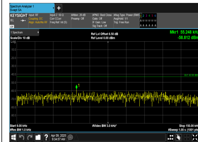
Band4-10MHz-16QAM-20000-1RB#49-0.009~0.15-PASS
