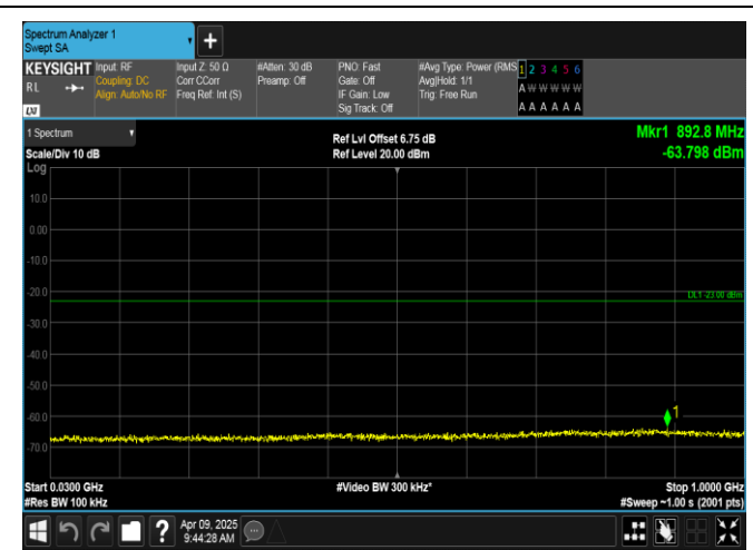
Band4-10MHz-16QAM-20175-1RB#49-30~1000-PASS
