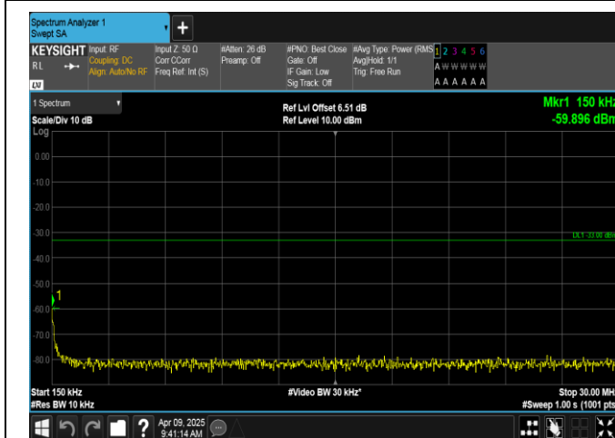
Band4-10MHz-QPSK-20175-1RB#0-0.15~30-PASS
