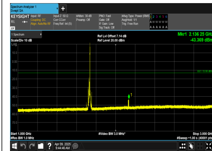
Band4-10MHz-16QAM-20175-1RB#49-1000~3000-PASS
