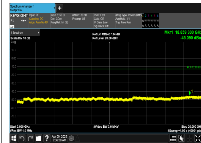
Band4-10MHz-QPSK-20000-50RB#0-3000~20000-PASS
