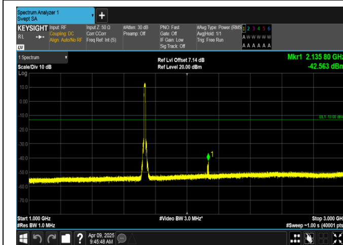
Band4-10MHz-QPSK-20175-50RB#0-1000~3000-PASS
