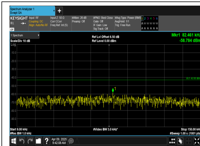
Band4-10MHz-16QAM-20175-1RB#0-0.009~0.15-PASS
