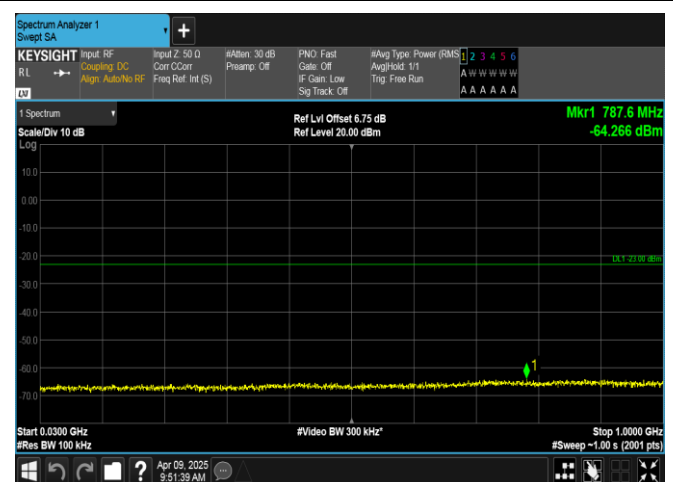
Band4-10MHz-16QAM-20350-1RB#0-30~1000-PASS
