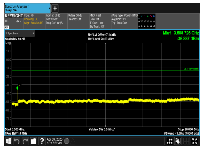
Band4-10MHz-QPSK-20350-1RB#49-3000~20000-PASS
