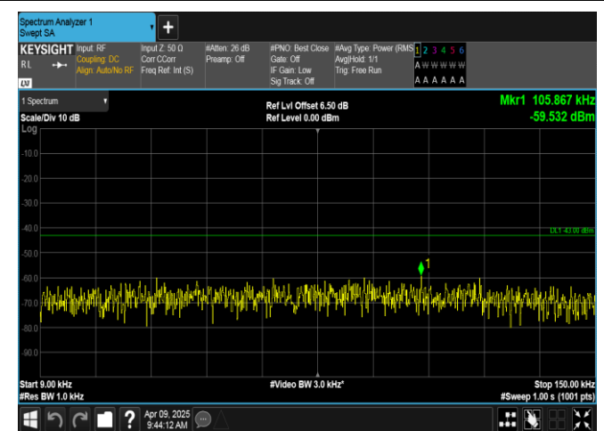
Band4-10MHz-16QAM-20175-1RB#49-0.009~0.15-PASS
