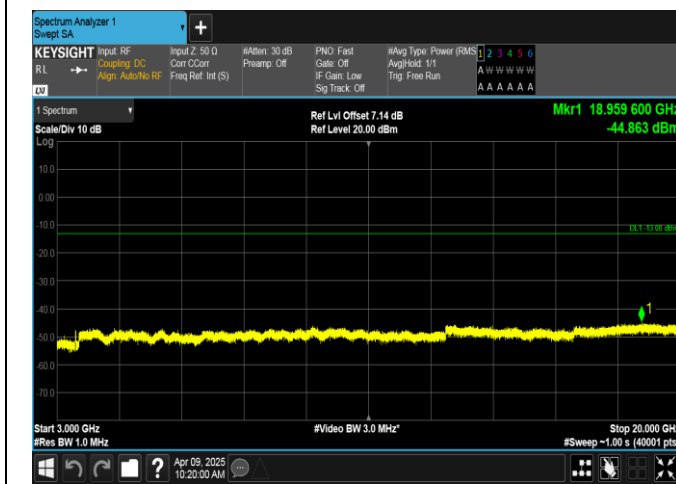
Band4-10MHz-QPSK-20350-50RB#0-3000~20000-PASS
