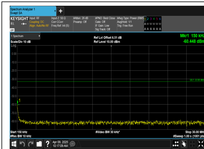
Band4-10MHz-QPSK-20350-1RB#49-0.15~30-PASS
