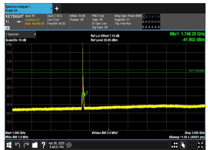
Band4-5MHz-16QAM-20175-1RB#0-1000~3000-PASS
