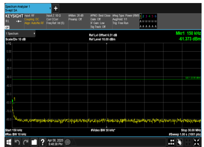
Band4-5MHz-QPSK-20175-1RB#24-0.15~30-PASS
