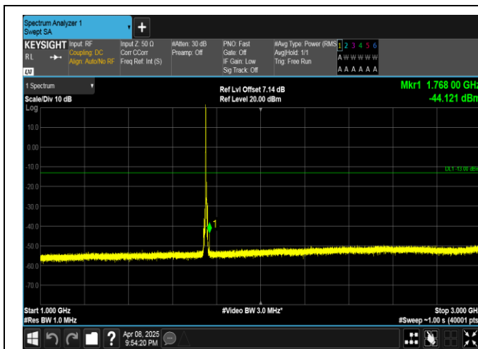
Band4-5MHz-16QAM-20375-1RB#0-1000~3000-PASS
