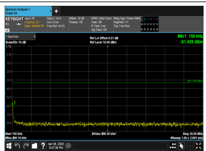
Band4-5MHz-16QAM-20175-1RB#0-0.15~30-PASS
