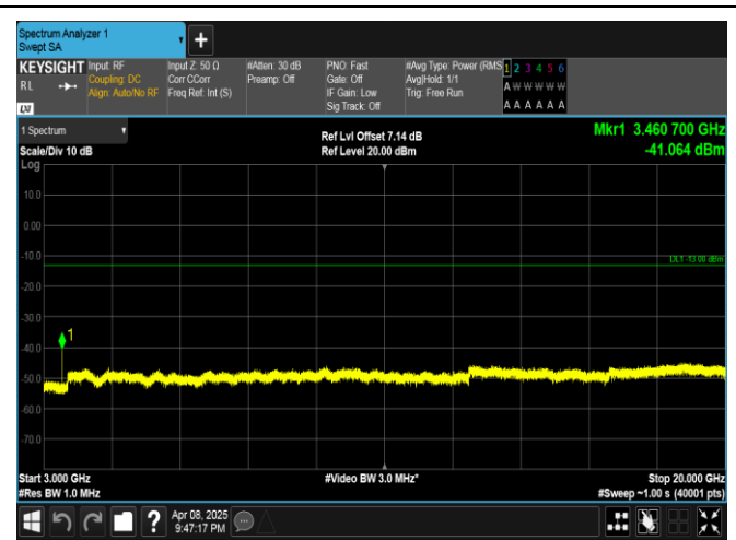
Band4-5MHz-QPSK-20175-1RB#0-3000~20000-PASS
