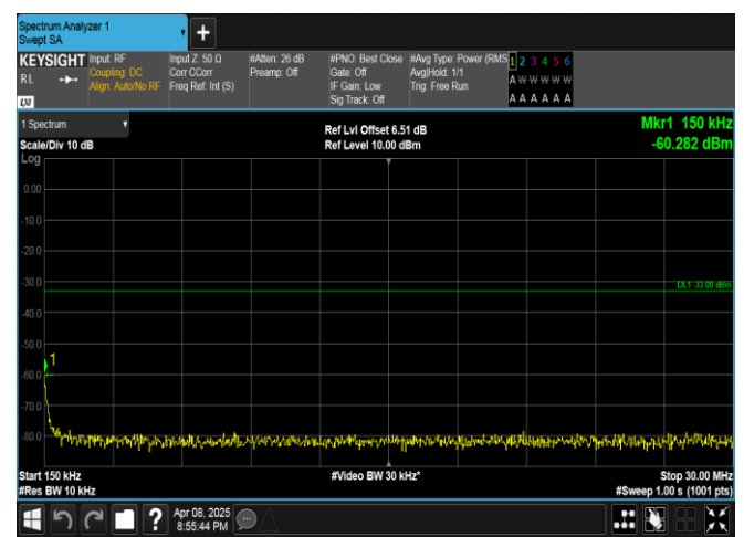
Band4-3MHz-16QAM-19965-1RB#14-0.15~30-PASS
