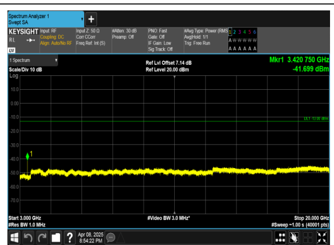
Band4-3MHz-16QAM-19965-1RB#0-3000~20000-PASS
