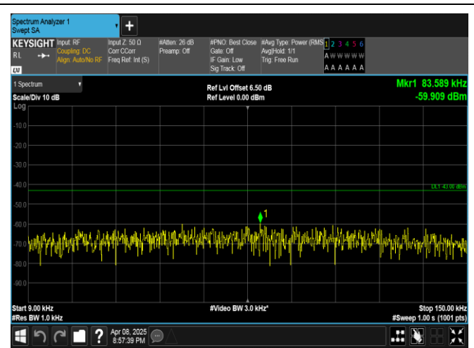
Band4-3MHz-16QAM-19965-15RB#0-0.009~0.15-PASS
