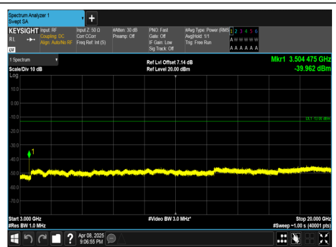
Band4-3MHz-16QAM-20385-1RB#0-3000~20000-PASS
