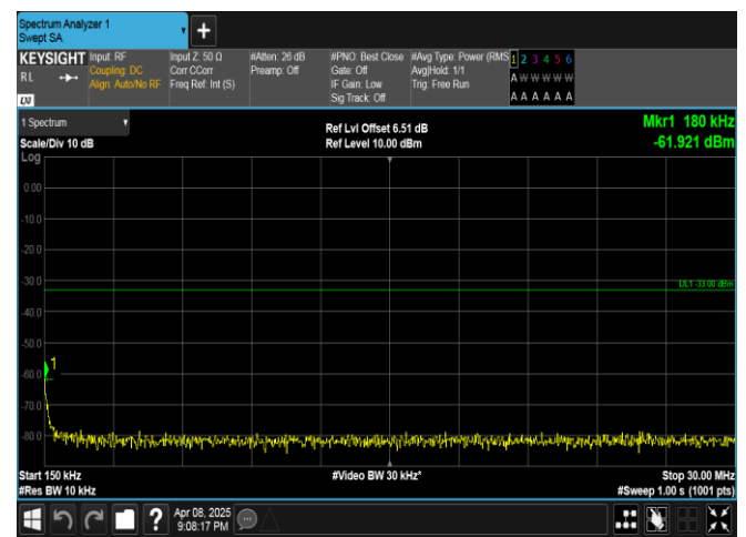
Band4-3MHz-16QAM-20385-1RB#14-0.15~30-PASS
