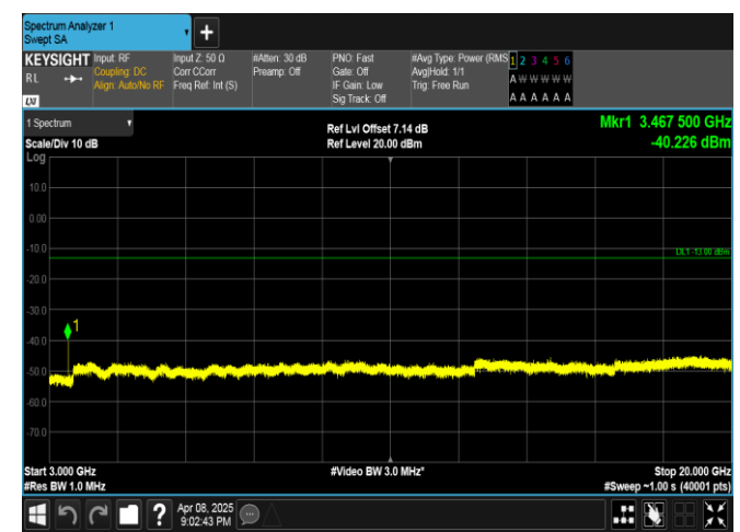
Band4-3MHz-16QAM-20175-1RB#14-3000~20000-PASS
