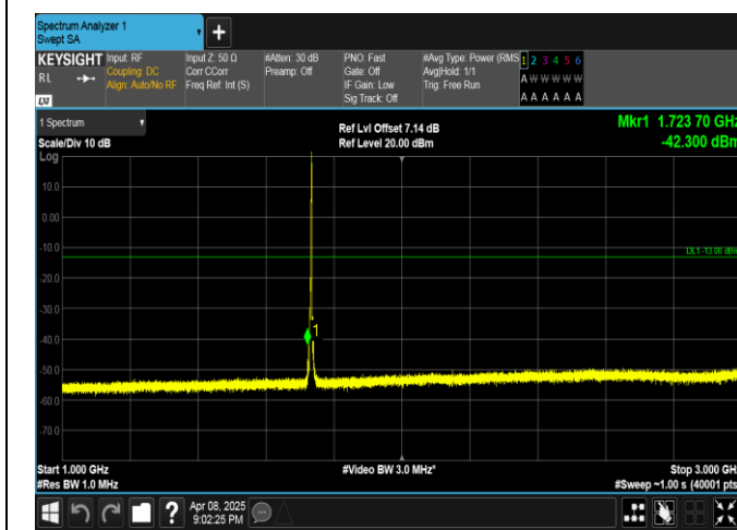
Band4-3MHz-16QAM-20175-1RB#14-1000~3000-PASS
