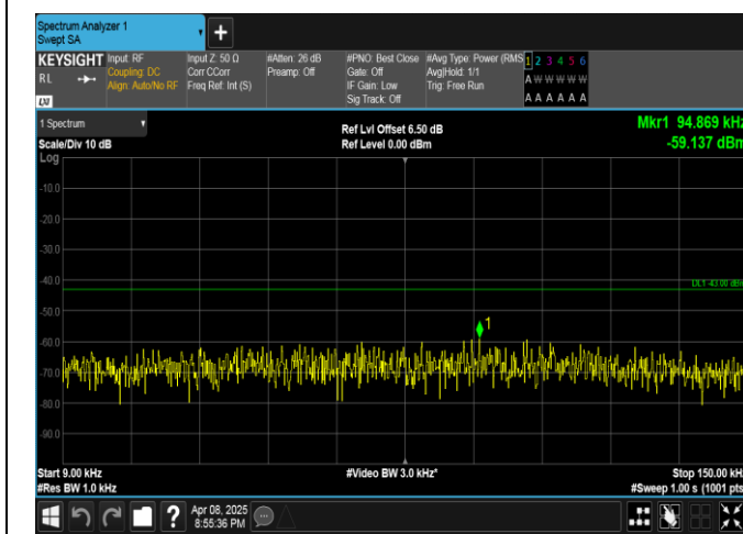
Band4-3MHz-16QAM-19965-1RB#14-0.009~0.15-PASS
