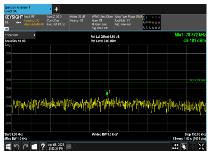
Band4-3MHz-16QAM-19965-1RB#0-0.009~0.15-PASS
