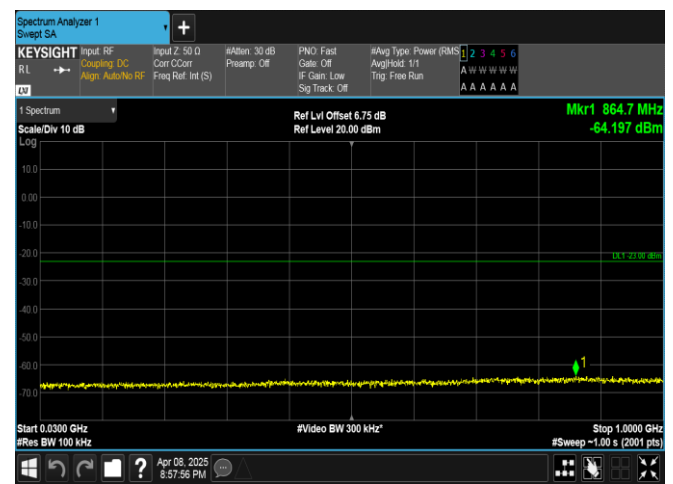
Band4-3MHz-16QAM-19965-15RB#0-30~1000-PASS
