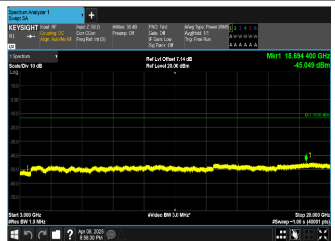
Band4-3MHz-16QAM-19965-15RB#0-3000~20000-PASS
