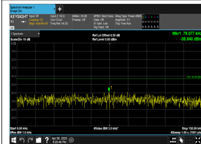
Band4-1.4MHz-QPSK-20393-6RB#0-0.009~0.15-PASS
