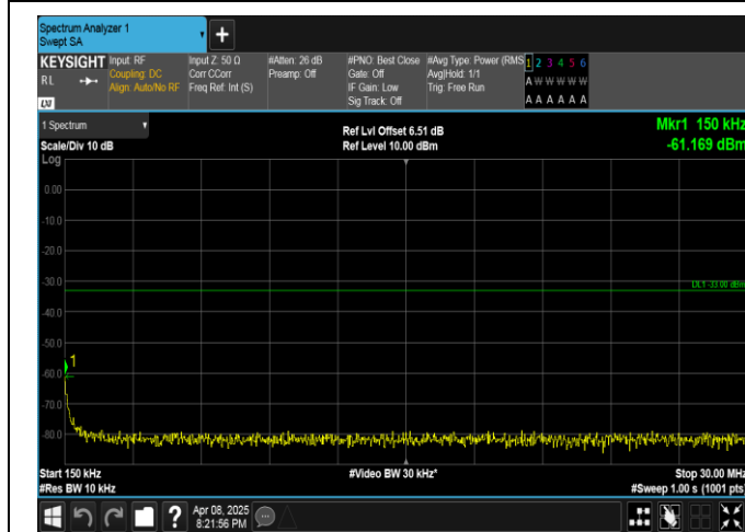
Band4-1.4MHz-16OAM-20393-6RB#0-0.15~30-PASS
