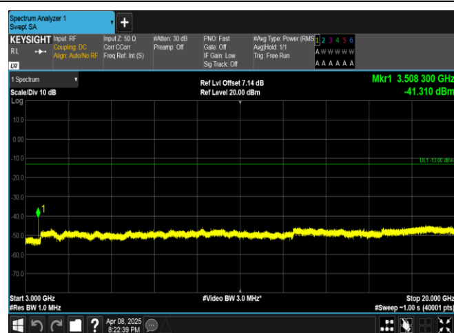
Band4-1.4MHz-16QAM-20393-6RB#0-3000~20000-PASS
