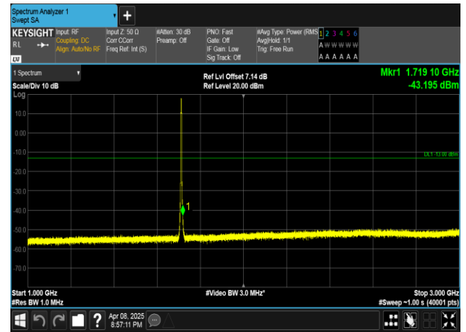
Band4-3MHz-QPSK-19965-15RB#0-1000~3000-PASS
