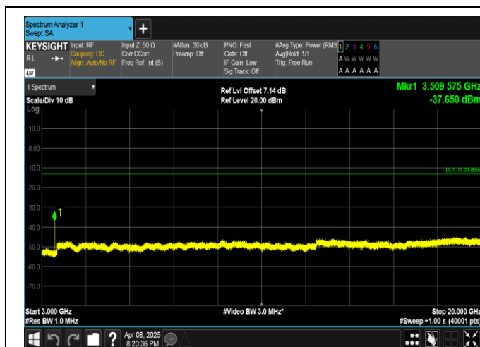
Band4-1.4MHz-16OAM-20393-1RB#5-3000~20000-PASS
