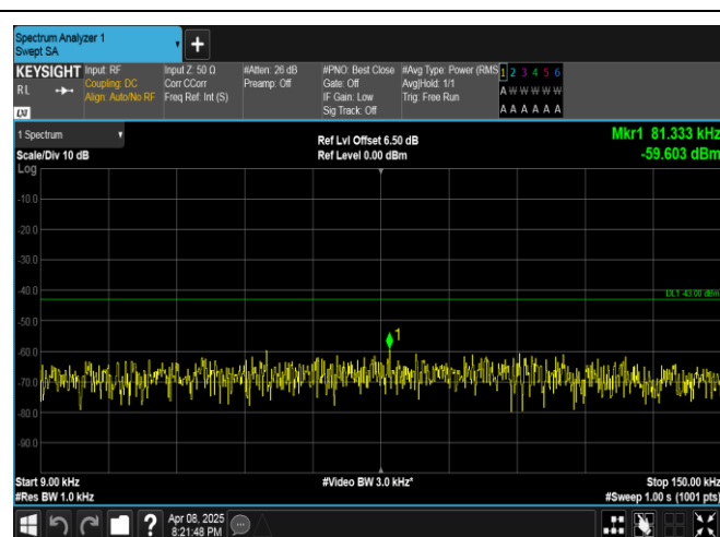
Band4-1.4MHz-16OAM-20393-6RB#0-0.009~0.15-PASS
