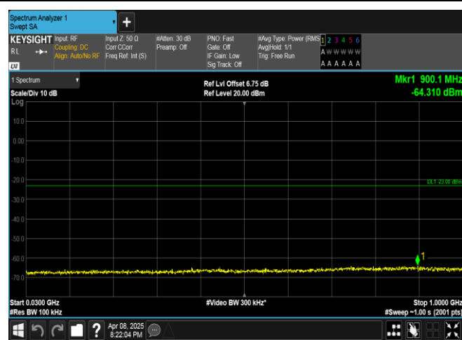
Band4-1.4MHz-16OAM-20393-6RB#0-30~1000-PASS
