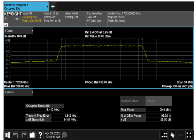
Band4-15MHz-QPSK-20175-75RB#0-PASS
