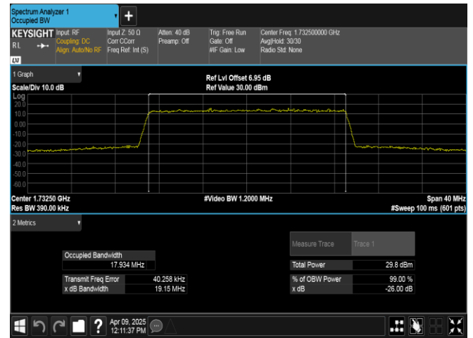
Band4-20MHz-QPSK-20175-100RB#0-PASS
