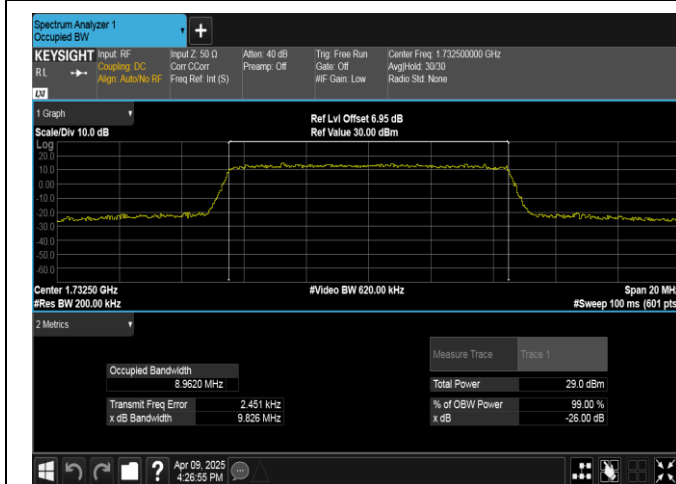
Band4-10MHz-16QAM-20175-50RB#0-PASS
