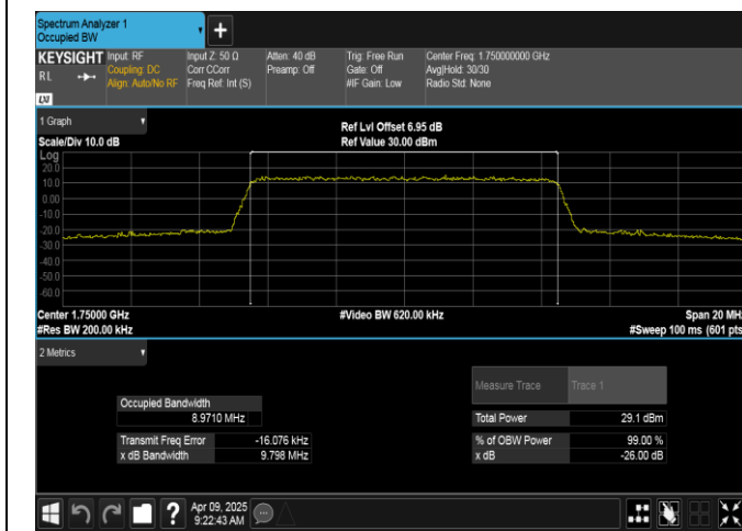
Band4-10MHz-QPSK-20350-50RB#0-PASS
