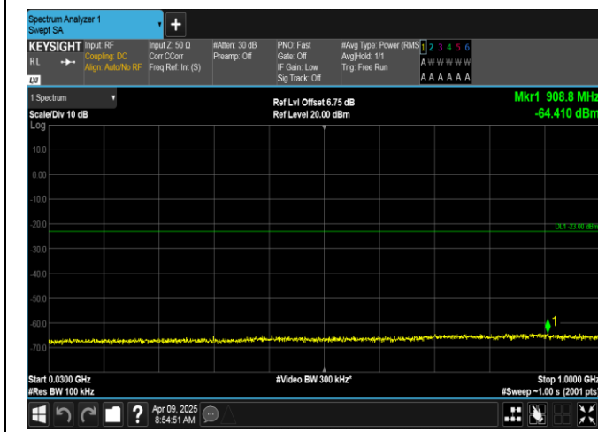
Band2-20MHz-16QAM-18900-100RB#0-30~1000-PASS
