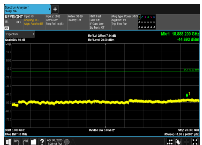
Band2-20MHz-QPSK-18700-1RB#99-3000~20000-PASS
