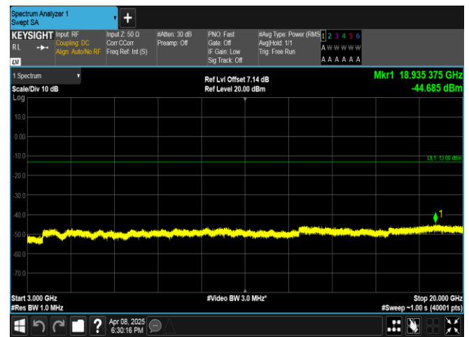
Band2-20MHz-16QAM-18700-1RB#0-3000~20000-PASS
