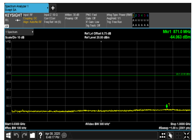
Band2-20MHz-QPSK-19100-1RB#99-30~1000-PASS
