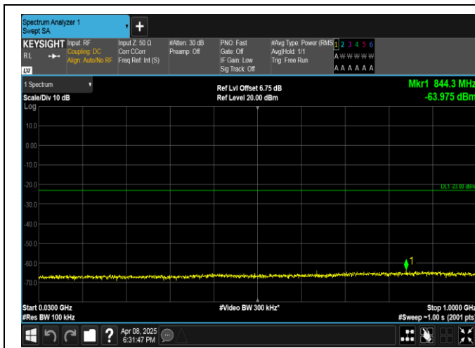
Band2-20MHz-16QAM-18700-1RB#99-30~1000-PASS
