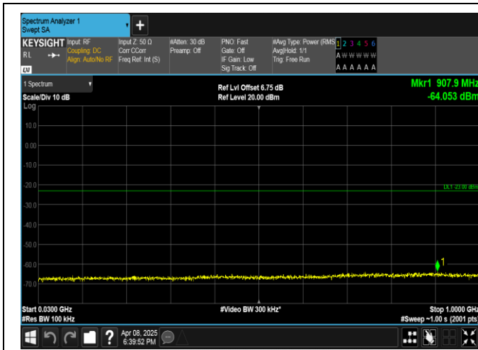
Band2-20MHz-QPSK-18900-1RB#99-30~1000-PASS
