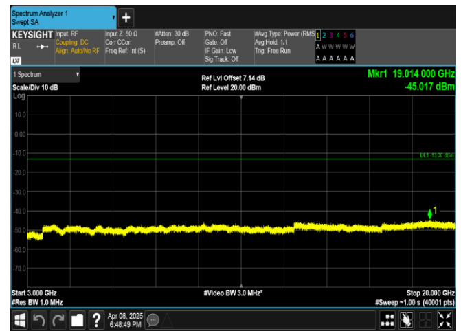
Band2-20MHz-16QAM-19100-1RB#0-3000~20000-PASS
