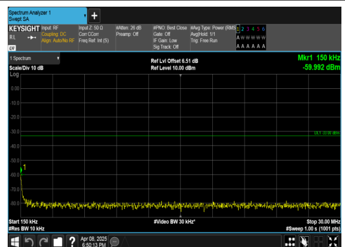
Band2-20MHz-16QAM-19100-1RB#99-0.15~30-PASS
