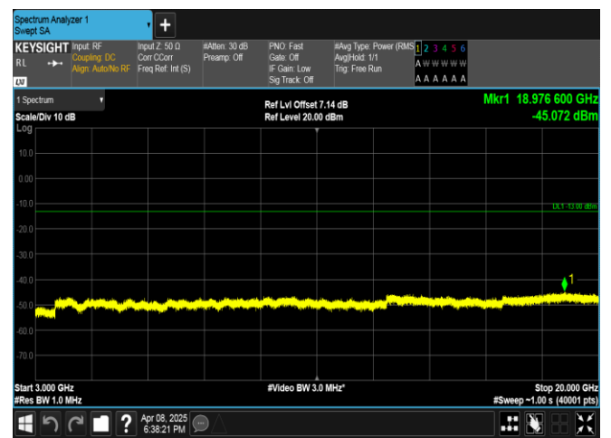
Band2-20MHz-QPSK-18900-1RB#0-3000~20000-PASS
