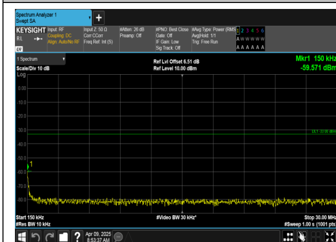
Band2-20MHz-16QAM-18700-100RB#0-0.15~30-PASS
