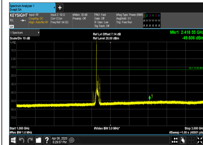
Band2-20MHz-16QAM-18700-1RB#0-1000~3000-PASS
