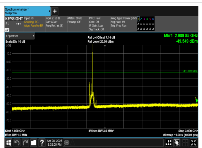
Band2-20MHz-16QAM-18700-1RB#99-1000~3000-PASS
