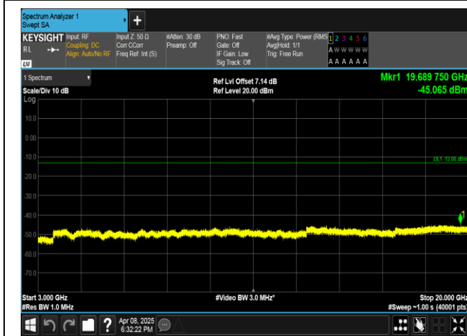
Band2-20MHz-16QAM-18700-1RB#99-3000~20000-PASS
