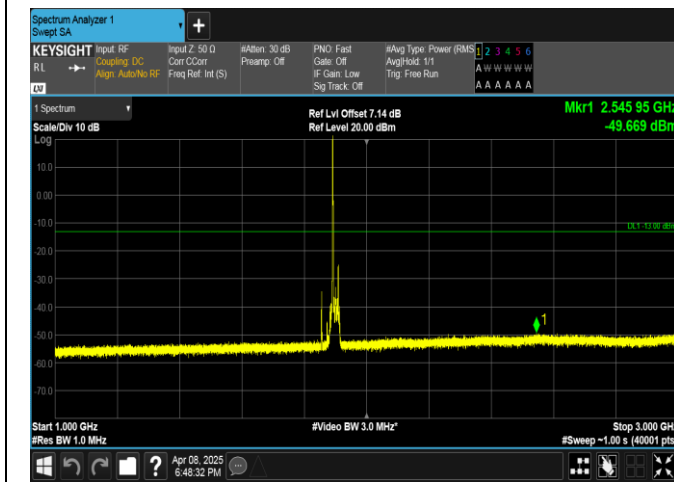
Band2-20MHz-16QAM-19100-1RB#0-1000~3000-PASS
