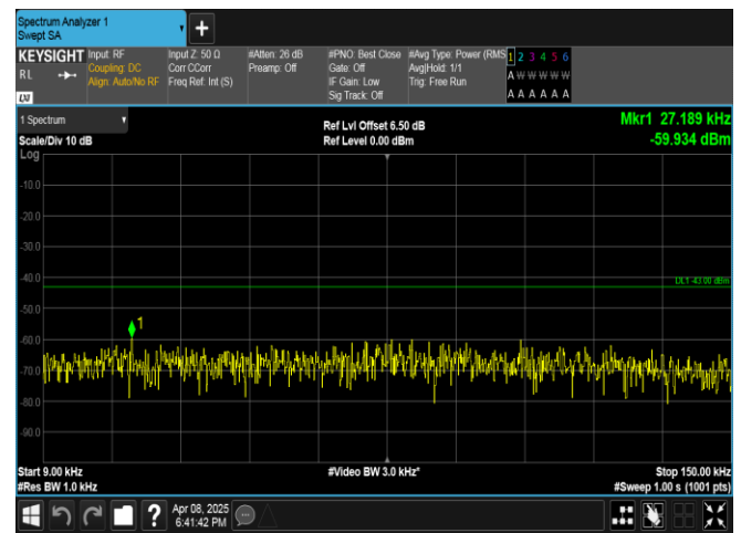
Band2-20MHz-QPSK-18900-100RB#0-0.009~0.15-PASS
