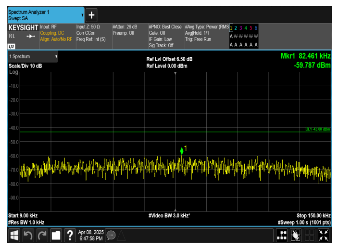
Band2-20MHz-16QAM-19100-1RB#0-0.009~0.15-PASS
