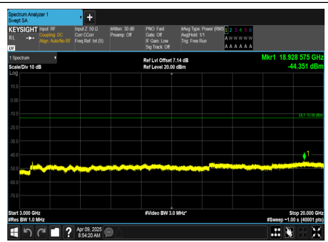
Band2-20MHz-16QAM-18700-100RB#0-3000~20000-PASS
