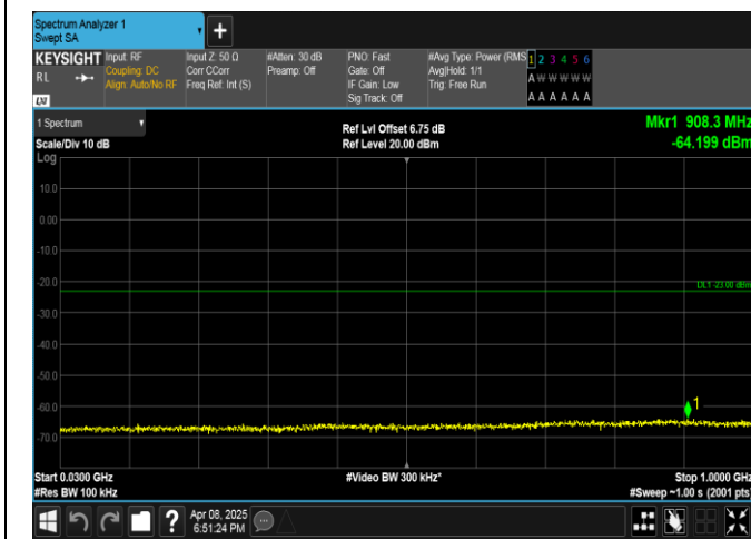
Band2-20MHz-QPSK-19100-100RB#0-30~1000-PASS
