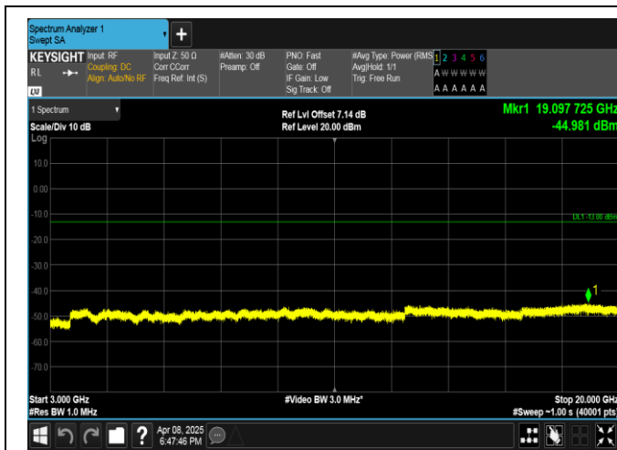
Band2-20MHz-QPSK-19100-1RB#0-3000~20000-PASS
