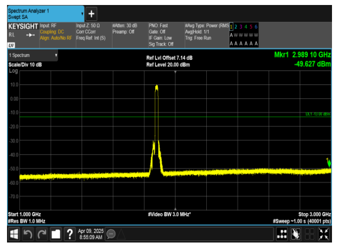
Band2-20MHz-16QAM-18900-100RB#0-1000~3000-PASS
