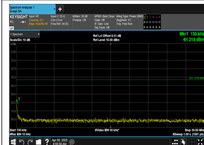
Band2-20MHz-16QAM-19100-100RB#0-0.15~30-PASS
