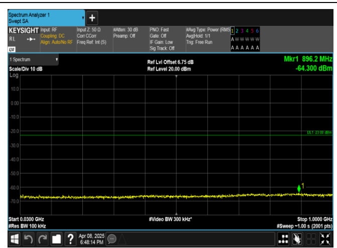
Band2-20MHz-16QAM-19100-1RB#0-30~1000-PASS
