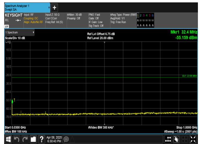
Band2-20MHz-QPSK-18700-1RB#99-30~1000-PASS
