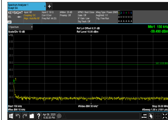
Band2-20MHz-QPSK-18700-1RB#99-0.15~30-PASS
