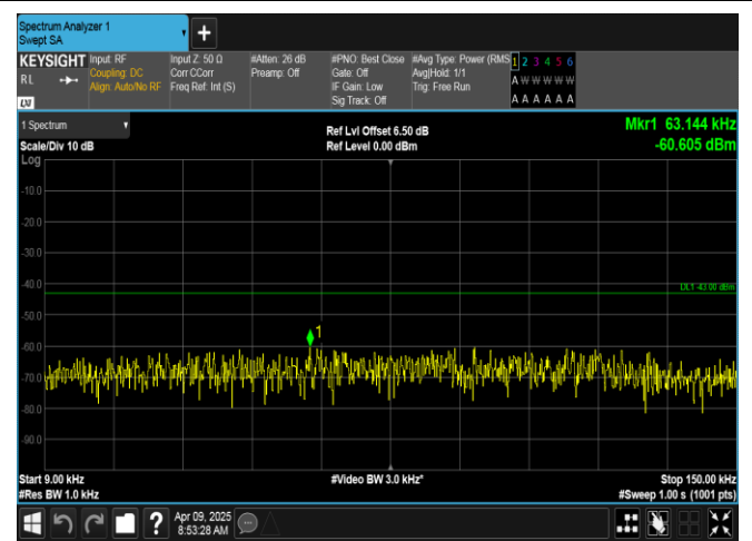
Band2-20MHz-16QAM-18700-100RB#0-0.009~0.15-PASS
