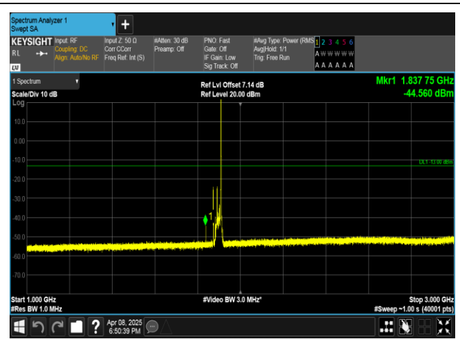
Band2-20MHz-16QAM-19100-1RB#99-1000~3000-PASS
