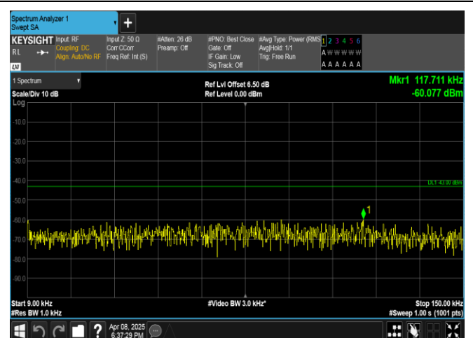
Band2-20MHz-QPSK-18900-1RB#0-0.009~0.15-PASS
