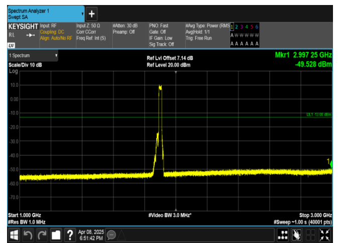
Band2-20MHz-QPSK-19100-100RB#0-1000~3000-PASS
