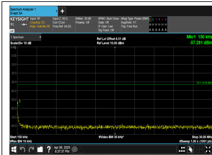
Band2-20MHz-QPSK-18900-1RB#0-0.15~30-PASS
