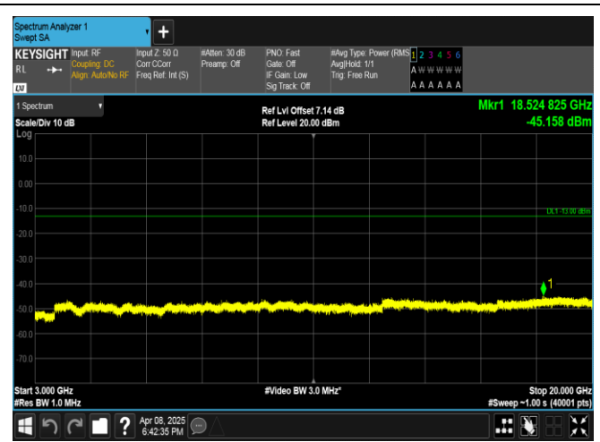
Band2-20MHz-QPSK-18900-100RB#0-3000~20000-PASS
