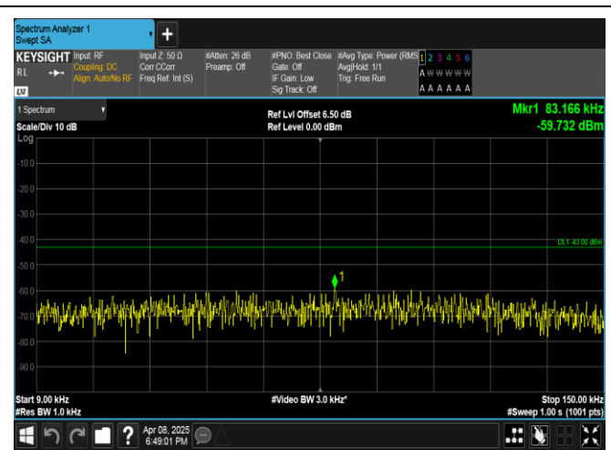
Band2-20MHz-QPSK-19100-1RB#99-0.009~0.15-PASS
