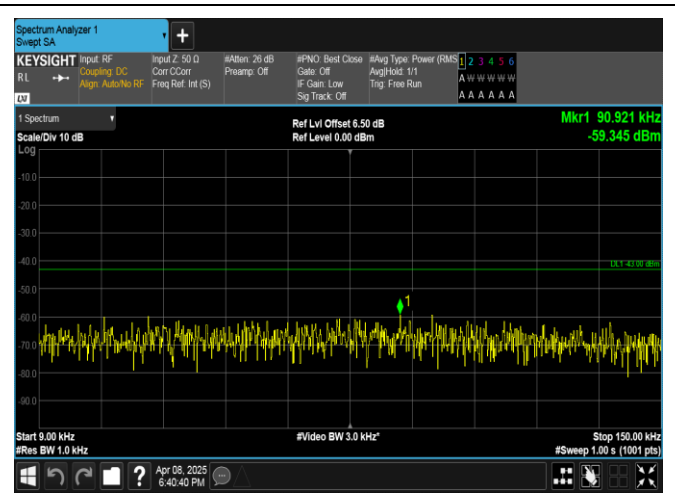
Band2-20MHz-16QAM-18900-1RB#99-0.009-0.15-PASS
