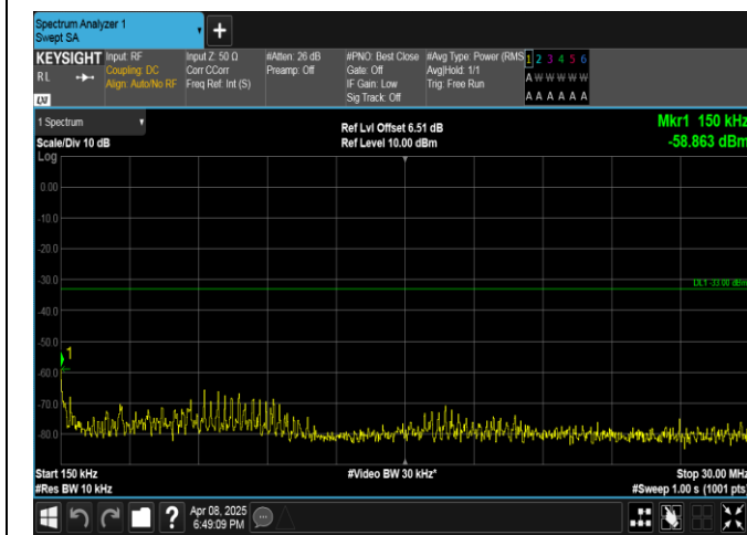
Band2-20MHz-QPSK-19100-1RB#99-0.15~30-PASS
