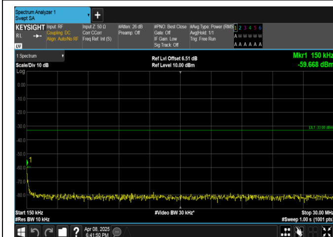
Band2-20MHz-QPSK-18900-100RB#0-0.15~30-PASS
