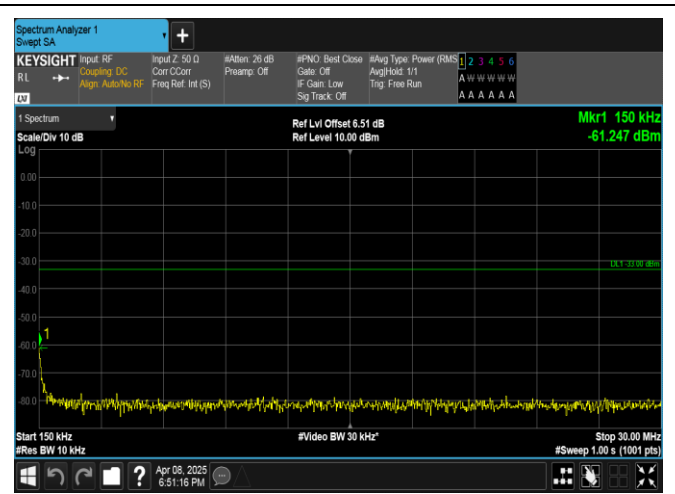
Band2-20MHz-QPSK-19100-100RB#0-0.15~30-PASS
