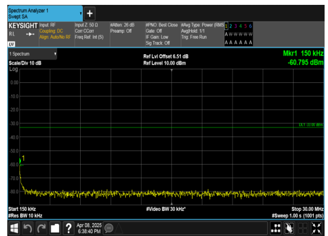
Band2-20MHz-16QAM-18900-1RB#0-0.15~30-PASS
