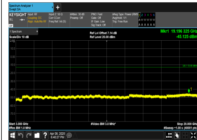
Band2-20MHz-QPSK-18900-1RB#99-3000~20000-PASS
