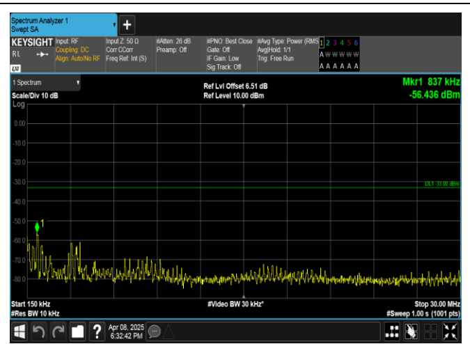
Band2-20MHz-QPSK-18700-100RB#0-0.15~30-PASS
