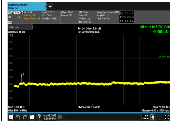
Band2-20MHz-16QAM-19100-1RB#99-3000~20000-PASS
