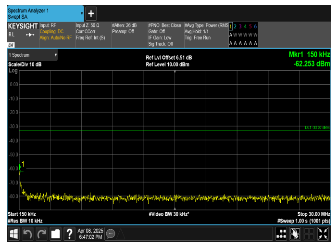
Band2-20MHz-QPSK-19100-1RB#0-0.15~30-PASS
