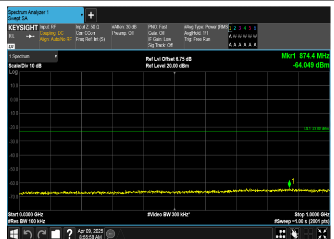
Band2-20MHz-16QAM-19100-100RB#0-30~1000-PASS
