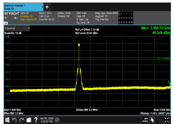
Band2-20MHz-QPSK-18700-100RB#0-1000~3000-PASS
