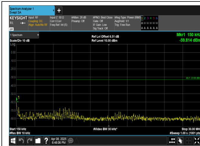
Band2-20MHz-16QAM-19100-1RB#0-0.15~30-PASS
