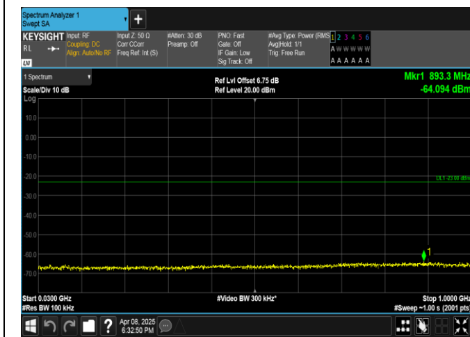
Band2-20MHz-QPSK-18700-100RB#0-30~1000-PASS
