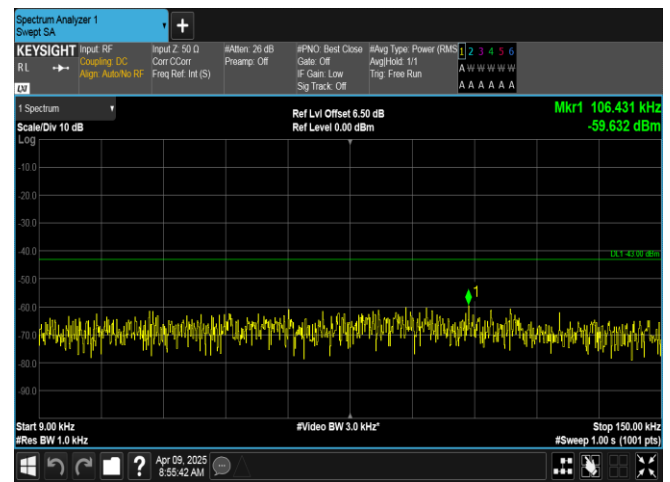
Band2-20MHz-16QAM-19100-100RB#0-0.009~0.15-PASS
