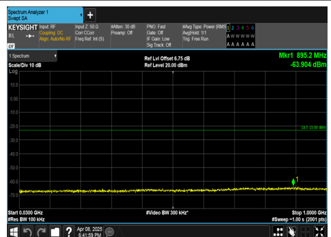
Band2-20MHz-QPSK-18900-100RB#0-30~1000-PASS
