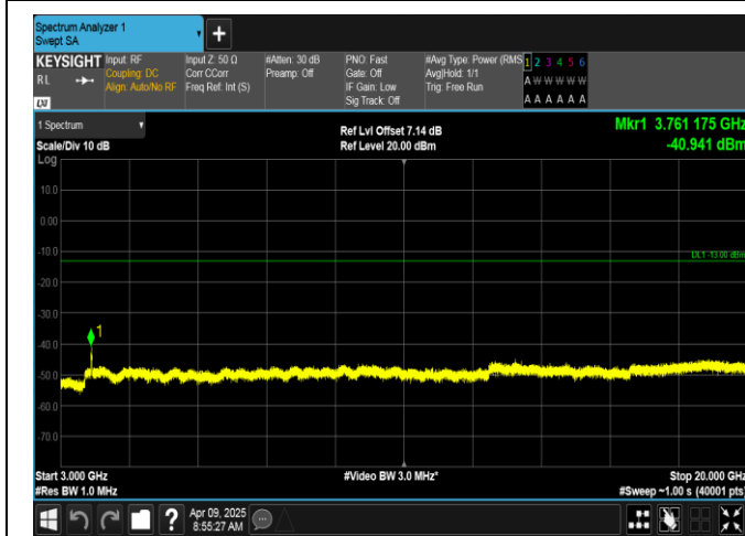
Band2-20MHz-16QAM-18900-100RB#0-3000~20000-PASS
