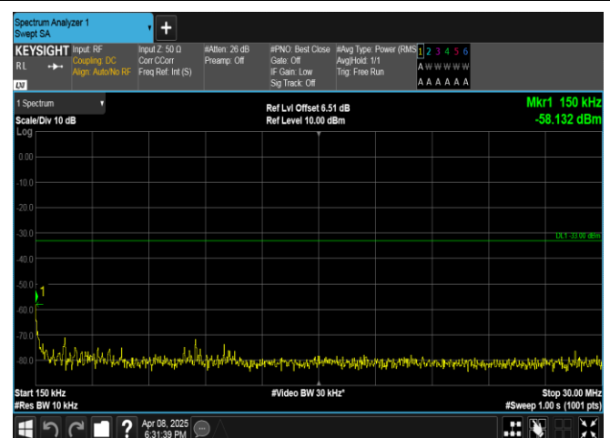
Band2-20MHz-16QAM-18700-1RB#99-0.15~30-PASS
