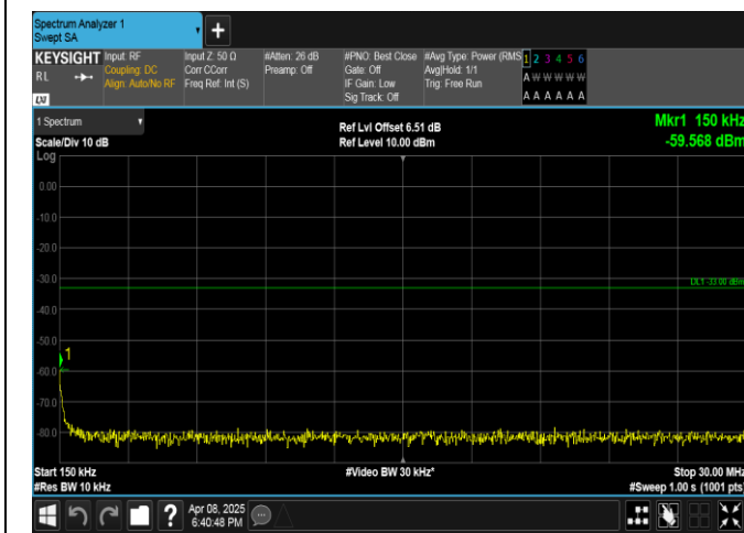
Band2-20MHz-16QAM-18900-1RB#99-0.15-30-PASS
