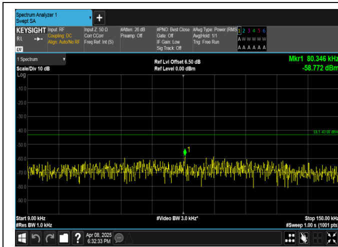
Band2-20MHz-QPSK-18700-100RB#0-0.009~0.15-PASS
