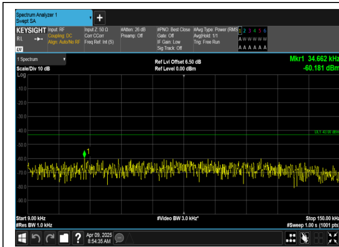
Band2-20MHz-16QAM-18900-100RB#0-0.009~0.15-PASS
