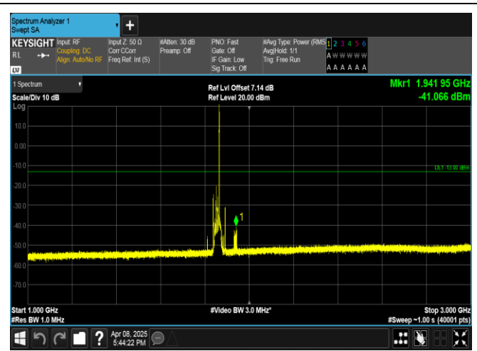
Band2-15MHz-16QAM-18675-1RB#74-1000~3000-PASS
