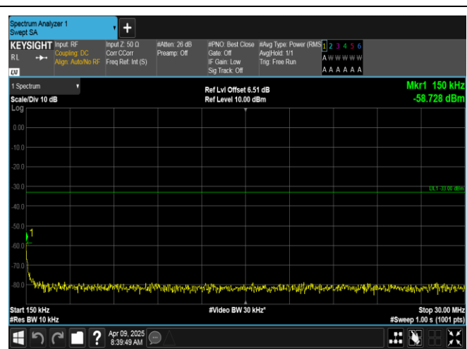
Band2-15MHz-16QAM-18900-75RB#0-0.15~30-PASS
