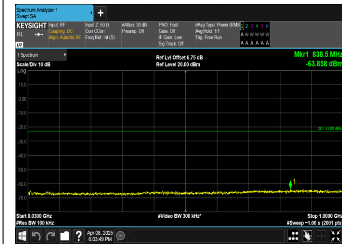
Band2-15MHz-QPSK-19125-75RB#0-30~1000-PASS
