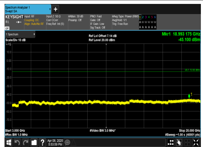
Band2-15MHz-16QAM-18900-1RB#74-3000-20000-PASS
