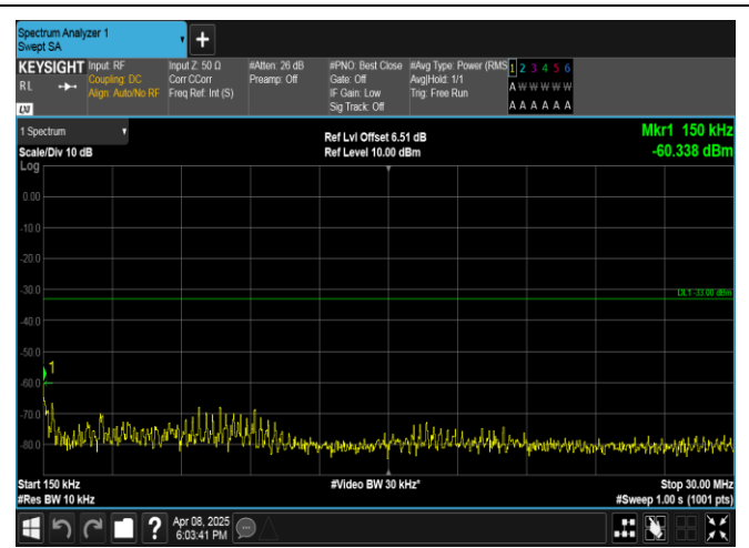
Band2-15MHz-QPSK-19125-75RB#0-0.15~30-PASS
