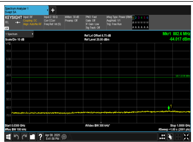
Band2-15MHz-16QAM-18675-1RB#0-30~1000-PASS
