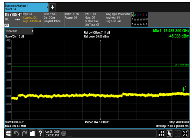
Band2-15MHz-16QAM-18675-1RB#0-3000~20000-PASS
