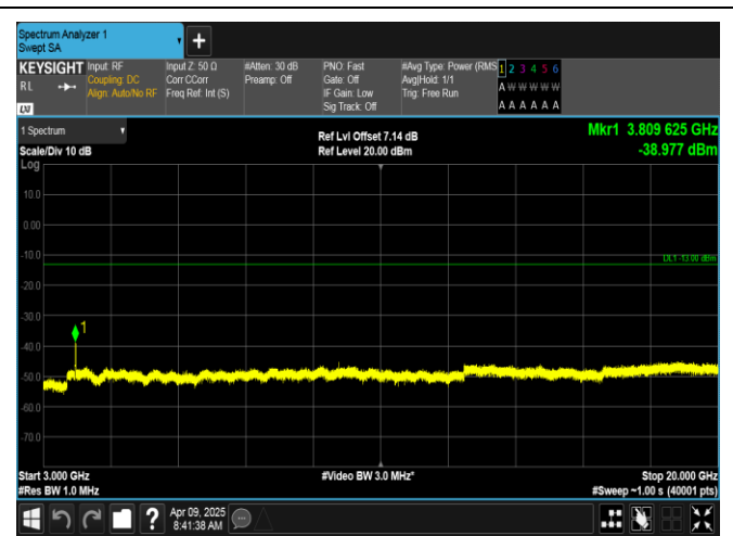
Band2-15MHz-16QAM-19125-75RB#0-3000~20000-PASS
