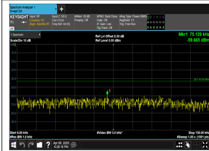
Band2-20MHz-QPSK-18700-1RB#0-0.009~0.15-PASS
