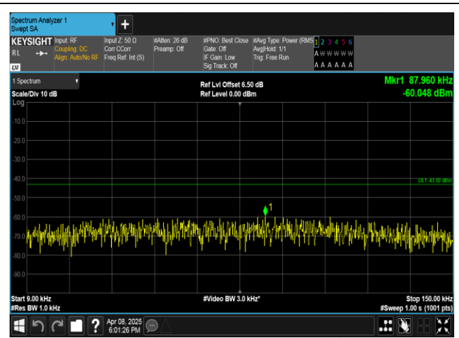
Band2-15MHz-QPSK-19125-1RB#74-0.009~0.15-PASS
