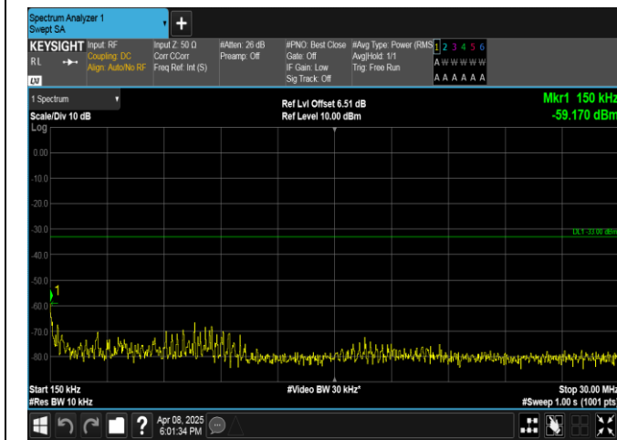
Band2-15MHz-QPSK-19125-1RB#74-0.15~30-PASS
