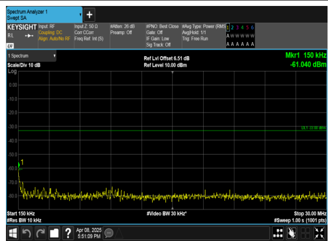
Band2-15MHz-16QAM-18900-1RB#0-0.15~30-PASS
