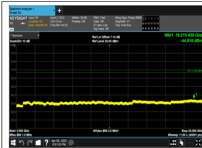
Band2-15MHz-16QAM-18900-1RB#0-3000-20000-PASS
