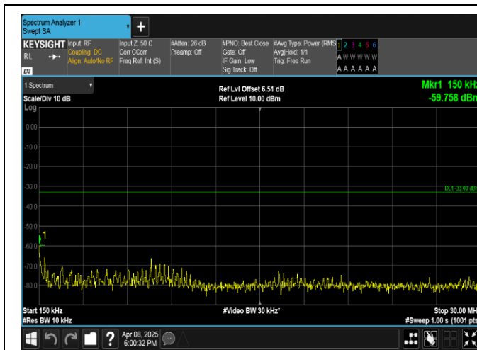
Band2-15MHz-16QAM-19125-1RB#0-0.15~30-PASS
