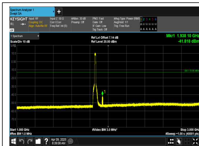
Band2-15MHz-16QAM-18675-75RB#0-1000~3000-PASS
