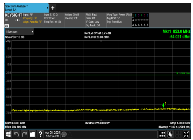
Band2-15MHz-16QAM-18900-1RB#74-30-1000-PASS
