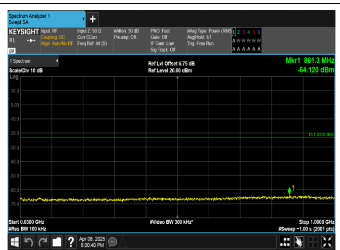
Band2-15MHz-16QAM-19125-1RB#0-30~1000-PASS
