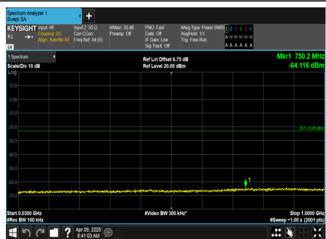
Band2-15MHz-16QAM-19125-75RB#0-30~1000-PASS
