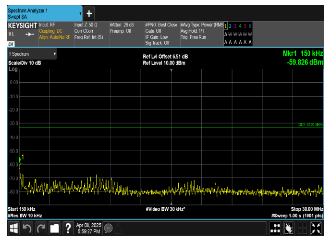
Band2-15MHz-QPSK-19125-1RB#0-0.15~30-PASS
