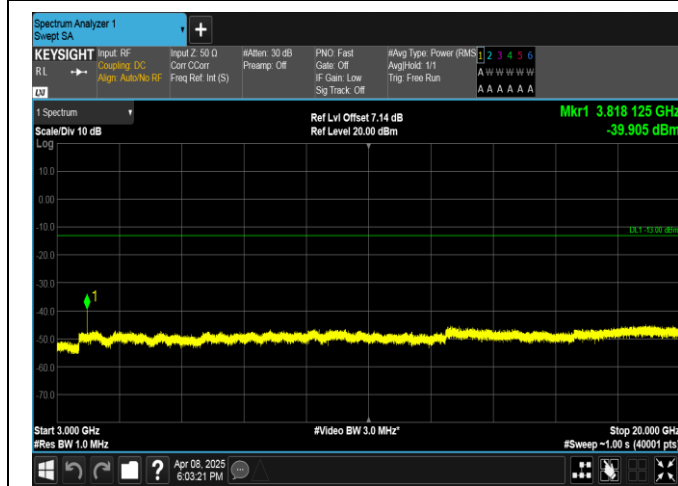
Band2-15MHz-16QAM-19125-1RB#74-3000~20000-PASS
