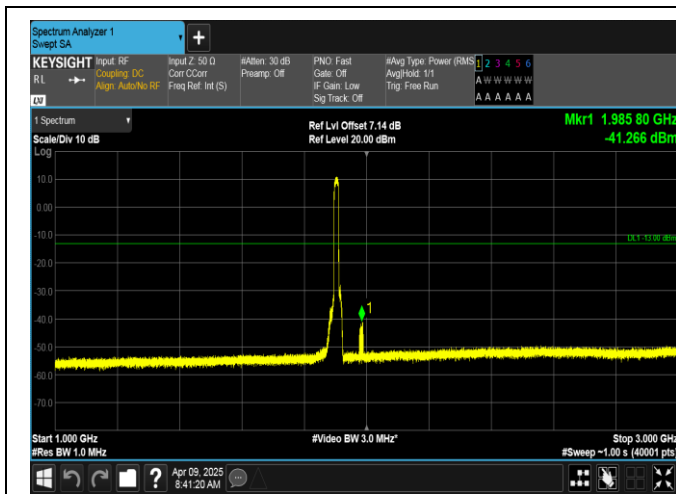
Band2-15MHz-16QAM-19125-75RB#0-1000~3000-PASS
