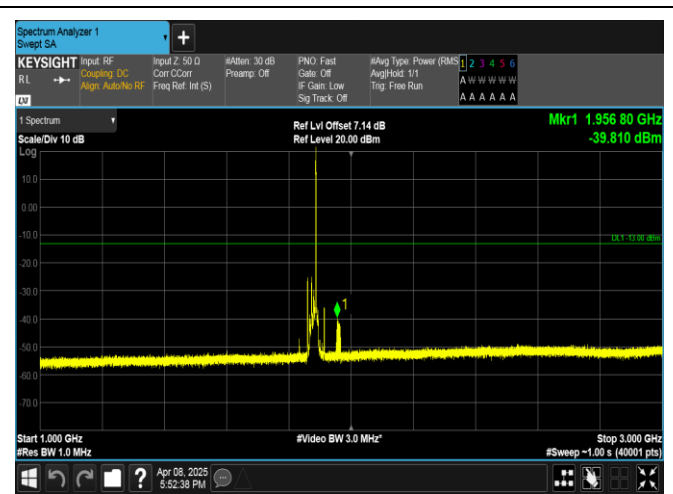
Band2-15MHz-QPSK-18900-1RB#74-1000~3000-PASS
