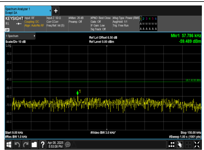
Band2-15MHz-16QAM-18900-1RB#74-0.009-0.15-PASS
