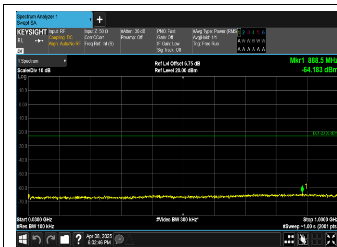
Band2-15MHz-16QAM-19125-1RB#74-30~1000-PASS
