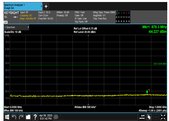
Band2-15MHz-QPSK-19125-1RB#74-30~1000-PASS
