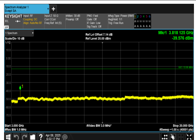
Band2-15MHz-QPSK-19125-1RB#74-3000~20000-PASS
