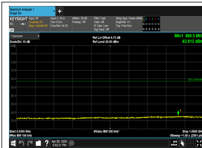
Band2-15MHz-QPSK-18900-1RB#74-30~1000-PASS
