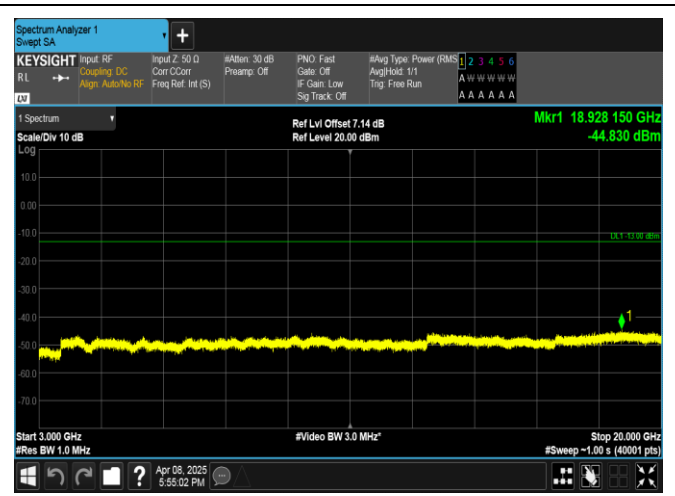
Band2-15MHz-QPSK-18900-75RB#0-3000~20000-PASS
