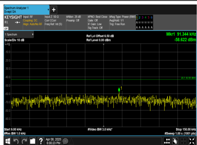
Band2-15MHz-16QAM-19125-1RB#0-0.009~0.15-PASS
