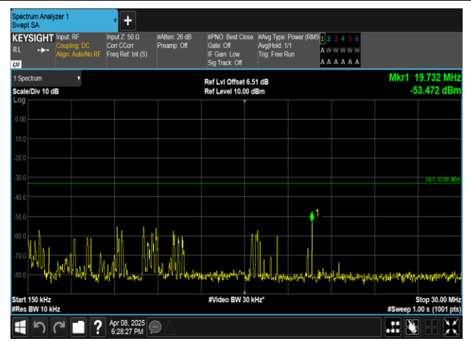
Band2-20MHz-QPSK-18700-1RB#0-0.15~30-PASS
