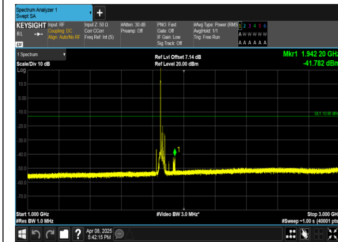
Band2-15MHz-16QAM-18675-1RB#0-1000~3000-PASS
