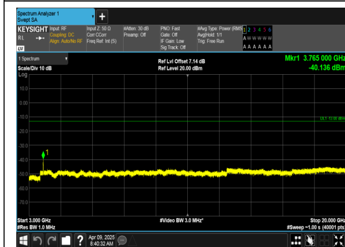
Band2-15MHz-16QAM-18900-75RB#0-3000~20000-PASS
