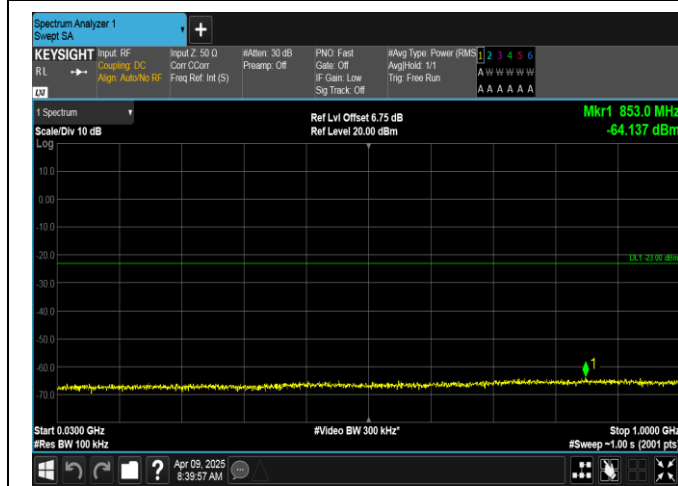
Band2-15MHz-16QAM-18900-75RB#0-30~1000-PASS
