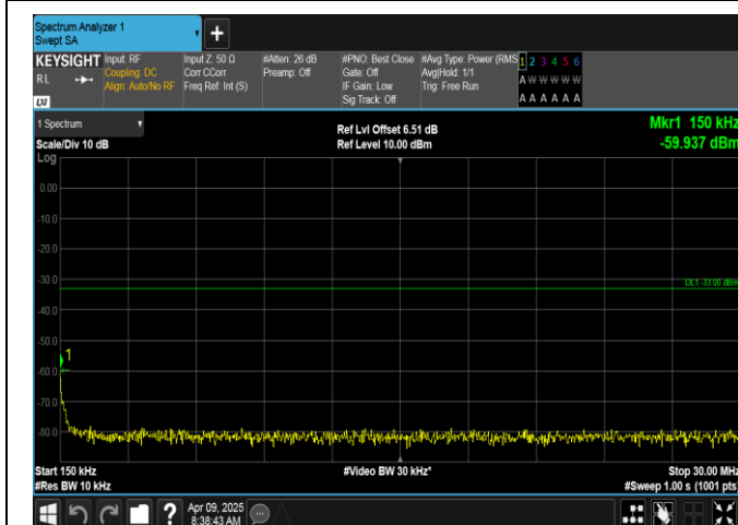
Band2-15MHz-16QAM-18675-75RB#0-0.15~30-PASS
