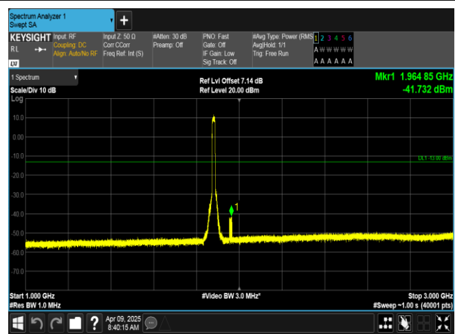
Band2-15MHz-16QAM-18900-75RB#0-1000~3000-PASS
