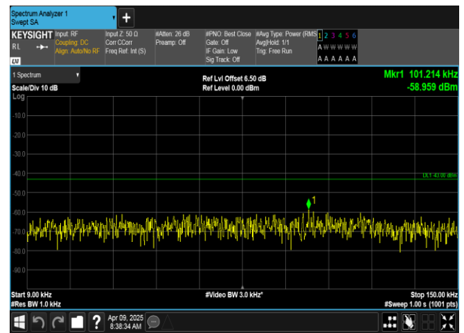
Band2-15MHz-16QAM-18675-75RB#0-0.009~0.15-PASS
