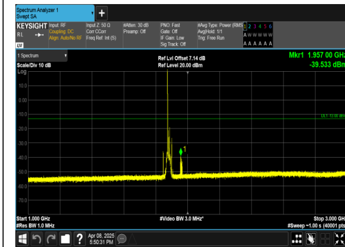
Band2-15MHz-QPSK-18900-1RB#0-1000~3000-PASS
