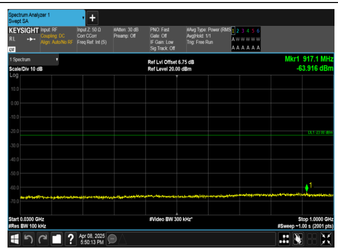
Band2-15MHz-QPSK-18900-1RB#0-30~1000-PASS
