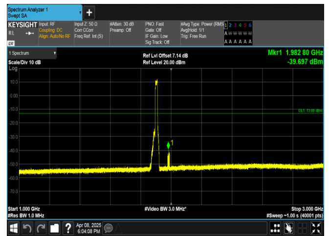
Band2-15MHz-QPSK-19125-75RB#0-1000~3000-PASS
