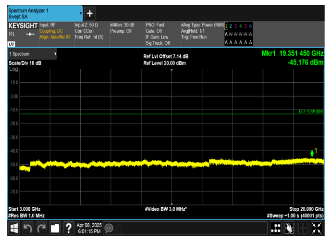
Band2-15MHz-16QAM-19125-1RB#0-3000~20000-PASS
