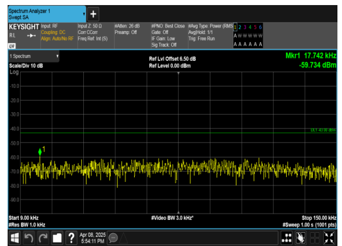
Band2-15MHz-QPSK-18900-75RB#0-0.009~0.15-PASS
