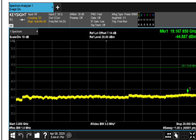
Band2-15MHz-16QAM-18675-1RB#74-3000~20000-PASS
