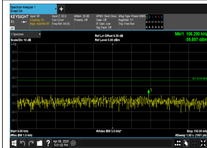
Band2-15MHz-16QAM-18900-1RB#0-0.009~0.15-PASS
