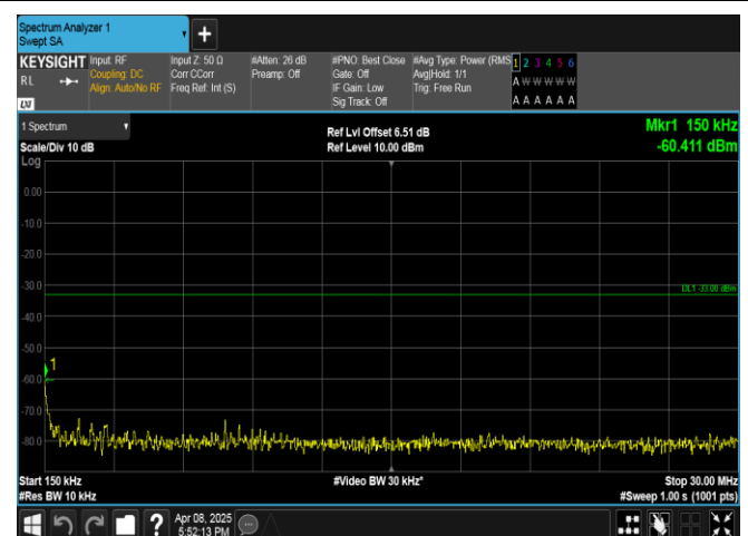
Band2-15MHz-QPSK-18900-1RB#74-0.15~30-PASS
