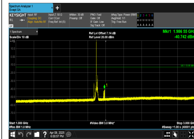
Band2-15MHz-16QAM-19125-1RB#0-1000~3000-PASS
