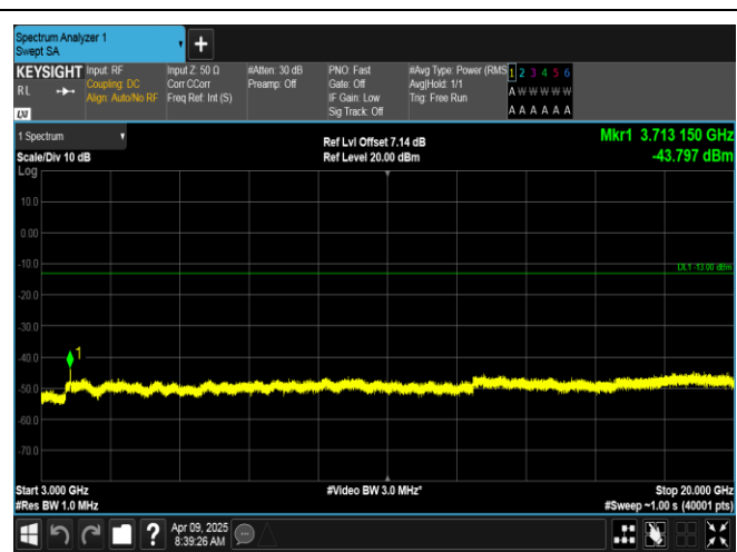
Band2-15MHz-16QAM-18675-75RB#0-3000~20000-PASS
