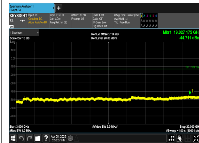
Band2-15MHz-QPSK-18900-1RB#74-3000~20000-PASS
