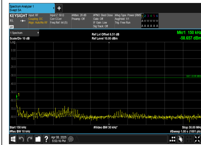
Band2-15MHz-16QAM-18900-1RB#74-0.15-30-PASS
