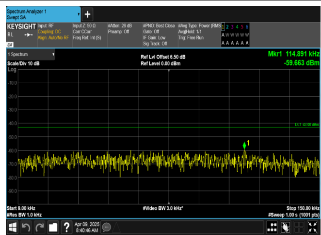
Band2-15MHz-16QAM-19125-75RB#0-0.009~0.15-PASS
