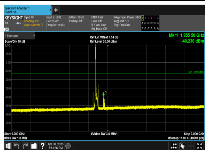
Band2-15MHz-16QAM-18900-1RB#0-1000~3000-PASS
