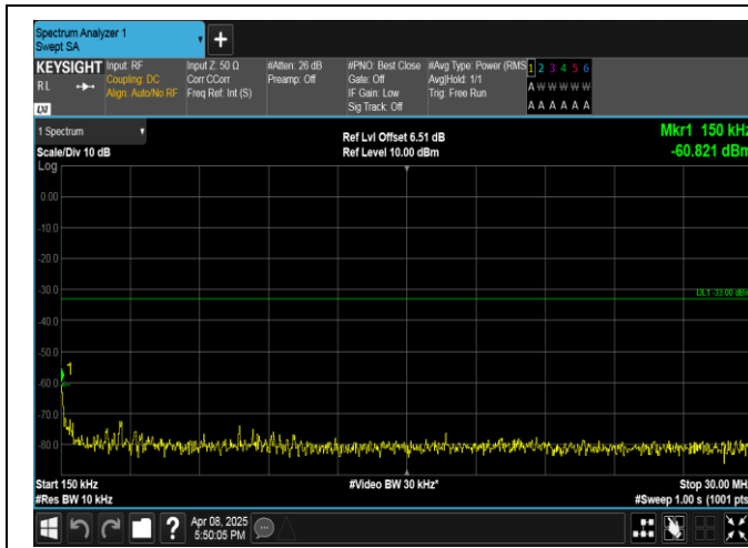
Band2-15MHz-QPSK-18900-1RB#0-0.15~30-PASS
