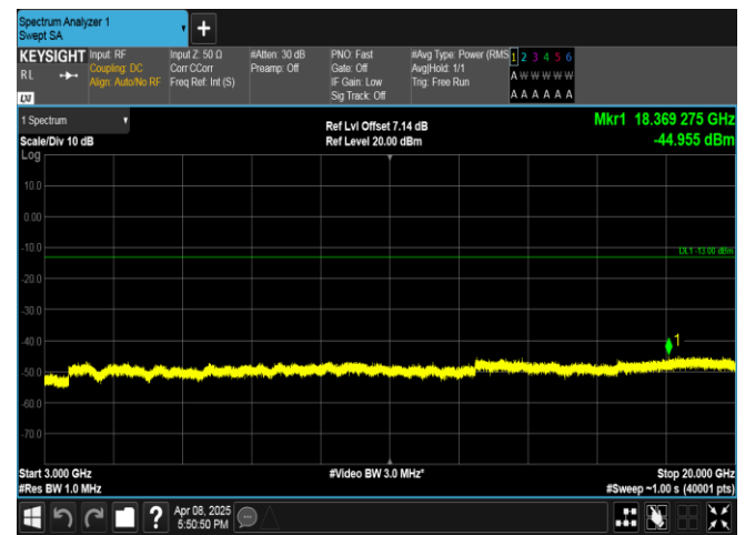
Band2-15MHz-QPSK-18900-1RB#0-3000~20000-PASS
