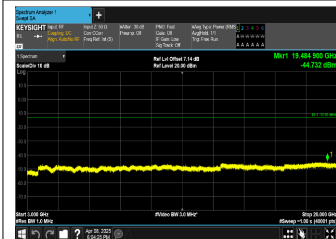
Band2-15MHz-QPSK-19125-75RB#0-3000~20000-PASS
