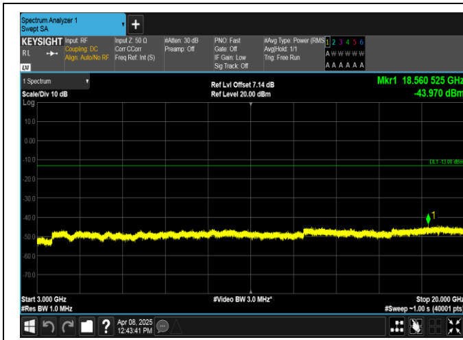
Band2-10MHz-16QAM-18900-1RB#0-3000~20000-PASS
