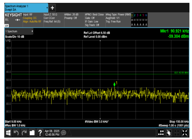
Band2-10MHz-QPSK-18900-50RB#0-0.009~0.15-PASS
