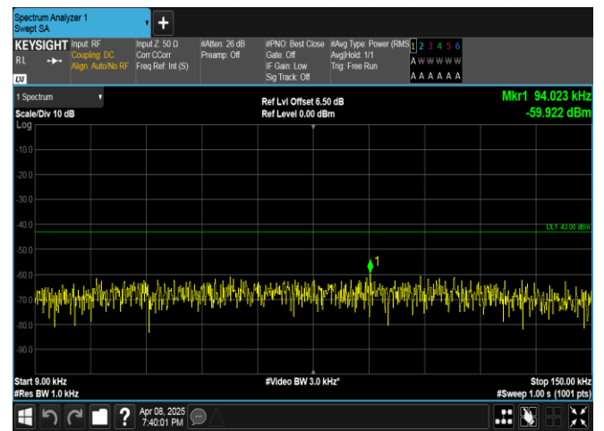
Band2-10MHz-16QAM-19150-50RB#0-0.009~0.15-PASS
