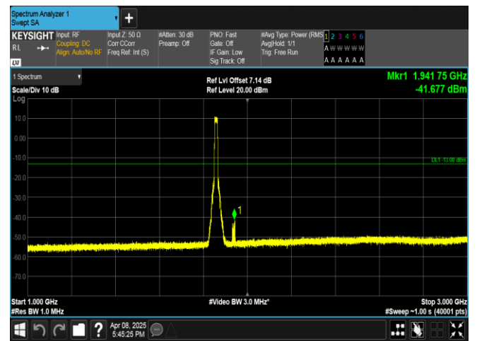
Band2-15MHz-QPSK-18675-75RB#0-1000~3000-PASS
