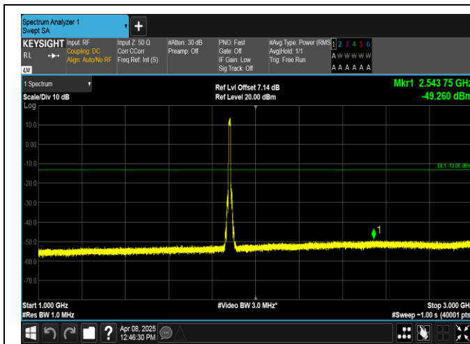
Band2-10MHz-QPSK-18900-50RB#0-1000~3000-PASS
