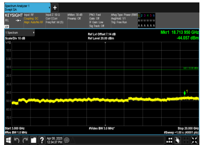
Band2-10MHz-16QAM-18650-1RB#0-3000~20000-PASS
