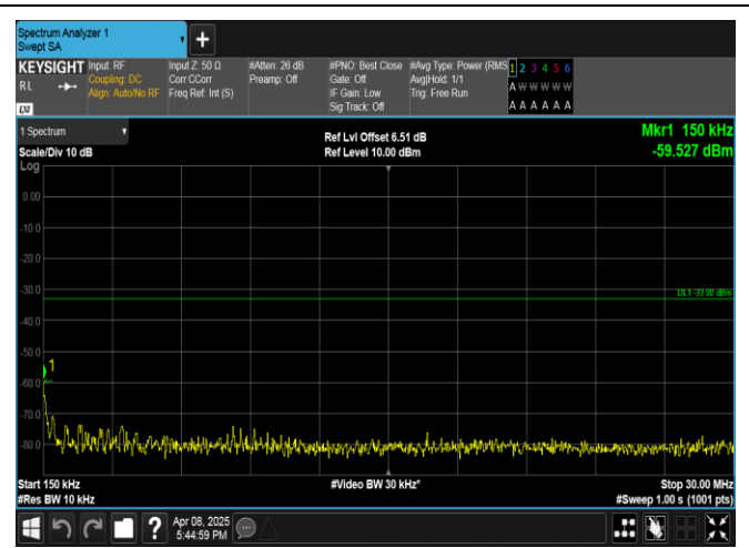
Band2-15MHz-QPSK-18675-75RB#0-0.15~30-PASS
