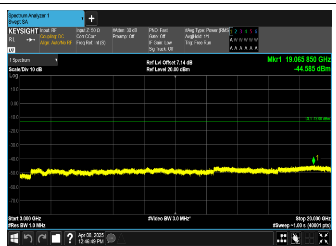
Band2-10MHz-QPSK-18900-50RB#0-3000~20000-PASS
