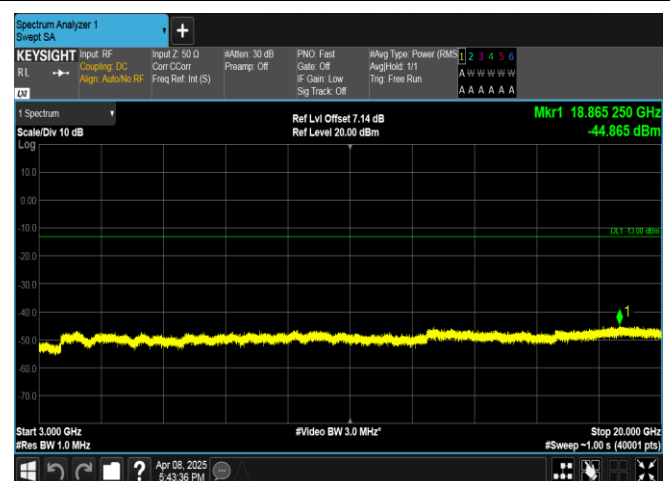
Band2-15MHz-QPSK-18675-1RB#74-3000~20000-PASS
