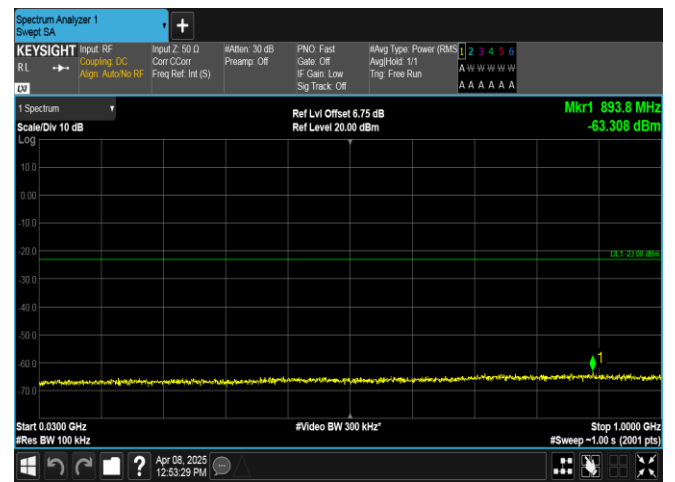
Band2-10MHz-QPSK-19150-1RB#49-30~1000-PASS
