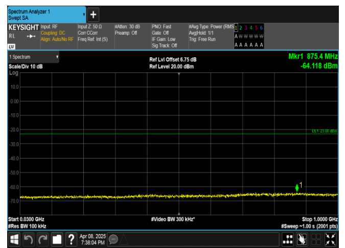
Band2-10MHz-16QAM-18650-50RB#0-30~1000-PASS
