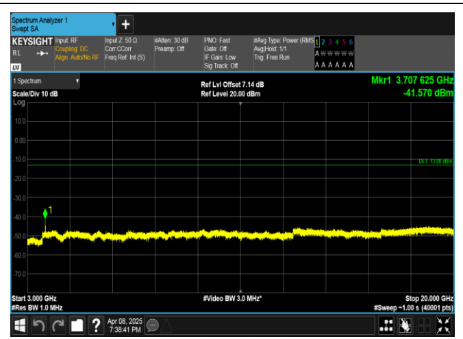
Band2-10MHz-16QAM-18650-50RB#0-3000~20000-PASS
