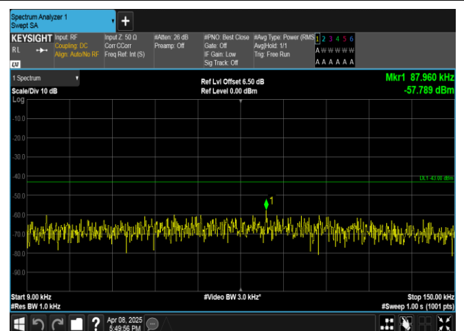
Band2-15MHz-QPSK-18900-1RB#0-0.009~0.15-PASS
