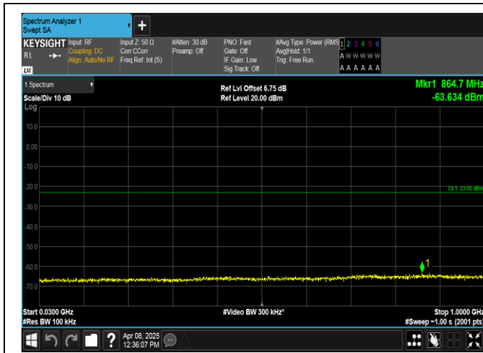
Band2-10MHz-16QAM-18650-1RB#49-30~1000-PASS
