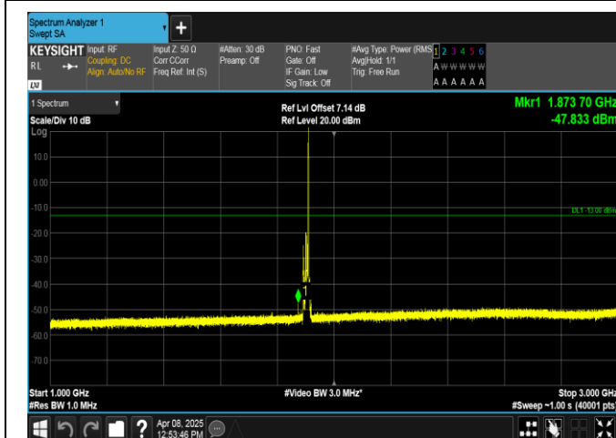
Band2-10MHz-QPSK-19150-1RB#49-1000~3000-PASS
