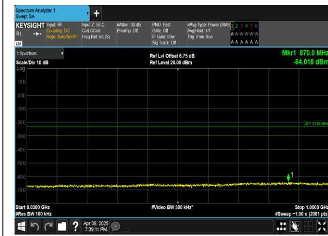
Band2-10MHz-16QAM-18900-50RB#0-30~1000-PASS
