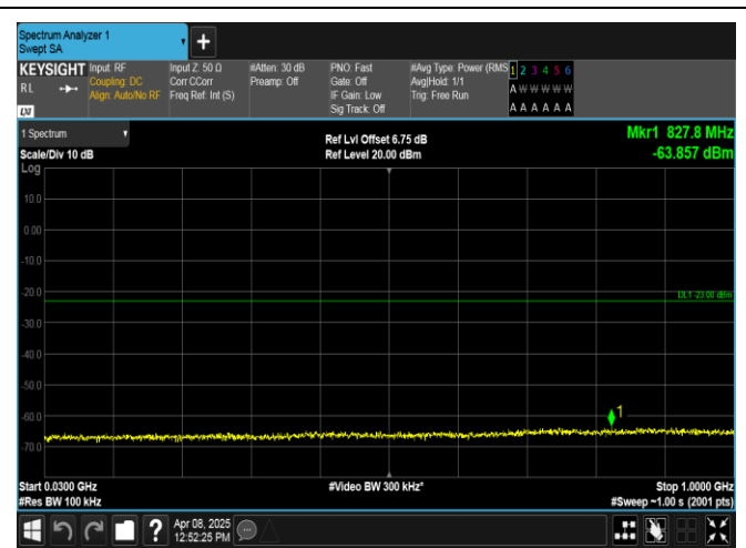
Band2-10MHz-16QAM-19150-1RB#0-30~1000-PASS
