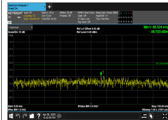
Band2-10MHz-16QAM-18900-1RB#0-0.009~0.15-PASS
