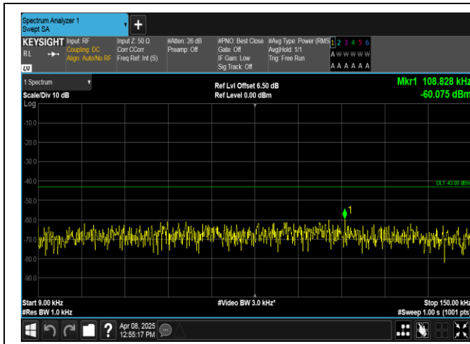
Band2-10MHz-QPSK-19150-50RB#0-0.009~0.15-PASS
