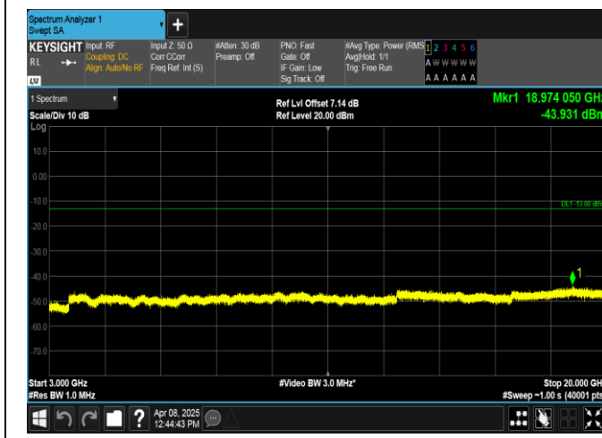
Band2-10MHz-QPSK-18900-1RB#49-3000~20000-PASS
