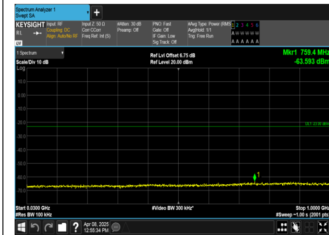
Band2-10MHz-QPSK-19150-50RB#0-30~1000-PASS
