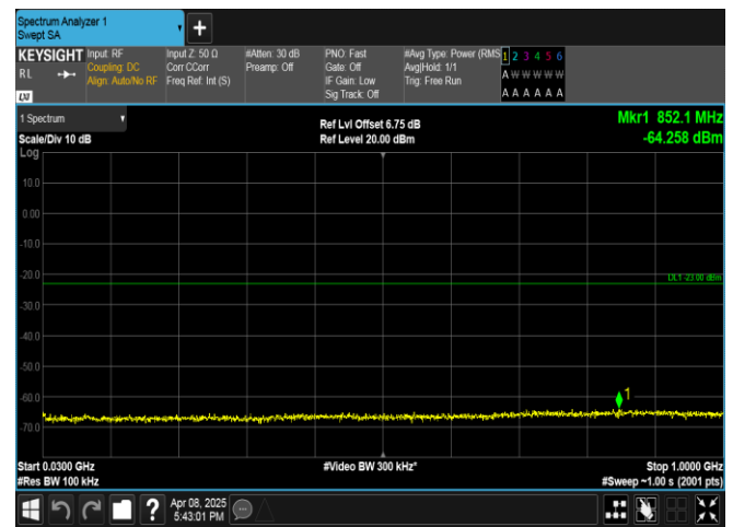
Band2-15MHz-QPSK-18675-1RB#74-30~1000-PASS
