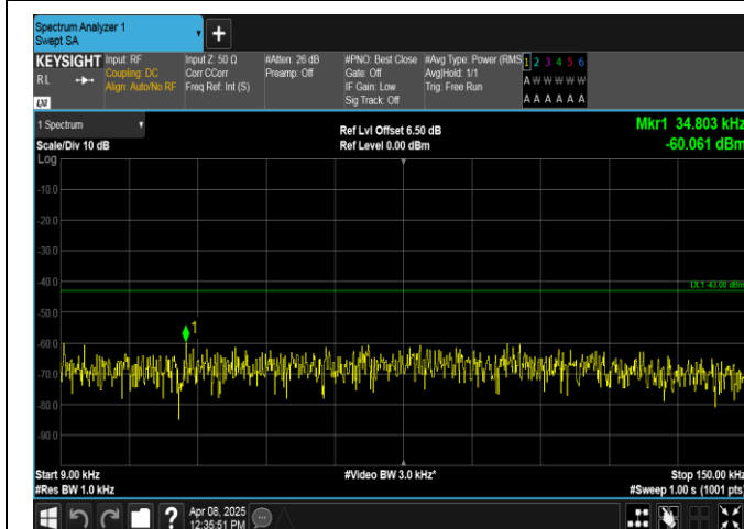
Band2-10MHz-16QAM-18650-1RB#49-0.009~0.15-PASS
