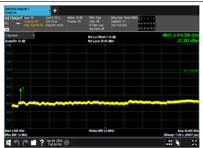
Band2-10MHz-16QAM-19150-50RB#0-3000~20000-PASS
