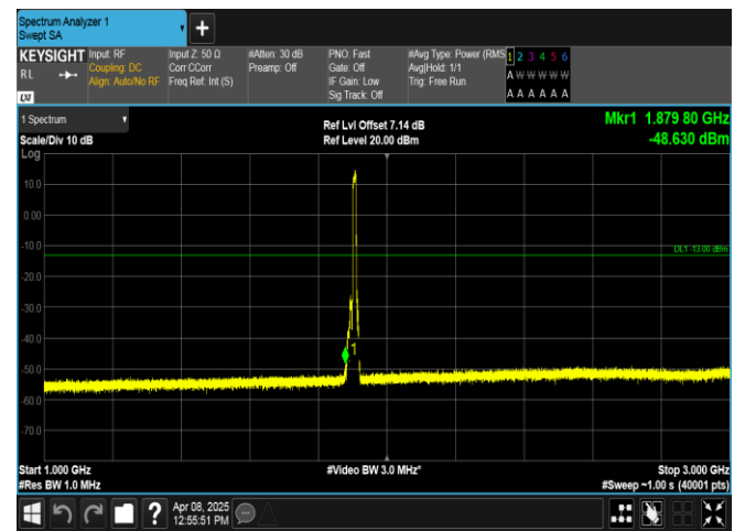
Band2-10MHz-QPSK-19150-50RB#0-1000~3000-PASS
