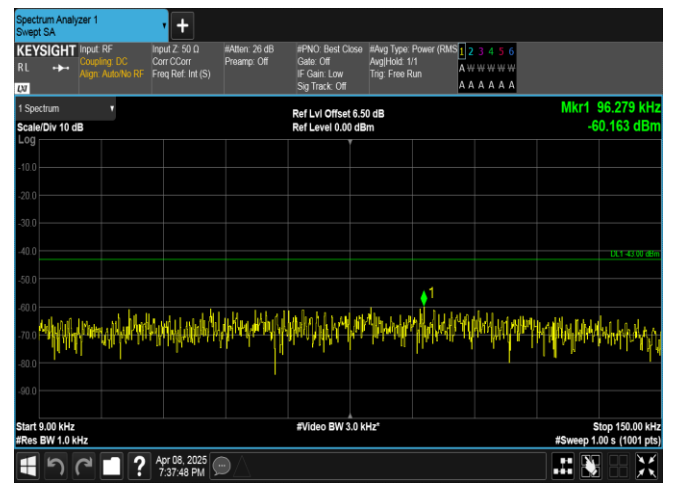
Band2-10MHz-16QAM-18650-50RB#0-0.009~0.15-PASS
