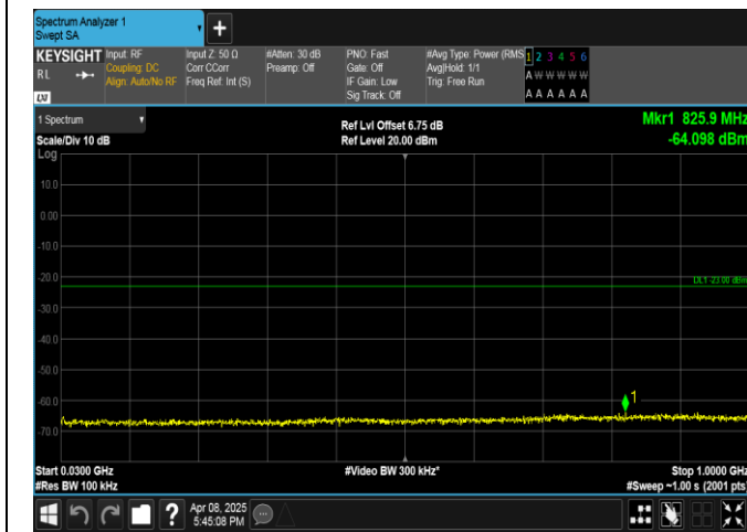
Band2-15MHz-QPSK-18675-75RB#0-30~1000-PASS
