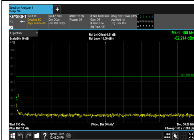
Band2-10MHz-QPSK-18900-50RB#0-0.15~30-PASS
