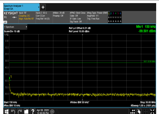
Band2-10MHz-16QAM-18650-1RB#49-0.15~30-PASS
