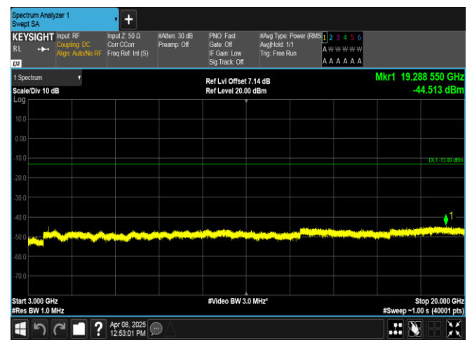
Band2-10MHz-16QAM-19150-1RB#0-3000~20000-PASS
