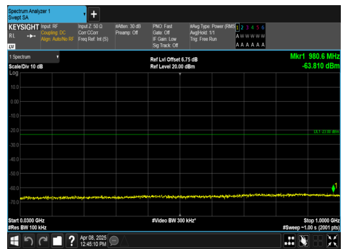
Band2-10MHz-16QAM-18900-1RB#49-30~1000-PASS
