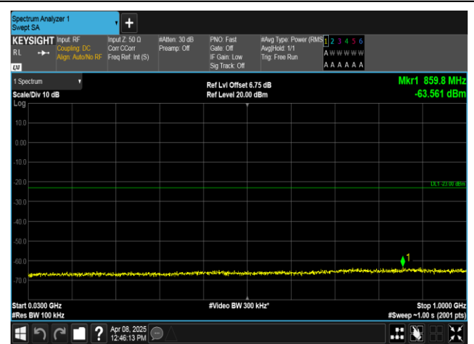
Band2-10MHz-QPSK-18900-50RB#0-30~1000-PASS
