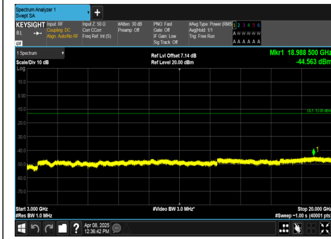
Band2-10MHz-16QAM-18650-1RB#49-3000~20000-PASS
