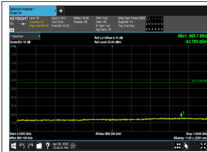
Band2-10MHz-16QAM-19150-1RB#49-30~1000-PASS
