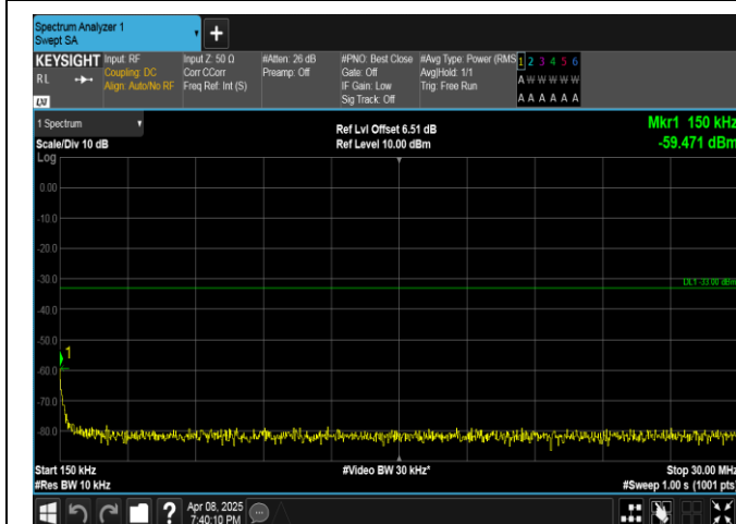
Band2-10MHz-16QAM-19150-50RB#0-0.15~30-PASS
