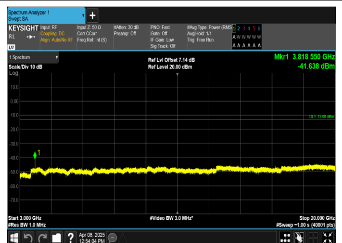
Band2-10MHz-QPSK-19150-1RB#49-3000~20000-PASS
