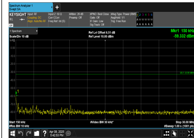
Band2-15MHz-QPSK-18675-1RB#74-0.15~30-PASS
