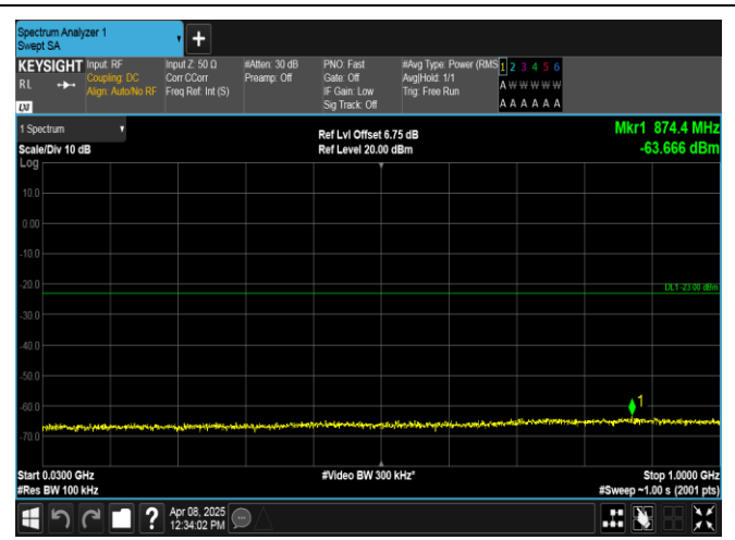
Band2-10MHz-16QAM-18650-1RB#0-30~1000-PASS
