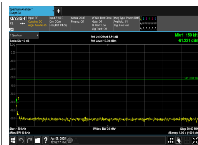
Band2-10MHz-16QAM-19150-1RB#0-0.15~30-PASS
