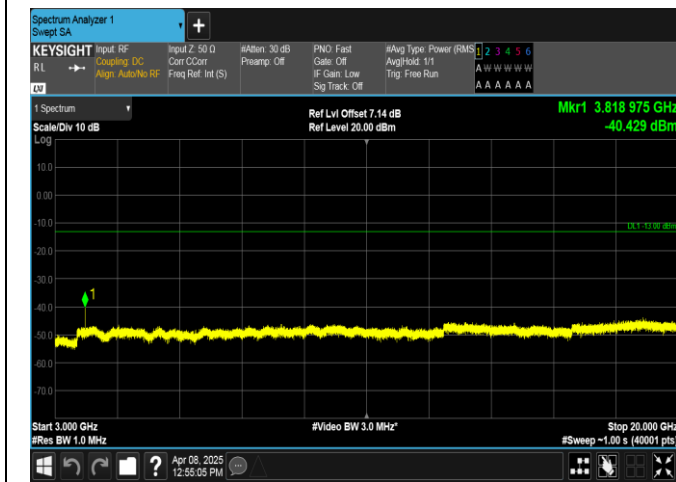
Band2-10MHz-16QAM-19150-1RB#49-3000~20000-PASS
