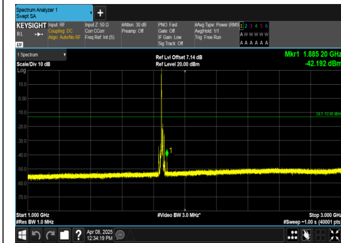
Band2-10MHz-16QAM-18650-1RB#0-1000~3000-PASS
