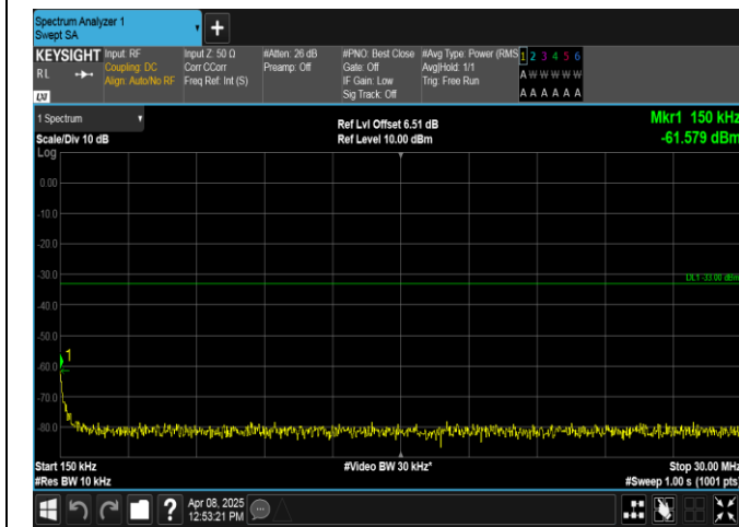
Band2-10MHz-QPSK-19150-1RB#49-0.15~30-PASS
