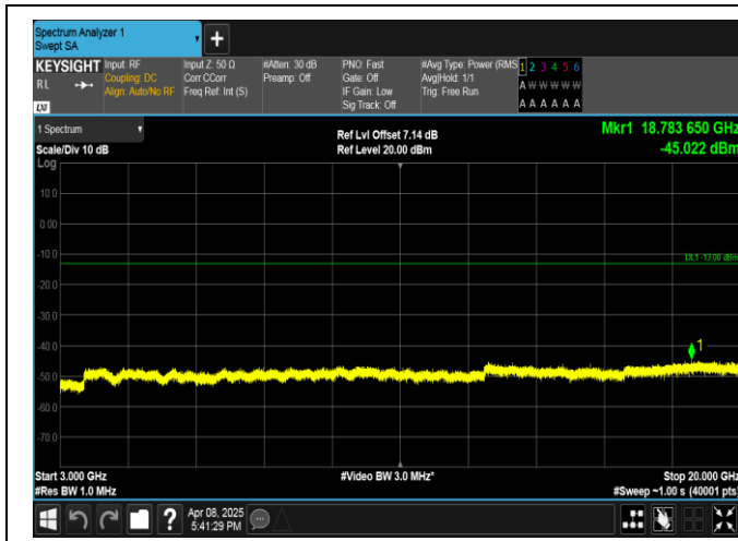
Band2-15MHz-QPSK-18675-1RB#0-3000~20000-PASS
