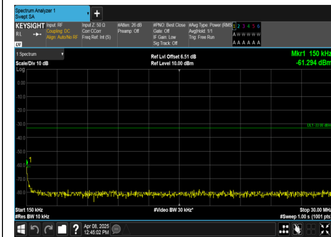
Band2-10MHz-16QAM-18900-1RB#49-0.15~30-PASS
