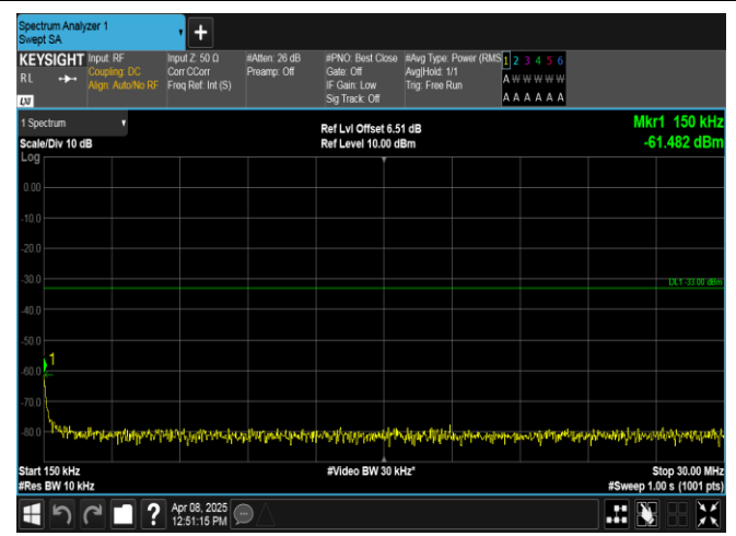
Band2-10MHz-QPSK-19150-1RB#0-0.15~30-PASS
