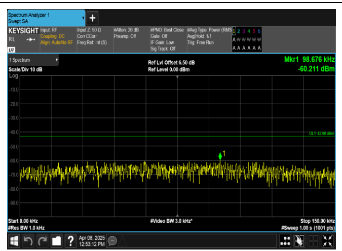
Band2-10MHz-QPSK-19150-1RB#49-0.009~0.15-PASS
