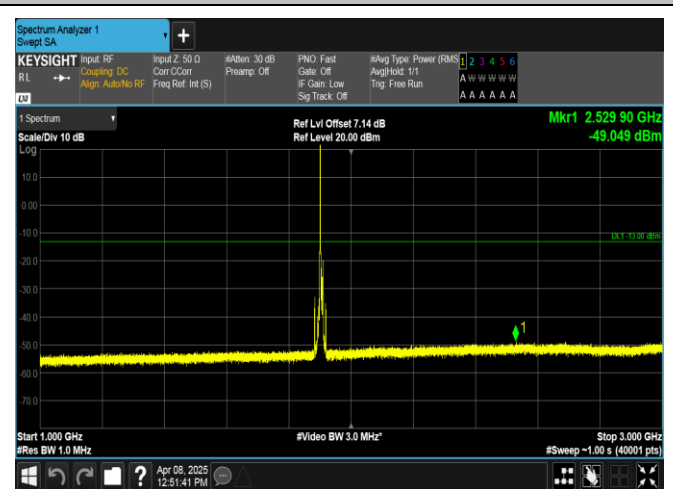
Band2-10MHz-QPSK-19150-1RB#0-1000~3000-PASS
