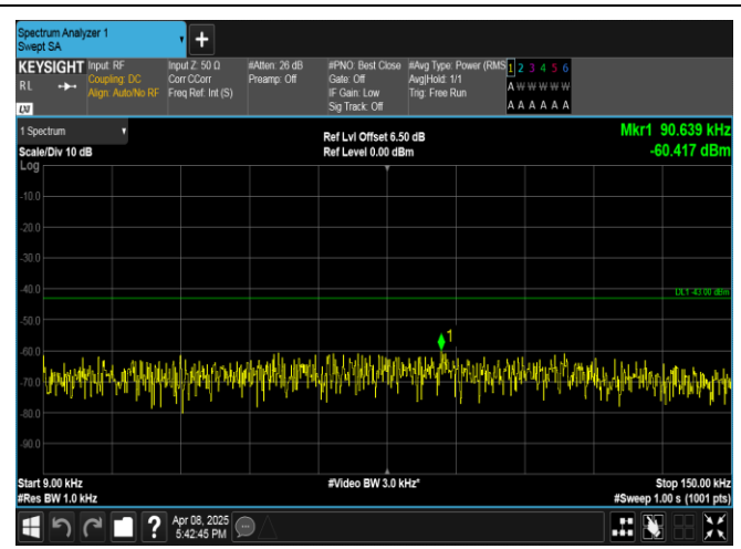
Band2-15MHz-QPSK-18675-1RB#74-0.009~0.15-PASS
