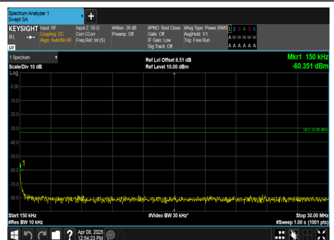
Band2-10MHz-16QAM-19150-1RB#49-0.15~30-PASS
