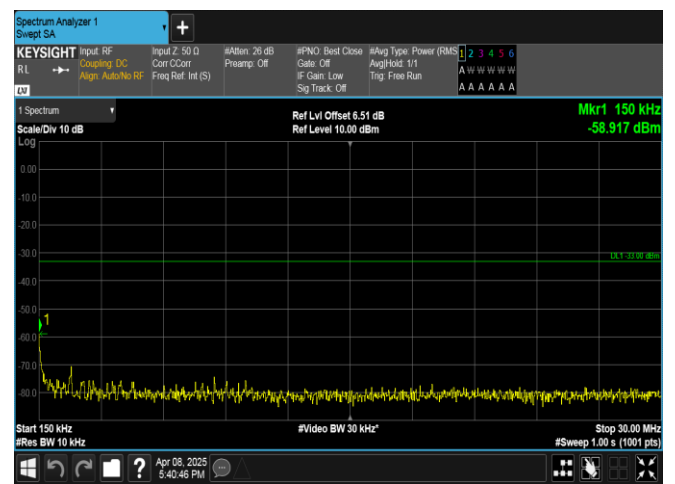
Band2-15MHz-QPSK-18675-1RB#0-0.15~30-PASS
