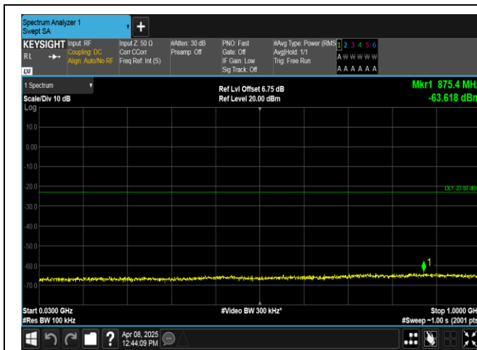
Band2-10MHz-QPSK-18900-1RB#49-30~1000-PASS
