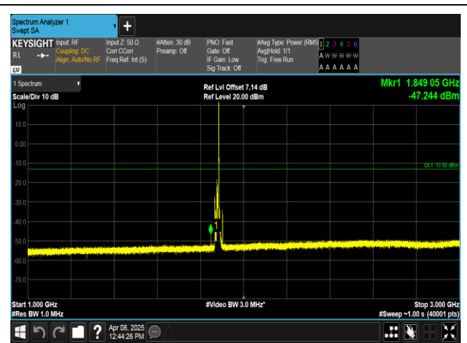
Band2-10MHz-QPSK-18900-1RB#49-1000~3000-PASS
