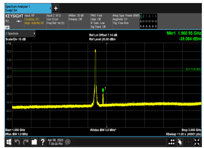
Band2-10MHz-16QAM-18900-50RB#0-1000~3000-PASS
