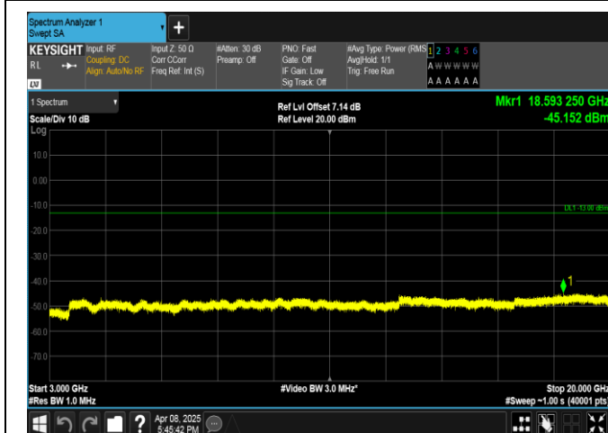
Band2-15MHz-QPSK-18675-75RB#0-3000~20000-PASS
