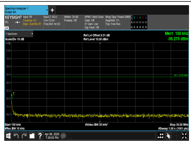
Band2-10MHz-16QAM-18900-50RB#0-0.15~30-PASS
