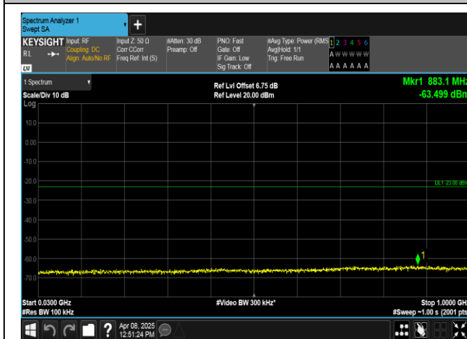
Band2-10MHz-QPSK-19150-1RB#0-30~1000-PASS
