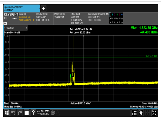
Band2-10MHz-16QAM-18650-1RB#49-1000~3000-PASS
