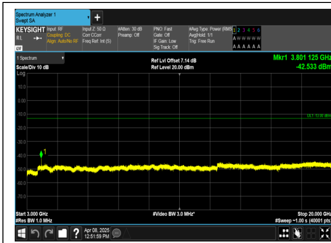
Band2-10MHz-QPSK-19150-1RB#0-3000~20000-PASS
