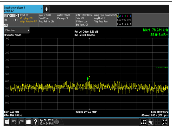
Band2-10MHz-16QAM-18900-1RB#49-0.009~0.15-PASS
