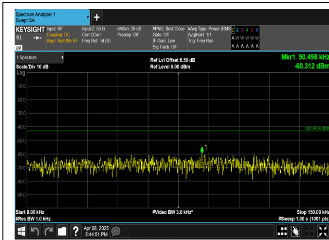
Band2-15MHz-QPSK-18675-75RB#0-0.009~0.15-PASS
