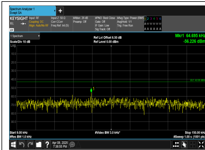
Band2-10MHz-16QAM-18900-50RB#0-0.009~0.15-PASS
