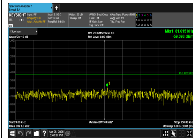
Band2-15MHz-QPSK-18675-1RB#0-0.009~0.15-PASS
