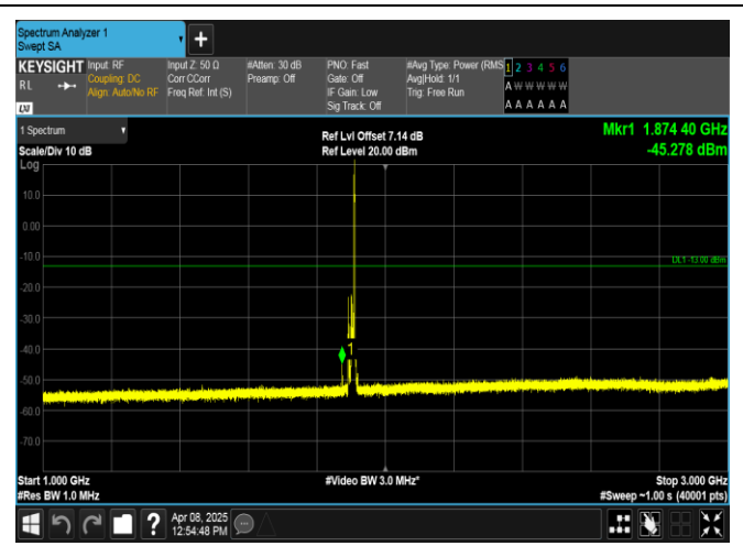
Band2-10MHz-16QAM-19150-1RB#49-1000~3000-PASS
