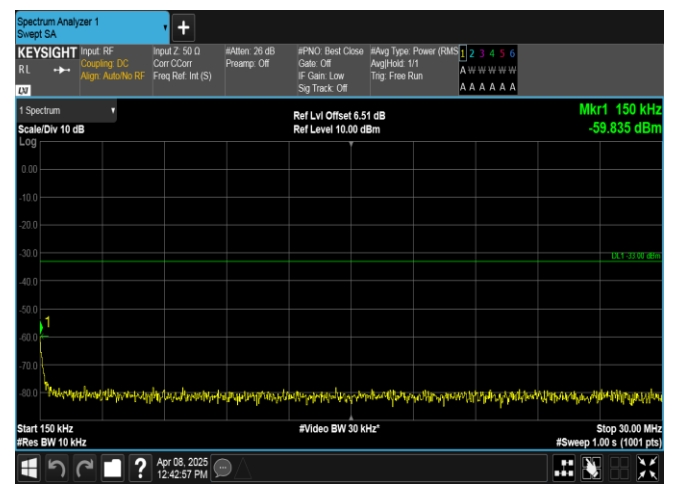
Band2-10MHz-16QAM-18900-1RB#0-0.15~30-PASS
