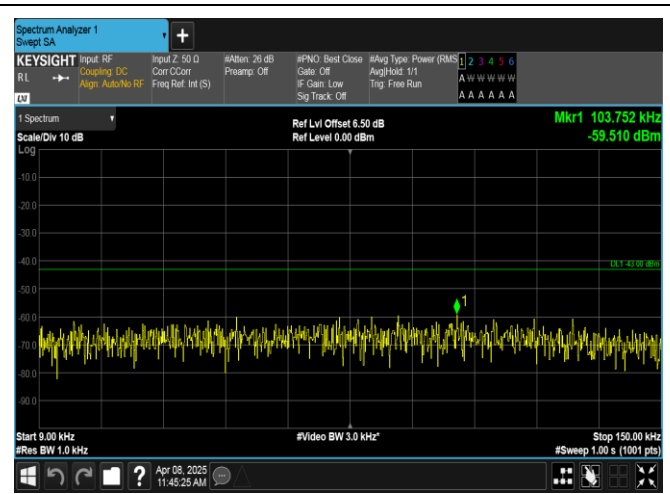
Band2-5MHz-QPSK-19175-1RB#24-0.009~0.15-PASS
