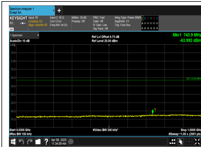
Band2-5MHz-16QAM-18625-1RB#24-30~1000-PASS
