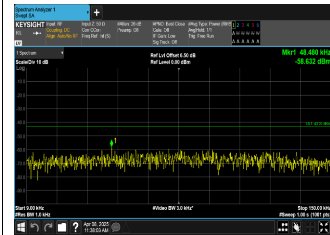
Band2-5MHz-16QAM-18900-1RB#0-0.009~0.15-PASS
