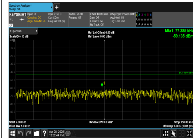
Band2-10MHz-QPSK-18650-1RB#0-0.009~0.15-PASS
