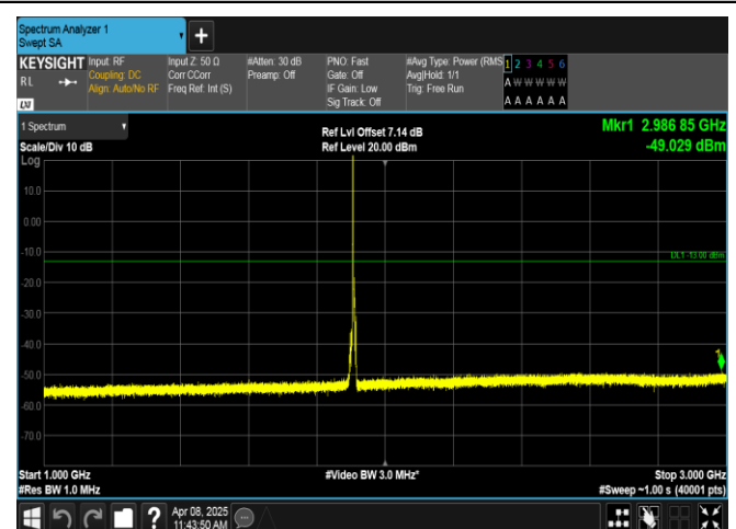
Band2-5MHz-QPSK-19175-1RB#0-1000~3000-PASS
