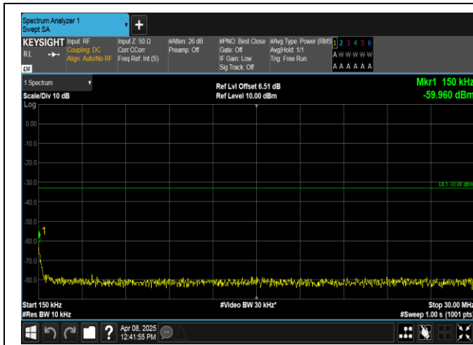
Band2-10MHz-QPSK-18900-1RB#0-0.15~30-PASS
