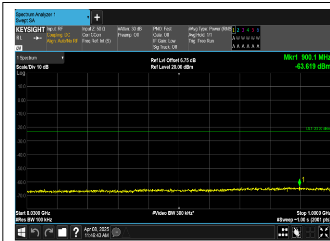
Band2-5MHz-16QAM-19175-1RB#24-30~1000-PASS
