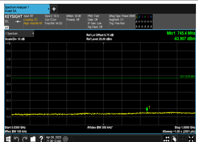
Band2-5MHz-16QAM-18625-25RB#0-30~1000-PASS
