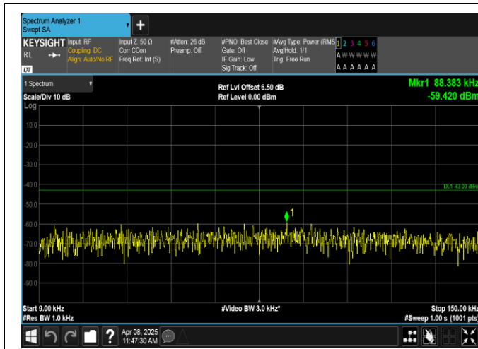
Band2-5MHz-QPSK-19175-25RB#0-0.009~0.15-PASS
