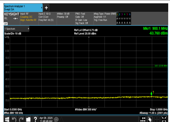
Band2-5MHz-16QAM-19175-25RB#0-30~1000-PASS
