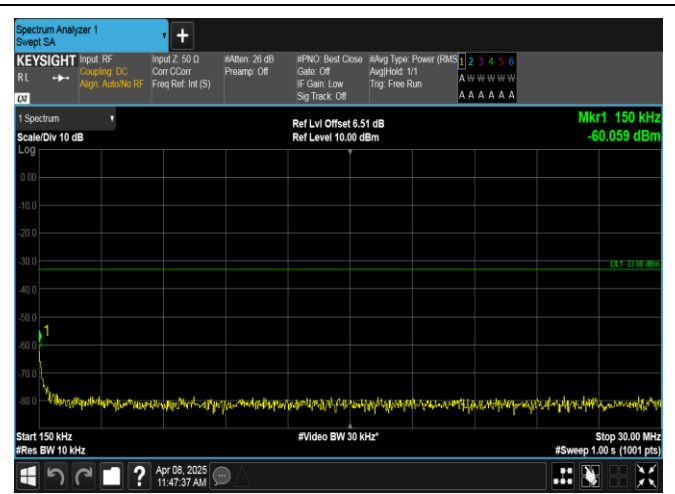
Band2-5MHz-QPSK-19175-25RB#0-0.15~30-PASS
