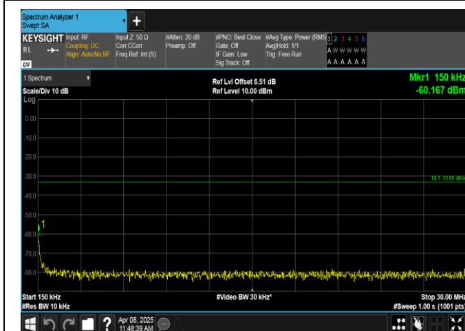
Band2-5MHz-16QAM-19175-25RB#0-0.15~30-PASS
