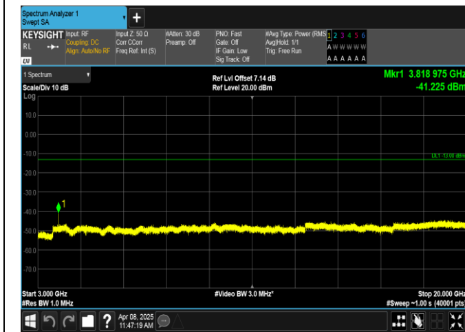
Band2-5MHz-16QAM-19175-1RB#24-3000~20000-PASS
