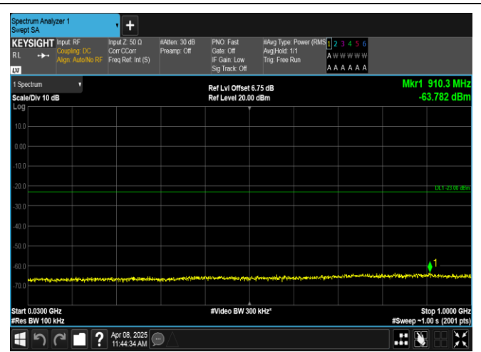
Band2-5MHz-16QAM-19175-1RB#0-30~1000-PASS
