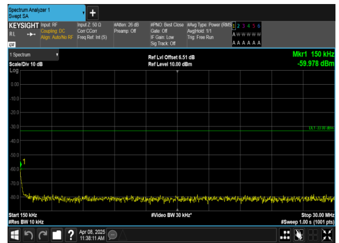
Band2-5MHz-16QAM-18900-1RB#0-0.15~30-PASS
