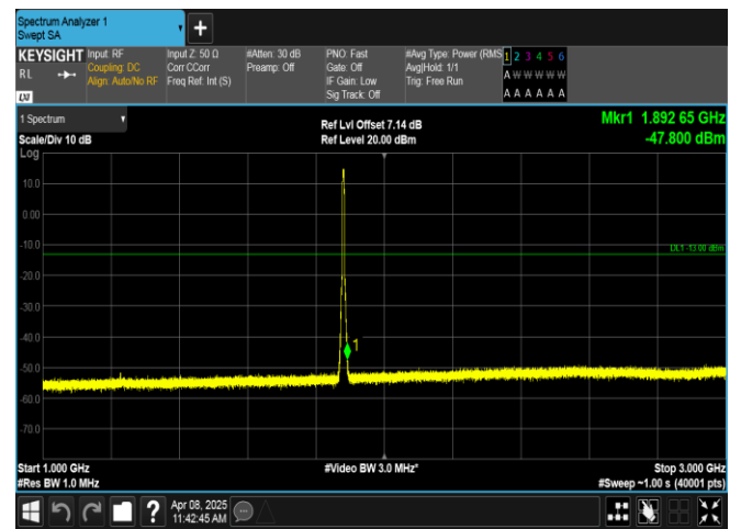
Band2-5MHz-16QAM-18900-25RB#0-1000~3000-PASS
