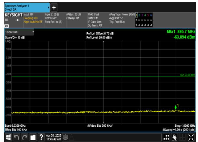
Band2-5MHz-QPSK-19175-1RB#24-30~1000-PASS
