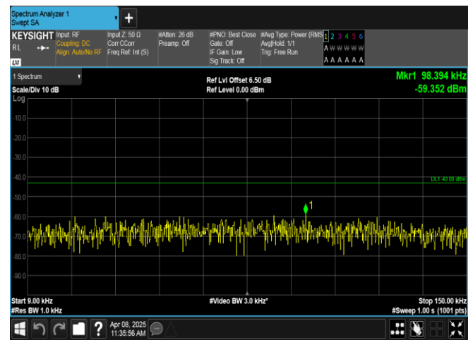
Band2-5MHz-16QAM-18625-25RB#0-0.009~0.15-PASS
