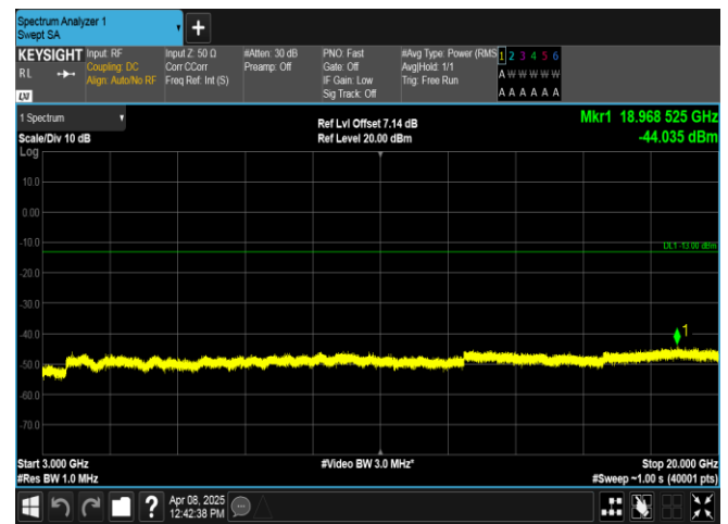
Band2-10MHz-QPSK-18900-1RB#0-3000~20000-PASS
