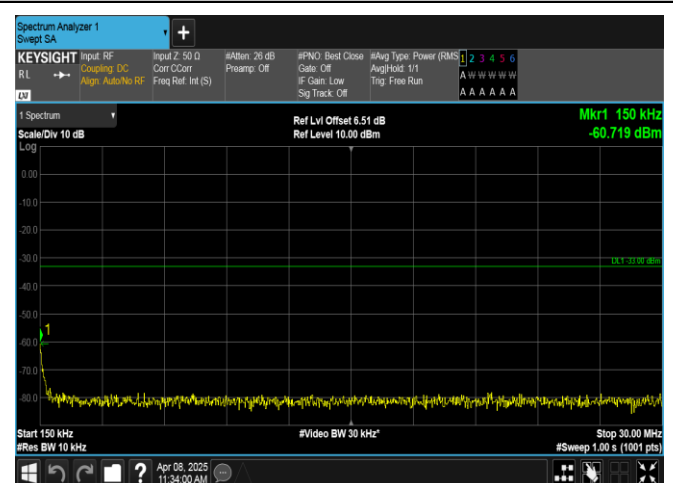
Band2-5MHz-16QAM-18625-1RB#24-0.15~30-PASS
