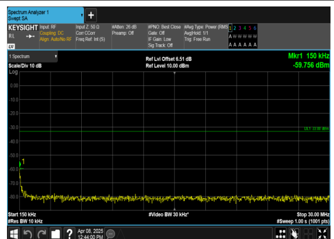
Band2-10MHz-QPSK-18900-1RB#49-0.15~30-PASS
