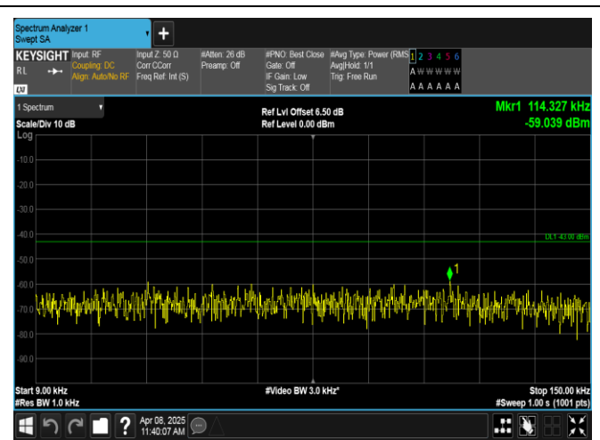
Band2-5MHz-16QAM-18900-1RB#24-0.009~0.15-PASS
