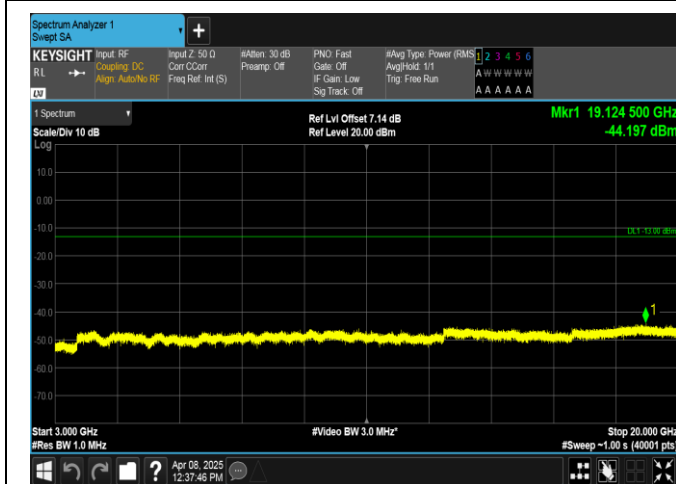
Band2-10MHz-QPSK-18650-50RB#0-3000~20000-PASS
