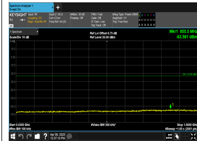
Band2-10MHz-QPSK-18650-50RB#0-30~1000-PASS
