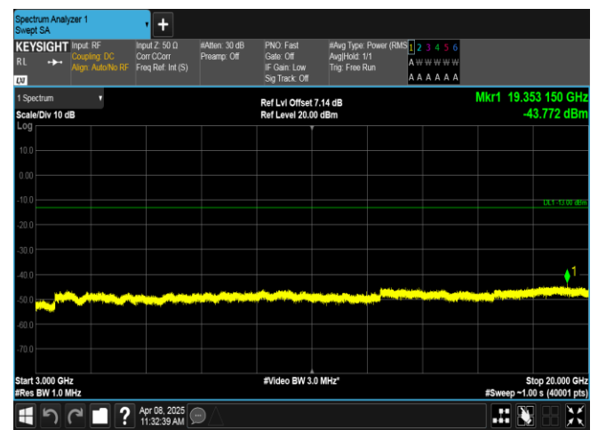
Band2-5MHz-16QAM-18625-1RB#0-3000~20000-PASS
