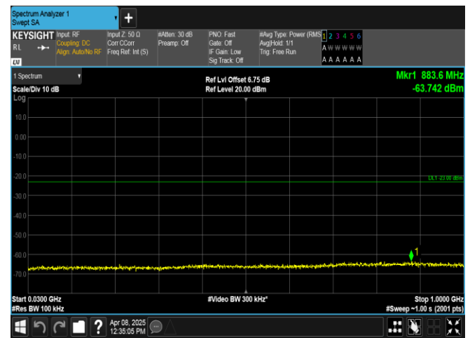
Band2-10MHz-QPSK-18650-1RB#49-30~1000-PASS
