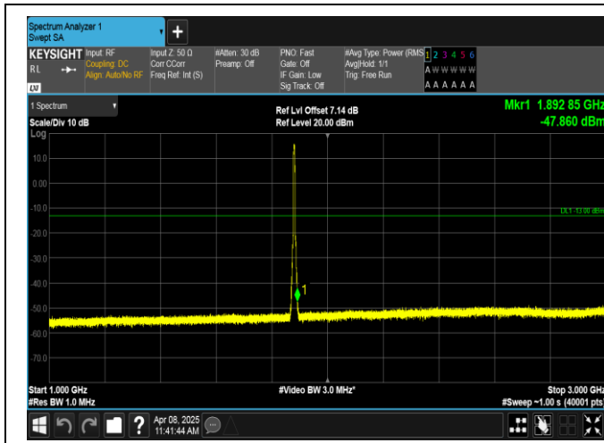
Band2-5MHz-QPSK-18900-25RB#0-1000~3000-PASS
