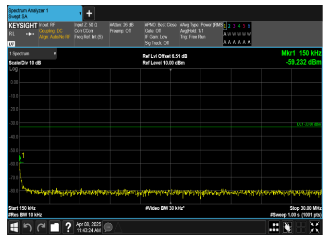
Band2-5MHz-QPSK-19175-1RB#0-0.15~30-PASS
