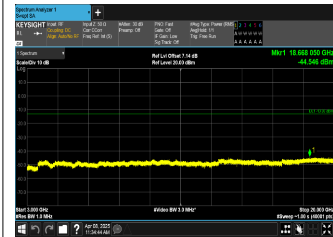
Band2-5MHz-16QAM-18625-1RB#24-3000~20000-PASS
