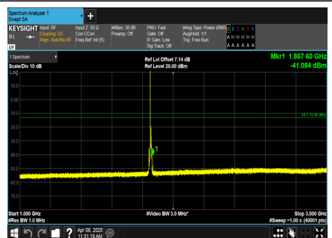
Band2-5MHz-QPSK-18625-1RB#0-1000~3000-PASS
