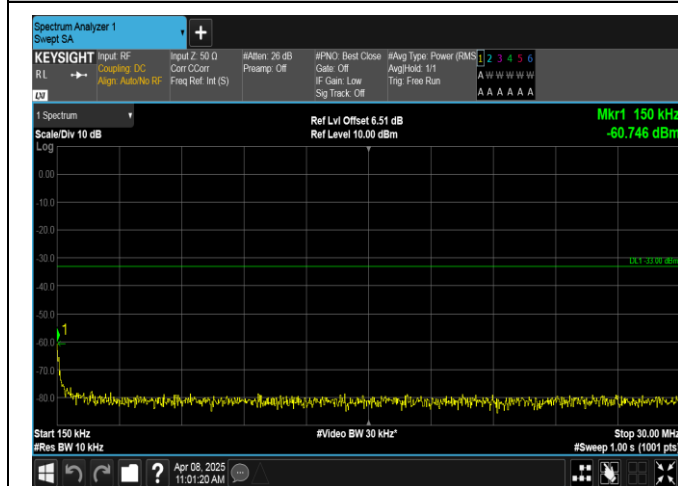
Band2-3MHz-16QAM-19185-15RB#0-0.15~30-PASS
