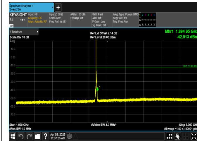
Band2-5MHz-QPSK-18900-1RB#0-1000~3000-PASS
