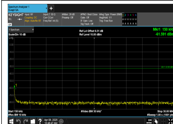
Band2-3MHz-16QAM-18615-15RB#0-0.15~30-PASS
