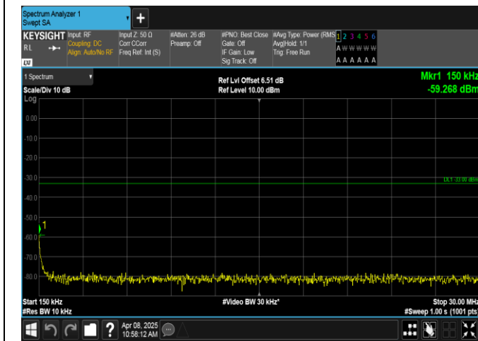
Band2-3MHz-QPSK-19185-1RB#14-0.15~30-PASS
