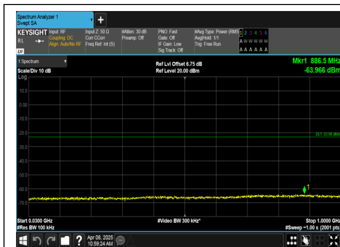
Band2-3MHz-16QAM-19185-1RB#14-30~1000-PASS
