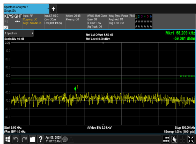
Band2-3MHz-16QAM-19185-15RB#0-0.009~0.15-PASS
