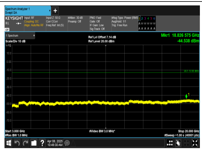
Band2-3MHz-16QAM-18615-15RB#0-3000~20000-PASS
