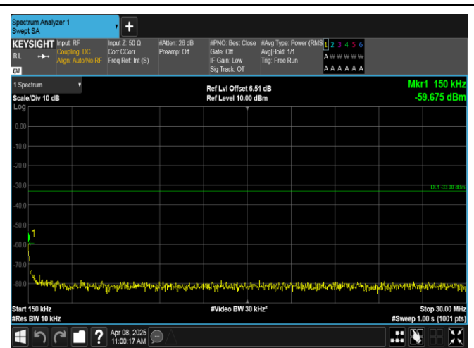
Band2-3MHz-QPSK-19185-15RB#0-0.15~30-PASS
