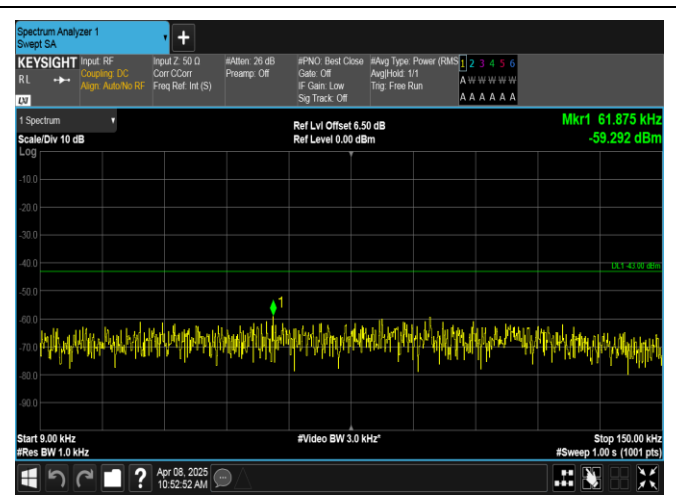
Band2-3MHz-16QAM-18900-1RB#14-0.009~0.15-PASS
