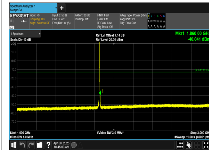
Band2-3MHz-16QAM-18615-1RB#0-1000~3000-PASS
