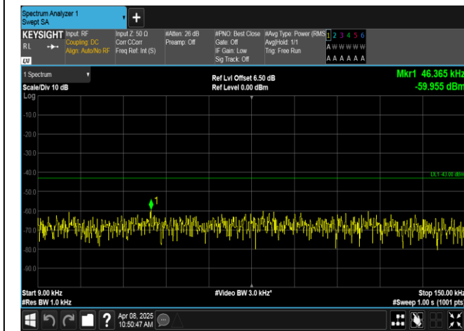
Band2-3MHz-16QAM-18900-1RB#0-0.009~0.15-PASS
