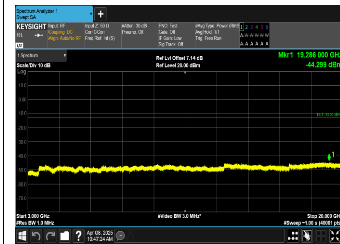
Band2-3MHz-16QAM-18615-1RB#14-3000~20000-PASS
