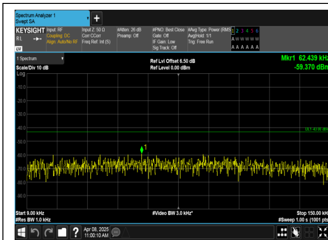
Band2-3MHz-QPSK-19185-15RB#0-0.009~0.15-PASS
