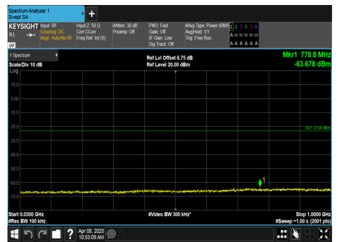
Band2-3MHz-16QAM-18900-1RB#14-30~1000-PASS
