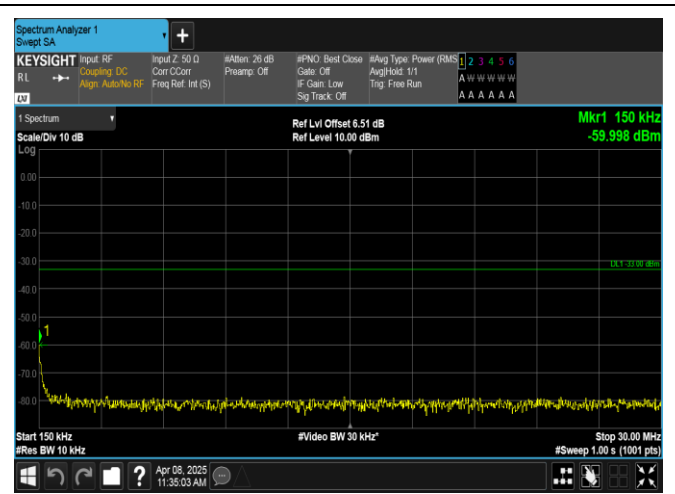
Band2-5MHz-QPSK-18625-25RB#0-0.15~30-PASS
