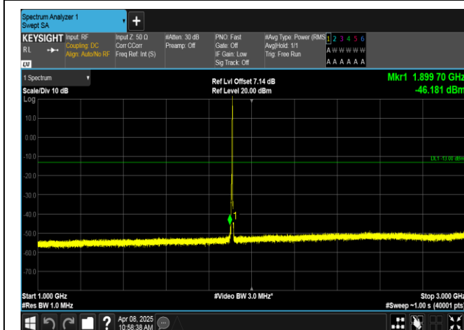
Band2-3MHz-QPSK-19185-1RB#14-1000~3000-PASS
