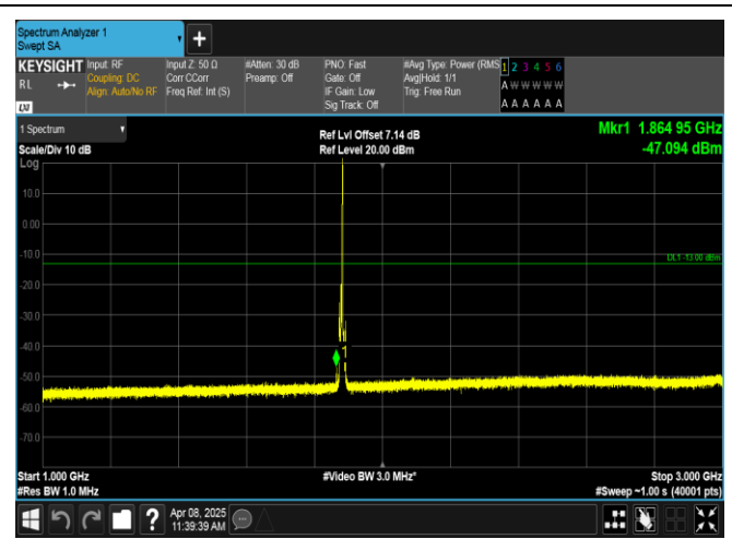
Band2-5MHz-QPSK-18900-1RB#24-1000~3000-PASS
