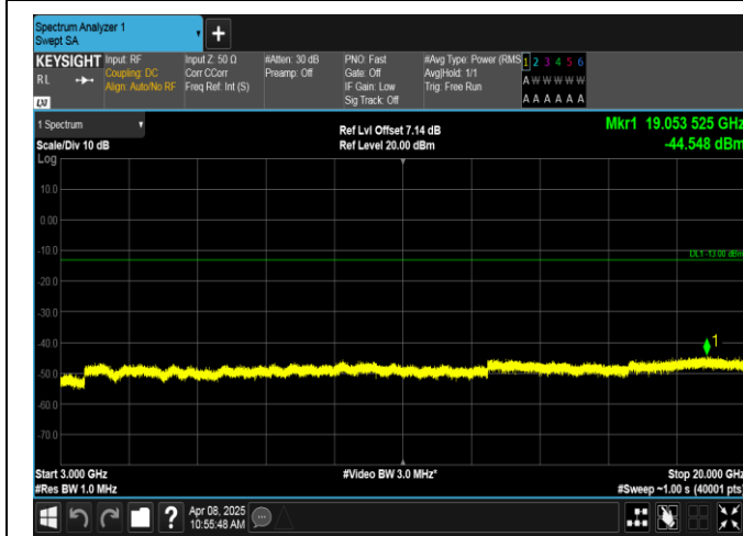
Band2-3MHz-16QAM-18900-15RB#0-3000~20000-PASS
