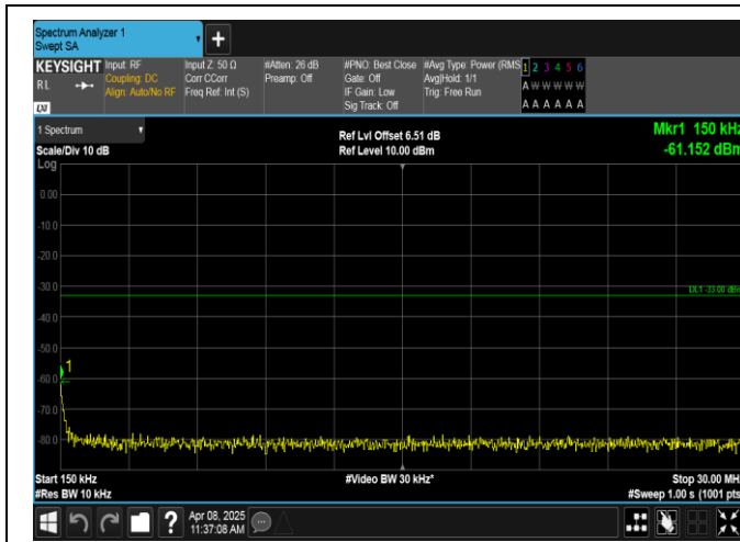
Band2-5MHz-QPSK-18900-1RB#0-0.15~30-PASS
