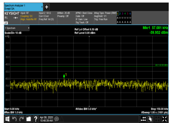
Band2-3MHz-16QAM-18615-15RB#0-0.009~0.15-PASS
