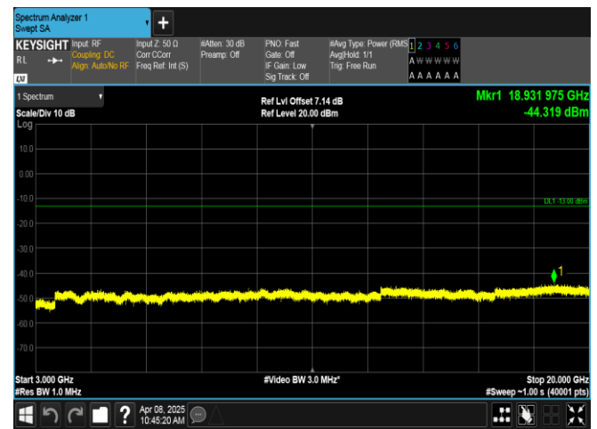
Band2-3MHz-16QAM-18615-1RB#0-3000~20000-PASS
