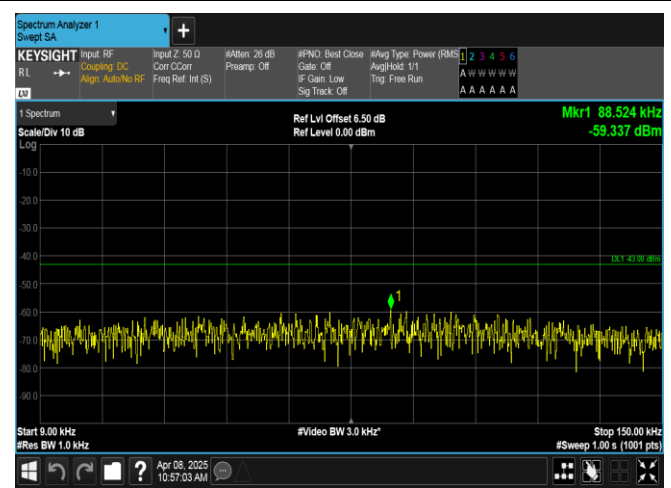
Band2-3MHz-16QAM-19185-1RB#0-0.009~0.15-PASS
