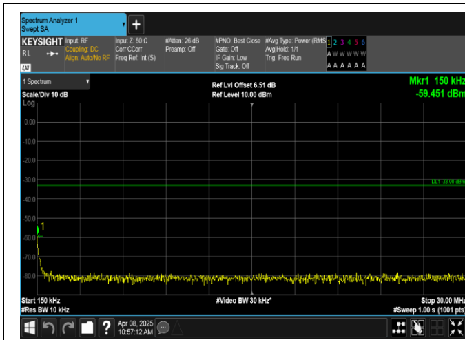
Band2-3MHz-16QAM-19185-1RB#0-0.15~30-PASS
