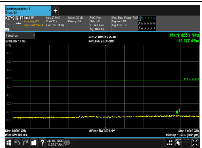
Band2-5MHz-QPSK-18900-1RB#0-30~1000-PASS
