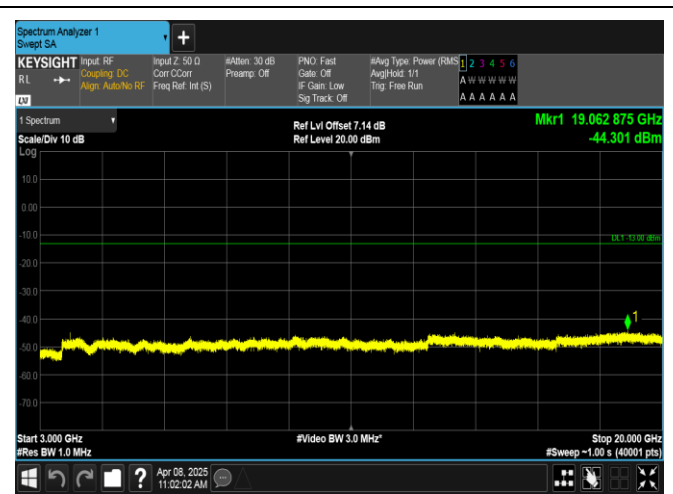
Band2-3MHz-16QAM-19185-15RB#0-3000~20000-PASS
