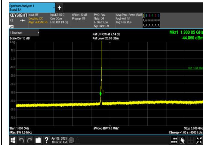
Band2-3MHz-16QAM-19185-1RB#0-1000~3000-PASS
