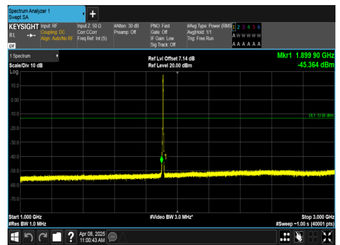
Band2-3MHz-QPSK-19185-15RB#0-1000~3000-PASS
