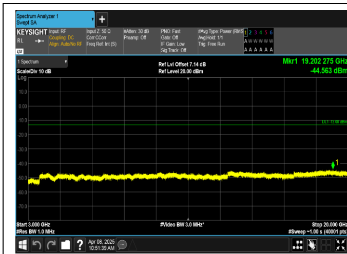
Band2-3MHz-16QAM-18900-1RB#0-3000~20000-PASS
