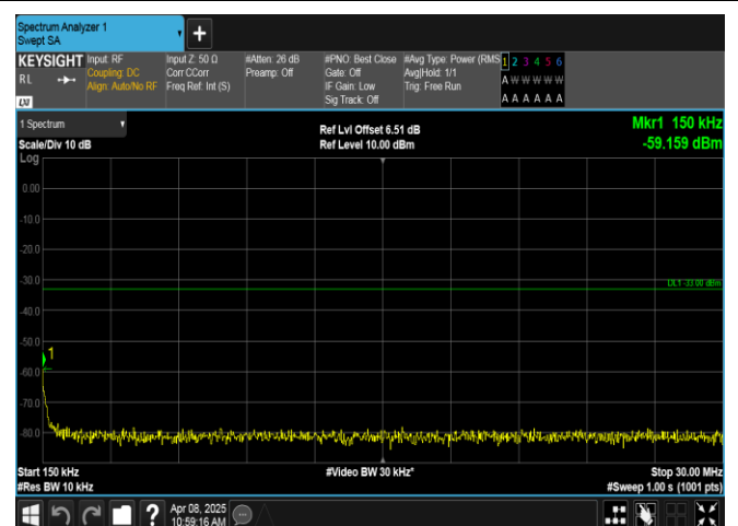
Band2-3MHz-16QAM-19185-1RB#14-0.15~30-PASS
