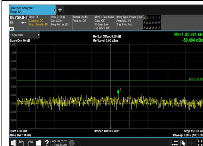
Band2-3MHz-16QAM-18615-1RB#14-0.009~0.15-PASS
