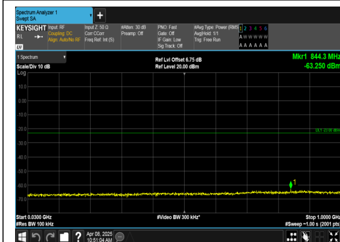
Band2-3MHz-16QAM-18900-1RB#0-30~1000-PASS
