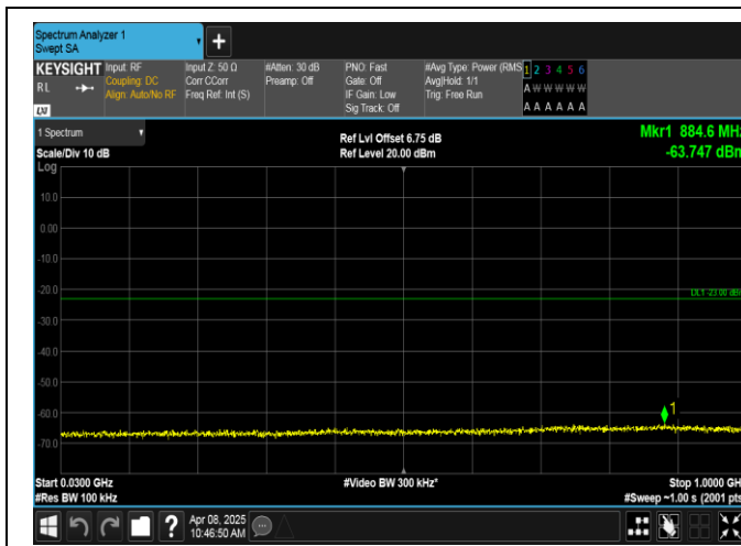
Band2-3MHz-16QAM-18615-1RB#14-30~1000-PASS
