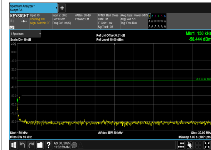
Band2-5MHz-QPSK-18625-1RB#24-0.15~30-PASS
