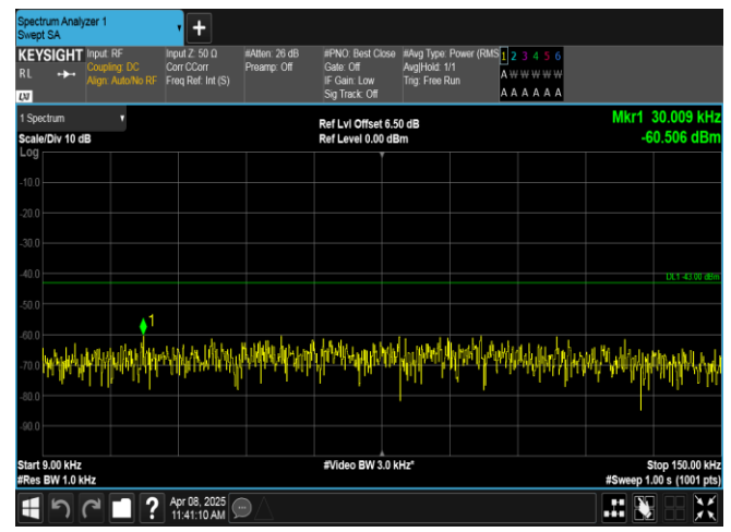
Band2-5MHz-QPSK-18900-25RB#0-0.009~0.15-PASS
