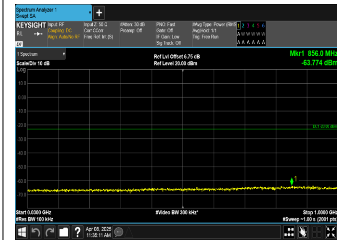
Band2-5MHz-QPSK-18625-25RB#0-30~1000-PASS
