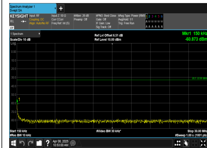
Band2-3MHz-16QAM-18900-1RB#14-0.15~30-PASS
