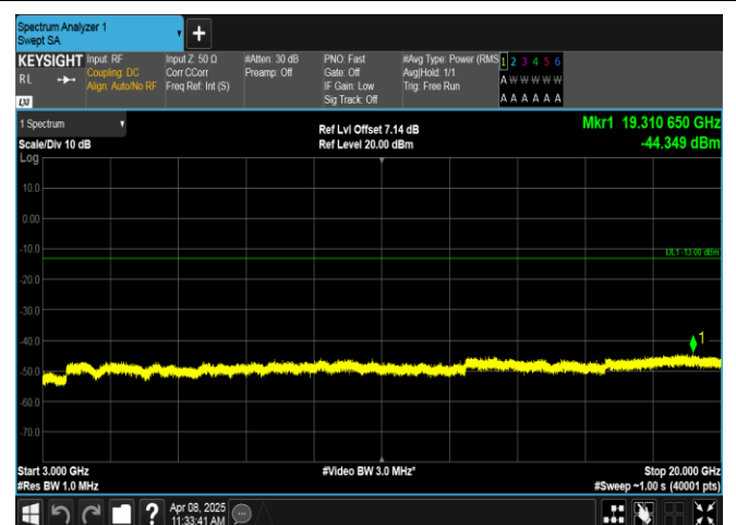
Band2-5MHz-QPSK-18625-1RB#24-3000~20000-PASS
