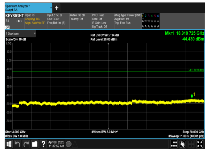
Band2-5MHz-QPSK-18900-1RB#0-3000~20000-PASS
