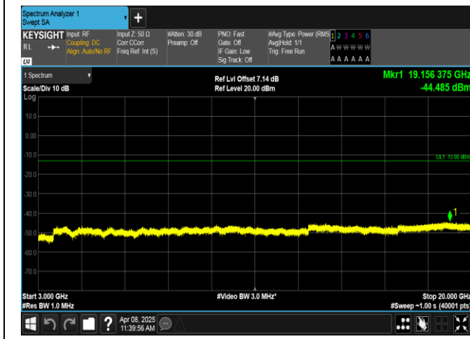
Band2-5MHz-QPSK-18900-1RB#24-3000~20000-PASS
