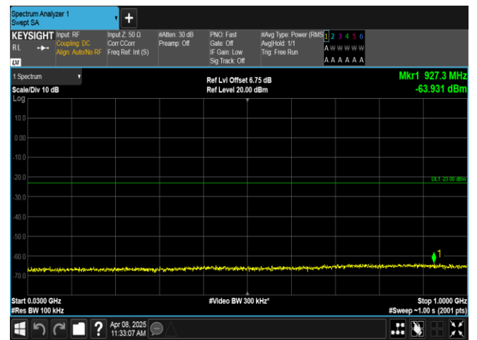
Band2-5MHz-QPSK-18625-1RB#24-30~1000-PASS
