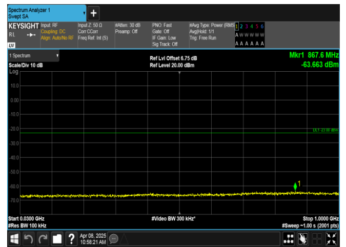
Band2-3MHz-QPSK-19185-1RB#14-30~1000-PASS
