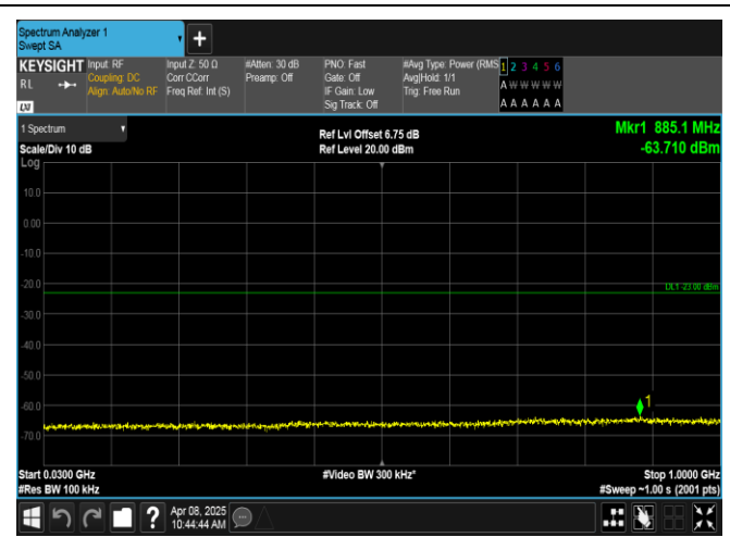
Band2-3MHz-16QAM-18615-1RB#0-30~1000-PASS
