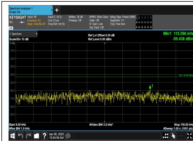
Band2-3MHz-16QAM-18900-15RB#0-0.009~0.15-PASS
