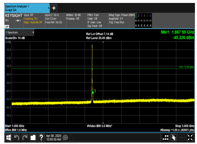
Band2-3MHz-16QAM-18900-15RB#0-1000~3000-PASS
