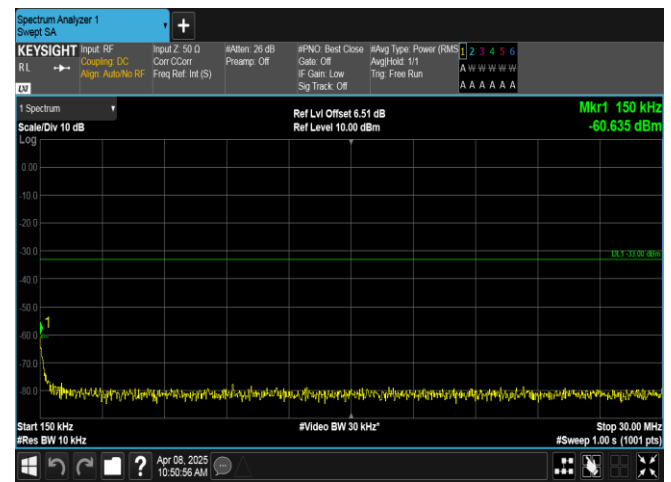
Band2-3MHz-16QAM-18900-1RB#0-0.15~30-PASS
