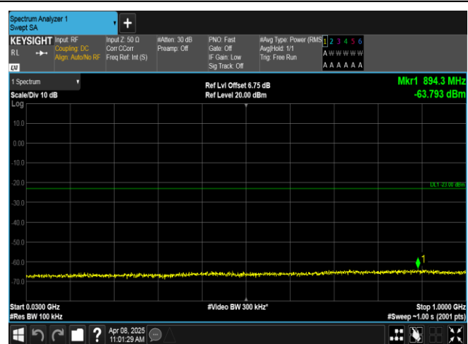
Band2-3MHz-16QAM-19185-15RB#0-30~1000-PASS
