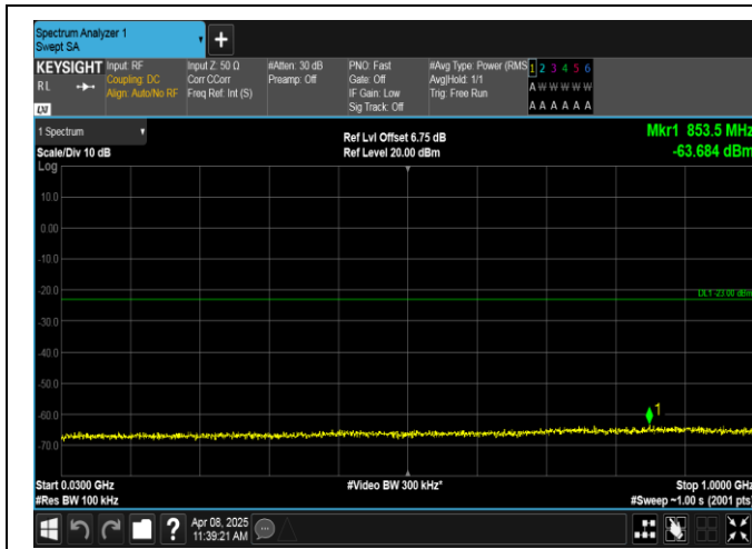
Band2-5MHz-QPSK-18900-1RB#24-30~1000-PASS
