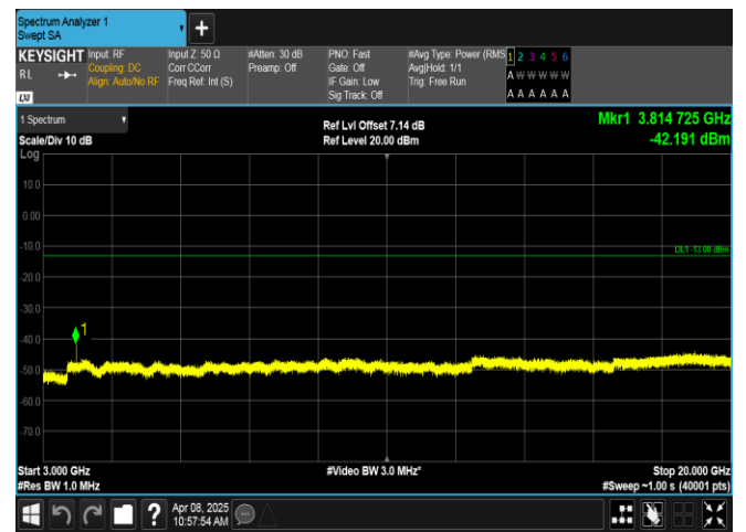
Band2-3MHz-16QAM-19185-1RB#0-3000~20000-PASS
