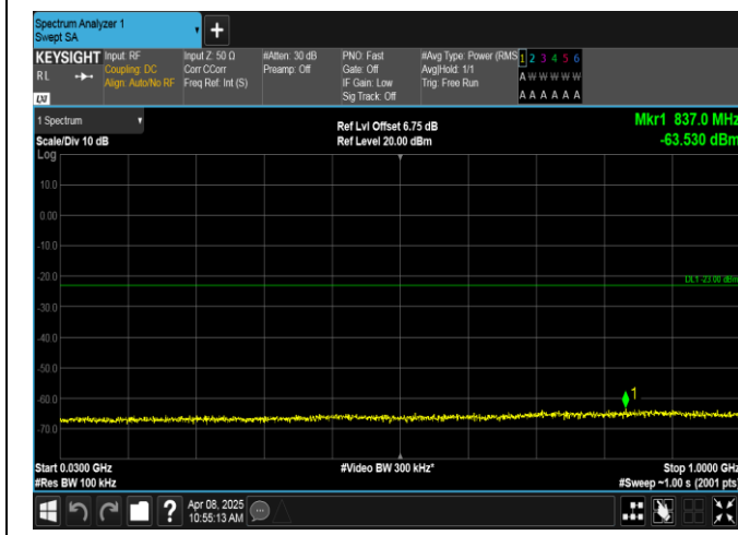
Band2-3MHz-16QAM-18900-15RB#0-30~1000-PASS
