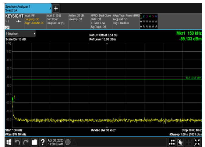
Band2-5MHz-QPSK-18625-1RB#0-0.15~30-PASS
