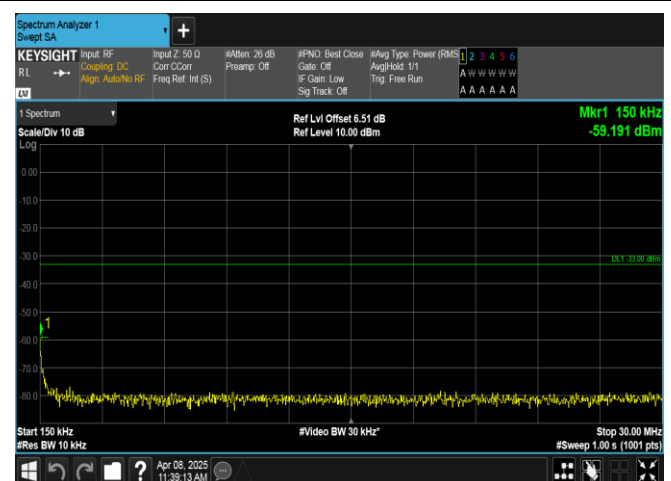
Band2-5MHz-QPSK-18900-1RB#24-0.15~30-PASS
