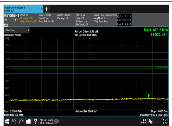
Band2-3MHz-16QAM-19185-1RB#0-30~1000-PASS
