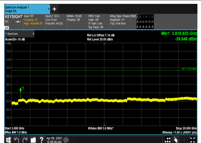
Band2-3MHz-QPSK-19185-1RB#14-3000~20000-PASS
