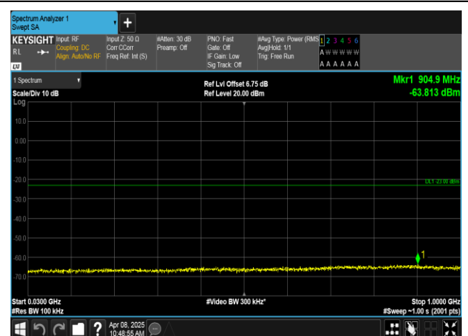
Band2-3MHz-16QAM-18615-15RB#0-30~1000-PASS
