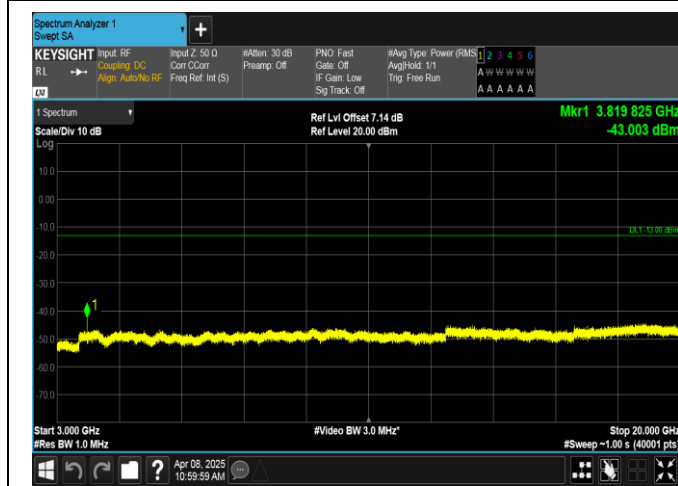
Band2-3MHz-16QAM-19185-1RB#14-3000~20000-PASS
