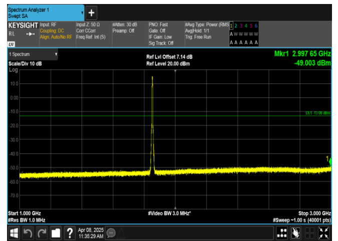
Band2-5MHz-QPSK-18625-25RB#0-1000~3000-PASS
