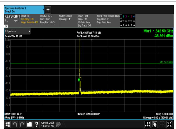
Band2-3MHz-16QAM-18615-1RB#14-1000~3000-PASS
