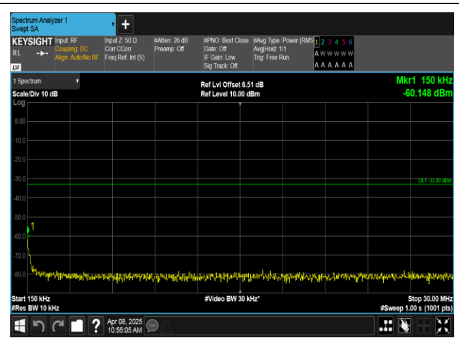
Band2-3MHz-16QAM-18900-15RB#0-0.15~30-PASS
