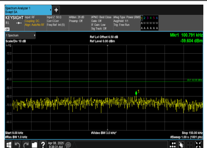
Band2-1.4MHz-16QAM-19193-1RB#0-0.009~0.15-PASS
