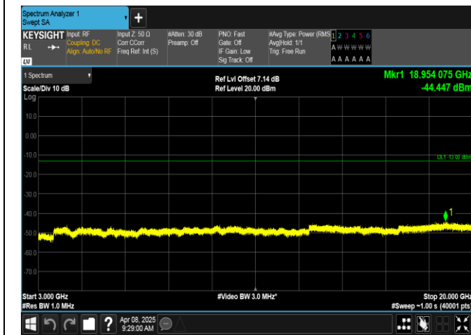
Band2-1.4MHz-16QAM-18607-1RB#5-3000~20000-PASS
