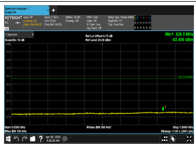
Band2-1.4MHz-16QAM-18607-1RB#0-30~1000-PASS
