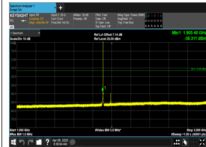
Band2-1.4MHz-16QAM-19193-1RB#0-1000~3000-PASS
