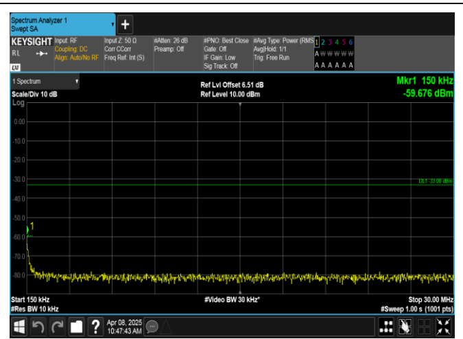
Band2-3MHz-QPSK-18615-15RB#0-0.15~30-PASS
