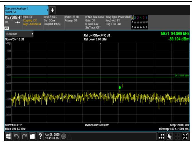
Band2-3MHz-QPSK-18615-1RB#14-0.009~0.15-PASS
