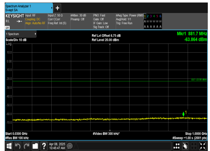
Band2-3MHz-QPSK-18615-1RB#14-30~1000-PASS
