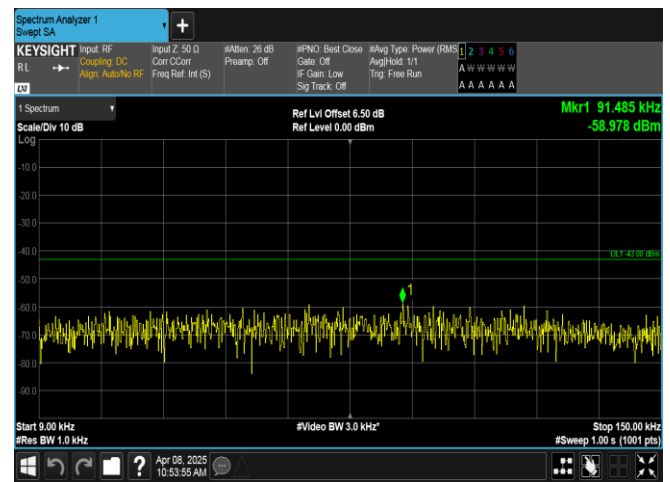
Band2-3MHz-QPSK-18900-15RB#0-0.009~0.15-PASS
