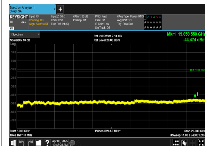
Band2-3MHz-QPSK-18615-15RB#0-3000~20000-PASS
