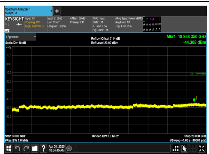
Band2-3MHz-QPSK-18900-15RB#0-3000~20000-PASS
