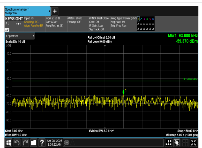
Band2-1.4MHz-16QAM-18900-1RB#5-0.009~0.15-PASS
