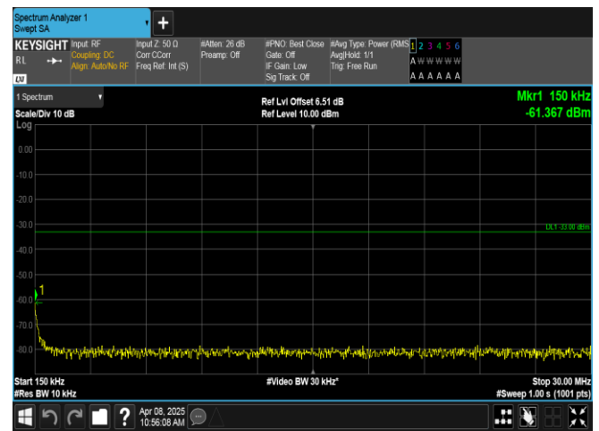
Band2-3MHz-QPSK-19185-1RB#0-0.15~30-PASS
