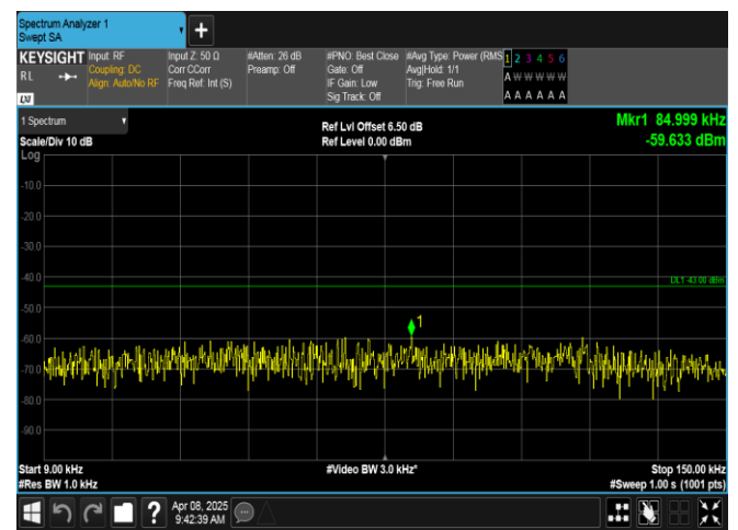
Band2-1.4MHz-16QAM-19193-6RB#0-0.009~0.15-PASS
