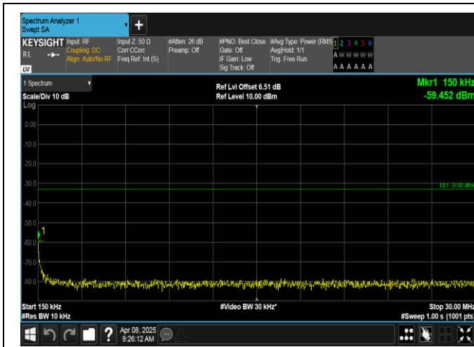
Band2-1.4MHz-16QAM-18607-1RB#0-0.15~30-PASS
