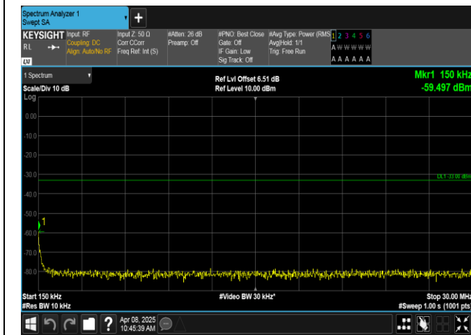
Band2-3MHz-QPSK-18615-1RB#14-0.15~30-PASS
