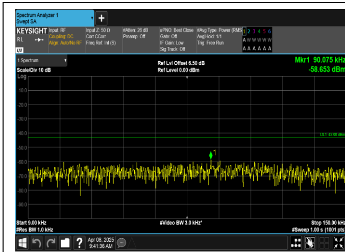
Band2-1.4MHz-QPSK-19193-6RB#0-0.009~0.15-PASS
