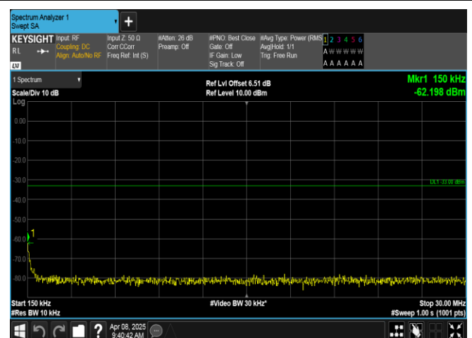
Band2-1.4MHz-16QAM-19193-1RB#5-0.15~30-PASS
