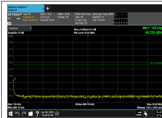
Band2-3MHz-QPSK-18900-1RB#0-0.15~30-PASS
