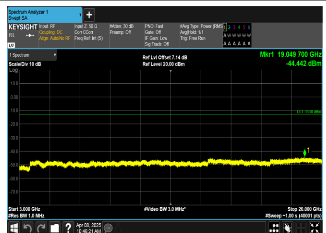
Band2-3MHz-QPSK-18615-1RB#14-3000~20000-PASS
