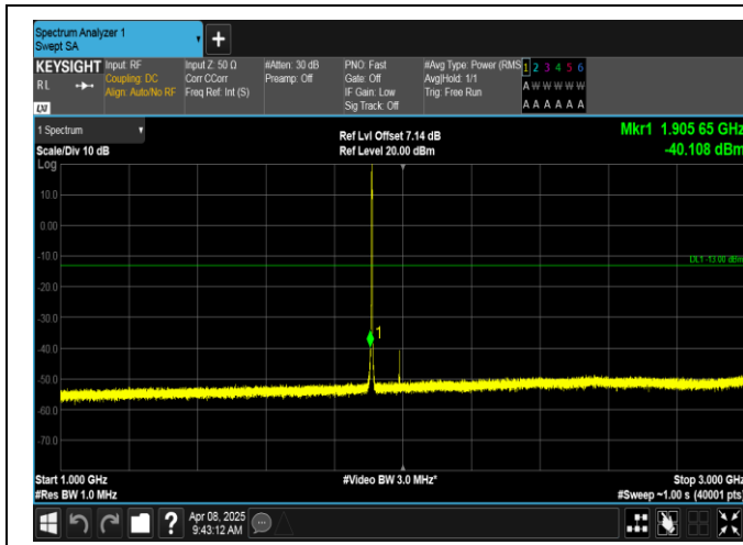
Band2-1.4MHz-16QAM-19193-6RB#0-1000~3000-PASS
