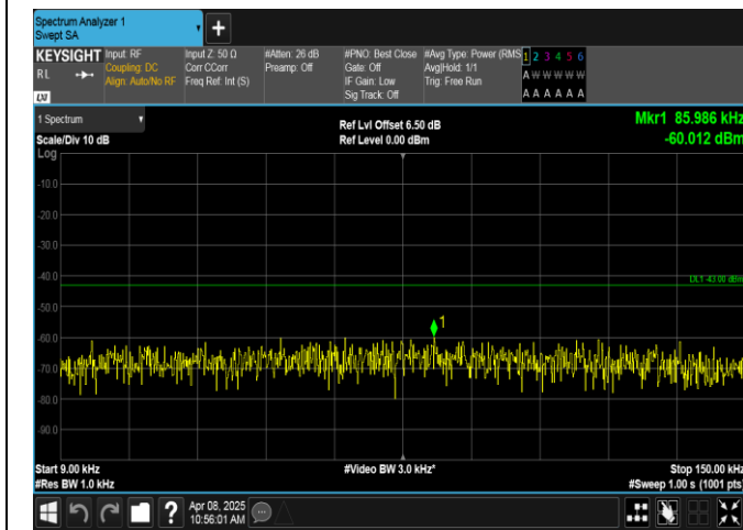
Band2-3MHz-QPSK-19185-1RB#0-0.009~0.15-PASS
