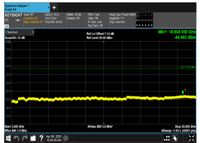
Band2-3MHz-QPSK-18900-1RB#0-3000~20000-PASS
