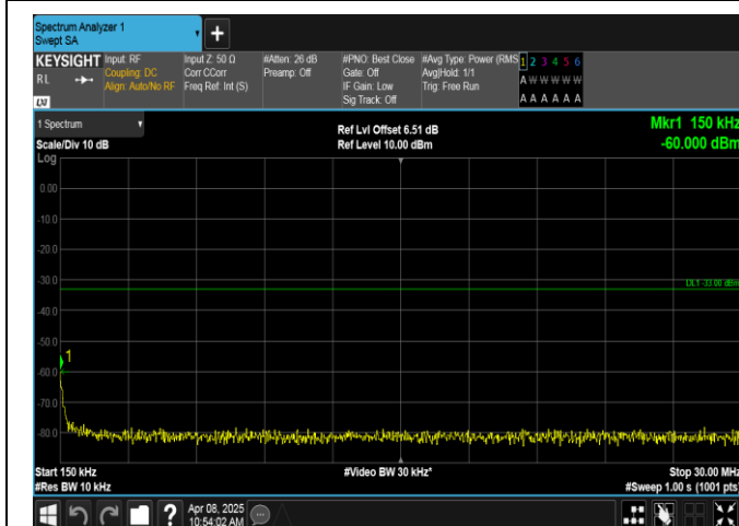
Band2-3MHz-QPSK-18900-15RB#0-0.15~30-PASS
