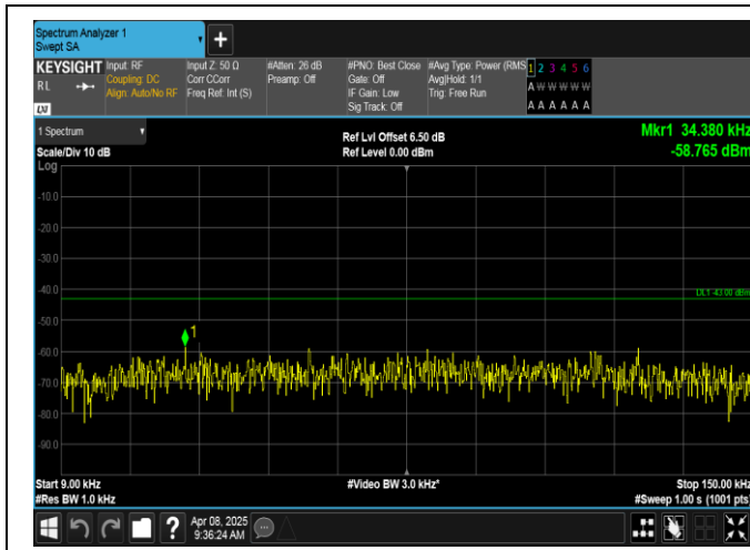
Band2-1.4MHz-16QAM-18900-6RB#0-0.009~0.15-PASS
