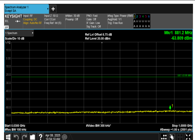
Band2-3MHz-QPSK-18900-15RB#0-30~1000-PASS
