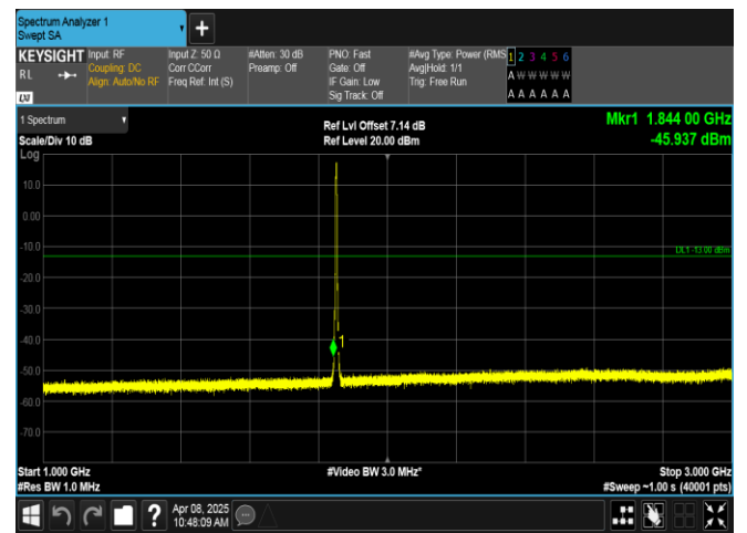
Band2-3MHz-QPSK-18615-15RB#0-1000~3000-PASS
