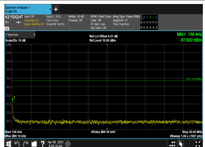
Band2-1.4MHz-16QAM-18607-1RB#5-0.15~30-PASS
