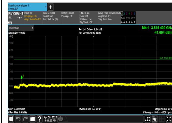
Band2-1.4MHz-16QAM-19193-1RB#5-3000~20000-PASS
