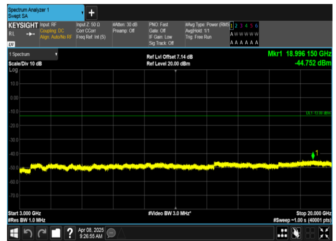
Band2-1.4MHz-16QAM-18607-1RB#0-3000~20000-PASS
