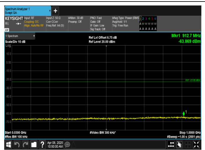
Band2-3MHz-QPSK-18900-1RB#0-30~1000-PASS
