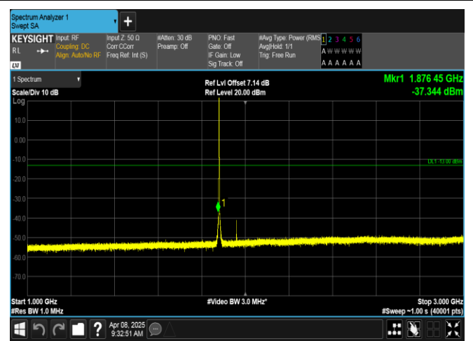
Band2-1.4MHz-16QAM-18900-1RB#0-1000~3000-PASS
