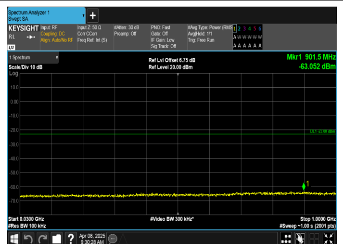
Band2-1.4MHz-16QAM-18607-6RB#0-30~1000-PASS
