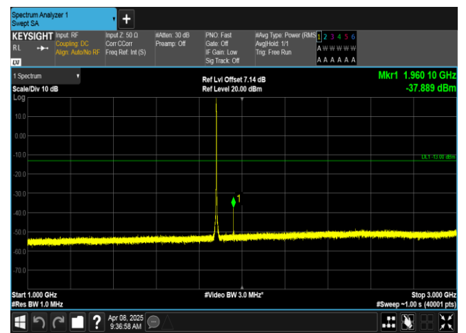
Band2-1.4MHz-16QAM-18900-6RB#0-1000~3000-PASS
