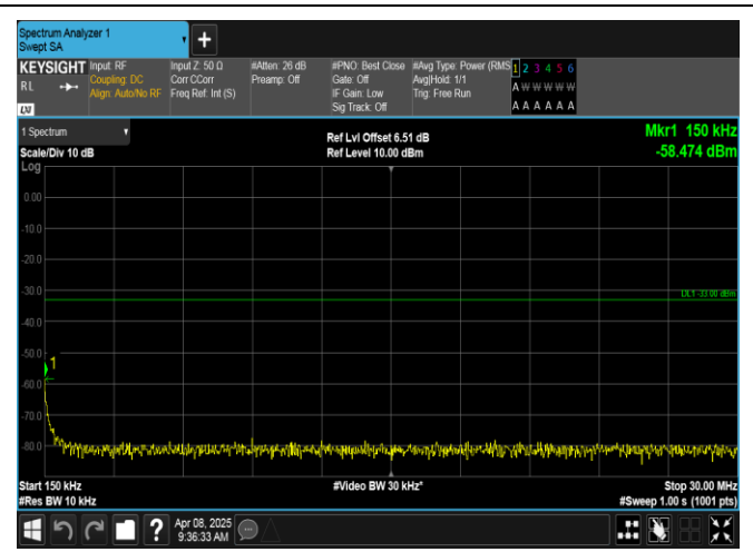
Band2-1.4MHz-16QAM-18900-6RB#0-0.15~30-PASS
