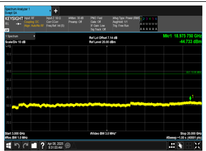
Band2-1.4MHz-16QAM-18607-6RB#0-3000~20000-PASS
