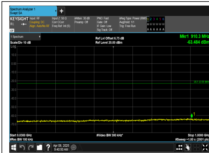
Band2-1.4MHz-16QAM-19193-1RB#5-30~1000-PASS
