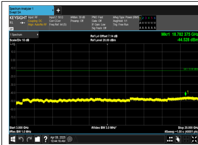
Band2-3MHz-QPSK-18615-1RB#0-3000~20000-PASS
