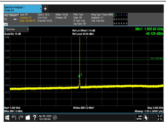
Band2-1.4MHz-16QAM-19193-1RB#5-1000~3000-PASS
