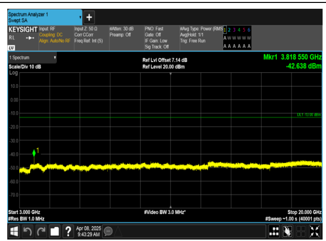
Band2-1.4MHz-16QAM-19193-6RB#0-3000~20000-PASS
