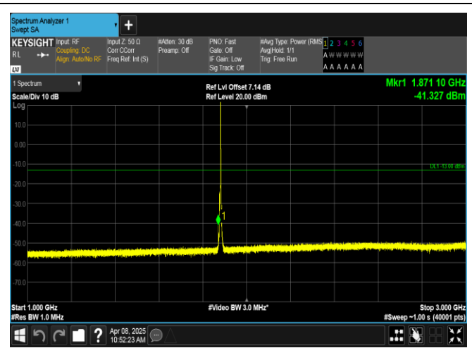
Band2-3MHz-QPSK-18900-1RB#14-1000~3000-PASS
