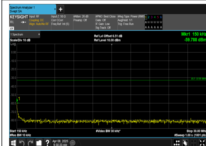
Band2-1.4MHz-16QAM-18607-6RB#0-0.15~30-PASS
