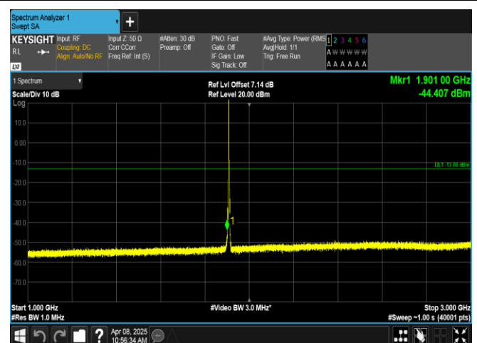
Band2-3MHz-QPSK-19185-1RB#0-1000~3000-PASS
