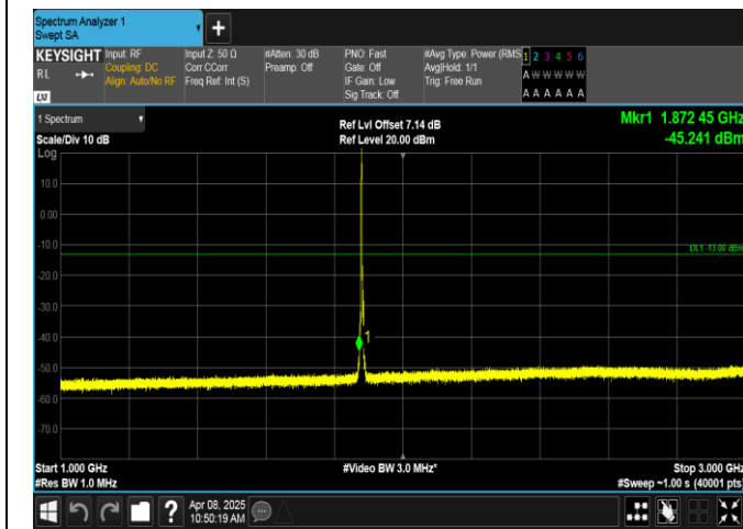
Band2-3MHz-QPSK-18900-1RB#0-1000~3000-PASS
