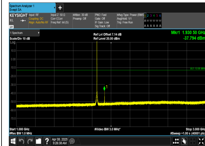
Band2-1.4MHz-16QAM-18607-1RB#0-1000~3000-PASS
