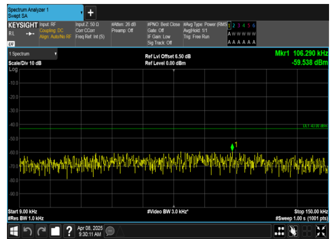
Band2-1.4MHz-16QAM-18607-6RB#0-0.009~0.15-PASS
