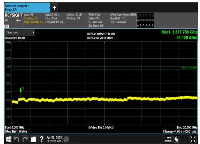
Band2-1.4MHz-16QAM-19193-1RB#0-3000~20000-PASS
