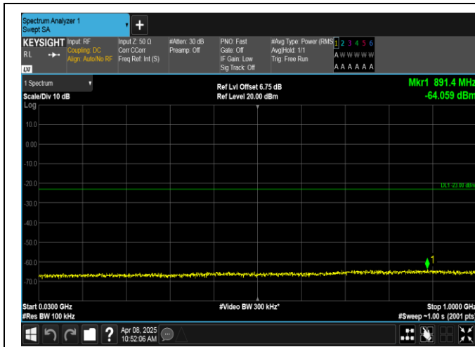
Band2-3MHz-QPSK-18900-1RB#14-30~1000-PASS
