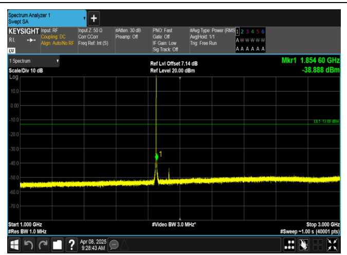
Band2-1.4MHz-16QAM-18607-1RB#5-1000~3000-PASS
