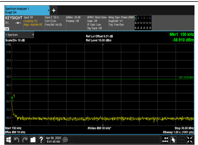
Band2-1.4MHz-QPSK-19193-6RB#0-0.15~30-PASS
