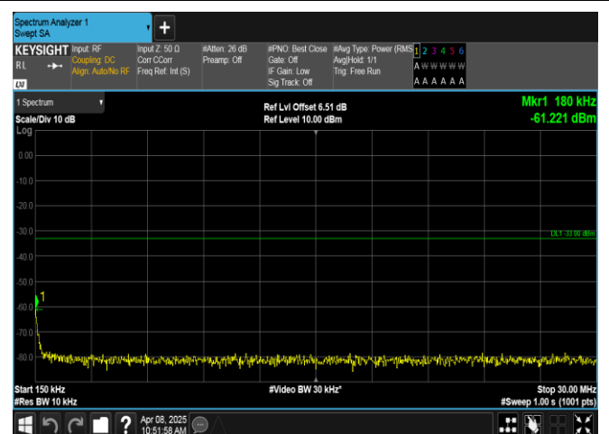
Band2-3MHz-QPSK-18900-1RB#14-0.15~30-PASS
