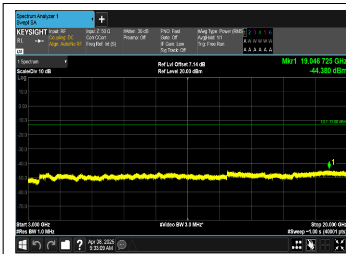
Band2-1.4MHz-16QAM-18900-1RB#0-3000~20000-PASS
