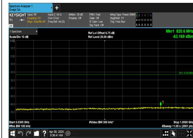
Band2-1.4MHz-16QAM-18900-6RB#0-30~1000-PASS
