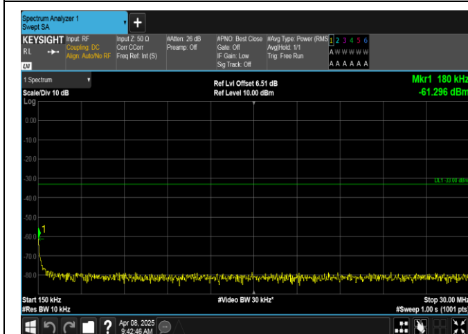
Band2-1.4MHz-16QAM-19193-6RB#0-0.15~30-PASS
