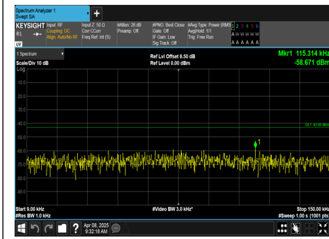
Band2-1.4MHz-16QAM-18900-1RB#0-0.009~0.15-PASS
