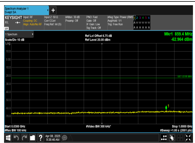
Band2-1.4MHz-16QAM-19193-1RB#0-30~1000-PASS
