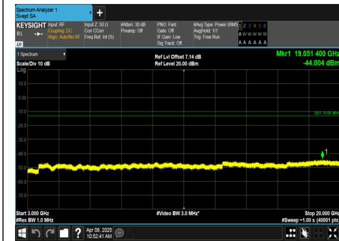
Band2-3MHz-QPSK-18900-1RB#14-3000~20000-PASS
