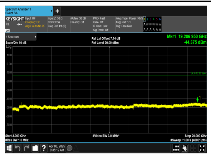
Band2-1.4MHz-16QAM-18900-1RB#5-3000~20000-PASS
