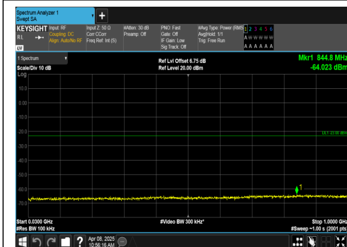
Band2-3MHz-QPSK-19185-1RB#0-30~1000-PASS
