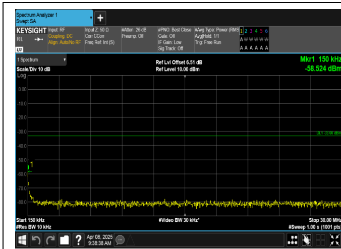
Band2-1.4MHz-16QAM-19193-1RB#0-0.15~30-PASS
