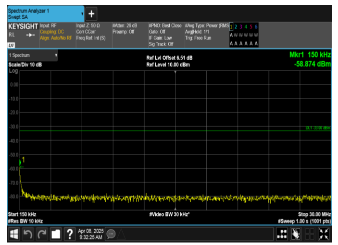
Band2-1.4MHz-16QAM-18900-1RB#0-0.15~30-PASS
