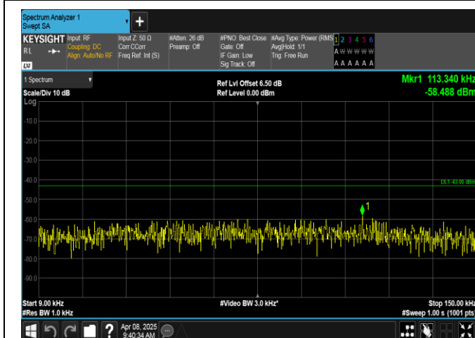
Band2-1.4MHz-16QAM-19193-1RB#5-0.009~0.15-PASS
