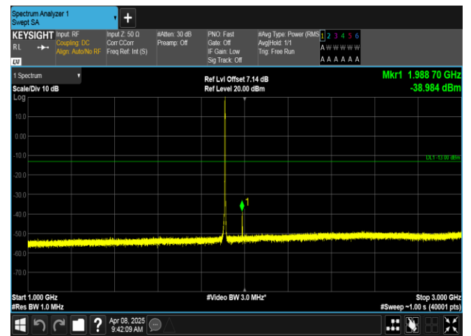
Band2-1.4MHz-QPSK-19193-6RB#0-1000~3000-PASS
