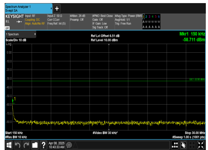
Band2-3MHz-QPSK-18615-1RB#0-0.15~30-PASS
