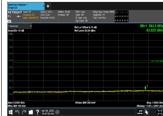
Band2-3MHz-QPSK-18615-15RB#0-30~1000-PASS
