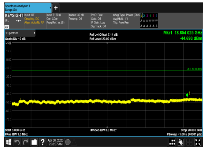
Band2-1.4MHz-QPSK-18900-1RB#0-3000~20000-PASS
