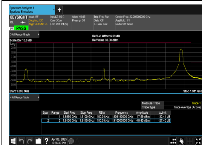
Band2-15MHz-QPSK-19125-1RB#74-PASS
