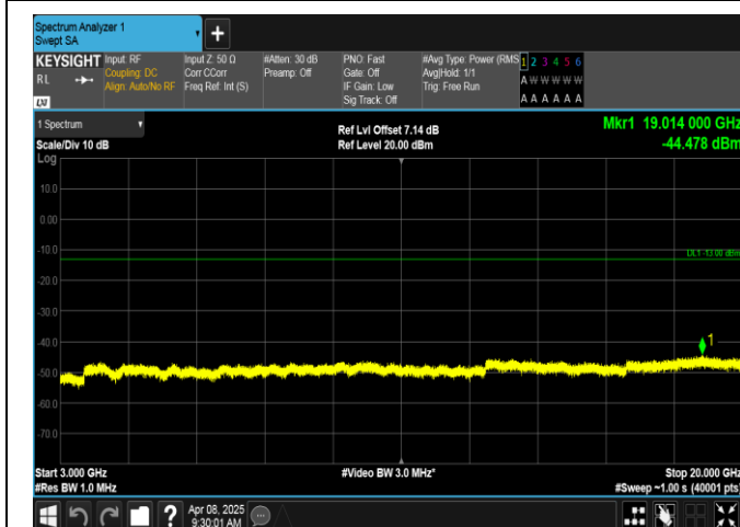
Band2-1.4MHz-QPSK-18607-6RB#0-3000~20000-PASS
