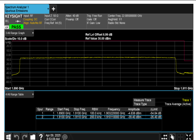
Band2-20MHz-16QAM-19100-100RB#0-PASS
