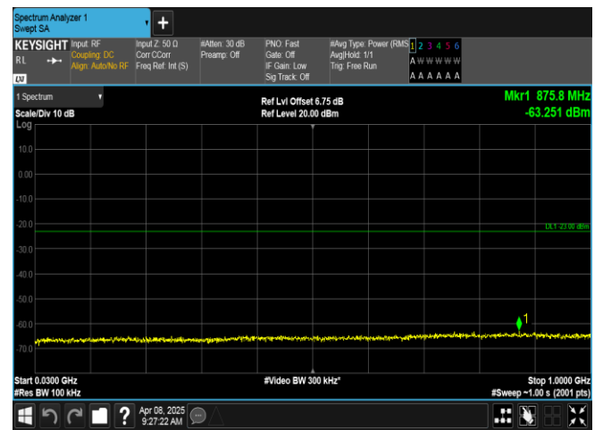
Band2-1.4MHz-QPSK-18607-1RB#5-30~1000-PASS
