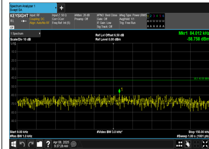
Band2-1.4MHz-QPSK-19193-1RB#0-0.009~0.15-PASS
