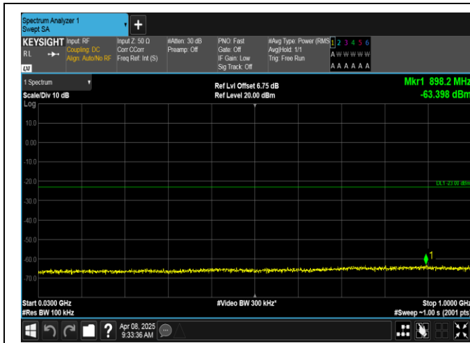
Band2-1.4MHz-QPSK-18900-1RB#5-30~1000-PASS
