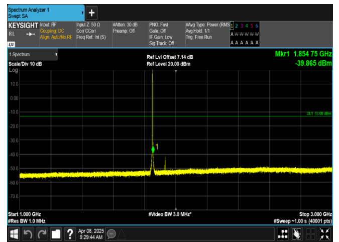
Band2-1.4MHz-QPSK-18607-6RB#0-1000~3000-PASS
