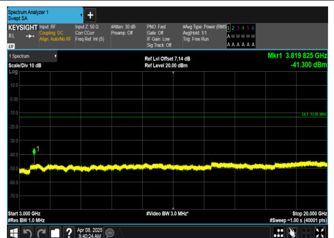
Band2-1.4MHz-QPSK-19193-1RB#5-3000~20000-PASS
