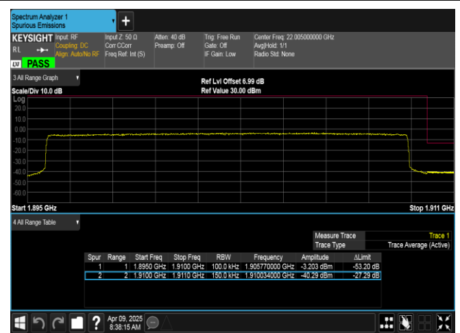
Band2-15MHz-16QAM-19125-75RB#0-PASS
