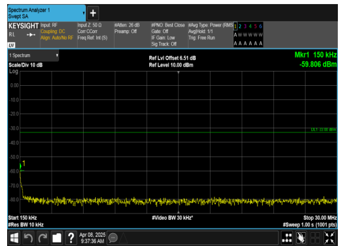
Band2-1.4MHz-QPSK-19193-1RB#0-0.15~30-PASS
