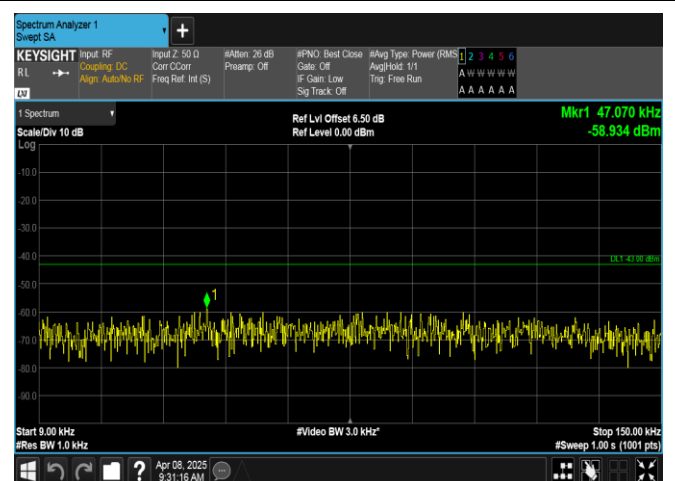
Band2-1.4MHz-QPSK-18900-1RB#0-0.009~0.15-PASS
