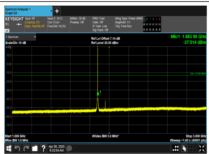
Band2-1.4MHz-QPSK-18900-1RB#5-1000~3000-PASS
