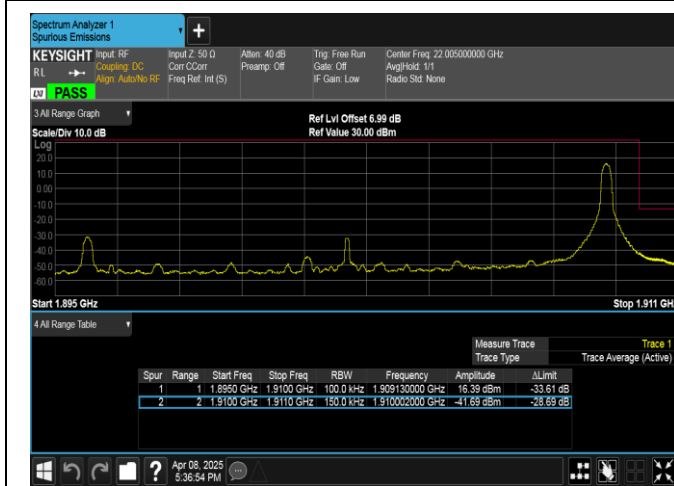
Band2-15MHz-16QAM-19125-1RB#74-PASS
