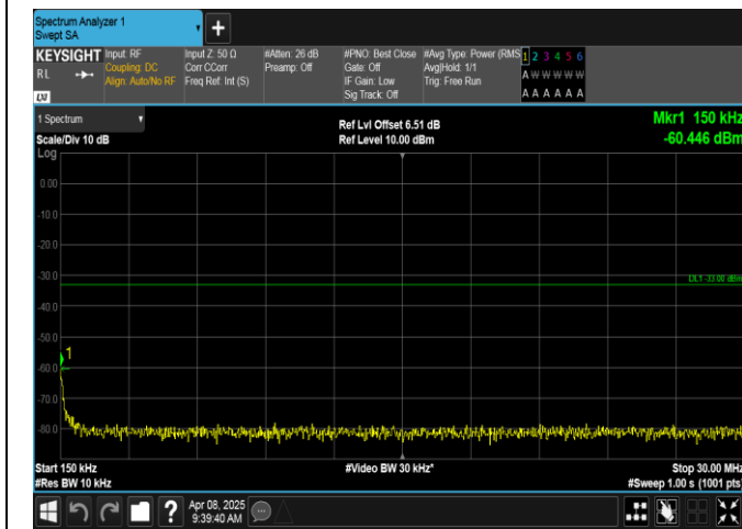
Band2-1.4MHz-QPSK-19193-1RB#5-0.15~30-PASS
