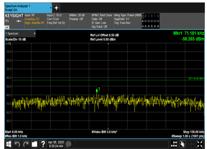
Band2-1.4MHz-QPSK-18900-6RB#0-0.009~0.15-PASS
