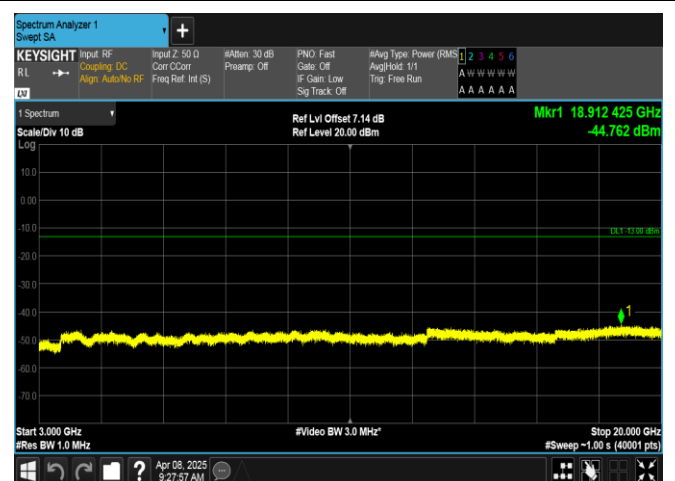
Band2-1.4MHz-QPSK-18607-1RB#5-3000~20000-PASS
