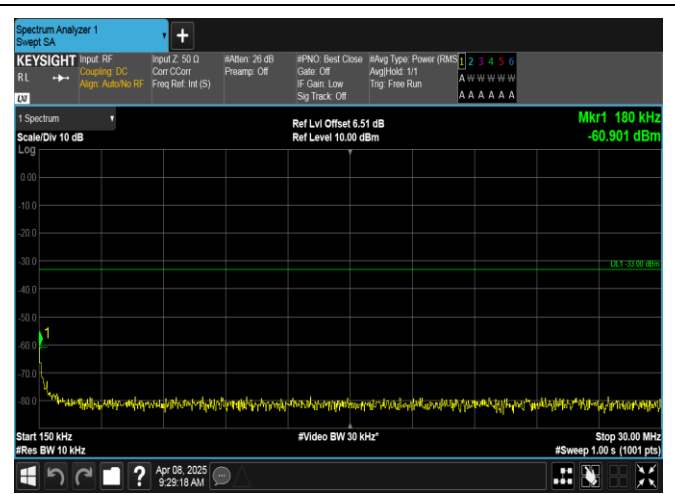
Band2-1.4MHz-QPSK-18607-6RB#0-0.15~30-PASS
