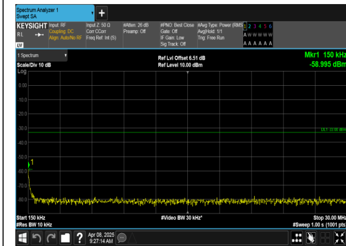
Band2-1.4MHz-QPSK-18607-1RB#5-0.15~30-PASS
