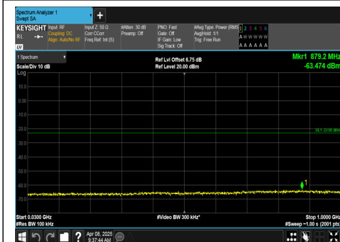
Band2-1.4MHz-QPSK-19193-1RB#0-30~1000-PASS
