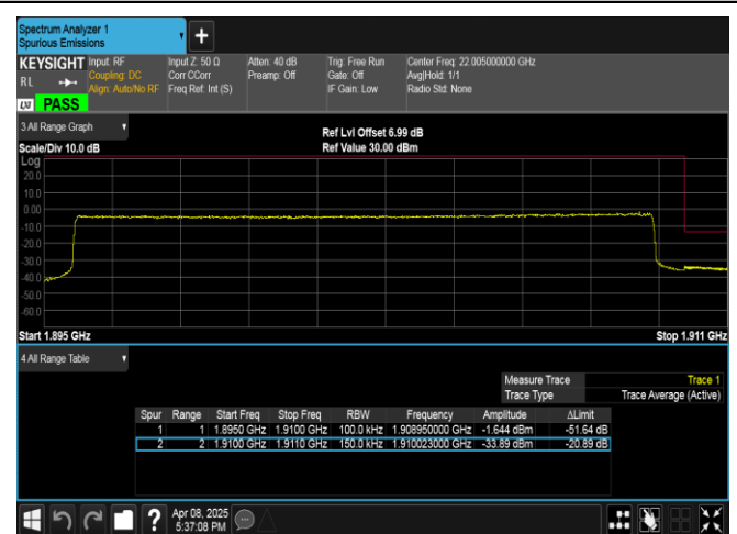
Band2-15MHz-QPSK-19125-75RB#0-PASS
