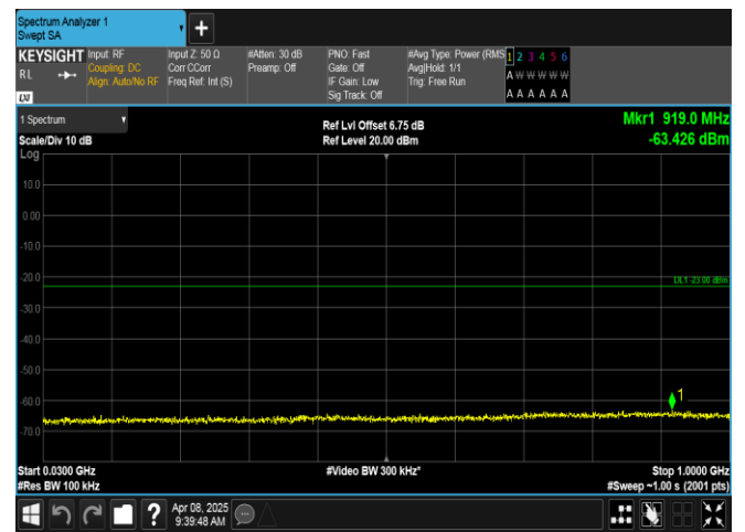
Band2-1.4MHz-QPSK-19193-1RB#5-30~1000-PASS
