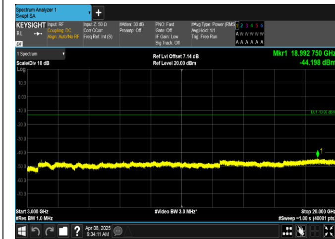
Band2-1.4MHz-QPSK-18900-1RB#5-3000~20000-PASS
