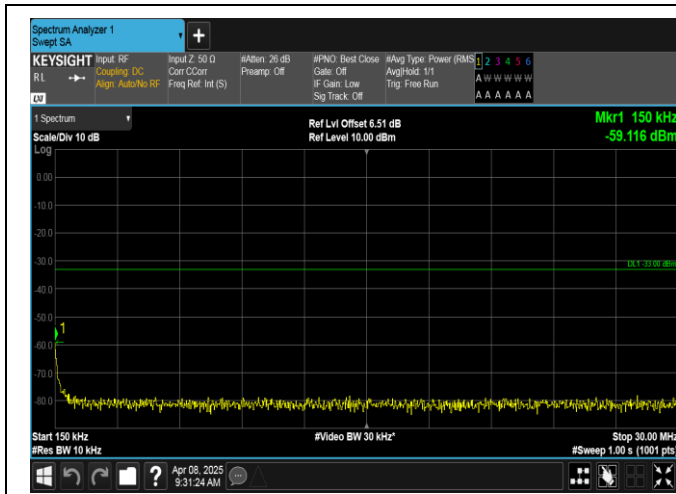
Band2-1.4MHz-QPSK-18900-1RB#0-0.15~30-PASS
