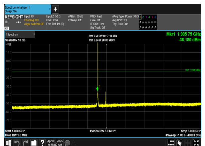
Band2-1.4MHz-QPSK-19193-1RB#0-1000~3000-PASS
