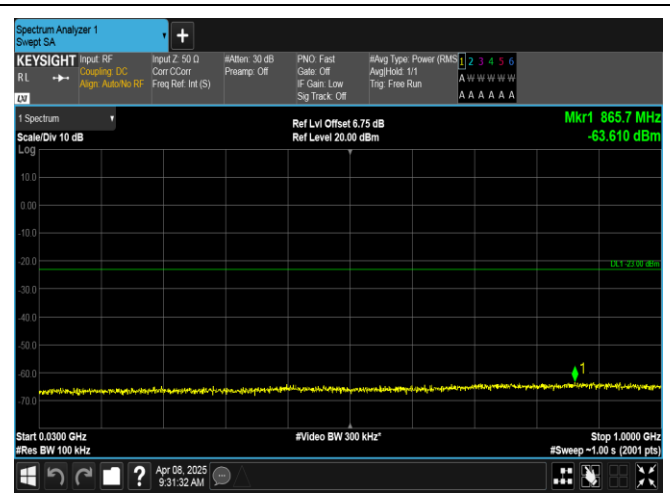
Band2-1.4MHz-QPSK-18900-1RB#0-30~1000-PASS
