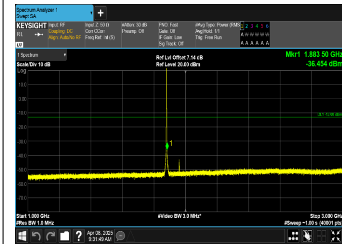
Band2-1.4MHz-QPSK-18900-1RB#0-1000~3000-PASS
