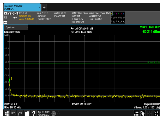
Band2-1.4MHz-QPSK-18900-1RB#5-0.15~30-PASS
