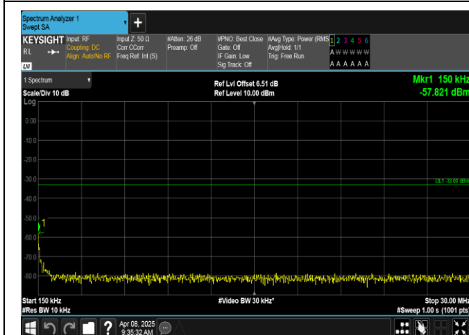
Band2-1.4MHz-QPSK-18900-6RB#0-0.15~30-PASS
