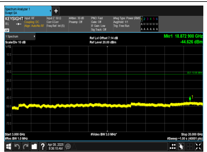
Band2-1.4MHz-QPSK-18900-6RB#0-3000~20000-PASS
