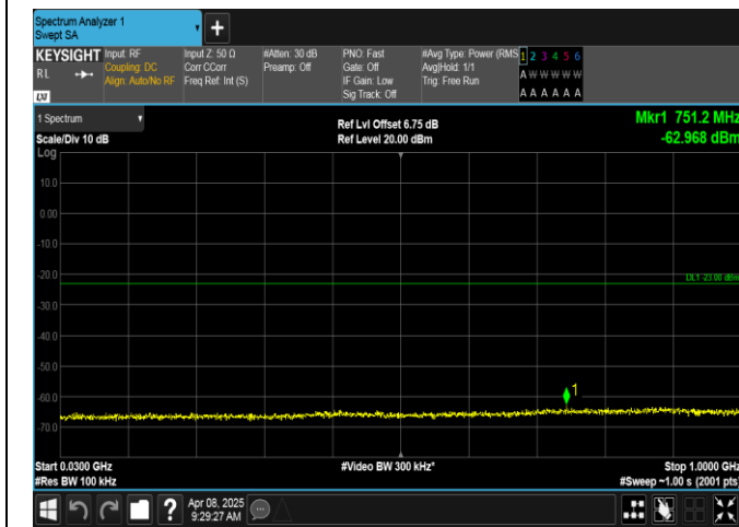
Band2-1.4MHz-QPSK-18607-6RB#0-30~1000-PASS
