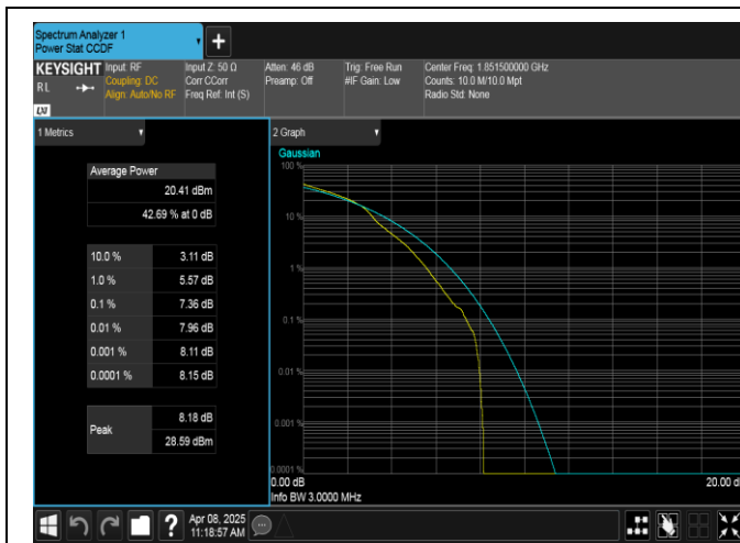
Band2-3MHz-16QAM-18615-1RB#0-PASS
