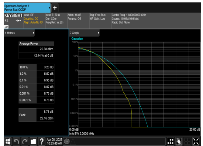
Band2-1.4MHz-16QAM-18900-6RB#0-PASS
