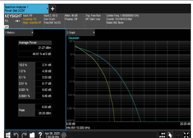
Band2-10MHz-QPSK-19150-50RB#0-PASS
