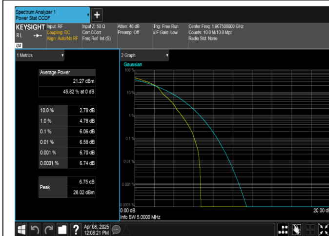
Band2-5MHz-16QAM-19175-1RB#0-PASS
