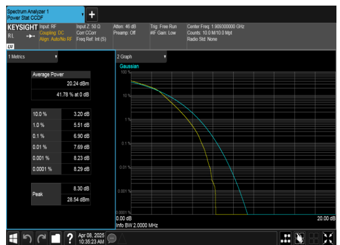
Band2-1.4MHz-16QAM-19193-6RB#0-PASS
