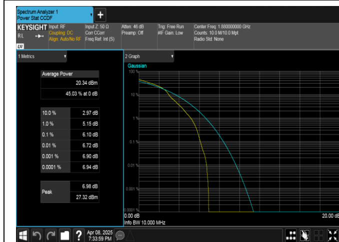
Band2-10MHz-16QAM-18900-1RB#0-PASS
