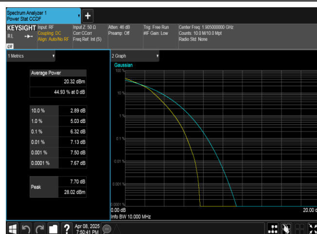
Band2-10MHz-16QAM-19150-50RB#0-PASS
