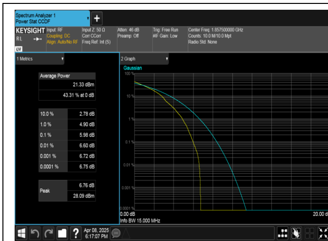
Band2-15MHz-QPSK-18675-1RB#0-PASS
