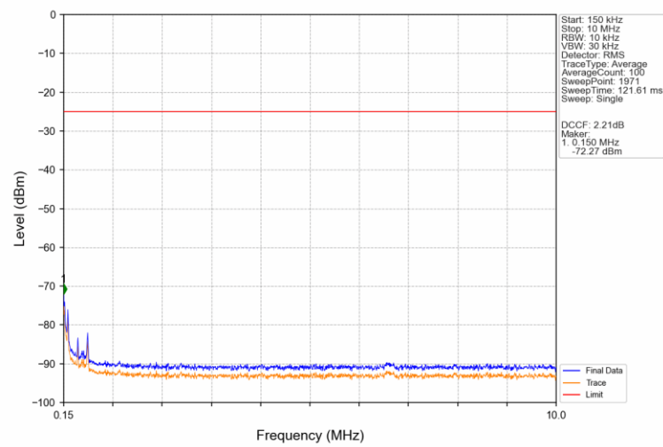
Band38_15MHz_16QAM_MCH_2595MHz_RB_1_0_NTNV
