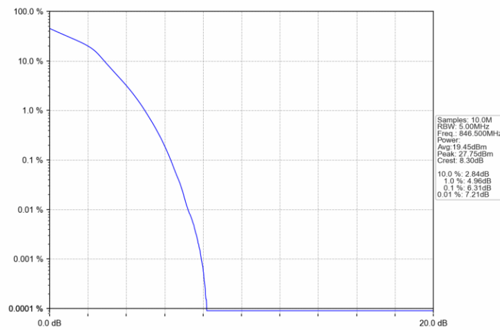
Band5_5MHz_16QAM_HCH_846.5MHz_RB_25_0_NTNV
