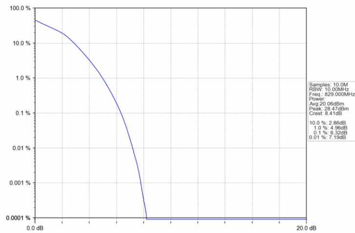
Band5_10MHz_16QAM_LCH_829MHz_RB_50_0_NTNV
