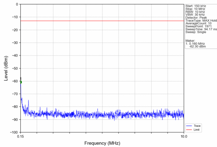
Band4_20MHz_16QAM_MCH_1732.5MHz_RB_1_0_NTNV
