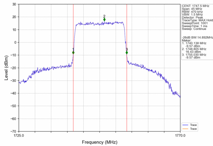
Band4_15MHz_16QAM_HCH_1747.5MHz_RB_75_0_NTNV
