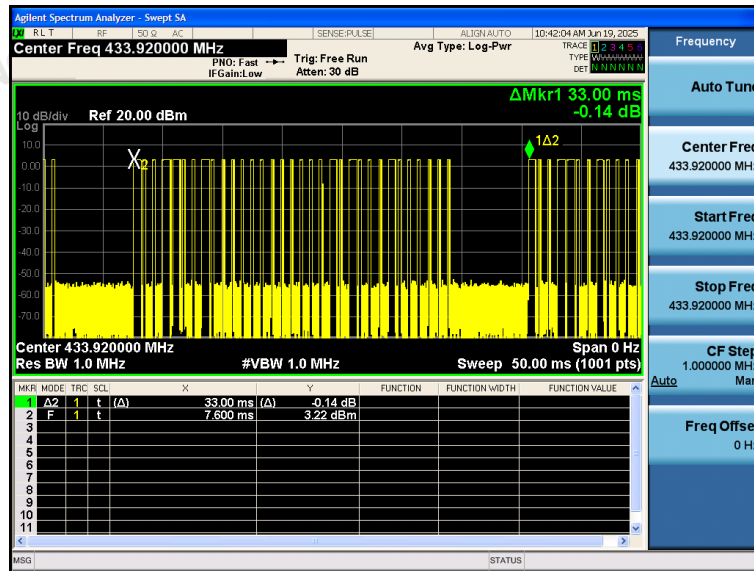
(Transmit cycle 33.0ms)
