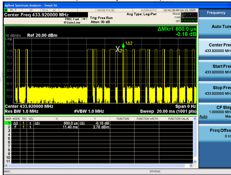
(Time per burst: 0.60ms*7pcs)
