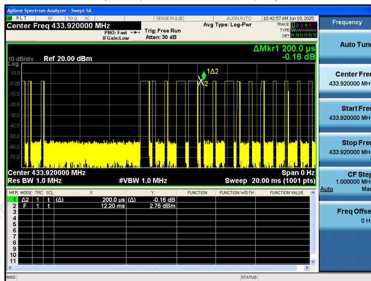
(Time per burst: 0.20 ms*26pcs)
