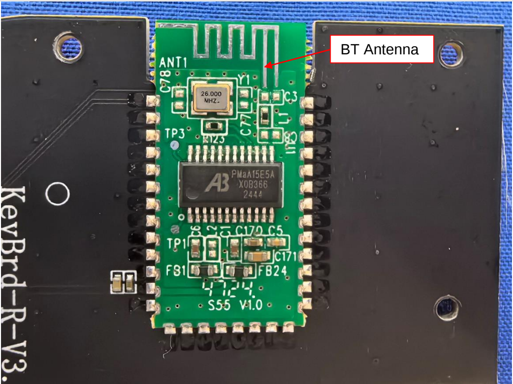
Internal View of EUT-53
