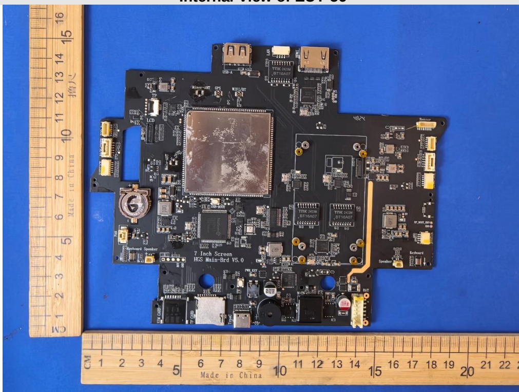
Internal View of EUT-56
