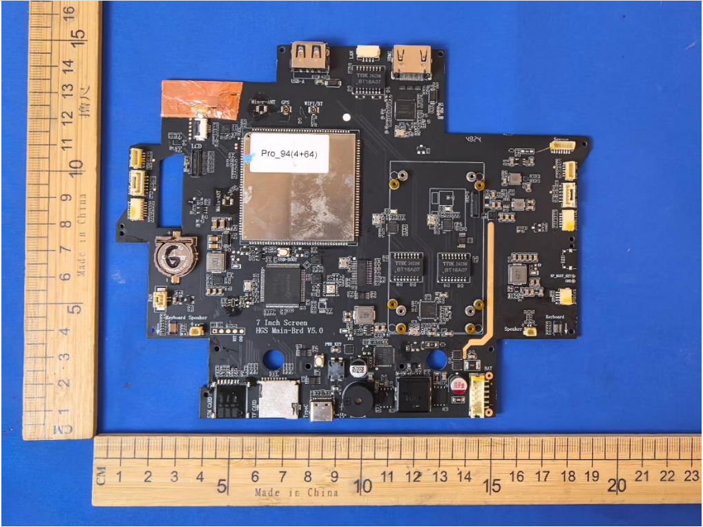
Internal View of EUT-54
