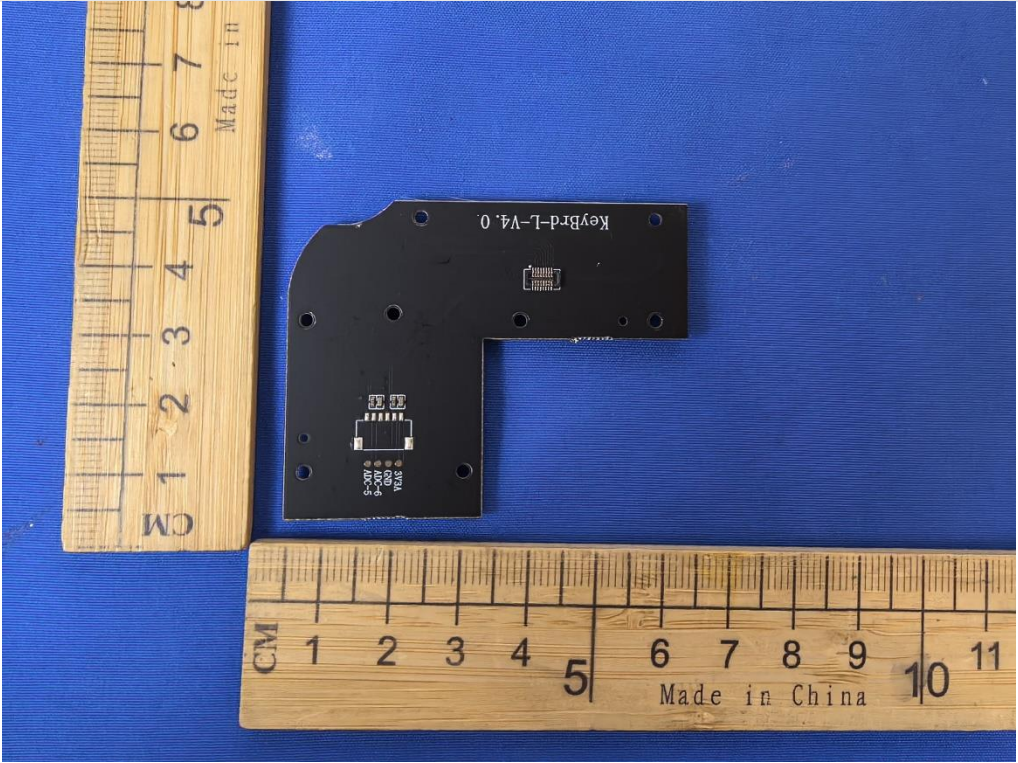
Internal View of EUT-50
