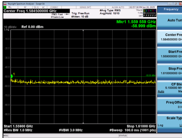
Band13-5MHz-QPSK-23255-1RB#0-Range5:1559~1610MHz
