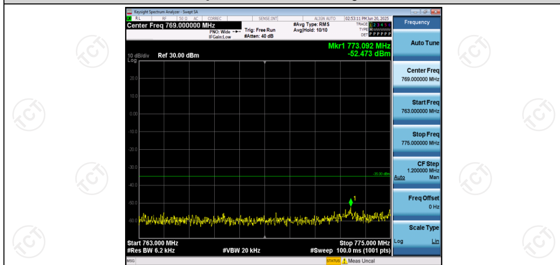
Band13-5MHz-QPSK-23205-1RB#0-Range3:763~775MHz
