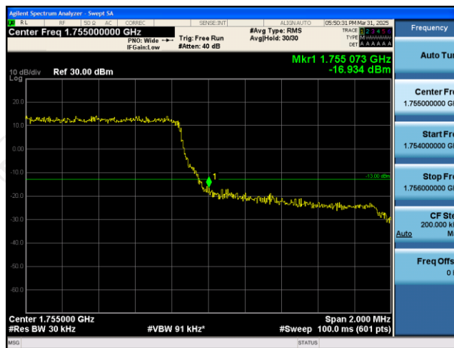
Band4-1.4MHz-QPSK-20393-6RB#0
