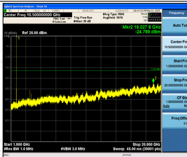
Band4-3MHz-16QAM-19965-1RB#0-Range2:1000~20000MHz
