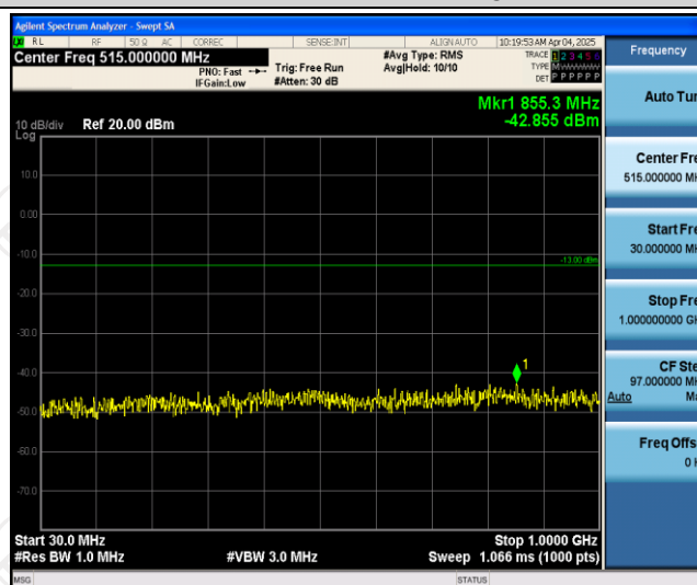
Band4-5MHz-16QAM-20375-1RB#0-Range1:30~1000MHz
