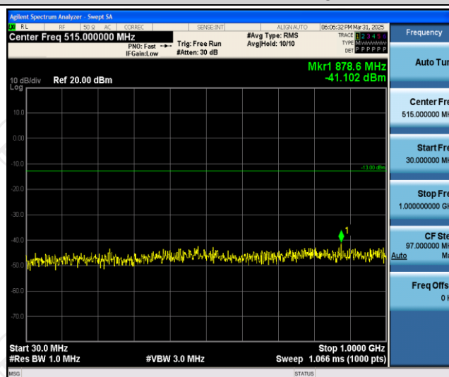
Band4-1.4MHz-16QAM-20393-1RB#0-Range1:30~1000MHz
