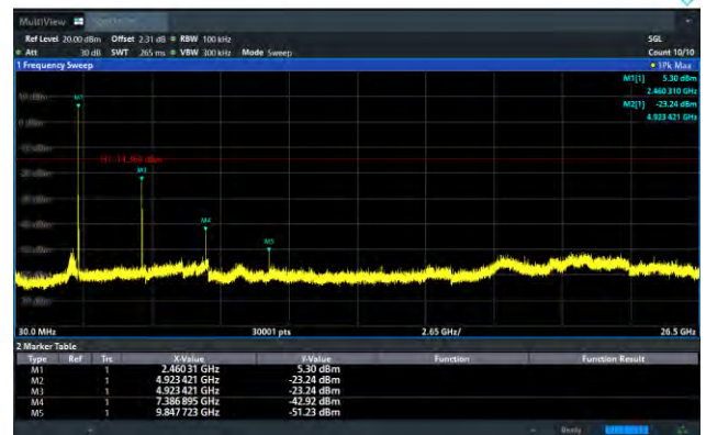
802.11b on Channel 11
