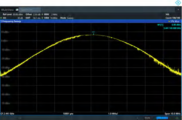
\pi/4 -DQPSK on Channel 39
