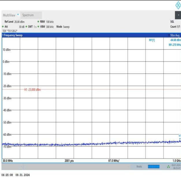
Band66_20MHz_QPSK_132572_1RB#99_30~1000_30~1000
