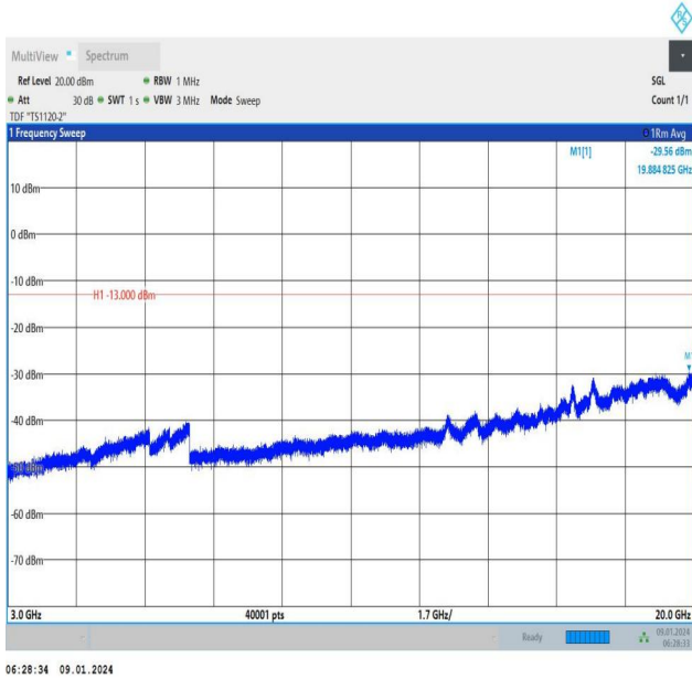
Band66_20MHz_QPSK_132572_100RB#0_3000~20000_3000~20000 0~20000
