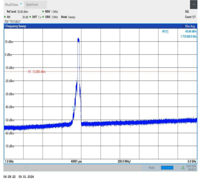
Band66_20MHz_QPSK_132572_100RB#0_1000~3000_1000~3000 ~3000
