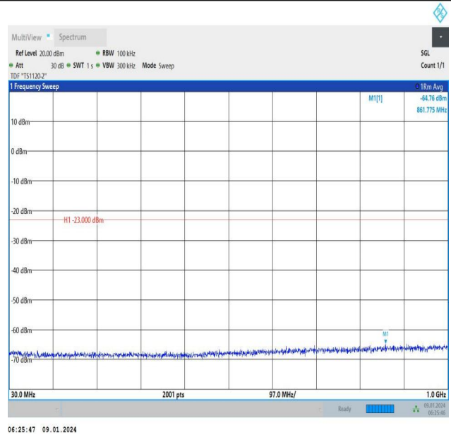
Band66_20MHz_16QAM_132572_1RB#99_30~1000_30~100 0
