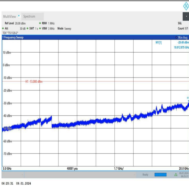
Band66_20MHz_QPSK_132572_1RB#99_3000~20000_3000~20000
