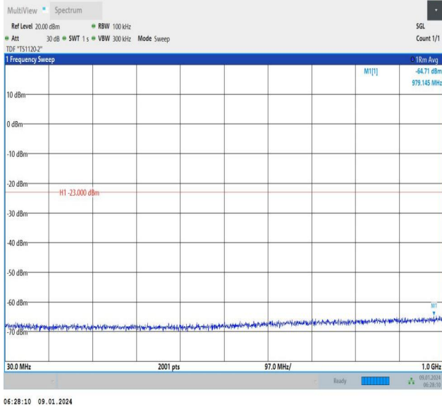
Band66_20MHz_QPSK_132572_100RB#0_30~1000_30~1000 0
