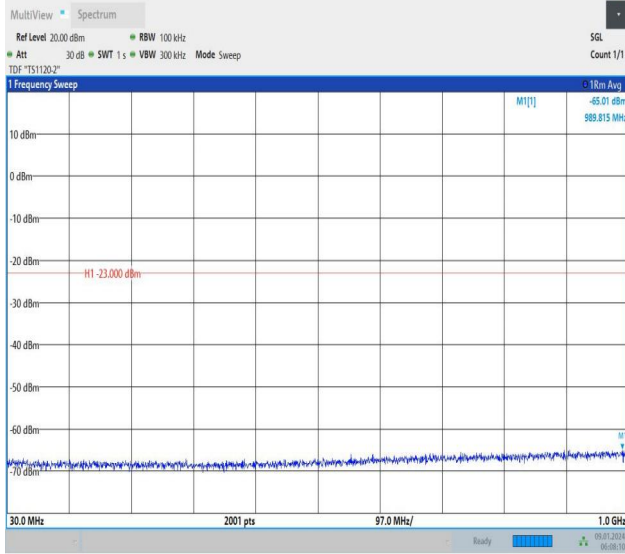
Band66_15MHz_16QAM_132047_1RB#0_30~1000_30~1000
