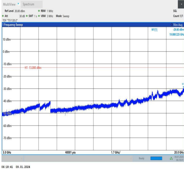
Band66_20MHz_QPSK_132072_1RB#0_3000~20000_3000~20000
