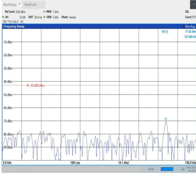
Band66_20MHz_QPSK_132072_1RB#0_0.009~0.15_0.009~0.15
