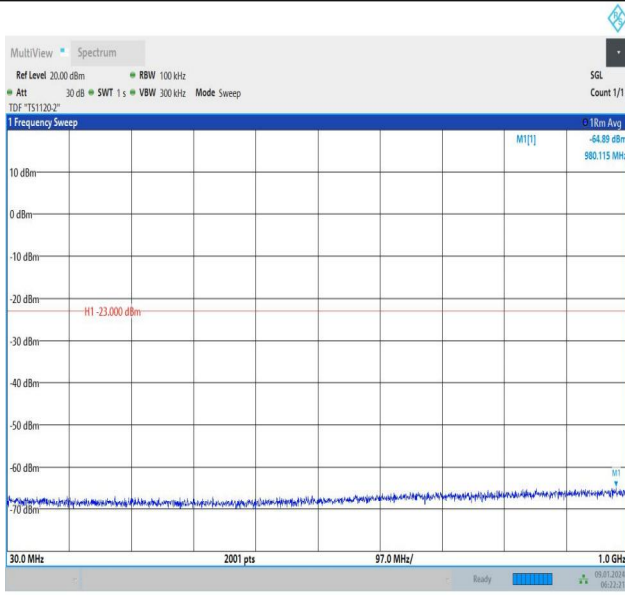
Band66_20MHz_QPSK_132322_1RB#99_30~1000_30~1000
