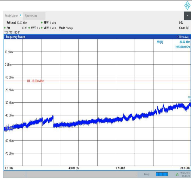
Band66_20MHz_16QAM_132072_1RB#0_3000~20000_3000~20000
