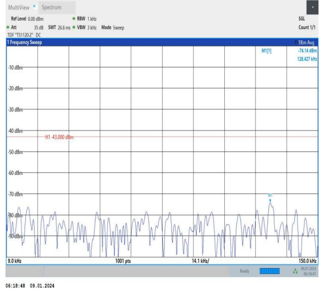
Band66_20MHz_16QAM_132072_1RB#0_0.009~0.15_0.009~0.15
