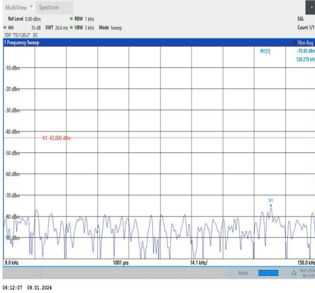
Band66_15MHz_16QAM_132322_1RB#74_0.009~0.15_0.009 ~0.15
