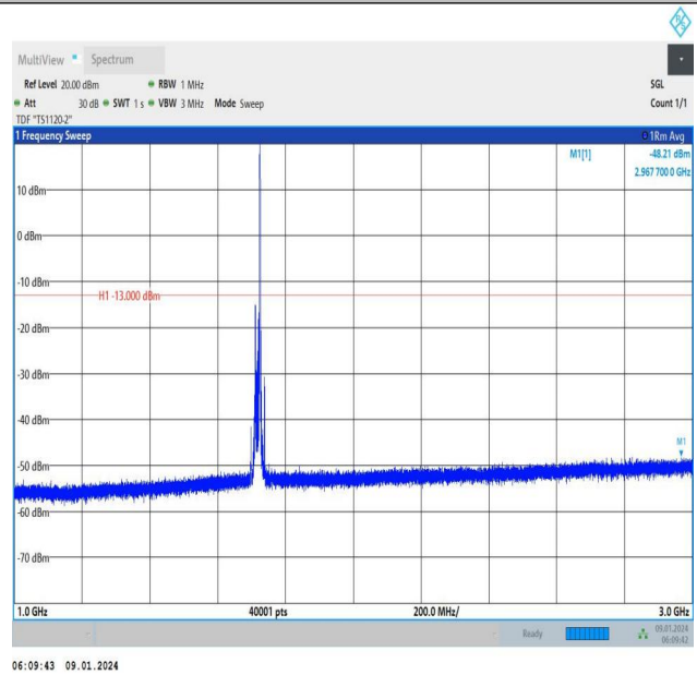
Band66_15MHz_16QAM_132047_1RB#74_1000~3000_1000 ~3000
