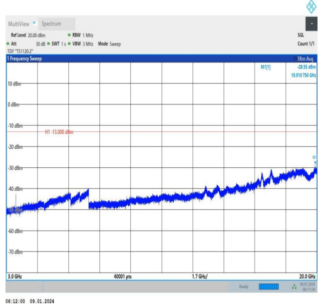
Band66_15MHz_QPSK_132322_1RB#74_3000~20000_3000~20000
