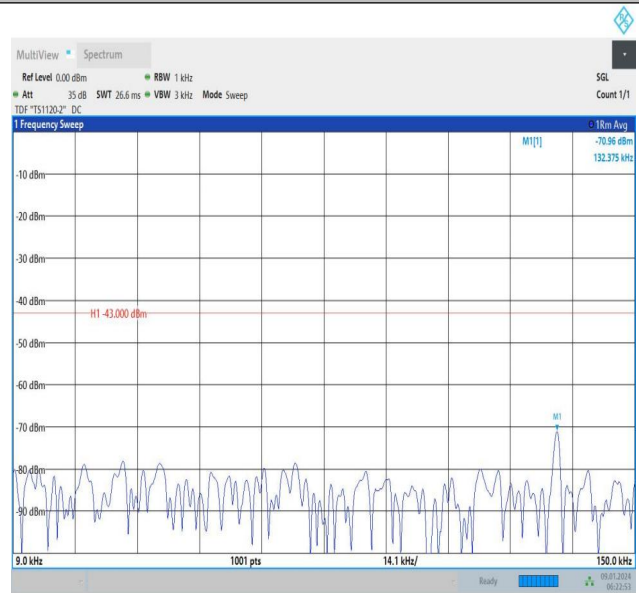
Band66_20MHz_QPSK_132322_1RB#99_1000~3000_1000~3000
