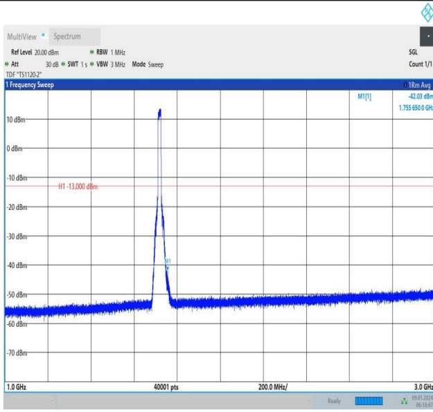
Band66_15MHz_QPSK_132047_75RB#0_1000~3000_1000~3000
