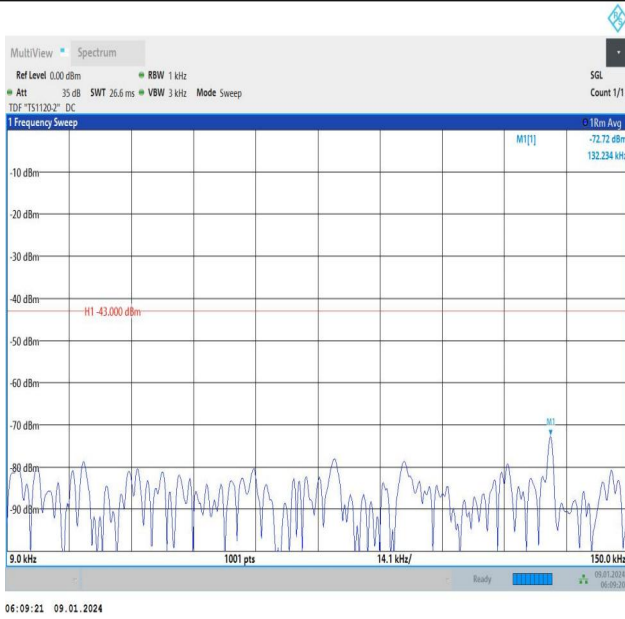
Band66_15MHz_16QAM_132047_1RB#74_0.009~0.15_0.009 ~0.15
