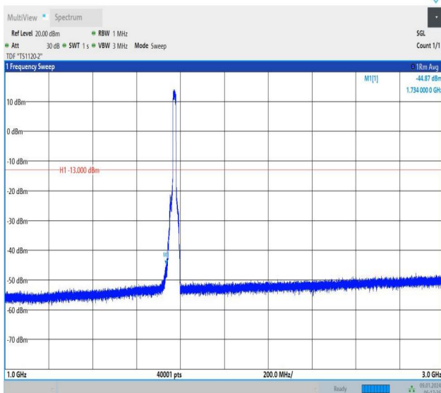
Band66_15MHz_QPSK_132597_75RB#0_1000~3000_1000~3000
