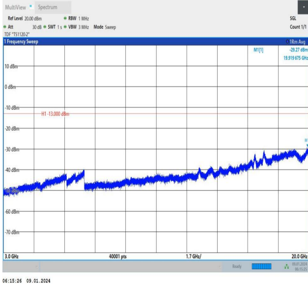
Band66_15MHz_16QAM_132597_1RB#74_3000~20000_300 0~20000
