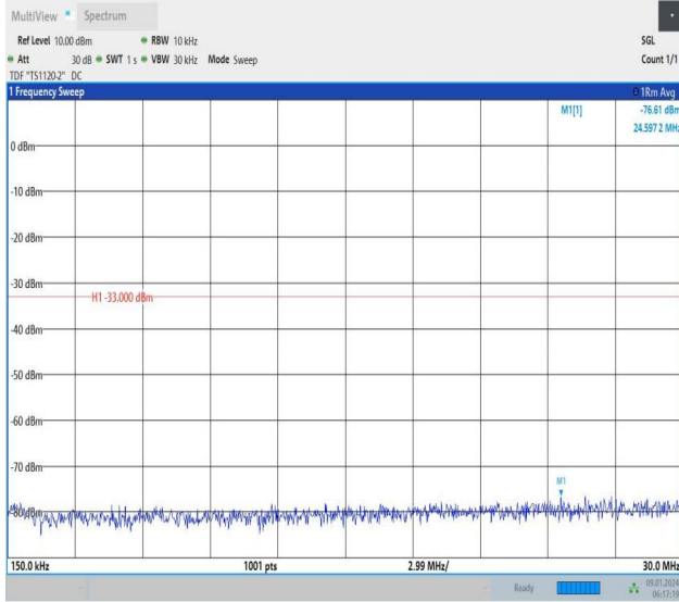
Band66_15MHz_QPSK_132597_75RB#0_0.15~30_0.15~30
