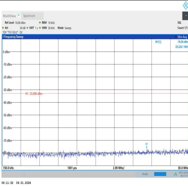
Band66_15MHz_QPSK_132322_1RB#74_0.15~30_0.15~30
