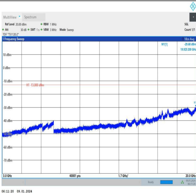
Band66_15MHz_16QAM_132322_1RB#0_3000~20000_3000~20000
