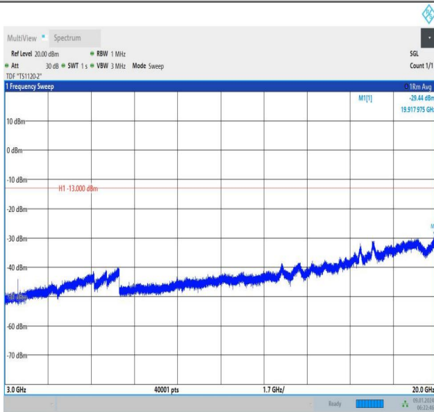
Band66_20MHz_QPSK_132322_1RB#99_3000~20000_3000~20000
