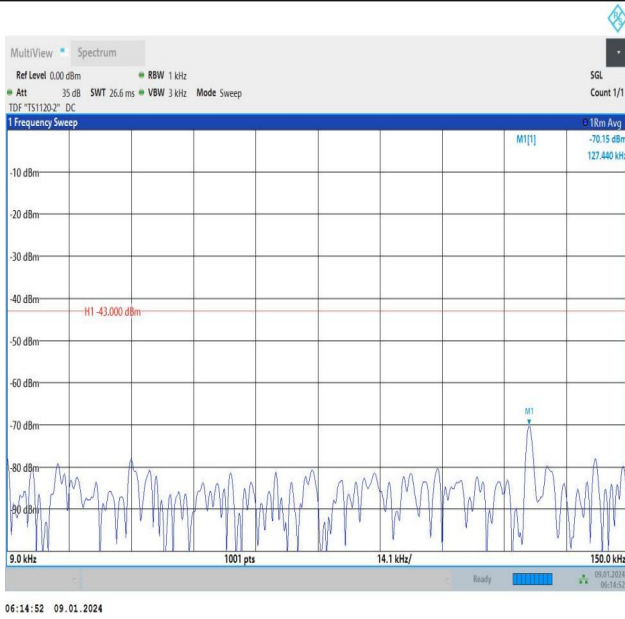
Band66_15MHz_16QAM_132597_1RB#74_0.009~0.15_0.009 ~0.15
