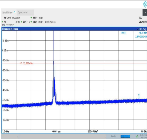
Band66_20MHz_16QAM_132072_1RB#0_1000~3000_1000~3000
