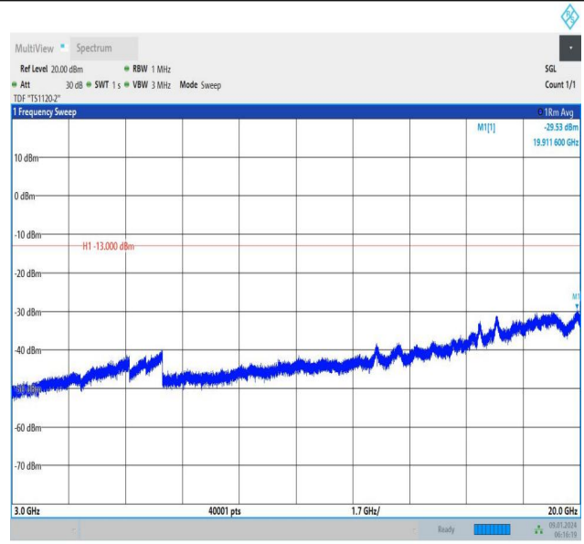
Band66_15MHz_QPSK_132047_75RB#0_3000~20000_3000~20000
