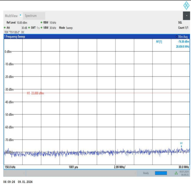
Band66_15MHz_16QAM_132047_1RB#74_0.15~30_0.15~30
