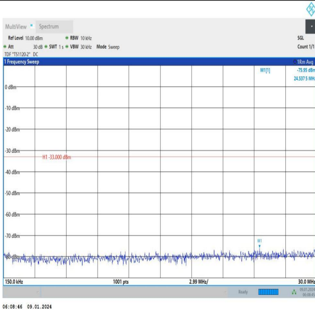
Band66_15MHz_QPSK_132047_1RB#74_0.15~30_0.15~30
