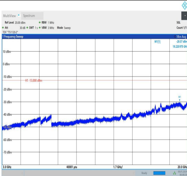
Band66_15MHz_16QAM_132047_1RB#0_3000~20000_3000~20000
