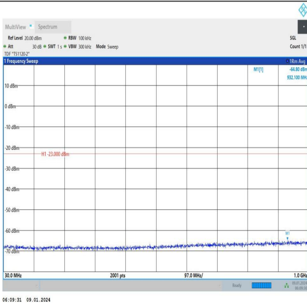
Band66_15MHz_16QAM_132047_1RB#74_30~1000_30~100 0
