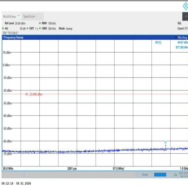
Band66_15MHz_16QAM_132322_1RB#74_30~1000_30~100 0
