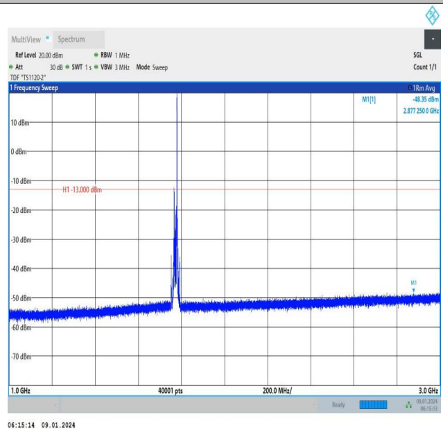
Band66_15MHz_16QAM_132597_1RB#74_1000~3000_1000 ~3000
