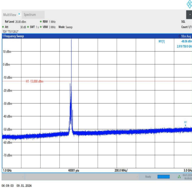
Band66_15MHz_QPSK_132047_1RB#74_1000~3000_1000~3000
