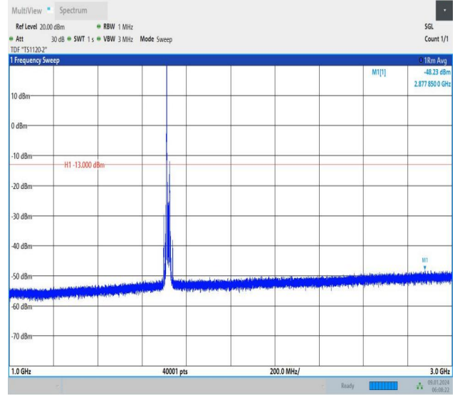
Band66_15MHz_16QAM_132047_1RB#0_1000~3000_1000~3000
