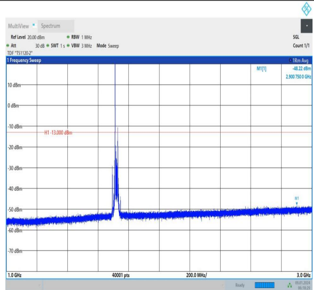
Band66_20MHz_QPSK_132072_1RB#0_1000~3000_1000~3000
