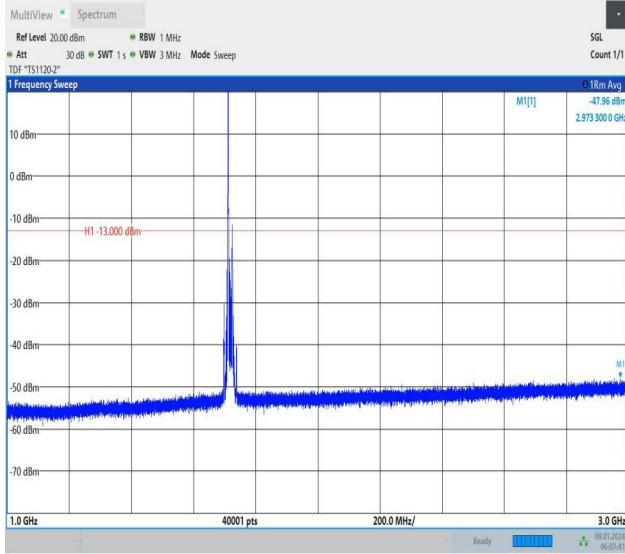
Band66_15MHz_QPSK_132047_1RB#0_1000~3000_1000~3000
