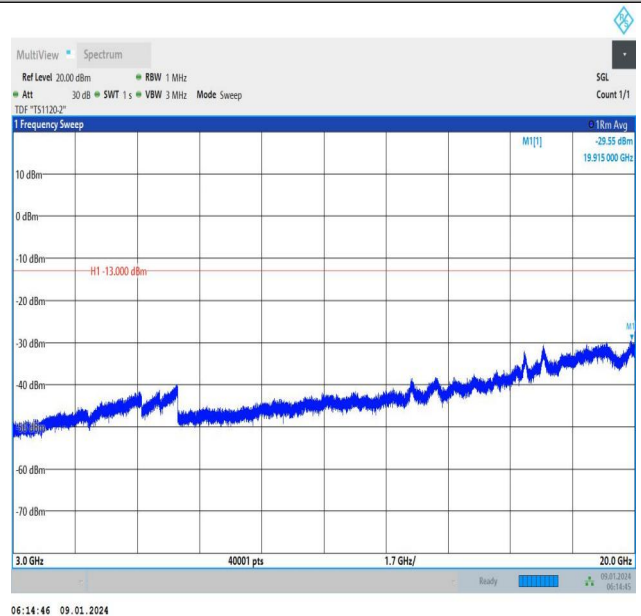
Band66_15MHz_QPSK_132597_1RB#74_3000~20000_3000~20000
