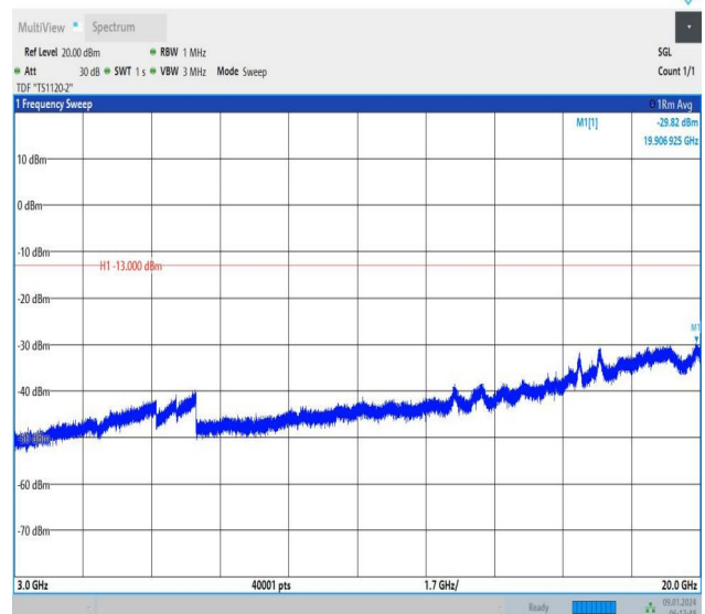
Band66_15MHz_QPSK_132597_75RB#0_3000~20000_3000~20000
