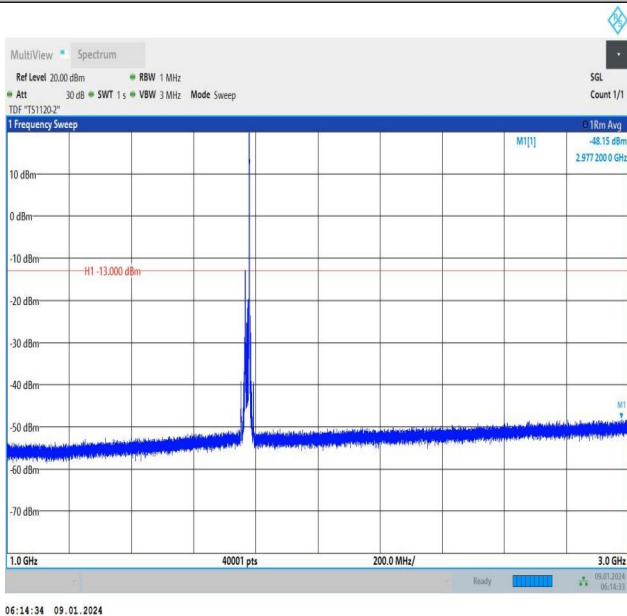
Band66_15MHz_QPSK_132597_1RB#74_1000~3000_1000~3000
