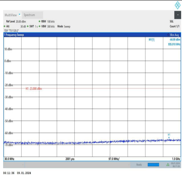
Band66_15MHz_QPSK_132322_1RB#74_30~1000_30~1000
