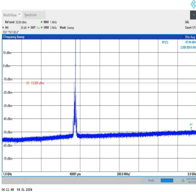
Band66_15MHz_QPSK_132322_1RB#74_1000~3000_1000~3000
