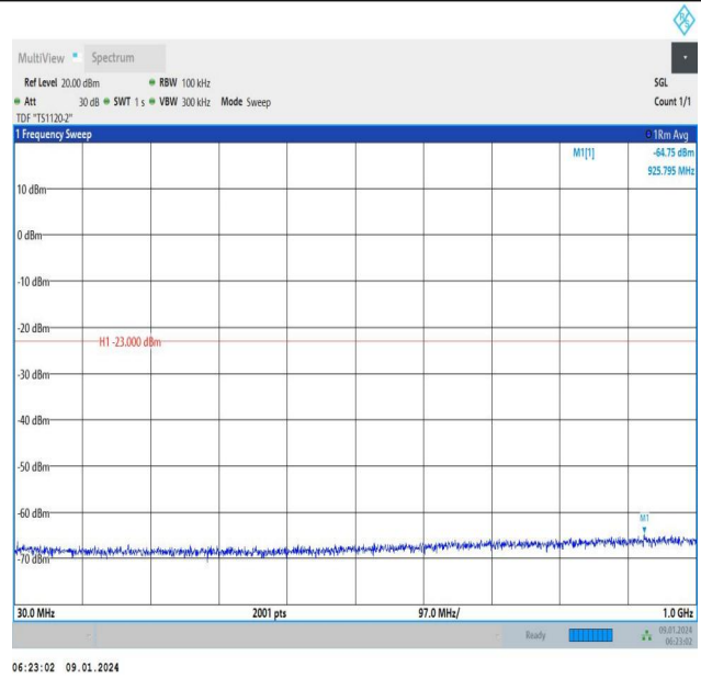
Band66_20MHz_16QAM_132322_1RB#99_30~1000_30~100
