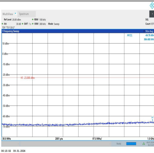
Band66_15MHz_16QAM_132597_1RB#74_30~1000_30~100 0
