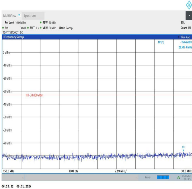
Band66_20MHz_16QAM_132072_1RB#0_0.15~30_0.15~30
