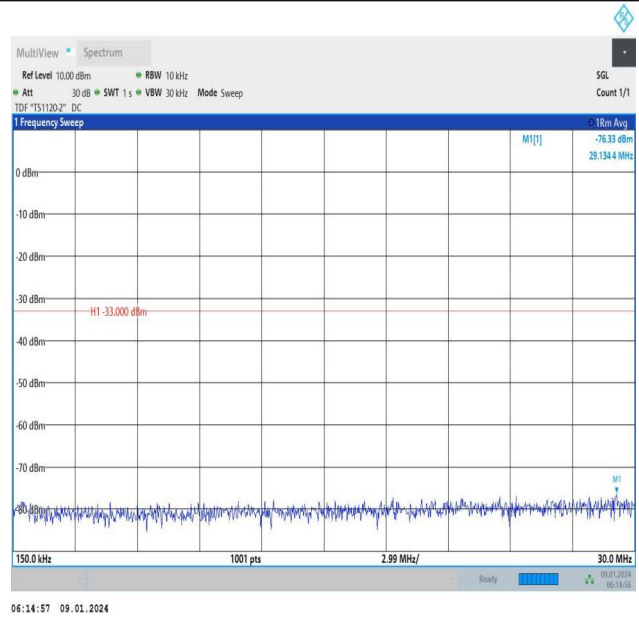
Band66_15MHz_16QAM_132597_1RB#74_0.15~30_0.15~30
