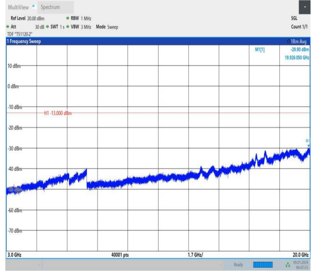
Band66_15MHz_QPSK_132047_1RB#0_3000~20000_3000~20000
