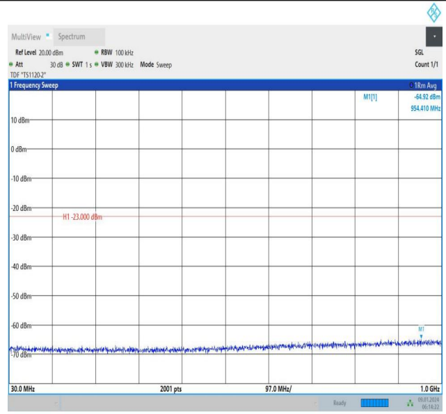
Band66_15MHz_QPSK_132597_1RB#74_30~1000_30~1000
