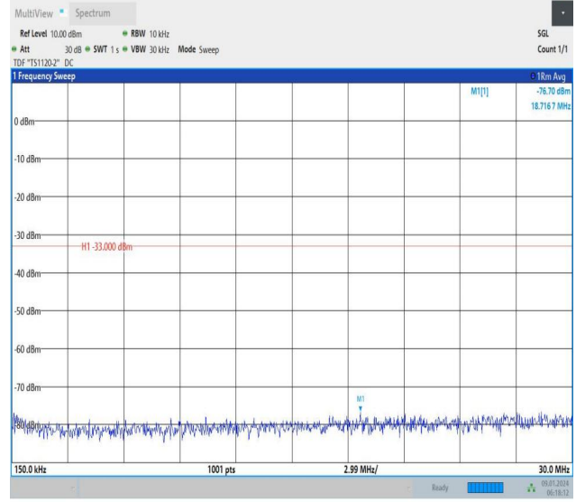
Band66_20MHz_QPSK_132072_1RB#0_0.15~30_0.15~30
