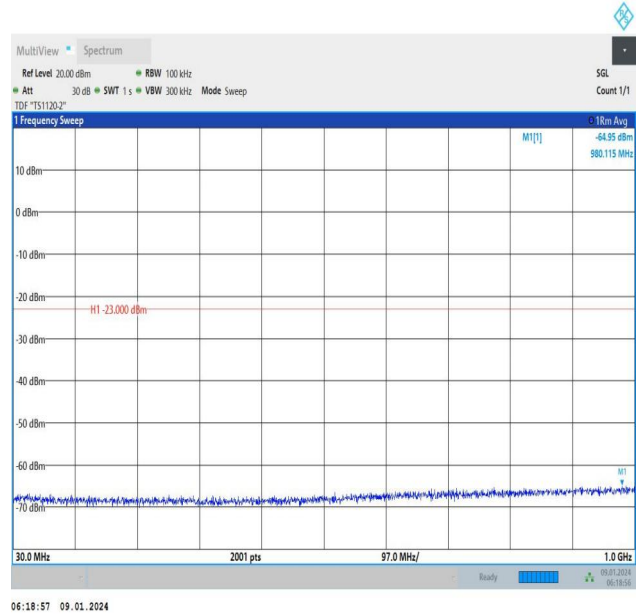
Band66_20MHz_16QAM_132072_1RB#0_30~1000_30~1000
