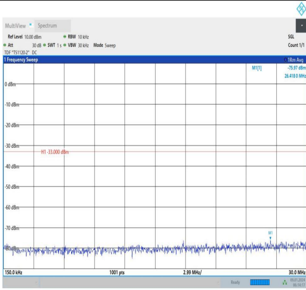
Band66_15MHz_QPSK_132597_1RB#74_0.15~30_0.15~30
