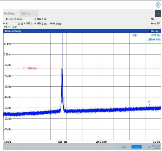
Band66_20MHz_QPSK_132322_1RB#99_1000~3000_1000~3000
