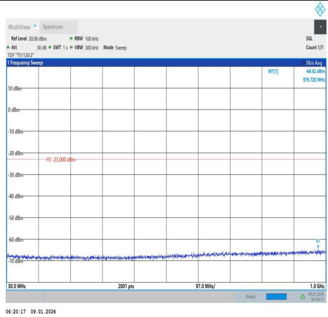
Band66_20MHz_16QAM_132072_1RB#99_30~1000_30~100
