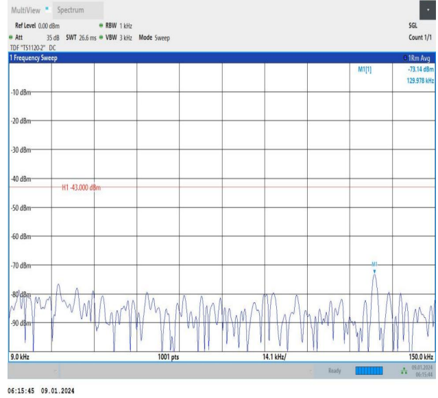
Band66_15MHz_QPSK_132047_75RB#0_0.009~0.15_0.009~ 0.15
