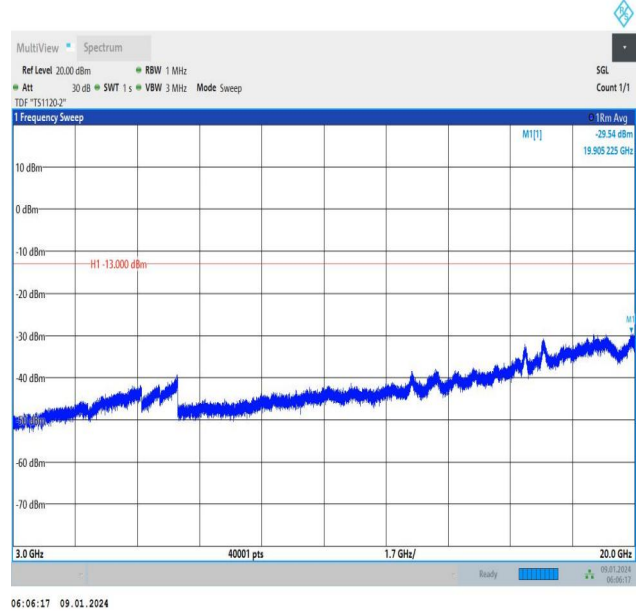
Band66_10MHz_QPSK_132322_50RB#0_3000~20000_3000~20000
