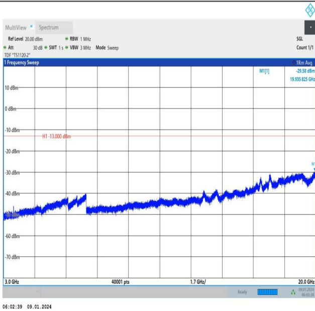
Band66_10MHz_QPSK_132622_1RB#0_3000~20000_3000~20000
