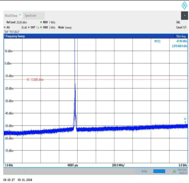
Band66_10MHz_QPSK_132622_1RB#0_1000~3000_1000~3000
