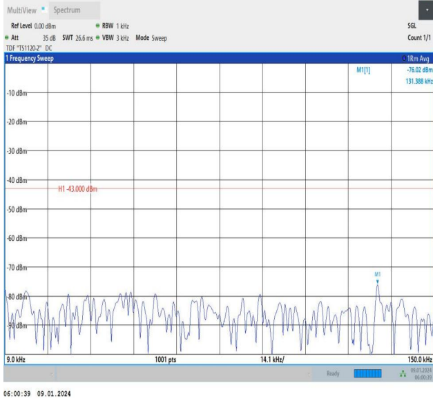
Band66_10MHz_QPSK_132322_1RB#49_0.009~0.15_0.009~0.15
