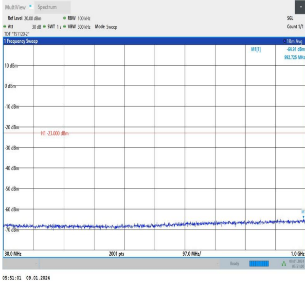
Band66_5MHz_QPSK_132322_25RB#0_30~1000_30~1000
