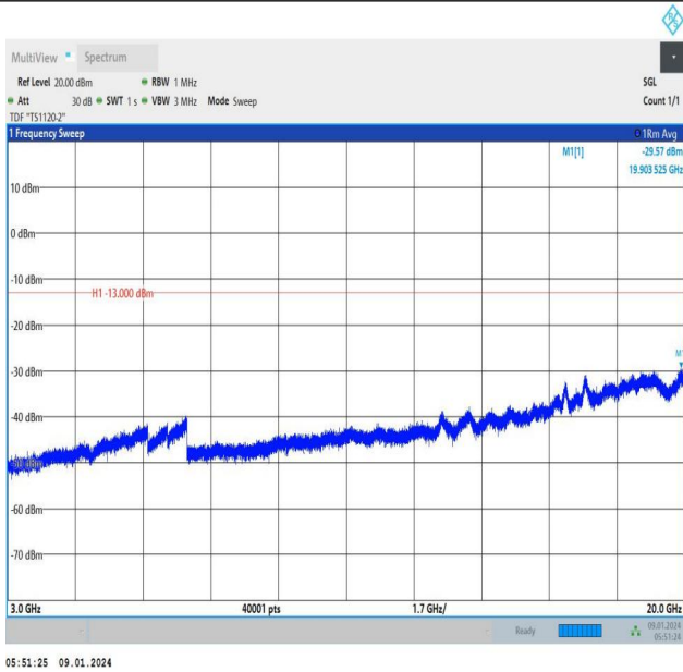
Band66_5MHz_QPSK_132322_25RB#0_3000~20000_3000~20000
