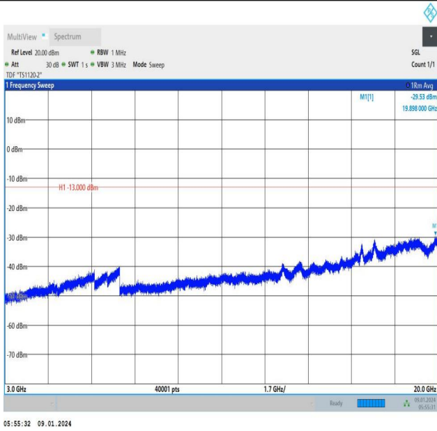
Band66_5MHz_QPSK_132647_25RB#0_3000~20000_3000~20000
