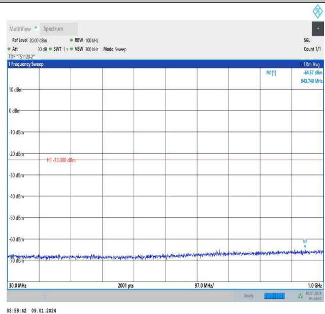
Band66_10MHz_16QAM_132022_1RB#49_30~1000_30~100
