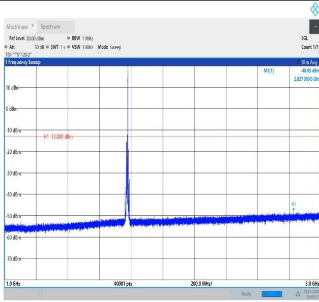
Band66_10MHz_16QAM_132622_1RB#49_1000~3000_1000 ~3000
