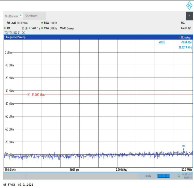
Band66_10MHz_QPSK_132022_1RB#49_0.15~30_0.15~30
