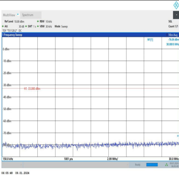
Band66_10MHz_QPSK_132322_50RB#0_0.15~30_0.15~30
