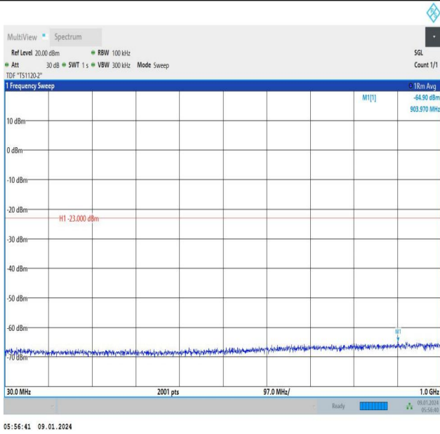
Band66_10MHz_QPSK_132022_1RB#0_30~1000_30~1000
