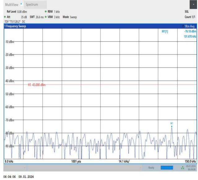
Band66_10MHz_16QAM_132622_1RB#49_0.009~0.15_0.009~0.15
