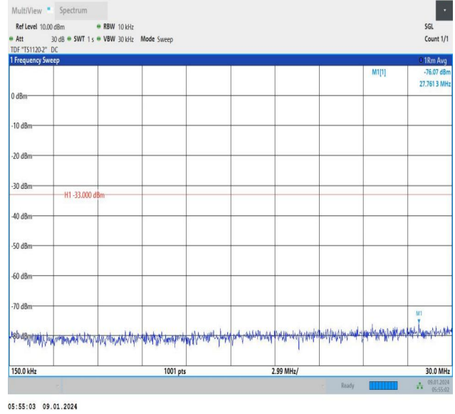
Band66_5MHz_QPSK_132647_25RB#0_0.15~30_0.15~30
