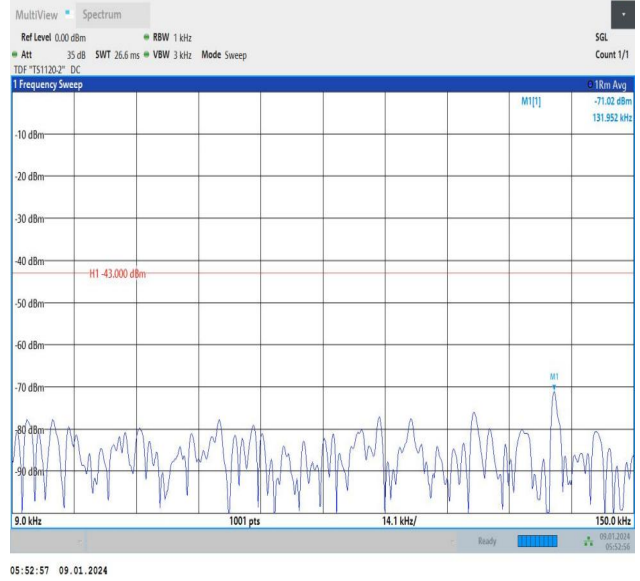
Band66_5MHz_16QAM_132647_1RB#0_0.009~0.15_0.009~0.15
