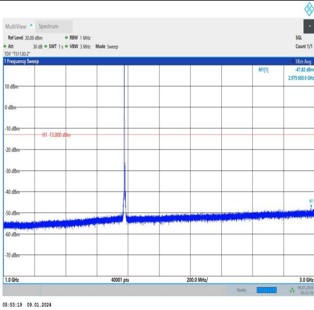
Band66_5MHz_16QAM_132647_1RB#0_1000~3000_1000~3000
