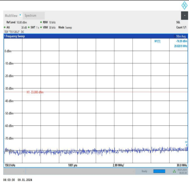
Band66_10MHz_QPSK_132622_1RB#49_0.15~30_0.15~30
