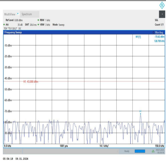
Band66_5MHz_16QAM_132647_1RB#24_0.009~0.15_0.009~0.15
