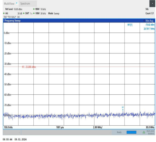
Band66_10MHz_QPSK_132322_1RB#49_0.15~30_0.15~30
