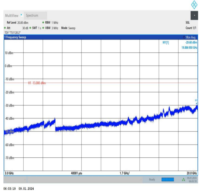
Band66_10MHz_16QAM_132622_1RB#0_3000~20000_3000~20000
