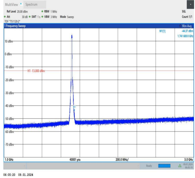
Band66_10MHz_QPSK_132022_50RB#0_1000~3000_1000~3000
