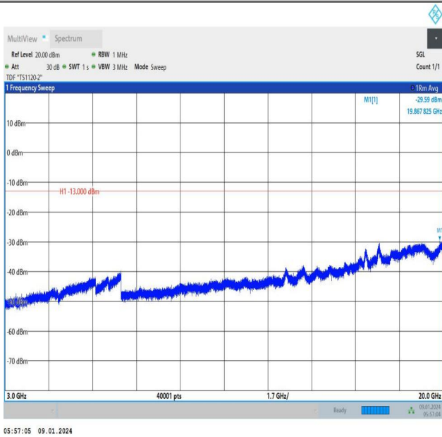
Band66_10MHz_QPSK_132022_1RB#0_3000~20000_3000~20000
