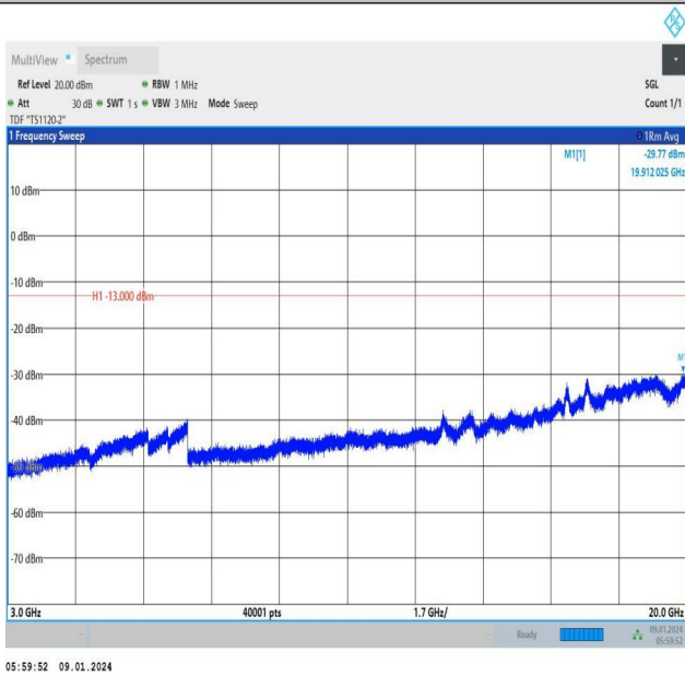
Band66_10MHz_QPSK_132322_1RB#0_3000~20000_3000~20000
