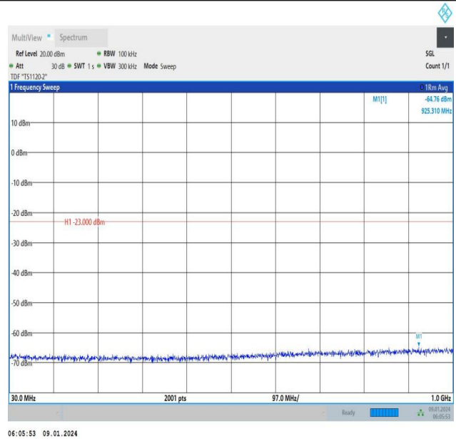
Band66_10MHz_QPSK_132322_50RB#0_30~1000_30~1000
