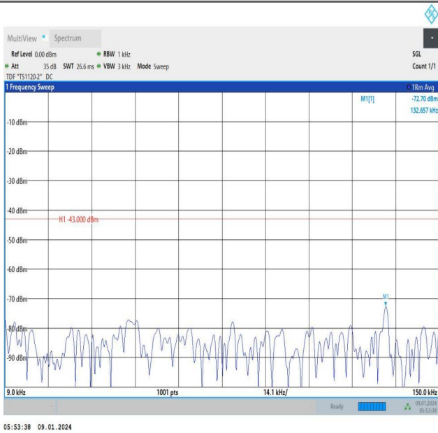
Band66_5MHz_QPSK_132647_1RB#24_0.009~0.15_0.009~0.15
