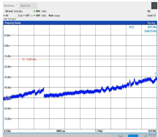
Band66_10MHz_16QAM_132022_1RB#0_3000~20000_3000~20000
