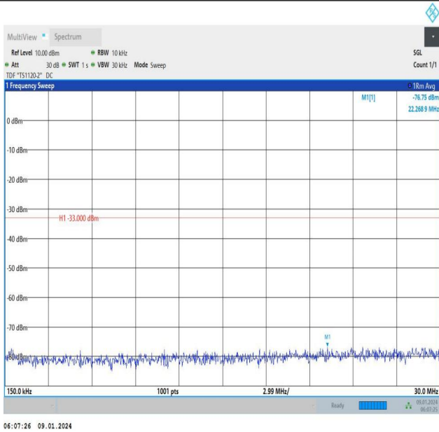
Band66_15MHz_QPSK_132047_1RB#0_0.15~30_0.15~30
