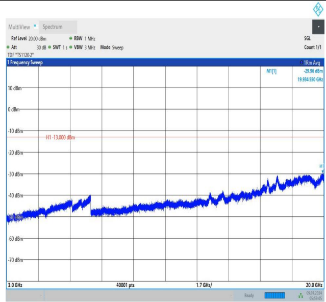
Band66_10MHz_16QAM_132022_1RB#49_3000~20000_300 0~20000
