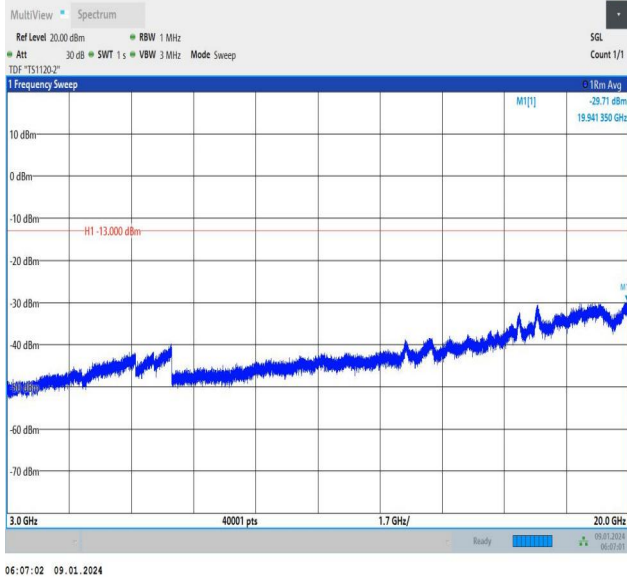
Band66_10MHz_QPSK_132622_50RB#0_3000~20000_3000~20000
