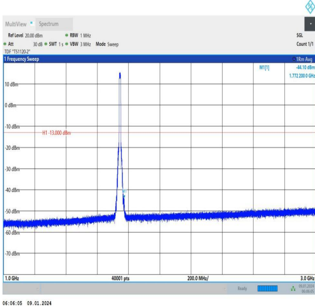
Band66_10MHz_QPSK_132322_50RB#0_1000~3000_1000~3000
