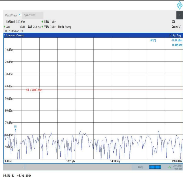
Band66_5MHz_16QAM_132322_25RB#0_0.009~0.15_0.009~0.15
