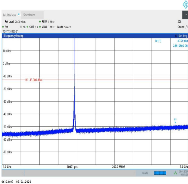
Band66_10MHz_16QAM_132622_1RB#0_1000~3000_1000~3000
