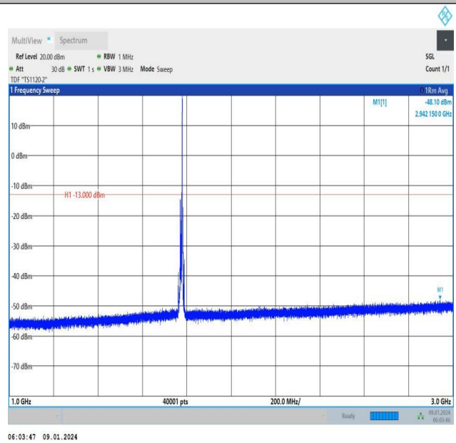
Band66_10MHz_QPSK_132622_1RB#49_1000~3000_1000~3000
