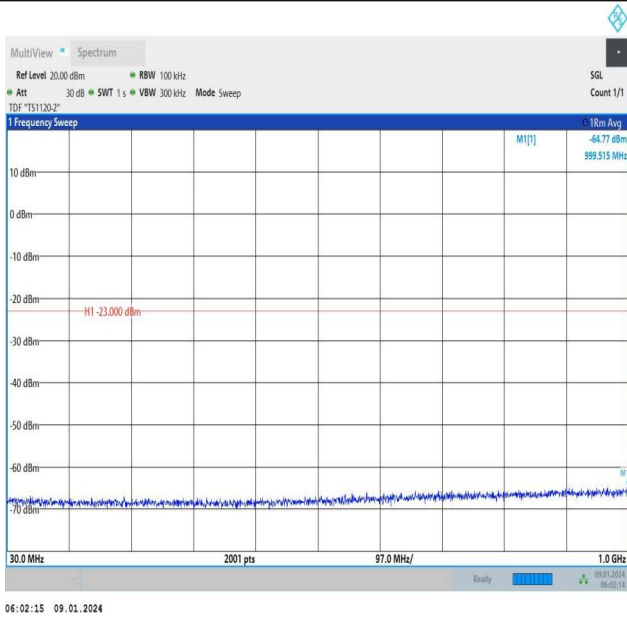
Band66_10MHz_QPSK_132622_1RB#0_30~1000_30~1000
