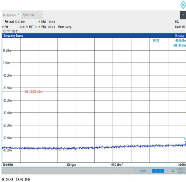
Band66_10MHz_QPSK_132322_1RB#49_30~1000_30~1000
