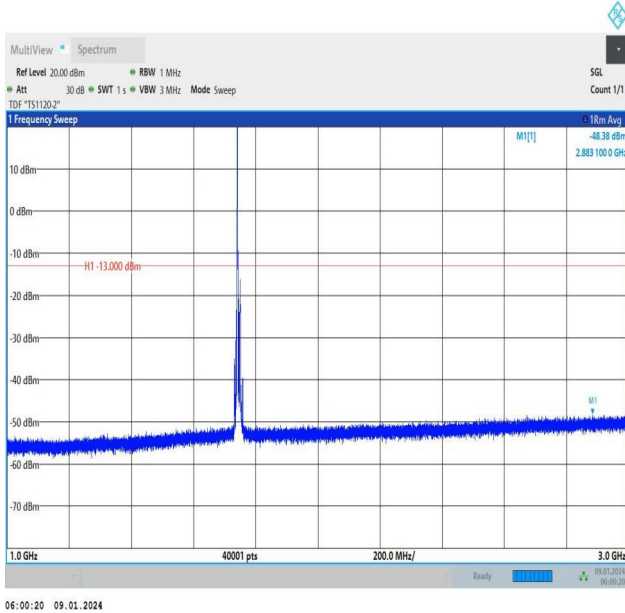
Band66_10MHz_16QAM_132322_1RB#0_1000~3000_1000~3000
