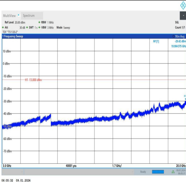
Band66_10MHz_QPSK_132022_50RB#0_3000~20000_3000~20000
