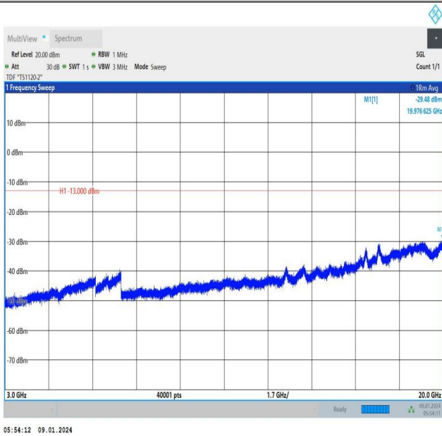
Band66_5MHz_QPSK_132647_1RB#24_3000~20000_3000~20000
