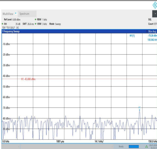
Band66_5MHz_16QAM_132647_25RB#0_1000~3000_1000~3000
