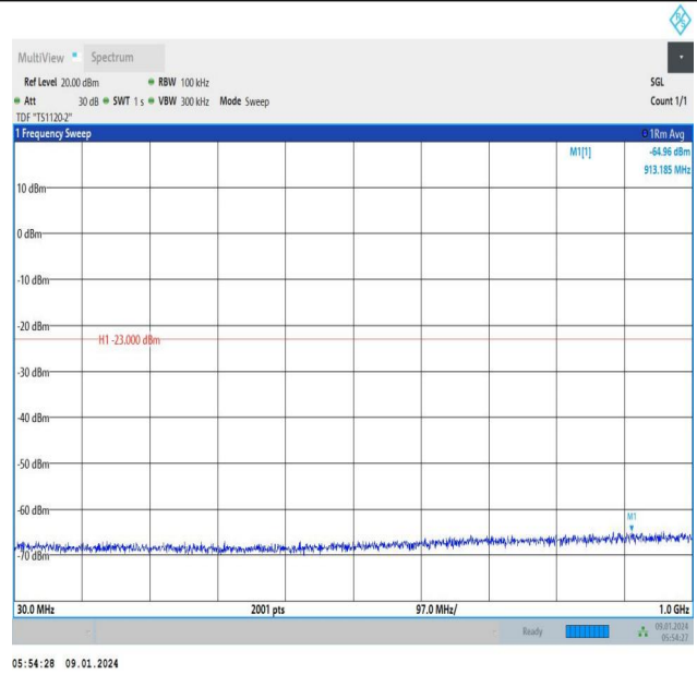
Band66_5MHz_16QAM_132647_1RB#24_30~1000_30~1000
