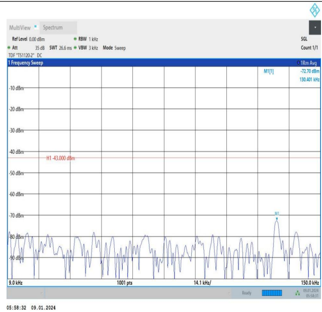
Band66_10MHz_16QAM_132022_1RB#49_0.009~0.15_0.009 ~0.15
