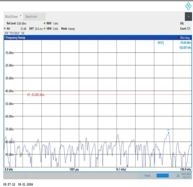
Band66_10MHz_16QAM_132022_1RB#0_0.009~0.15_0.009~0.15
