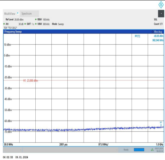
Band66_10MHz_16QAM_132622_1RB#0_30~1000_30~1000
