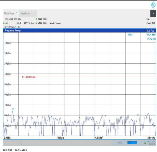
Band66_10MHz_16QAM_132322_1RB#0_0.009~0.15_0.009~0.15
