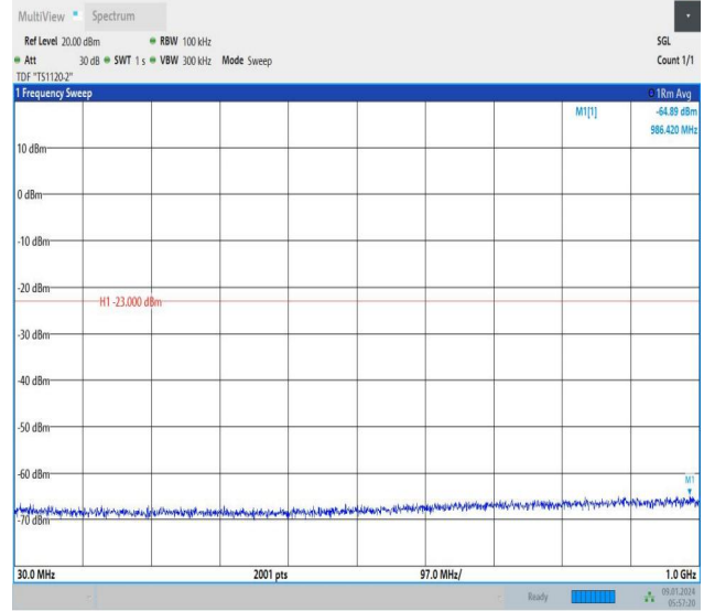
Band66_10MHz_16QAM_132022_1RB#0_30~1000_30~1000
