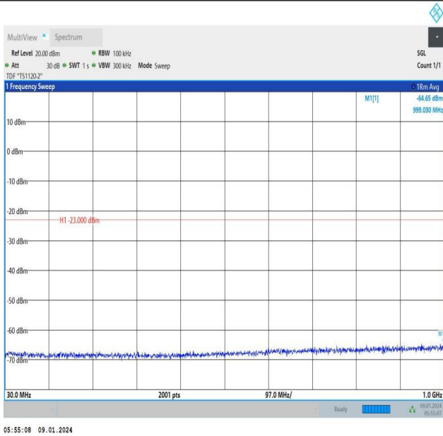
Band66_5MHz_QPSK_132647_25RB#0_30~1000_30~1000
