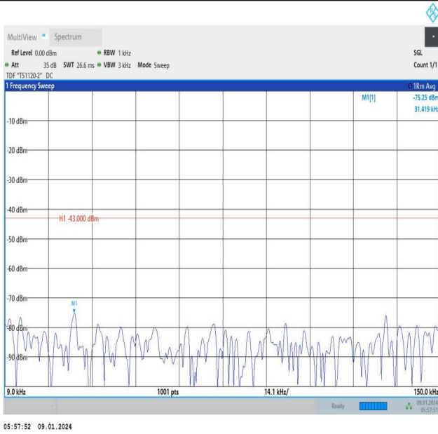
Band66_10MHz_QPSK_132022_1RB#49_0.009~0.15_0.009~0.15
