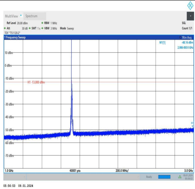
Band66_10MHz_QPSK_132022_1RB#0_1000~3000_1000~3000
