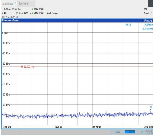
Band66_10MHz_16QAM_132022_1RB#0_0.15~30_0.15~30
