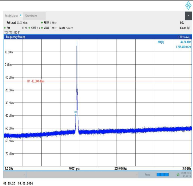
Band66_5MHz_QPSK_132647_25RB#0_1000~3000_1000~3000
