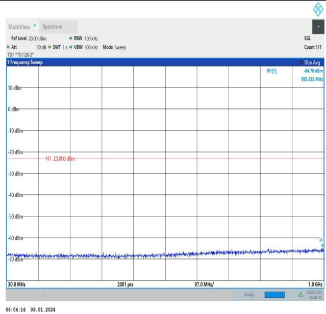
Band66_10MHz_16QAM_132622_1RB#49_30~1000_30~100 0
