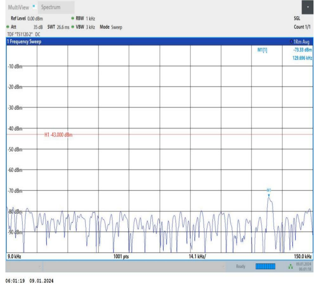
Band66_10MHz_16QAM_132322_1RB#49_0.009~0.15_0.009~0.15
