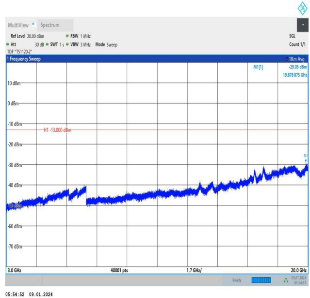
Band66_5MHz_16QAM_132647_1RB#24_3000~20000_3000~20000
