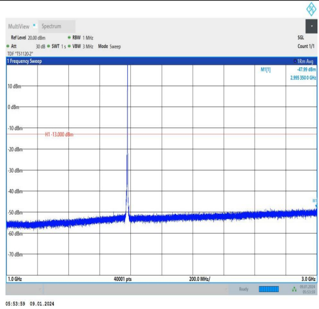
Band66_5MHz_QPSK_132647_1RB#24_1000~3000_1000~3000
