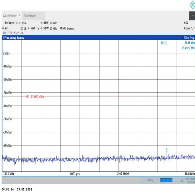
Band66_10MHz_16QAM_132322_1RB#49_0.15~30_0.15~30
