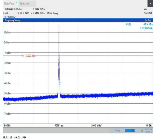
Band66_5MHz_QPSK_132322_25RB#0_1000~3000_1000~3000
