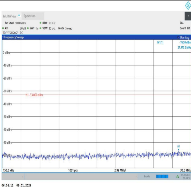
Band66_10MHz_16QAM_132622_1RB#49_0.15~30_0.15~30
