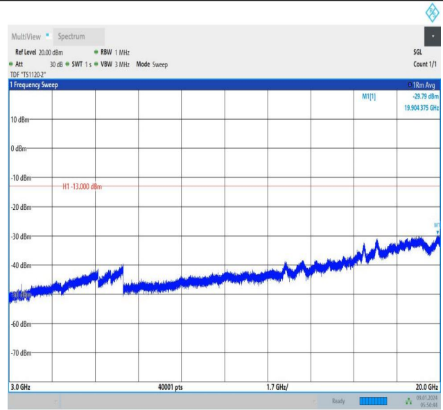
Band66_5MHz_16QAM_132322_1RB#24_3000~20000_3000~20000
