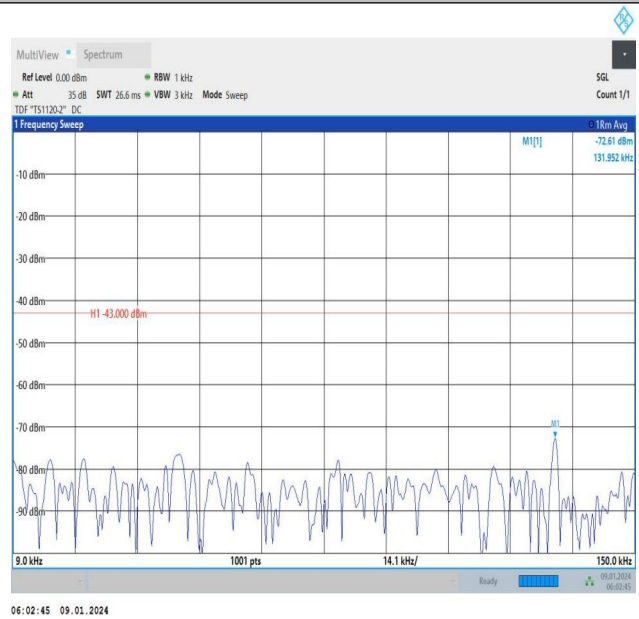
Band66_10MHz_16QAM_132622_1RB#0_0.009~0.15_0.009~0.15
