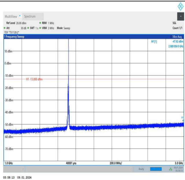
Band66_10MHz_QPSK_132022_1RB#49_1000~3000_1000~3000
