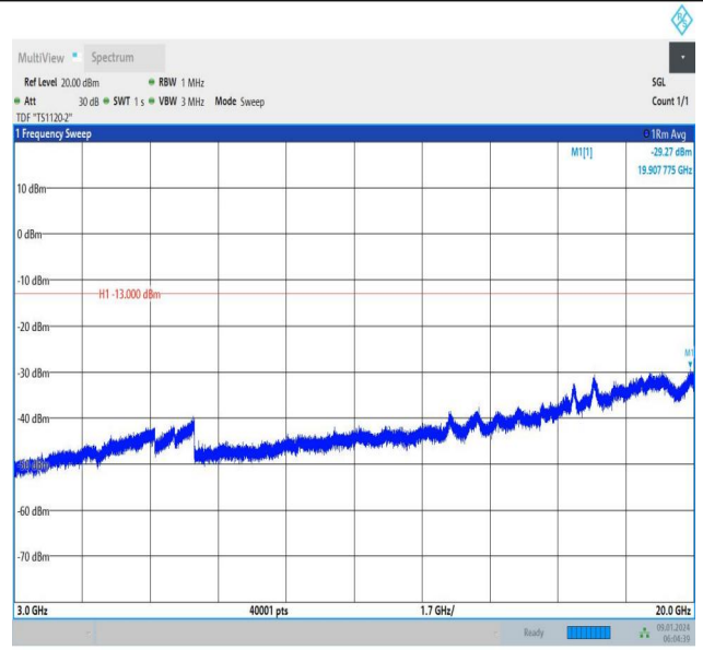
Band66_10MHz_16QAM_132622_1RB#49_3000~20000_300 0~20000
