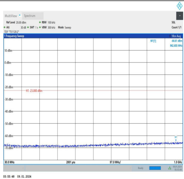
Band66_5MHz_16QAM_132647_25RB#0_30~1000_30~1000
