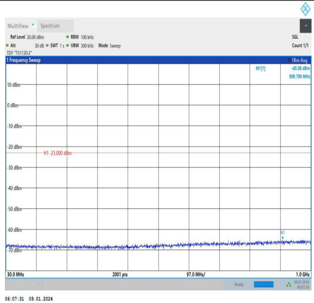
Band66_15MHz_QPSK_132047_1RB#0_30~1000_30~1000
