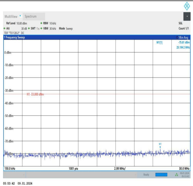
Band66_5MHz_QPSK_132647_1RB#24_0.15~30_0.15~30
