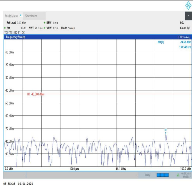
Band66_5MHz_16QAM_132647_25RB#0_0.009~0.15_0.009~0.15
