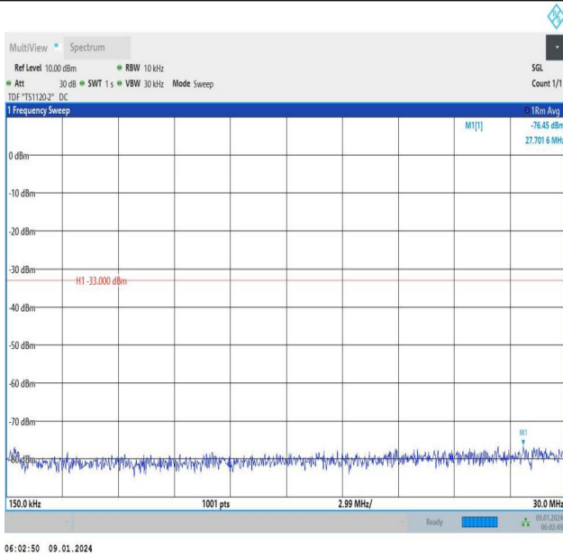
Band66_10MHz_16QAM_132622_1RB#0_0.15~30_0.15~30
