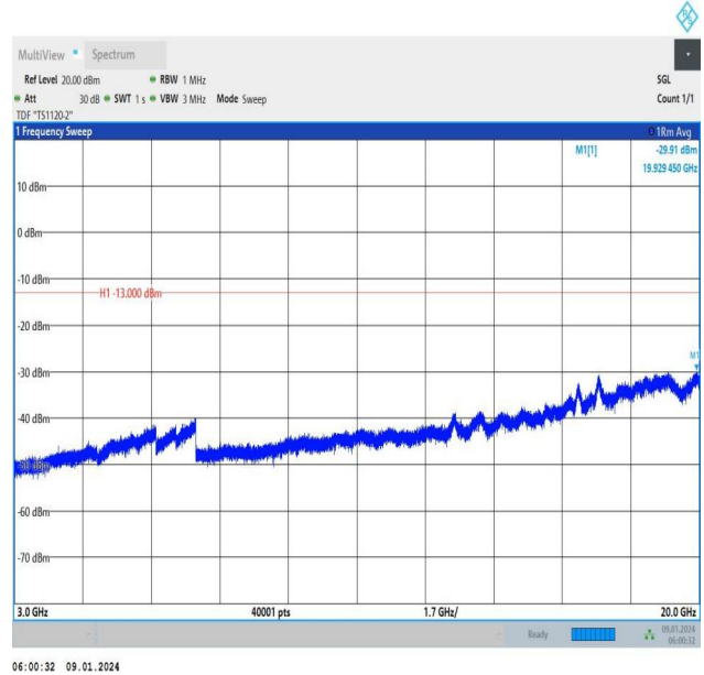
Band66_10MHz_16QAM_132322_1RB#0_3000~20000_3000~20000
