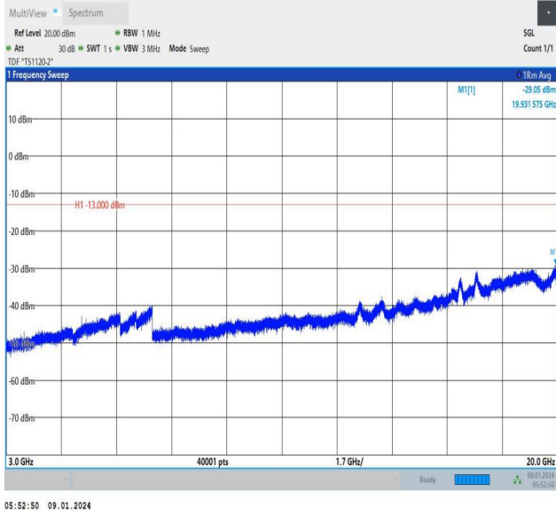
Band66_5MHz_QPSK_132647_1RB#0_3000~20000_3000~20000
