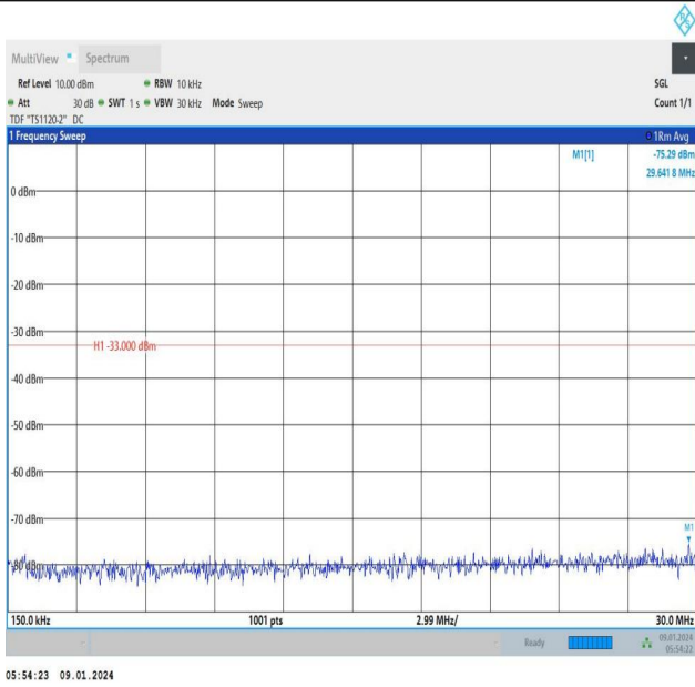
Band66_5MHz_16QAM_132647_1RB#24_0.15~30_0.15~30
