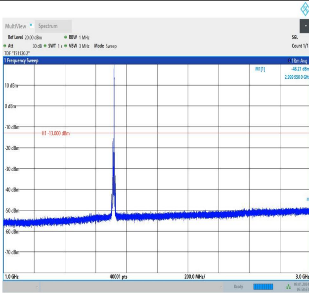
Band66_10MHz_16QAM_132022_1RB#49_1000~3000_1000 ~3000
