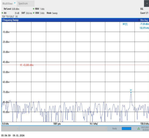
Band66_5MHz_QPSK_132647_25RB#0_0.009~0.15_0.009~0.15
