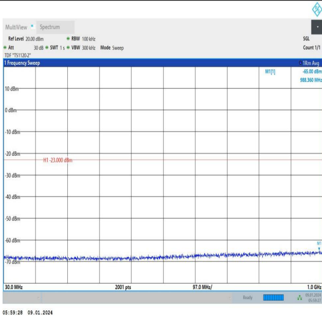
Band66_10MHz_QPSK_132322_1RB#0_30~1000_30~1000
