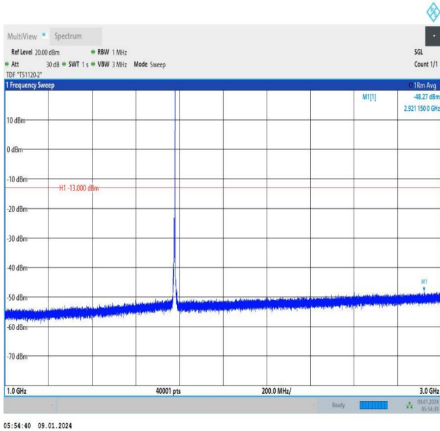
Band66_5MHz_16QAM_132647_1RB#24_1000~3000_1000~3000
