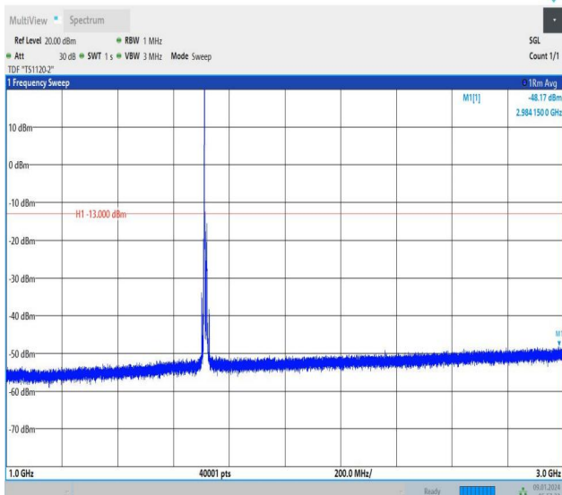
Band66_10MHz_16QAM_132022_1RB#0_1000~3000_1000~3000
