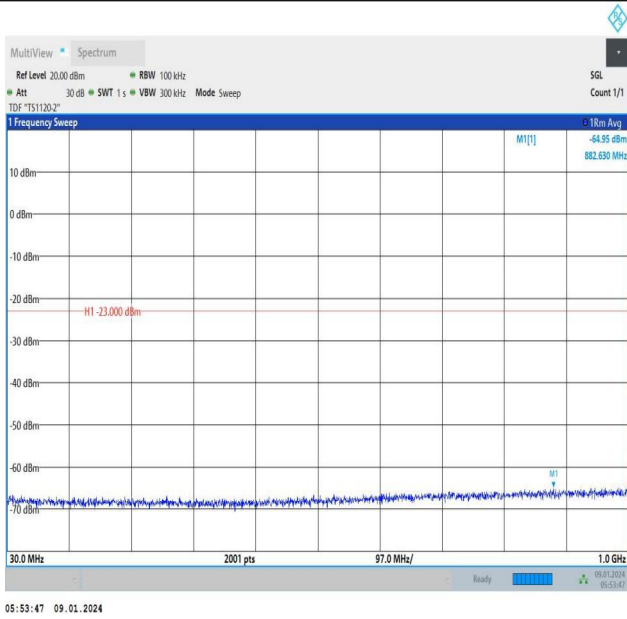
Band66_5MHz_QPSK_132647_1RB#24_30~1000_30~1000
