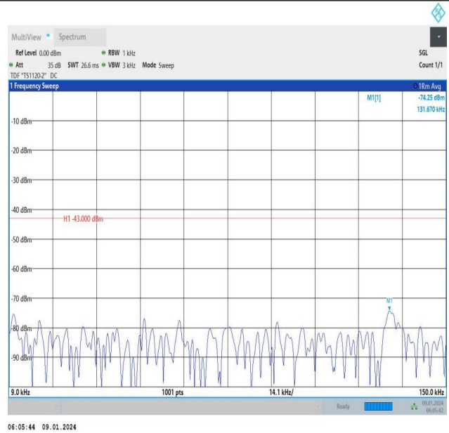
Band66_10MHz_QPSK_132322_50RB#0_0.009~0.15_0.009~0.15
