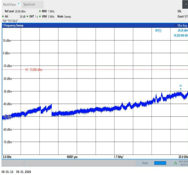
Band66_10MHz_QPSK_132322_1RB#49_3000~20000_3000~20000
