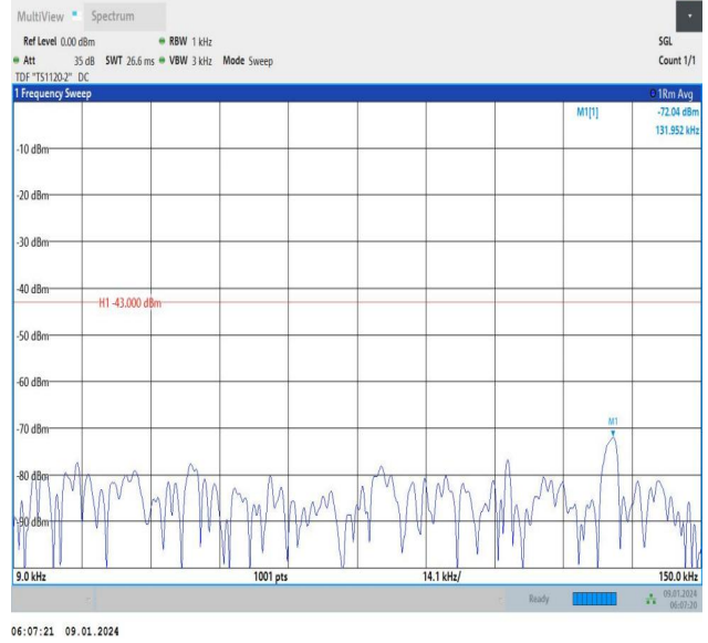
Band66_15MHz_QPSK_132047_1RB#0_0.009~0.15_0.009~0.15
