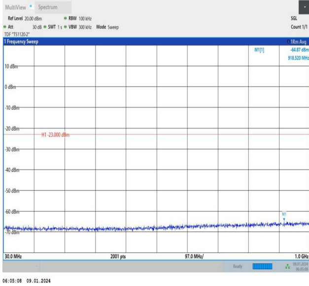
Band66_10MHz_QPSK_132022_50RB#0_30~1000_30~1000
