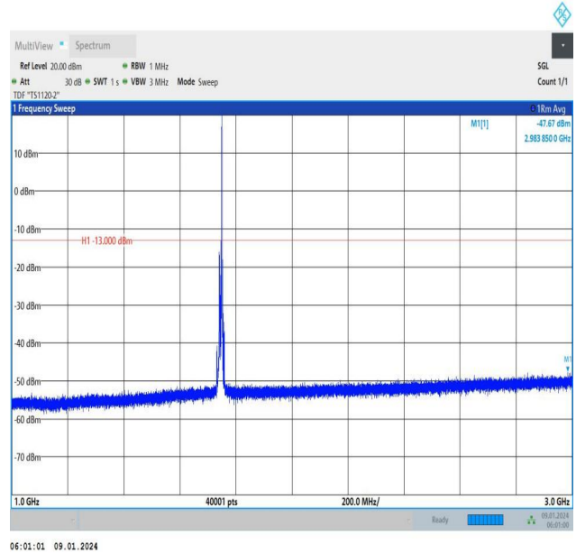
Band66_10MHz_QPSK_132322_1RB#49_1000~3000_1000~3000
