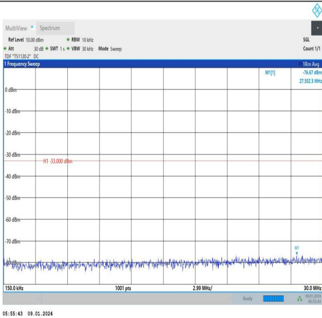
Band66_5MHz_16QAM_132647_25RB#0_0.15~30_0.15~30
