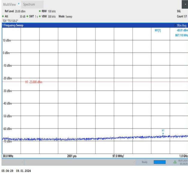
Band66_3MHz_QPSK_131987_15RB#0_30~1000_30~1000
