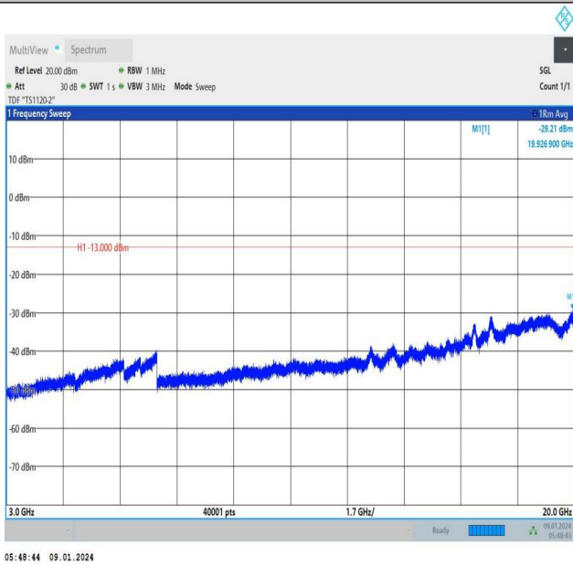
Band66_5MHz_QPSK_132322_1RB#0_3000~20000_3000~2 0000
