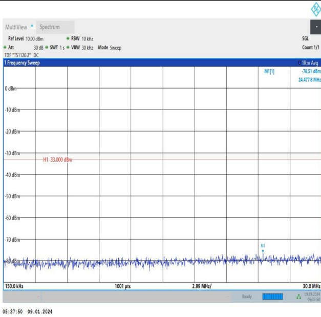
Band66_3MHz_16QAM_132322_1RB#14_0.15~30_0.15~30
