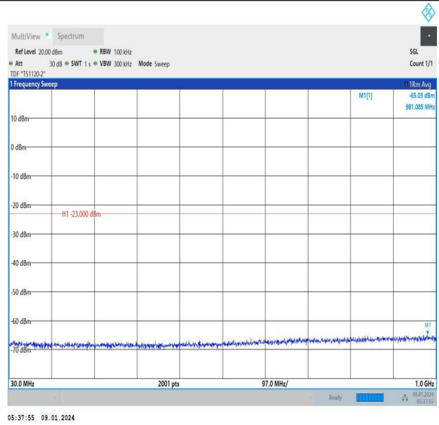
Band66_3MHz_16QAM_132322_1RB#14_30~1000_30~1000
