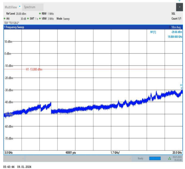
Band66_3MHz_16QAM_132657_15RB#0_3000~20000_3000~20000
