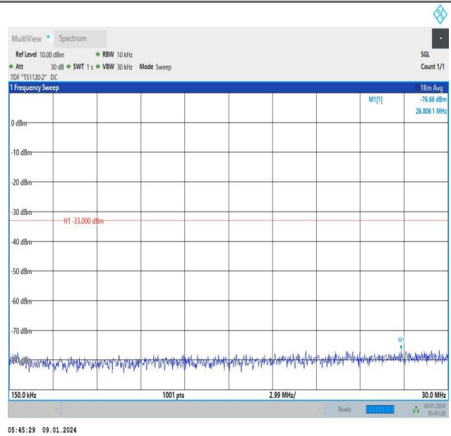
Band66_5MHz_QPSK_131997_1RB#24_0.15~30_0.15~30
