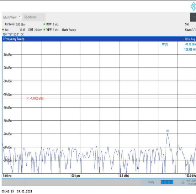
Band66_5MHz_QPSK_131997_1RB#24_0.009~0.15_0.009~0.15
