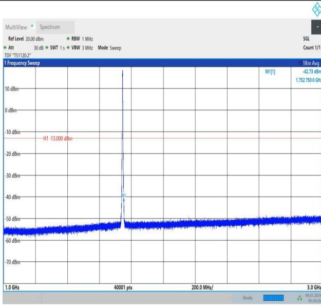
Band66_3MHz_16QAM_132322_15RB#0_1000~3000_1000~3000
