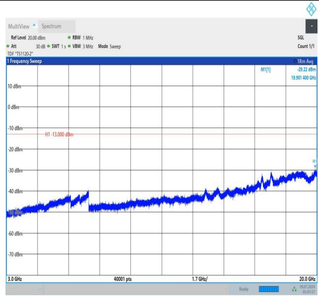
Band66_5MHz_16QAM_131997_25RB#0_3000~20000_3000~20000
