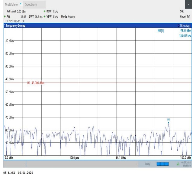
Band66_3MHz_16QAM_132657_1RB#14_0.009~0.15_0.009~0.15
