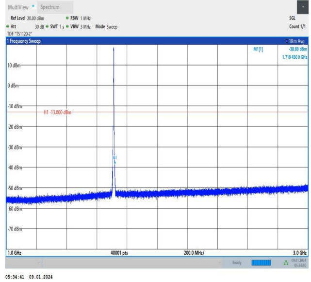
Band66_3MHz_QPSK_131987_15RB#0_1000~3000_1000~3000
