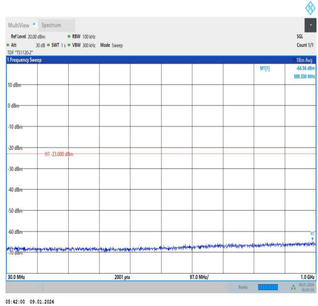
Band66_3MHz_16QAM_132657_1RB#14_30~1000_30~1000
