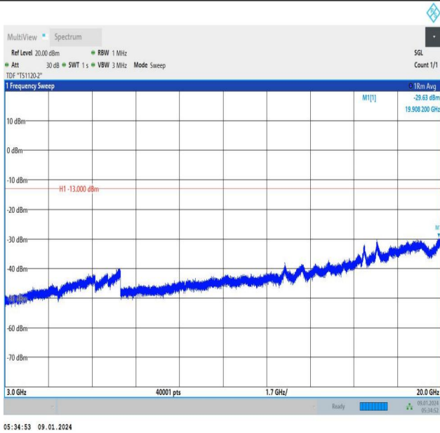
Band66_3MHz_QPSK_131987_15RB#0_3000~20000_3000~20000
