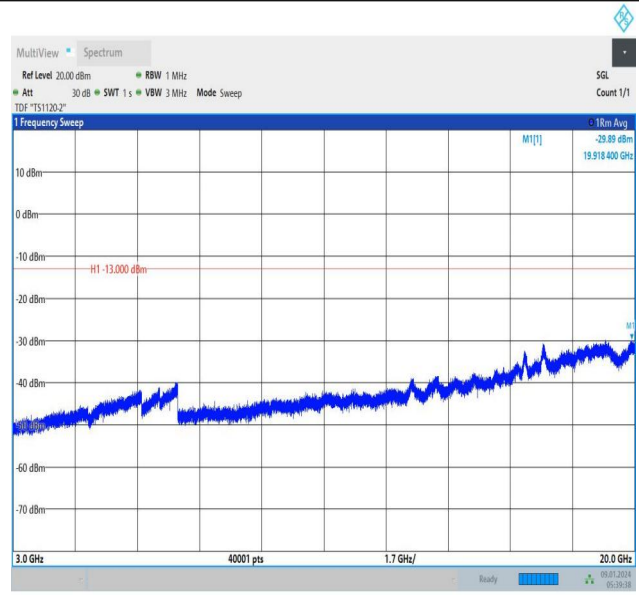
Band66_3MHz_16QAM_132322_15RB#0_3000~20000_3000~20000
