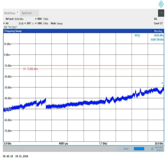
Band66_5MHz_16QAM_131997_1RB#0_3000~20000_3000~20000
