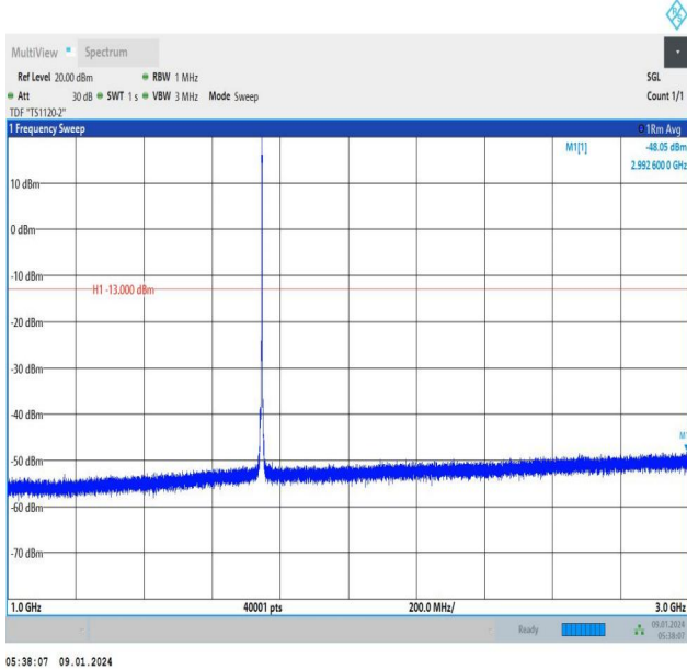
Band66_3MHz_16QAM_132322_1RB#14_1000~3000_1000~3000
