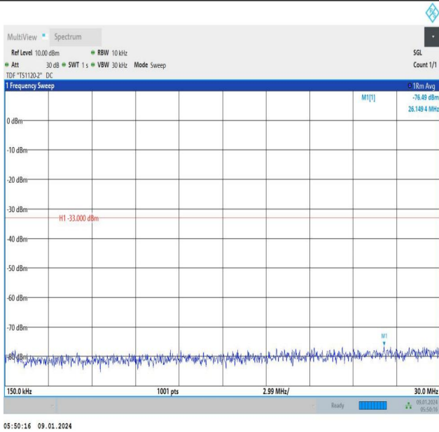
Band66_5MHz_16QAM_132322_1RB#24_0.15~30_0.15~30
