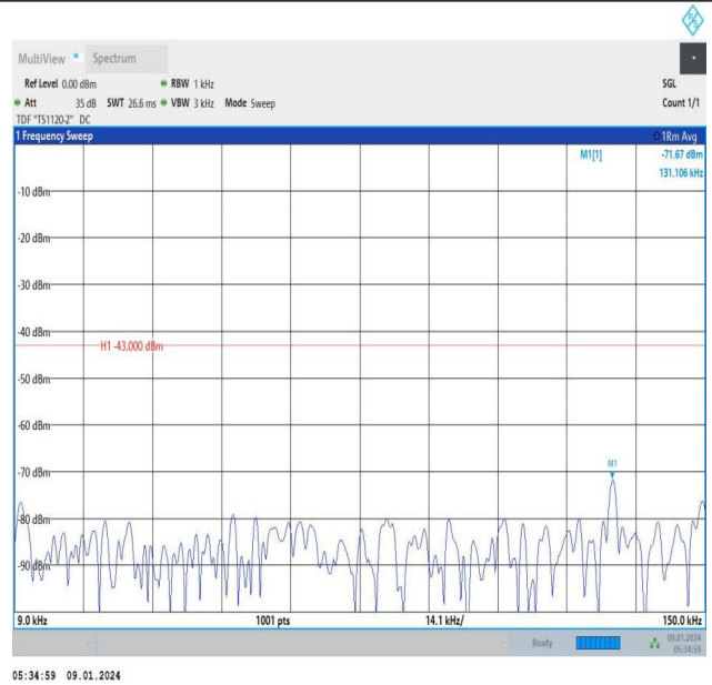
Band66_3MHz_16QAM_131987_15RB#0_0.009~0.15_0.009~0.15
