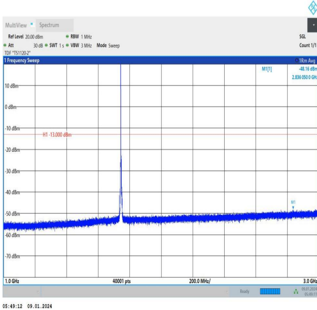
Band66_5MHz_16QAM_132322_1RB#0_1000~3000_1000~3000
