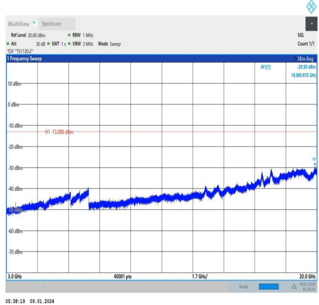
Band66_3MHz_16QAM_132322_1RB#14_3000~20000_3000~20000
