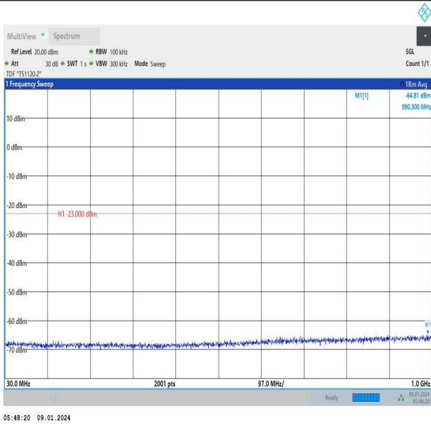
Band66_5MHz_QPSK_132322_1RB#0_30~1000_30~1000
