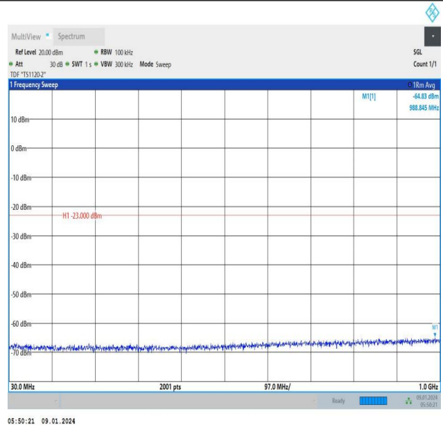
Band66_5MHz_16QAM_132322_1RB#24_30~1000_30~1000
