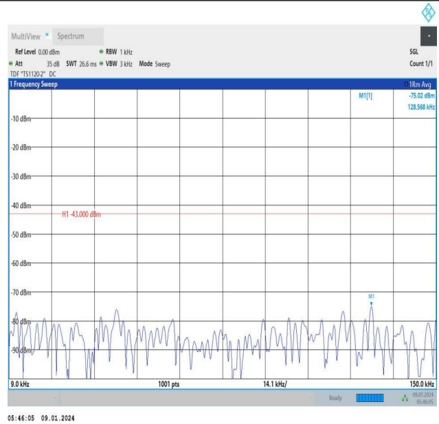
Band66_5MHz_16QAM_131997_1RB#24_0.009~0.15_0.009~0.15
