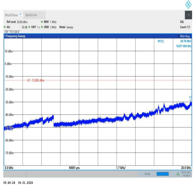
Band66_5MHz_16QAM_132322_1RB#0_3000~20000_3000~20000
