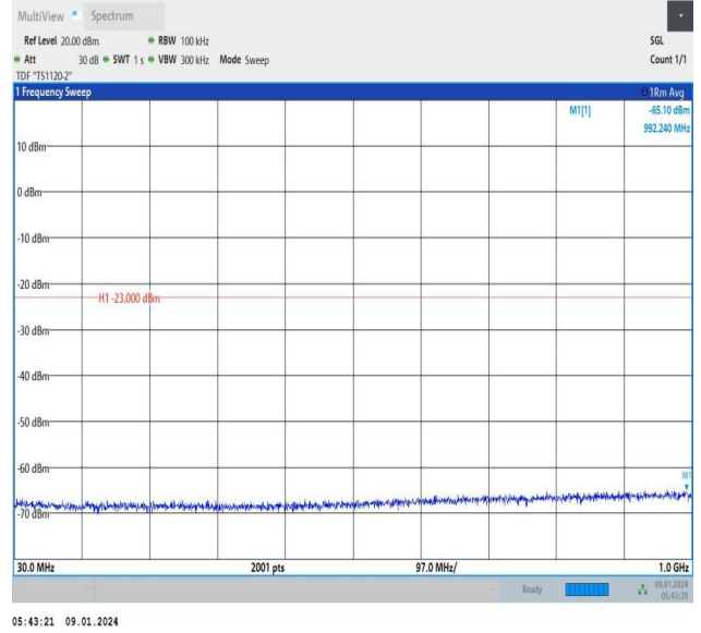
Band66_3MHz_16QAM_132657_15RB#0_30~1000_30~1000
