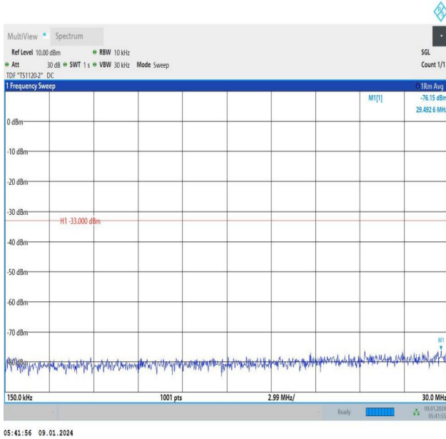
Band66_3MHz_16QAM_132657_1RB#14_0.15~30_0.15~30
