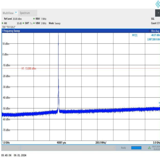
Band66_5MHz_16QAM_131997_1RB#0_1000~3000_1000~3000
