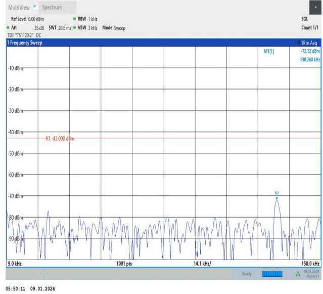
Band66_5MHz_16QAM_132322_1RB#24_0.009~0.15_0.009~0.15
