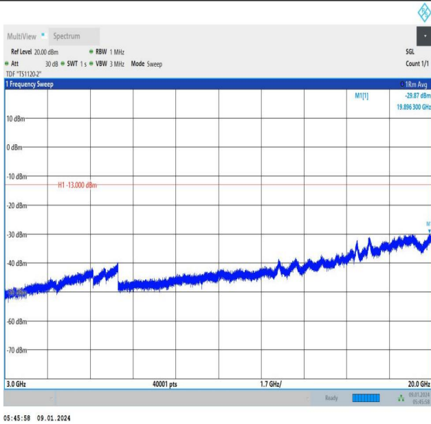
Band66_5MHz_QPSK_131997_1RB#24_3000~20000_3000~20000
