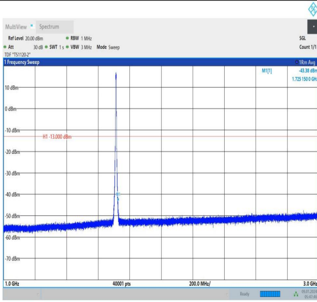
Band66_5MHz_16QAM_131997_25RB#0_1000~3000_1000~3000
