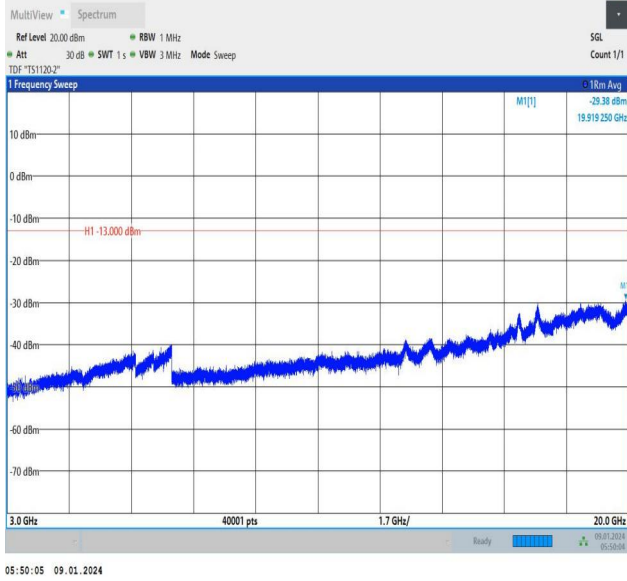
Band66_5MHz_QPSK_132322_1RB#24_3000~20000_3000~20000
