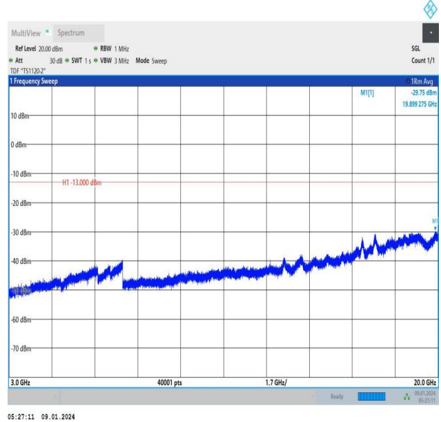
Band66_1.4MHz_16QAM_132322_6RB#0_3000~20000_3000~20000
