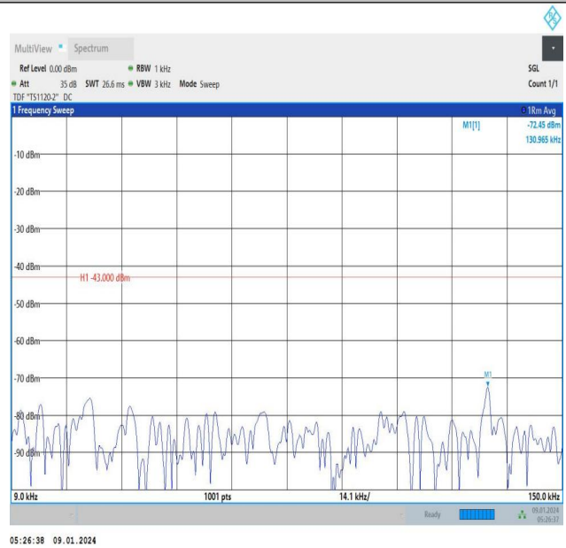
Band66_1.4MHz_16QAM_132322_6RB#0_0.009~0.15_0.009~0.15
