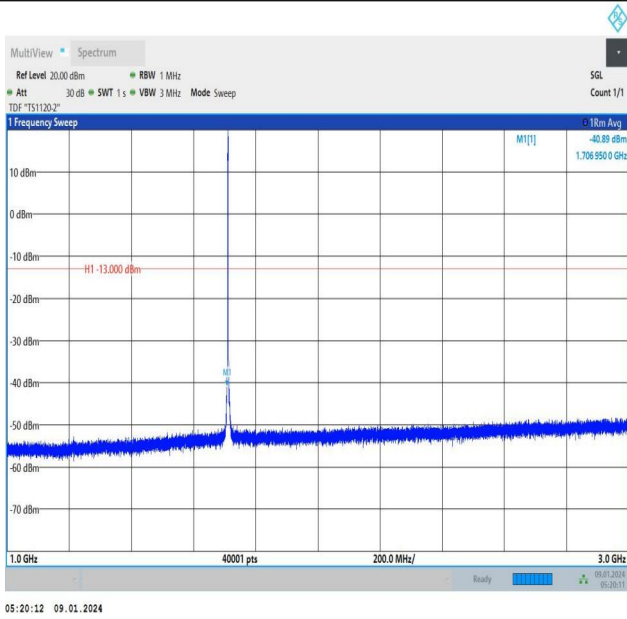
Band66_1.4MHz_16QAM_131979_1RB#0_1000~3000_1000~3000
