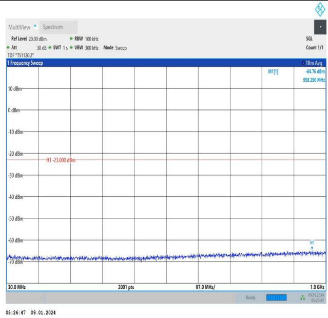
Band66_1.4MHz_16QAM_132322_6RB#0_30~1000_30~1000
