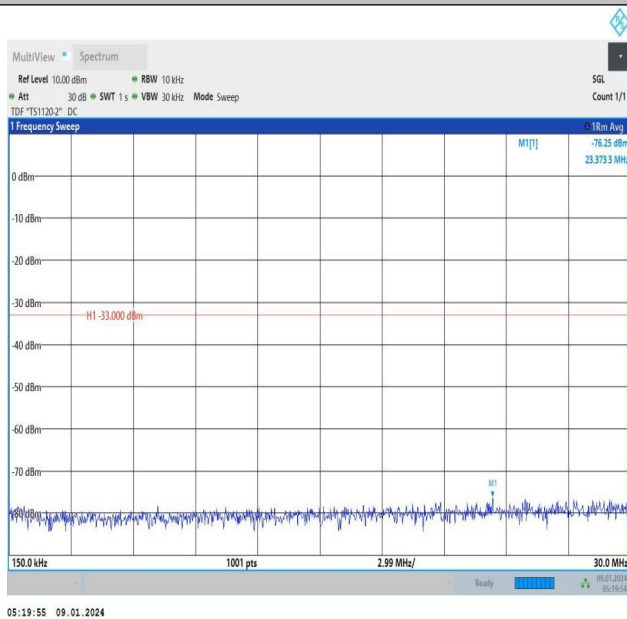
Band66_1.4MHz_16QAM_131979_1RB#0_0.15~30_0.15~30
