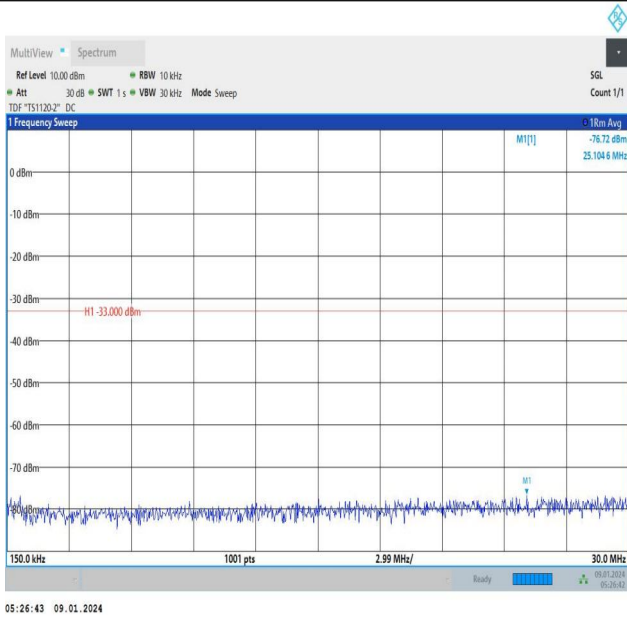
Band66_1.4MHz_16QAM_132322_6RB#0_0.15~30_0.15~30
