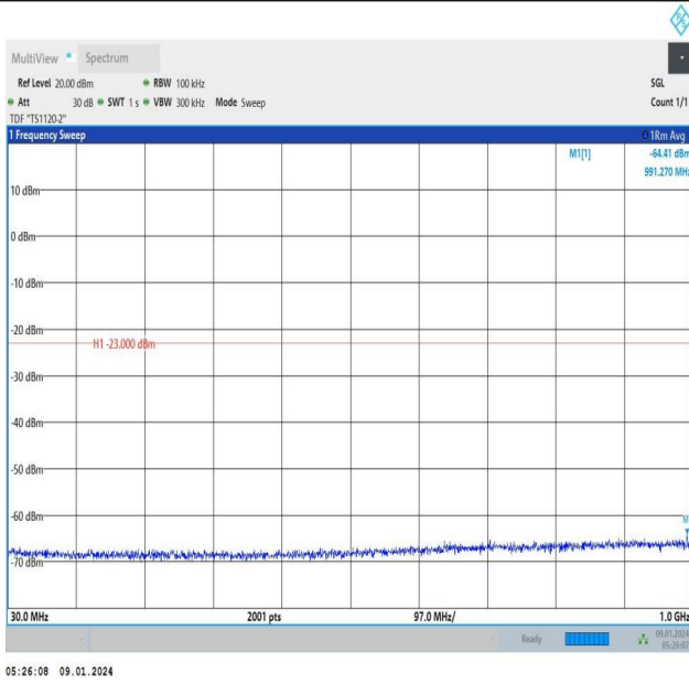
Band66_1.4MHz_QPSK_132322_6RB#0_30~1000_30~1000
