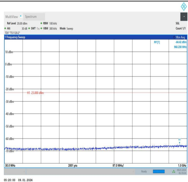
Band66_1.4MHz_16QAM_131979_1RB#0_30~1000_30~1000
