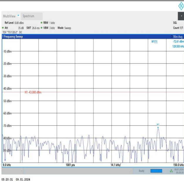
Band66_1.4MHz_QPSK_131979_1RB#5_0.009~0.15_0.009~0.15
