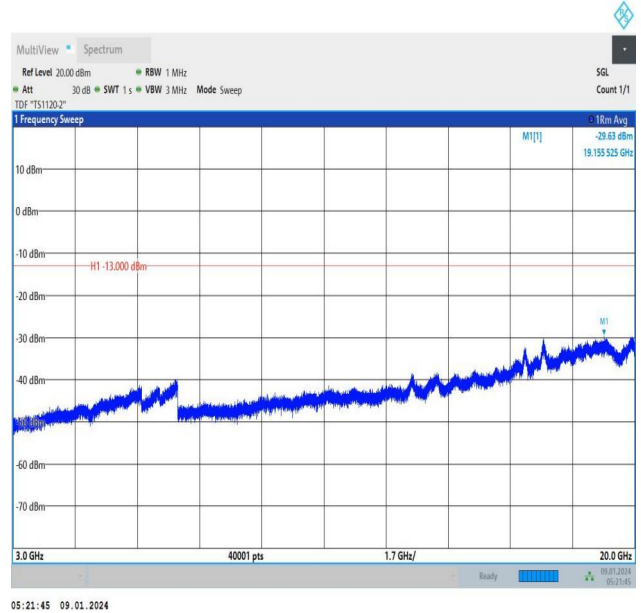
Band66_1.4MHz_16QAM_131979_1RB#5_3000~20000_3000~20000
