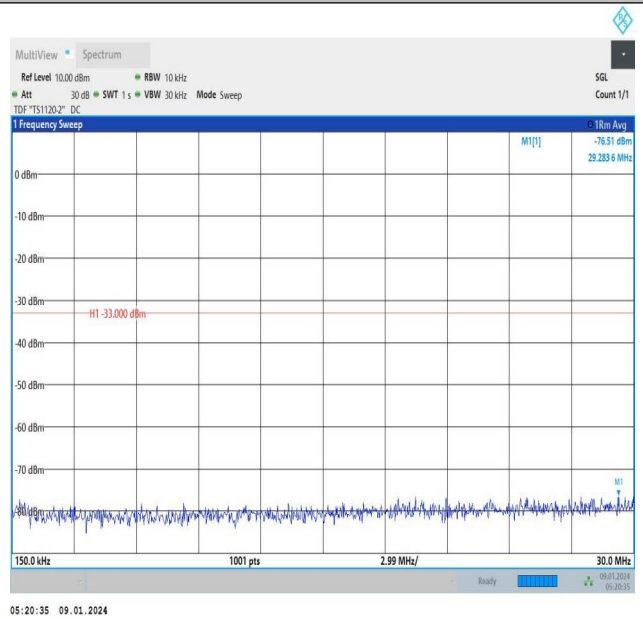
Band66_1.4MHz_QPSK_131979_1RB#5_0.15~30_0.15~30
