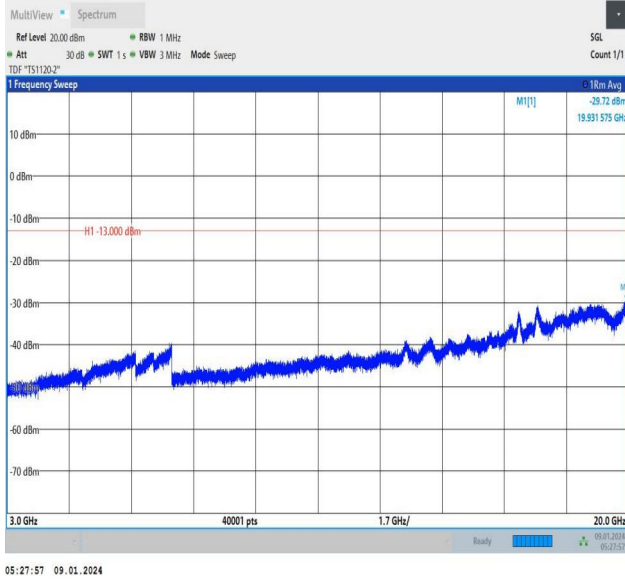
Band66_1.4MHz_QPSK_132665_1RB#0_3000~20000_3000~20000
