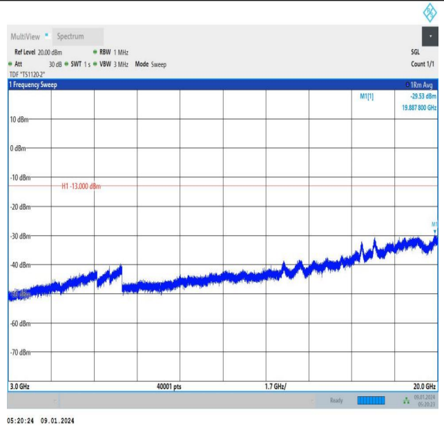
Band66_1.4MHz_16QAM_131979_1RB#0_3000~20000_3000~20000
