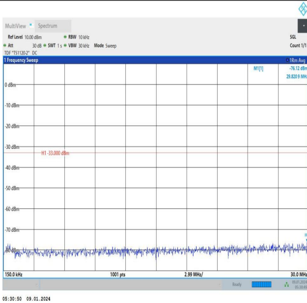
Band66_1.4MHz_16QAM_132665_6RB#0_0.15~30_0.15~30
