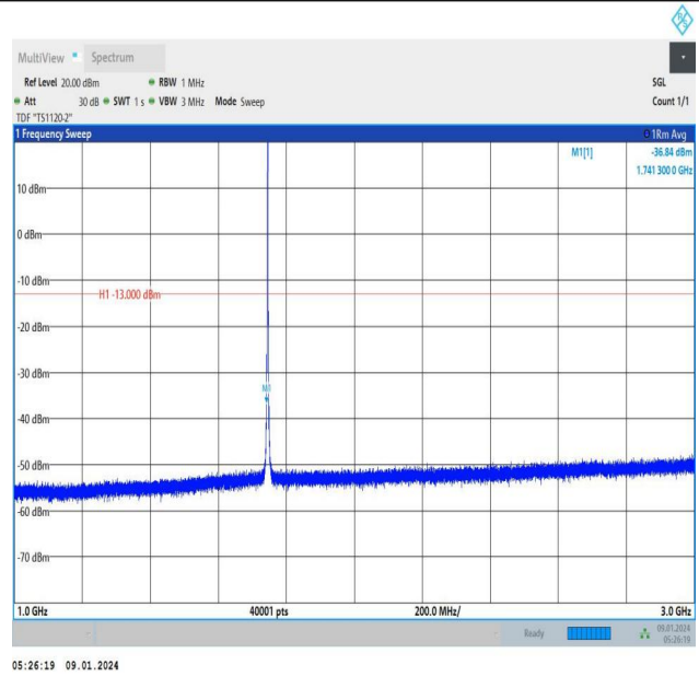
Band66_1.4MHz_QPSK_132322_6RB#0_1000~3000_1000~3000
