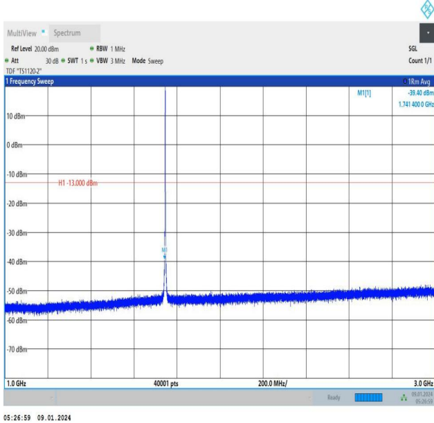
Band66_1.4MHz_16QAM_132322_6RB#0_1000~3000_1000~3000
