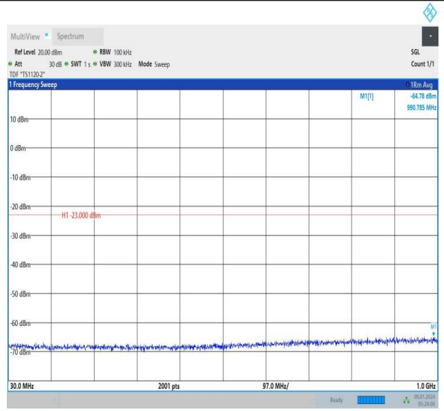
Band66_1.4MHz_16QAM_132322_1RB#0_30~1000_30~1000
