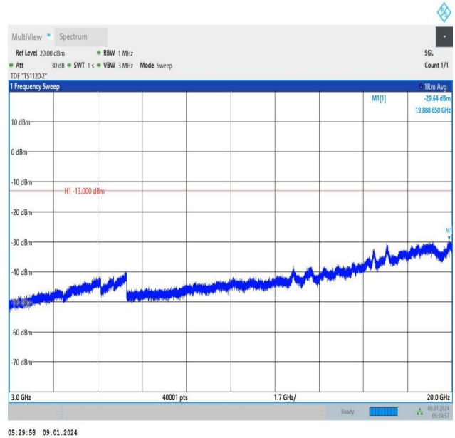
Band66_1.4MHz_16QAM_132665_1RB#5_3000~20000_3000~20000
