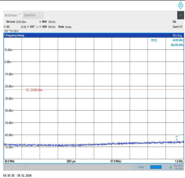
Band66_1.4MHz_16QAM_132665_6RB#0_30~1000_30~1000
