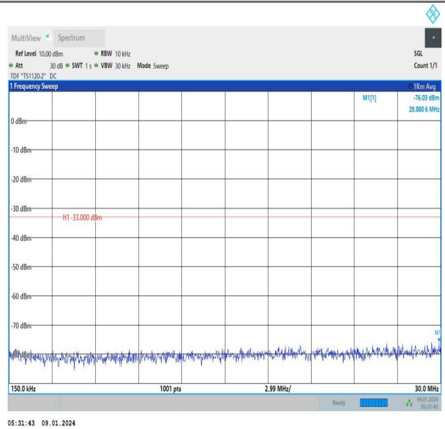
Band66_3MHz_QPSK_131987_1RB#0_0.15~30_0.15~30
