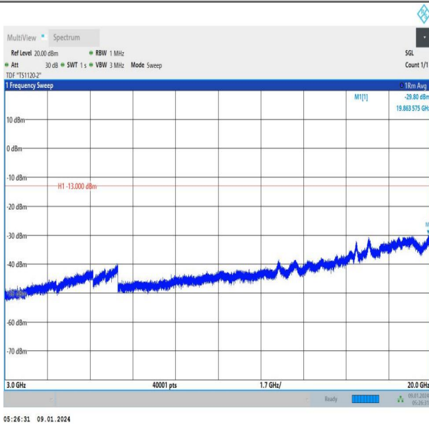
Band66_1.4MHz_QPSK_132322_6RB#0_3000~20000_3000~20000
