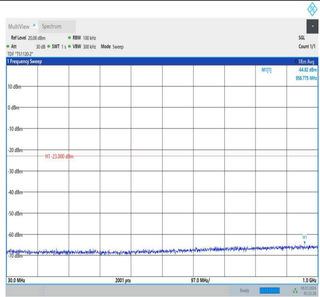
Band66_3MHz_16QAM_131987_1RB#0_30~1000_30~1000
