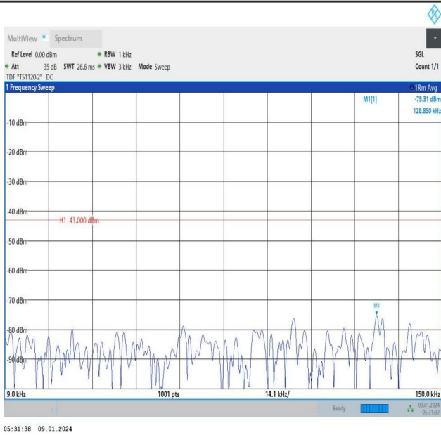
Band66_3MHz_QPSK_131987_1RB#0_0.009~0.15_0.009~0.15
