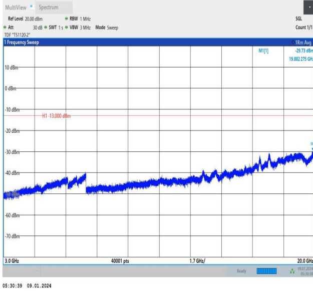
Band66_1.4MHz_QPSK_132665_6RB#0_3000~20000_3000~20000
