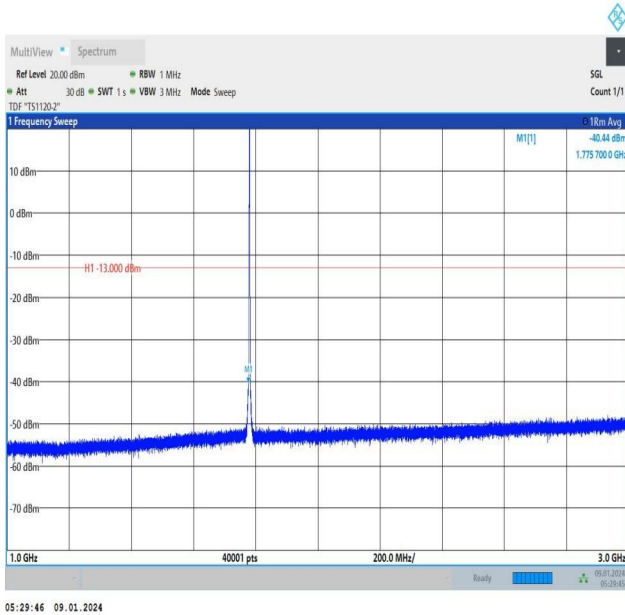
Band66_1.4MHz_16QAM_132665_1RB#5_1000~3000_1000~3000
