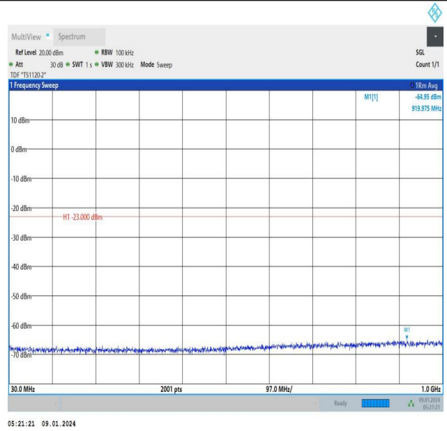
Band66_1.4MHz_16QAM_131979_1RB#5_30~1000_30~1000
