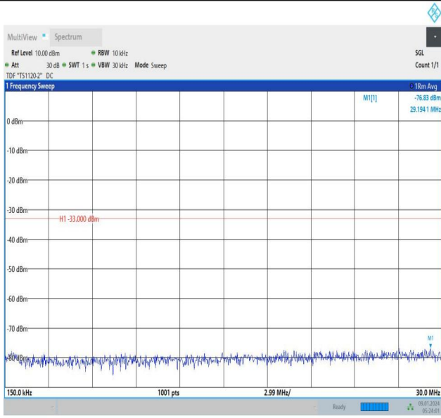
Band66_1.4MHz_16QAM_132322_1RB#0_0.15~30_0.15~30
