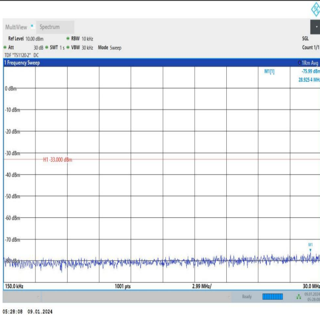
Band66_1.4MHz_16QAM_132665_1RB#0_0.15~30_0.15~30
