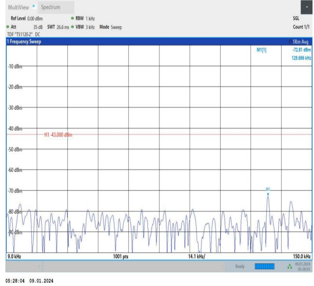
Band66_1.4MHz_16QAM_132665_1RB#0_0.009~0.15_0.009~0.15
