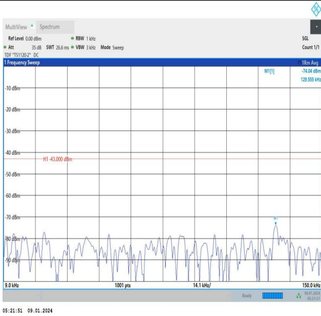
Band66_1.4MHz_QPSK_131979_6RB#0_0.009~0.15_0.009~0.15
