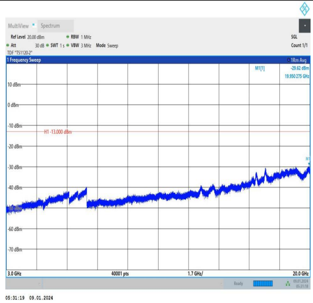
Band66_1.4MHz_16QAM_132665_6RB#0_3000~20000_3000~20000
