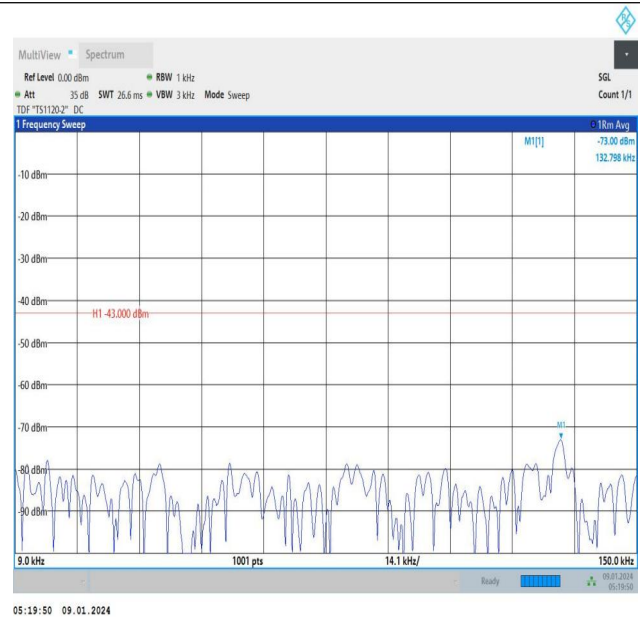
Band66_1.4MHz_16QAM_131979_1RB#0_0.009~0.15_0.009 ~0.15
