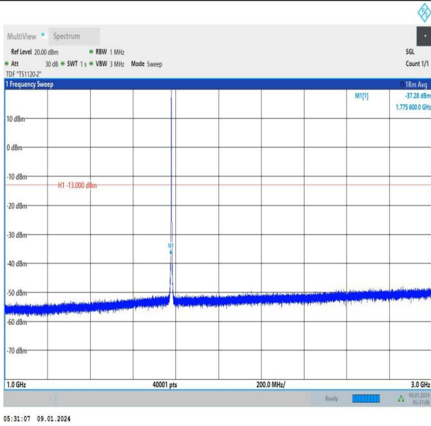
Band66_1.4MHz_16QAM_132665_6RB#0_1000~3000_1000~3000
