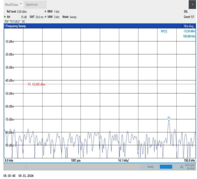
Band66_1.4MHz_16QAM_132665_6RB#0_0.009~0.15_0.009~0.15
