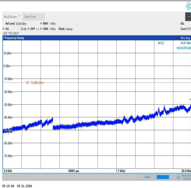
Band66_1.4MHz_QPSK_131979_1RB#0_3000~20000_3000~ 20000
