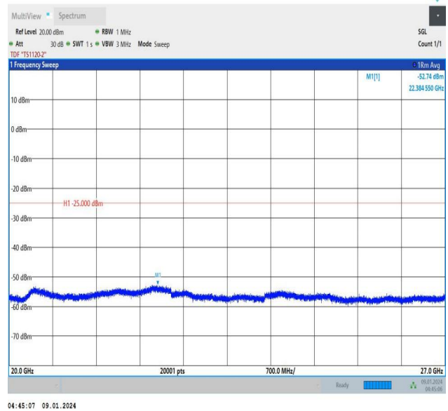
Band41_5MHz_16QAM_40620_25RB#0_20000~27000_20000~27000
