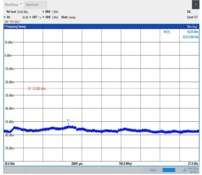
Band41_15MHz_QPSK_39725_1RB#0_20000~27000_20000~27000
