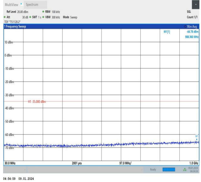
Band41_10MHz_16QAM_41540_1RB#0_30~1000_30~1000
