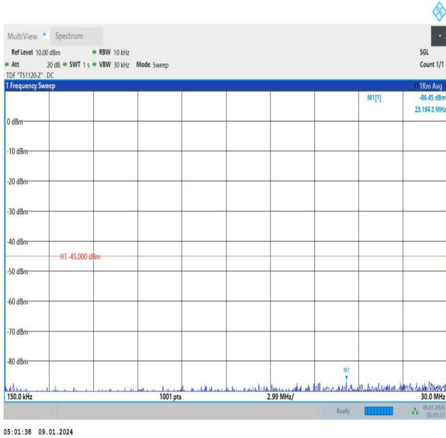
Band41_15MHz_QPSK_40620_1RB#0_0.15~30_0.15~30
