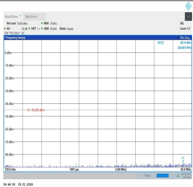
Band41_5MHz_QPSK_40620_25RB#0_0.15~30_0.15~30
