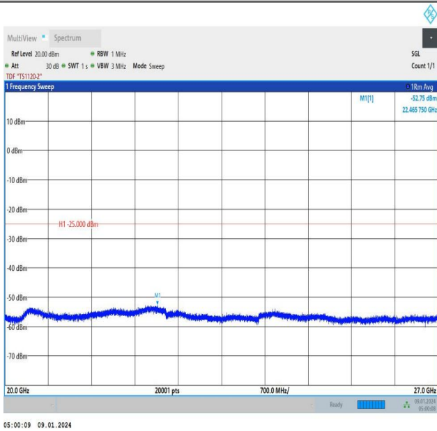
Band41_15MHz_16QAM_39725_1RB#0_20000~27000_2000~27000
