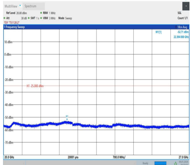
Band41_10MHz_QPSK_40620_50RB#0_20000~27000_20000~27000
