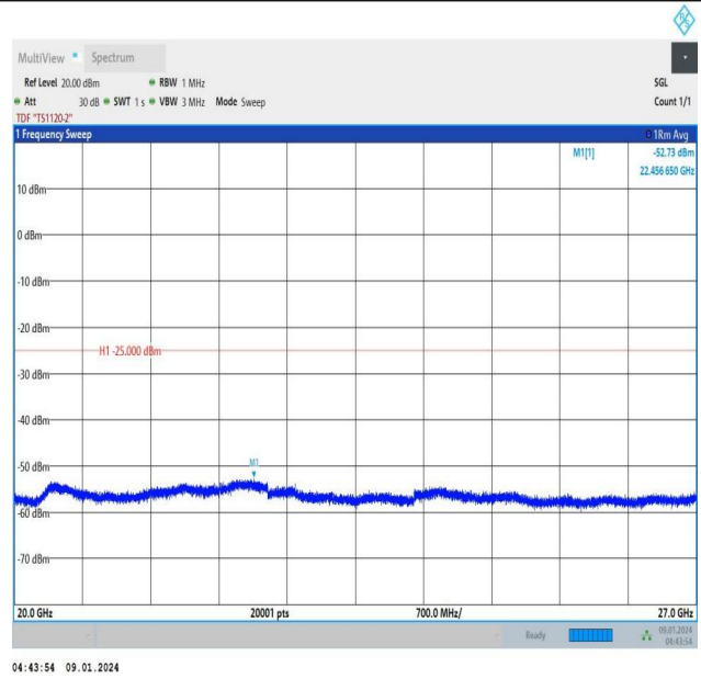
Band41_5MHz_16QAM_40620_1RB#24_20000~27000_20000~27000
