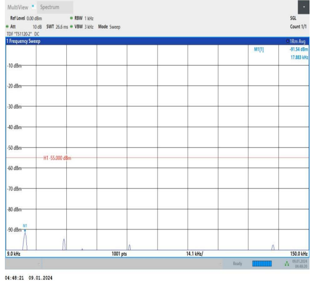
Band41_5MHz_16QAM_41565_25RB#0_0.009~0.15_0.009~0.15
