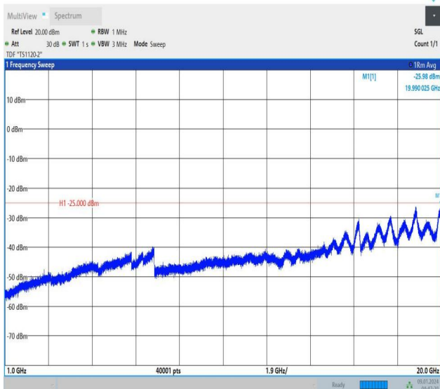
Band41_5MHz_16QAM_41565_1RB#24_1000~20000_1000~20000
