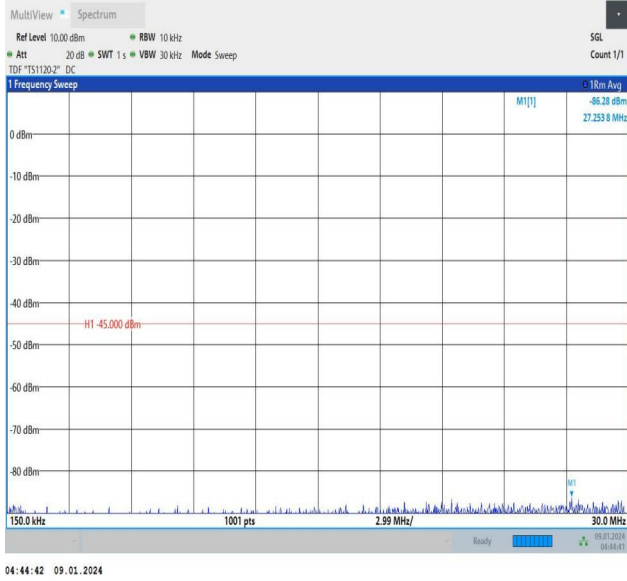
Band41_5MHz_16QAM_40620_25RB#0_0.15~30_0.15~30
