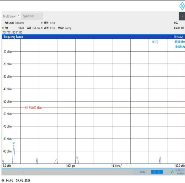
Band41_5MHz_QPSK_40620_25RB#0_0.009~0.15_0.009~0.15
