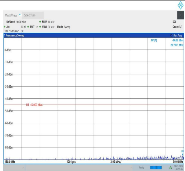
Band41_10MHz_16QAM_39700_1RB#49_20000~27000_20000~27000
