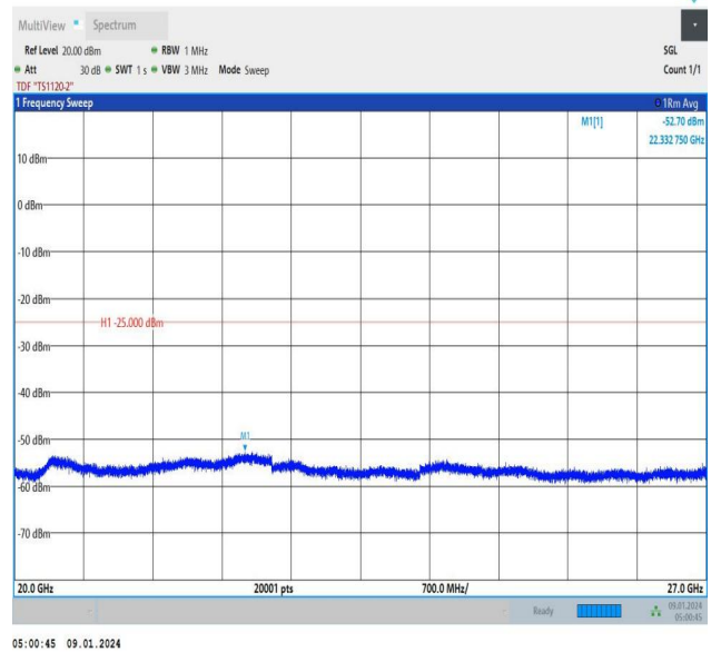
Band41_15MHz_QPSK_39725_1RB#74_20000~27000_2000~27000
