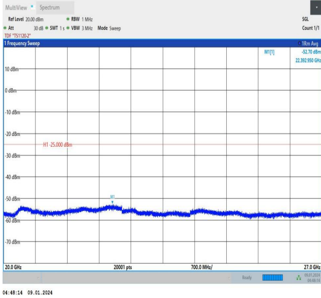
Band41_5MHz_QPSK_41565_25RB#0_20000~27000_20000~27000
