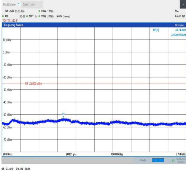
Band41_15MHz_16QAM_39725_1RB#74_20000~27000_20000~27000
