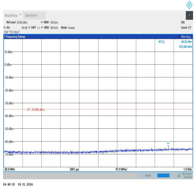
Band41_5MHz_16QAM_41565_25RB#0_30~1000_30~1000
