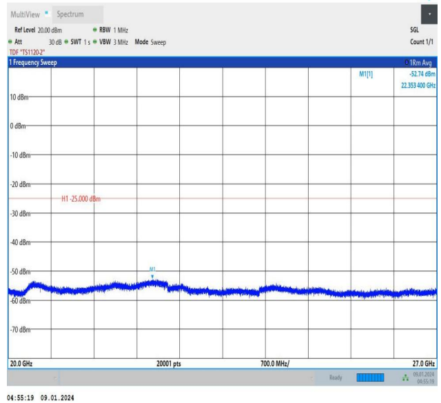
Band41_10MHz_16QAM_41540_1RB#0_20000~27000_20000~27000
