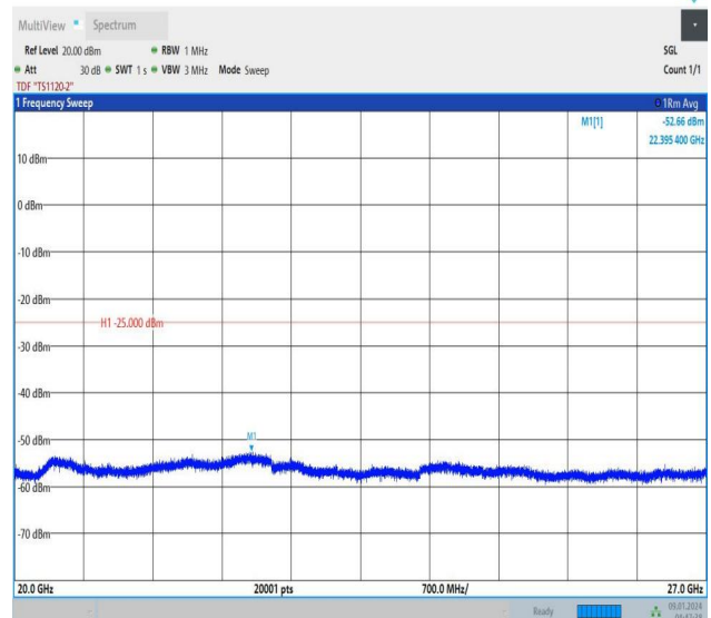
Band41_5MHz_16QAM_41565_1RB#24_20000~27000_20000~27000
