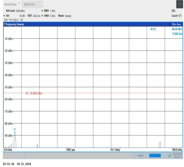
Band41_15MHz_QPSK_40620_1RB#0_0.009~0.15_0.009~0.15
