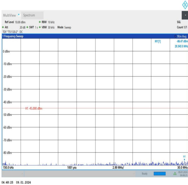
Band41_5MHz_16QAM_41565_25RB#0_0.15~30_0.15~30
