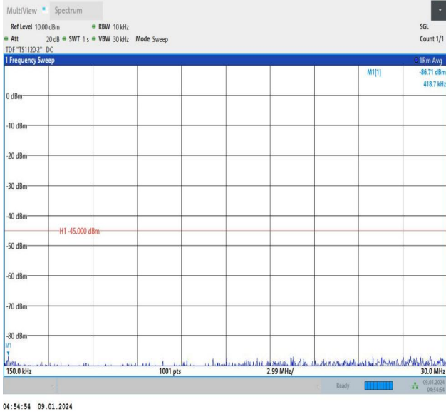
Band41_10MHz_16QAM_41540_1RB#0_0.15~30_0.15~30
