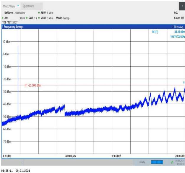
Band41_10MHz_16QAM_41540_1RB#0_1000~20000_1000~20000
