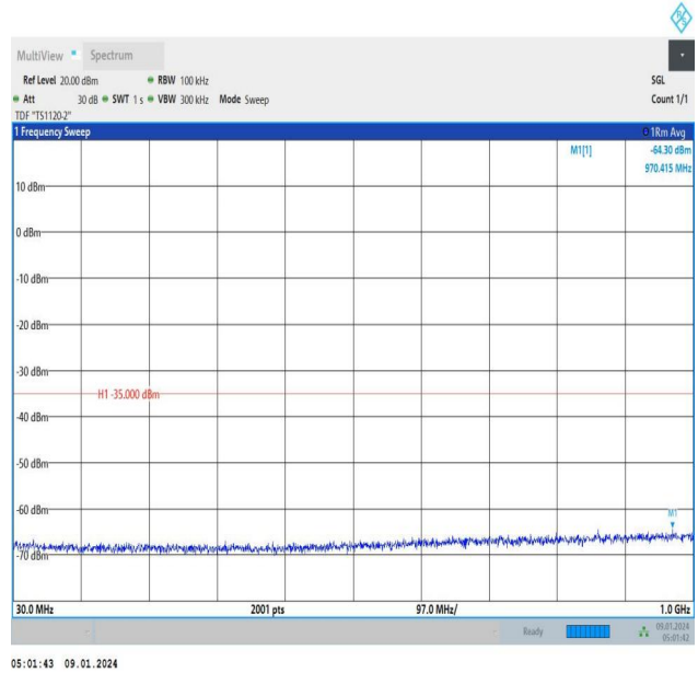
Band41_15MHz_QPSK_40620_1RB#0_30~1000_30~1000
