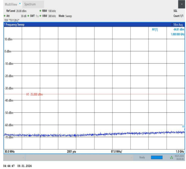
Band41_5MHz_16QAM_40620_25RB#0_30~1000_30~1000
