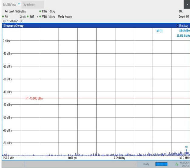
Band41_10MHz_QPSK_40620_50RB#0_0.15~30_0.15~30
