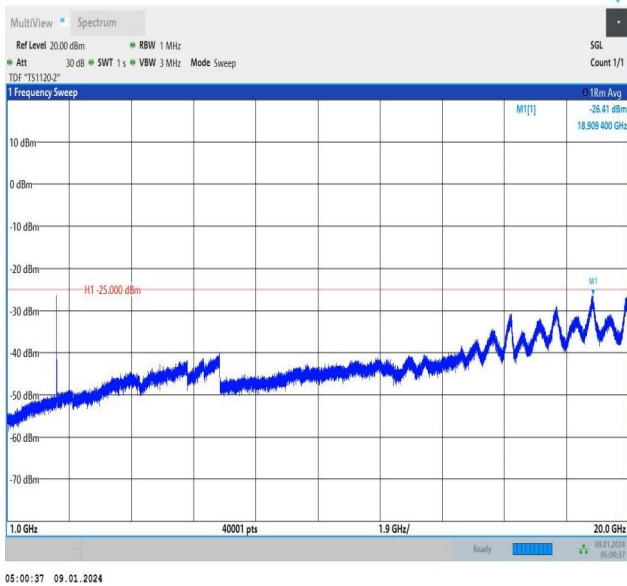
Band41_15MHz_QPSK_39725_1RB#74_1000~20000_1000~20000
