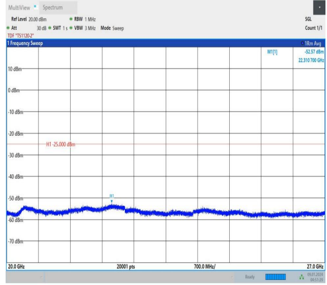
Band41_10MHz_16QAM_39700_1RB#49_20000~27000_20000~27000
