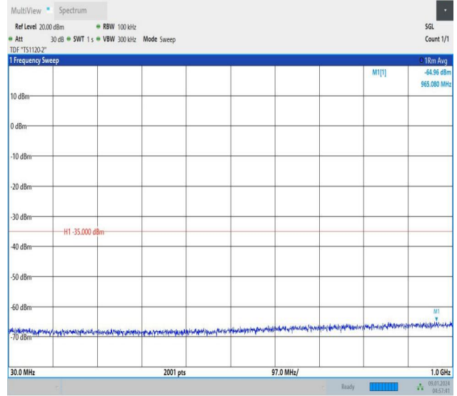
Band41_10MHz_QPSK_40620_50RB#0_30~1000_30~1000
