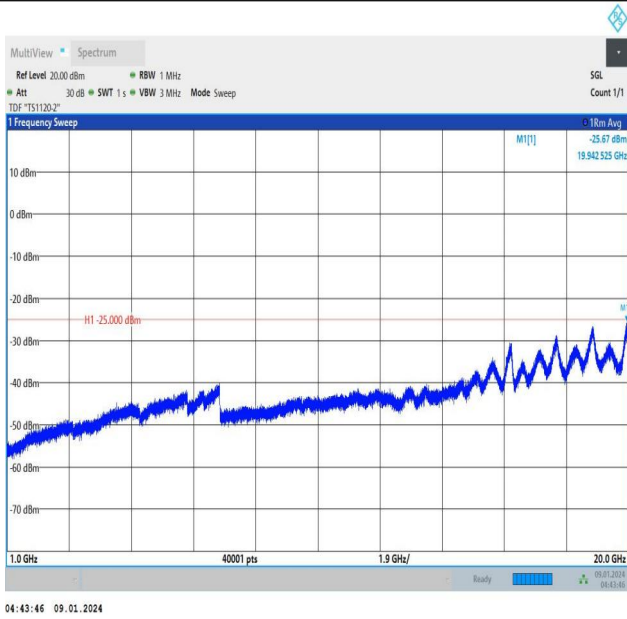
Band41_5MHz_16QAM_40620_1RB#24_1000~20000_1000~20000
