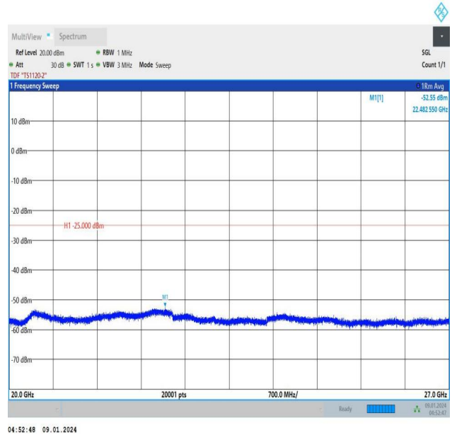
Band41_10MHz_16QAM_40620_1RB#0_20000~27000_20000~27000
