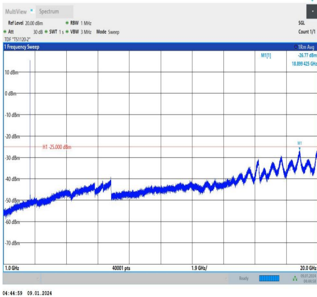
Band41_5MHz_16QAM_40620_25RB#0_1000~20000_1000~20000
