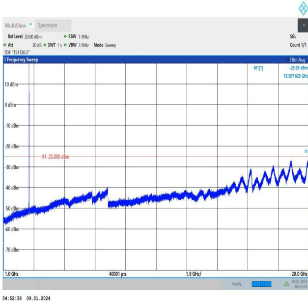
Band41_10MHz_16QAM_40620_1RB#0_1000~20000_1000~20000
