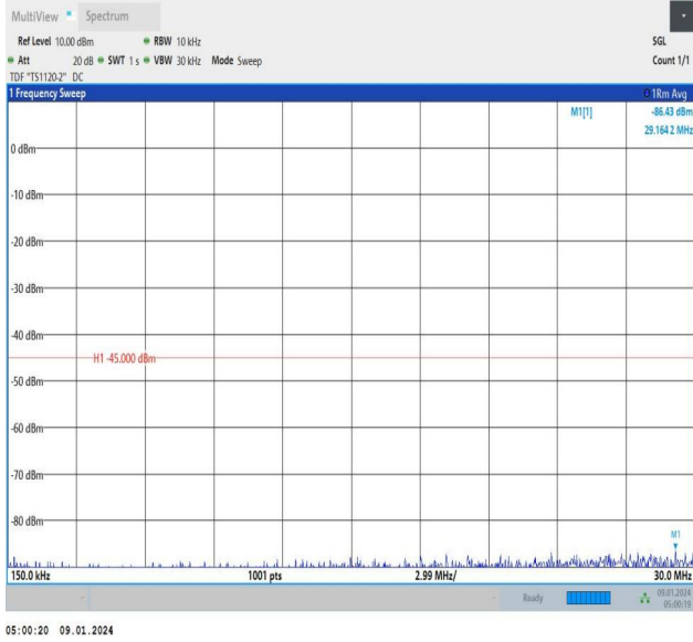
Band41_15MHz_QPSK_39725_1RB#74_0.15~30_0.15~30
