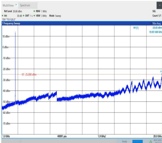
Band41_10MHz_QPSK_40620_50RB#0_1000~20000_1000~20000
