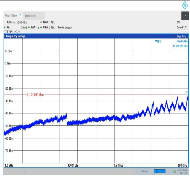
Band41_5MHz_QPSK_40620_1RB#0_1000~20000_1000~20000
