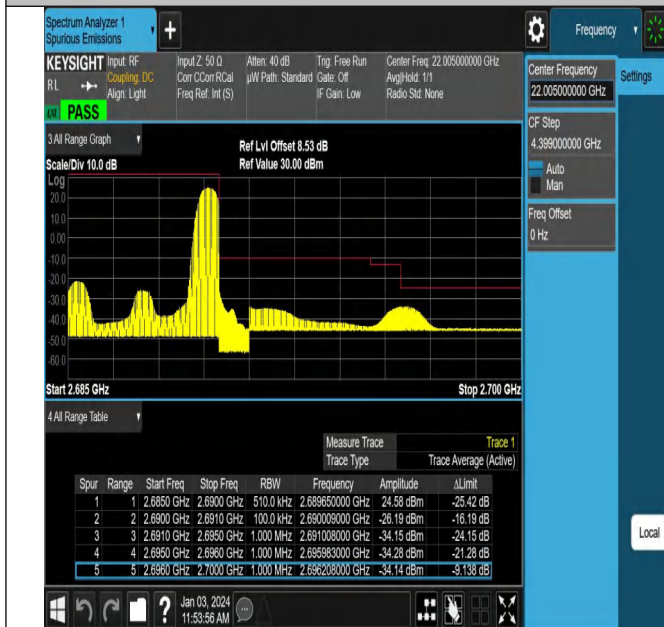
Band41_5MHz_16QAM_41565_1RB#24
