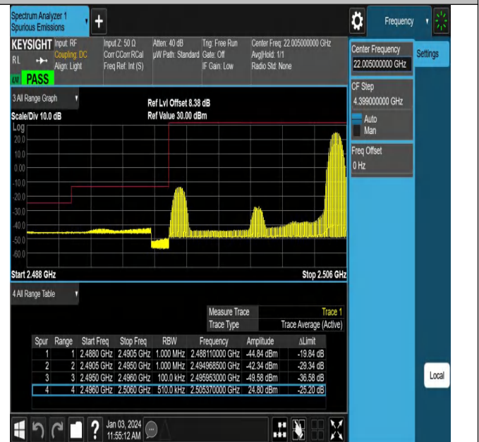
Band41_10MHz_16QAM_39700_1RB#49
