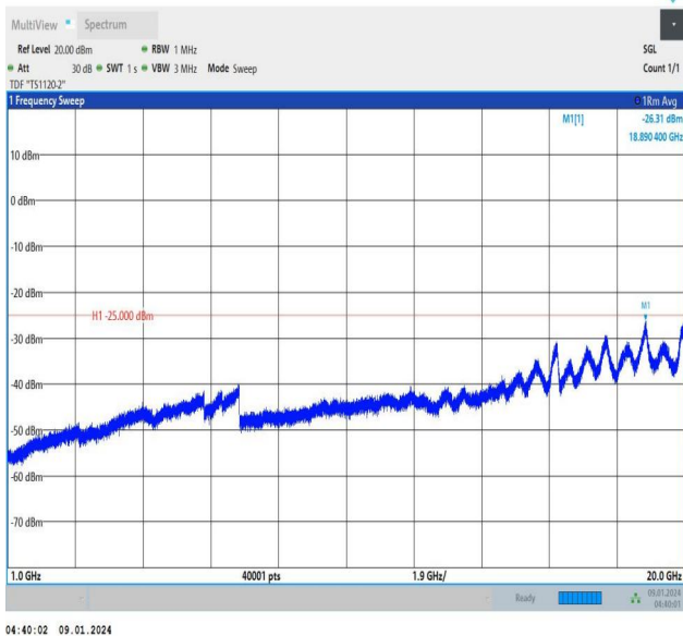
Band41_5MHz_16QAM_39675_1RB#24_1000~20000_1000~20000
