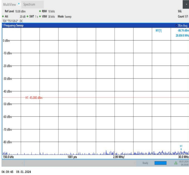
Band41_5MHz_16QAM_39675_1RB#24_0.15~30_0.15~30
