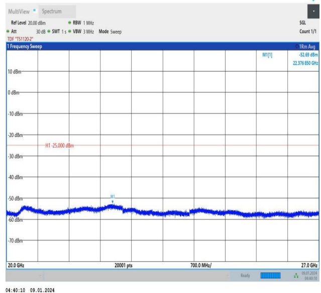
Band41_5MHz_16QAM_39675_1RB#24_20000~27000_20000~27000
