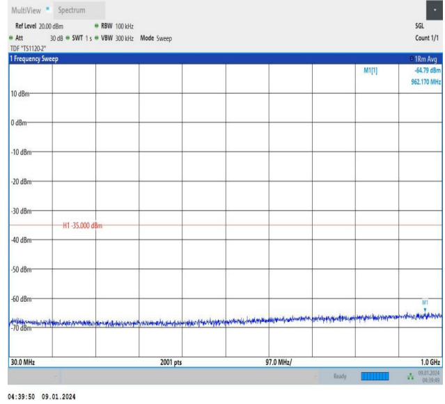
Band41_5MHz_16QAM_39675_1RB#24_30~1000_30~1000
