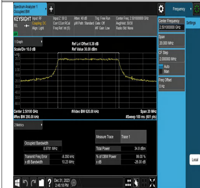
Band41-10MHz-QPSK-39700-50RB#0-PASS
