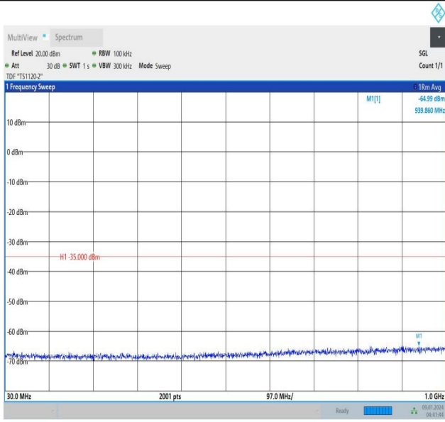
Band41_5MHz_QPSK_40620_1RB#0_30~1000_30~1000
