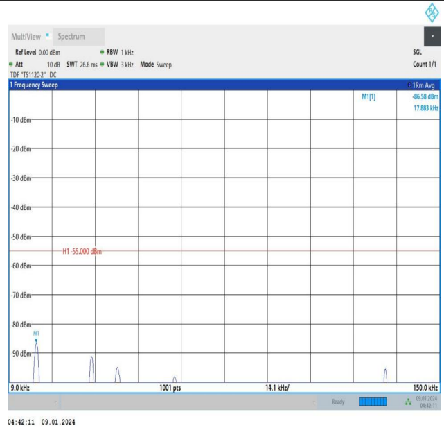
Band41_5MHz_16QAM_40620_1RB#0_0.009~0.15_0.009~0.15
