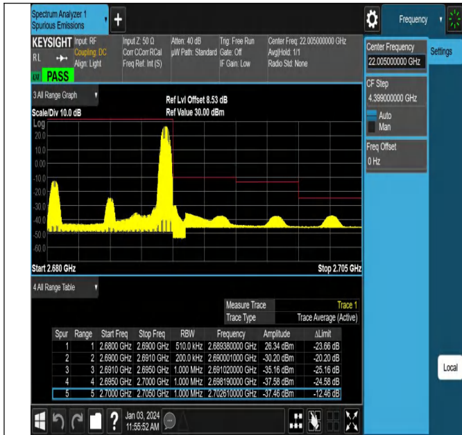
Band41_10MHz_QPSK_41540_1RB#49
