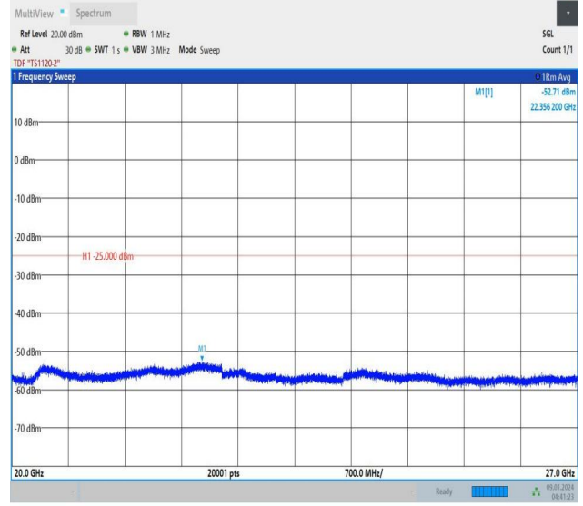
Band41_5MHz_16QAM_39675_25RB#0_20000~27000_20000~27000
