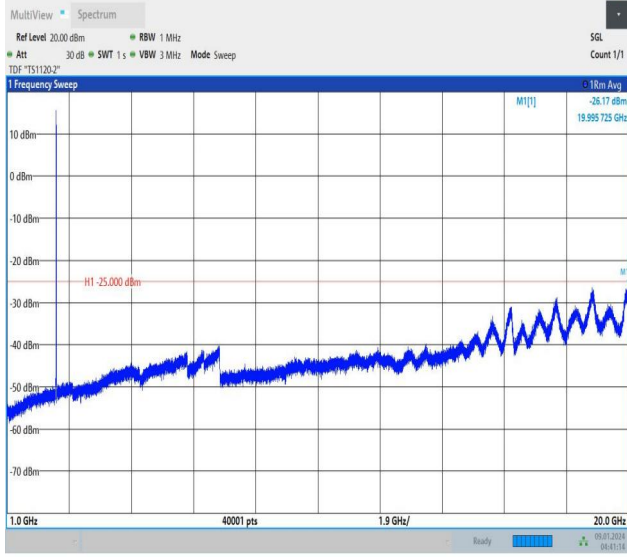
Band41_5MHz_16QAM_39675_25RB#0_1000~20000_1000~20000
