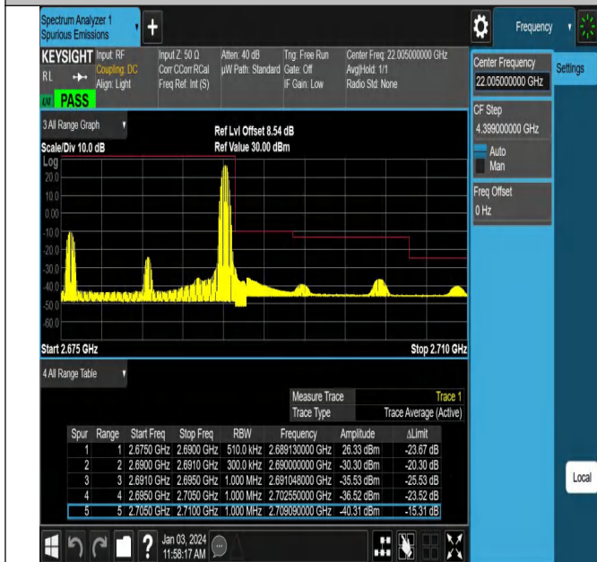
Band41_15MHz_QPSK_41515_1RB#74
