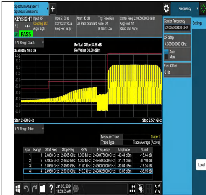
Band41_5MHz_16QAM_39675_25RB#0
