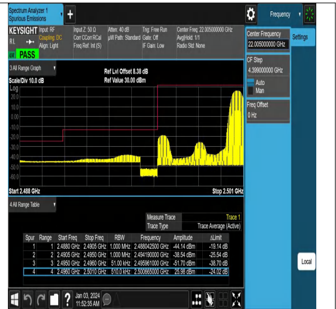
Band41_5MHz_QPSK_39675_1RB#24
