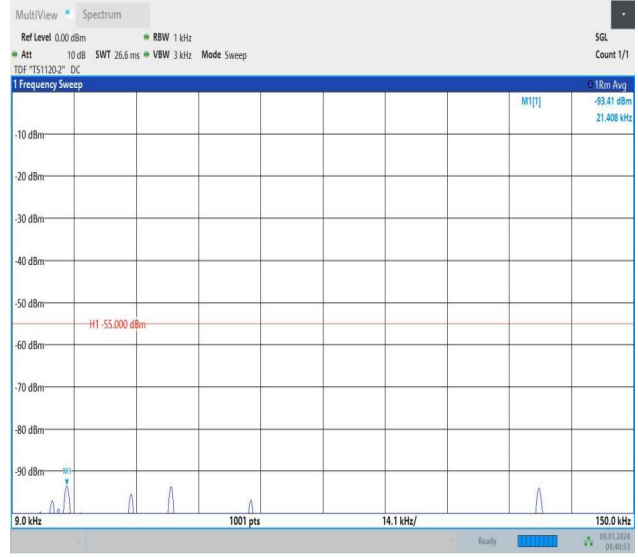
Band41_5MHz_16QAM_39675_25RB#0_0.009~0.15_0.009~0.15
