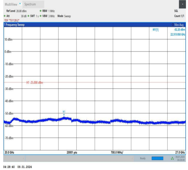
Band38_20MHz_16QAM_37850_1RB#0_20000~27000_2000~27000
