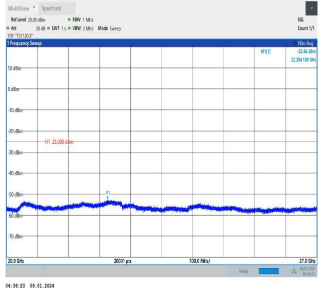
Band38_20MHz_QPSK_38000_100RB#0_20000~27000_20000~27000
