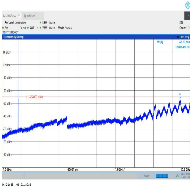
Band38_15MHz_QPSK_38000_1RB#74_1000~20000_1000~20000
