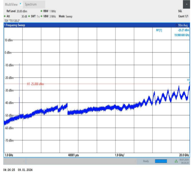
Band38_15MHz_QPSK_38000_75RB#0_1000~20000_1000~20000
