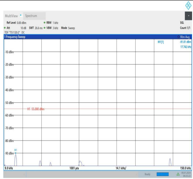
Band38_15MHz_QPSK_37825_75RB#0_0.009~0.15_0.009~0.15
