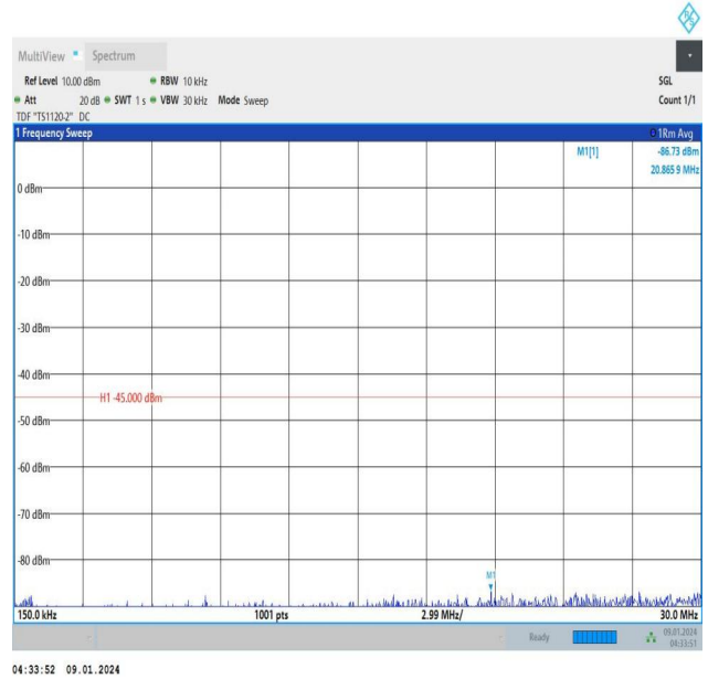
Band38_20MHz_QPSK_38150_1RB#99_0.15~30_0.15~30
