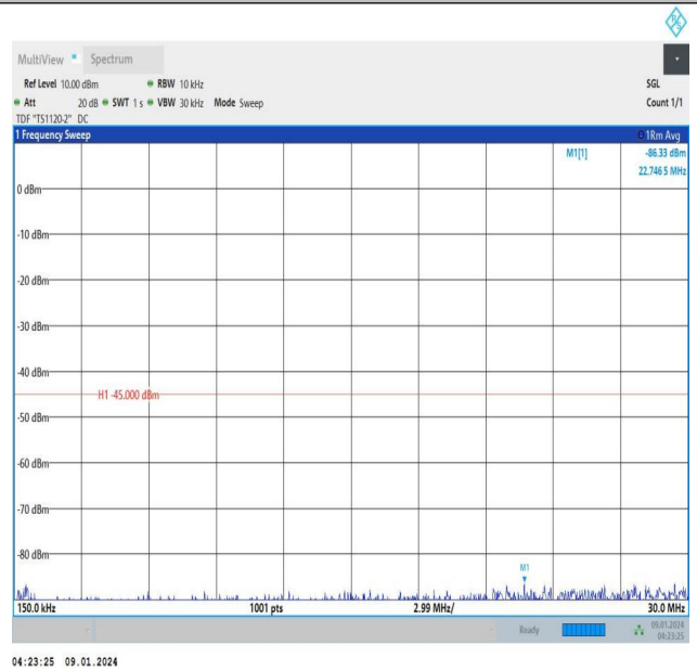
Band38_15MHz_16QAM_38175_1RB#0_0.15~30_0.15~30
