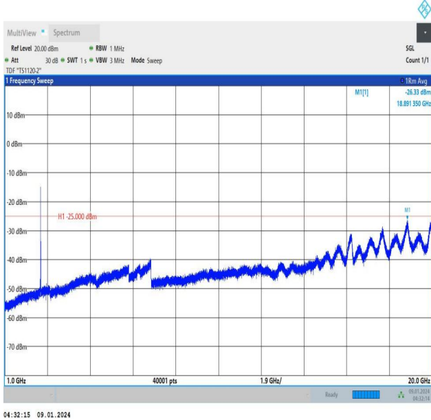
Band38_20MHz_16QAM_38000_1RB#99_1000~20000_1000~20000
