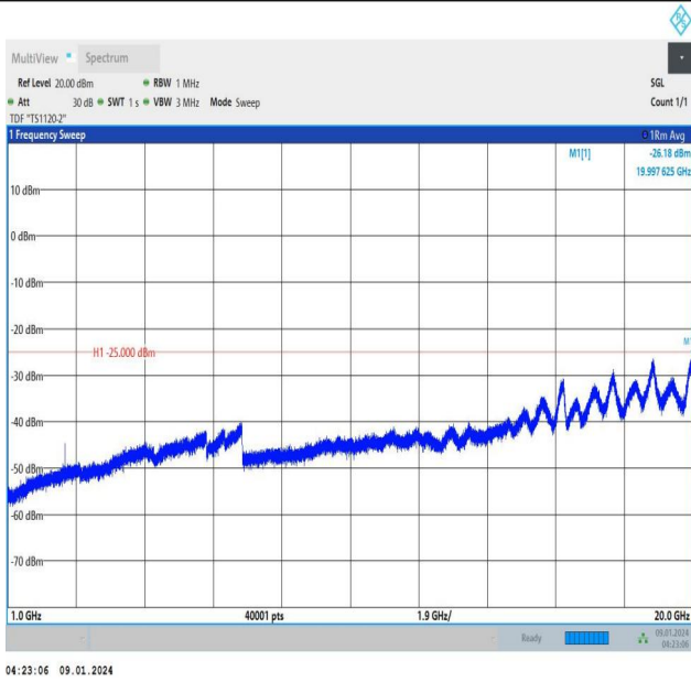
Band38_15MHz_QPSK_38175_1RB#0_1000~20000_1000~20000
