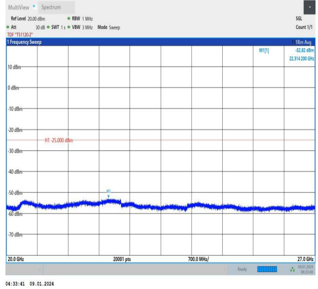
Band38_20MHz_16QAM_38150_1RB#0_20000~27000_20000~27000
