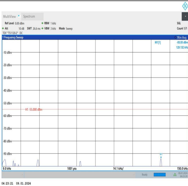
Band38_15MHz_16QAM_38175_1RB#0_0.009~0.15_0.009~0.15
