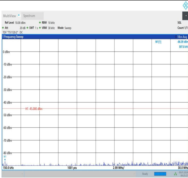
Band38_15MHz_16QAM_38175_1RB#74_20000~27000_20000~27000
