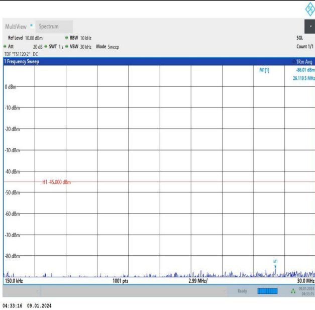
Band38_20MHz_16QAM_38150_1RB#0_0.15~30_0.15~30
