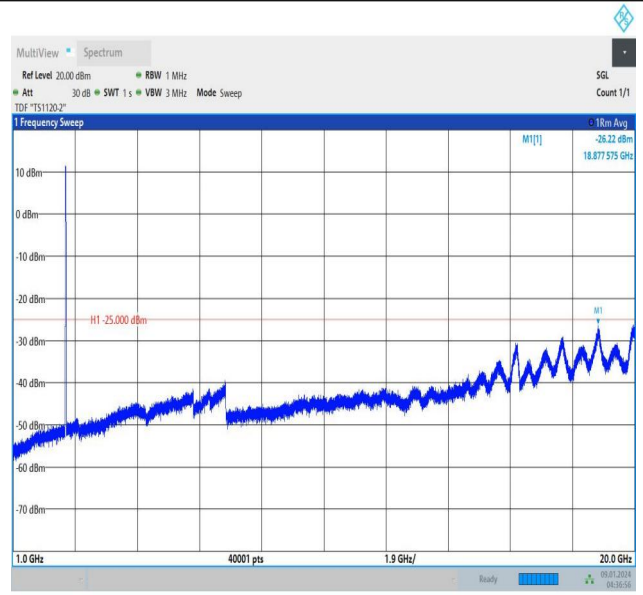
Band38_20MHz_QPSK_38150_100RB#0_1000~20000_1000~20000
