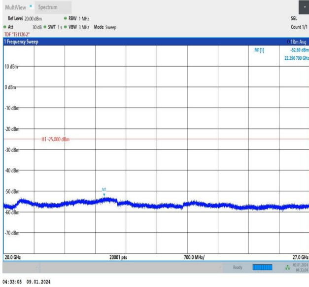
Band38_20MHz_QPSK_38150_1RB#0_20000~27000_20000~27000
