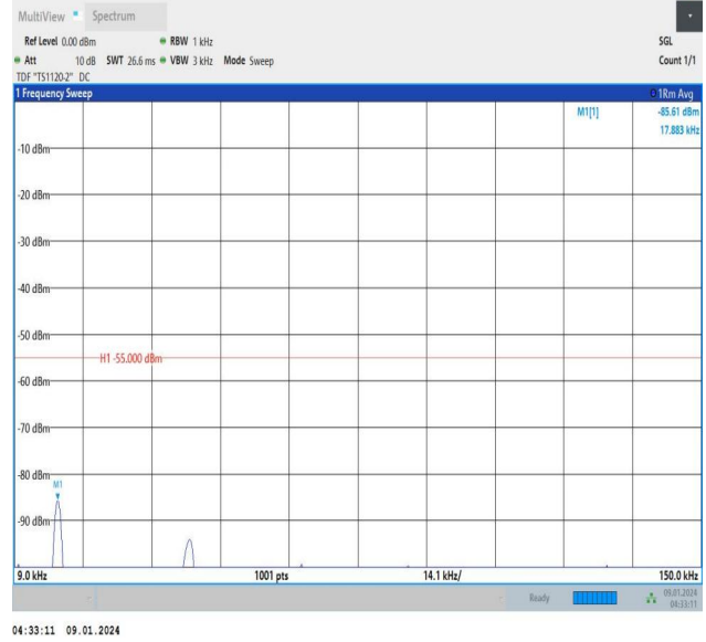
Band38_20MHz_16QAM_38150_1RB#0_0.009~0.15_0.009~0.15
