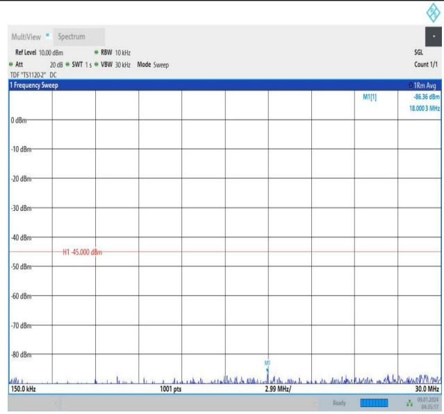
Band38_20MHz_QPSK_37850_100RB#0_0.15~30_0.15~30
