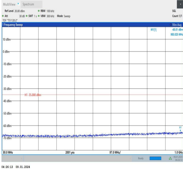
Band38_15MHz_QPSK_38000_75RB#0_30~1000_30~1000
