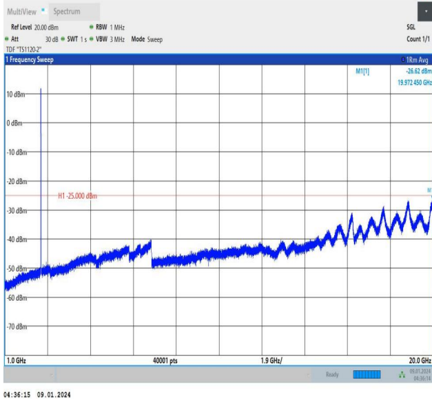
Band38_20MHz_QPSK_38000_100RB#0_1000~20000_1000~20000
