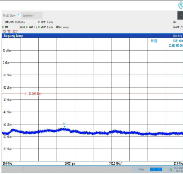
Band38_15MHz_16QAM_38175_1RB#74_20000~27000_20000~27000
