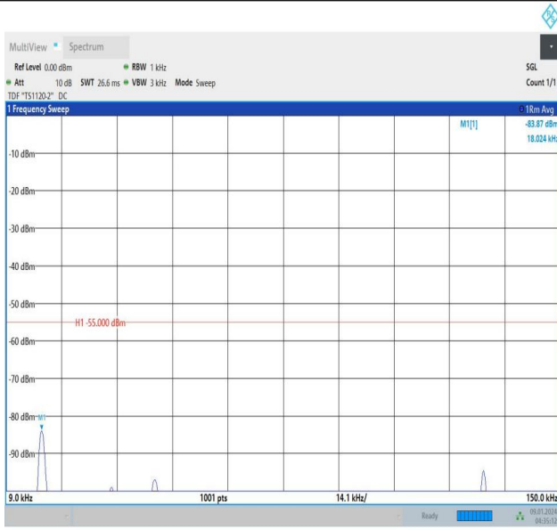
Band38_20MHz_QPSK_37850_100RB#0_0.009~0.15_0.009~0.15
