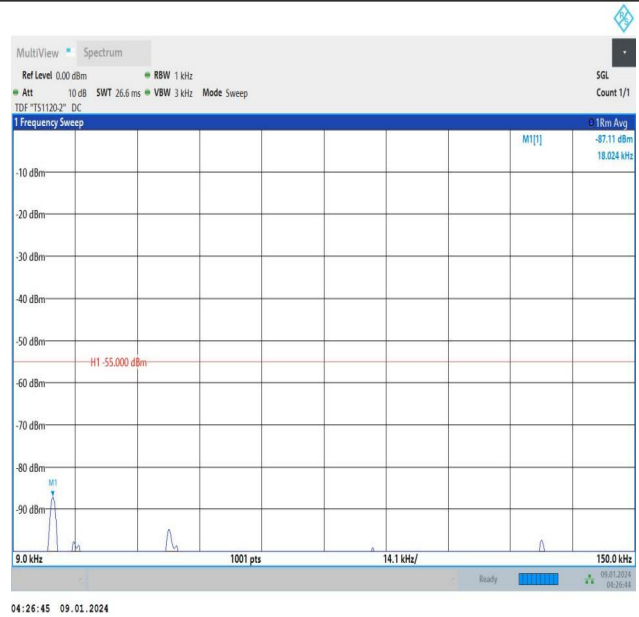
Band38_15MHz_QPSK_38175_75RB#0_0.009~0.15_0.009~0.15
