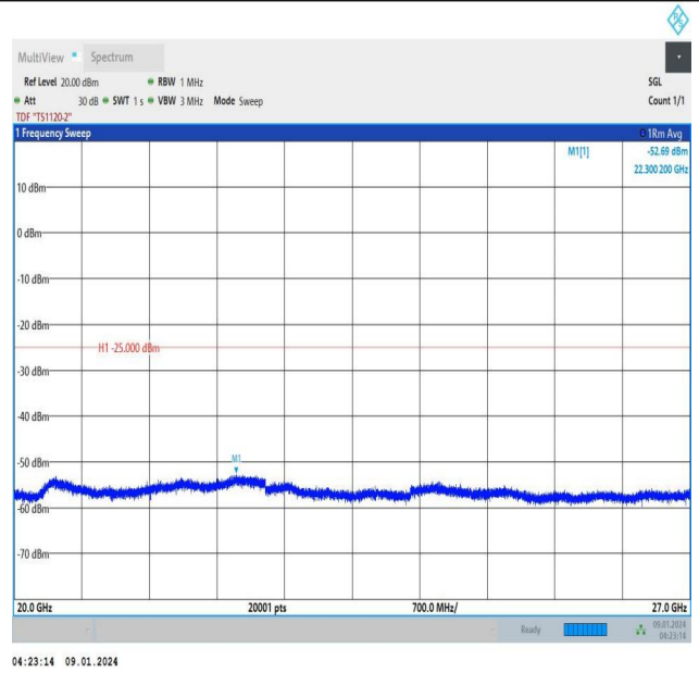
Band38_15MHz_QPSK_38175_1RB#0_20000~27000_20000~27000
