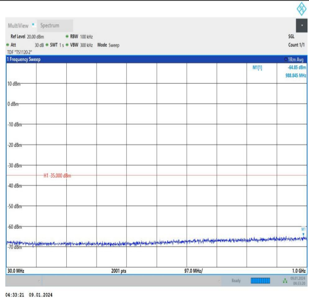
Band38_20MHz_16QAM_38150_1RB#0_30~1000_30~1000
