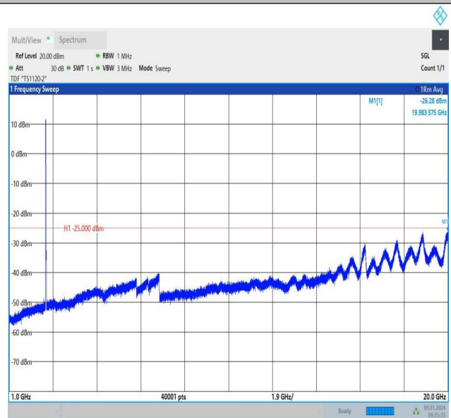
Band38_20MHz_QPSK_37850_100RB#0_1000~20000_1000~20000
