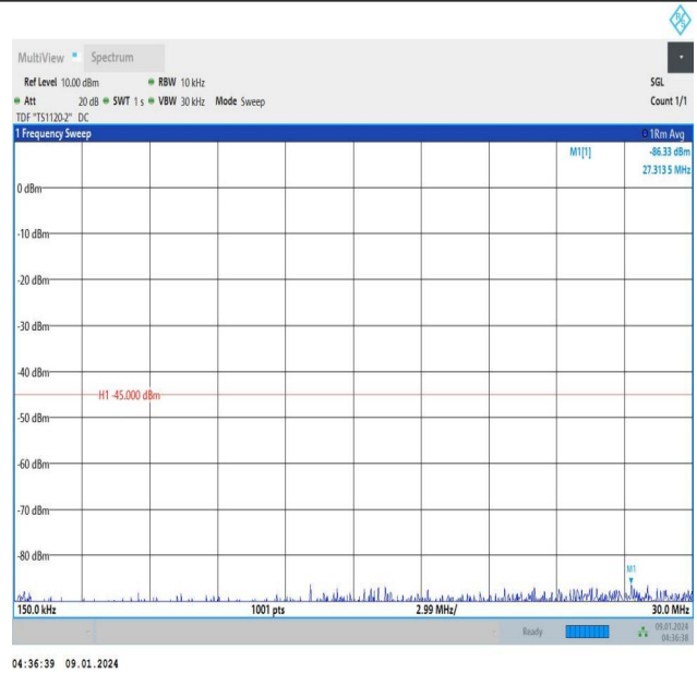
Band38_20MHz_QPSK_38150_100RB#0_0.15~30_0.15~30
