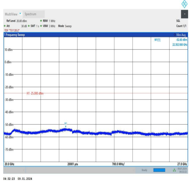
Band38_20MHz_16QAM_38000_1RB#99_20000~27000_20000~27000
