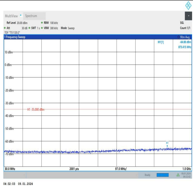
Band38_20MHz_16QAM_38000_1RB#99_30~1000_30~1000
