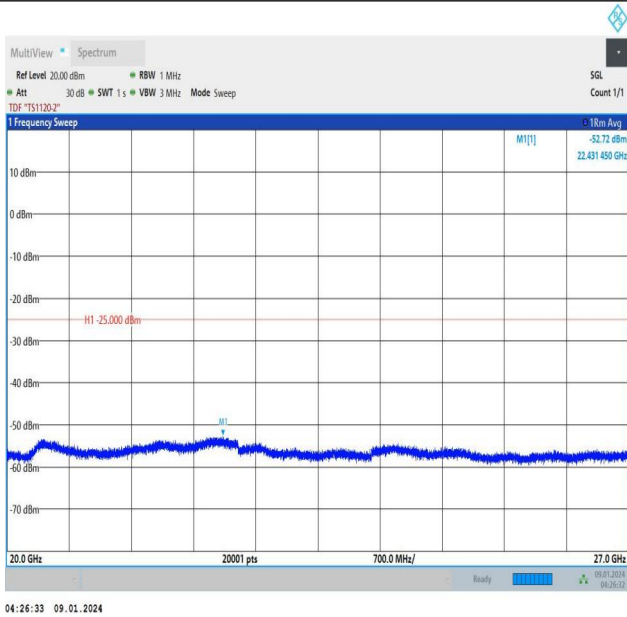
Band38_15MHz_QPSK_38000_75RB#0_20000~27000_20000~27000
