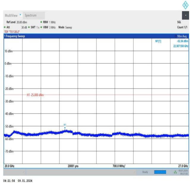
Band38_15MHz_QPSK_38000_1RB#74_20000~27000_20000~27000
