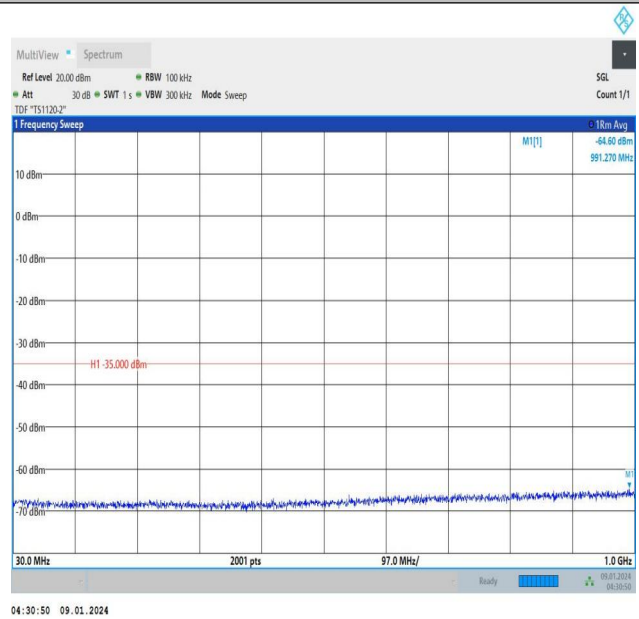
Band38_20MHz_16QAM_38000_1RB#0_30~1000_30~1000
