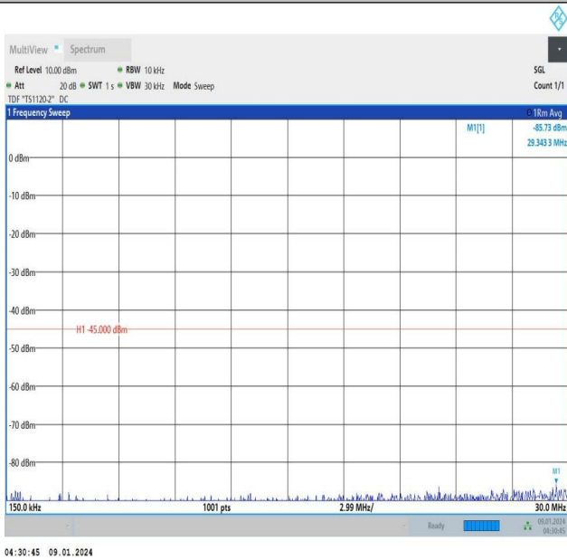
Band38_20MHz_16QAM_38000_1RB#0_0.15~30_0.15~30
