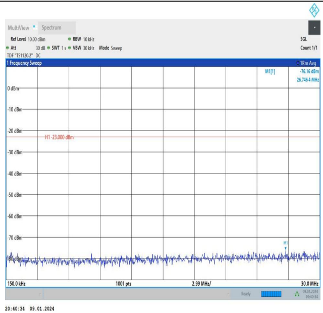
Band26_10MHz_QPSK_26840_1RB#0_0.15~30_0.15~30
