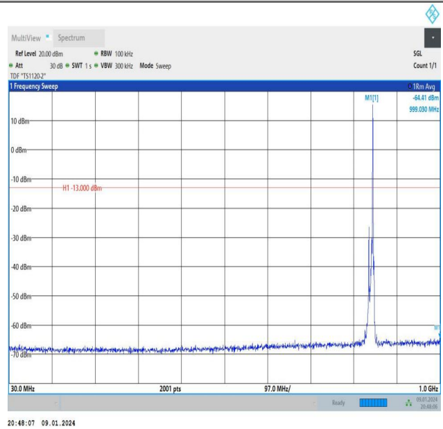
Band26_10MHz_16QAM_26990_1RB#49_30~1000_30~1000
