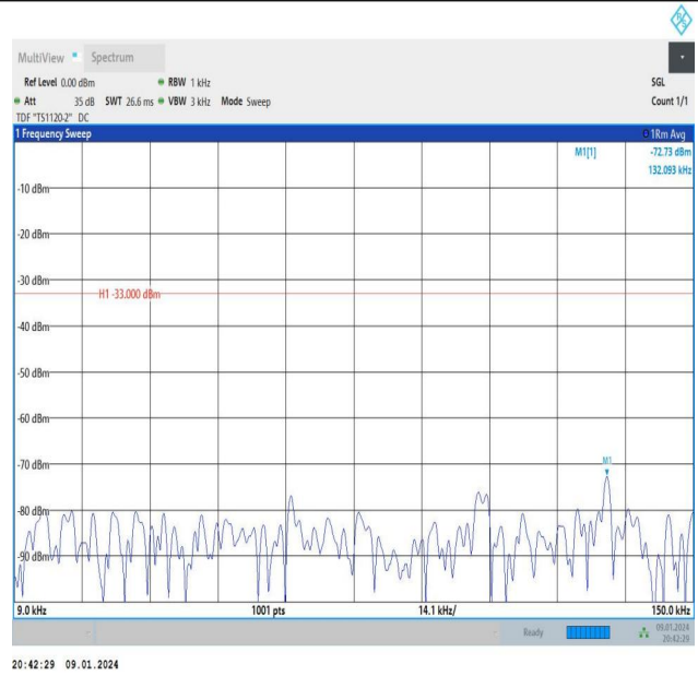
Band26_10MHz_16QAM_26840_1RB#49_0.009~0.15_0.009~0.15
