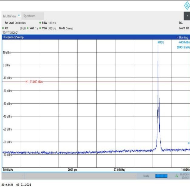
Band26_10MHz_QPSK_26915_1RB#0_30~1000_30~1000
