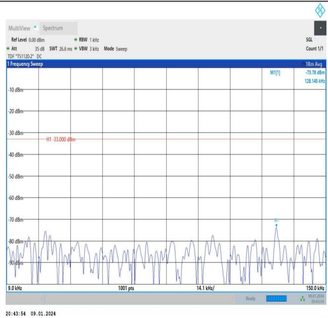
Band26_10MHz_16QAM_26915_1RB#0_0.009~0.15_0.009~0.15
