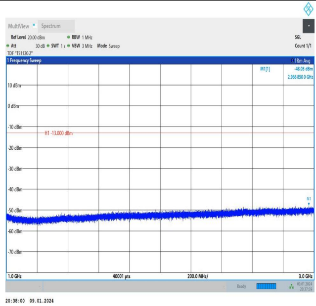
Band26_5MHz_QPSK_27015_1RB#24_1000~3000_1000~3000
