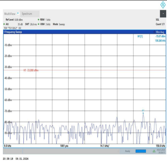
Band26_5MHz_16QAM_27015_1RB#24_0.009~0.15_0.009~0.15
