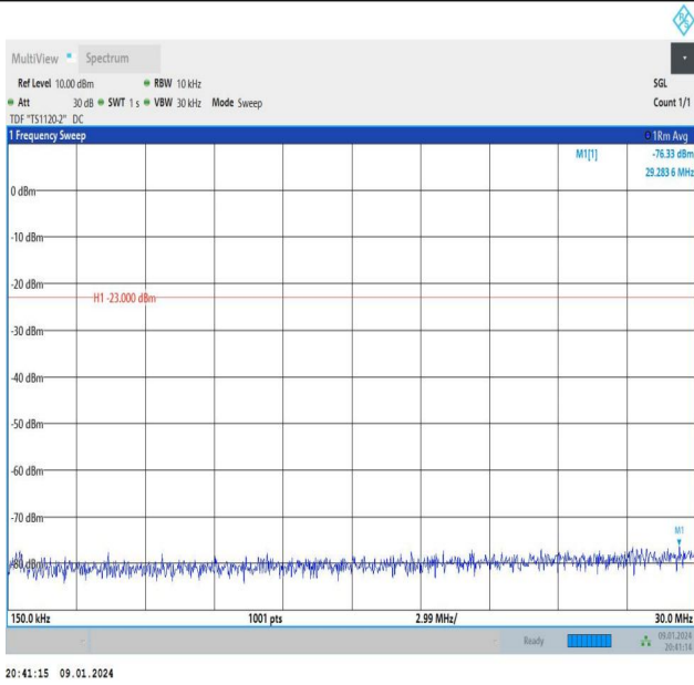
Band26_10MHz_16QAM_26840_1RB#0_0.15~30_0.15~30
