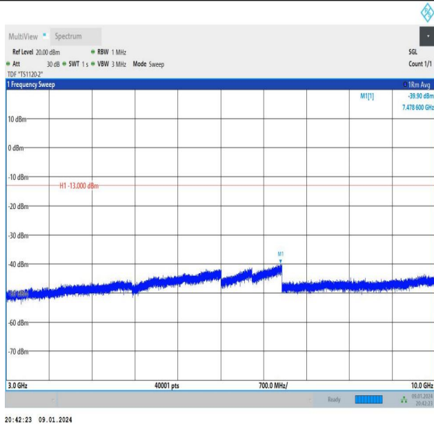
Band26_10MHz_QPSK_26840_1RB#49_3000~10000_3000~10000
