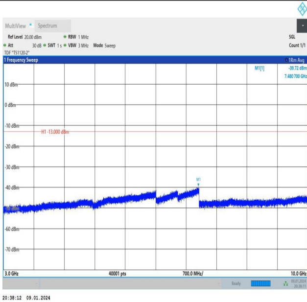
Band26_5MHz_QPSK_27015_1RB#24_3000~10000_3000~10000
