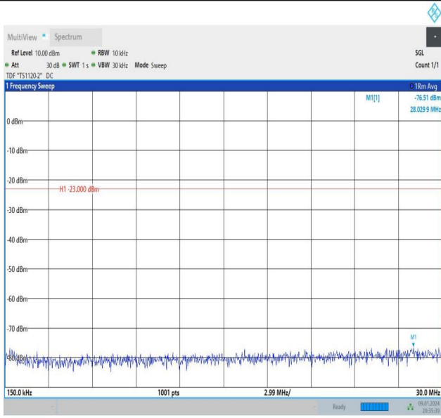
Band26_5MHz_16QAM_26915_25RB#0_0.15~30_0.15~30
