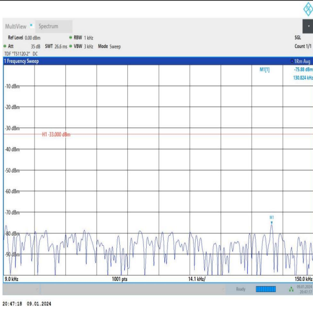
Band26_10MHz_QPSK_26990_1RB#49_0.009~0.15_0.009~0.15
