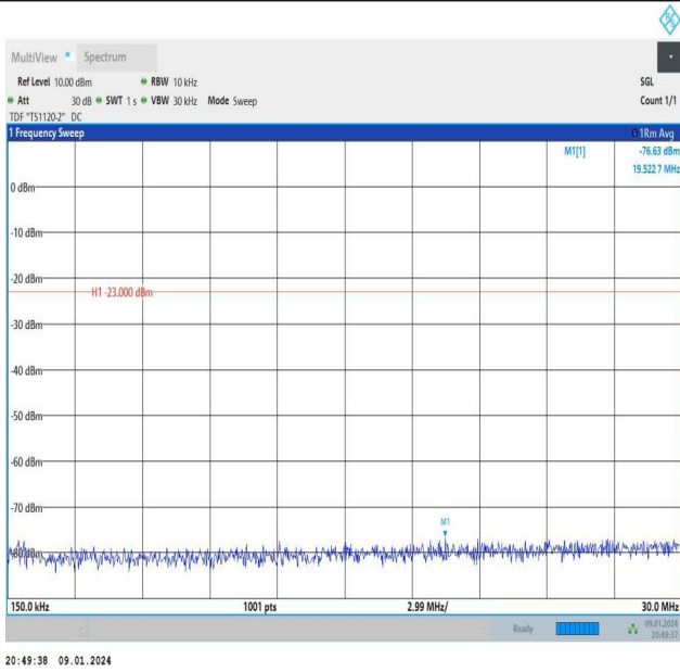
Band26_10MHz_QPSK_26915_50RB#0_0.15~30_0.15~30
