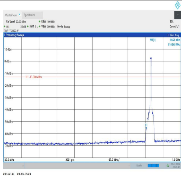
Band26_10MHz_QPSK_26915_50RB#0_30~1000_30~1000
