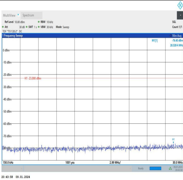
Band26_10MHz_16QAM_26915_1RB#0_0.15~30_0.15~30
