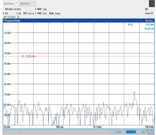
Band26_15MHz_QPSK_26865_1RB#0_0.009~0.15_0.009~0.15
