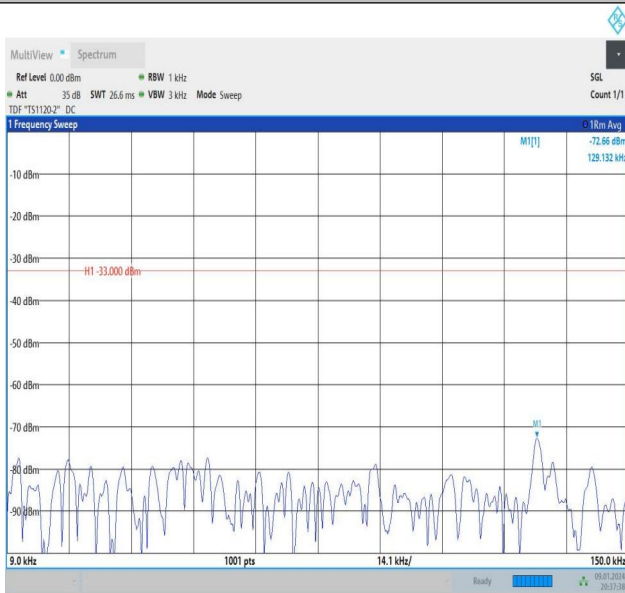
Band26_5MHz_16QAM_27015_1RB#0_1000~3000_1000~3000 00
