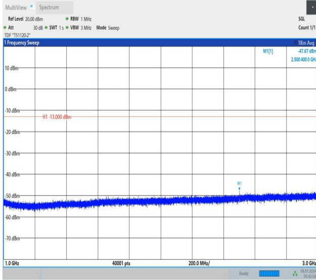
Band26_10MHz_16QAM_26840_1RB#49_1000~3000_1000~3000
