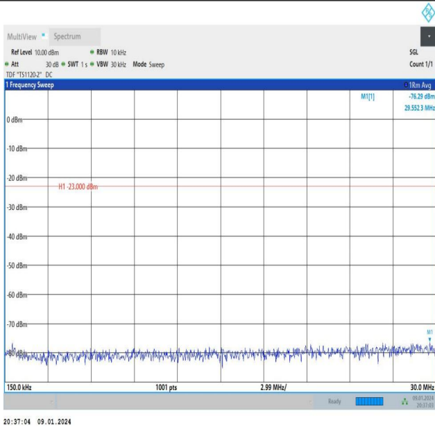
Band26_5MHz_16QAM_27015_1RB#0_0.15~30_0.15~30
