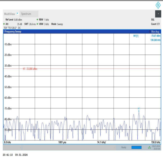
Band26_10MHz_16QAM_26840_1RB#0_0.009~0.15_0.009~0.15
