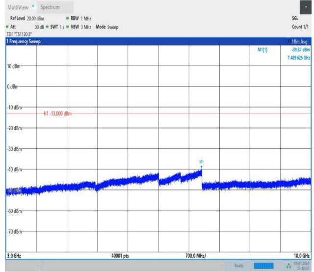
Band26_10MHz_16QAM_26990_1RB#49_3000~10000_3000~10000
