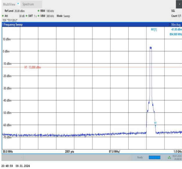
Band26_10MHz_QPSK_26840_50RB#0_30~1000_30~1000
