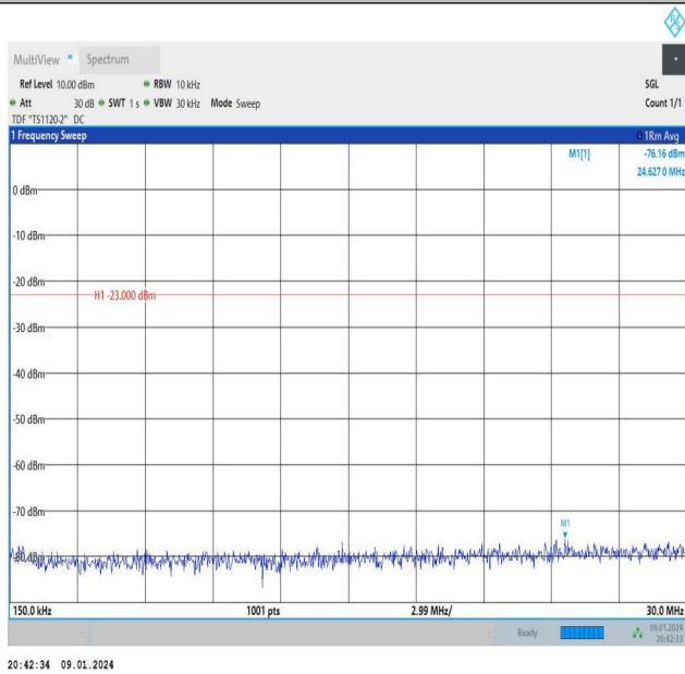
Band26_10MHz_16QAM_26840_1RB#49_0.15~30_0.15~30
