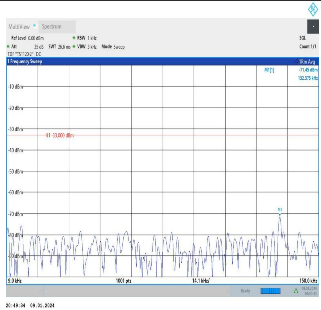
Band26_10MHz_QPSK_26915_50RB#0_0.009~0.15_0.009~0.15
