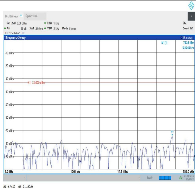
Band26_10MHz_16QAM_26990_1RB#49_0.009~0.15_0.009~0.15
