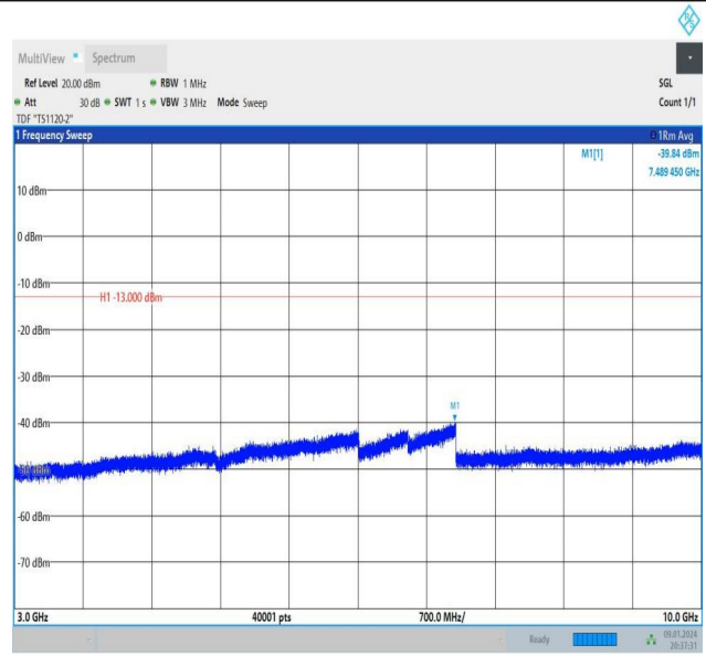
Band26_5MHz_16QAM_27015_1RB#0_3000~10000_3000~10000 0000
