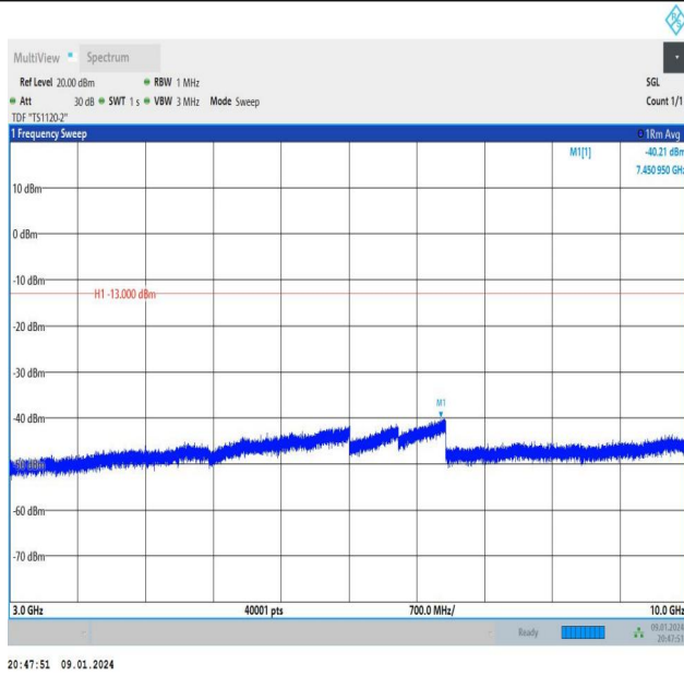
Band26_10MHz_QPSK_26990_1RB#49_3000~10000_3000~10000
