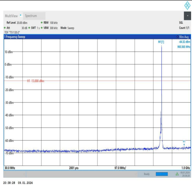
Band26_5MHz_16QAM_27015_1RB#24_30~1000_30~1000
