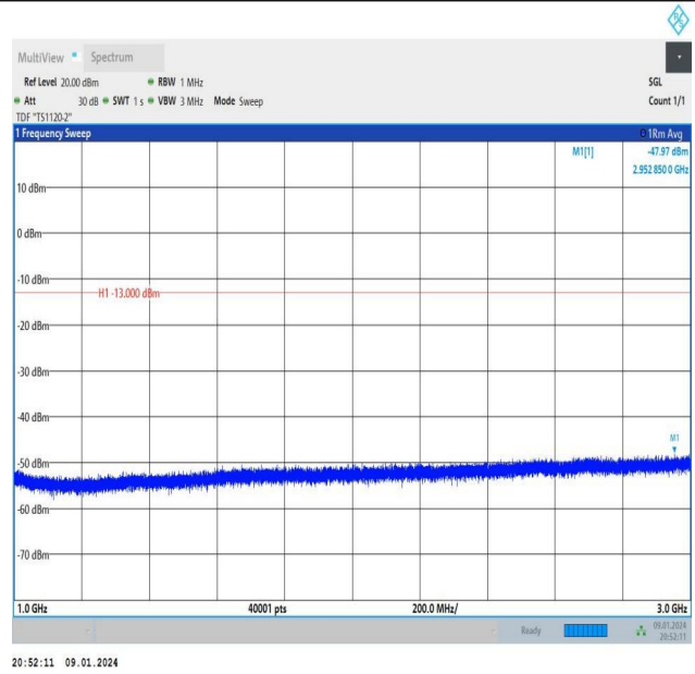
Band26_15MHz_16QAM_26865_1RB#0_1000~3000_1000~3000
