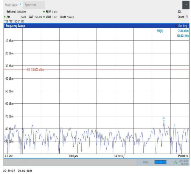
Band26_5MHz_16QAM_27015_25RB#0_0.009~0.15_0.009~0.15
