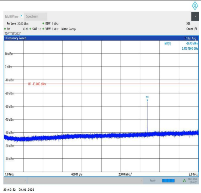
Band26_10MHz_QPSK_26840_1RB#0_1000~3000_1000~3000
