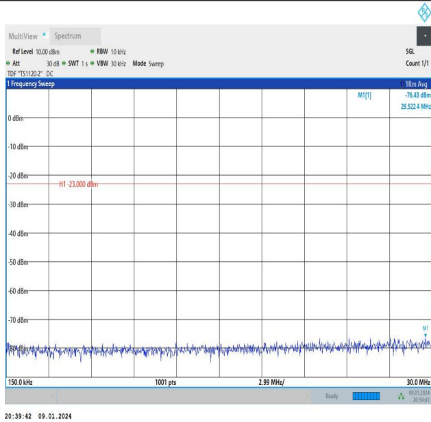
Band26_5MHz_16QAM_27015_25RB#0_0.15~30_0.15~30
