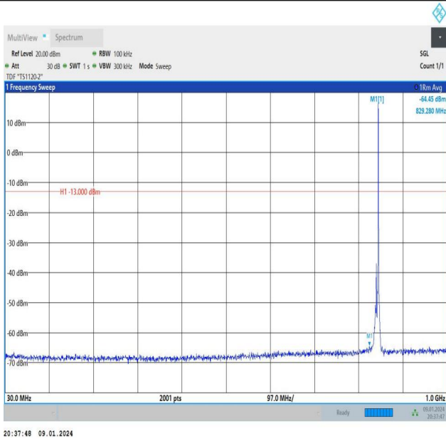
Band26_5MHz_QPSK_27015_1RB#24_30~1000_30~1000
