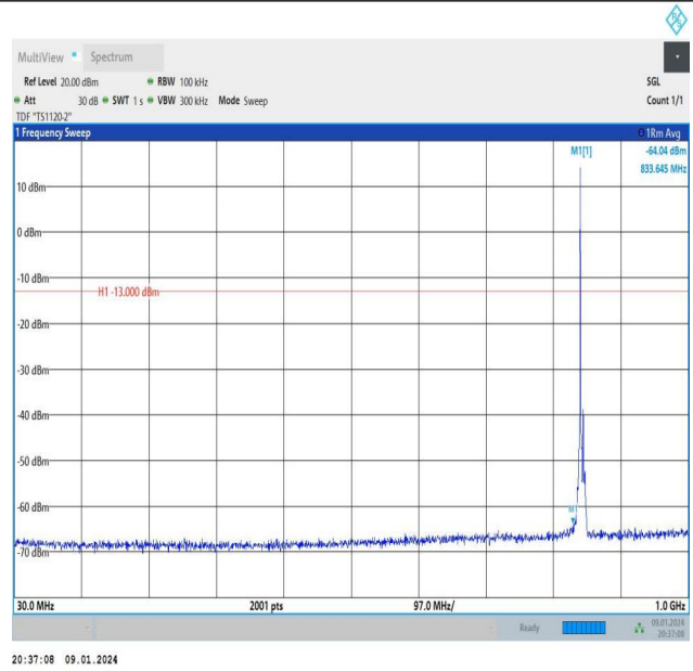
Band26_5MHz_16QAM_27015_1RB#0_30~1000_30~1000
