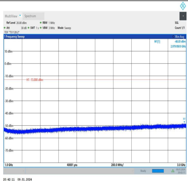
Band26_10MHz_QPSK_26840_1RB#49_1000~3000_1000~3000
