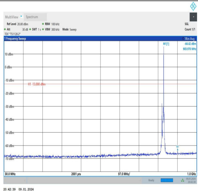
Band26_10MHz_16QAM_26840_1RB#49_30~1000_30~1000
