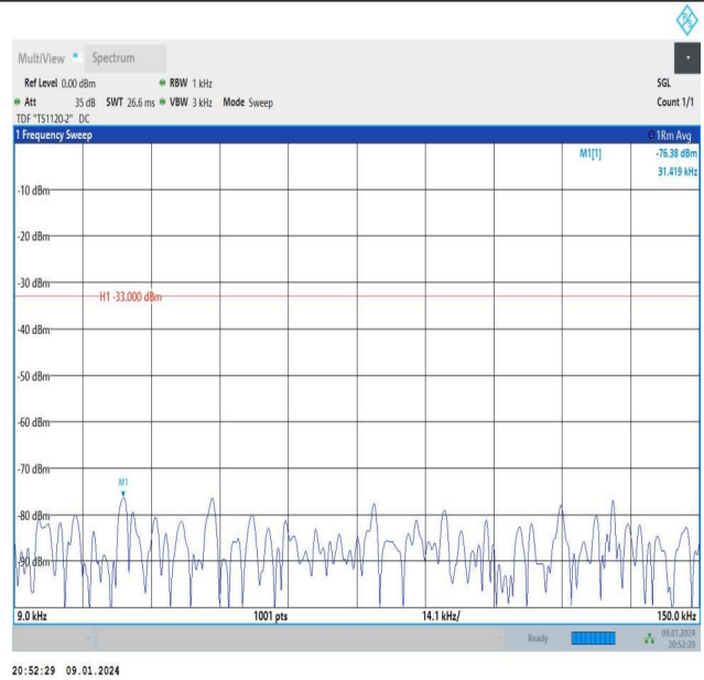
Band26_15MHz_QPSK_26865_1RB#74_0.009~0.15_0.009~0.15
