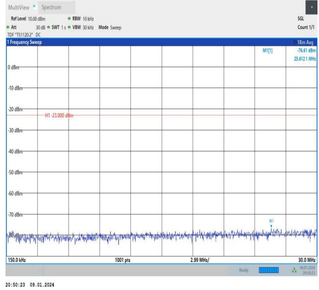
Band26_10MHz_QPSK_26990_50RB#0_0.15~30_0.15~30
