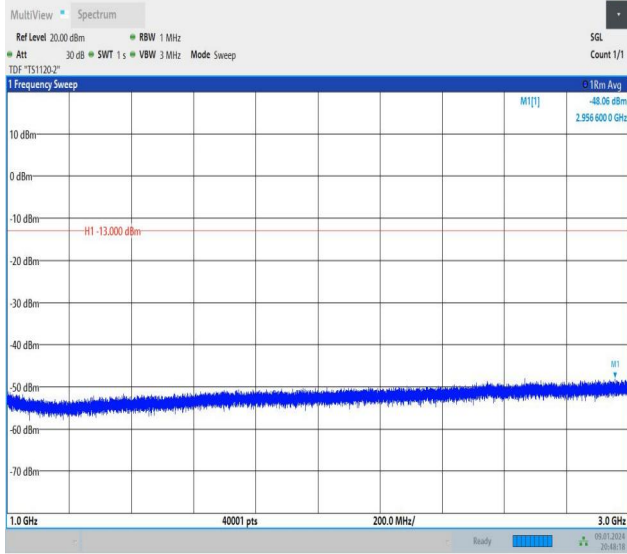
Band26_10MHz_16QAM_26990_1RB#49_1000~3000_1000~3000
