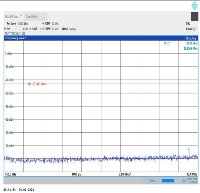
Band26_10MHz_QPSK_26840_1RB#49_0.15~30_0.15~30
