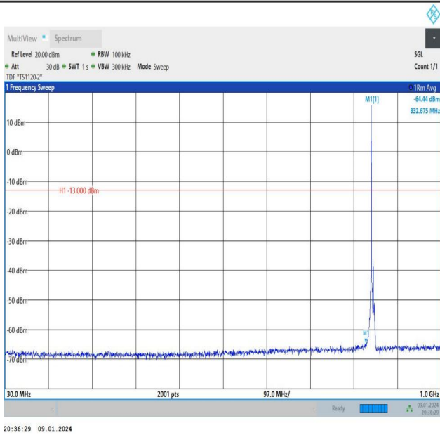
Band26_5MHz_QPSK_27015_1RB#0_30~1000_30~1000
