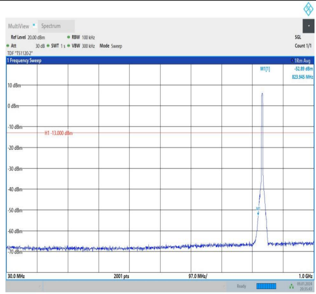
Band26_5MHz_16QAM_26915_25RB#0_30~1000_30~1000
