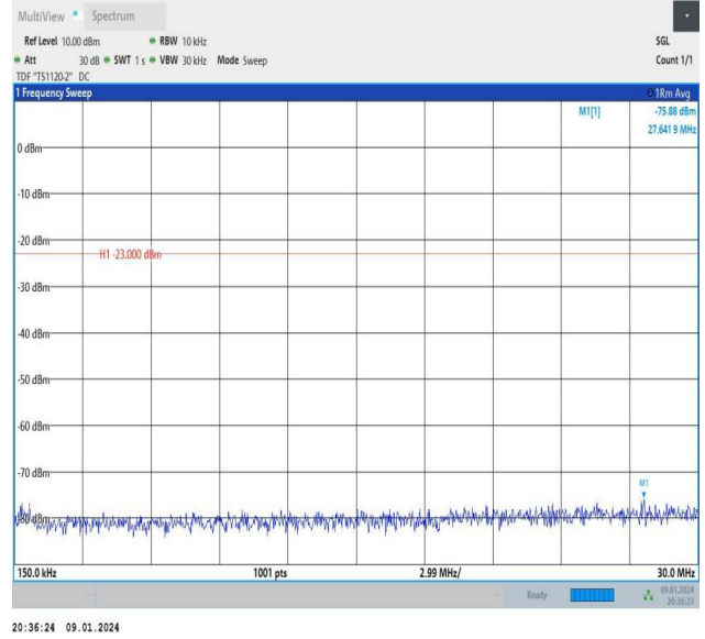
Band26_5MHz_QPSK_27015_1RB#0_0.15~30_0.15~30
