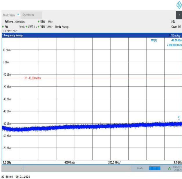
Band26_5MHz_16QAM_27015_1RB#24_1000~3000_1000~3000
