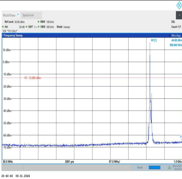
Band26_10MHz_QPSK_26840_1RB#0_30~1000_30~1000
