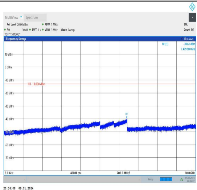
Band26_5MHz_16QAM_26915_25RB#0_3000~10000_3000~10000
