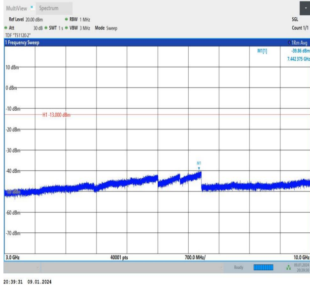
Band26_5MHz_QPSK_27015_25RB#0_3000~10000_3000~10000
