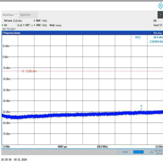
Band26_5MHz_16QAM_26915_25RB#0_1000~3000_1000~3000
