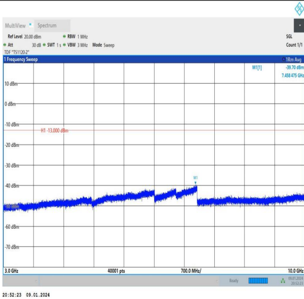
Band26_15MHz_16QAM_26865_1RB#0_3000~10000_3000~10000
