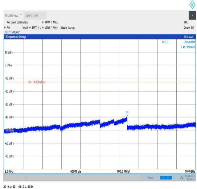
Band26_10MHz_16QAM_26840_1RB#0_3000~10000_3000~10000
