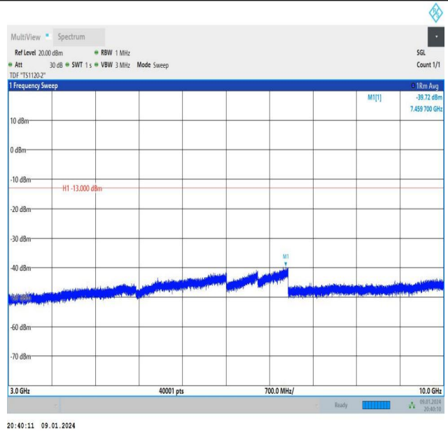
Band26_5MHz_16QAM_27015_25RB#0_3000~10000_3000~10000
