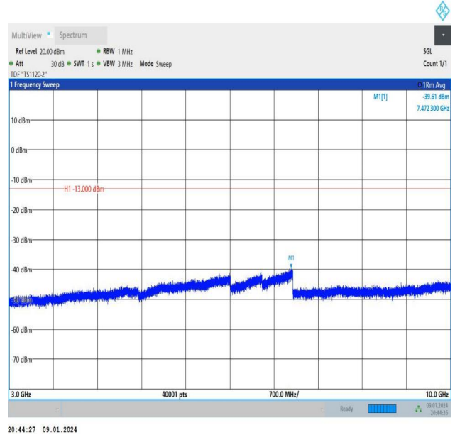
Band26_10MHz_16QAM_26915_1RB#0_3000~10000_3000~10000
