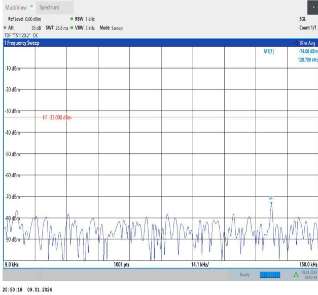
Band26_10MHz_QPSK_26990_50RB#0_0.009~0.15_0.009~0.15
