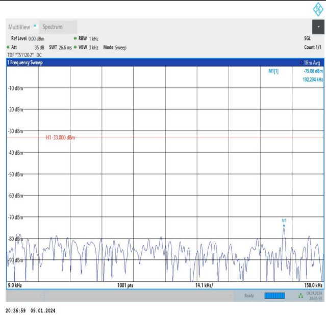
Band26_5MHz_16QAM_27015_1RB#0_0.009~0.15_0.009~0.15
