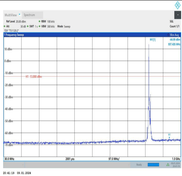
Band26_10MHz_16QAM_26840_1RB#0_30~1000_30~1000
