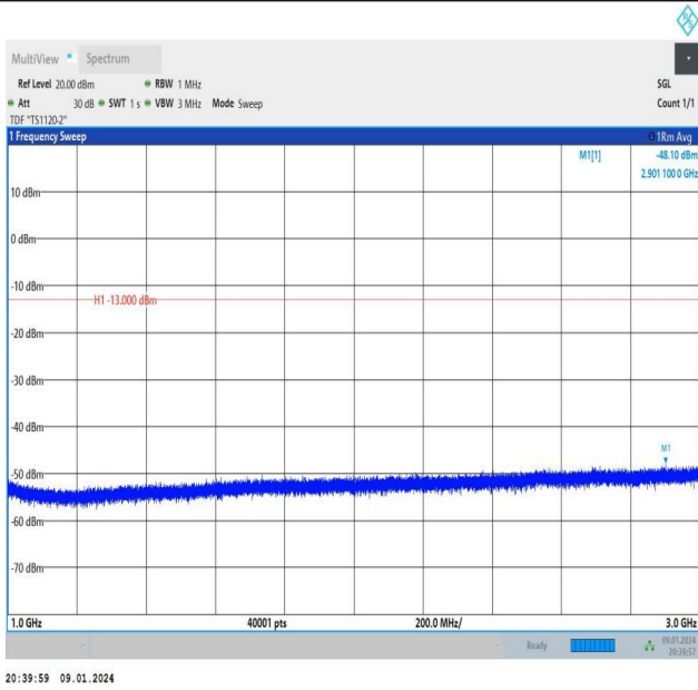
Band26_5MHz_16QAM_27015_25RB#0_1000~3000_1000~3000
