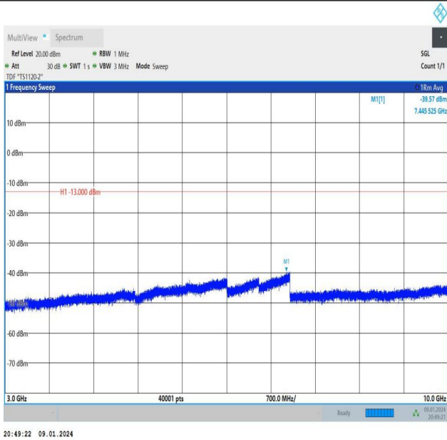
Band26_10MHz_QPSK_26840_50RB#0_3000~10000_3000~10000
