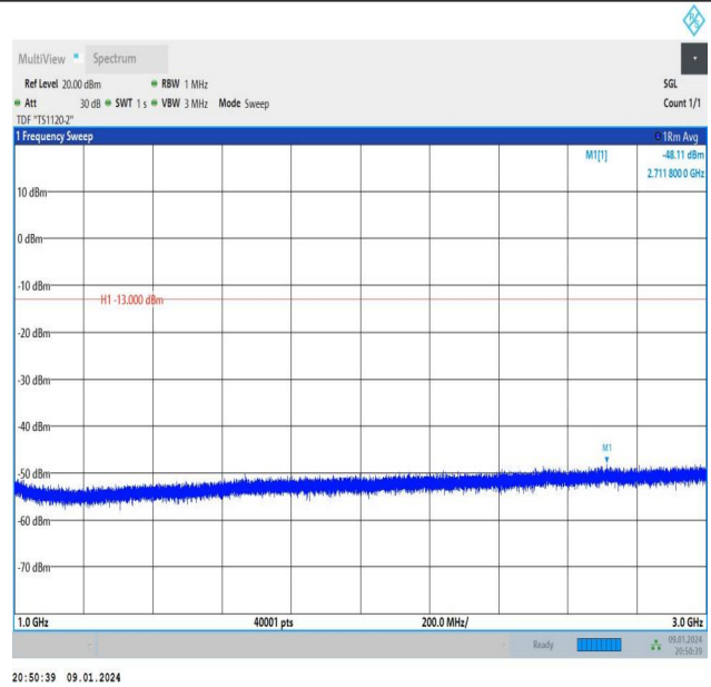
Band26_10MHz_QPSK_26990_50RB#0_1000~3000_1000~3000
