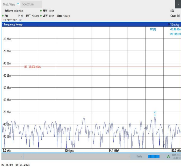
Band26_5MHz_QPSK_27015_1RB#0_0.009~0.15_0.009~0.1
