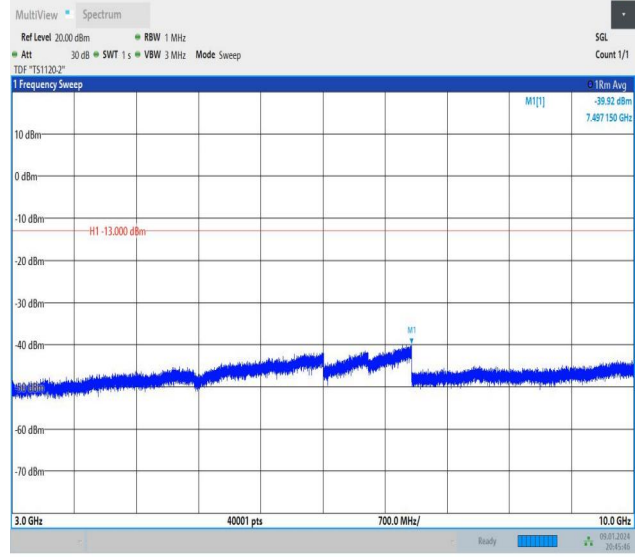
Band26_10MHz_16QAM_26915_1RB#49_3000~10000_3000~10000
