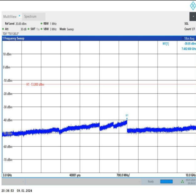
Band26_5MHz_QPSK_27015_1RB#0_3000~10000_3000~10000
