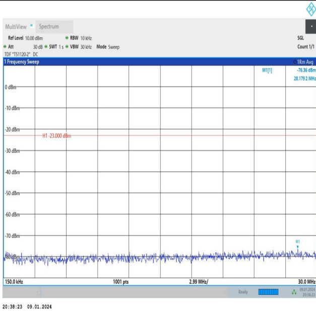
Band26_5MHz_16QAM_27015_1RB#24_0.15~30_0.15~30
