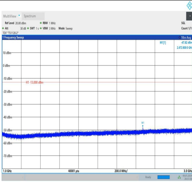
Band26_15MHz_QPSK_26865_1RB#0_1000~3000_1000~30 00
