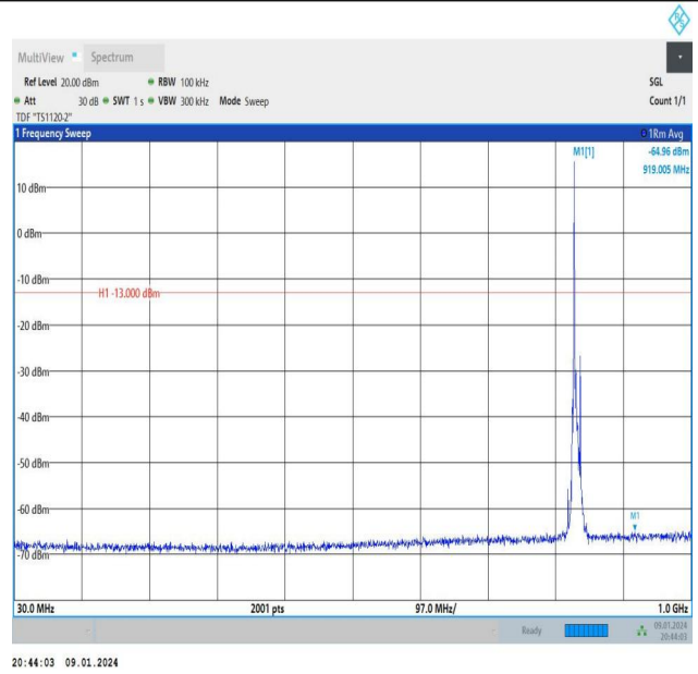
Band26_10MHz_16QAM_26915_1RB#0_30~1000_30~1000
