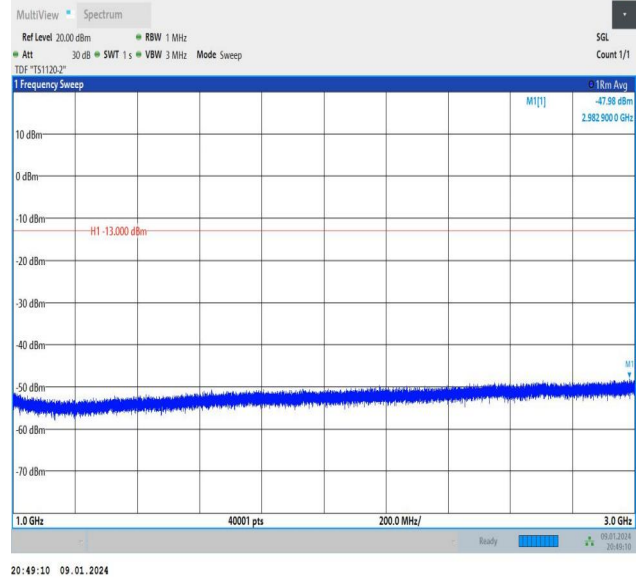
Band26_10MHz_QPSK_26840_50RB#0_1000~3000_1000~3000
