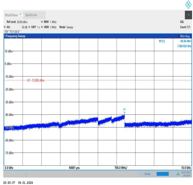
Band26_10MHz_QPSK_26915_50RB#0_3000~10000_3000~10000
