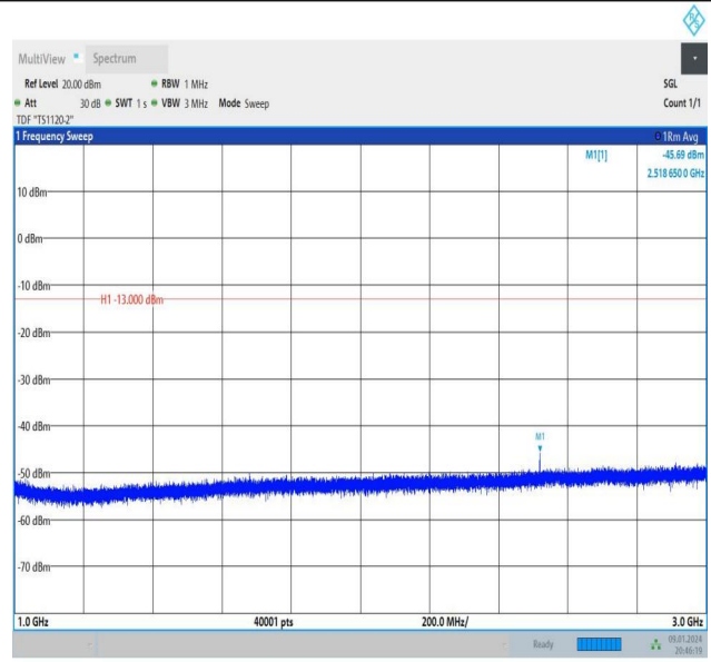
Band26_10MHz_QPSK_26990_1RB#0_1000~3000_1000~3000
