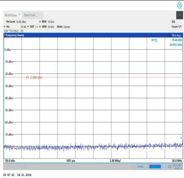
Band26_10MHz_QPSK_26990_1RB#49_0.15~30_0.15~30
