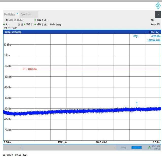
Band26_10MHz_QPSK_26990_1RB#49_1000~3000_1000~3000
