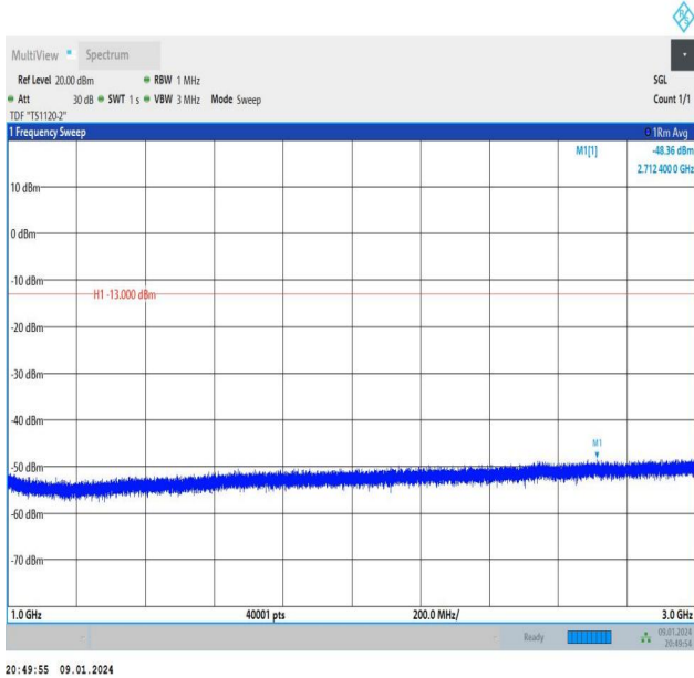
Band26_10MHz_QPSK_26915_50RB#0_1000~3000_1000~3000
