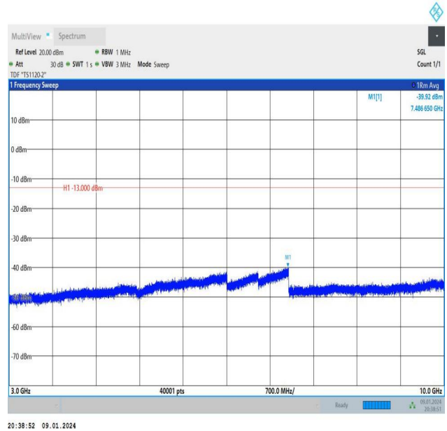
Band26_5MHz_16QAM_27015_1RB#24_3000~10000_3000~10000
