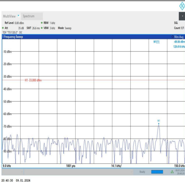
Band26_10MHz_QPSK_26840_1RB#0_0.009~0.15_0.009~0.15
