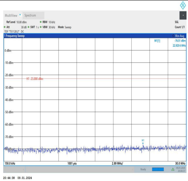
Band26_10MHz_QPSK_26915_1RB#49_0.15~30_0.15~30
