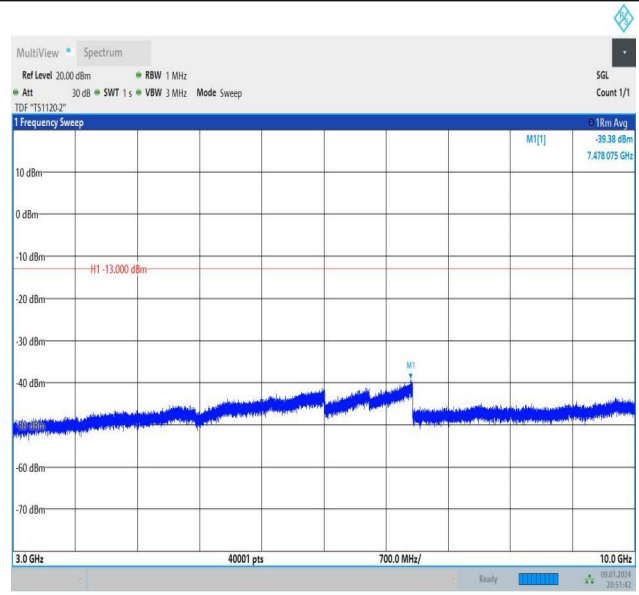
Band26_15MHz_QPSK_26865_1RB#0_3000~10000_3000~1 0000
