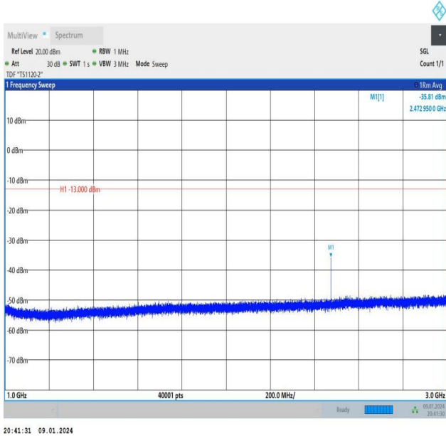
Band26_10MHz_16QAM_26840_1RB#0_1000~3000_1000~3000
