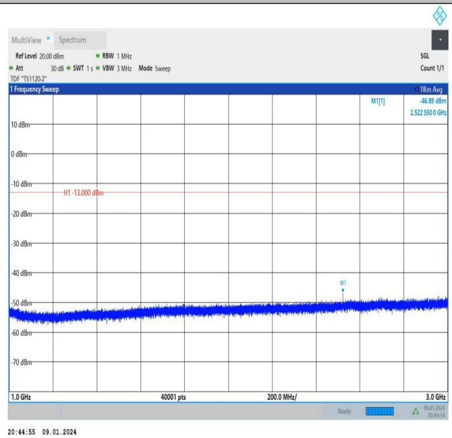
Band26_10MHz_QPSK_26915_1RB#49_1000~3000_1000~3000
