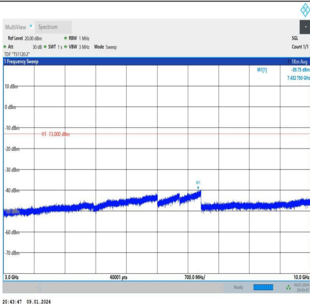
Band26_10MHz_QPSK_26915_1RB#0_3000~10000_3000~10000 0000
