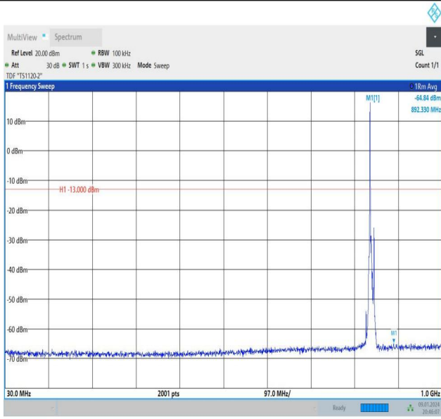
Band26_10MHz_QPSK_26990_1RB#0_30~1000_30~1000
