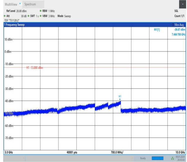
Band26_10MHz_16QAM_26840_1RB#49_3000~10000_3000~10000
