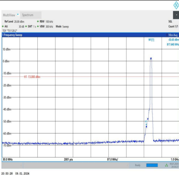
Band26_10MHz_QPSK_26990_50RB#0_30~1000_30~1000
