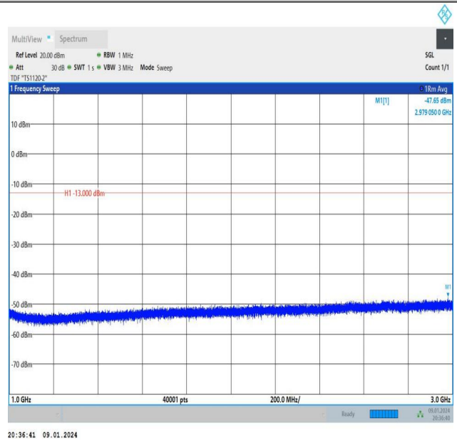
Band26_5MHz_QPSK_27015_1RB#0_1000~3000_1000~300
