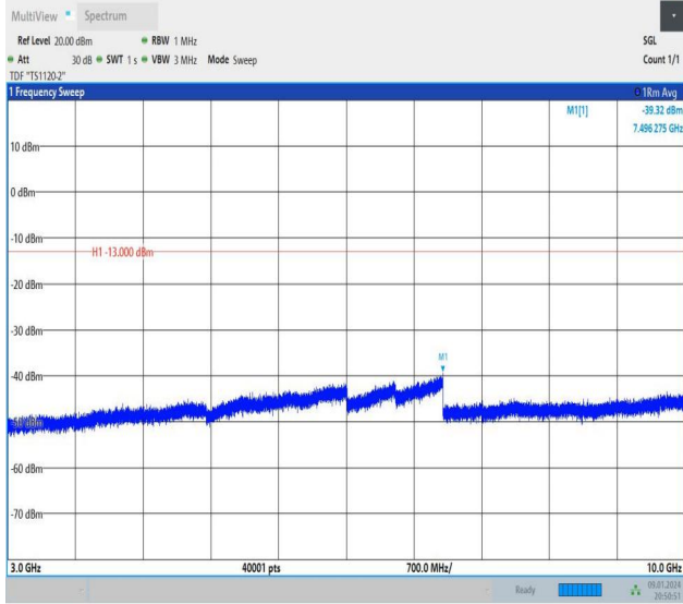
Band26_10MHz_QPSK_26990_50RB#0_3000~10000_3000~10000
