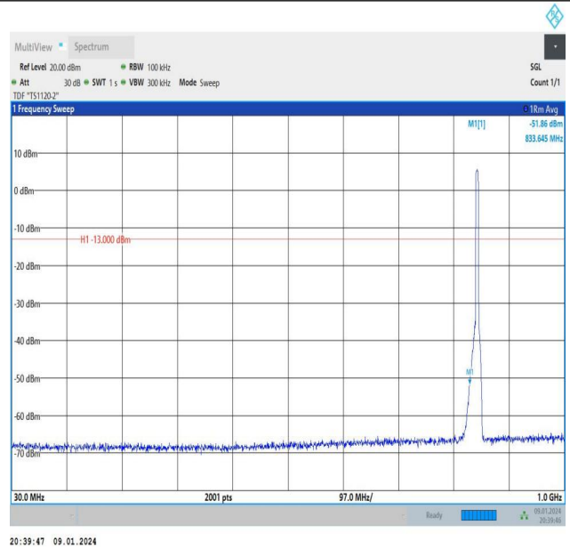
Band26_5MHz_16QAM_27015_25RB#0_30~1000_30~1000
