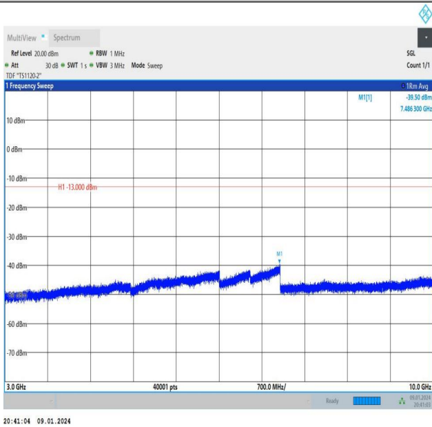
Band26_10MHz_QPSK_26840_1RB#0_3000~10000_3000~10000
