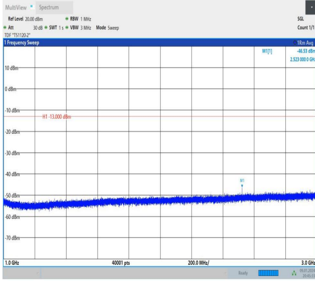
Band26_10MHz_16QAM_26915_1RB#49_1000~3000_1000~3000
