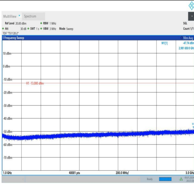
Band26_5MHz_16QAM_27015_1RB#0_1000~3000_1000~3000 00
