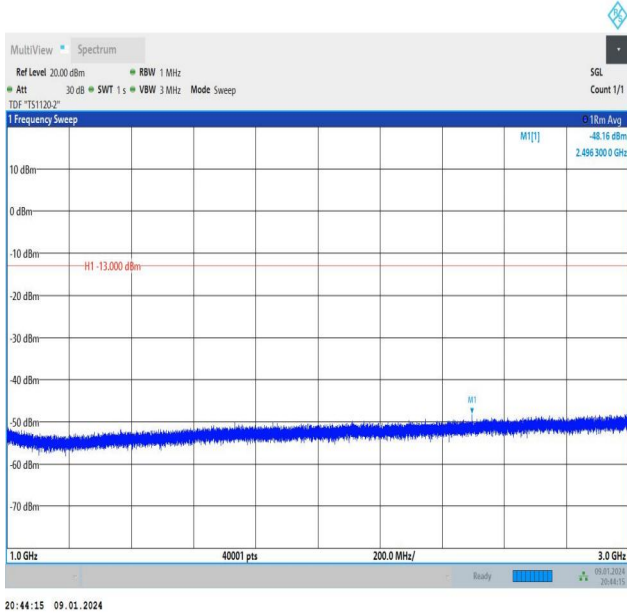
Band26_10MHz_16QAM_26915_1RB#0_1000~3000_1000~3000
