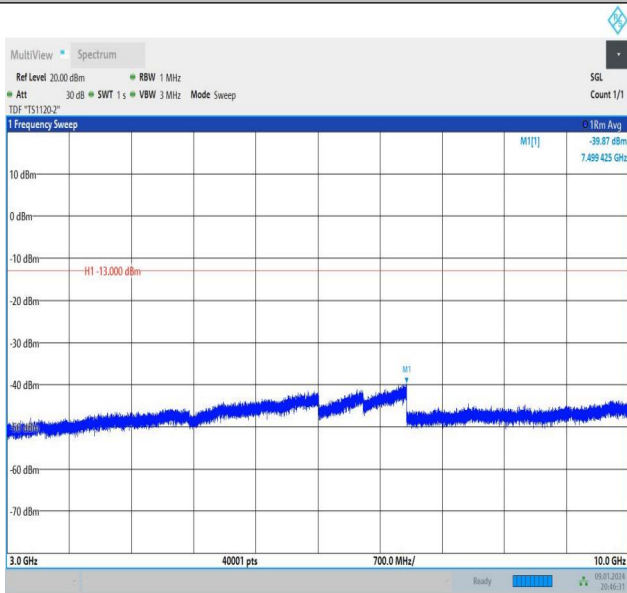
Band26_10MHz_QPSK_26990_1RB#0_3000~10000_3000~10000
