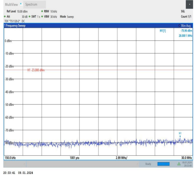
Band26_5MHz_QPSK_26915_1RB#24_0.15~30_0.15~30
