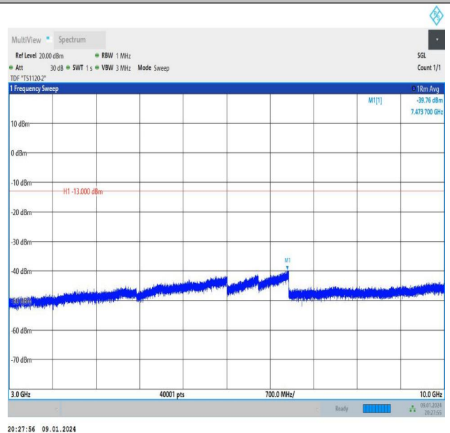
Band26_3MHz_16QAM_27025_15RB#0_3000~10000_3000~10000
