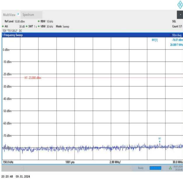
Band26_3MHz_16QAM_26915_1RB#0_0.15~30_0.15~30
