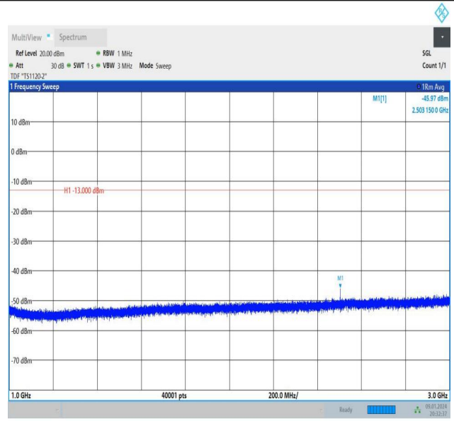
Band26_5MHz_QPSK_26915_1RB#0_1000~3000_1000~300
