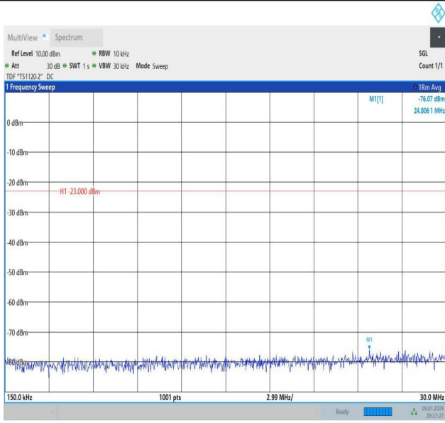
Band26_3MHz_16QAM_27025_15RB#0_0.15~30_0.15~30
