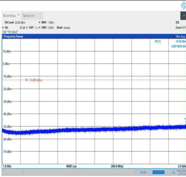
Band26_1.4MHz_16QAM_27033_6RB#0_1000~3000_1000~3000
