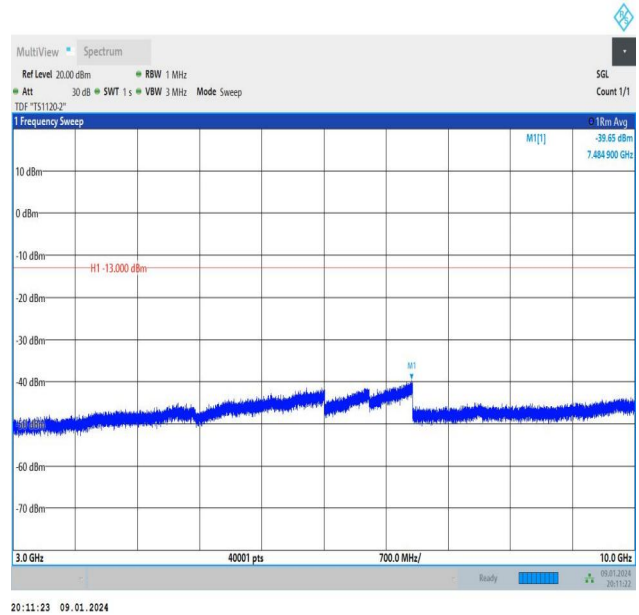
Band26_1.4MHz_16QAM_26915_6RB#0_3000~10000_3000~10000
