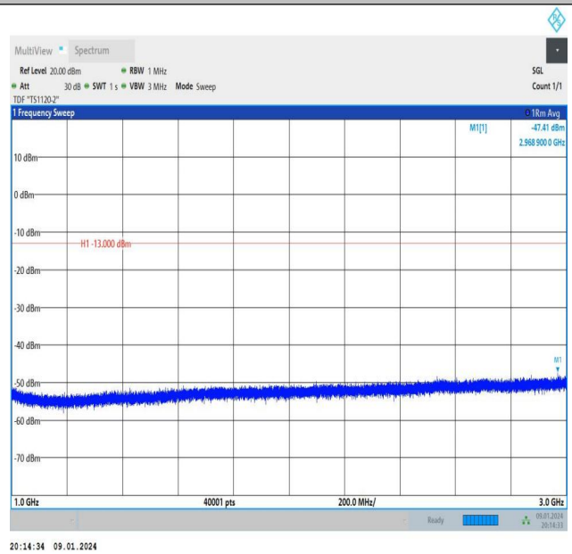
Band26_1.4MHz_QPSK_27033_6RB#0_1000~3000_1000~30
