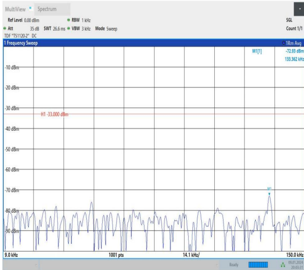
Band26_1.4MHz_QPSK_26797_1RB#0_0.009~0.15_0.009~0.15
