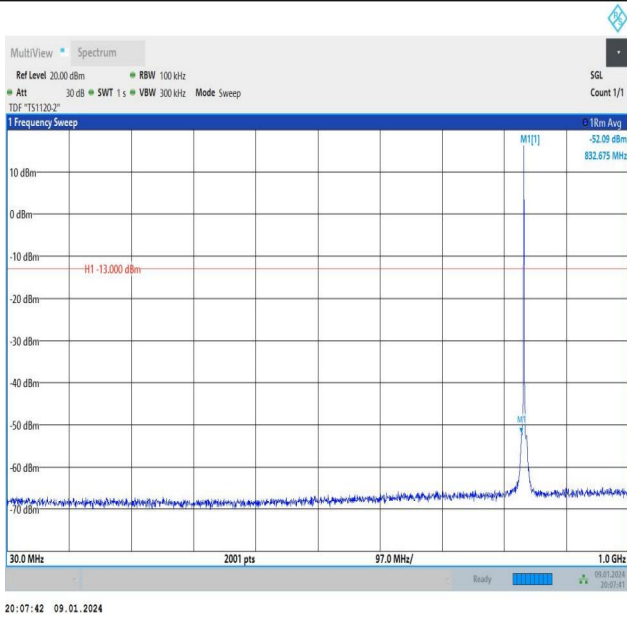
Band26_1.4MHz_QPSK_26915_1RB#0_30~1000_30~1000
