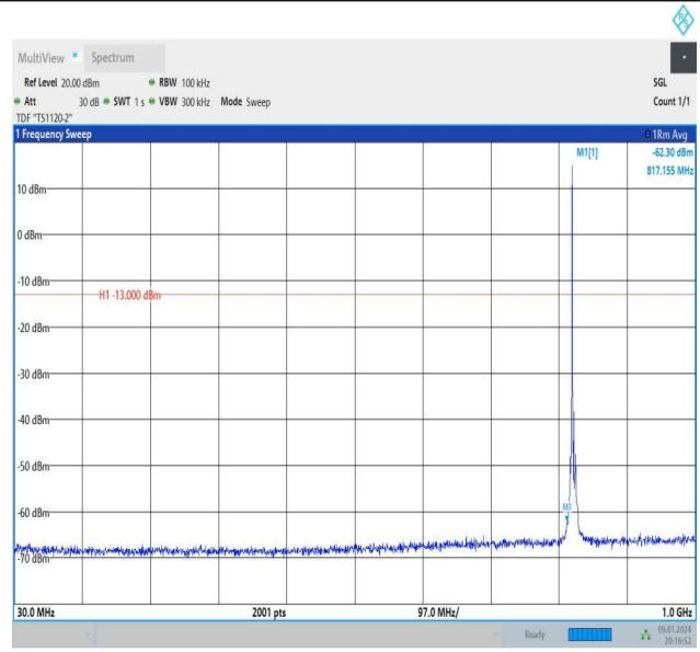
Band26_3MHz_16QAM_26805_1RB#0_30~1000_30~1000
