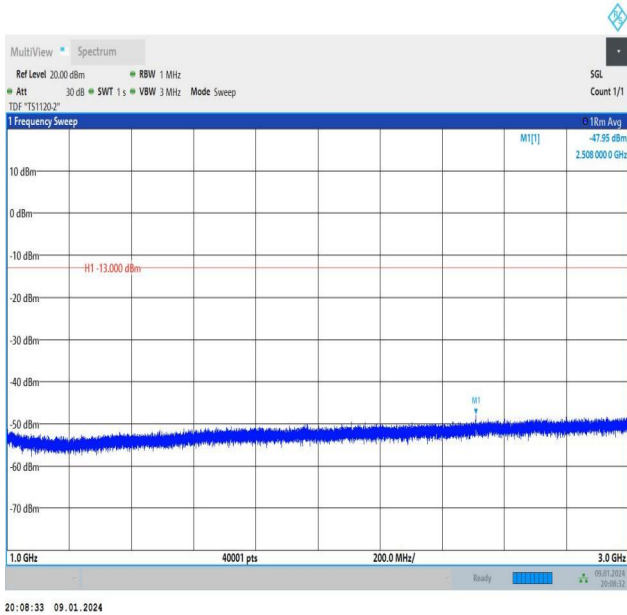
Band26_1.4MHz_16QAM_26915_1RB#0_1000~3000_1000~3000
