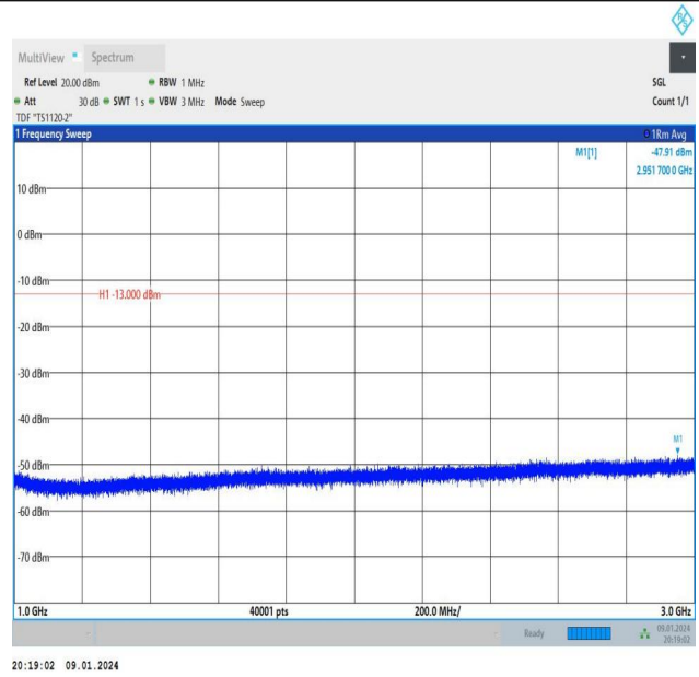
Band26_3MHz_QPSK_26805_15RB#0_1000~3000_1000~3000
