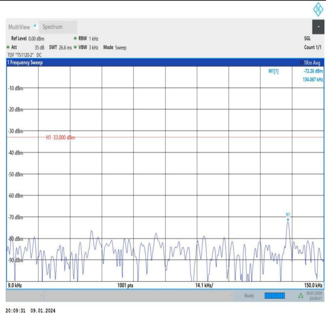
Band26_1.4MHz_16QAM_26915_1RB#5_0.009~0.15_0.009~0.15
