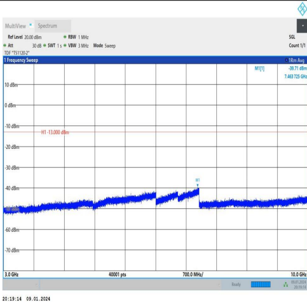
Band26_3MHz_QPSK_26805_15RB#0_3000~10000_3000~10000
