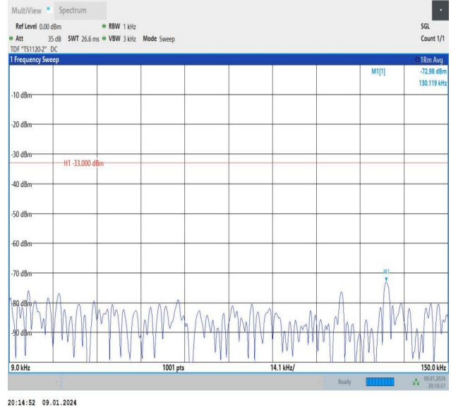
Band26_1.4MHz_16QAM_27033_6RB#0_0.009~0.15_0.009~0.15
