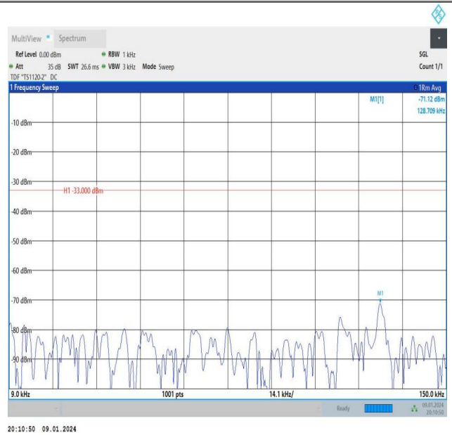
Band26_1.4MHz_16QAM_26915_6RB#0_0.009~0.15_0.009~0.15
