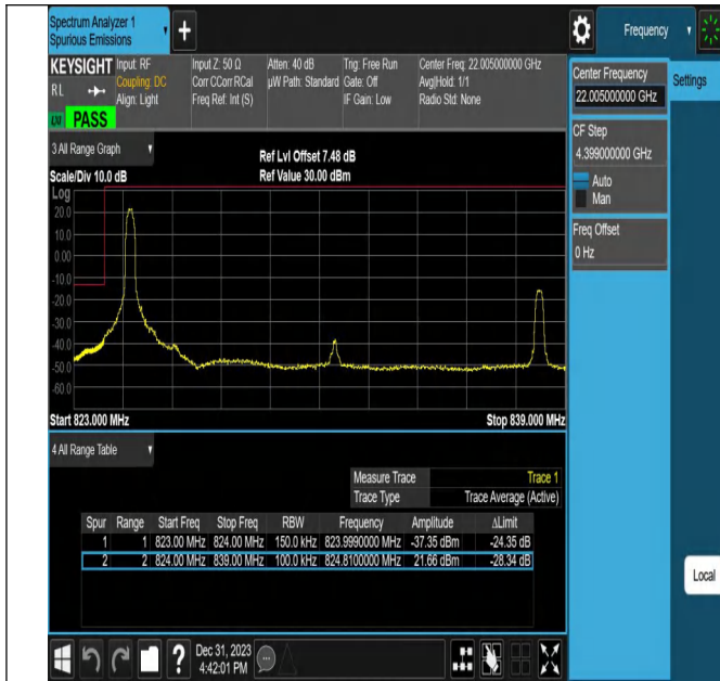
Band26_15MHz_16QAM_26865_1RB#0
