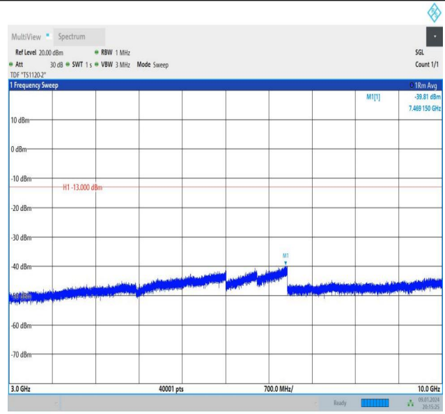
Band26_1.4MHz_16QAM_27033_6RB#0_3000~10000_3000~10000
