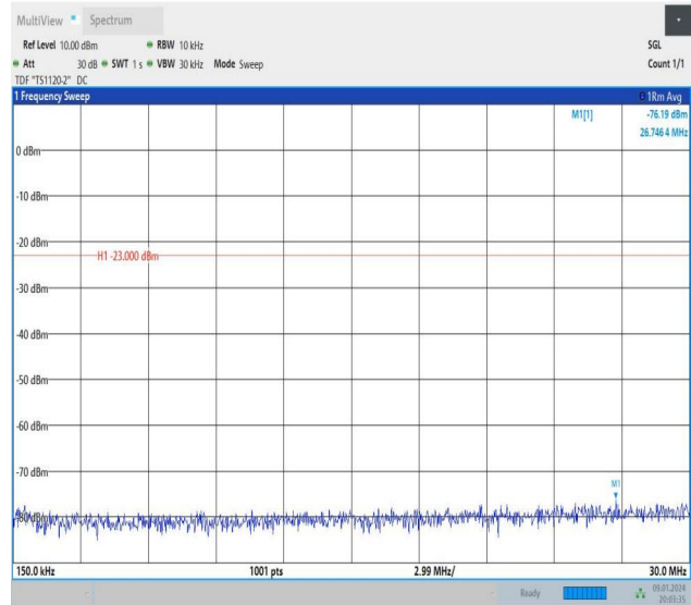
Band26_1.4MHz_QPSK_26797_1RB#0_0.15~30_0.15~30
