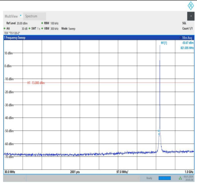
Band26_1.4MHz_16QAM_26797_1RB#5_30~1000_30~1000
