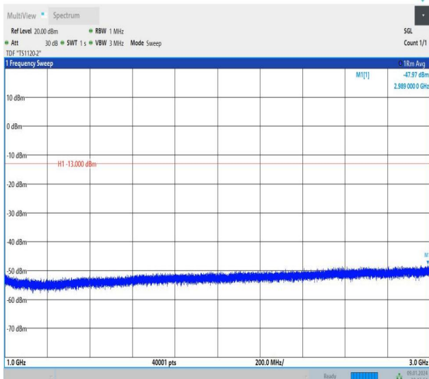
Band26_1.4MHz_16QAM_27033_1RB#5_1000~3000_1000~3000
