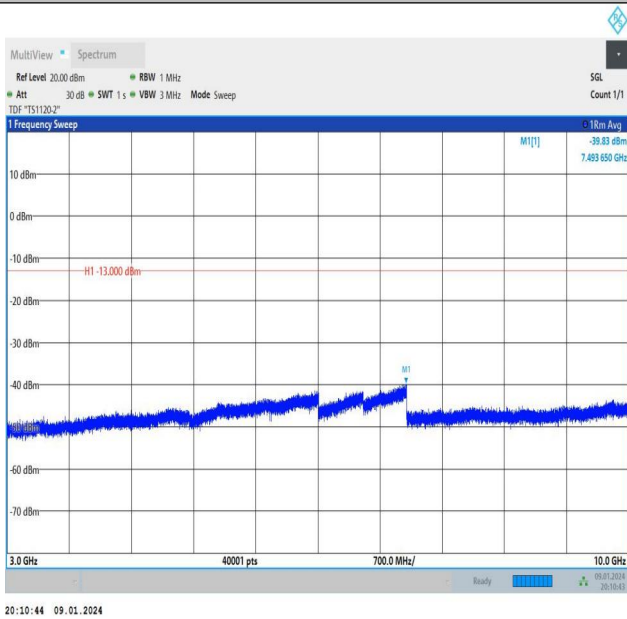
Band26_1.4MHz_QPSK_26915_6RB#0_3000~10000_3000~10000 0000
