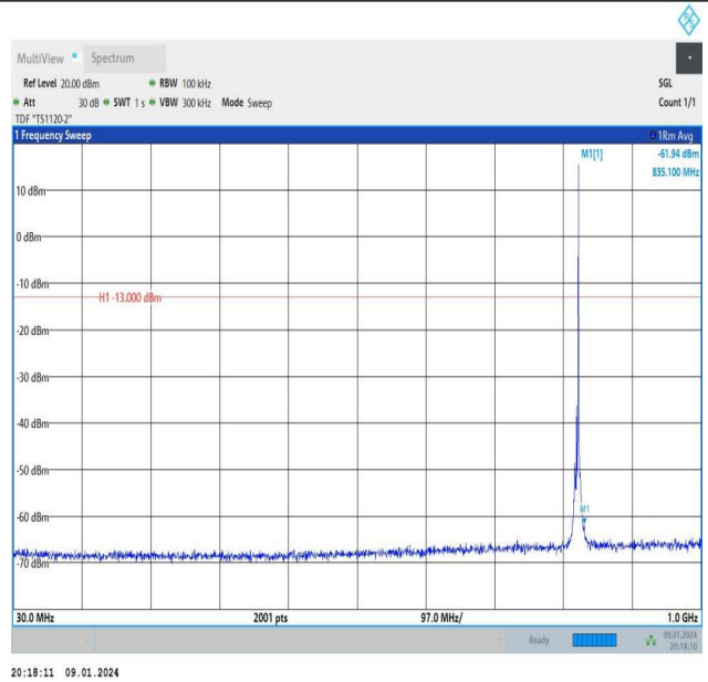
Band26_3MHz_16QAM_26805_1RB#14_30~1000_30~1000
