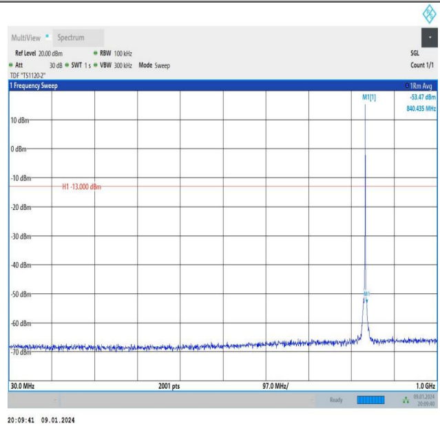
Band26_1.4MHz_16QAM_26915_1RB#5_30~1000_30~1000
