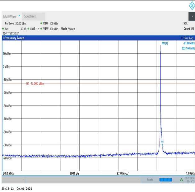
Band26_3MHz_QPSK_26805_1RB#0_30~1000_30~1000
