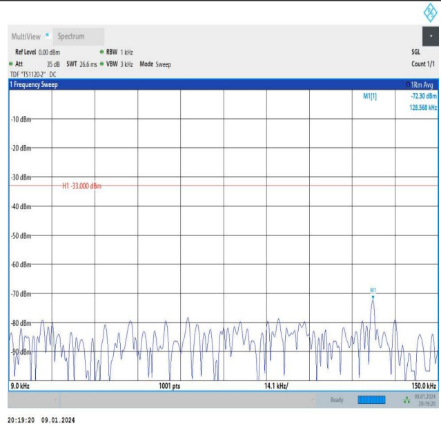
Band26_3MHz_16QAM_26805_15RB#0_0.009~0.15_0.009~0.15
