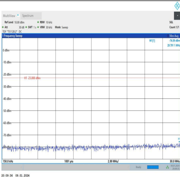
Band26_1.4MHz_16QAM_26915_1RB#5_0.15~30_0.15~30
