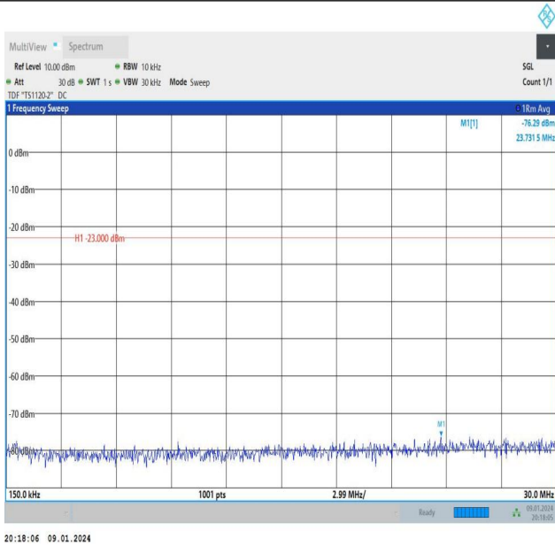
Band26_3MHz_16QAM_26805_1RB#14_0.15~30_0.15~30
