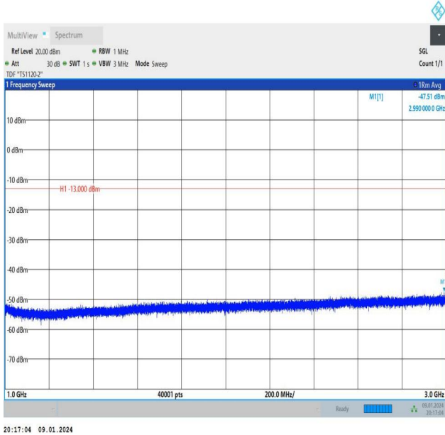
Band26_3MHz_16QAM_26805_1RB#0_1000~3000_1000~3000
