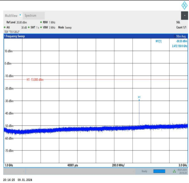
Band26_3MHz_QPSK_26805_1RB#0_1000~3000_1000~300
