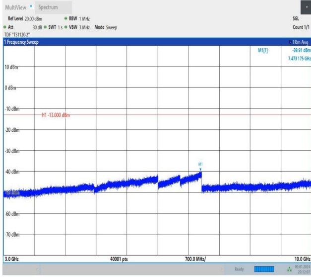
Band26_1.4MHz_QPSK_27033_1RB#0_3000~10000_3000~10000
