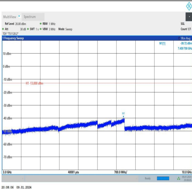
Band26_1.4MHz_QPSK_26915_1RB#0_3000~10000_3000~10000 0000
