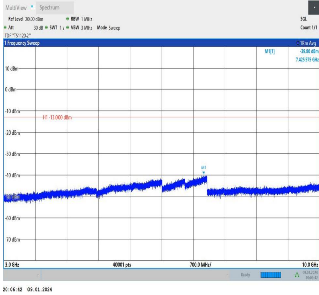
Band26_1.4MHz_QPSK_26797_6RB#0_3000~10000_3000~10000
