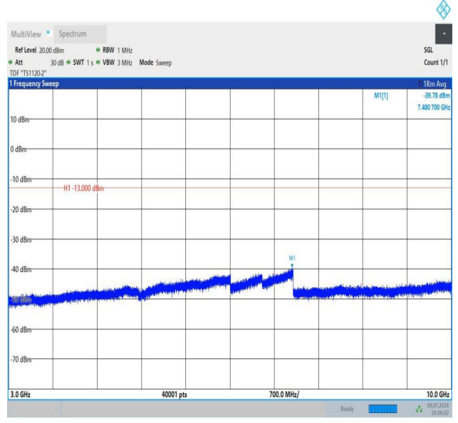
Band26_1.4MHz_16QAM_26797_1RB#5_3000~10000_3000~10000
