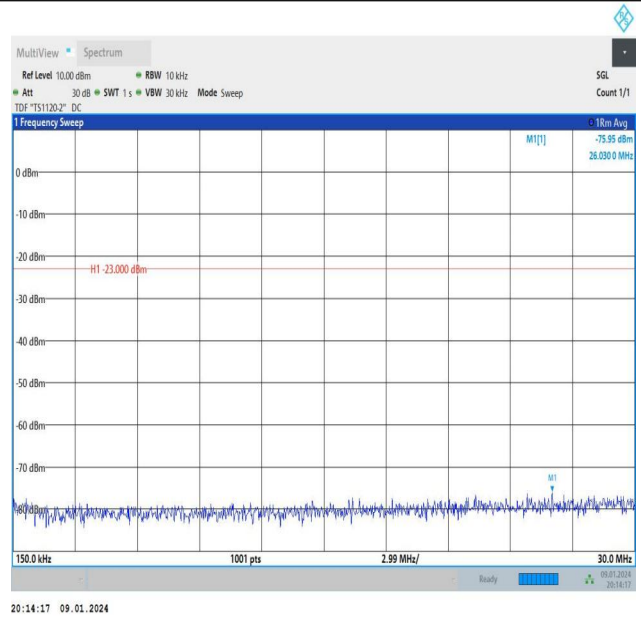
Band26_1.4MHz_QPSK_27033_6RB#0_0.15~30_0.15~30
