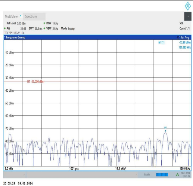
Band26_1.4MHz_16QAM_26797_1RB#5_0.009~0.15_0.009~0.15
