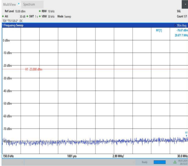
Band26_1.4MHz_16QAM_27033_1RB#5_0.15~30_0.15~30
