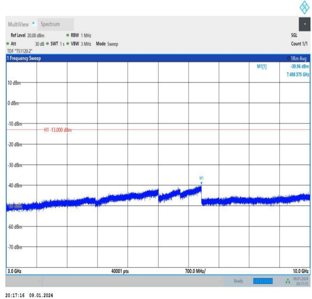
Band26_3MHz_16QAM_26805_1RB#0_3000~10000_3000~10000
