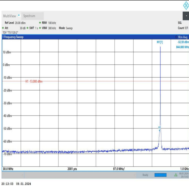
Band26_1.4MHz_QPSK_27033_1RB#5_30~1000_30~1000
