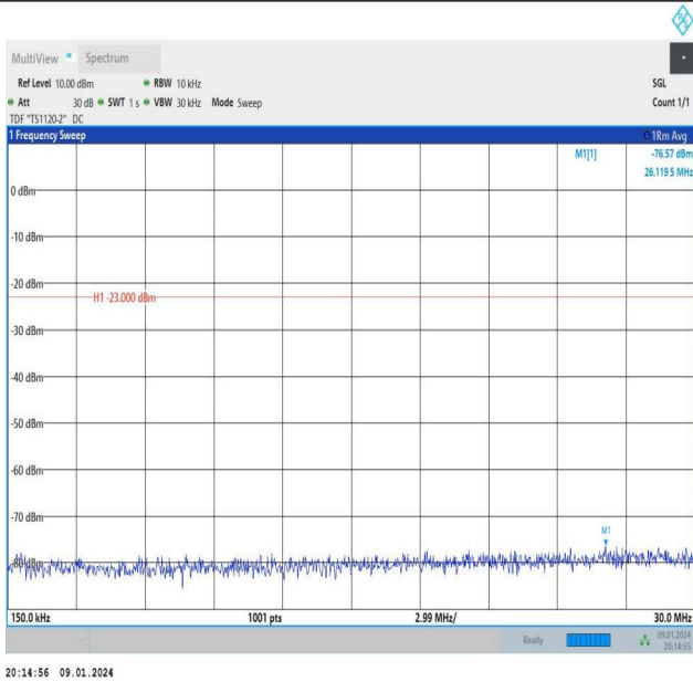
Band26_1.4MHz_16QAM_27033_6RB#0_0.15~30_0.15~30
