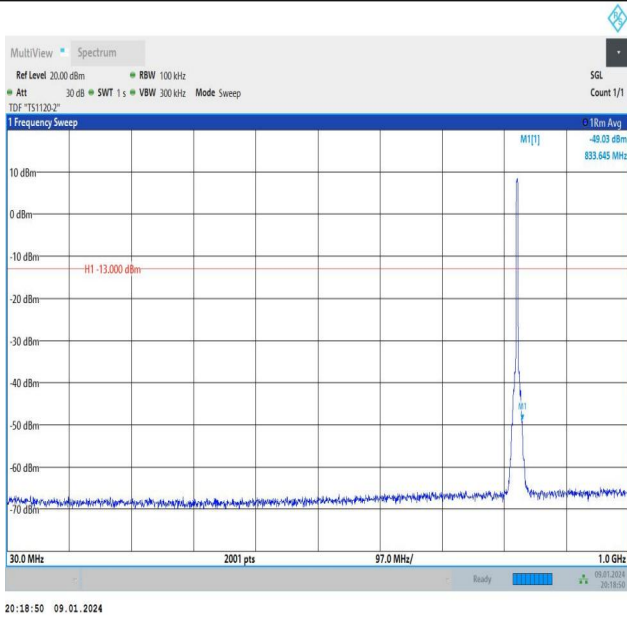
Band26_3MHz_QPSK_26805_15RB#0_30~1000_30~1000
