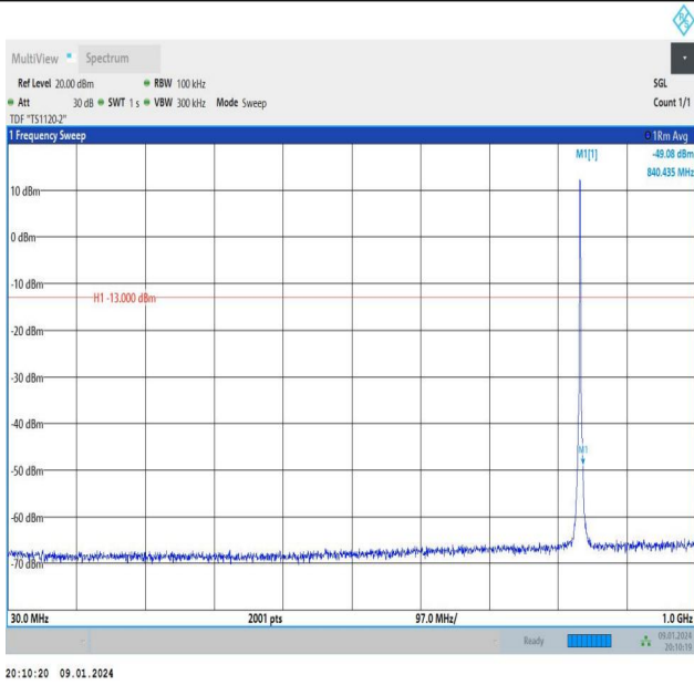
Band26_1.4MHz_QPSK_26915_6RB#0_30~1000_30~1000
