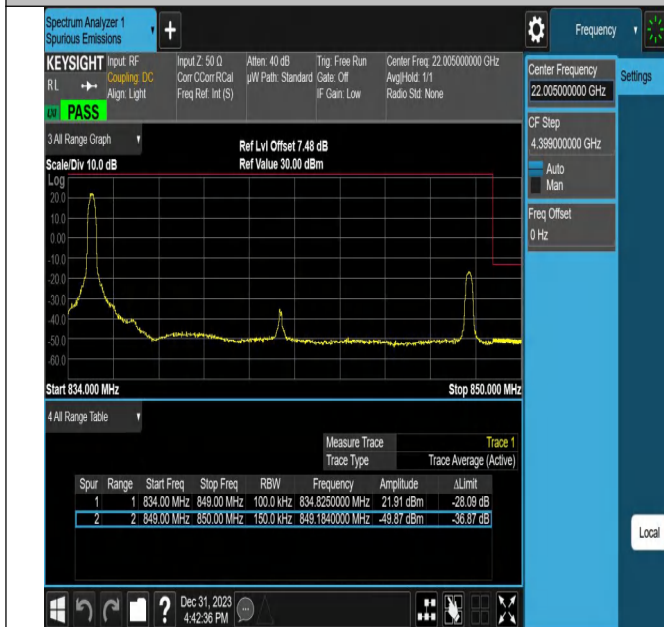
Band26_15MHz_16QAM_26965_1RB#0
