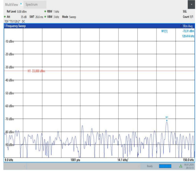
Band26_1.4MHz_16QAM_27033_1RB#0_0.009~0.15_0.009~0.15
