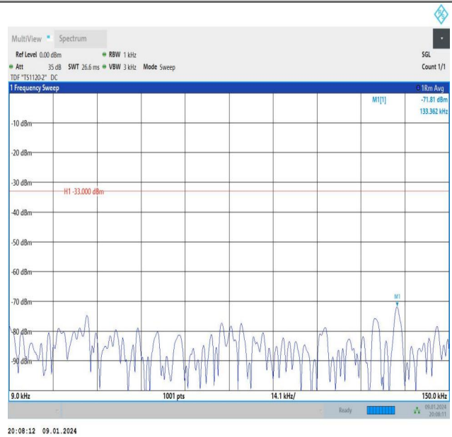
Band26_1.4MHz_16QAM_26915_1RB#0_0.009~0.15_0.009~0.15
