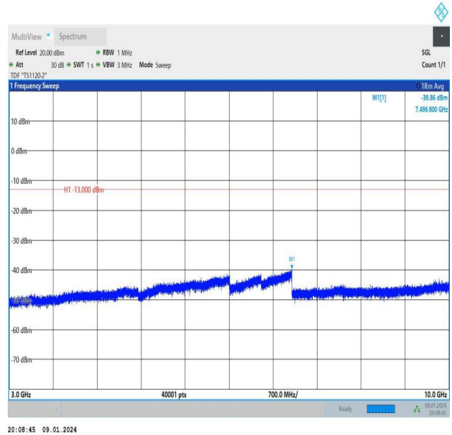
Band26_1.4MHz_16QAM_26915_1RB#0_3000~10000_3000~10000
