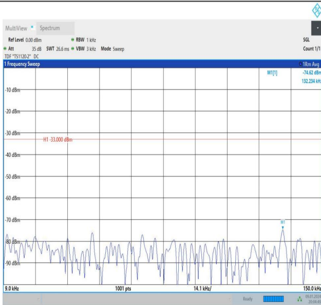
Band26_1.4MHz_16QAM_26797_1RB#0_1000~3000_1000~3000
