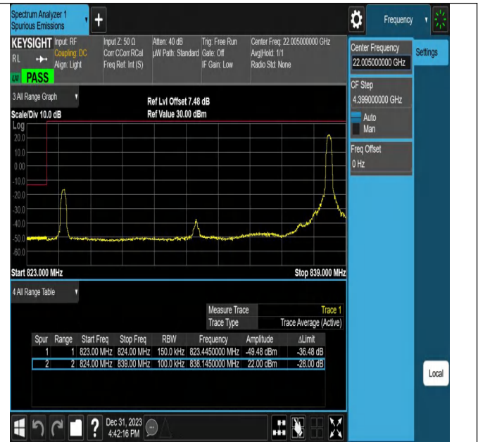
Band26_15MHz_16QAM_26865_1RB#74
