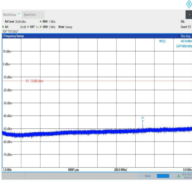
Band26_1.4MHz_16QAM_26797_1RB#5_1000~3000_1000~3000
