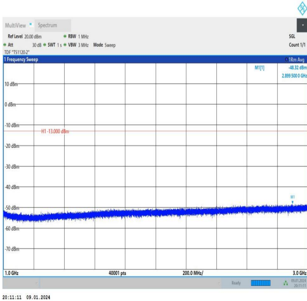
Band26_1.4MHz_16QAM_26915_6RB#0_1000~3000_1000~3000
