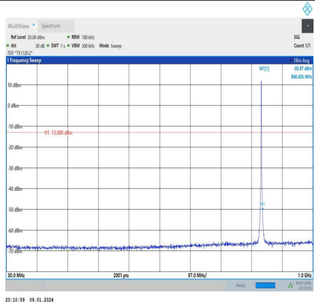
Band26_1.4MHz_16QAM_26915_6RB#0_30~1000_30~1000
