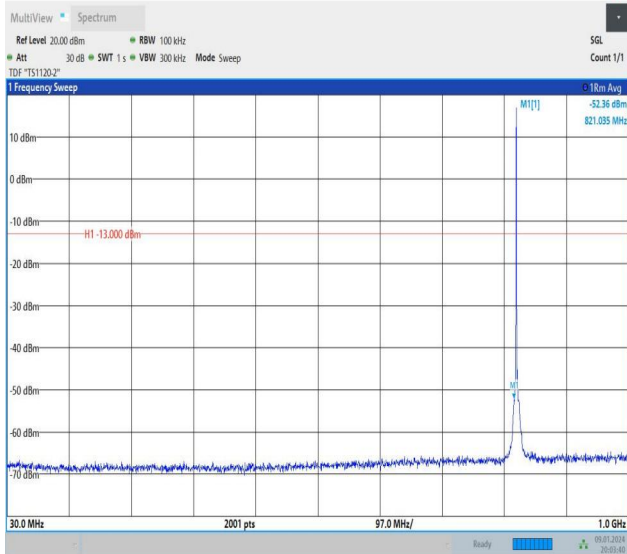
Band26_1.4MHz_QPSK_26797_1RB#0_30~1000_30~1000
