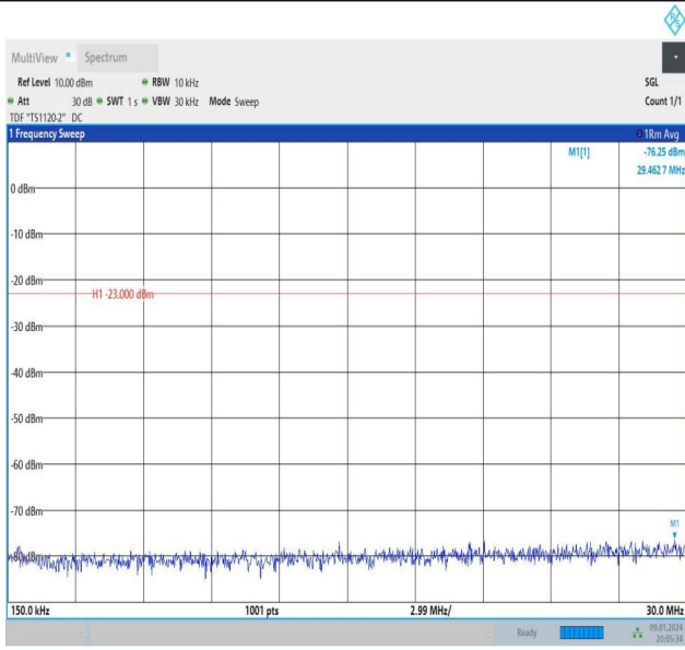
Band26_1.4MHz_16QAM_26797_1RB#5_0.15~30_0.15~30
