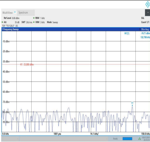
Band26_1.4MHz_16QAM_26915_1RB#5_1000~3000_1000~3000
