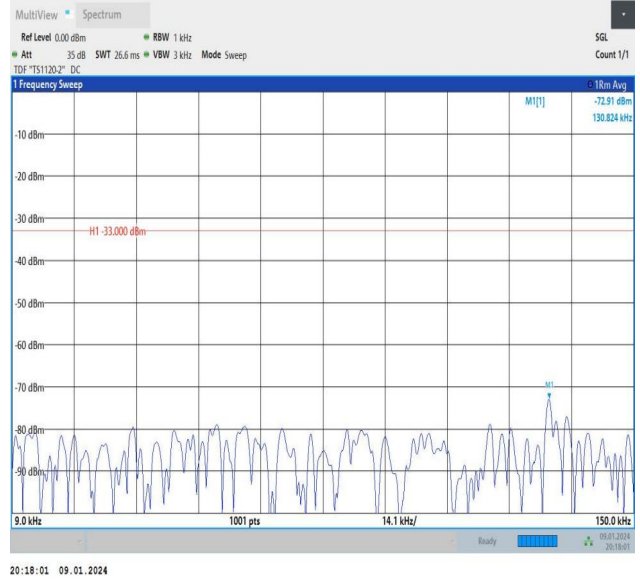
Band26_3MHz_16QAM_26805_1RB#14_0.009~0.15_0.009~0.15
