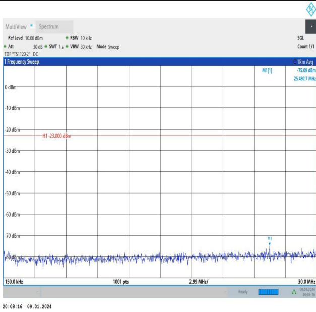
Band26_1.4MHz_16QAM_26915_1RB#0_0.15~30_0.15~30
