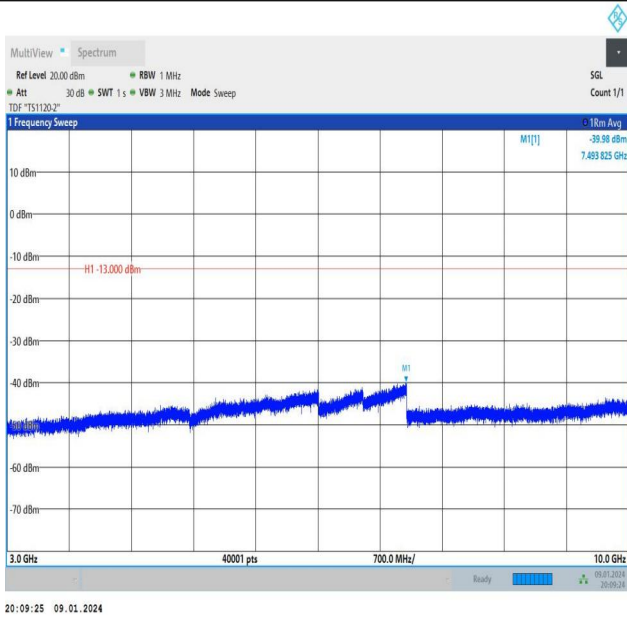
Band26_1.4MHz_QPSK_26915_1RB#5_3000~10000_3000~10000
