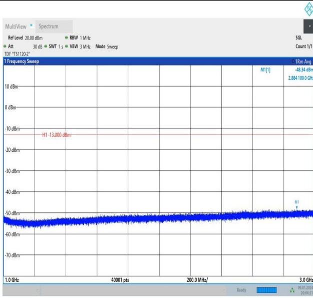
Band26_1.4MHz_16QAM_26797_1RB#0_1000~3000_1000~3000
