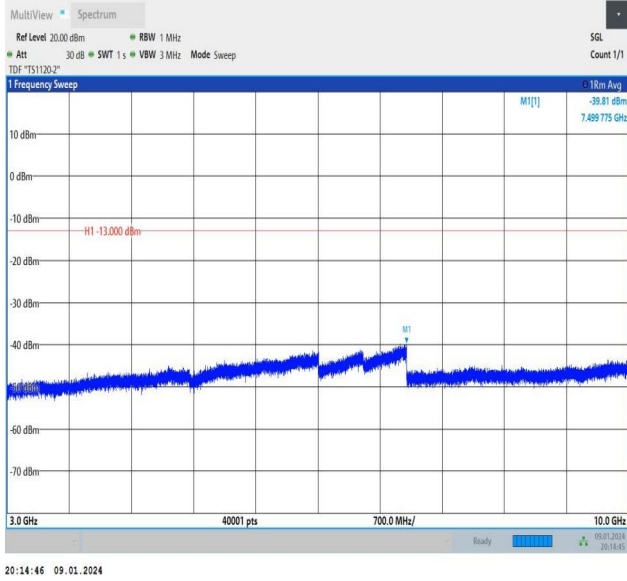
Band26_1.4MHz_QPSK_27033_6RB#0_3000~10000_3000~10000
