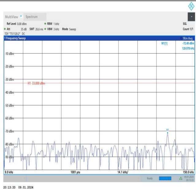
Band26_1.4MHz_16QAM_27033_1RB#5_0.009~0.15_0.009~0.15
