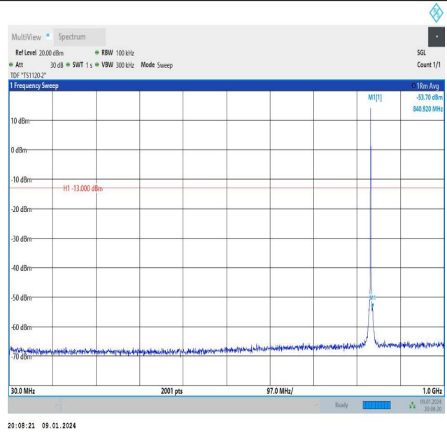
Band26_1.4MHz_16QAM_26915_1RB#0_30~1000_30~1000
