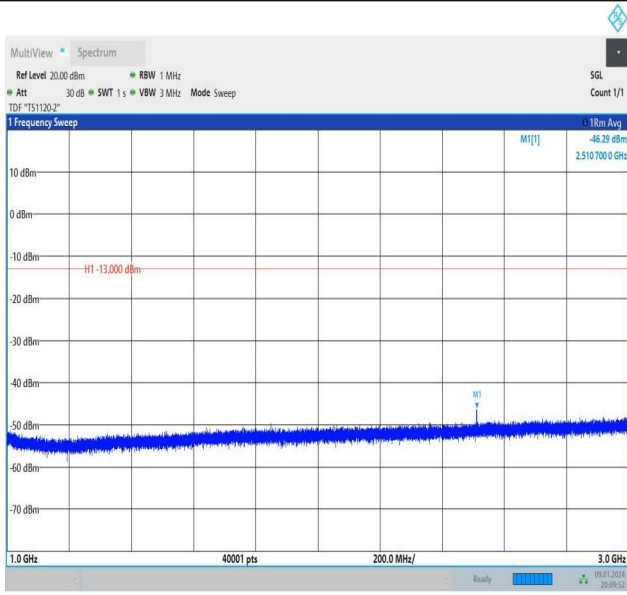
Band26_1.4MHz_16QAM_26915_1RB#5_1000~3000_1000~3000
