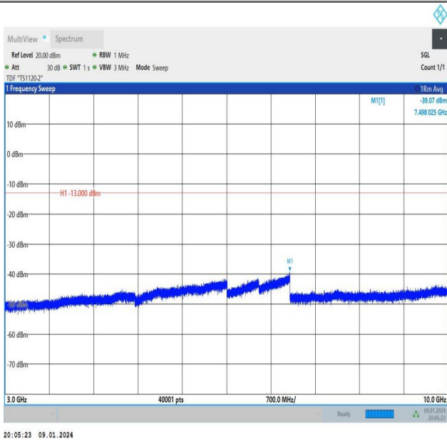
Band26_1.4MHz_QPSK_26797_1RB#5_3000~10000_3000~10000 0000
