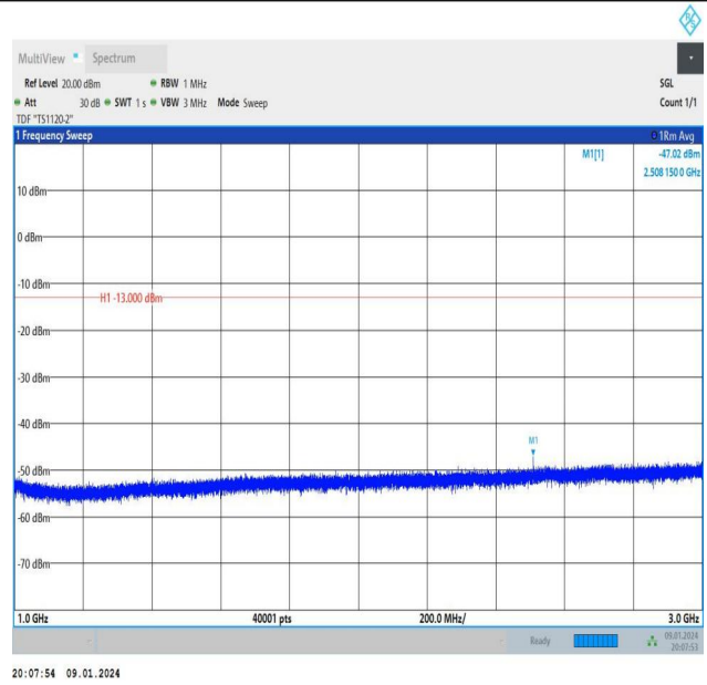
Band26_1.4MHz_QPSK_26915_1RB#0_1000~3000_1000~3000 00
