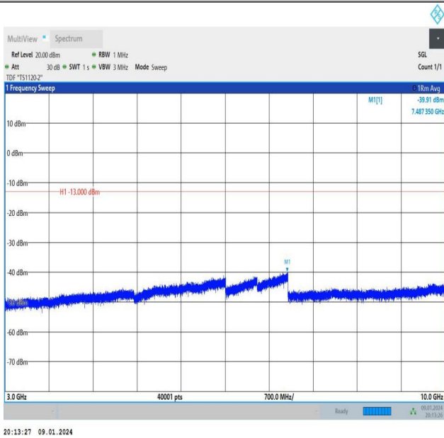
Band26_1.4MHz_QPSK_27033_1RB#5_3000~10000_3000~10000
