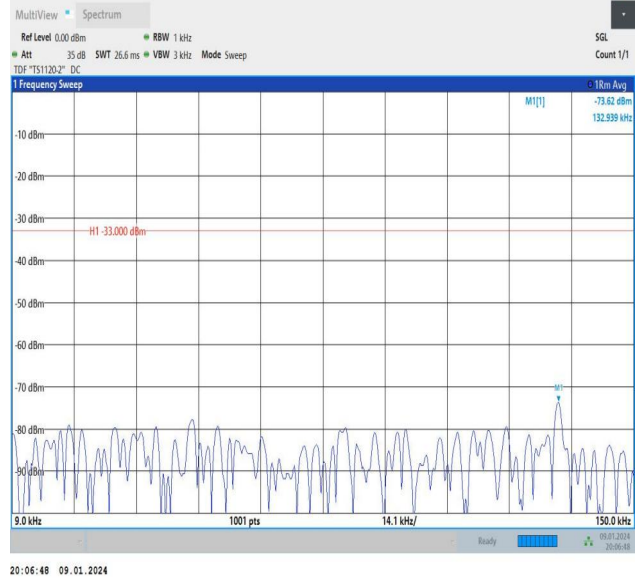
Band26_1.4MHz_16QAM_26797_6RB#0_0.009~0.15_0.009~0.15
