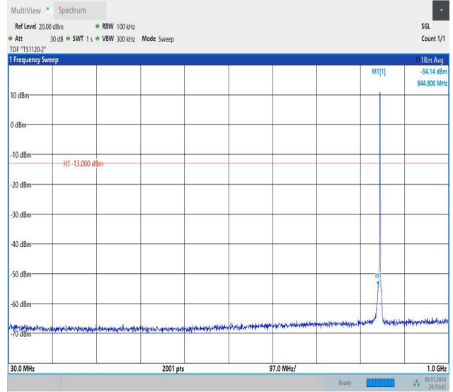
Band26_1.4MHz_16QAM_27033_1RB#5_30~1000_30~1000
