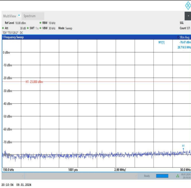
Band26_1.4MHz_16QAM_26915_6RB#0_0.15~30_0.15~30
