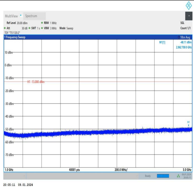
Band26_1.4MHz_QPSK_26797_1RB#5_1000~3000_1000~3000 00
