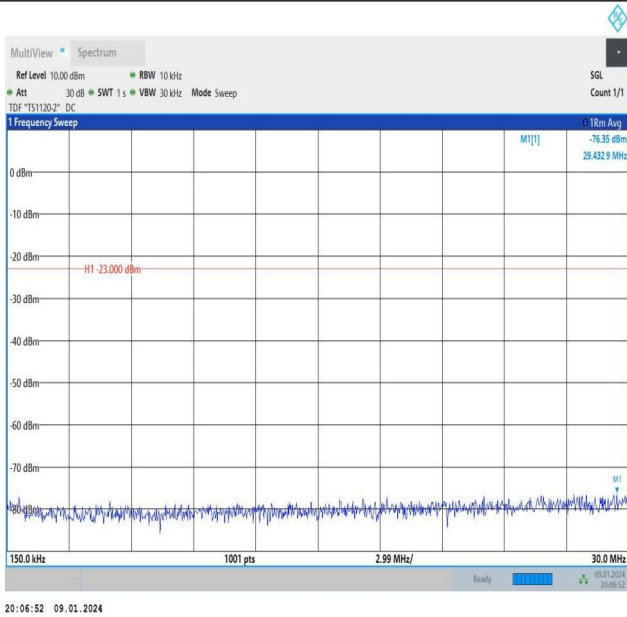
Band26_1.4MHz_16QAM_26797_6RB#0_0.15~30_0.15~30
