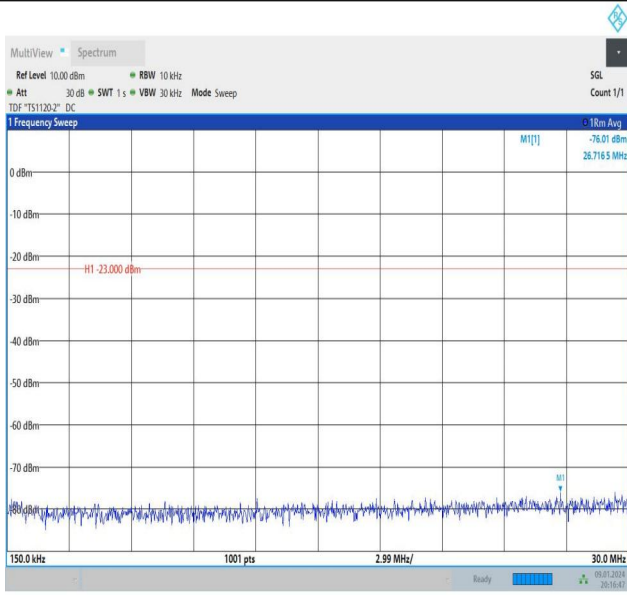
Band26_3MHz_16QAM_26805_1RB#0_0.15~30_0.15~30
