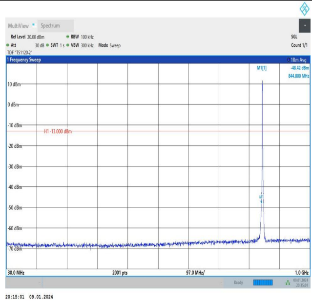
Band26_1.4MHz_16QAM_27033_6RB#0_30~1000_30~1000
