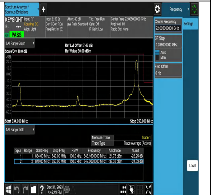
Band26_15MHz_16QAM_26965_1RB#74
