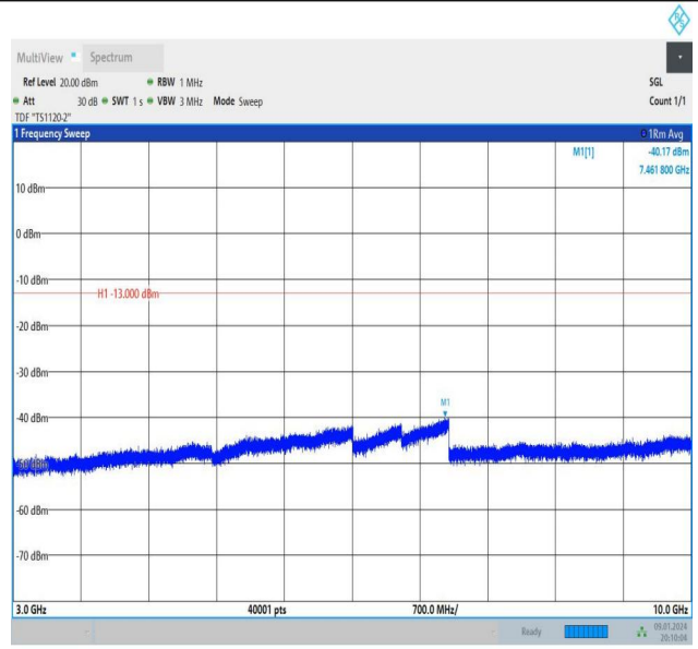
Band26_1.4MHz_16QAM_26915_1RB#5_3000~10000_3000~10000
