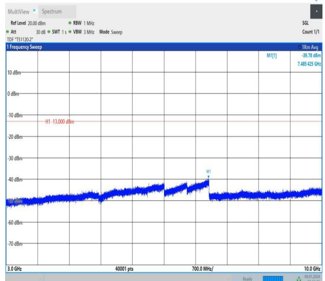
Band26_1.4MHz_16QAM_27033_1RB#5_3000~10000_3000~10000
