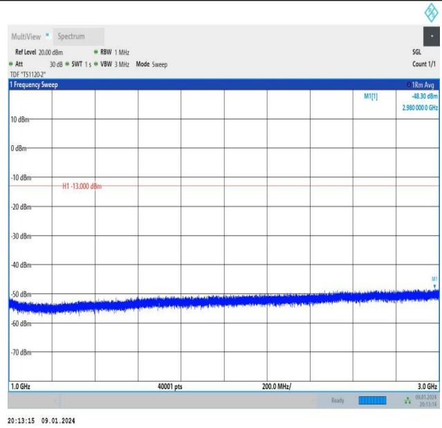
Band26_1.4MHz_QPSK_27033_1RB#5_1000~3000_1000~3000
