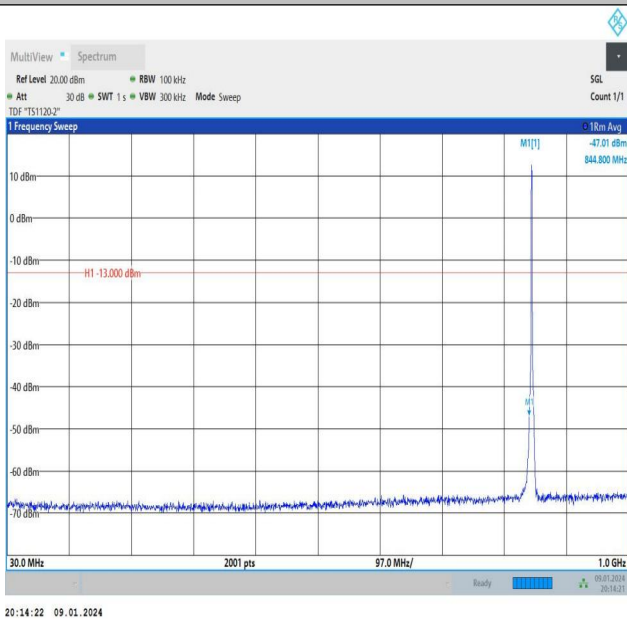
Band26_1.4MHz_QPSK_27033_6RB#0_30~1000_30~1000
