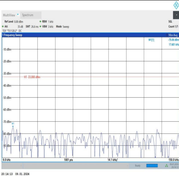
Band26_1.4MHz_QPSK_27033_6RB#0_0.009~0.15_0.009~0.
