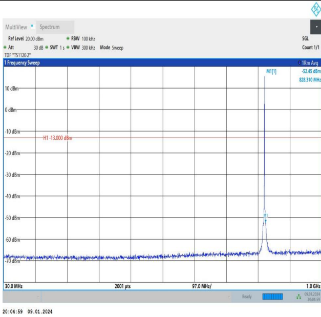
Band26_1.4MHz_QPSK_26797_1RB#5_30~1000_30~1000
