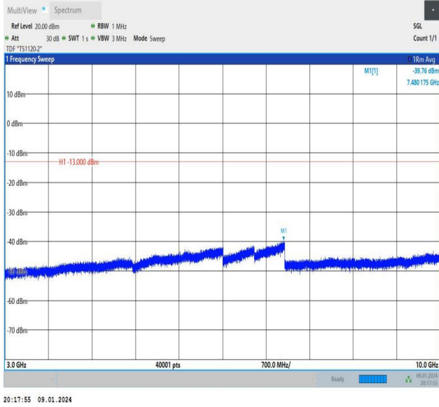
Band26_3MHz_QPSK_26805_1RB#14_3000~10000_3000~10000
