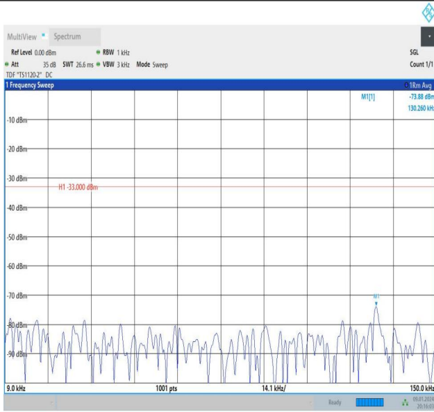
Band26_1.4MHz_16QAM_27033_6RB#0_1000~3000_1000~3000
