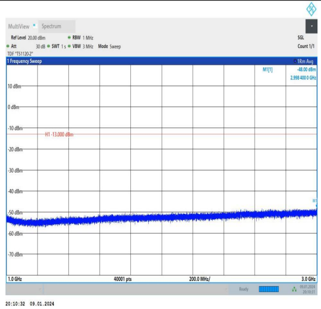
Band26_1.4MHz_QPSK_26915_6RB#0_1000~3000_1000~3000 00
