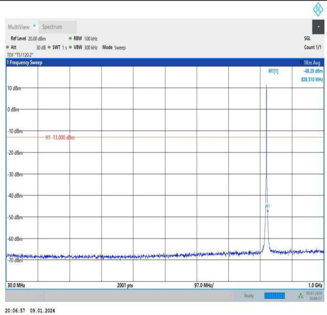
Band26_1.4MHz_16QAM_26797_6RB#0_30~1000_30~1000
